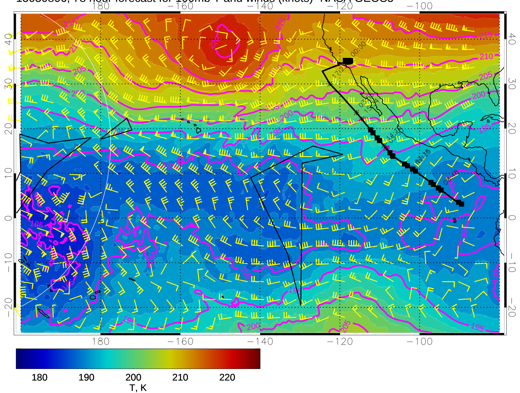
15030806, 78 hour forecast for 100mb T and winds (knots)- NASA GEOS5
