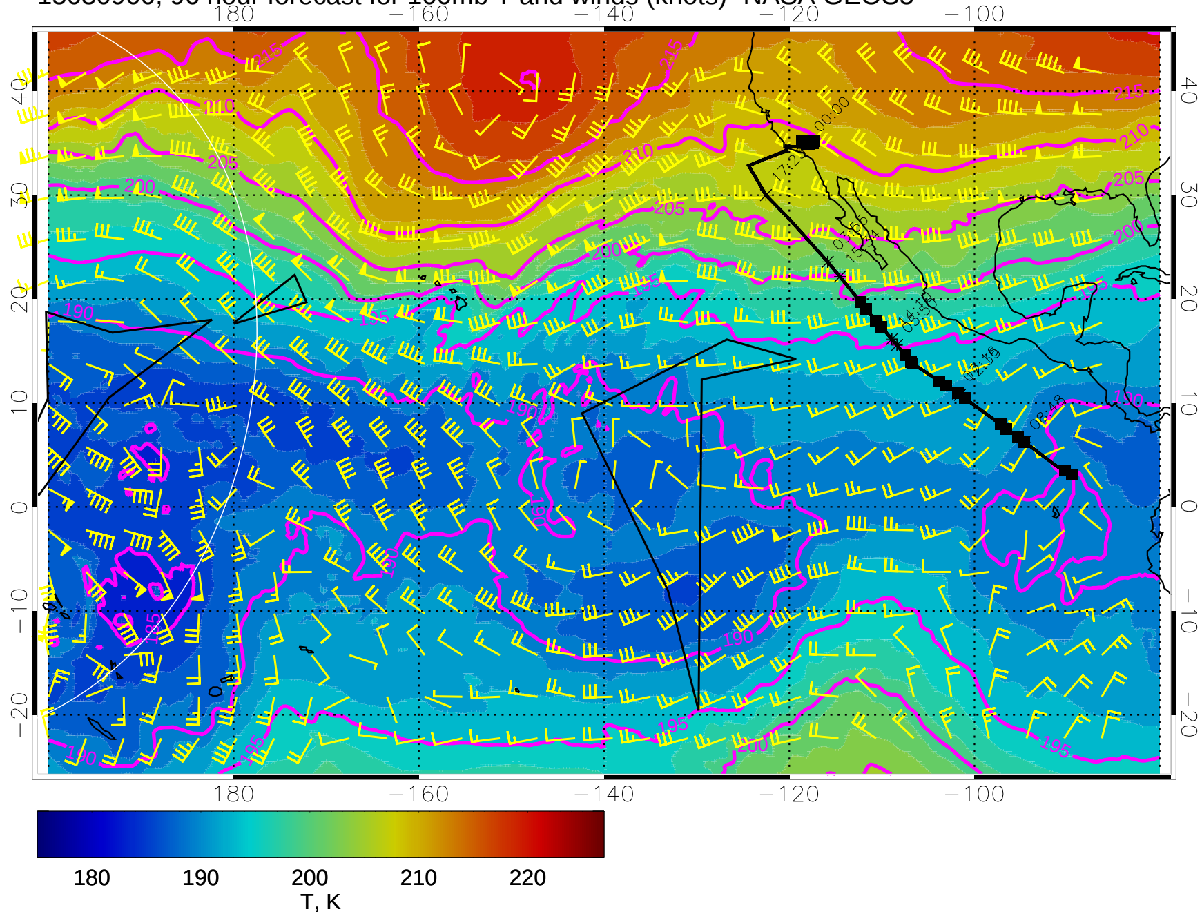
15030900, 96 hour forecast for 100mb T and winds (knots)- NASA GEOS5
