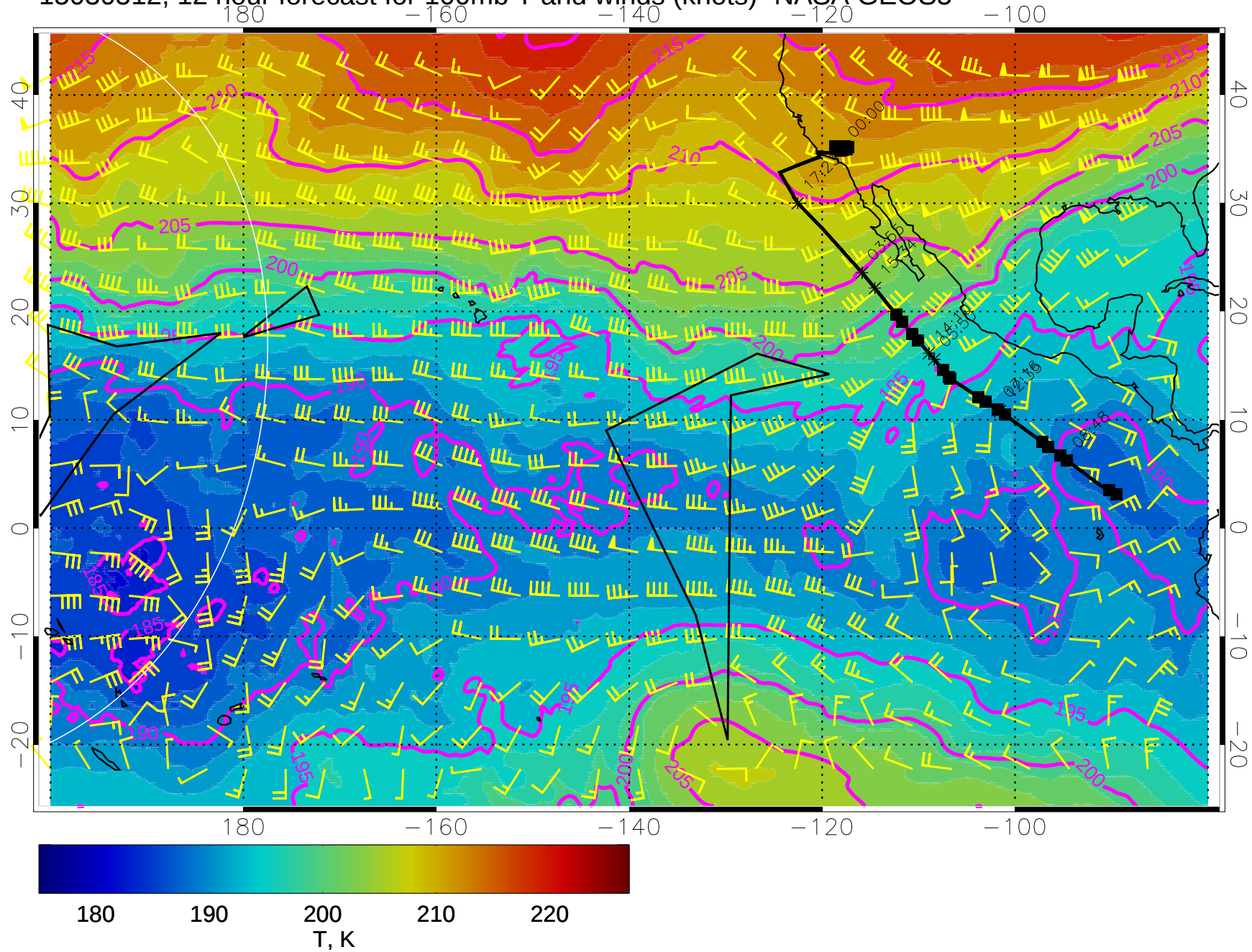
15030512, 12 hour forecast for 100mb T and winds (knots)- NASA GEOS5
