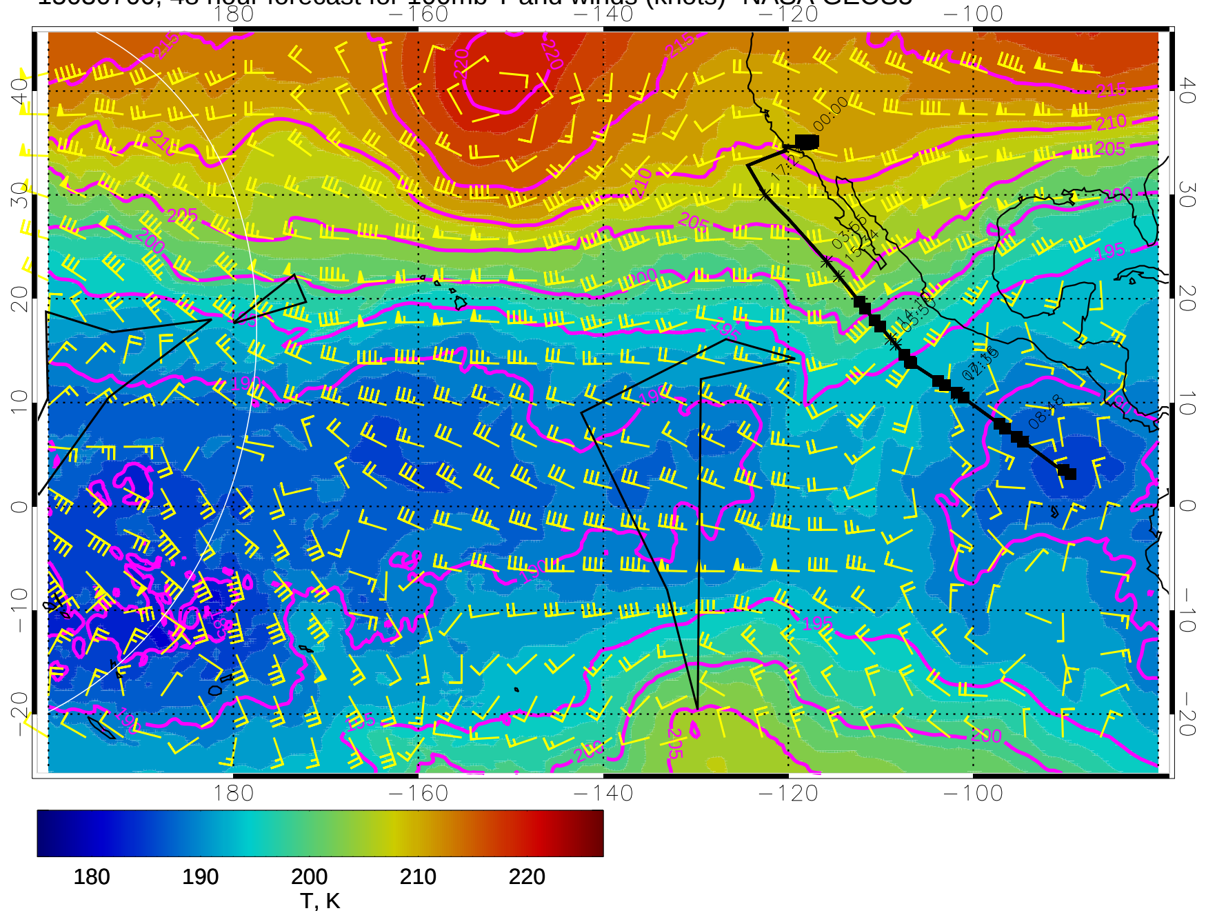
15030700, 48 hour forecast for 100mb T and winds (knots)- NASA GEOS5
