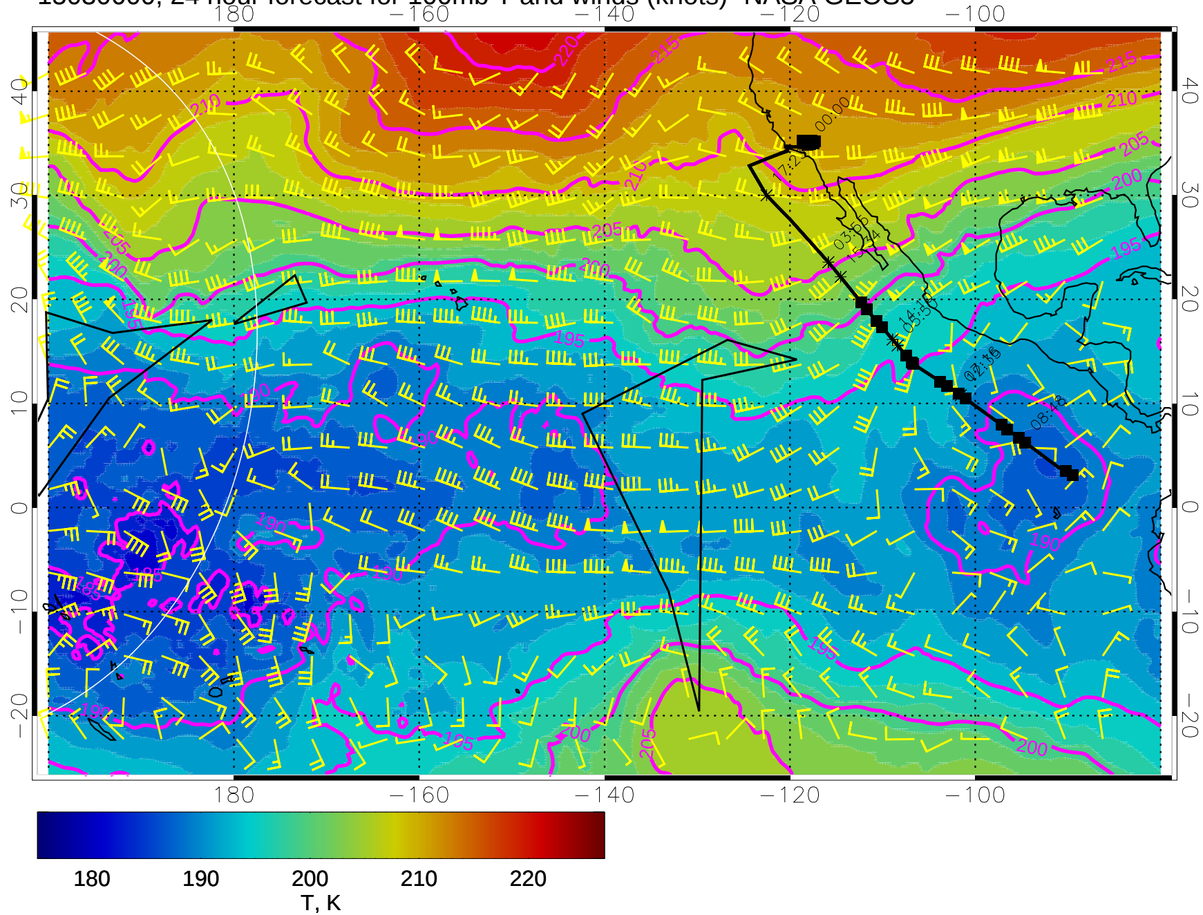
15030600, 24 hour forecast for 100mb T and winds (knots)- NASA GEOS5
