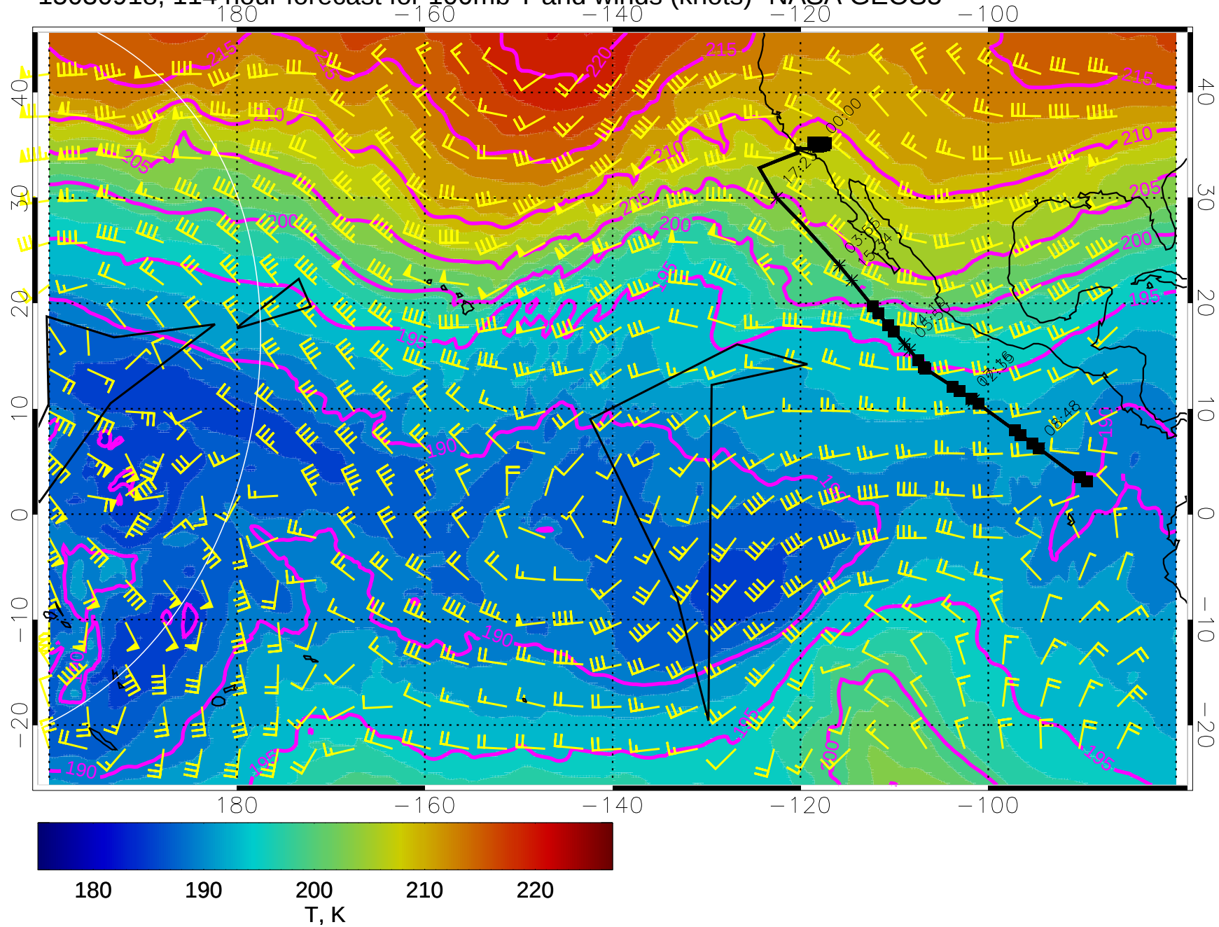
15030918, 114 hour forecast for 100mb T and winds (knots)- NASA GEOS5
