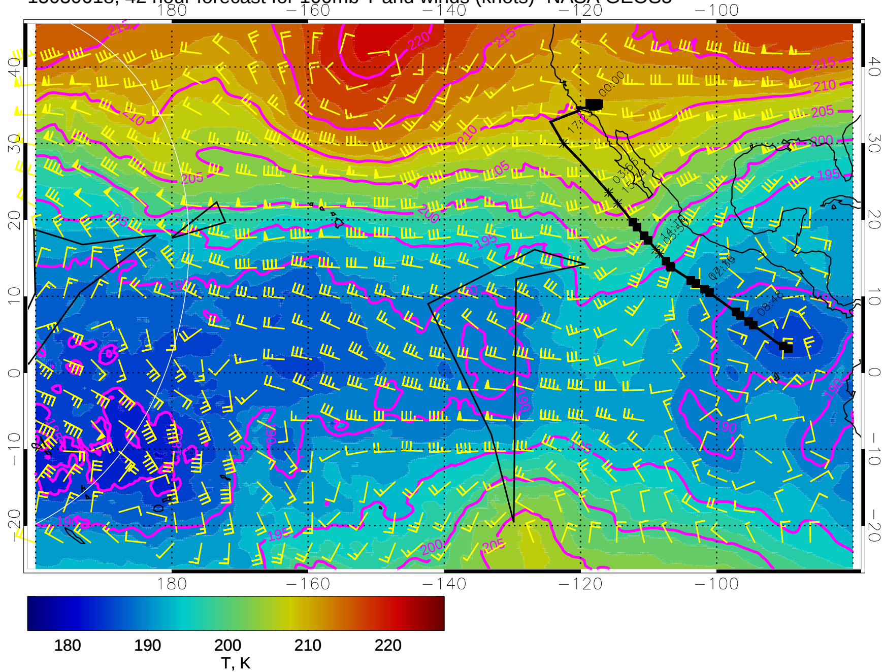
15030618, 42 hour forecast for 100mb T and winds (knots)- NASA GEOS5
