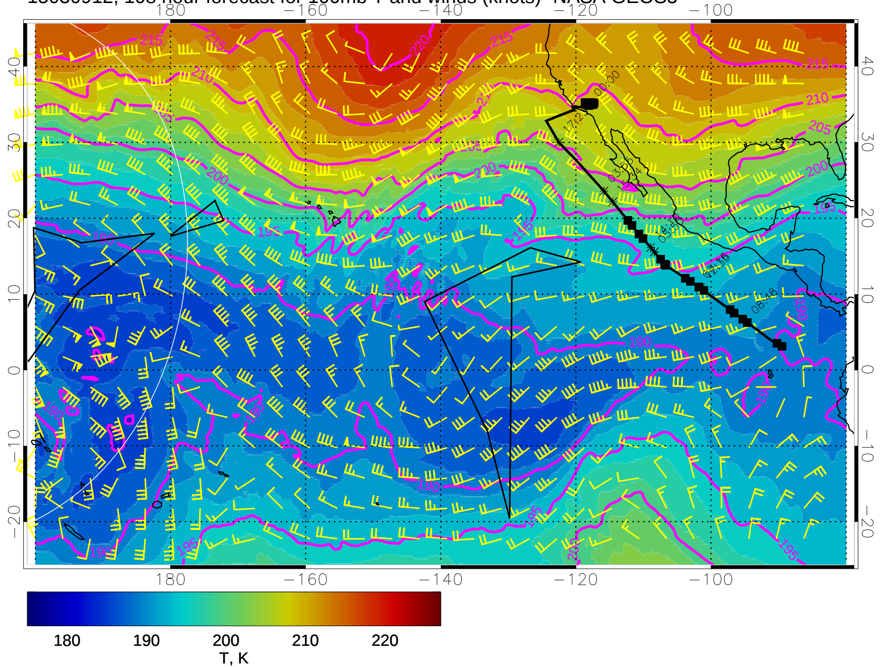
15030912, 108 hour forecast for 100mb T and winds (knots)- NASA GEOS5
