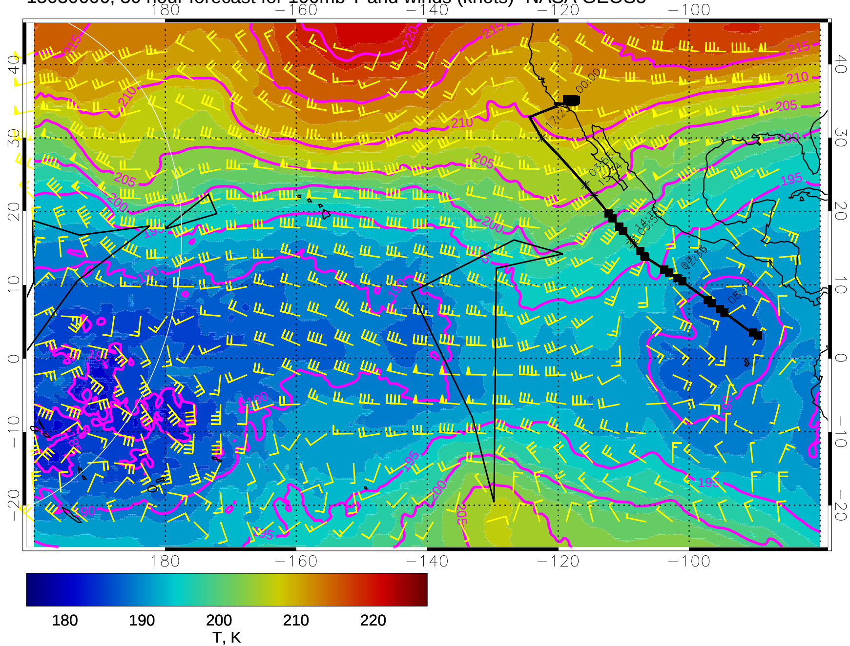
15030606, 30 hour forecast for 100mb T and winds (knots)- NASA GEOS5
