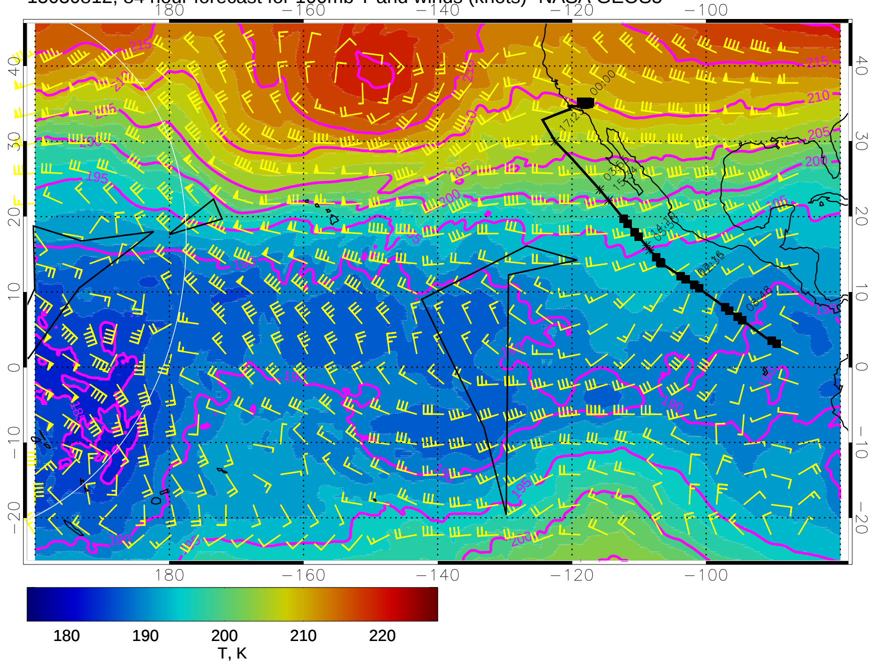
15030812, 84 hour forecast for 100mb T and winds (knots)- NASA GEOS5
