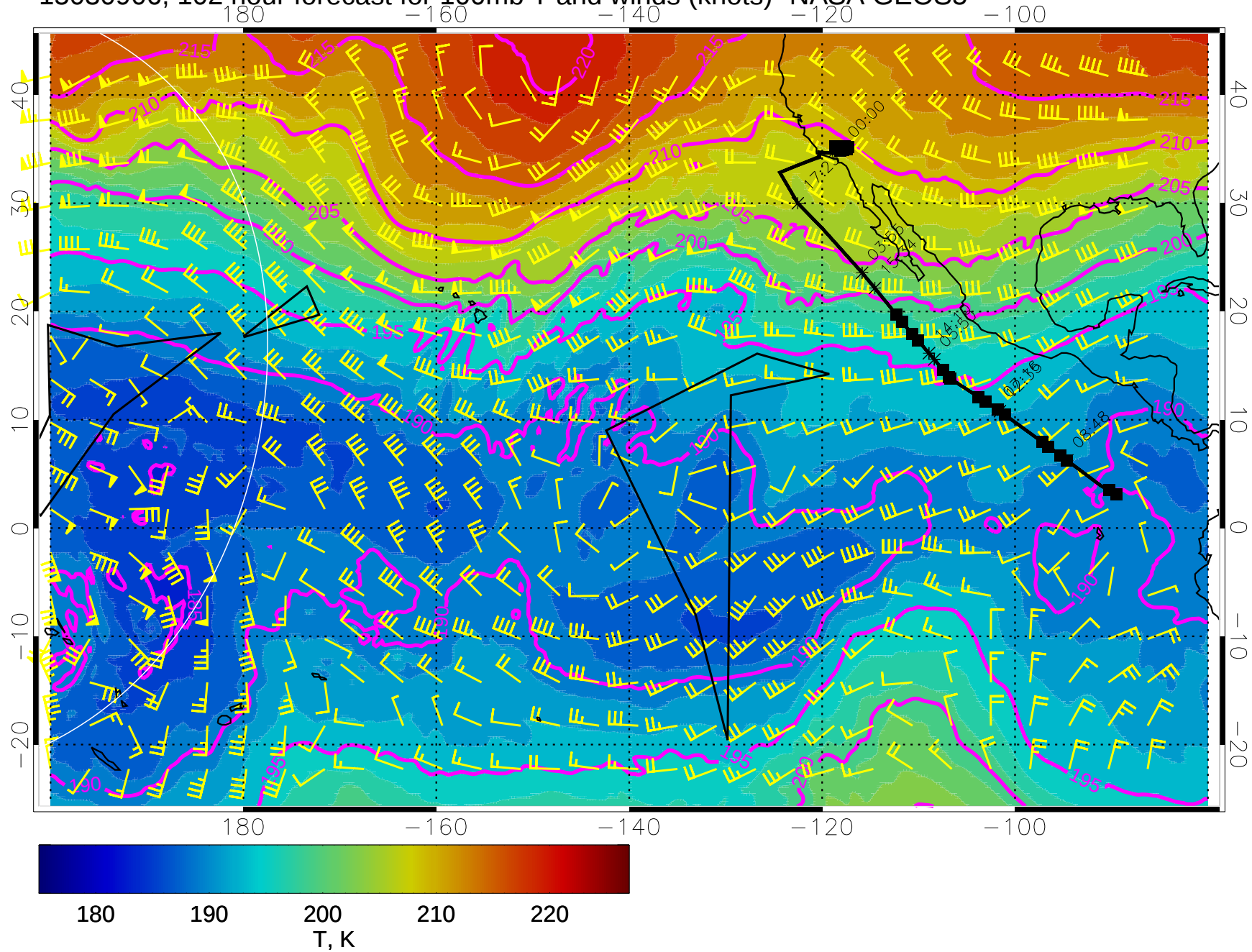
15030906, 102 hour forecast for 100mb T and winds (knots)- NASA GEOS5
