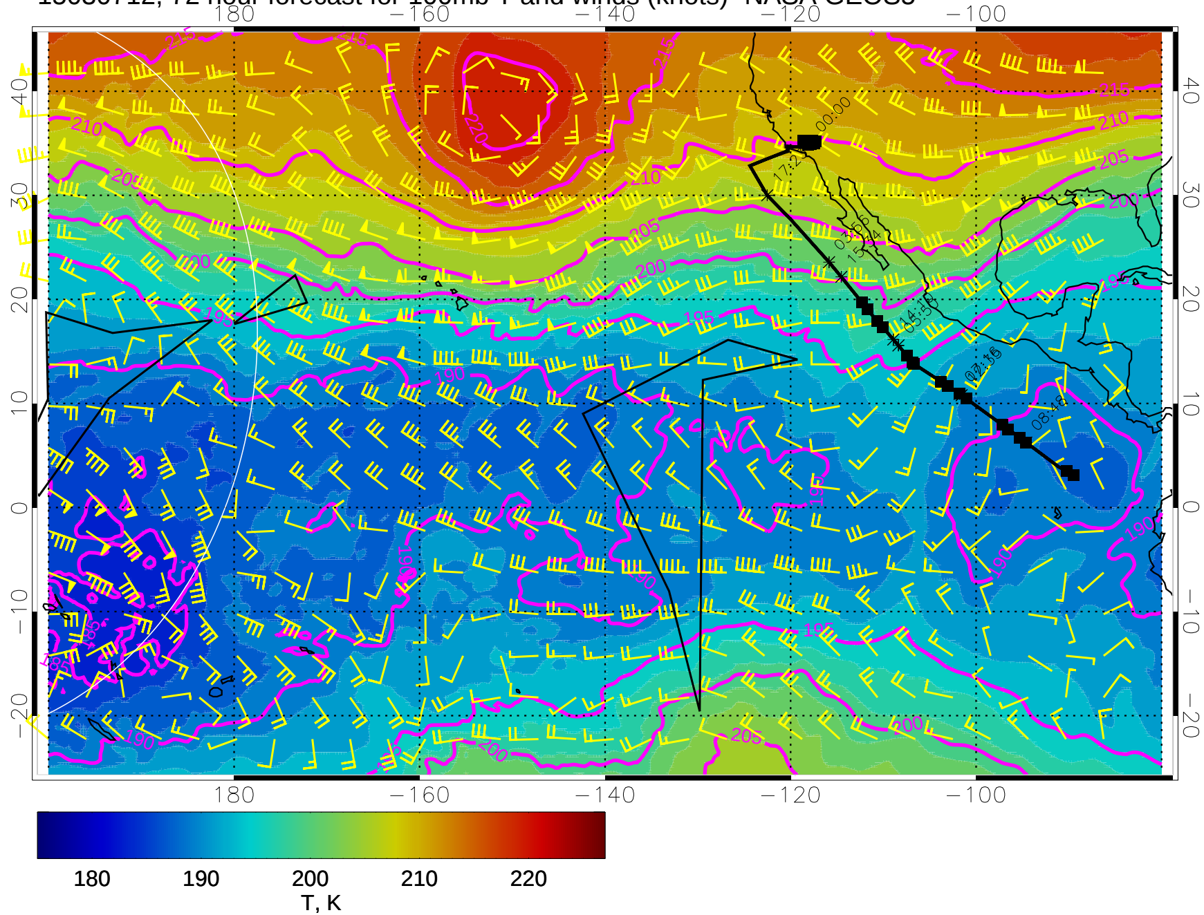
15030712, 72 hour forecast for 100mb T and winds (knots)- NASA GEOS5
