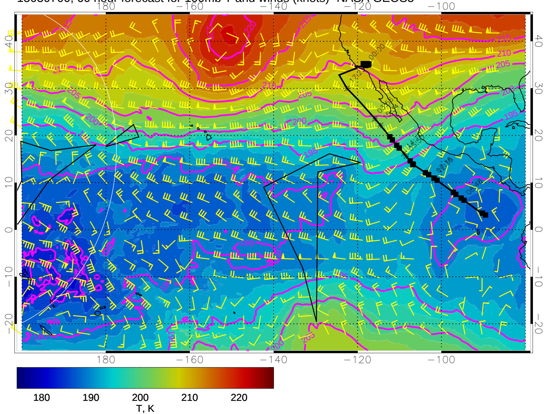
15030700, 60 hour forecast for 100mb T and winds (knots)- NASA GEOS5
