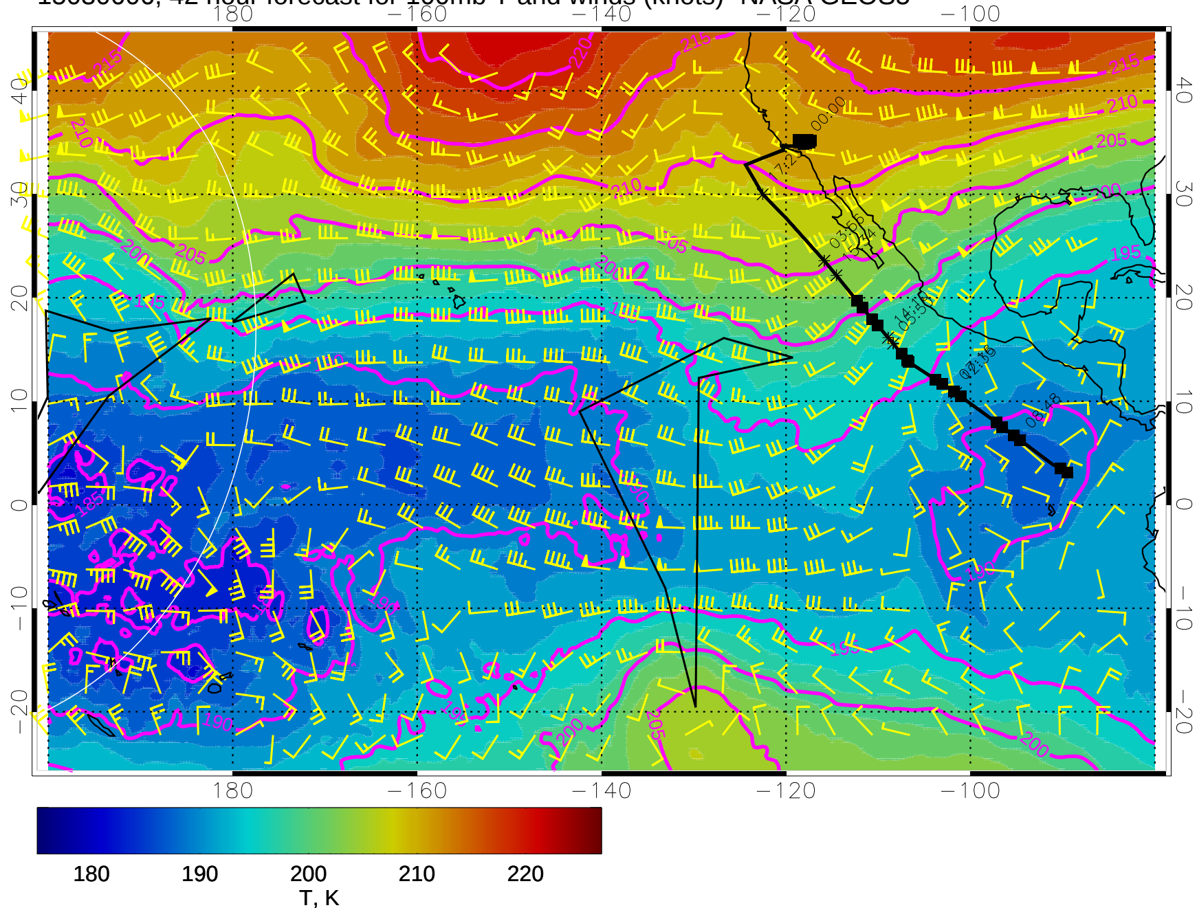
15030606, 42 hour forecast for 100mb T and winds (knots)- NASA GEOS5
