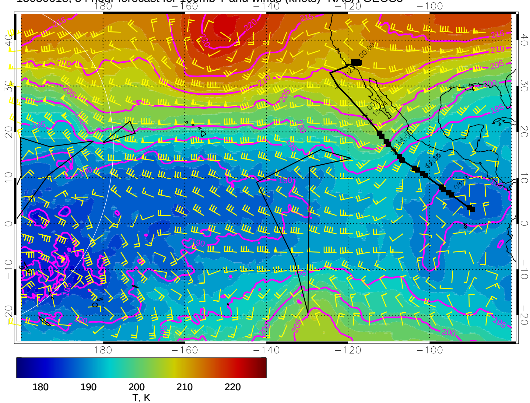
15030618, 54 hour forecast for 100mb T and winds (knots)- NASA GEOS5
