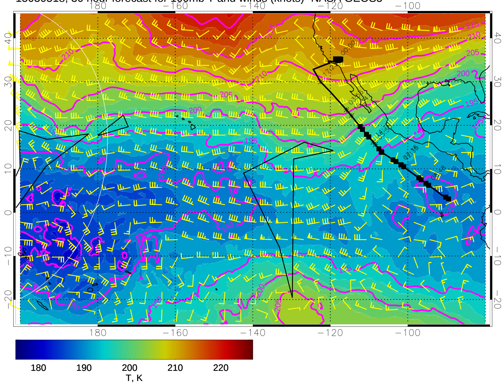
15030518, 30 hour forecast for 100mb T and winds (knots)- NASA GEOS5
