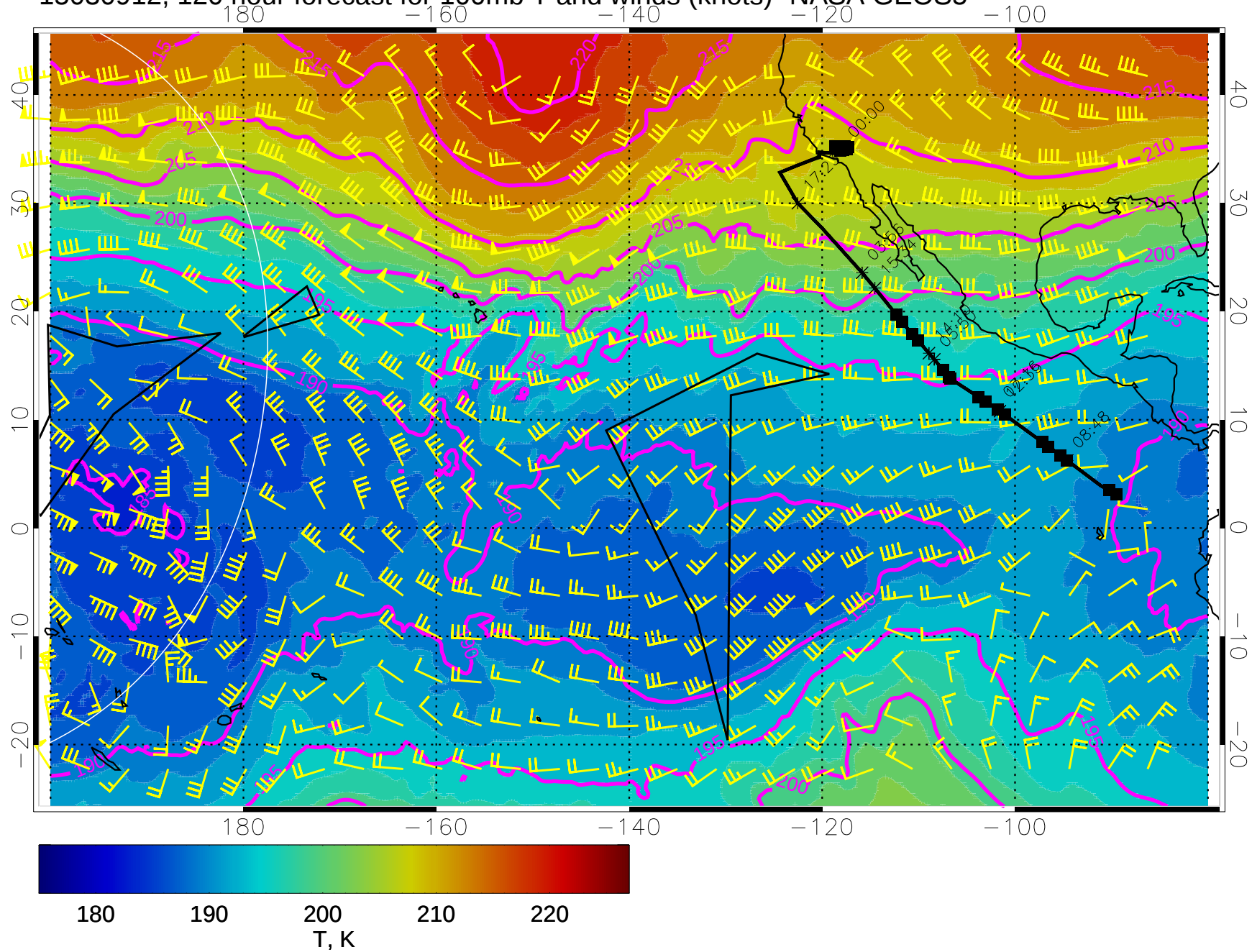
15030912, 120 hour forecast for 100mb T and winds (knots)- NASA GEOS5
