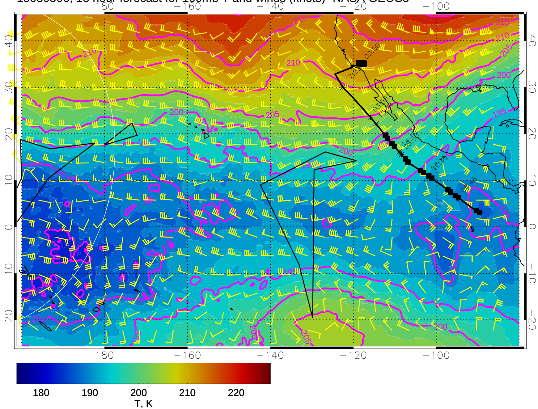
15030506, 18 hour forecast for 100mb T and winds (knots)- NASA GEOS5
