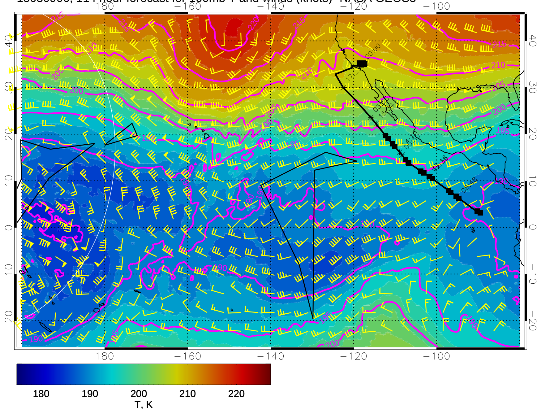
15030906, 114 hour forecast for 100mb T and winds (knots)- NASA GEOS5
