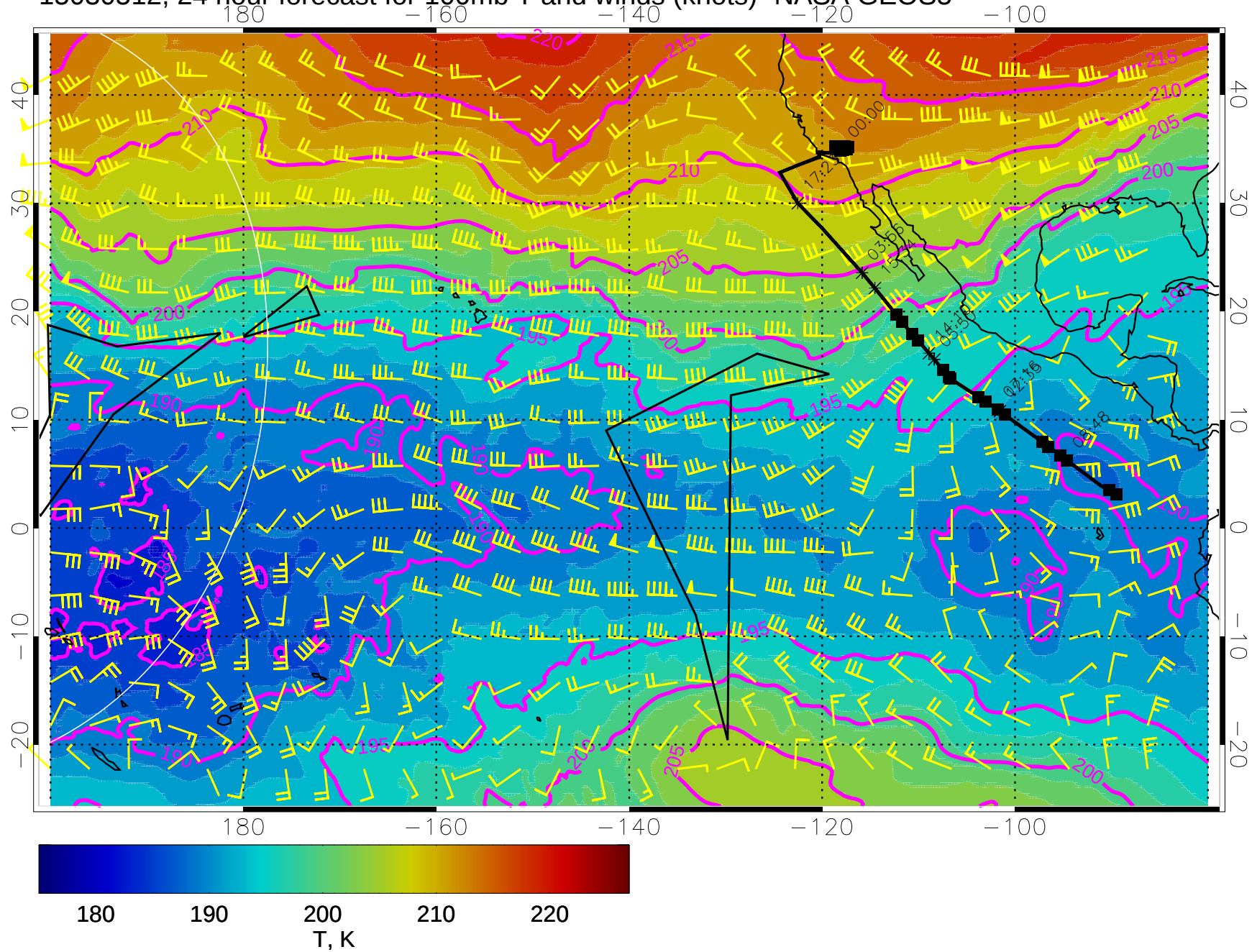
15030512, 24 hour forecast for 100mb T and winds (knots)- NASA GEOS5
