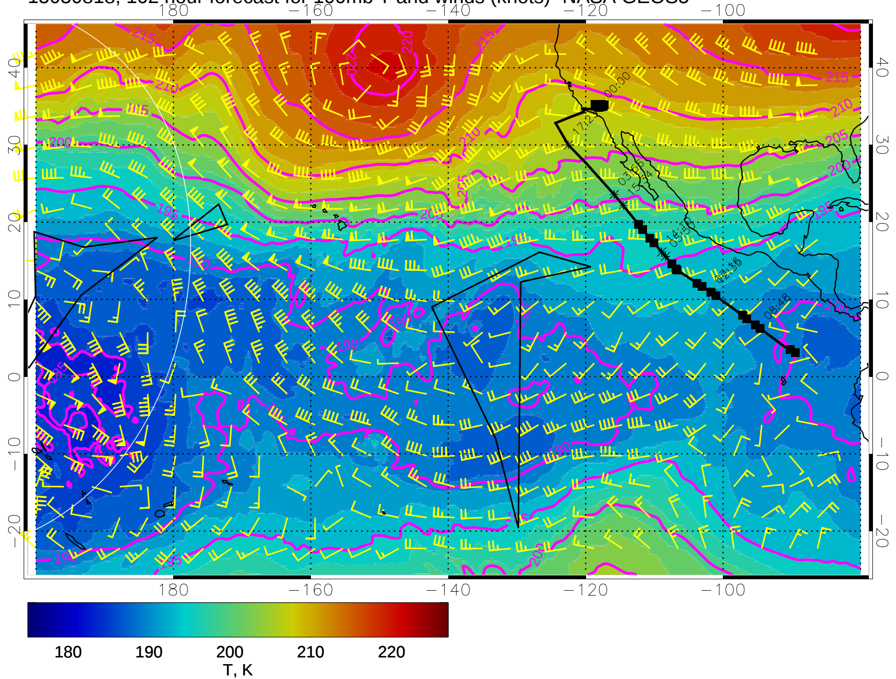
15030818, 102 hour forecast for 100mb T and winds (knots)- NASA GEOS5
