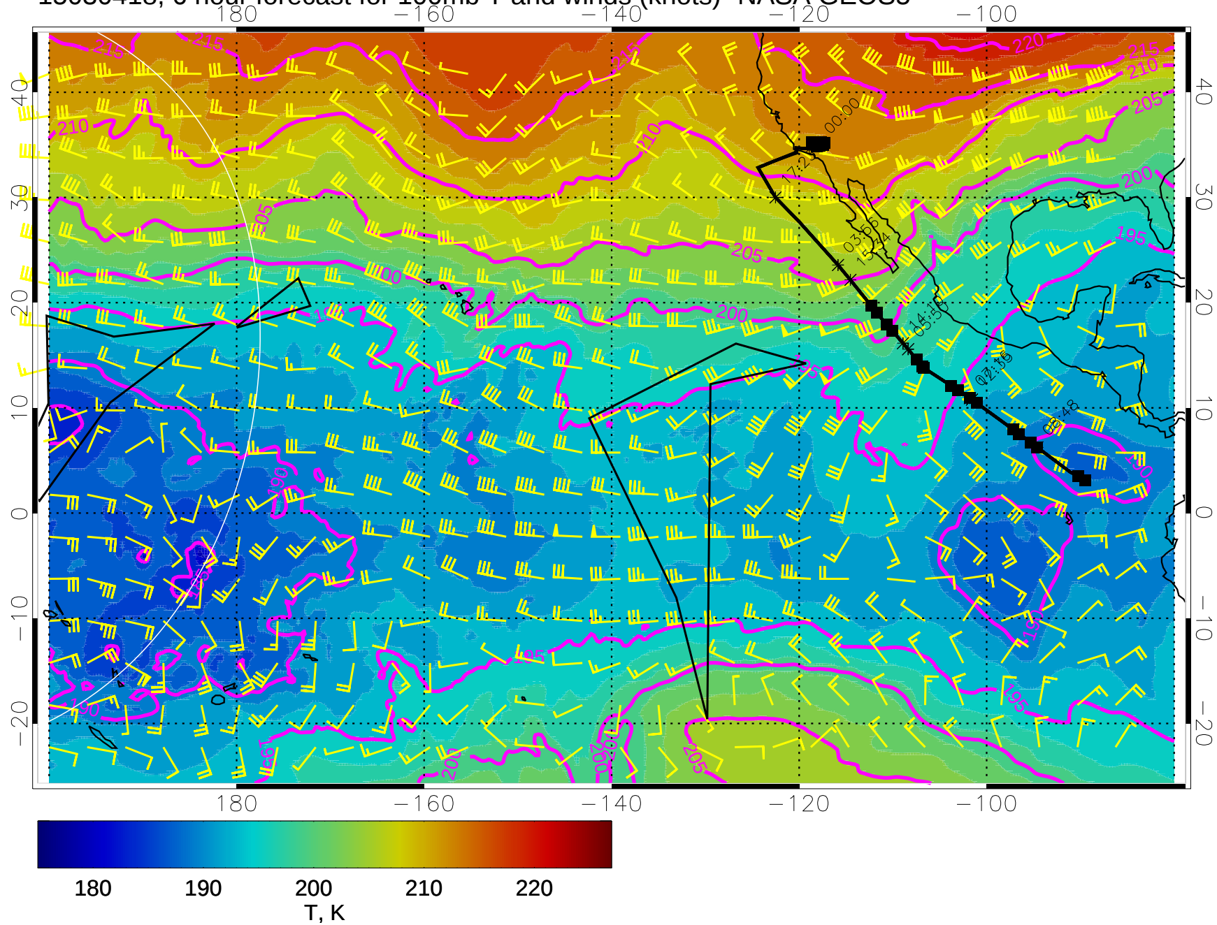
15030418, 6 hour forecast for 100mb T and winds (knots)- NASA GEOS5
