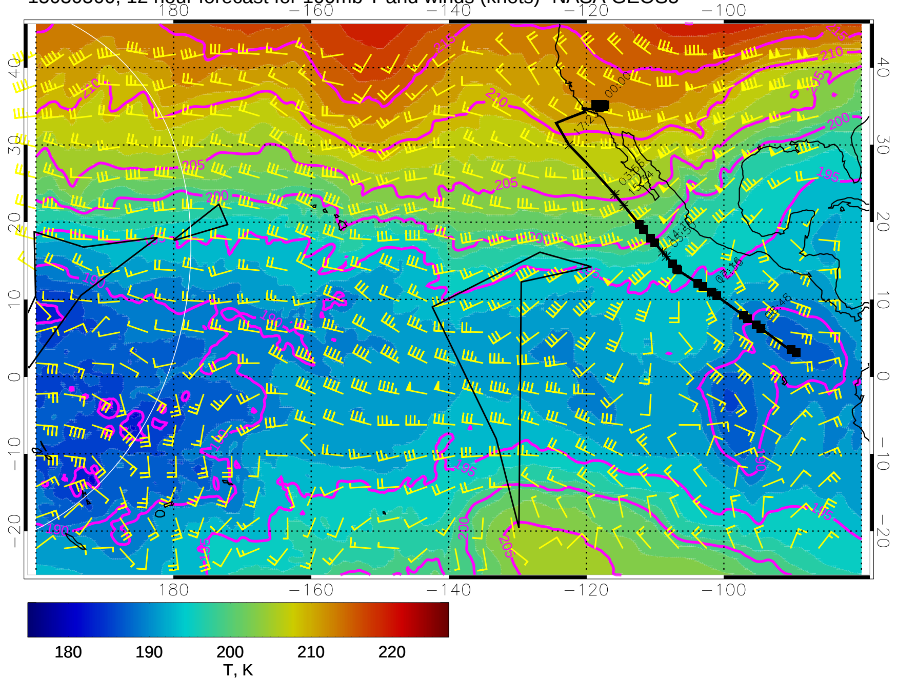
15030500, 12 hour forecast for 100mb T and winds (knots)- NASA GEOS5
