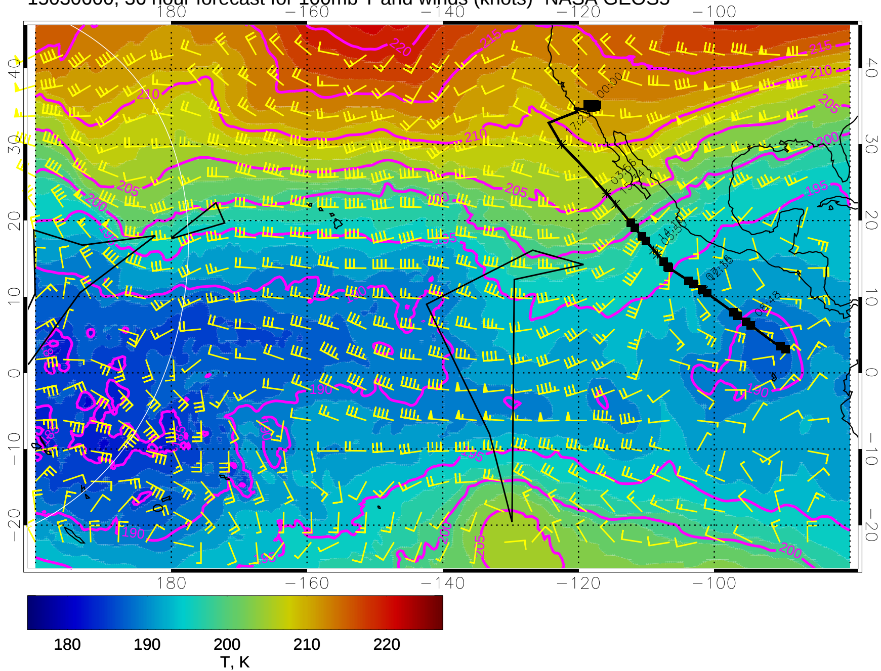
15030600, 36 hour forecast for 100mb T and winds (knots)- NASA GEOS5
