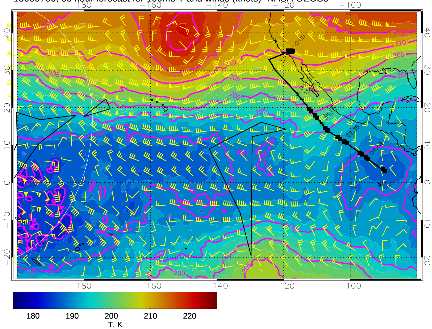
15030706, 66 hour forecast for 100mb T and winds (knots)- NASA GEOS5
