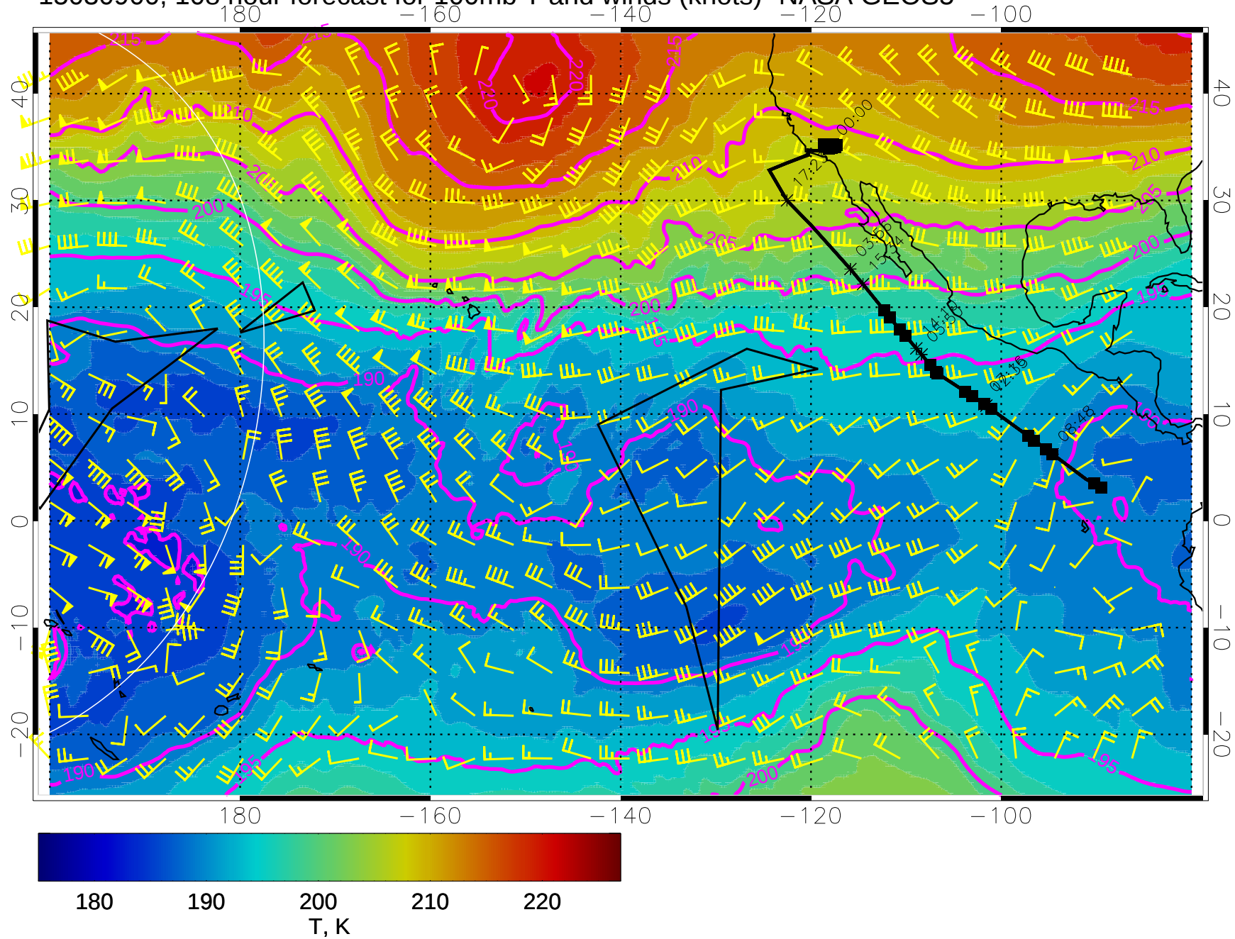
15030900, 108 hour forecast for 100mb T and winds (knots)- NASA GEOS5
