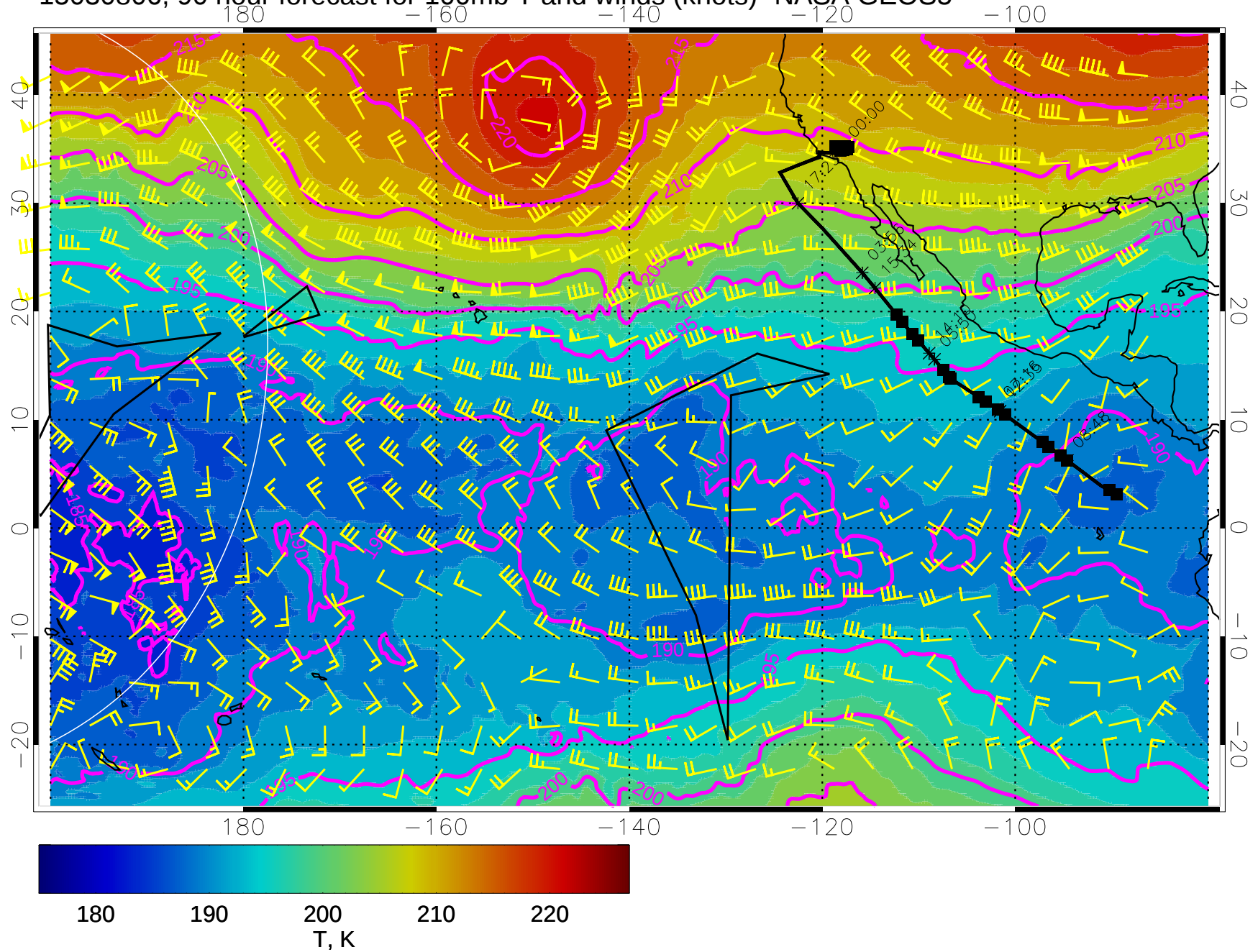
15030806, 90 hour forecast for 100mb T and winds (knots)- NASA GEOS5
