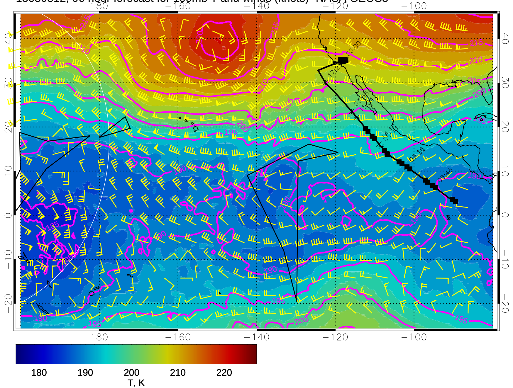
15030812, 96 hour forecast for 100mb T and winds (knots)- NASA GEOS5
