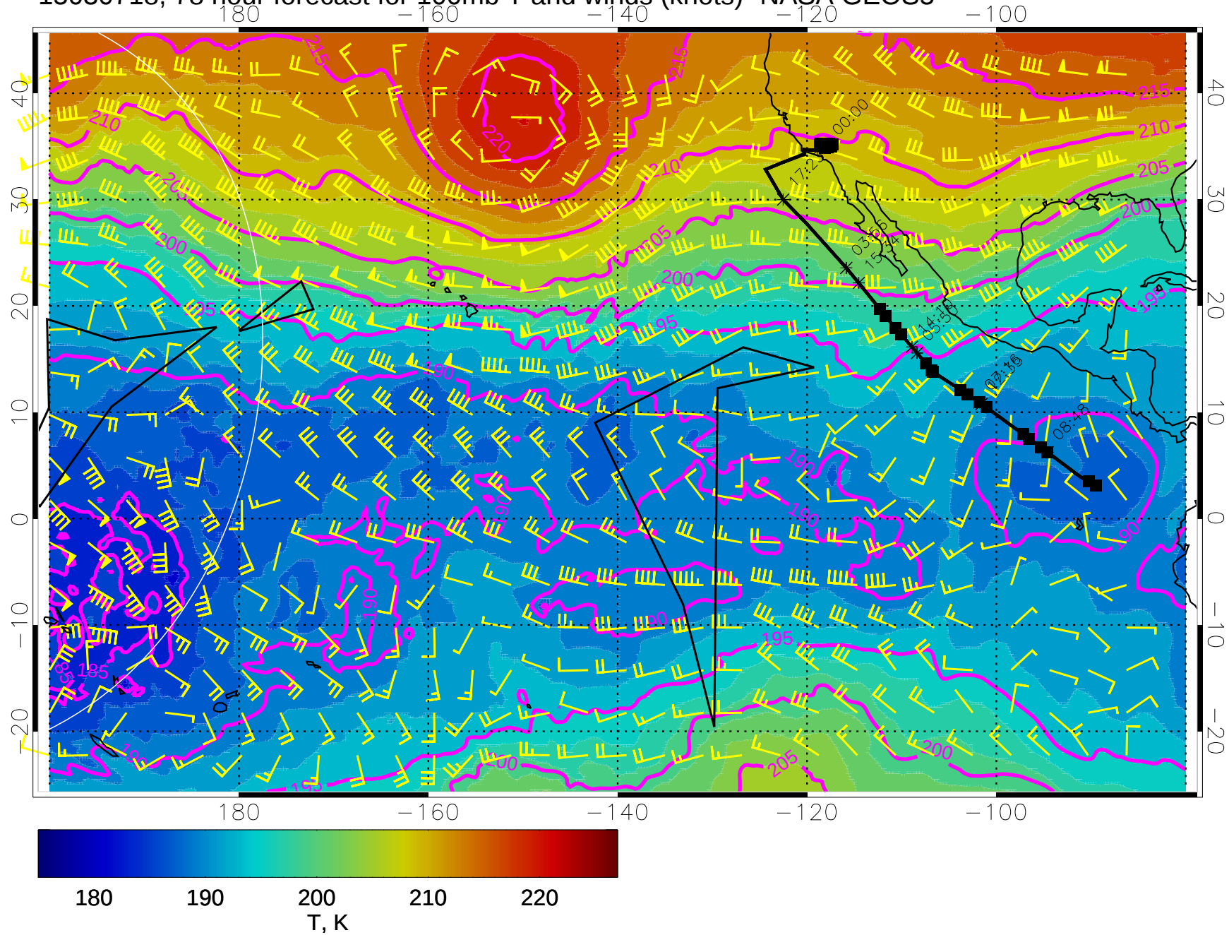
15030718, 78 hour forecast for 100mb T and winds (knots)- NASA GEOS5
