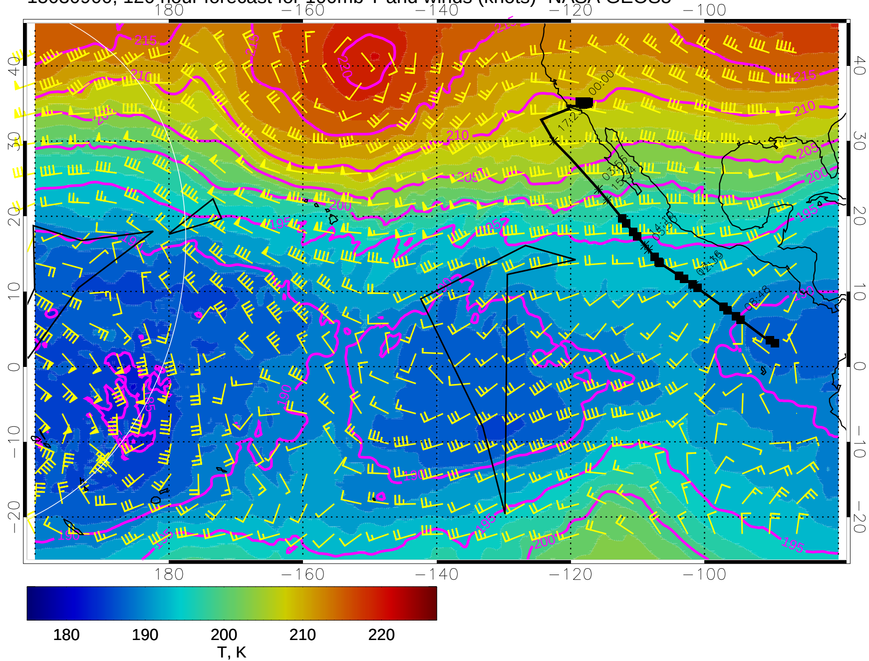
15030900, 120 hour forecast for 100mb T and winds (knots)- NASA GEOS5
