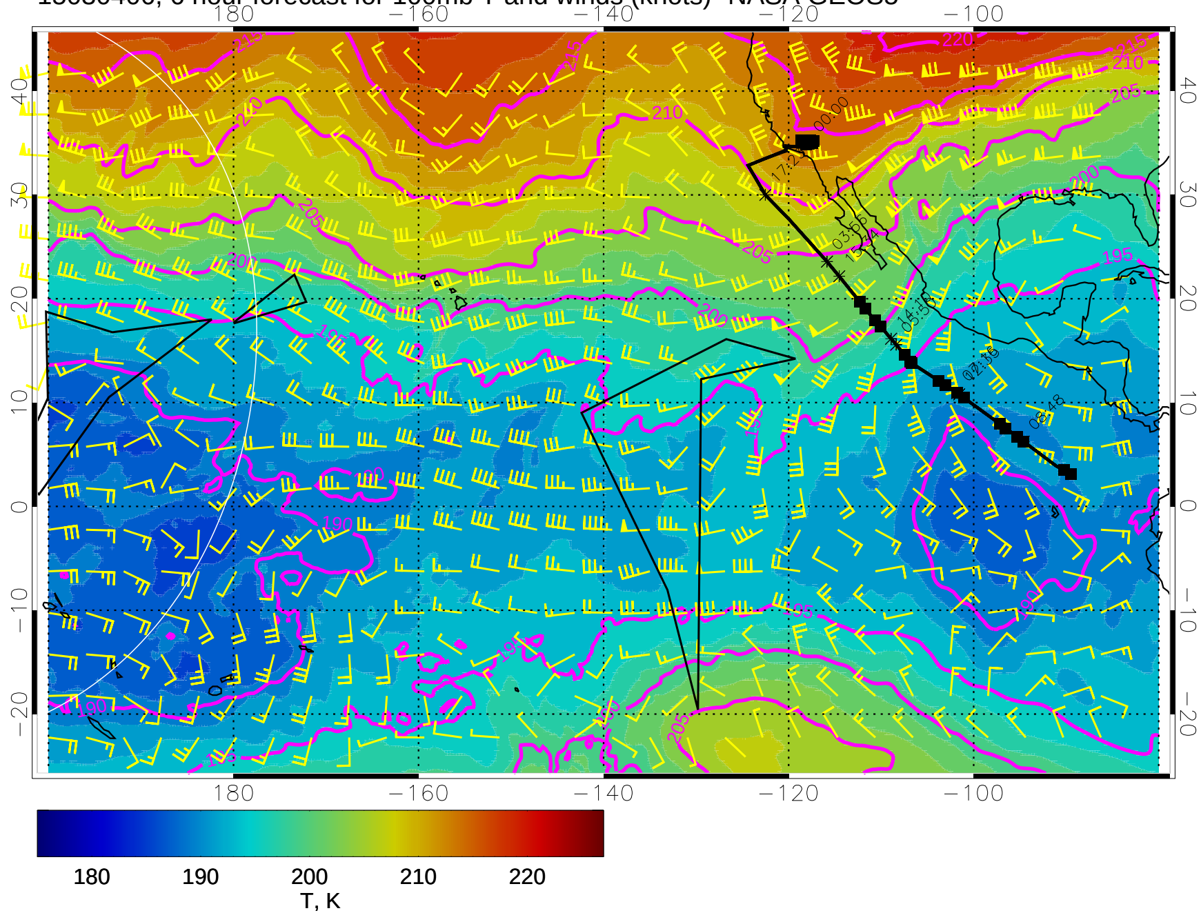
15030406, 6 hour forecast for 100mb T and winds (knots)- NASA GEOS5
