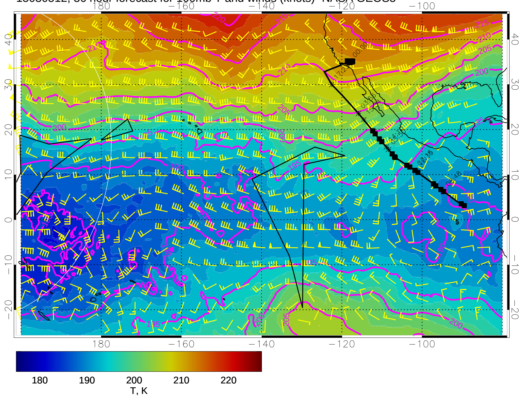
15030512, 36 hour forecast for 100mb T and winds (knots)- NASA GEOS5
