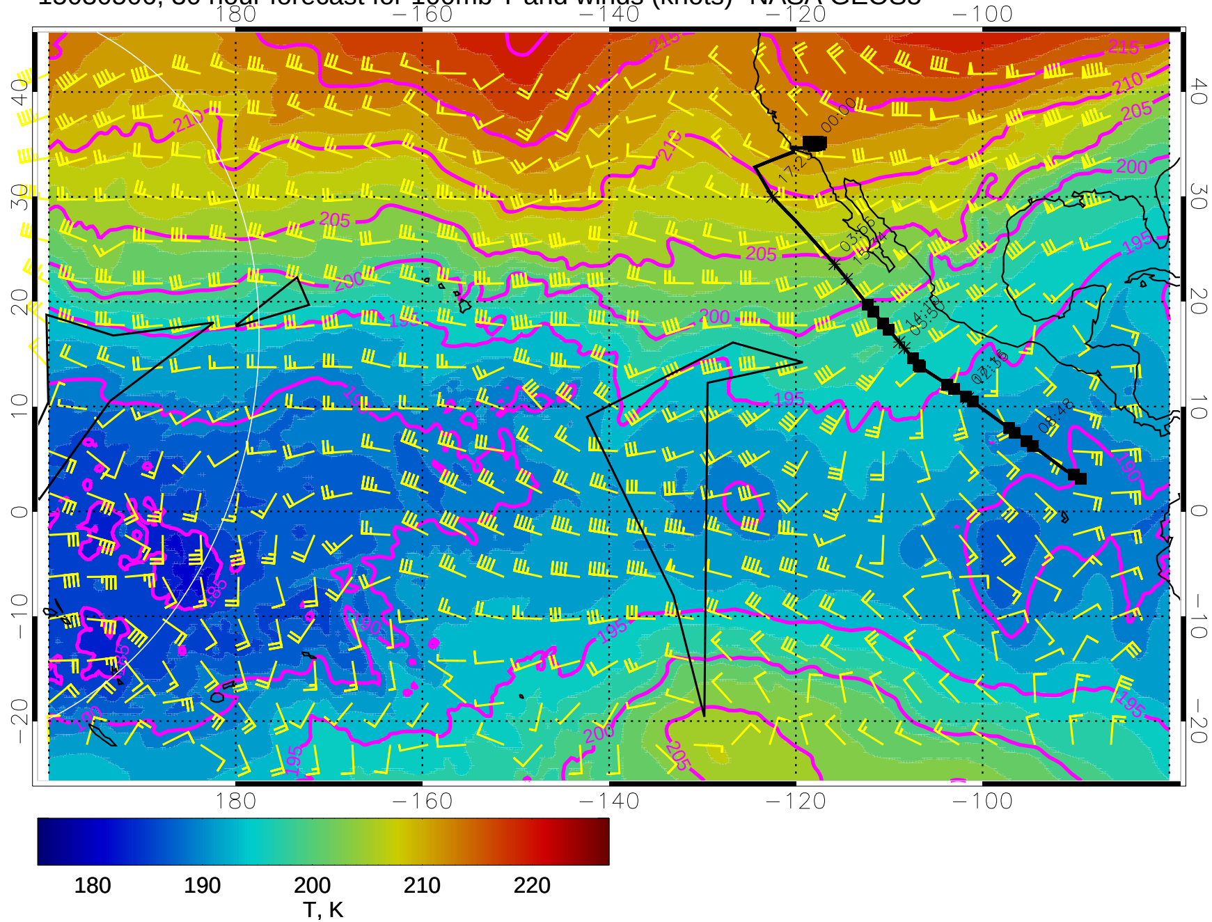
15030506, 30 hour forecast for 100mb T and winds (knots)- NASA GEOS5
