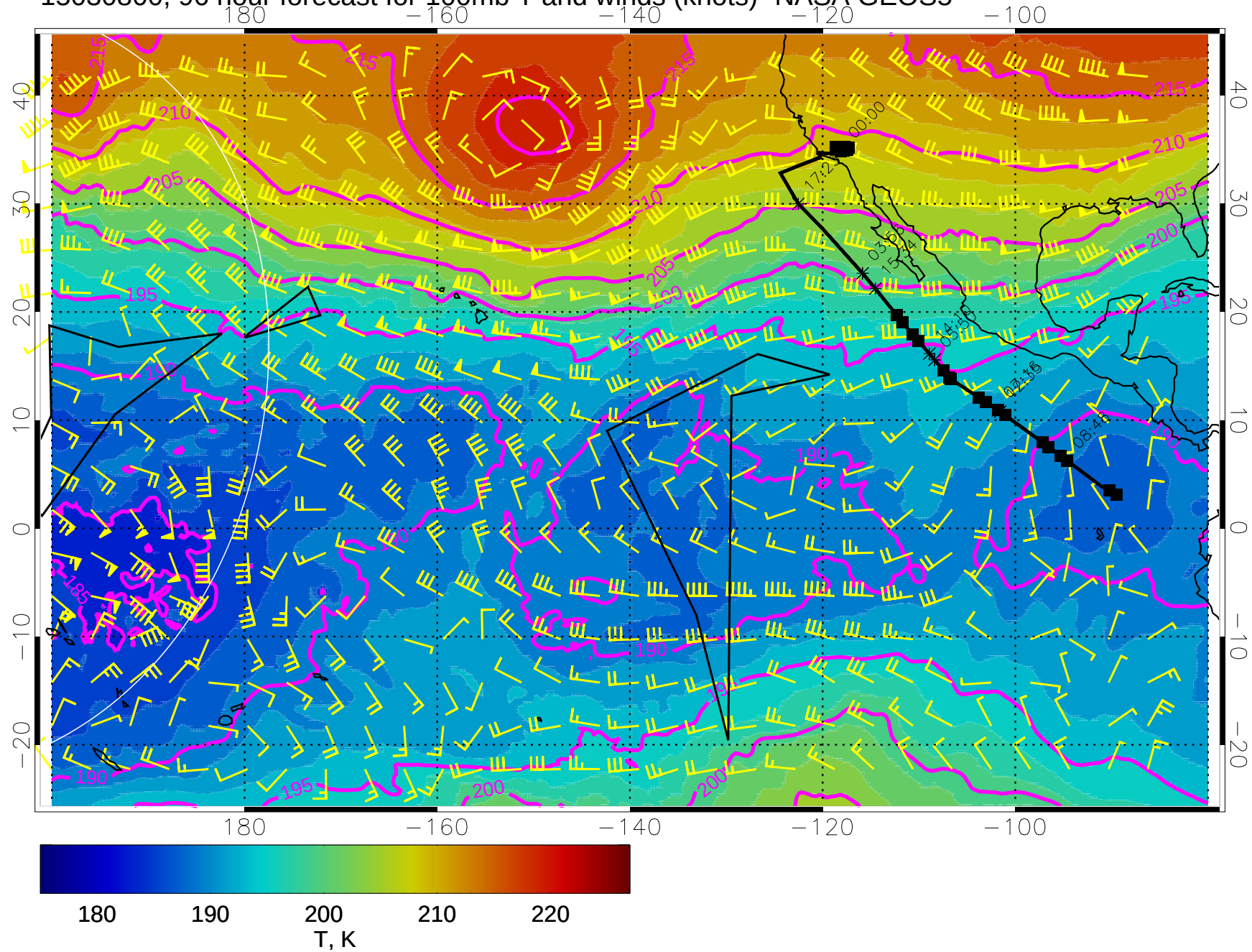
15030800, 96 hour forecast for 100mb T and winds (knots)- NASA GEOS5
