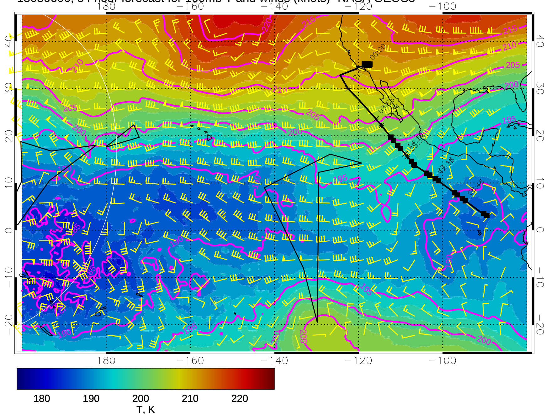
15030606, 54 hour forecast for 100mb T and winds (knots)- NASA GEOS5
