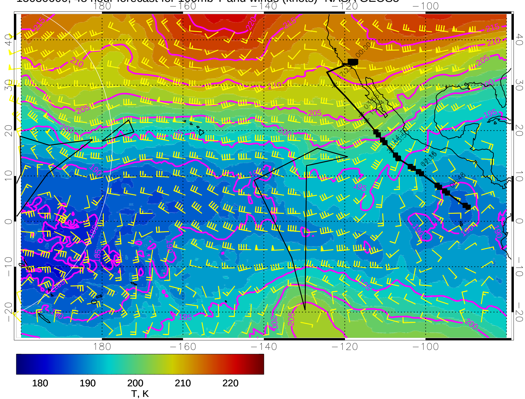
15030600, 48 hour forecast for 100mb T and winds (knots)- NASA GEOS5
