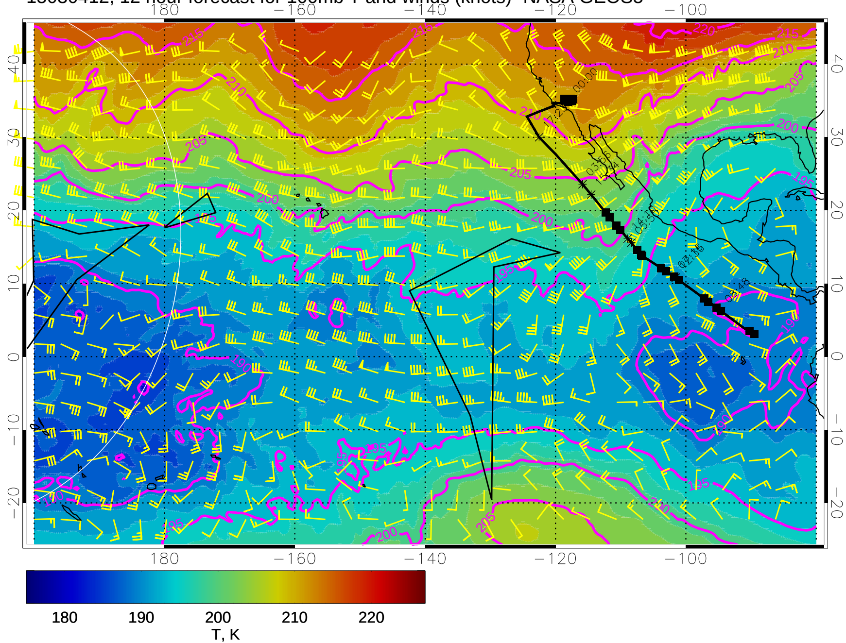
15030412, 12 hour forecast for 100mb T and winds (knots)- NASA GEOS5
