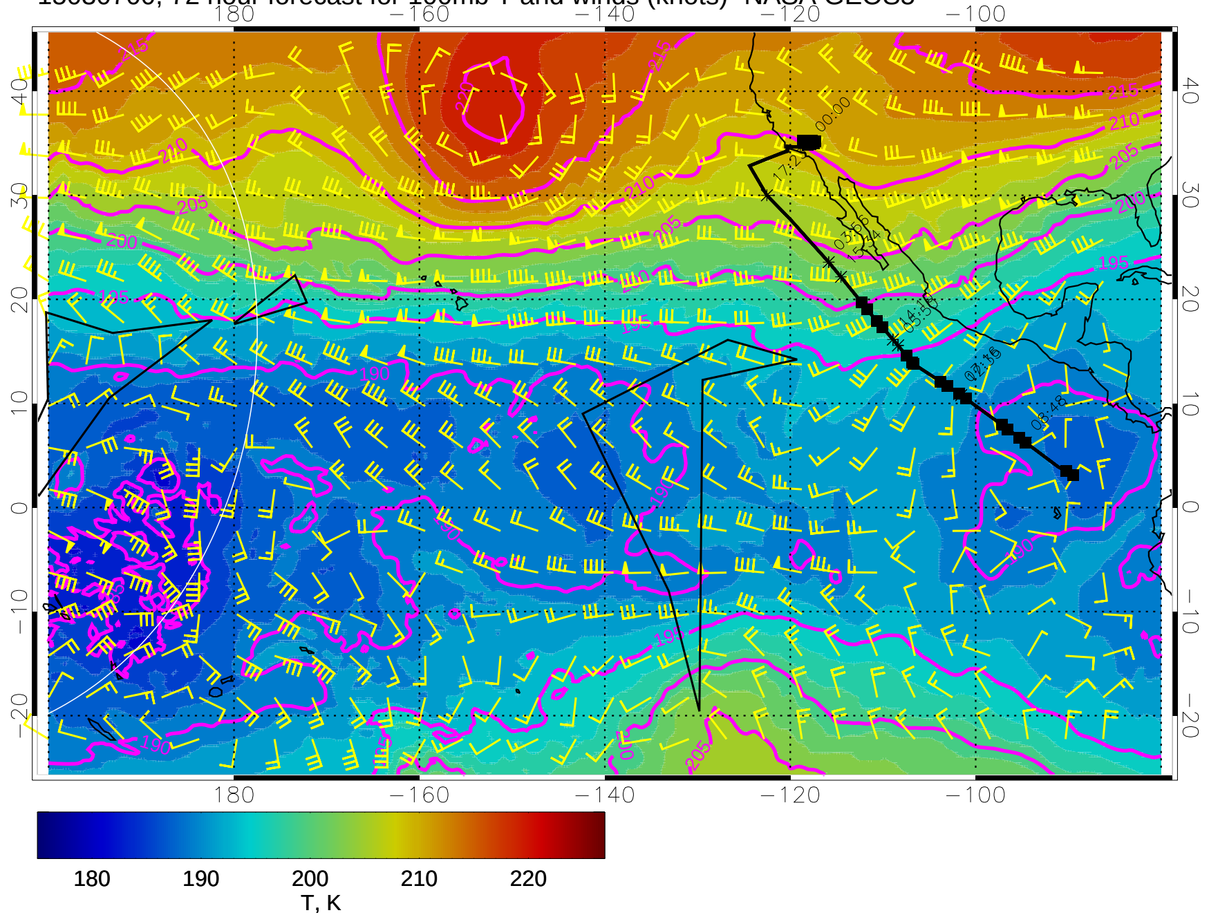
15030700, 72 hour forecast for 100mb T and winds (knots)- NASA GEOS5
