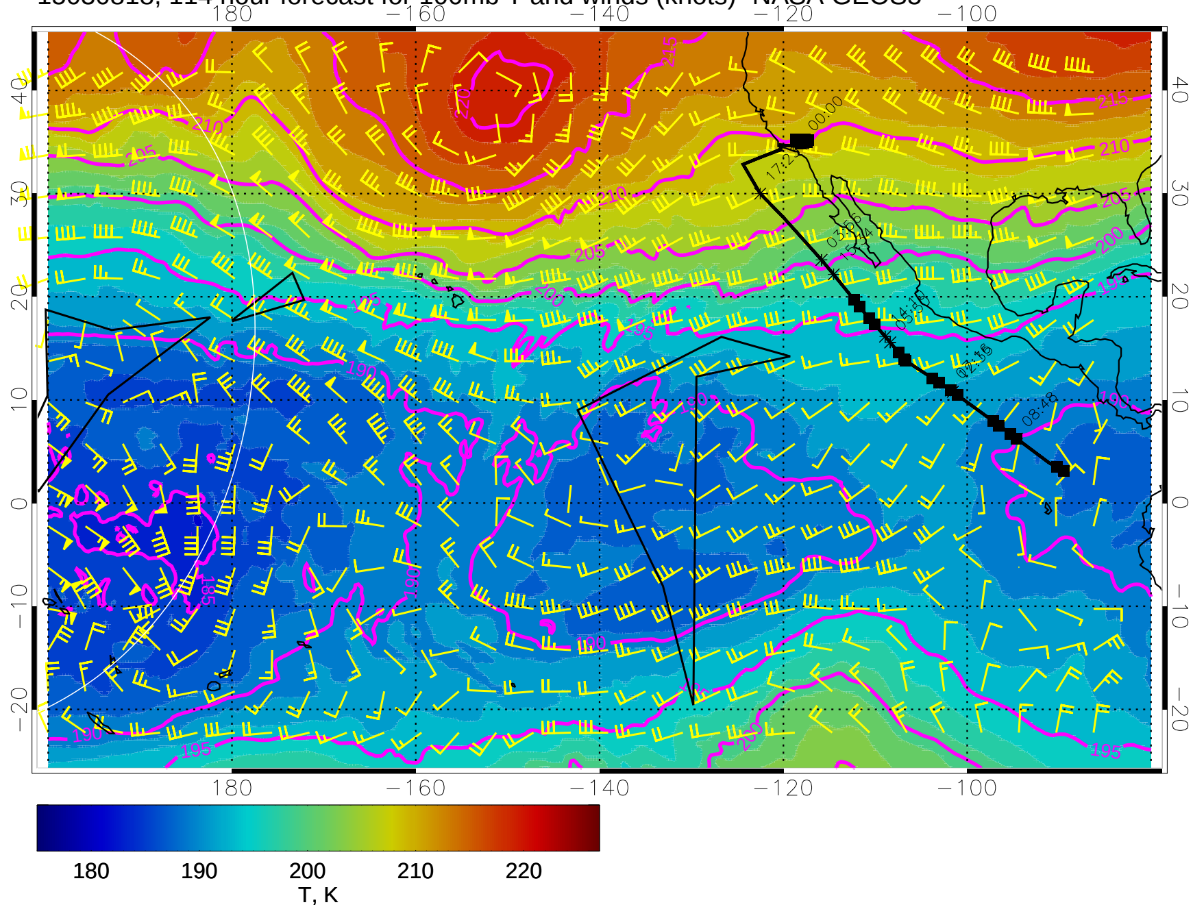
15030818, 114 hour forecast for 100mb T and winds (knots)- NASA GEOS5
