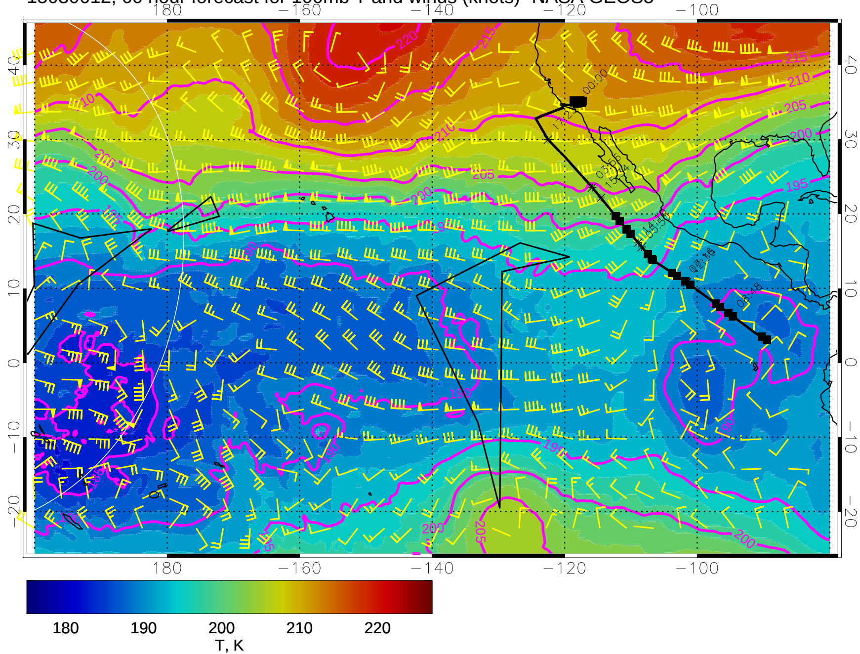
15030612, 60 hour forecast for 100mb T and winds (knots)- NASA GEOS5
