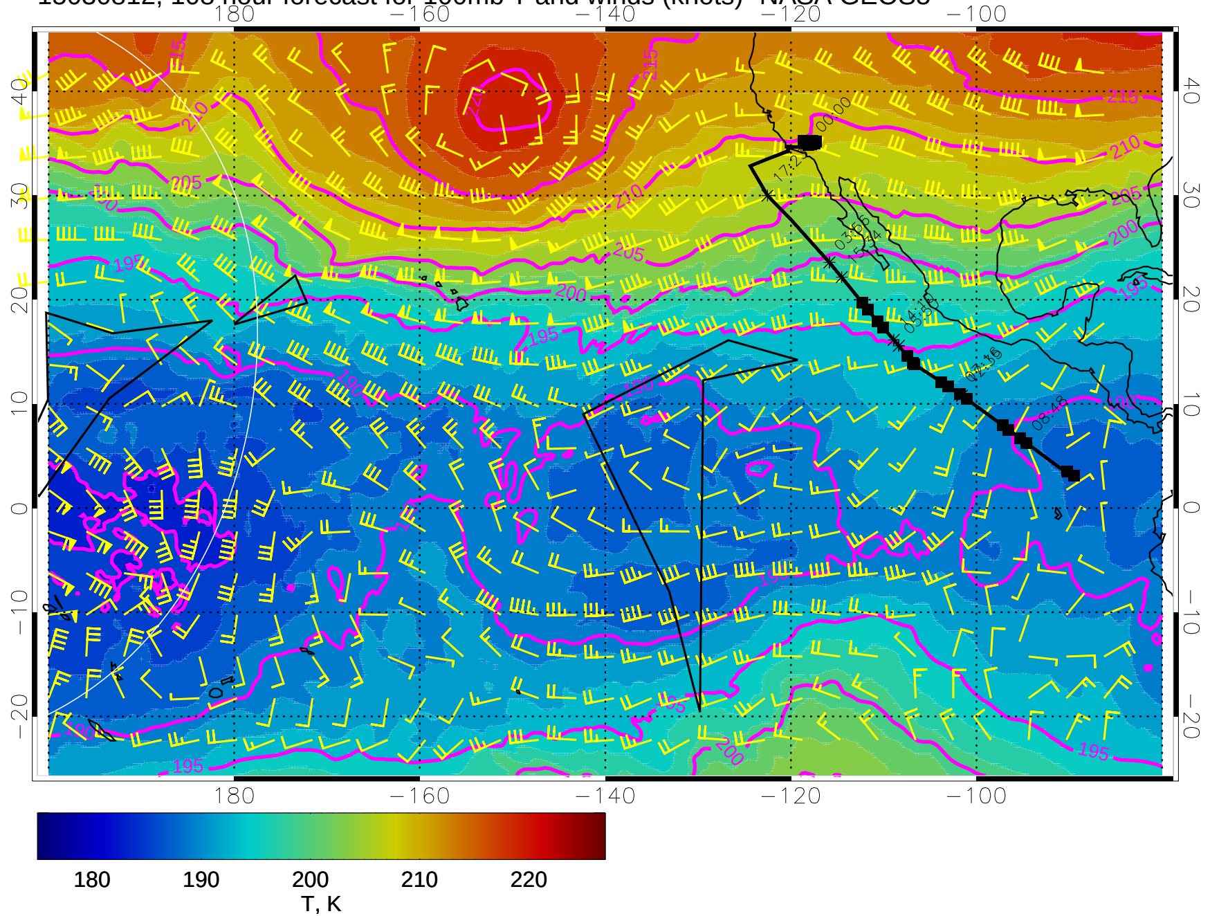
15030812, 108 hour forecast for 100mb T and winds (knots)- NASA GEOS5
