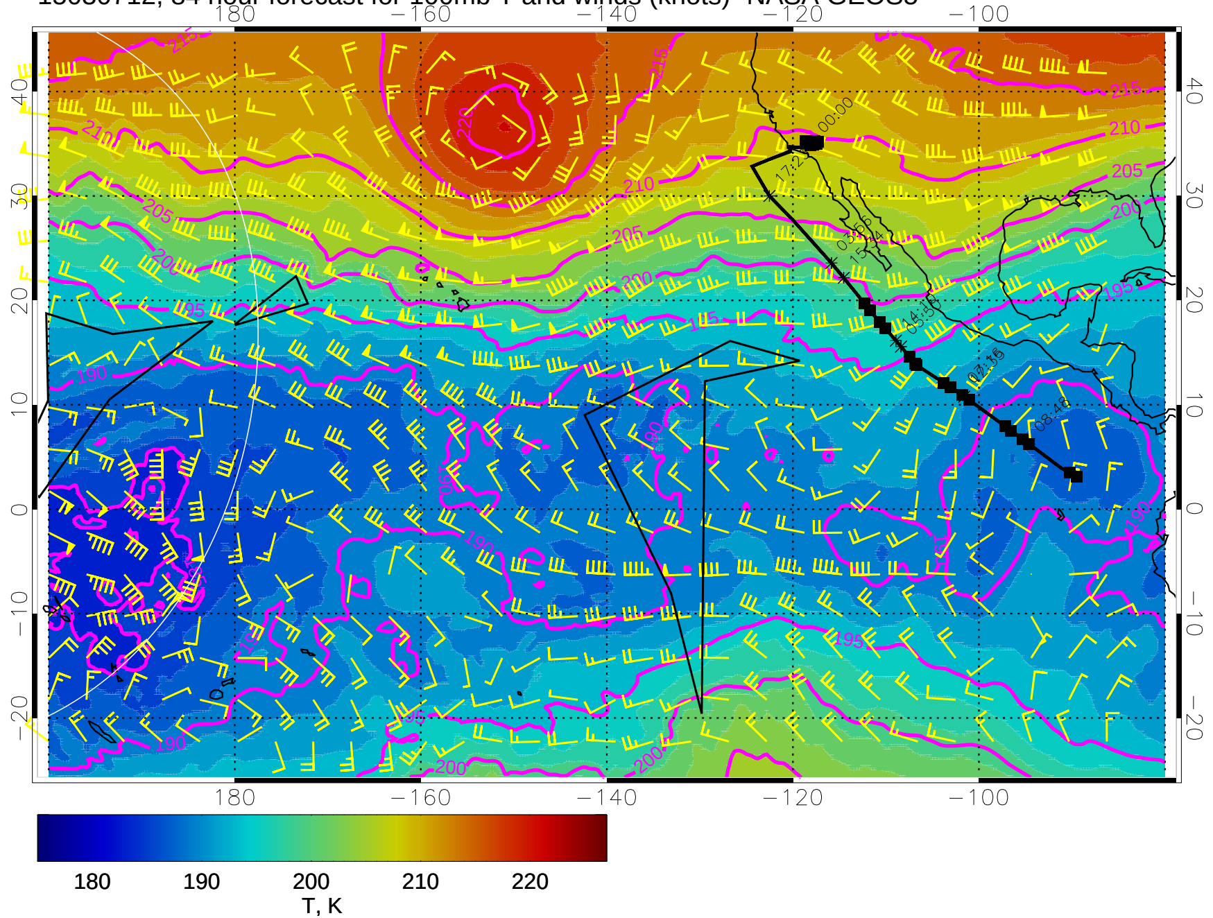
15030712, 84 hour forecast for 100mb T and winds (knots)- NASA GEOS5
