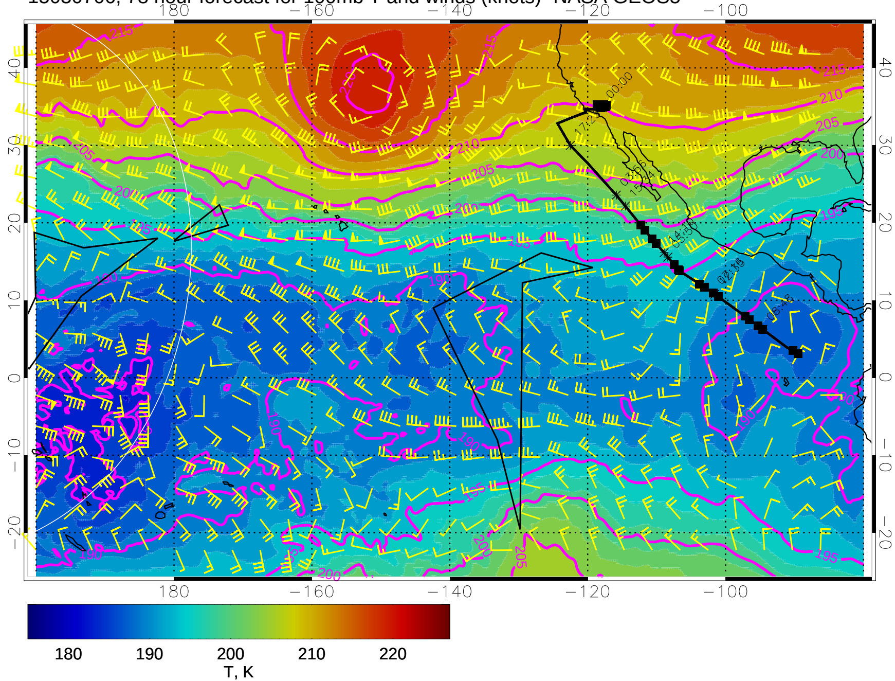
15030706, 78 hour forecast for 100mb T and winds (knots)- NASA GEOS5
