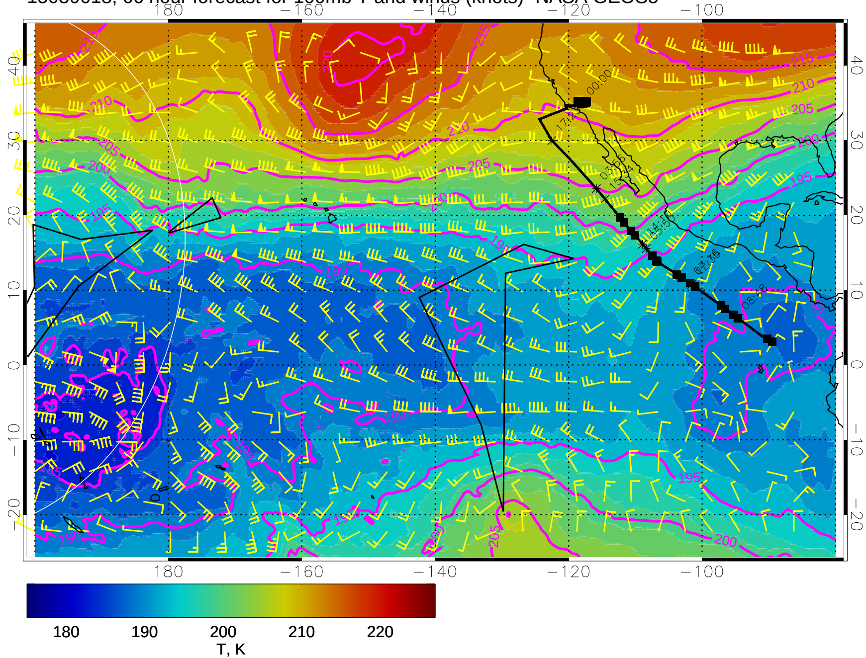
15030618, 66 hour forecast for 100mb T and winds (knots)- NASA GEOS5
