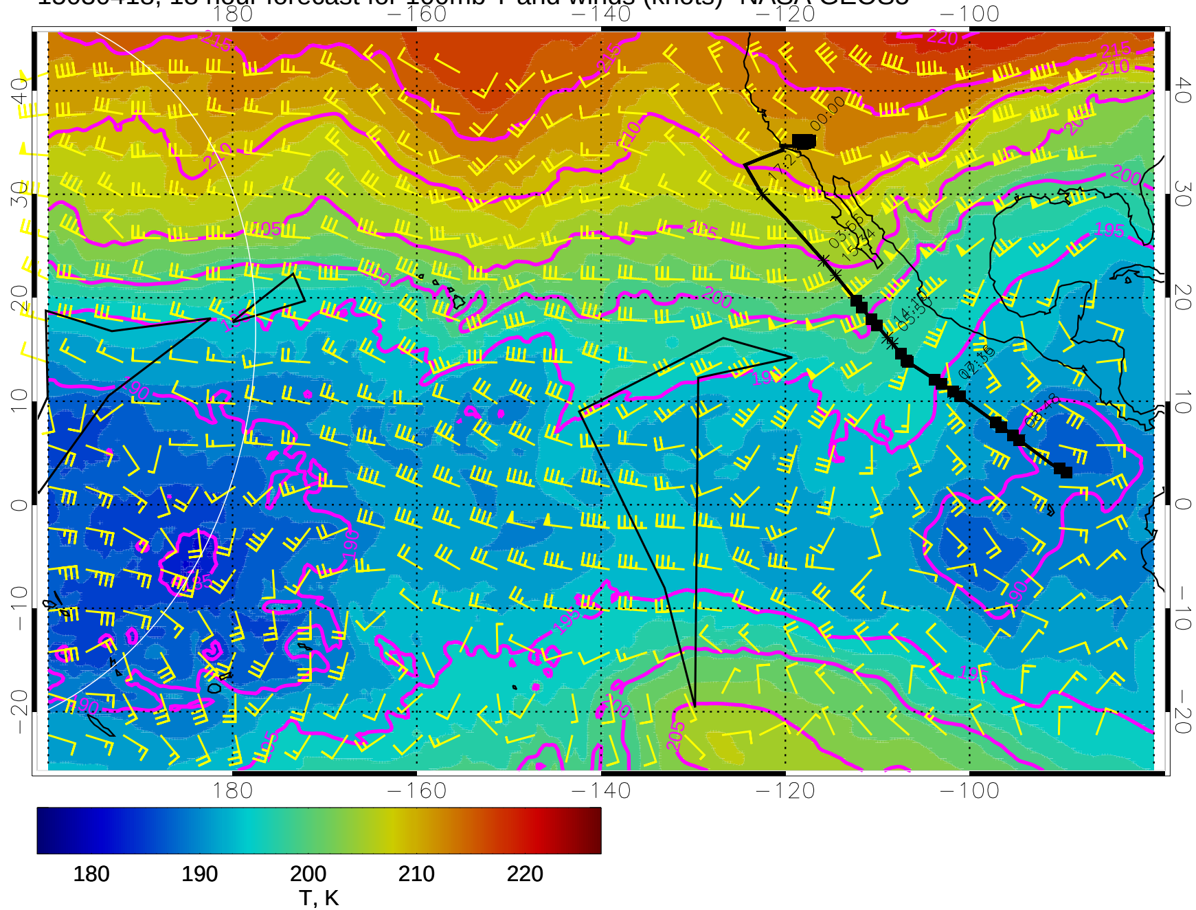
15030418, 18 hour forecast for 100mb T and winds (knots)- NASA GEOS5
