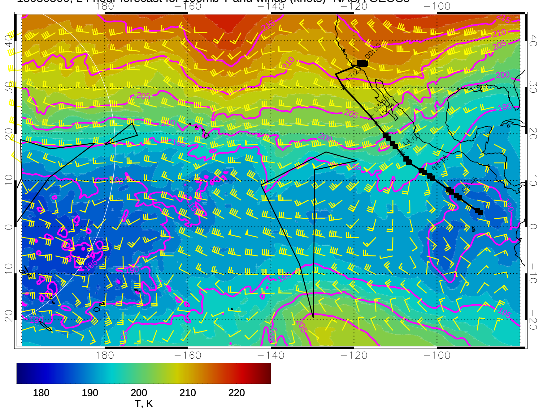
15030500, 24 hour forecast for 100mb T and winds (knots)- NASA GEOS5
