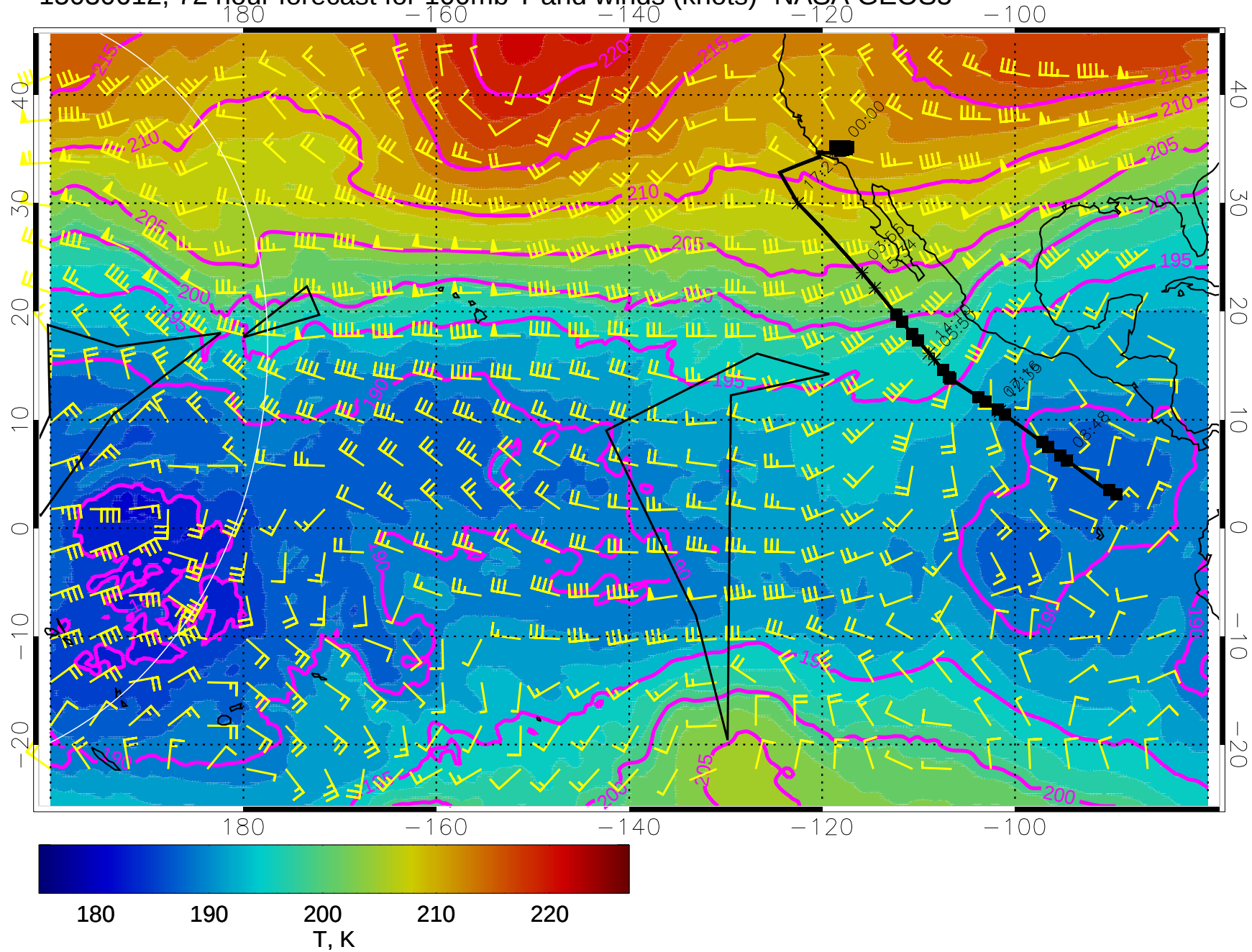
15030612, 72 hour forecast for 100mb T and winds (knots)- NASA GEOS5
