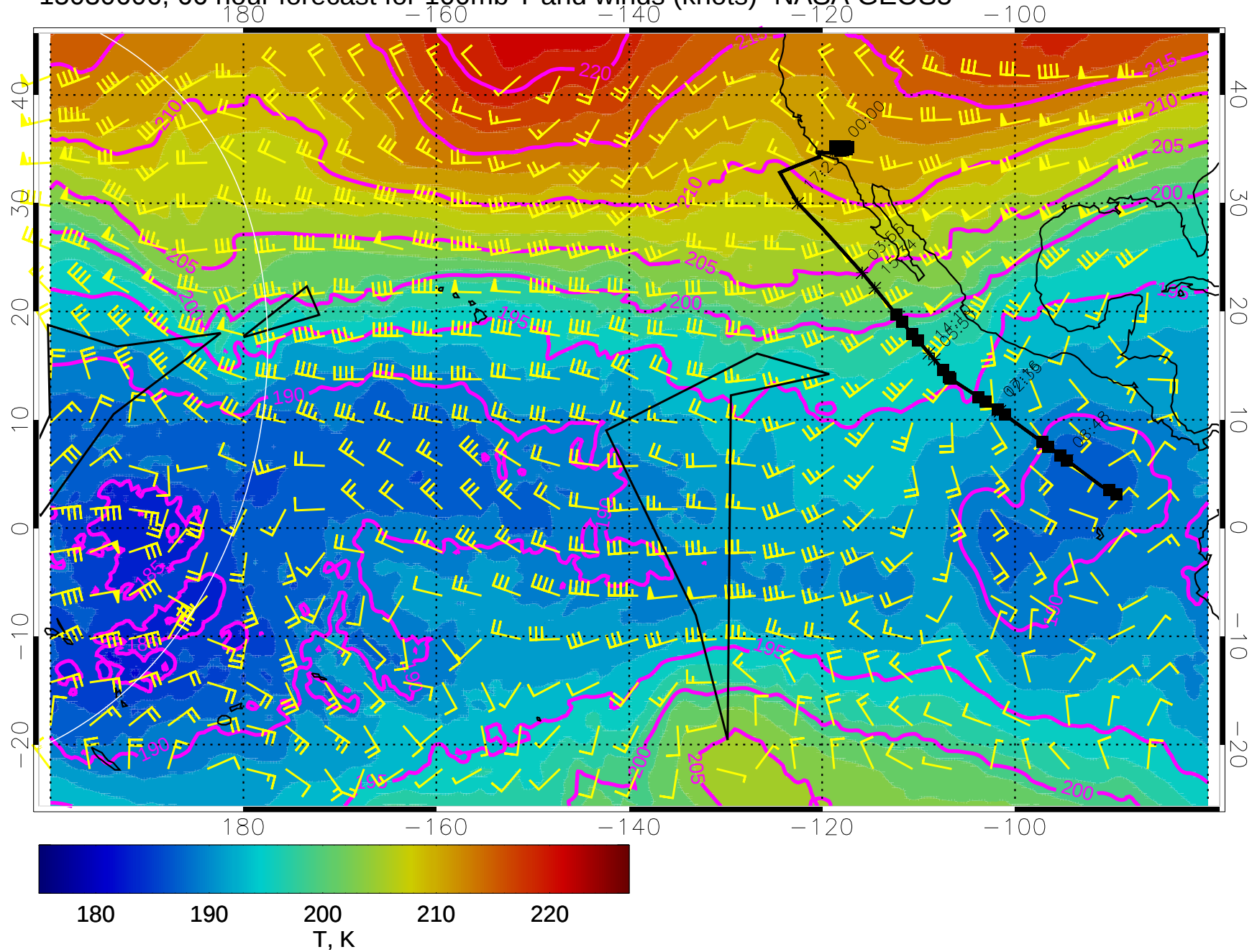
15030606, 66 hour forecast for 100mb T and winds (knots)- NASA GEOS5
