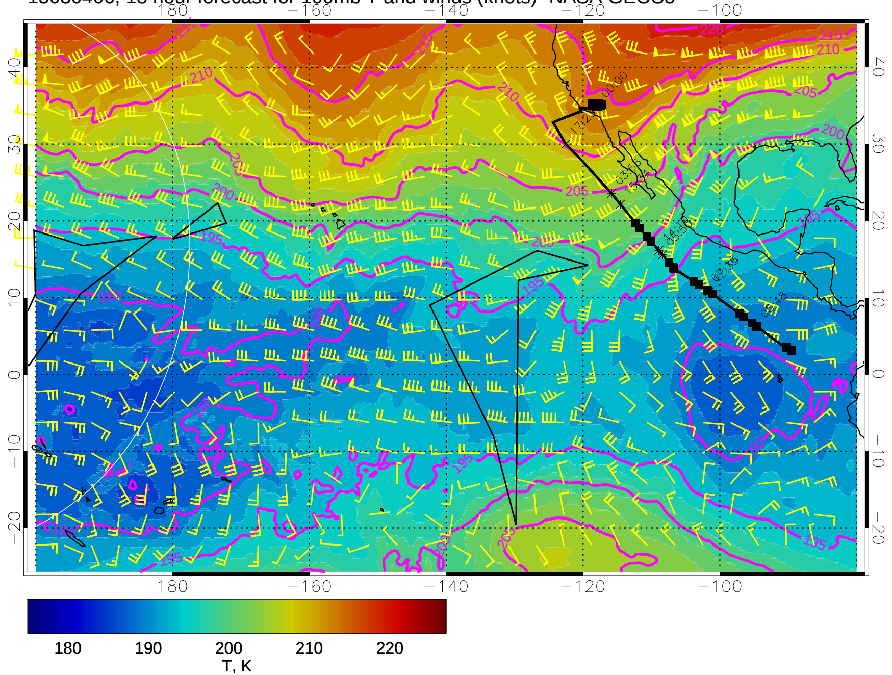
15030406, 18 hour forecast for 100mb T and winds (knots)- NASA GEOS5
