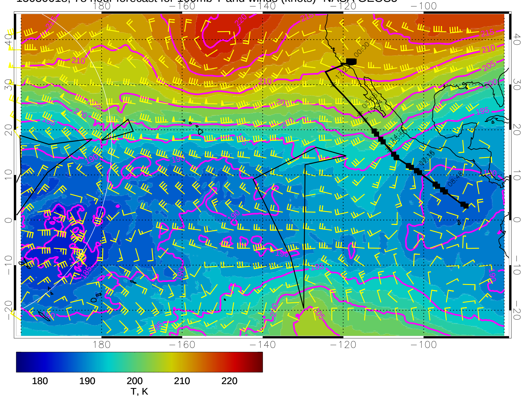
15030618, 78 hour forecast for 100mb T and winds (knots)- NASA GEOS5
