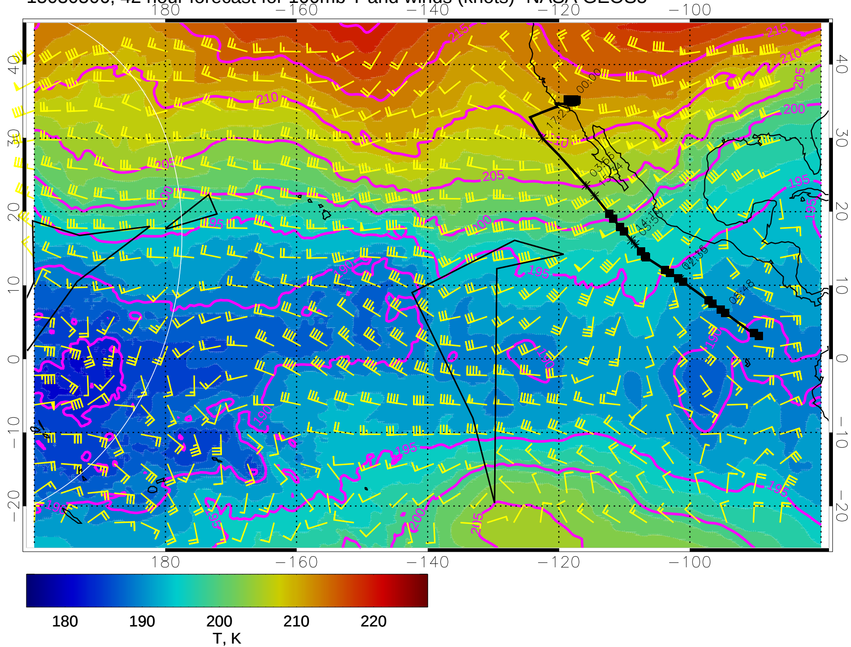
15030506, 42 hour forecast for 100mb T and winds (knots)- NASA GEOS5
