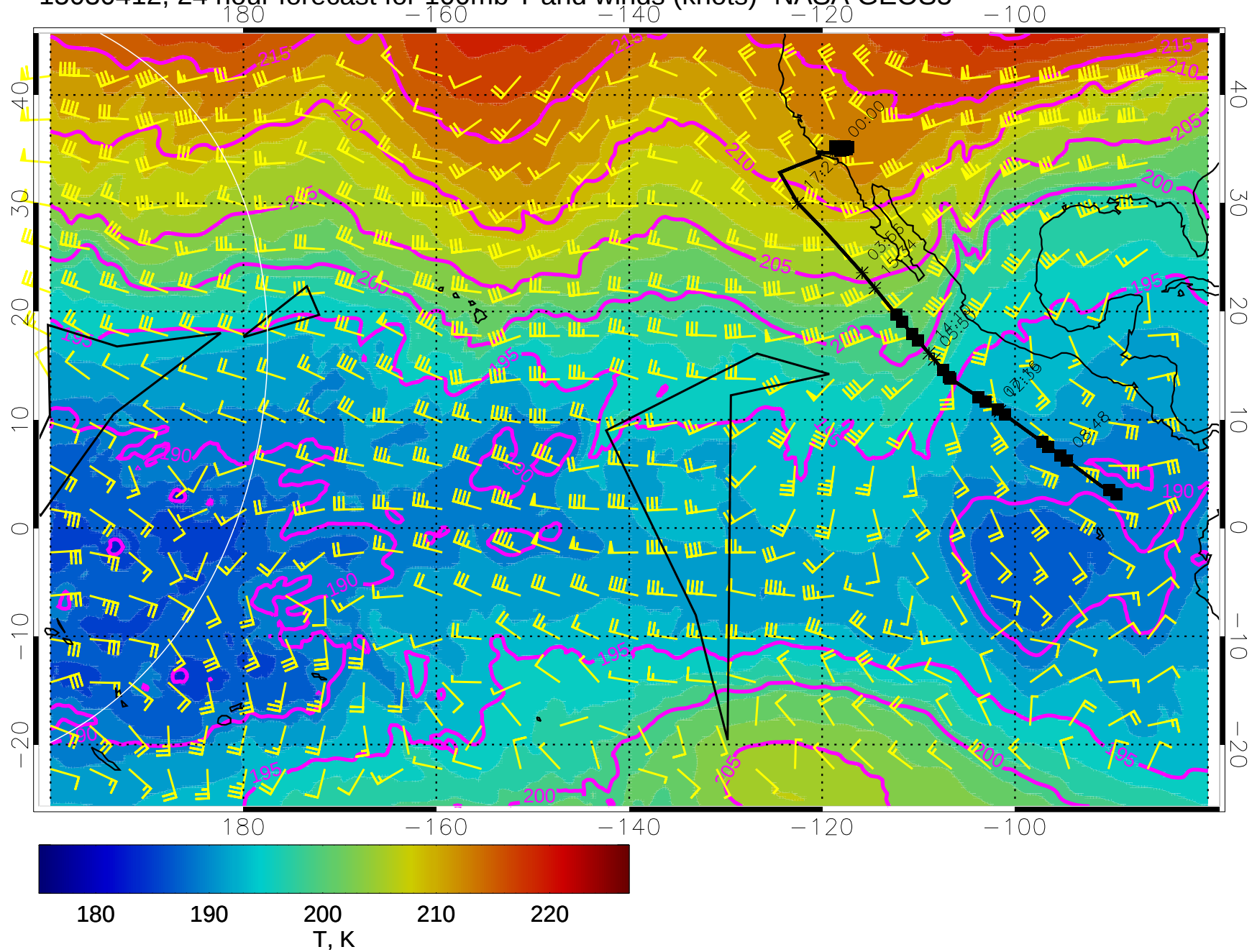
15030412, 24 hour forecast for 100mb T and winds (knots)- NASA GEOS5
