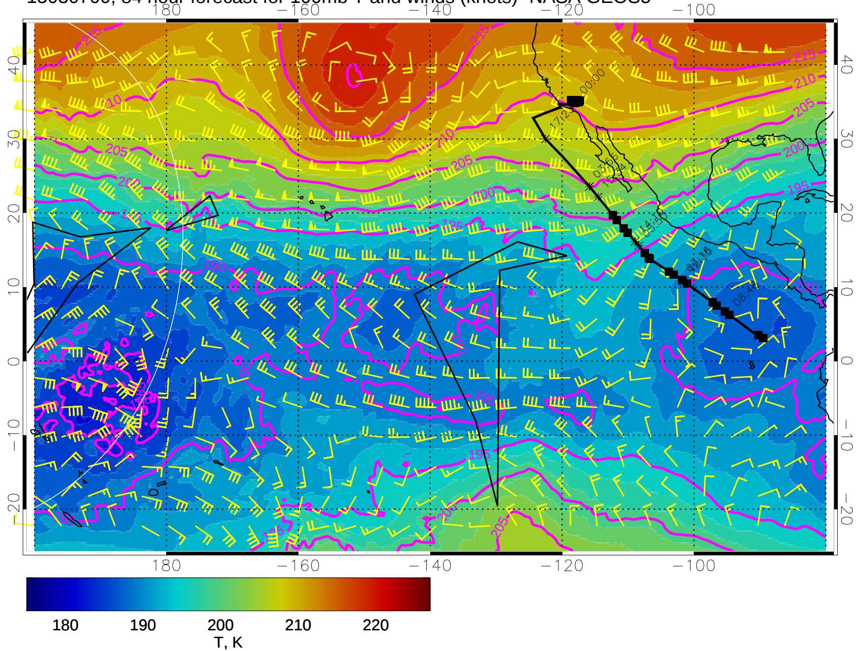
15030700, 84 hour forecast for 100mb T and winds (knots)- NASA GEOS5
