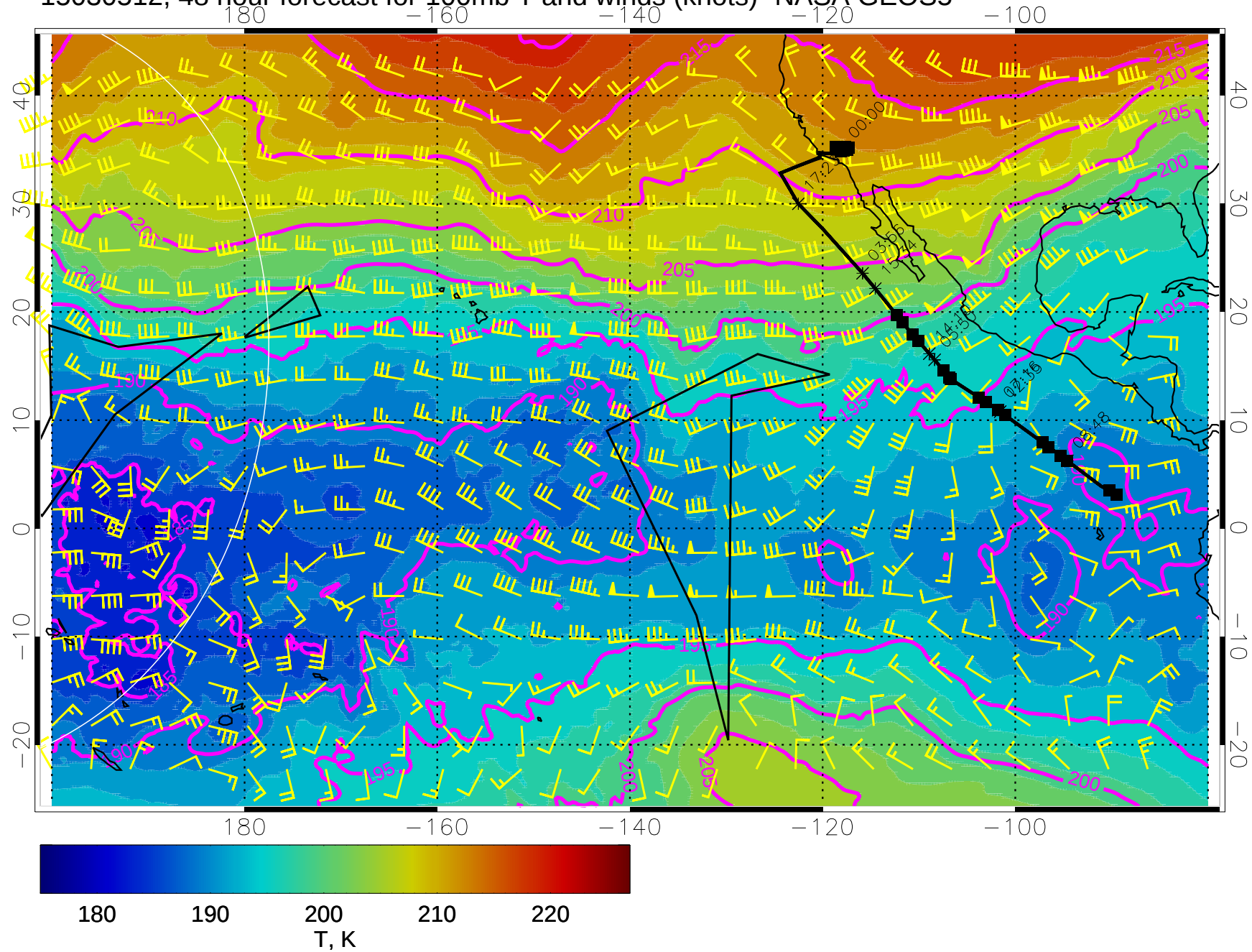
15030512, 48 hour forecast for 100mb T and winds (knots)- NASA GEOS5
