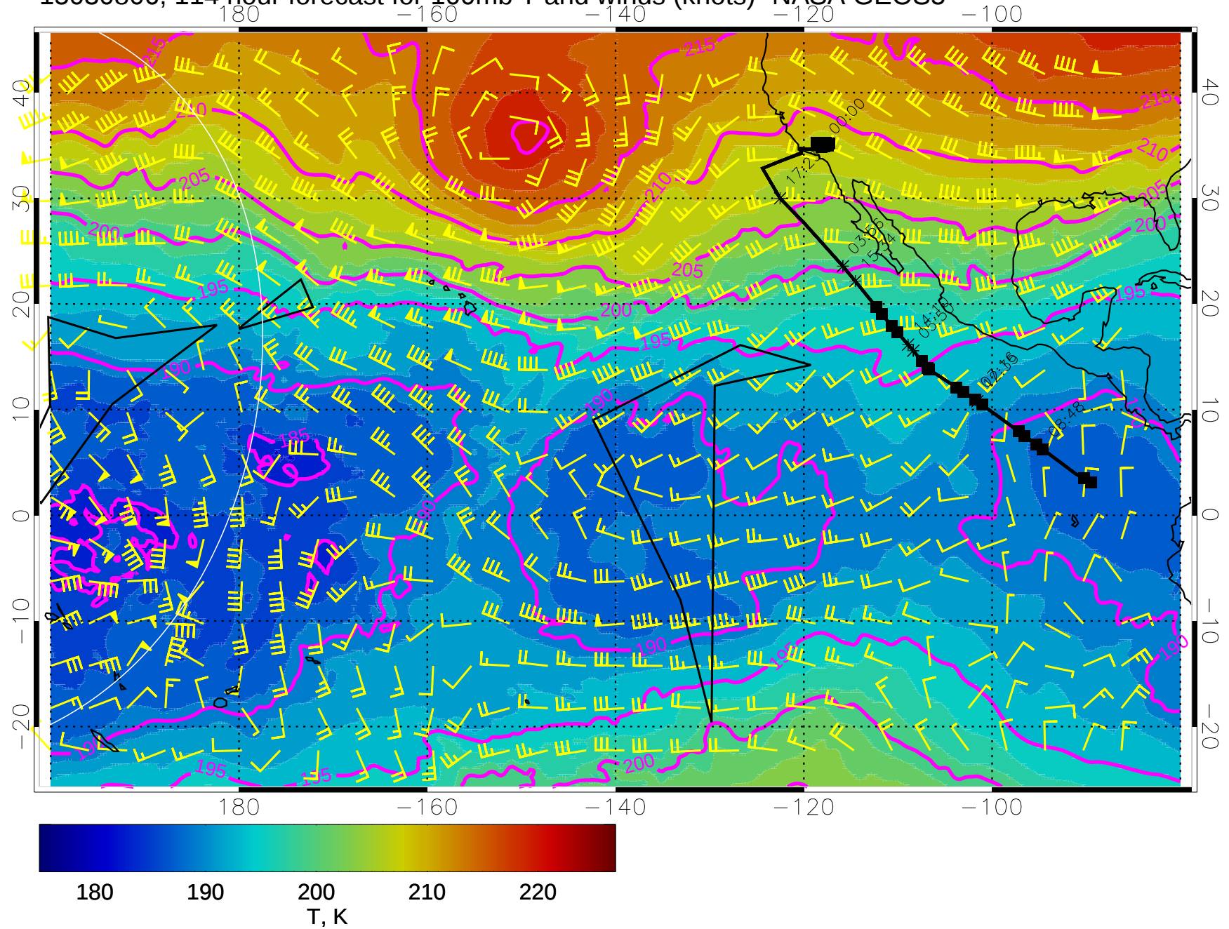
15030806, 114 hour forecast for 100mb T and winds (knots)- NASA GEOS5
