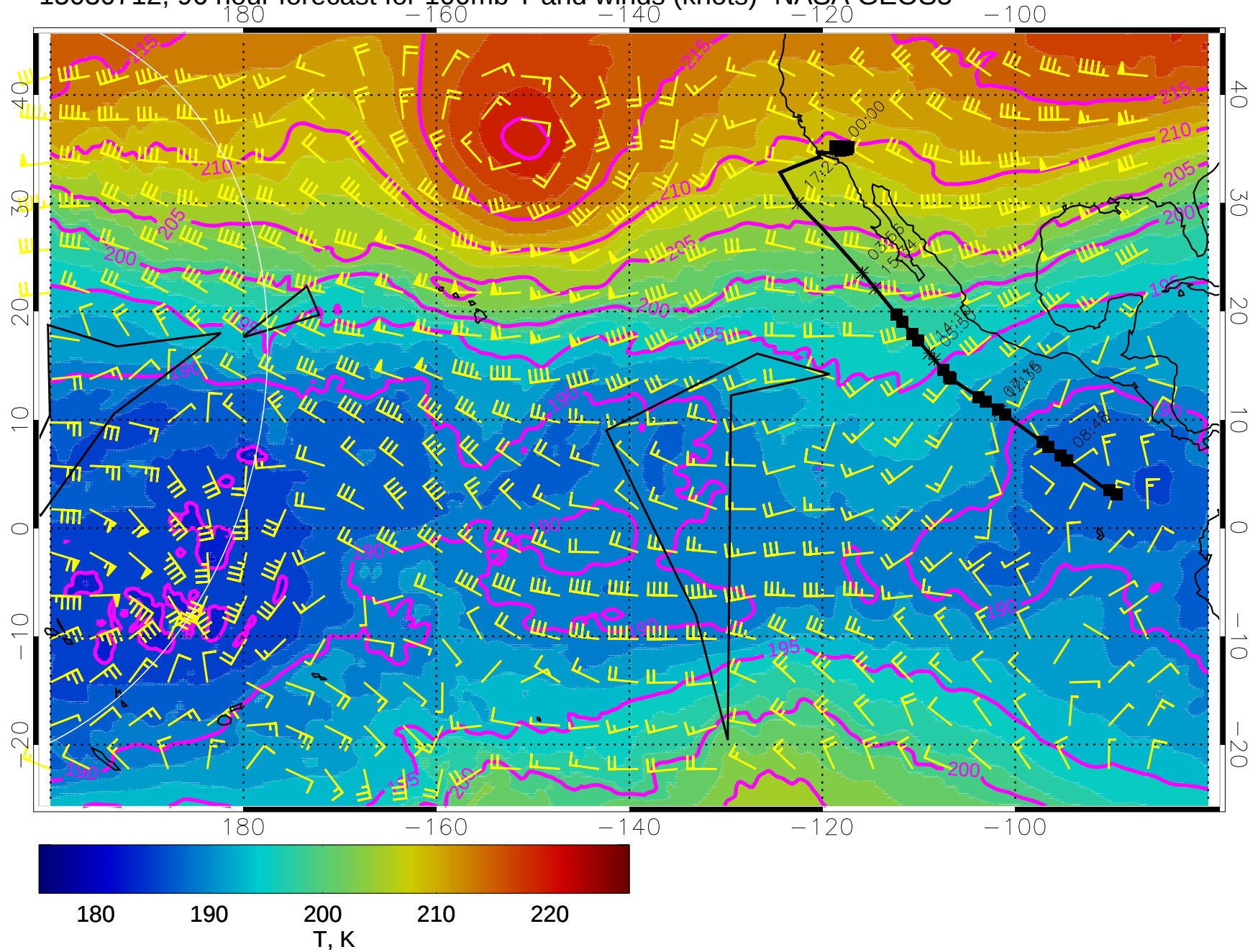
15030712, 96 hour forecast for 100mb T and winds (knots)- NASA GEOS5
