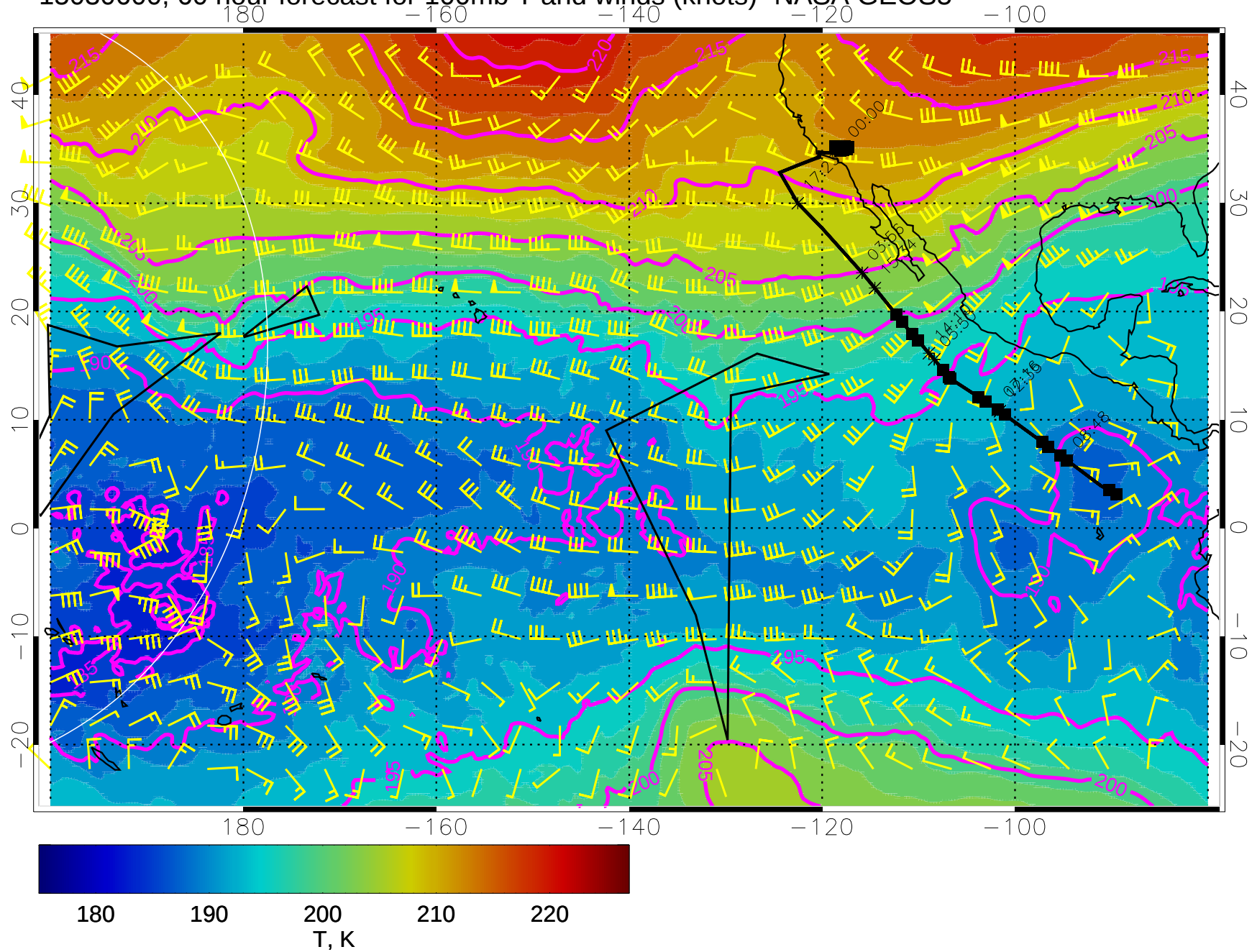
15030600, 60 hour forecast for 100mb T and winds (knots)- NASA GEOS5
