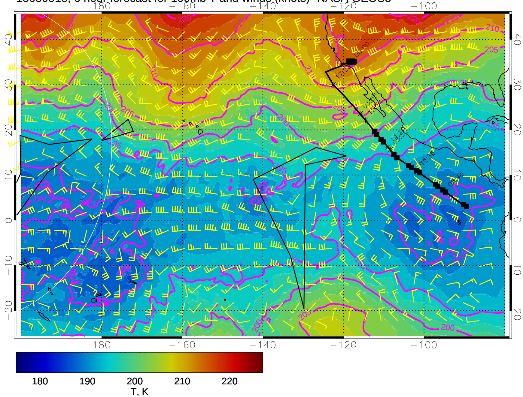
15030318, 6 hour forecast for 100mb T and winds (knots)- NASA GEOS5
