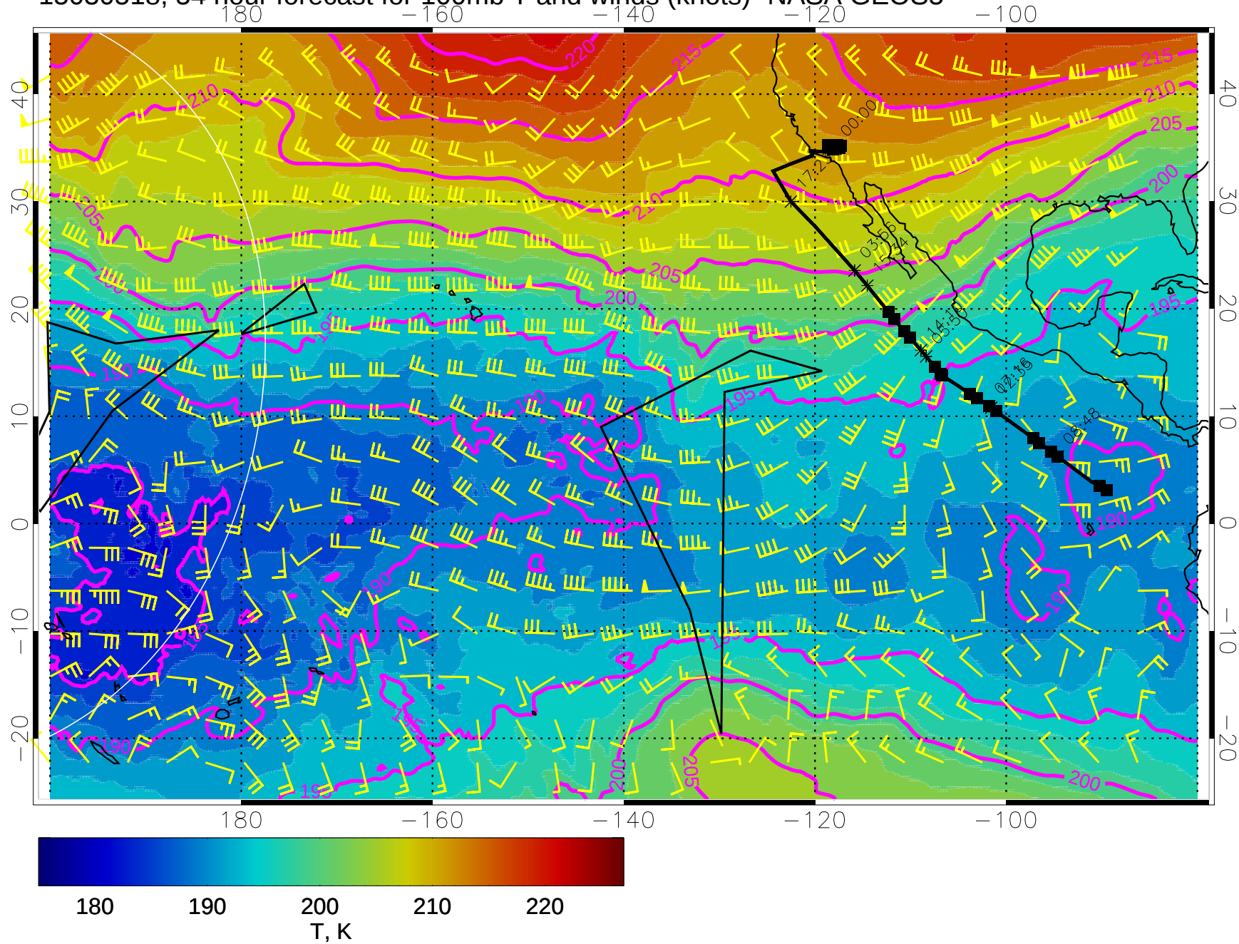
15030518, 54 hour forecast for 100mb T and winds (knots)- NASA GEOS5
