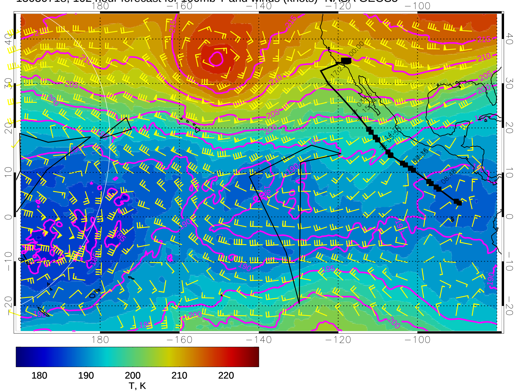
15030718, 102 hour forecast for 100mb T and winds (knots)- NASA GEOS5
