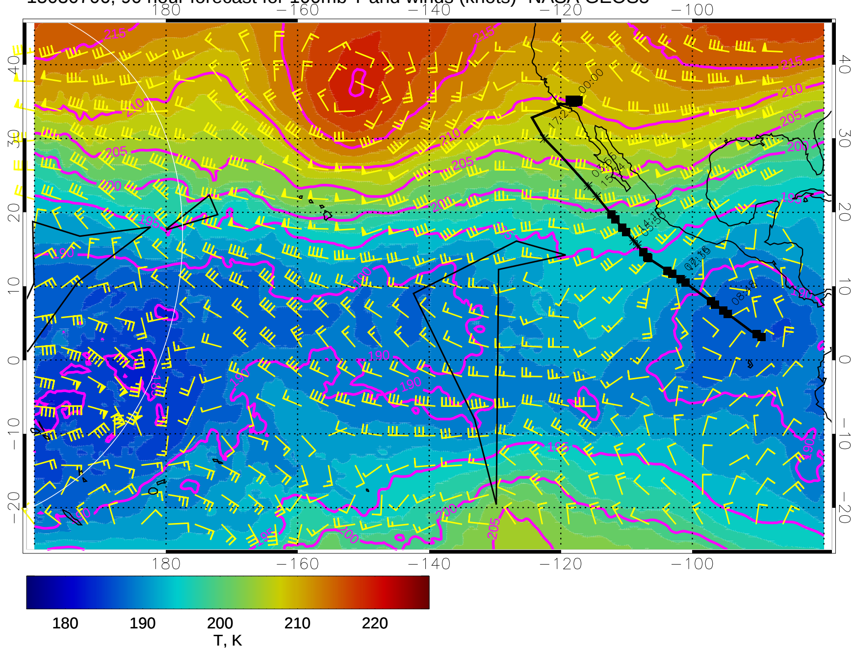
15030706, 90 hour forecast for 100mb T and winds (knots)- NASA GEOS5
