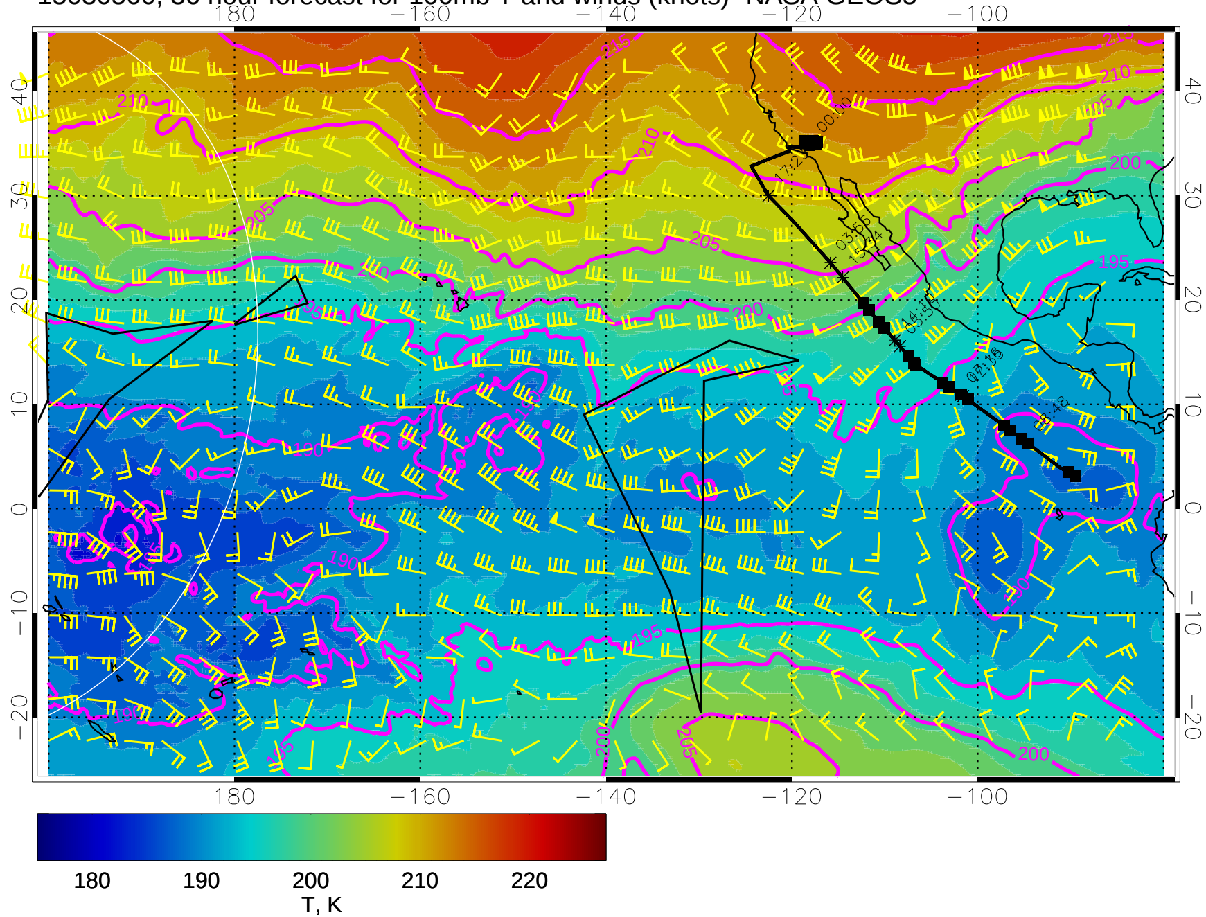
15030500, 36 hour forecast for 100mb T and winds (knots)- NASA GEOS5
