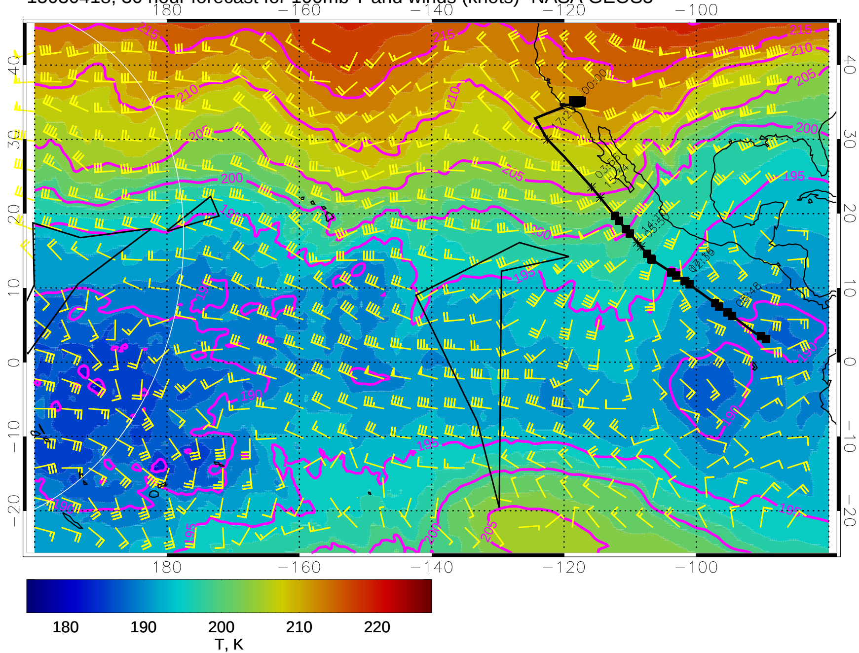
15030418, 30 hour forecast for 100mb T and winds (knots)- NASA GEOS5
