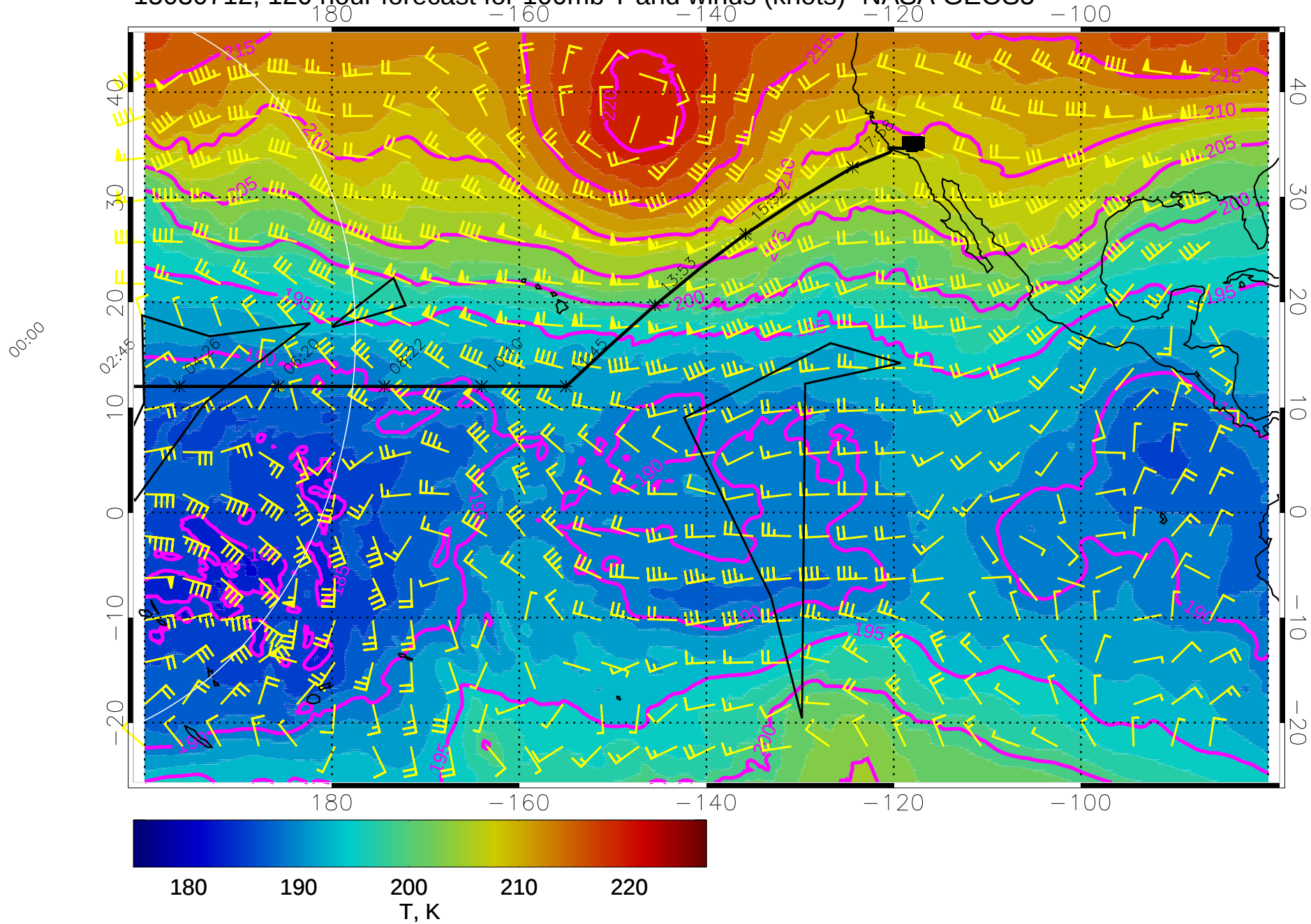
15030712, 120 hour forecast for 100mb T and winds (knots)- NASA GEOS5
