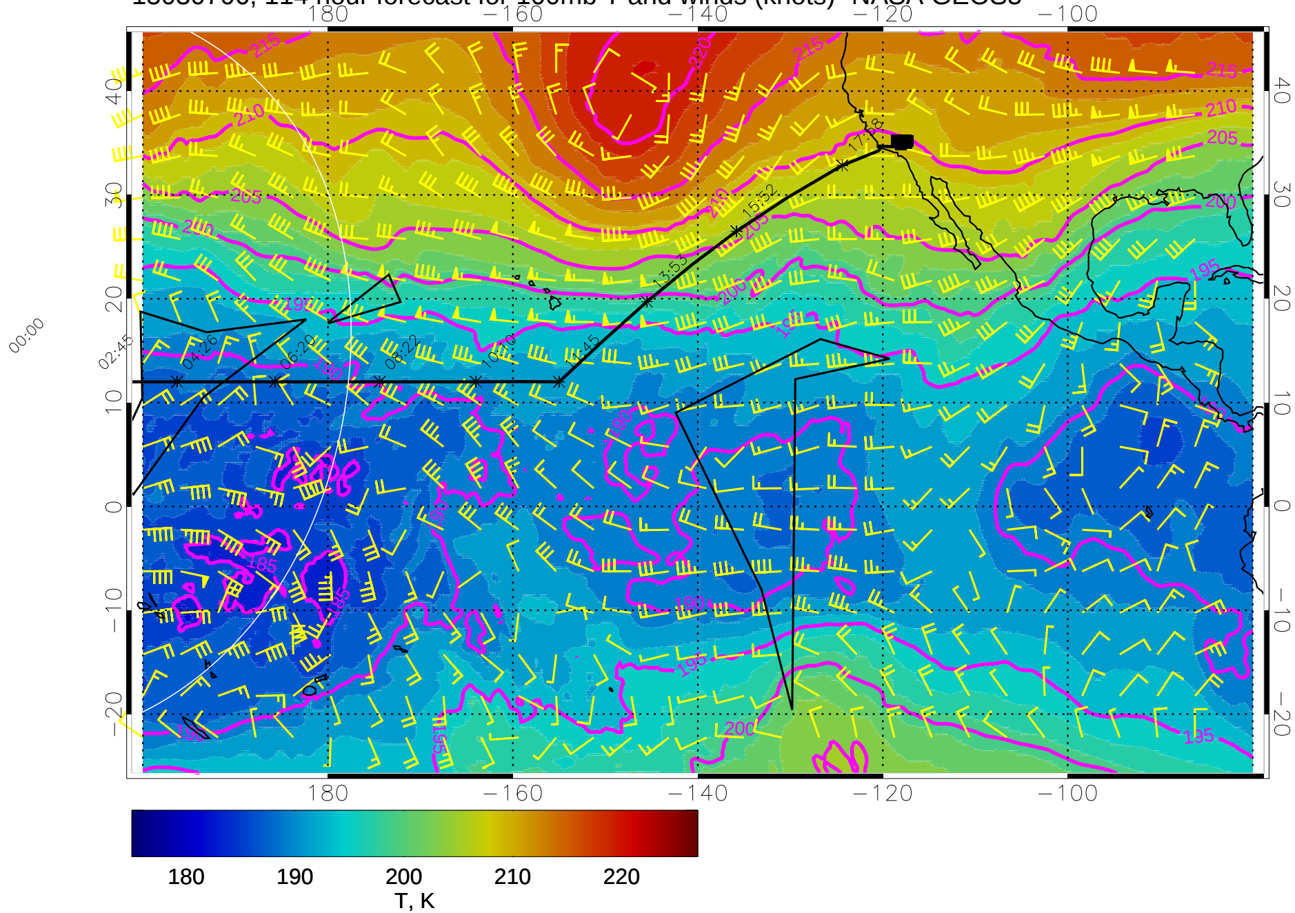
15030706, 114 hour forecast for 100mb T and winds (knots)- NASA GEOS5
