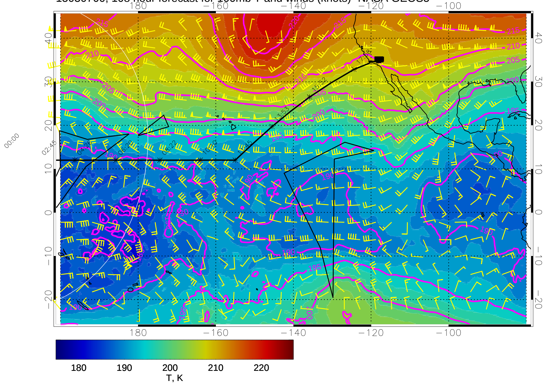
15030700, 108 hour forecast for 100mb T and winds (knots)- NASA GEOS5
