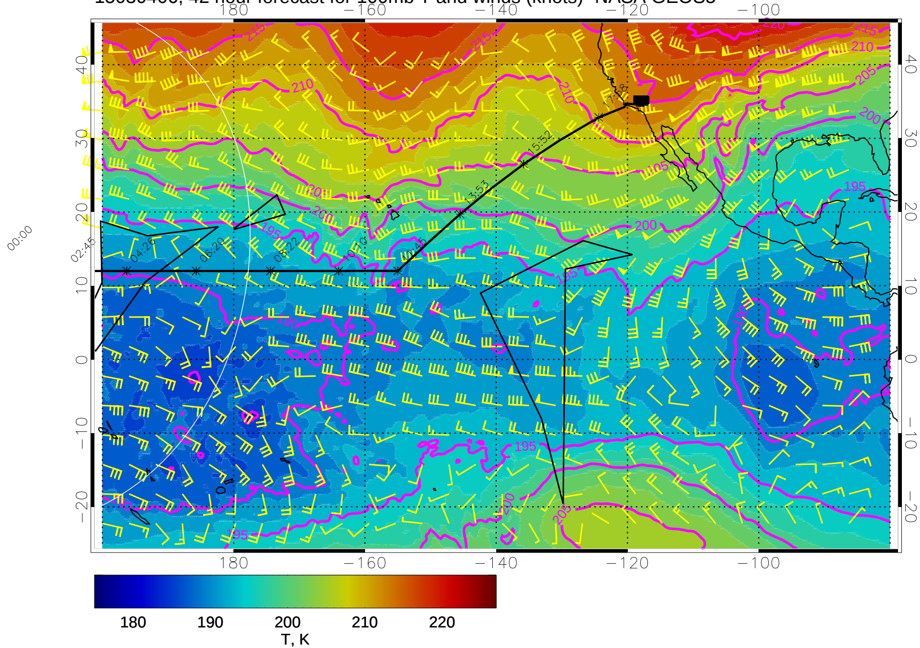
15030406, 42 hour forecast for 100mb T and winds (knots)- NASA GEOS5
