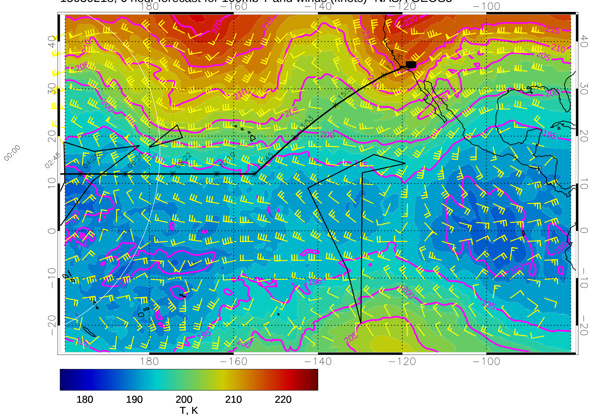
15030218, 6 hour forecast for 100mb T and winds (knots)- NASA GEOS5
