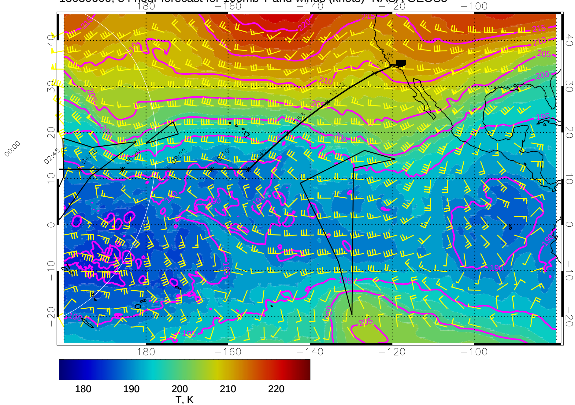
15030600, 84 hour forecast for 100mb T and winds (knots)- NASA GEOS5
