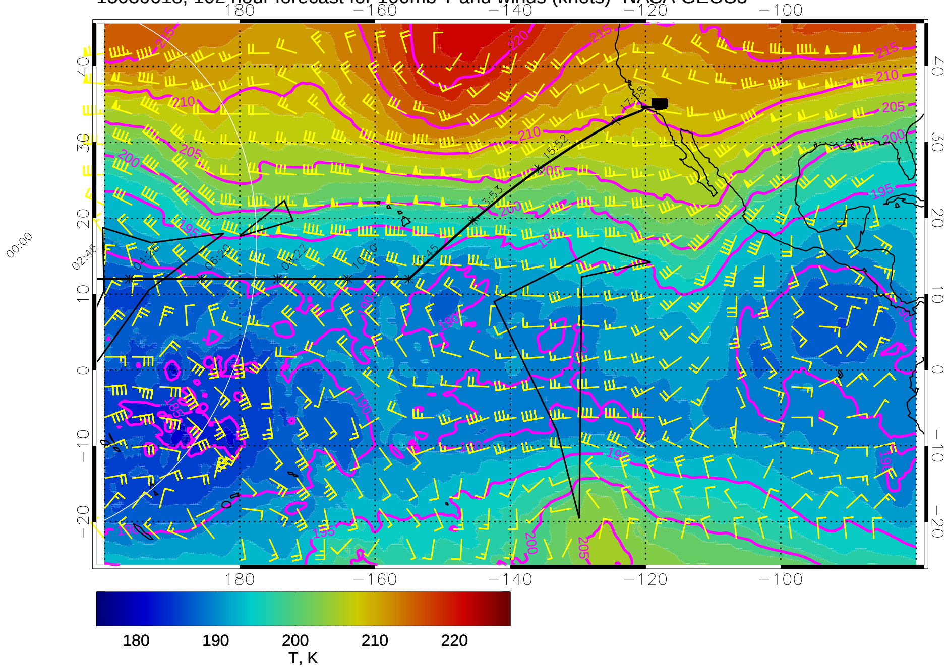
15030618, 102 hour forecast for 100mb T and winds (knots)- NASA GEOS5
