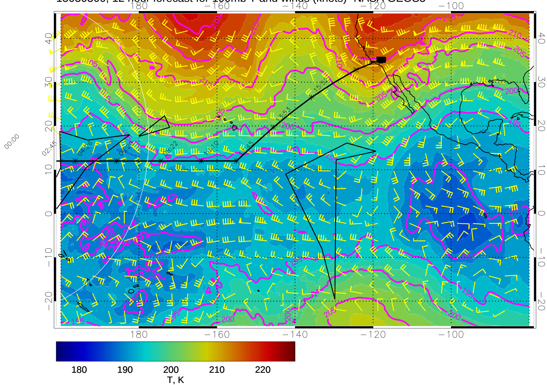
15030300, 12 hour forecast for 100mb T and winds (knots)- NASA GEOS5
