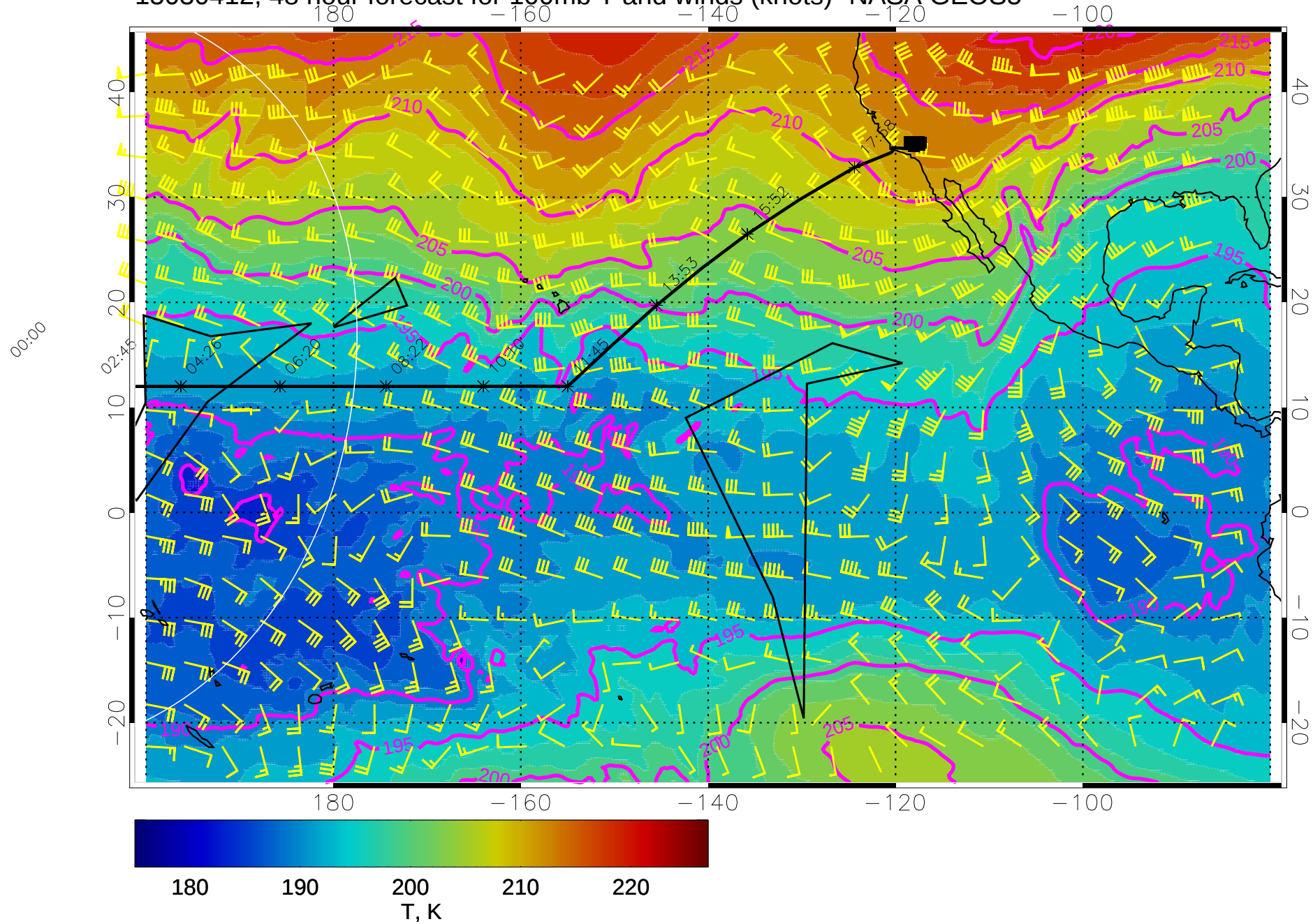
15030412, 48 hour forecast for 100mb T and winds (knots)- NASA GEOS5
