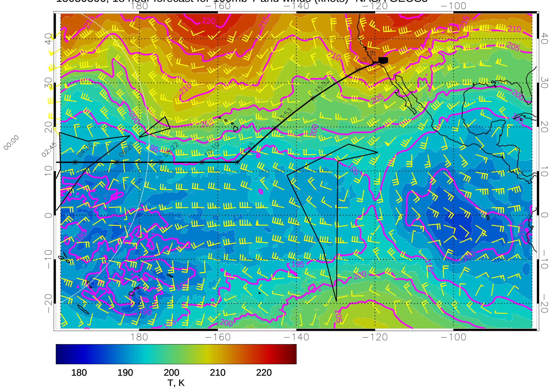
15030306, 18 hour forecast for 100mb T and winds (knots)- NASA GEOS5
