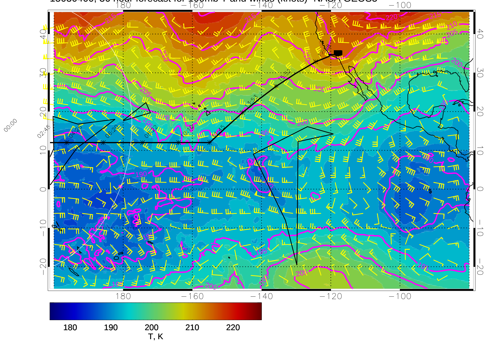
15030400, 36 hour forecast for 100mb T and winds (knots)- NASA GEOS5
