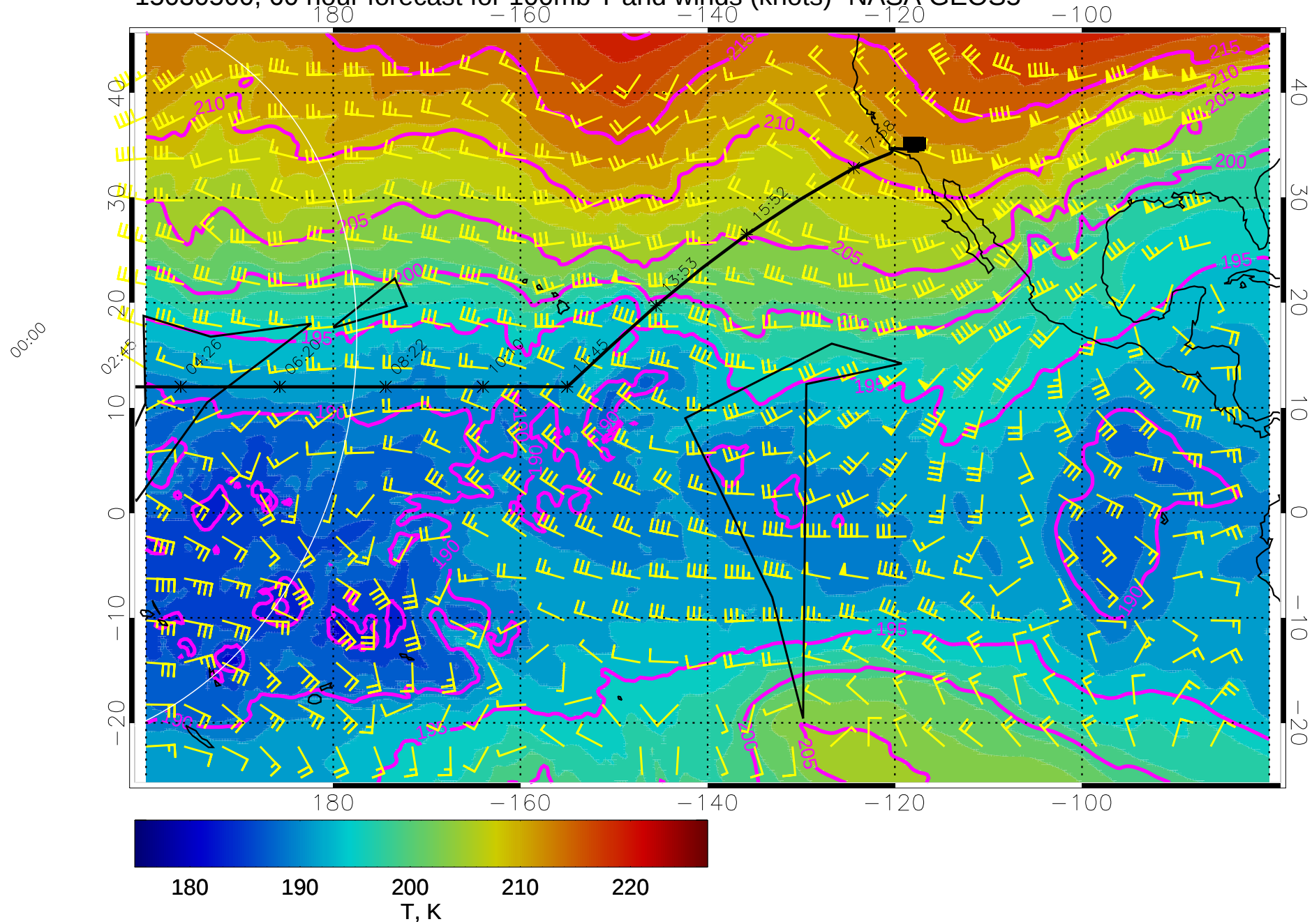
15030500, 60 hour forecast for 100mb T and winds (knots)- NASA GEOS5
