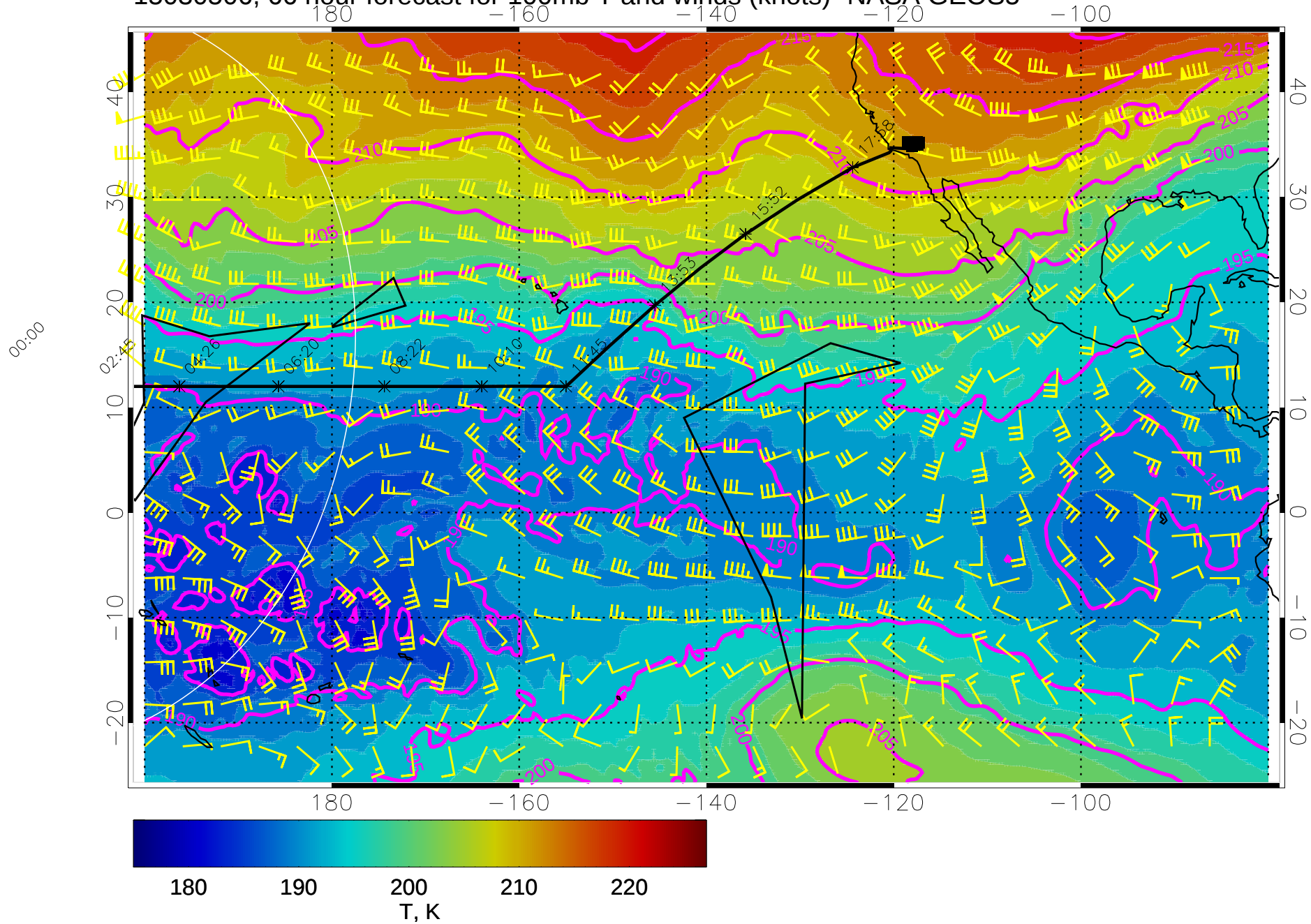
15030506, 66 hour forecast for 100mb T and winds (knots)- NASA GEOS5
