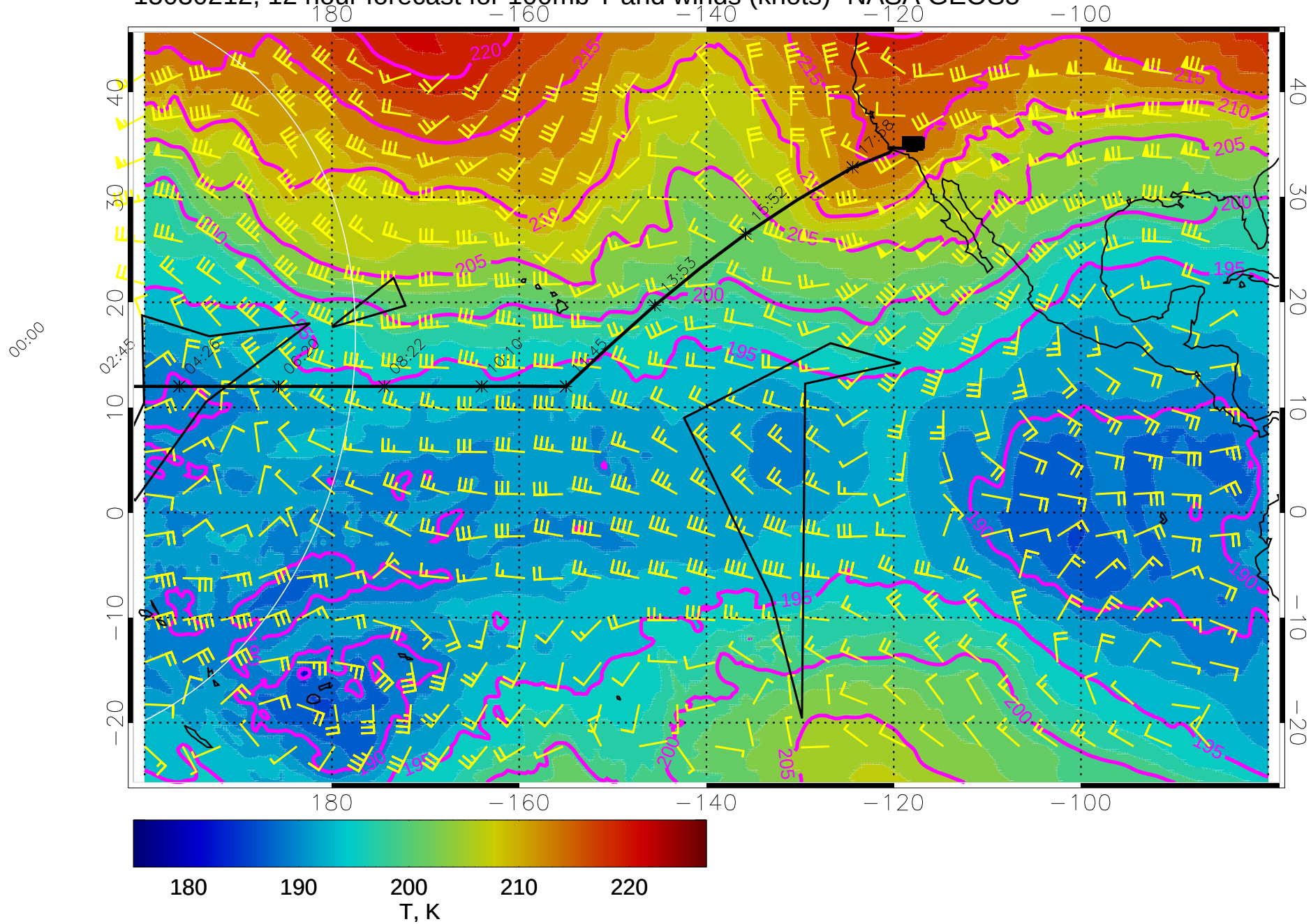
15030212, 12 hour forecast for 100mb T and winds (knots)- NASA GEOS5
