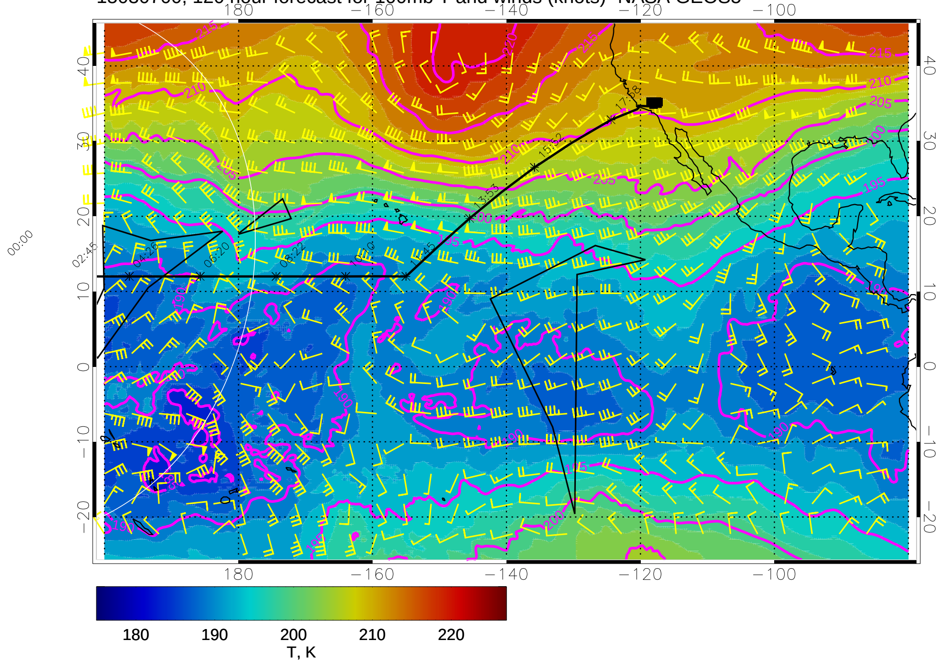
15030700, 120 hour forecast for 100mb T and winds (knots)- NASA GEOS5
