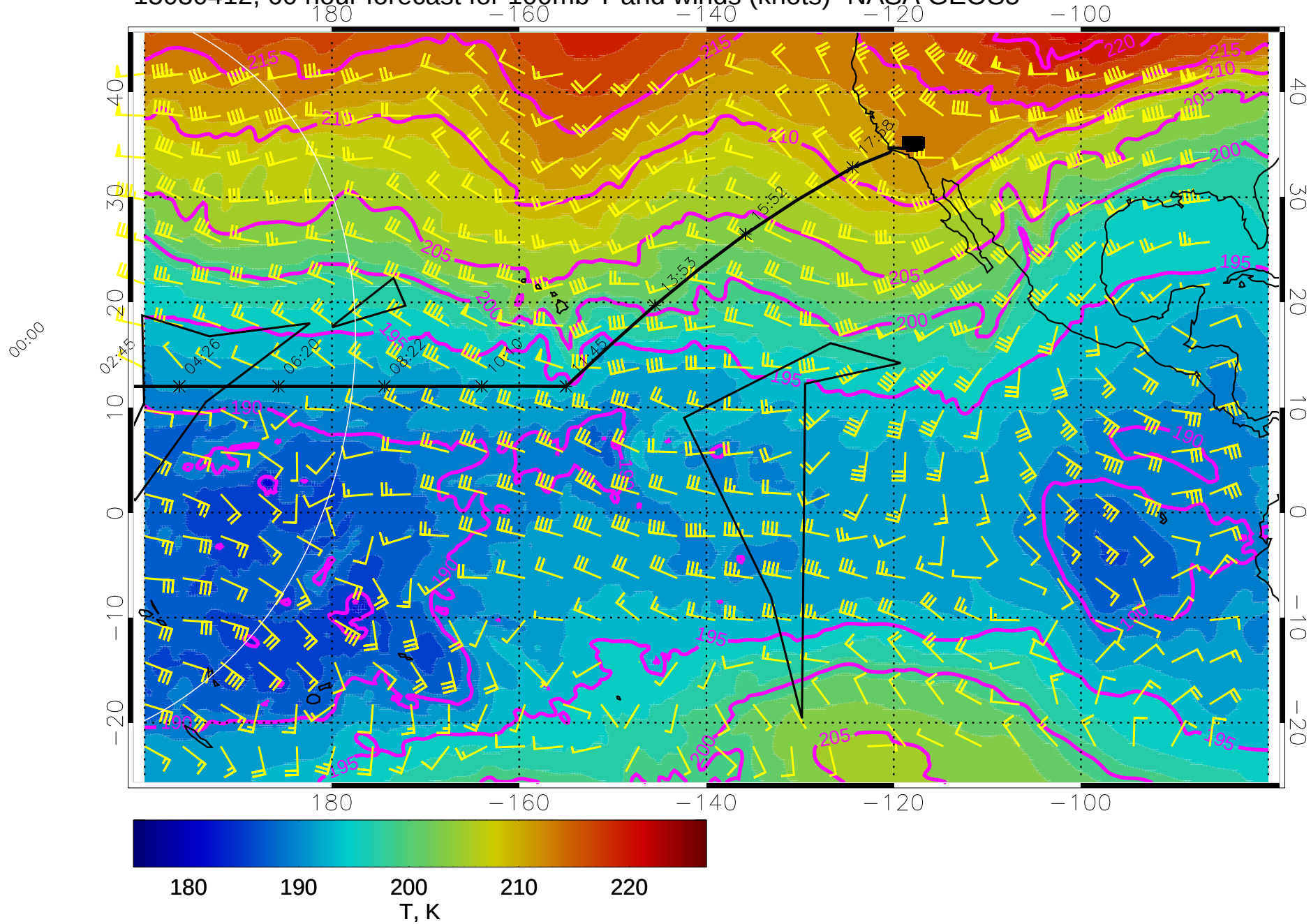
15030412, 60 hour forecast for 100mb T and winds (knots)- NASA GEOS5
