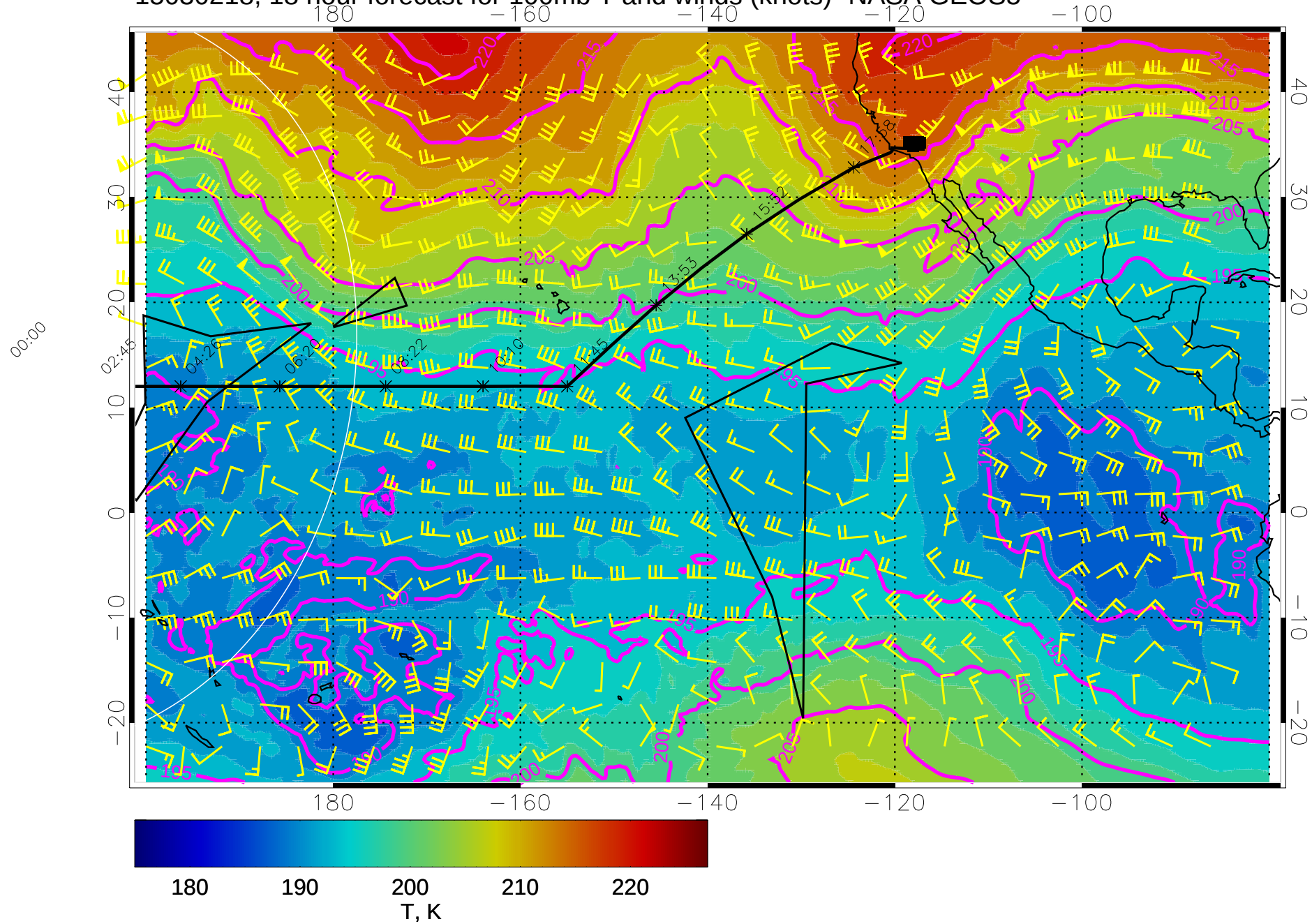
15030218, 18 hour forecast for 100mb T and winds (knots)- NASA GEOS5
