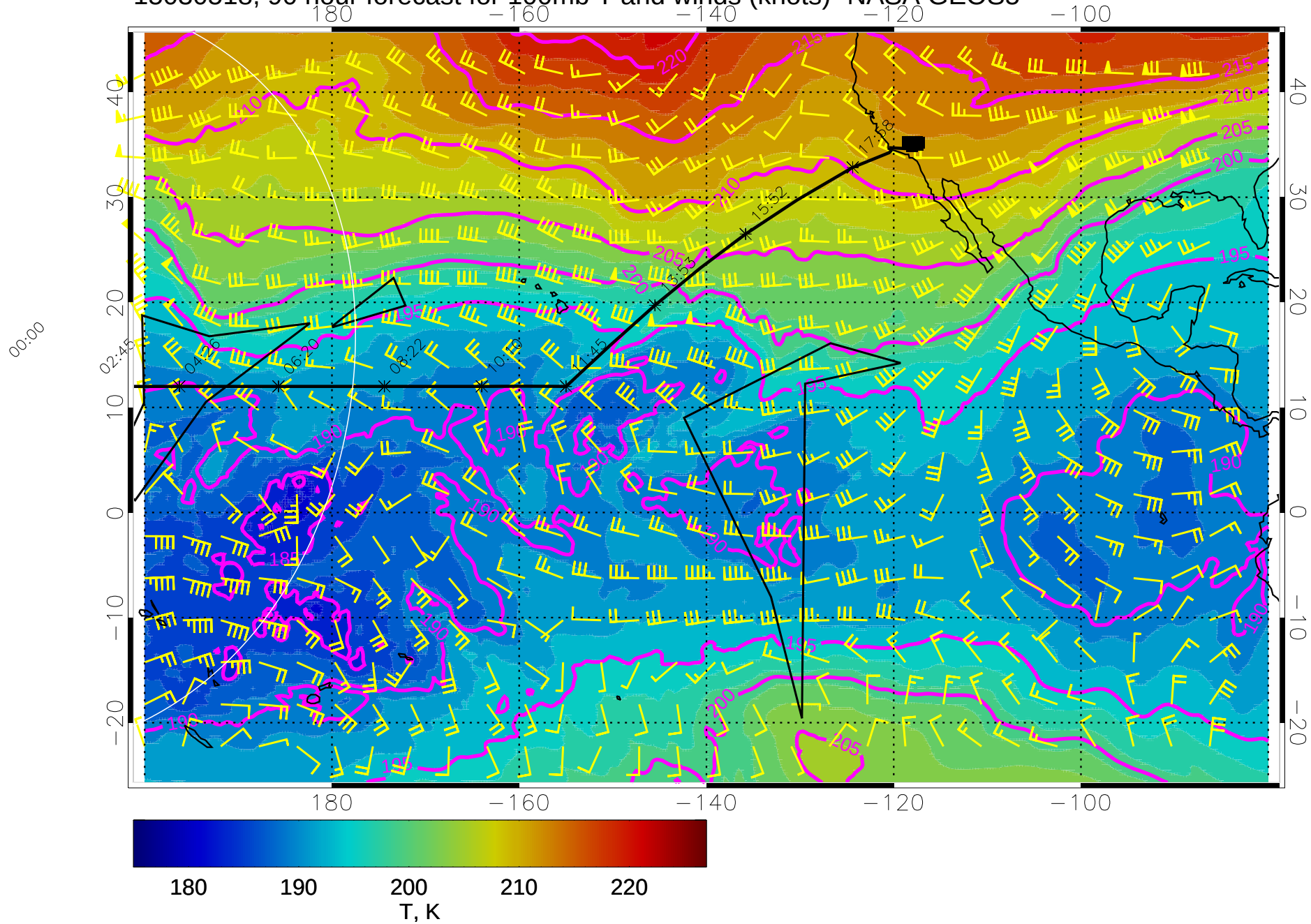
15030518, 90 hour forecast for 100mb T and winds (knots)- NASA GEOS5
