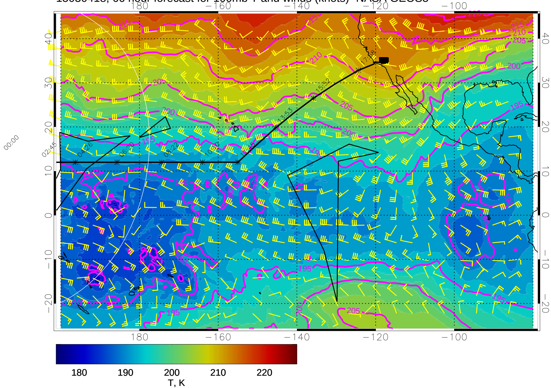
15030418, 66 hour forecast for 100mb T and winds (knots)- NASA GEOS5
