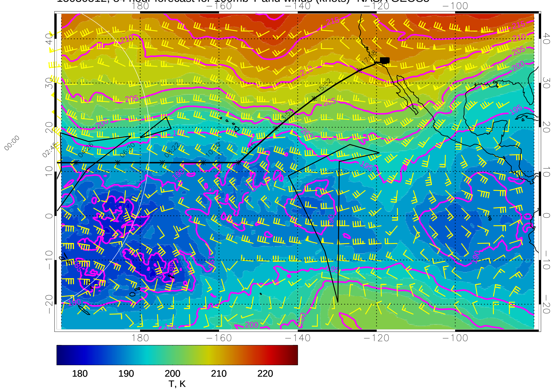
15030512, 84 hour forecast for 100mb T and winds (knots)- NASA GEOS5
