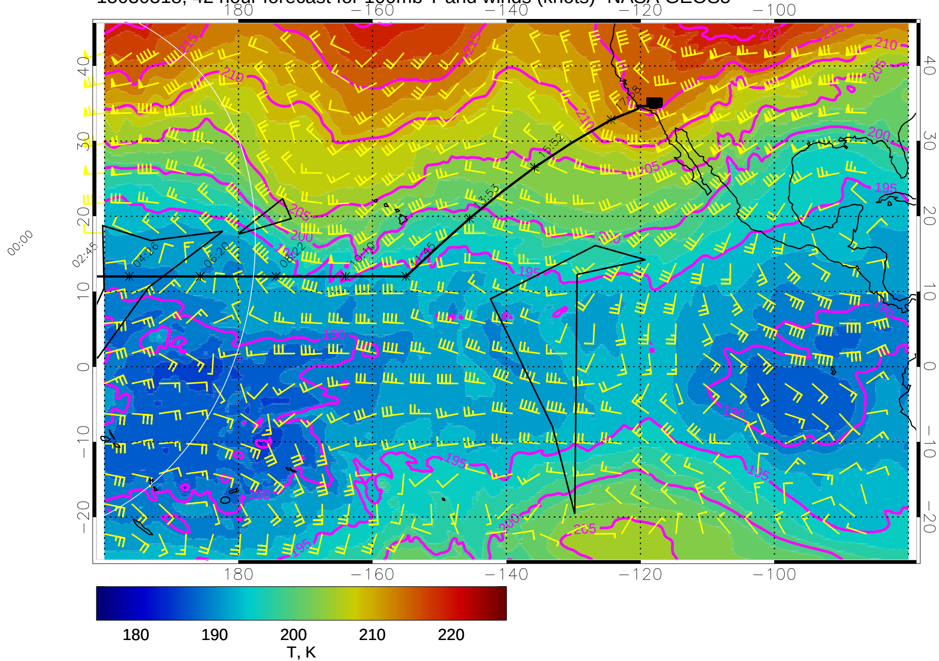
15030318, 42 hour forecast for 100mb T and winds (knots)- NASA GEOS5
