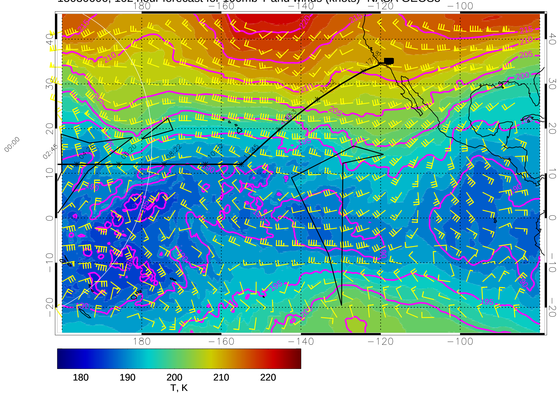
15030606, 102 hour forecast for 100mb T and winds (knots)- NASA GEOS5
