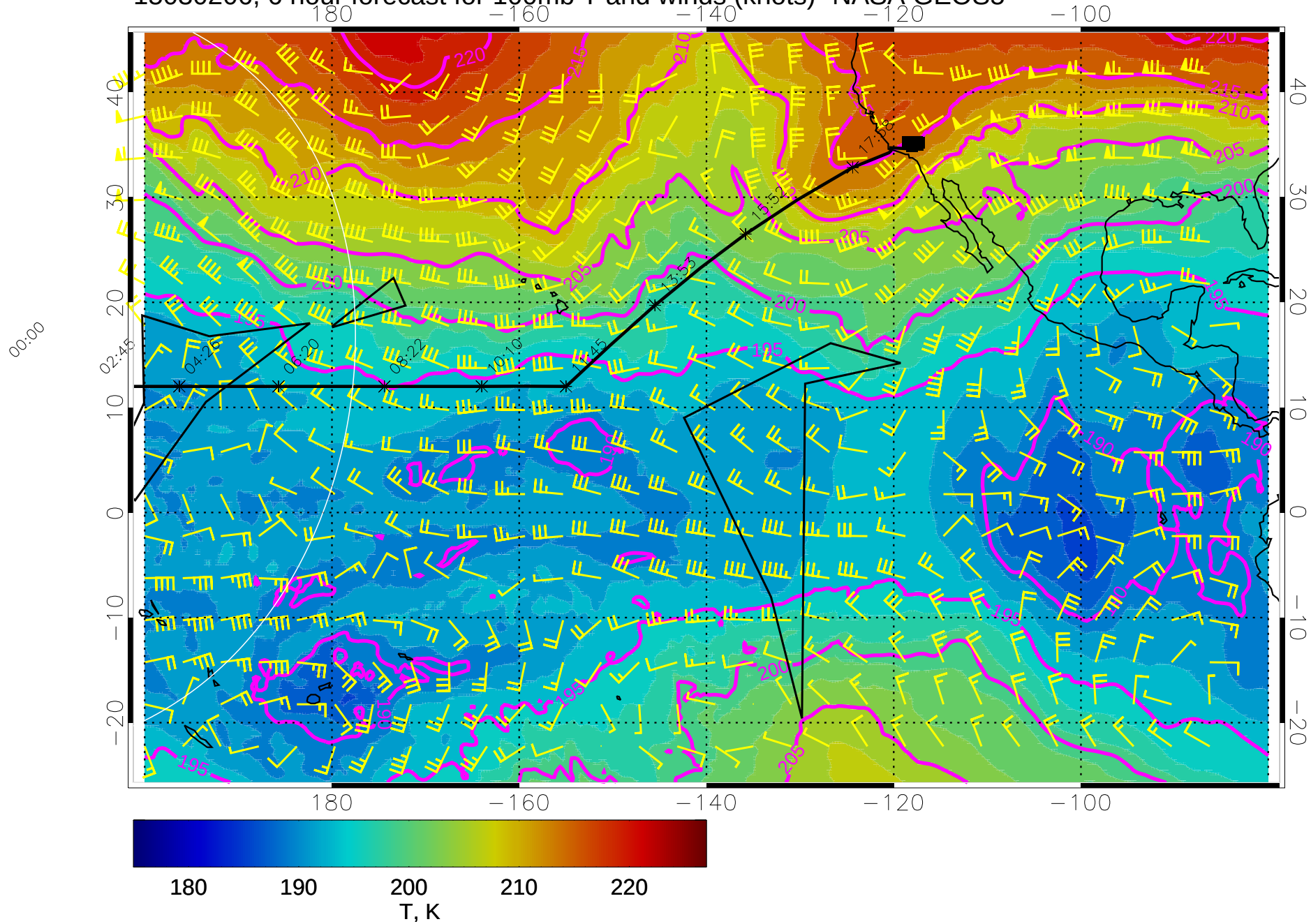
15030206, 6 hour forecast for 100mb T and winds (knots)- NASA GEOS5
