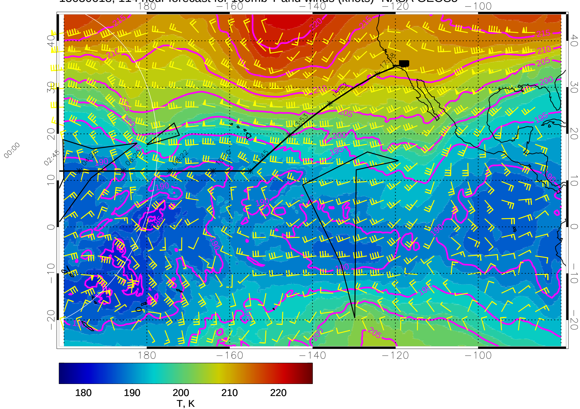
15030618, 114 hour forecast for 100mb T and winds (knots)- NASA GEOS5
