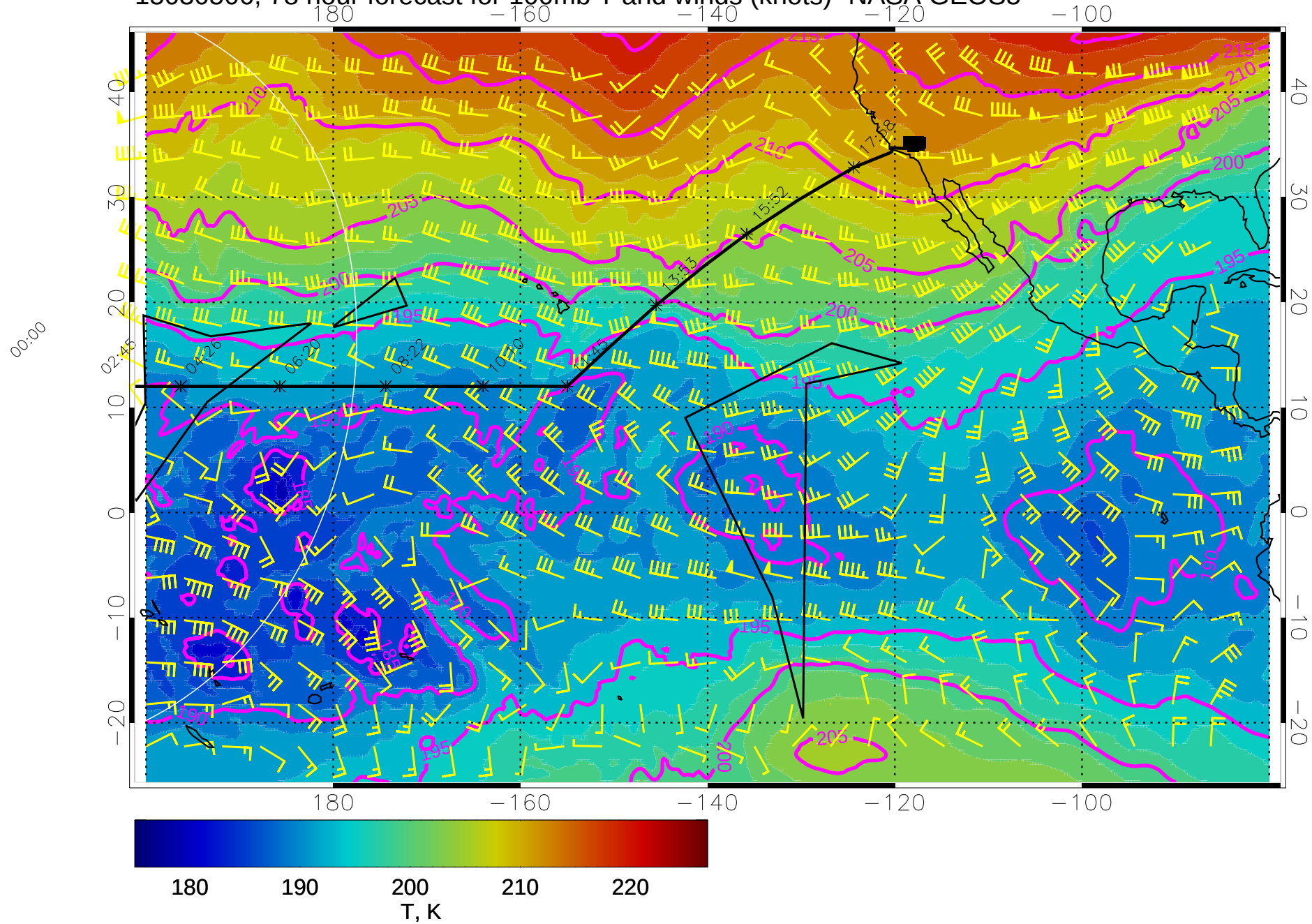
15030506, 78 hour forecast for 100mb T and winds (knots)- NASA GEOS5
