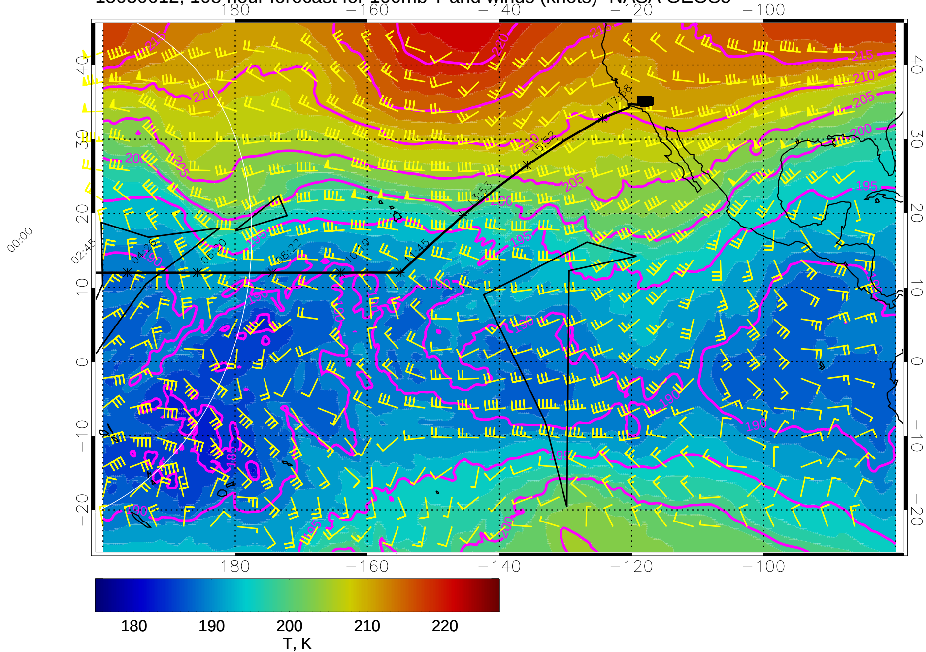
15030612, 108 hour forecast for 100mb T and winds (knots)- NASA GEOS5
