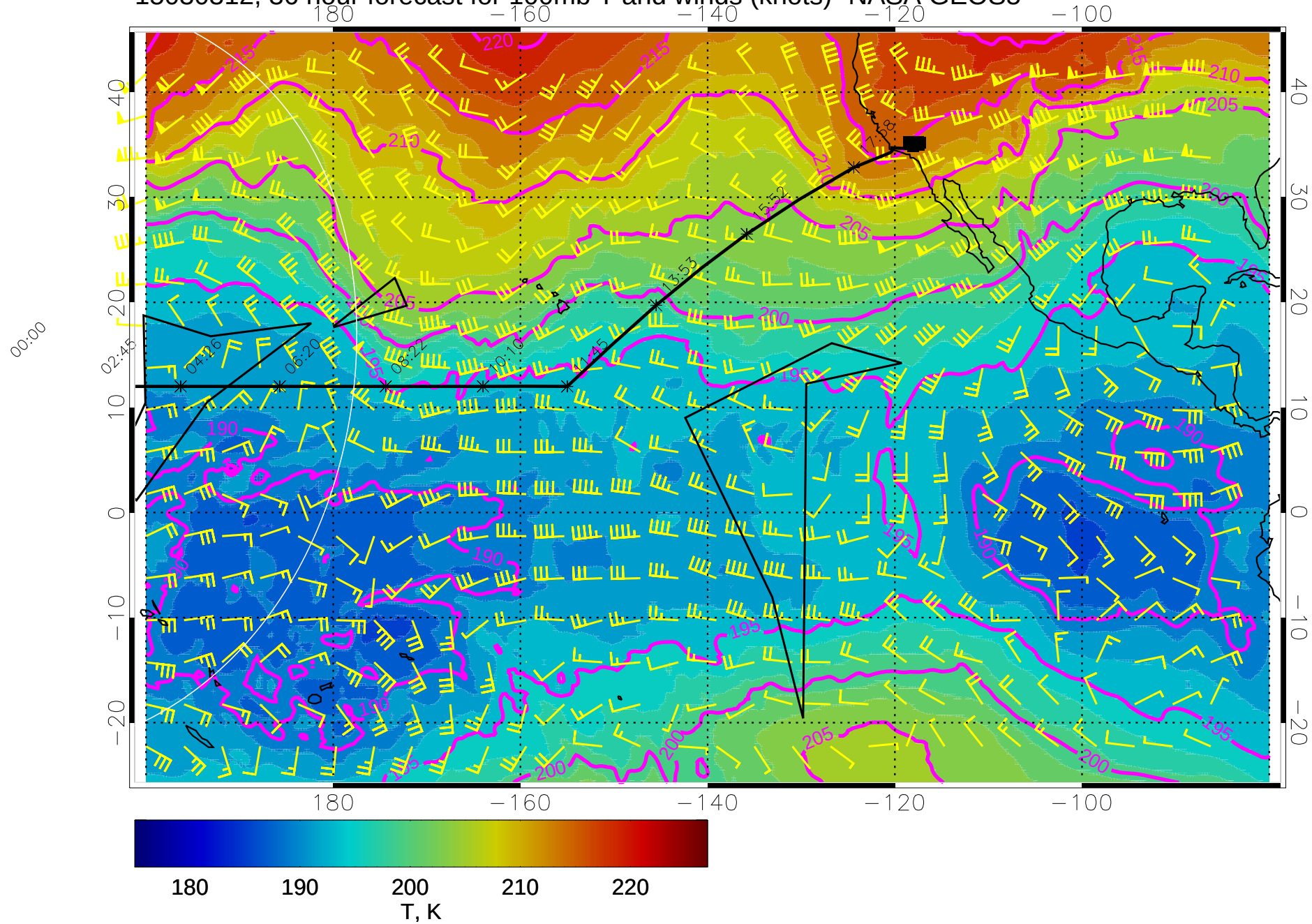
15030312, 36 hour forecast for 100mb T and winds (knots)- NASA GEOS5
