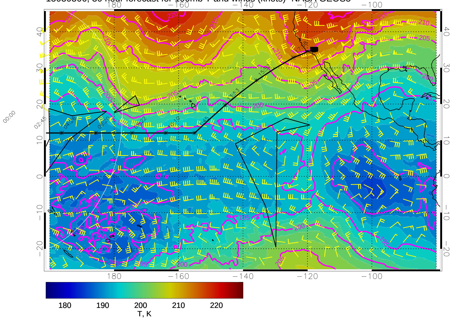
15030306, 30 hour forecast for 100mb T and winds (knots)- NASA GEOS5
