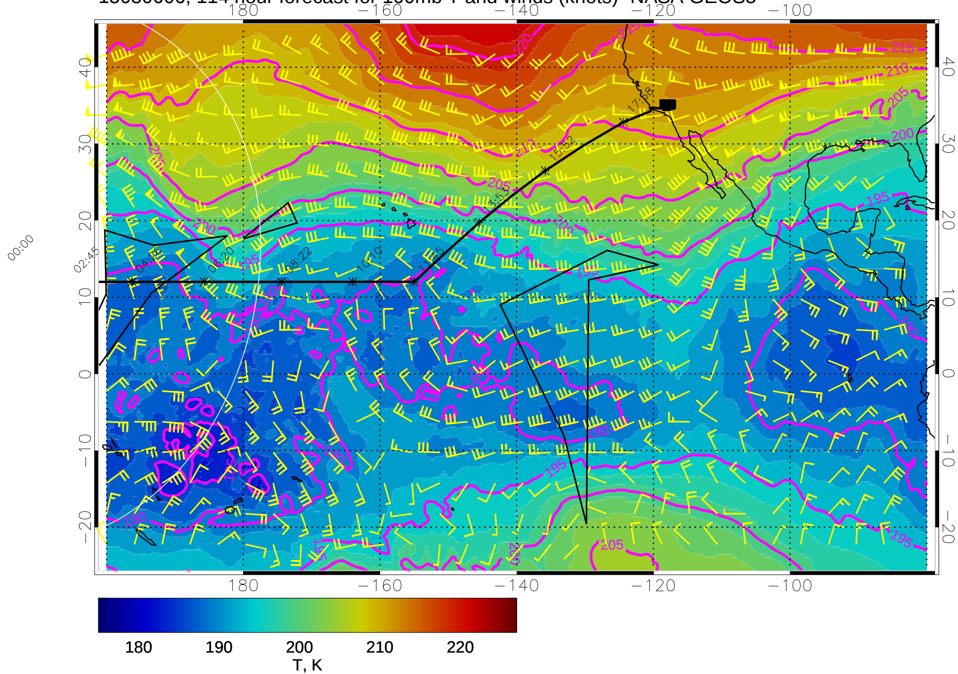
15030606, 114 hour forecast for 100mb T and winds (knots)- NASA GEOS5
