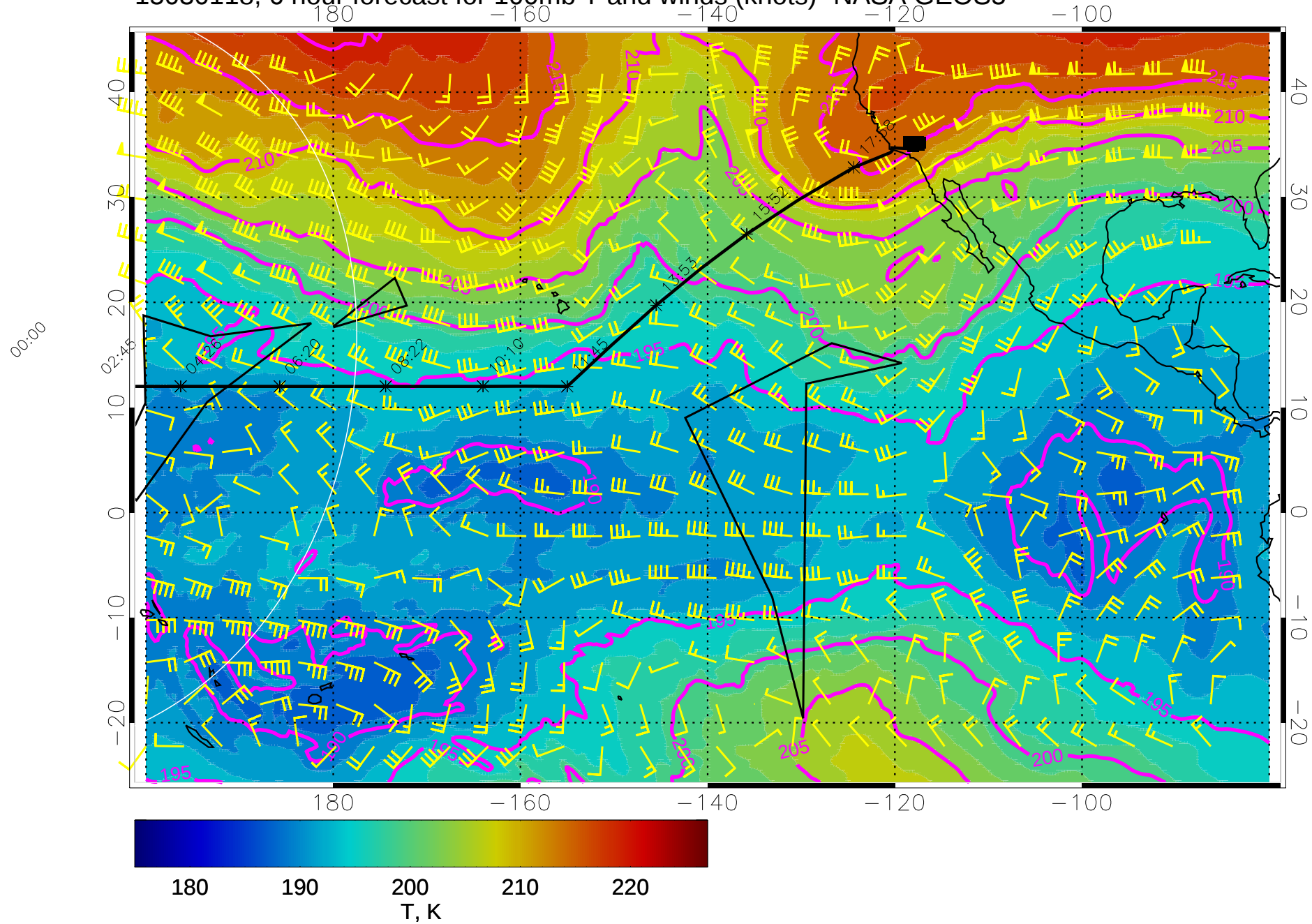
15030118, 6 hour forecast for 100mb T and winds (knots)- NASA GEOS5
