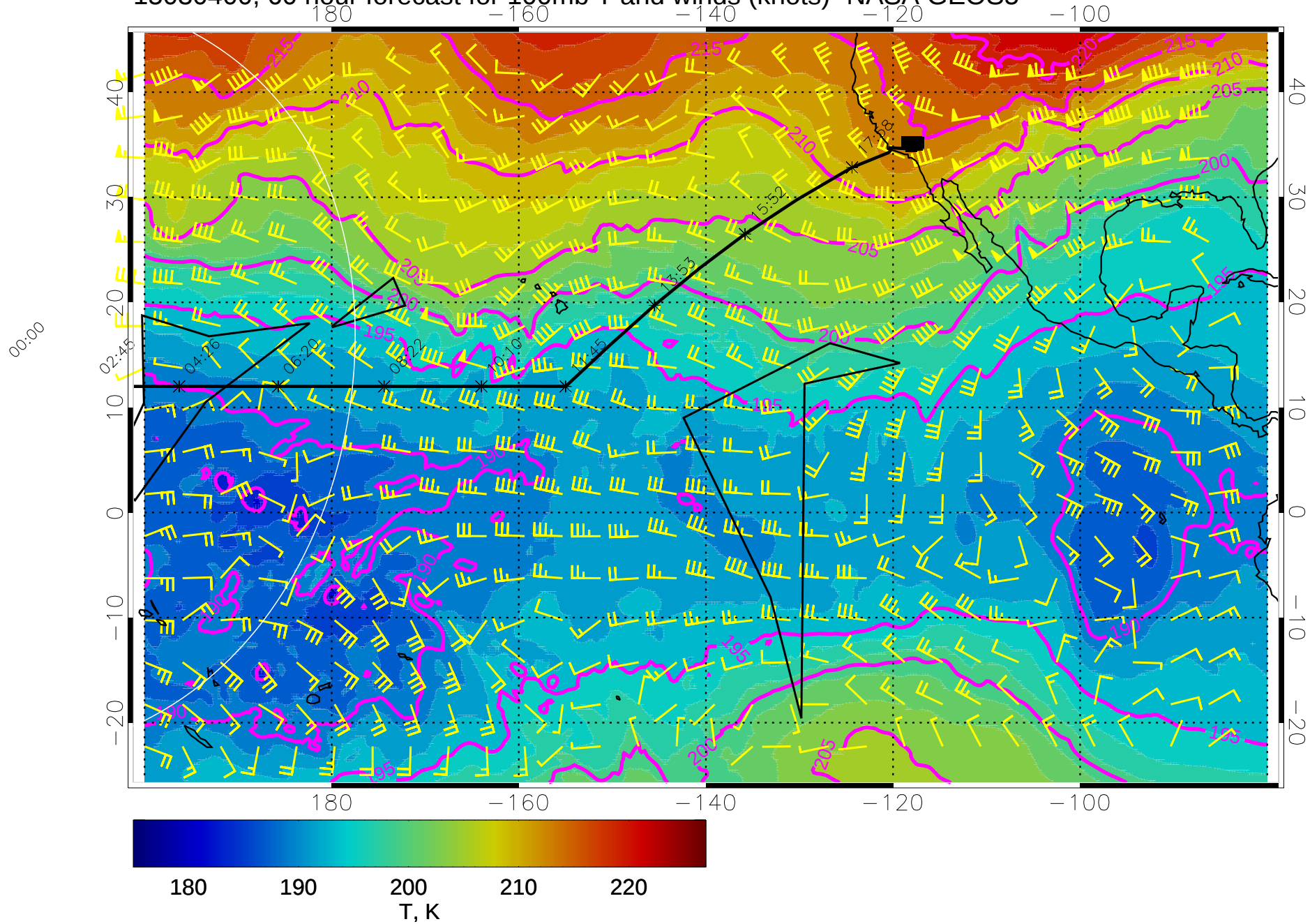
15030400, 60 hour forecast for 100mb T and winds (knots)- NASA GEOS5
