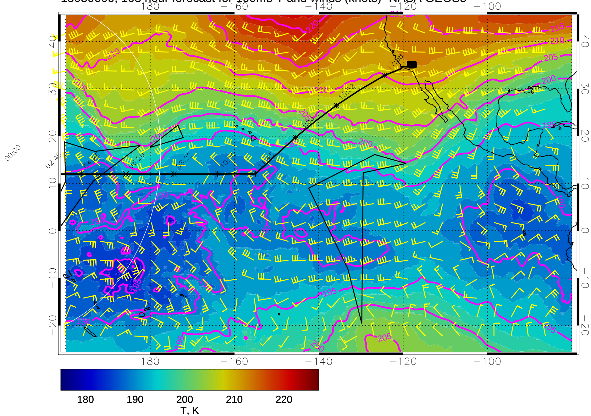
15030600, 108 hour forecast for 100mb T and winds (knots)- NASA GEOS5
