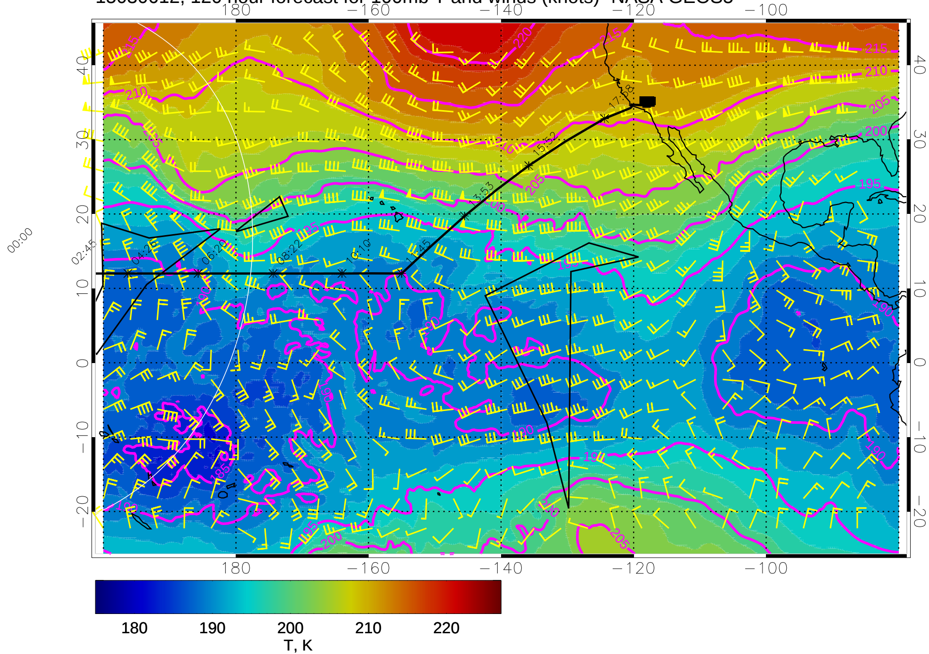
15030612, 120 hour forecast for 100mb T and winds (knots)- NASA GEOS5
