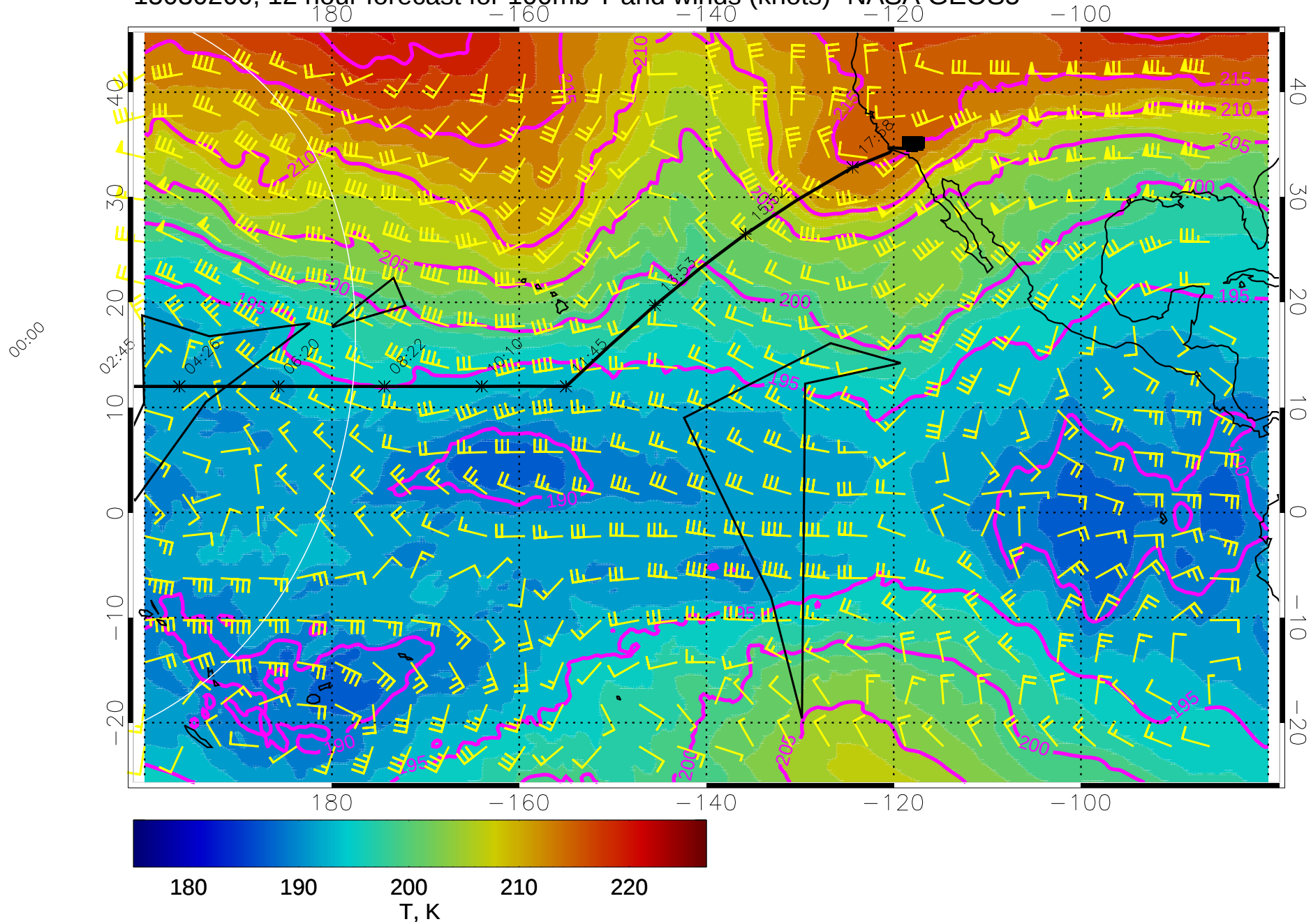
15030200, 12 hour forecast for 100mb T and winds (knots)- NASA GEOS5
