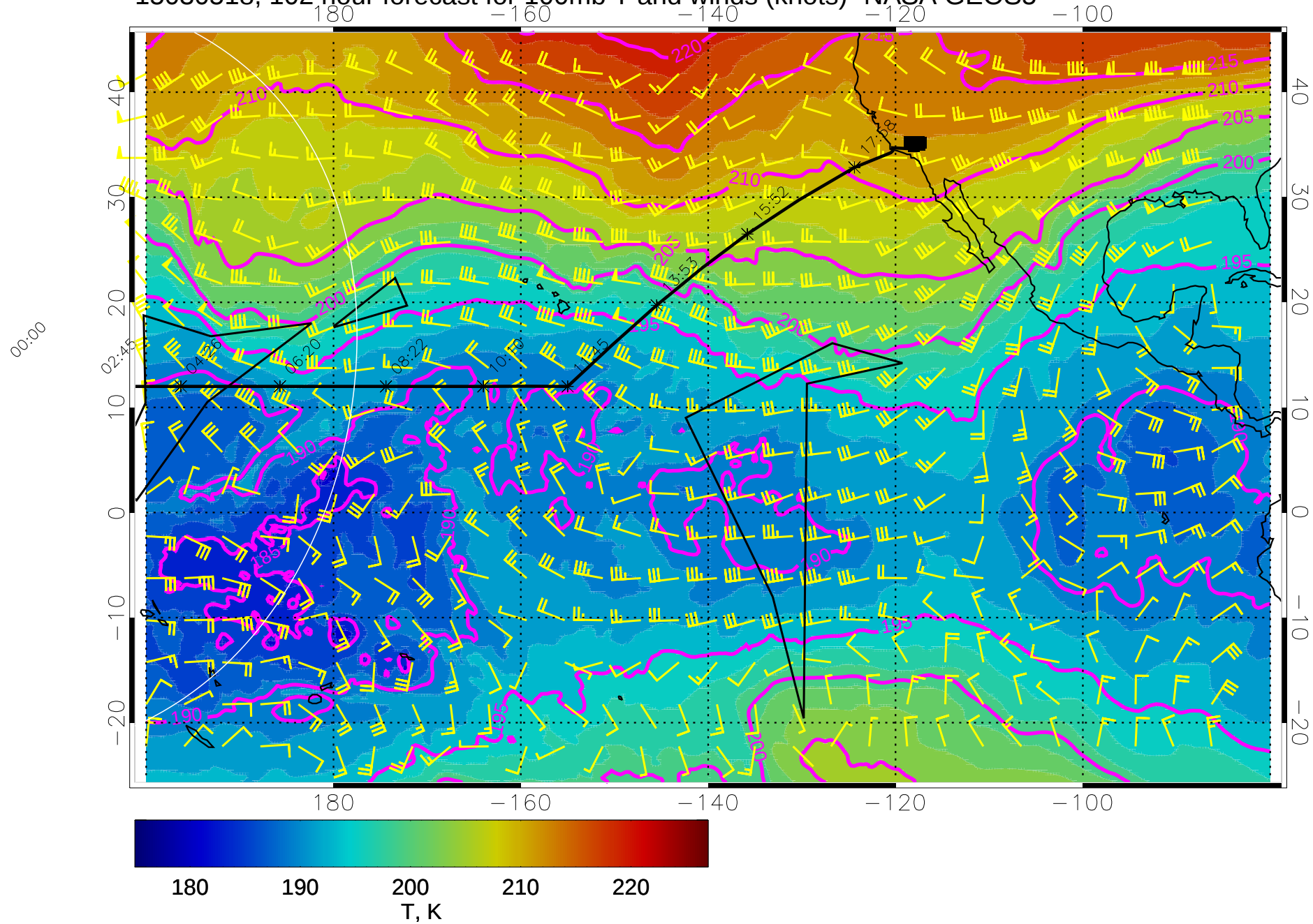
15030518, 102 hour forecast for 100mb T and winds (knots)- NASA GEOS5
