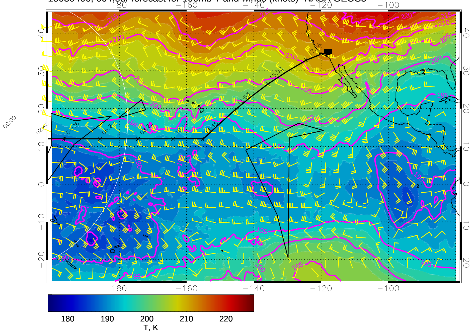
15030406, 66 hour forecast for 100mb T and winds (knots)- NASA GEOS5
