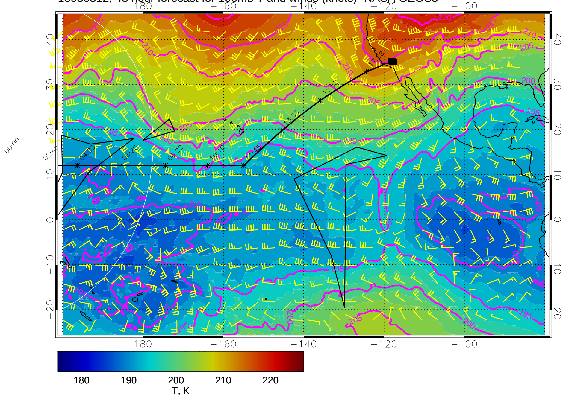
15030312, 48 hour forecast for 100mb T and winds (knots)- NASA GEOS5
