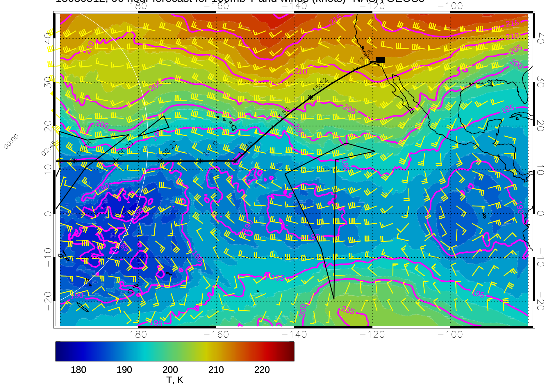
15030512, 96 hour forecast for 100mb T and winds (knots)- NASA GEOS5
