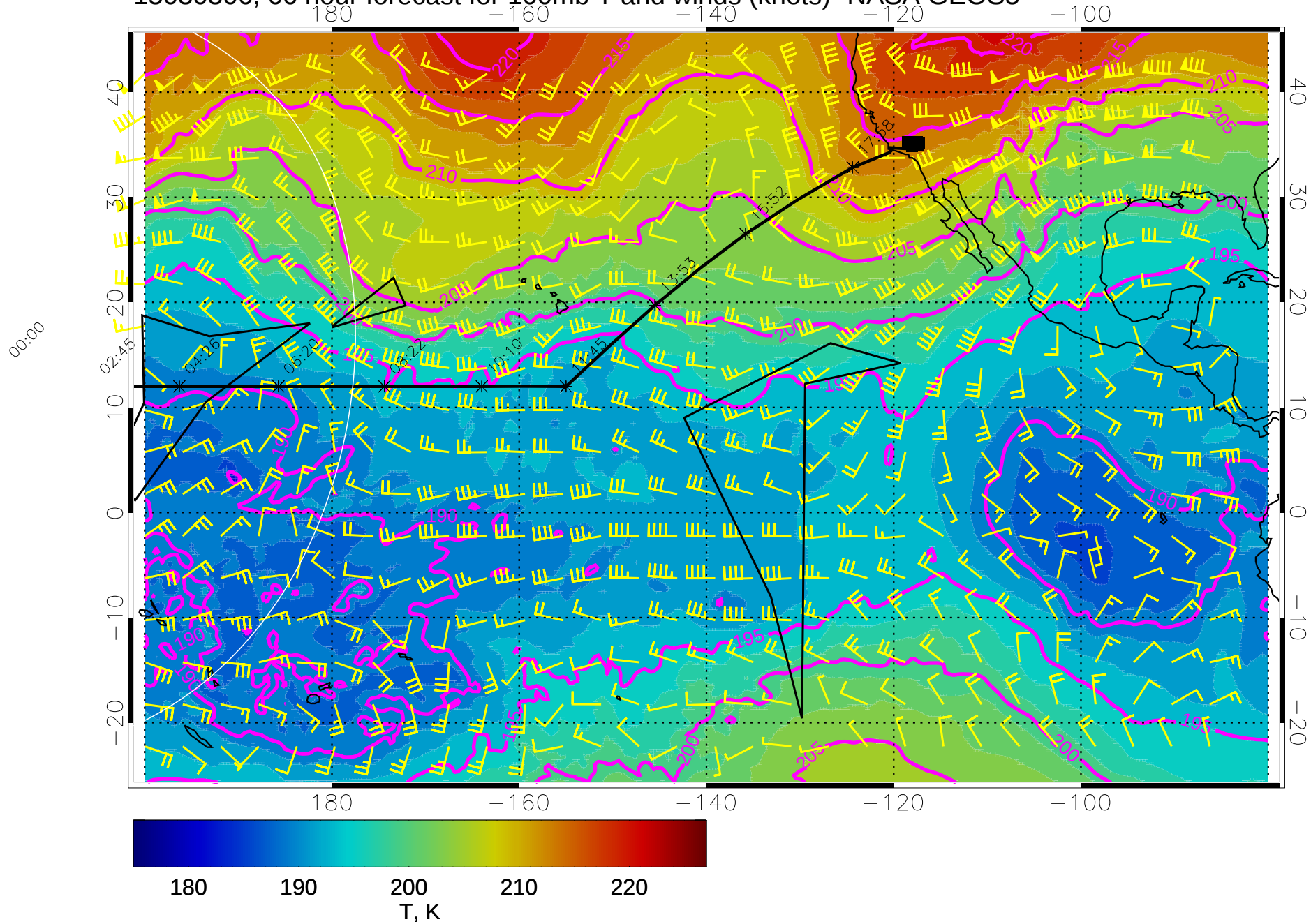
15030306, 66 hour forecast for 100mb T and winds (knots)- NASA GEOS5
