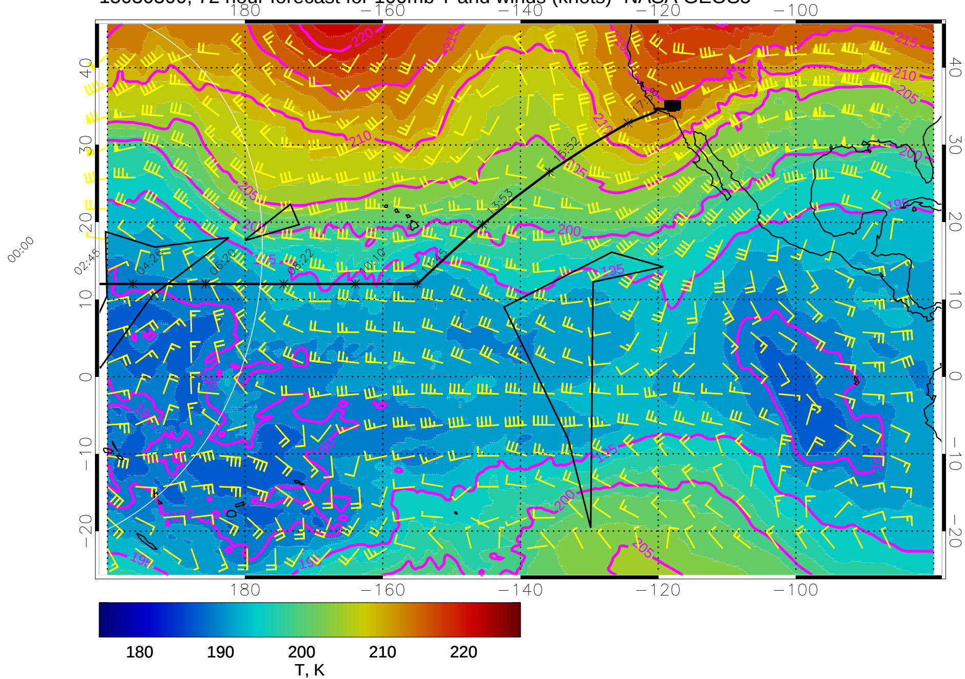
15030300, 72 hour forecast for 100mb T and winds (knots)- NASA GEOS5
