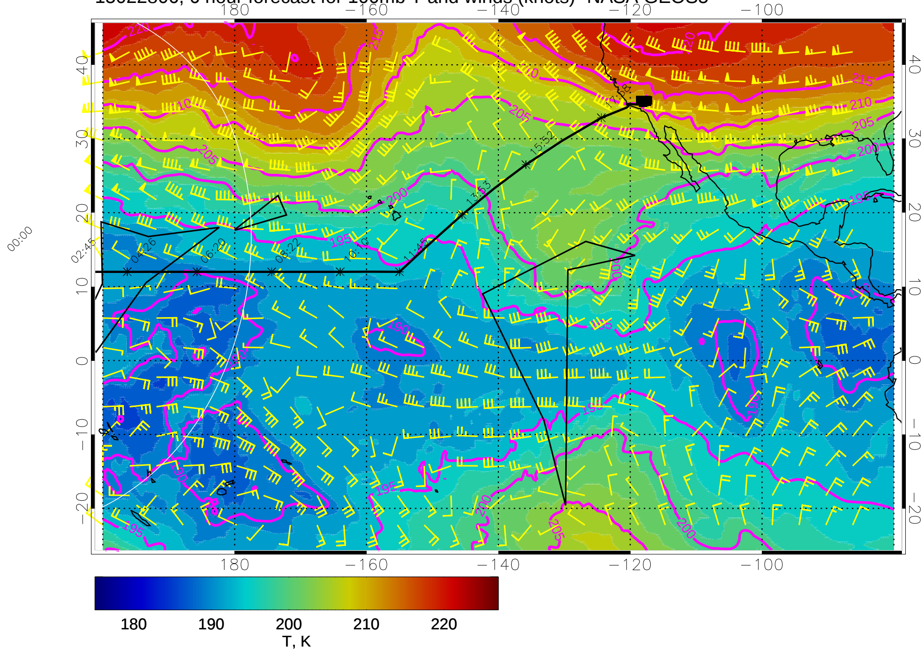
15022806, 6 hour forecast for 100mb T and winds (knots)- NASA GEOS5
