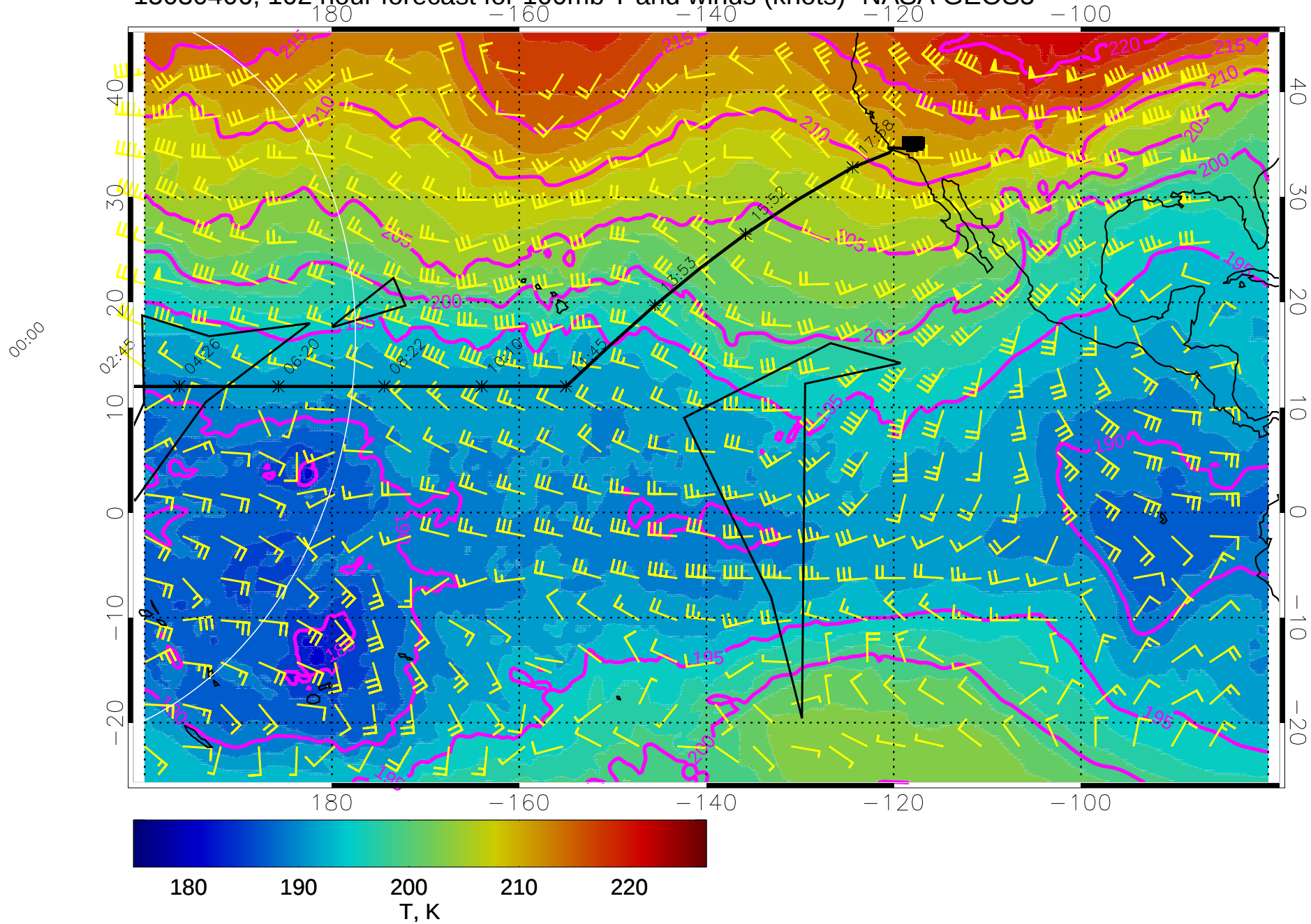
15030406, 102 hour forecast for 100mb T and winds (knots)- NASA GEOS5
