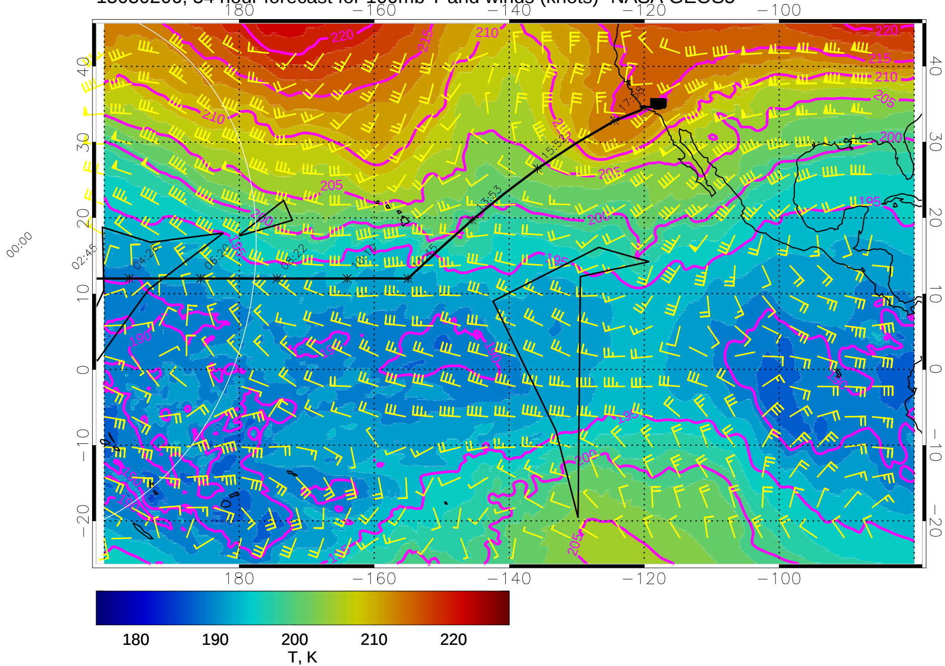
15030206, 54 hour forecast for 100mb T and winds (knots)- NASA GEOS5
