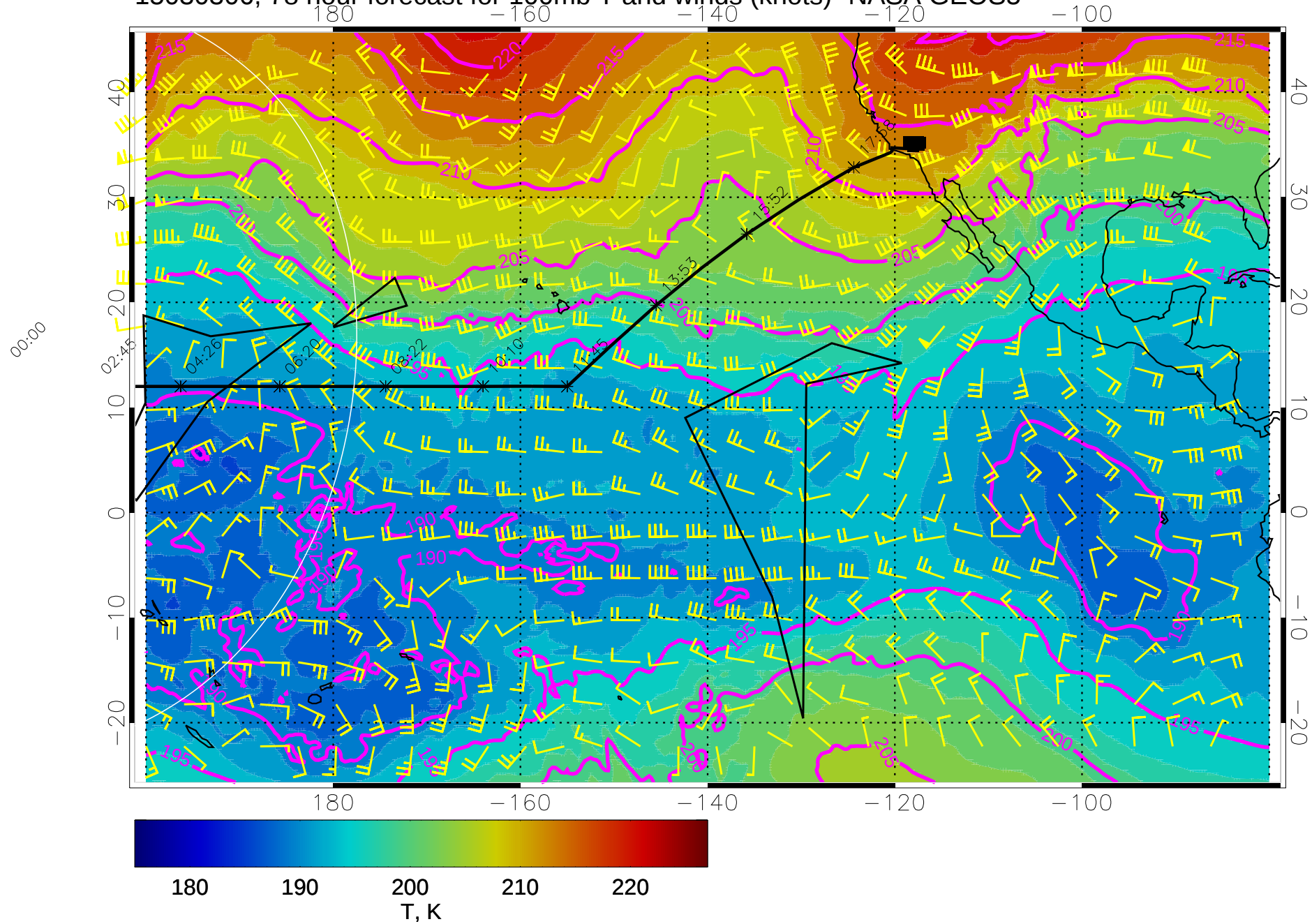
15030306, 78 hour forecast for 100mb T and winds (knots)- NASA GEOS5
