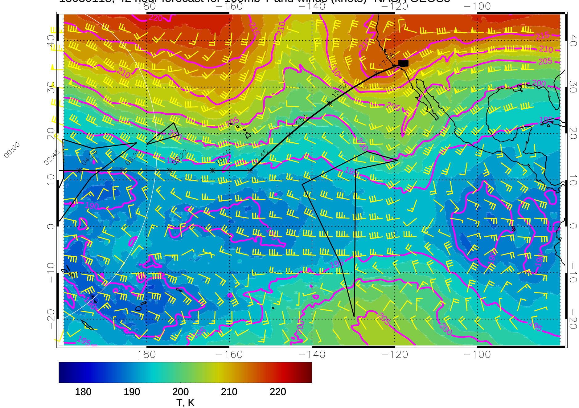
15030118, 42 hour forecast for 100mb T and winds (knots)- NASA GEOS5
