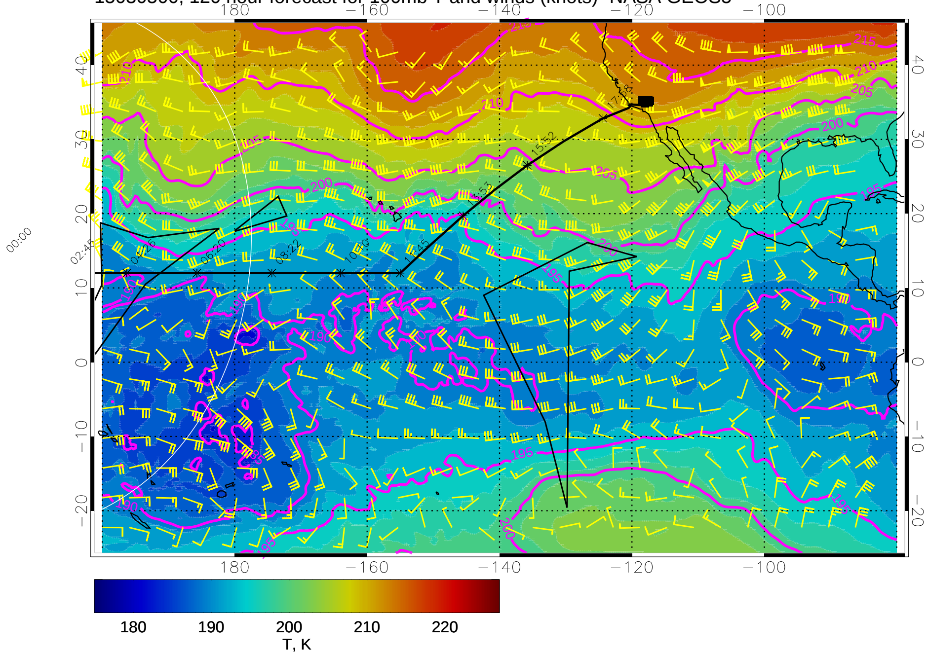
15030500, 120 hour forecast for 100mb T and winds (knots)- NASA GEOS5
