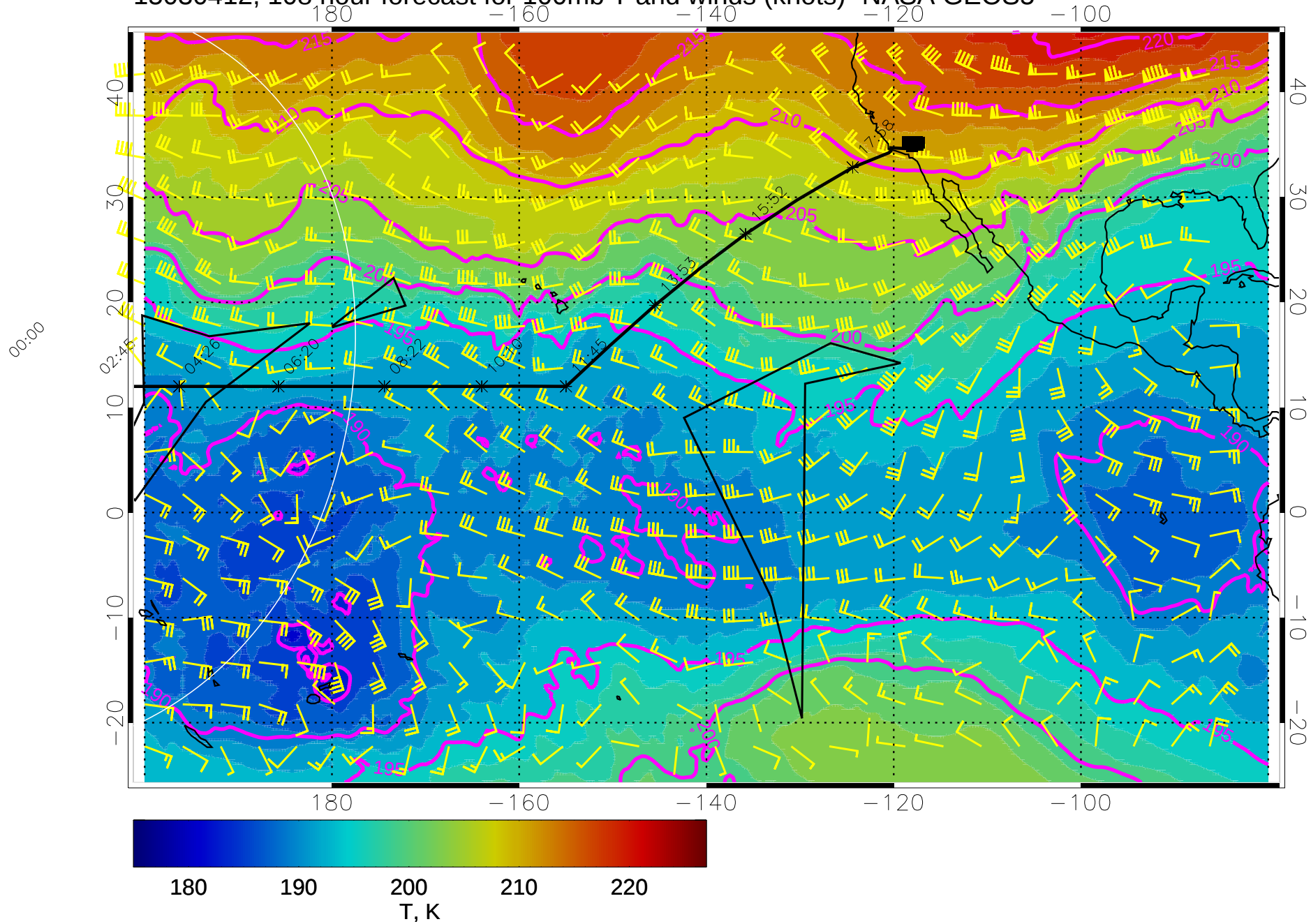
15030412, 108 hour forecast for 100mb T and winds (knots)- NASA GEOS5
