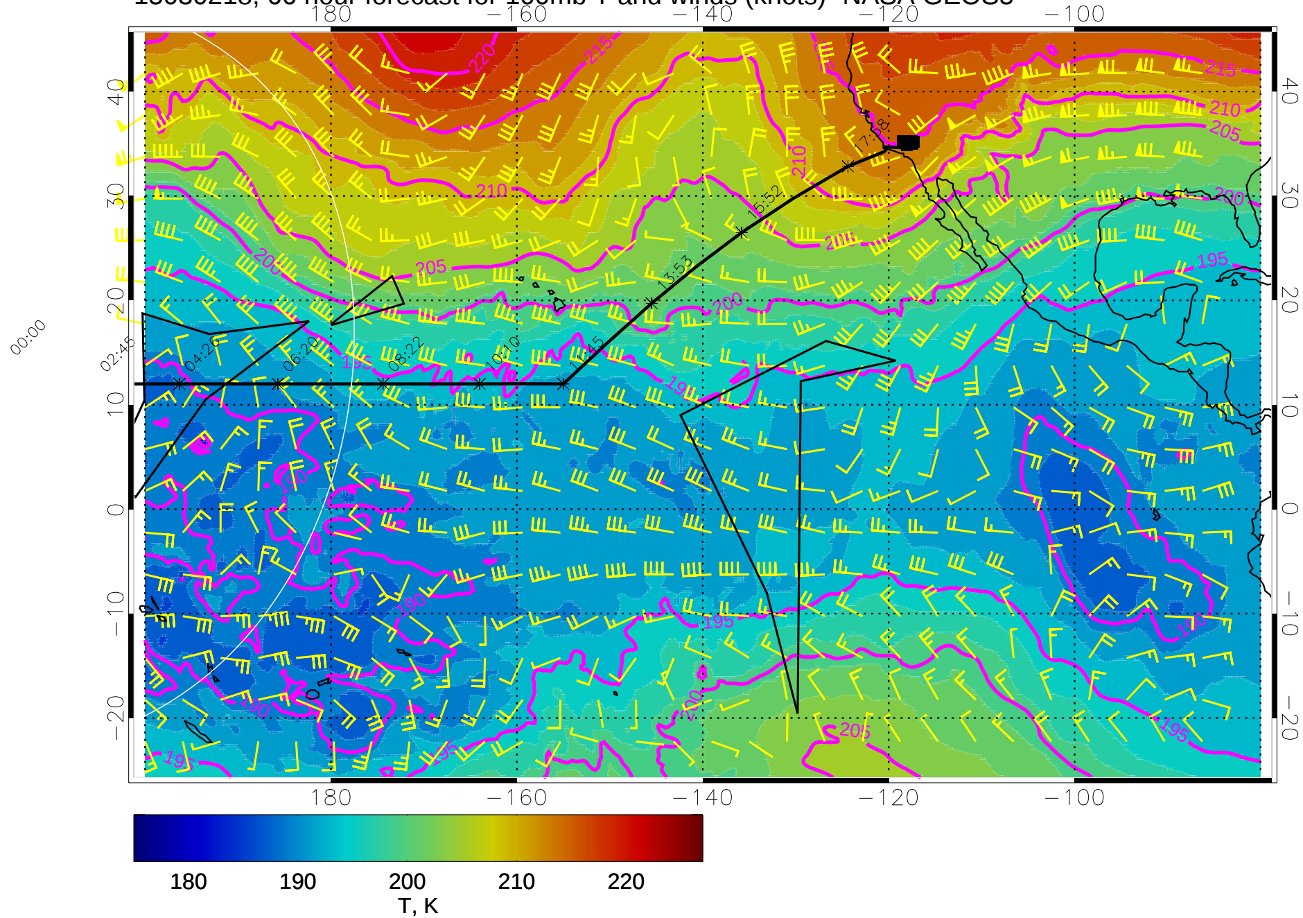
15030218, 66 hour forecast for 100mb T and winds (knots)- NASA GEOS5
