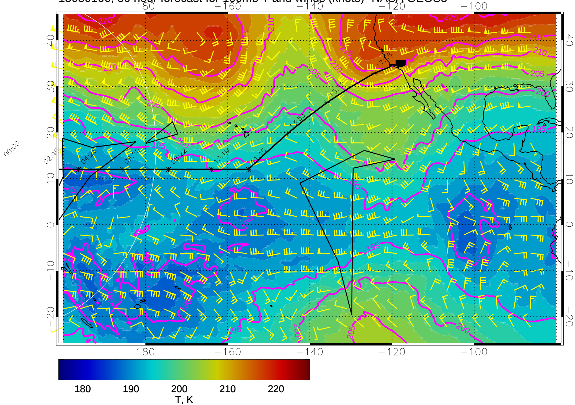
15030106, 30 hour forecast for 100mb T and winds (knots)- NASA GEOS5
