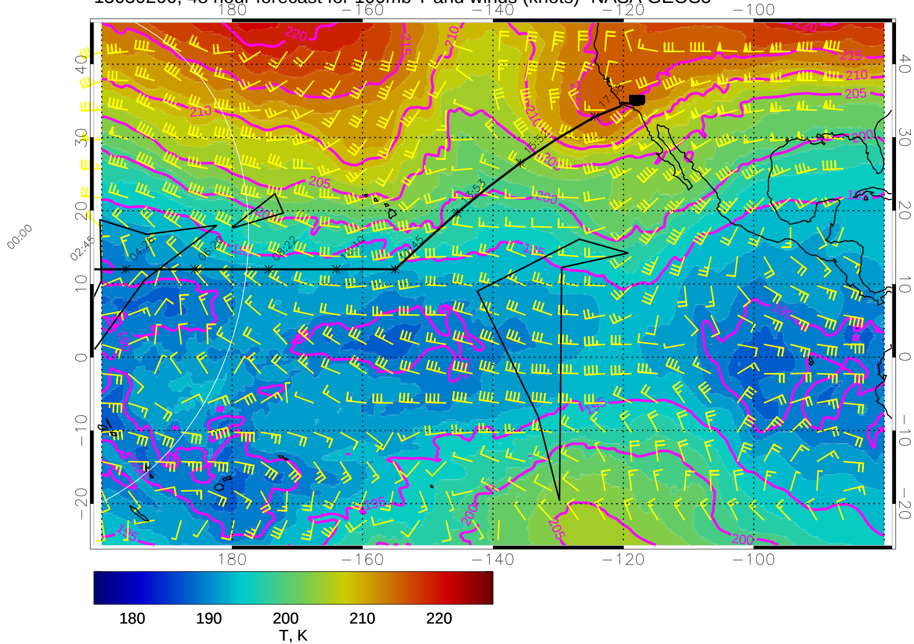
15030200, 48 hour forecast for 100mb T and winds (knots)- NASA GEOS5
