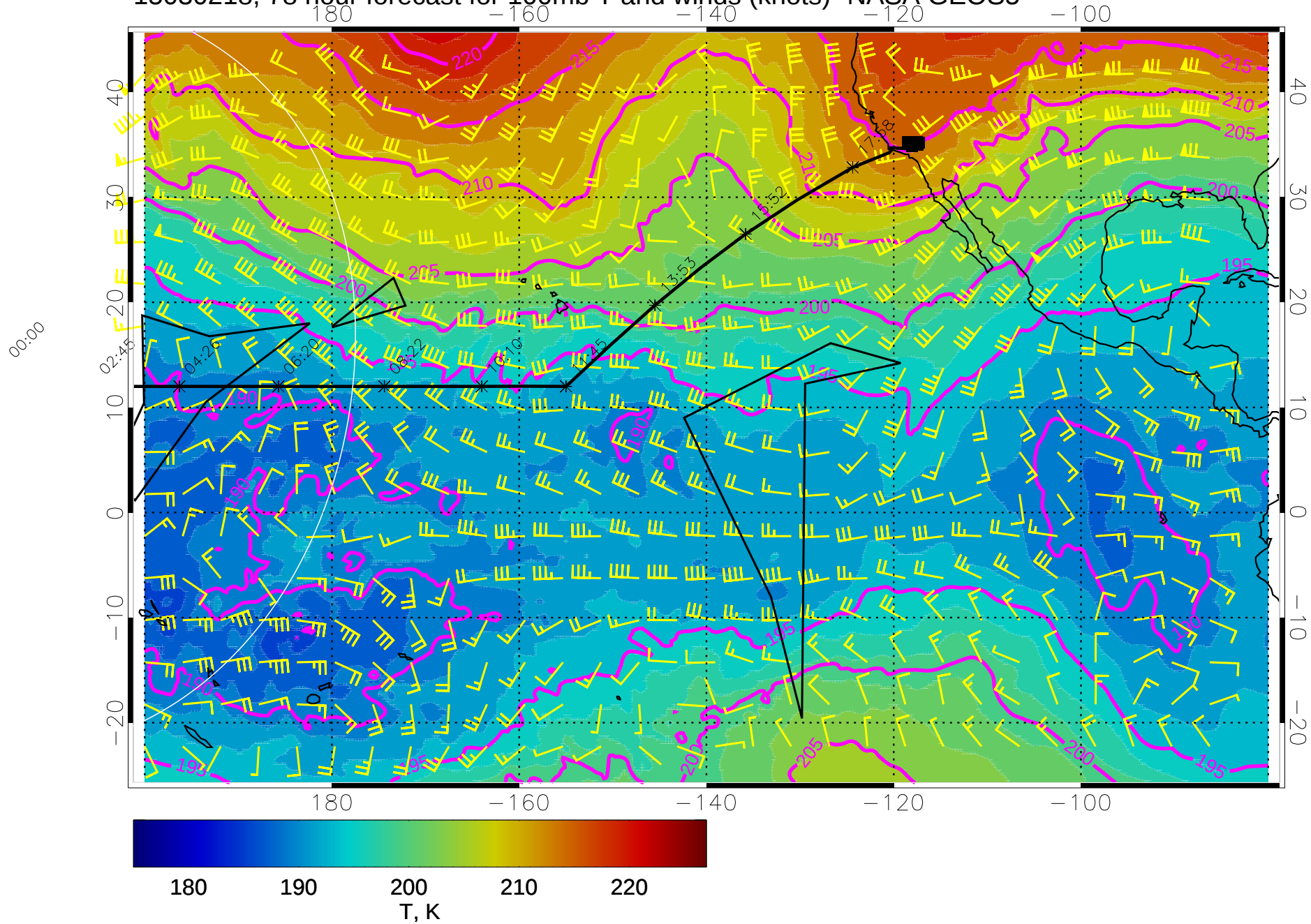
15030218, 78 hour forecast for 100mb T and winds (knots)- NASA GEOS5
