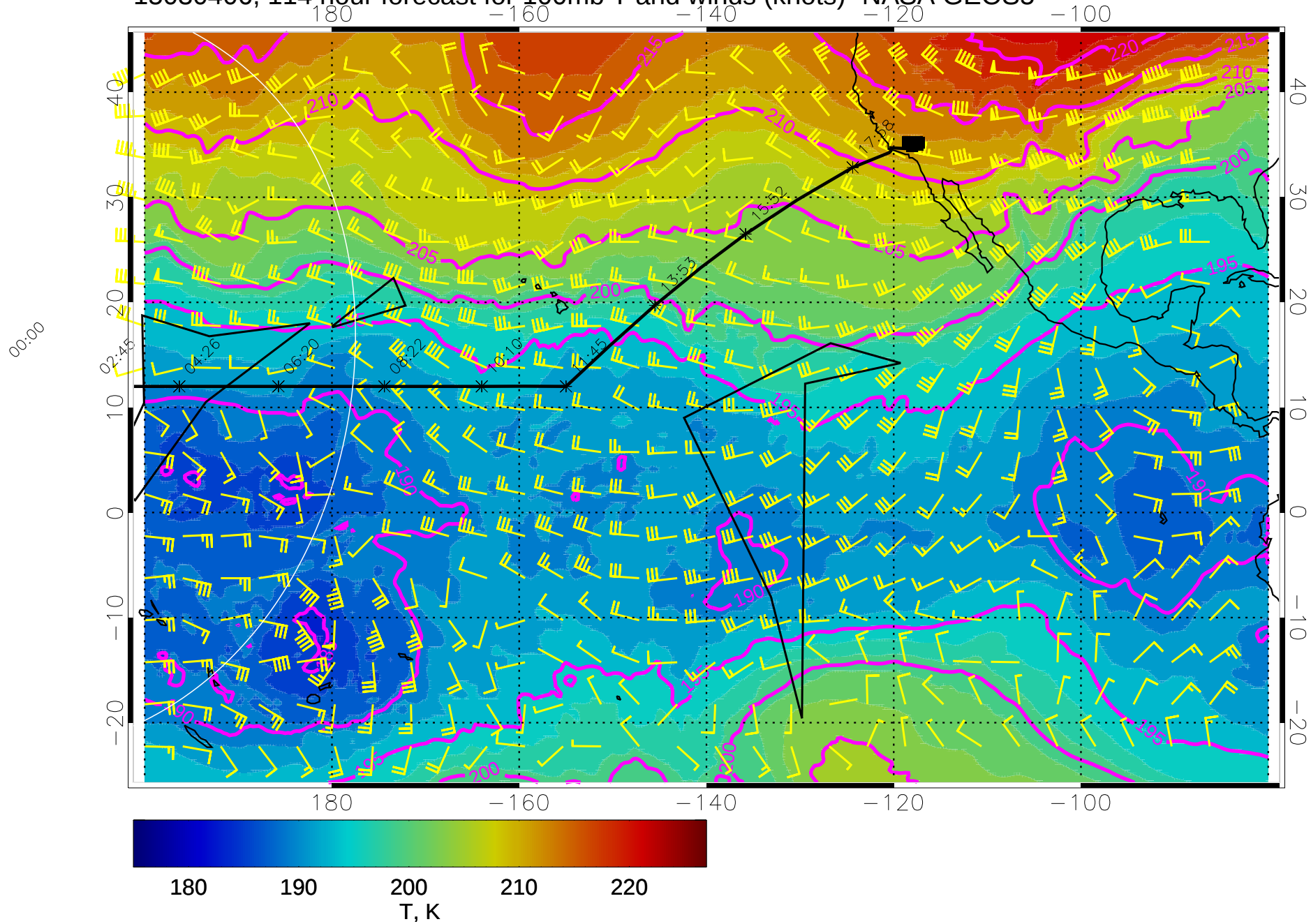
15030406, 114 hour forecast for 100mb T and winds (knots)- NASA GEOS5
