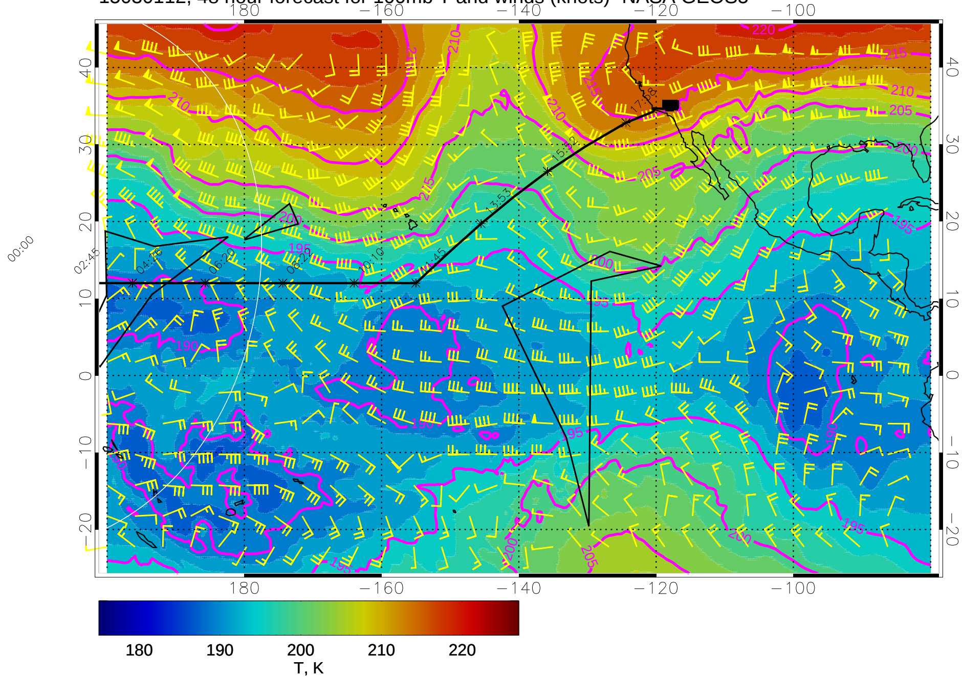
15030112, 48 hour forecast for 100mb T and winds (knots)- NASA GEOS5
