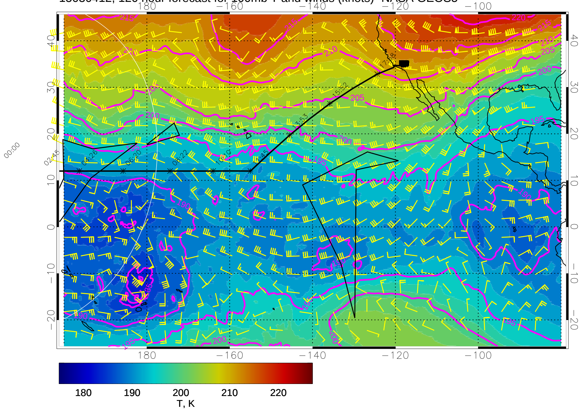
15030412, 120 hour forecast for 100mb T and winds (knots)- NASA GEOS5
