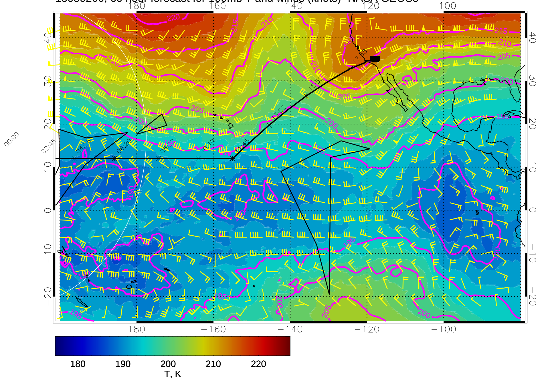
15030200, 60 hour forecast for 100mb T and winds (knots)- NASA GEOS5
