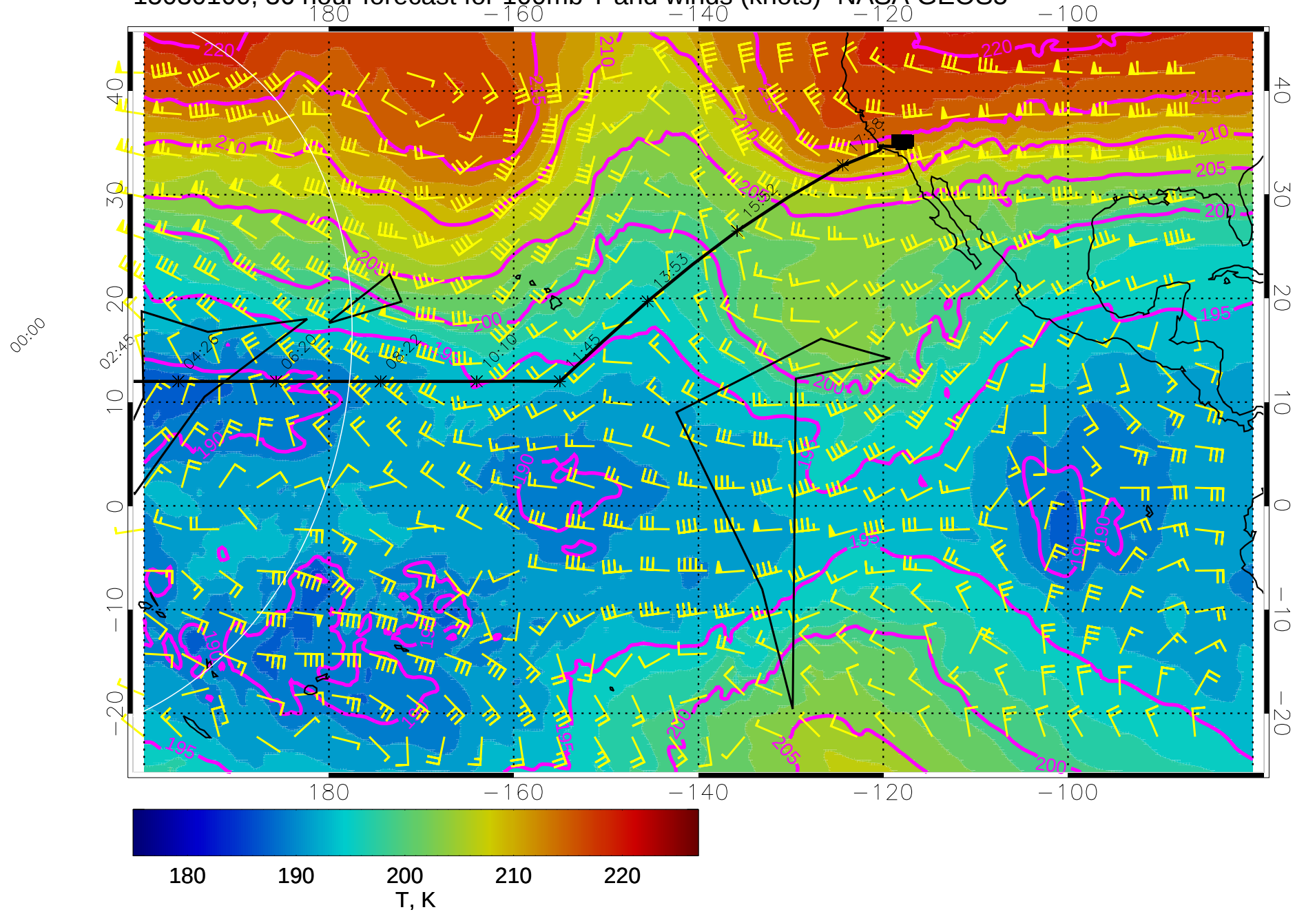
15030100, 36 hour forecast for 100mb T and winds (knots)- NASA GEOS5
