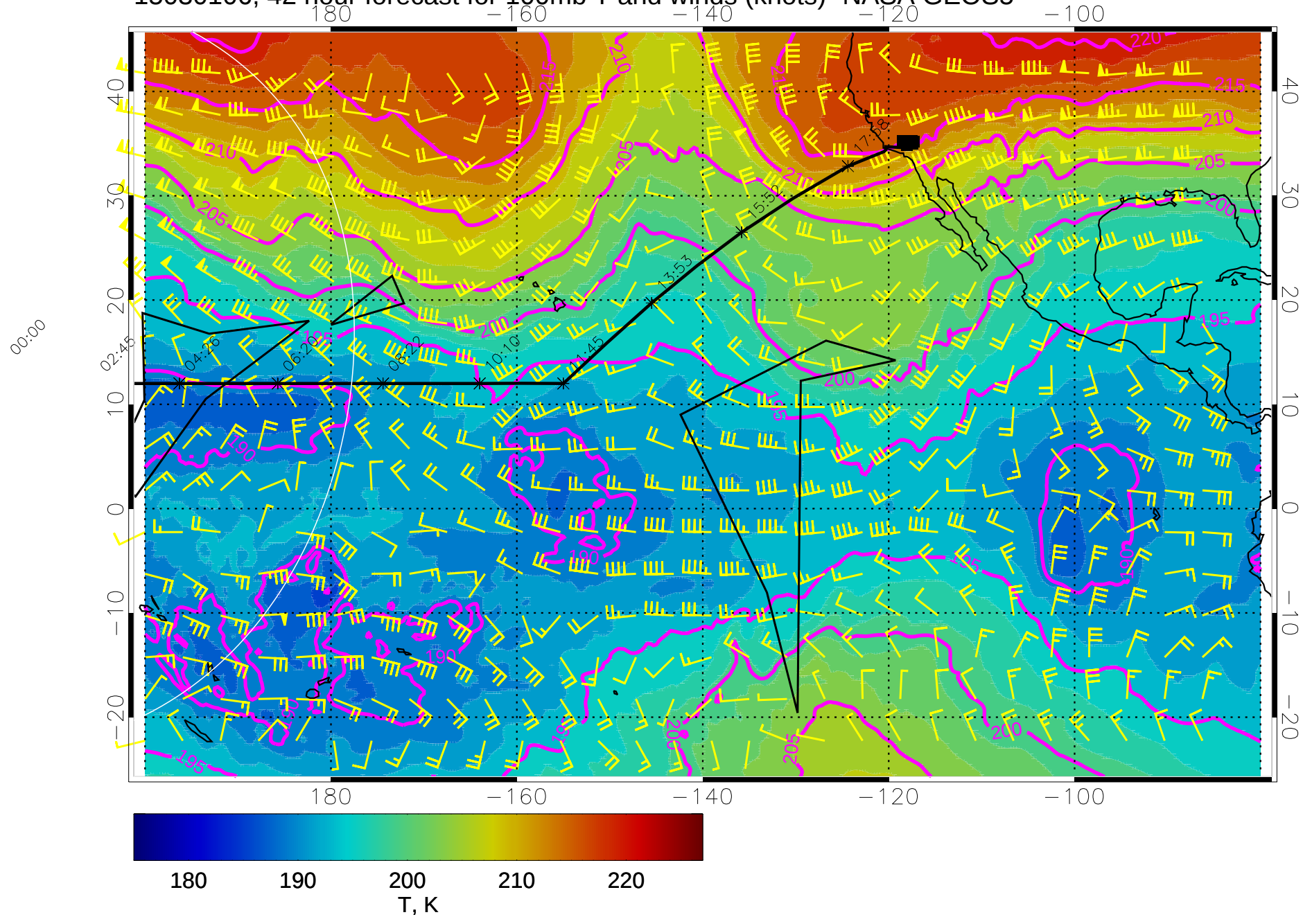
15030106, 42 hour forecast for 100mb T and winds (knots)- NASA GEOS5
