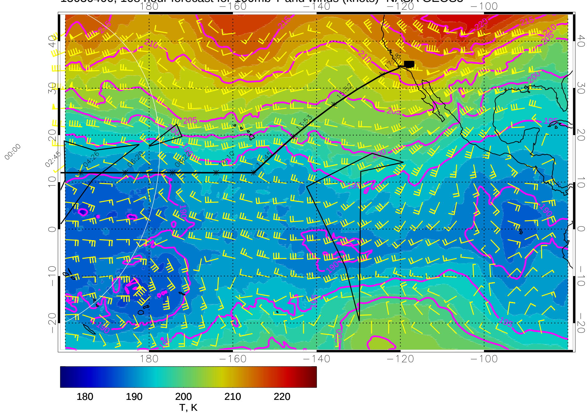
15030400, 108 hour forecast for 100mb T and winds (knots)- NASA GEOS5
