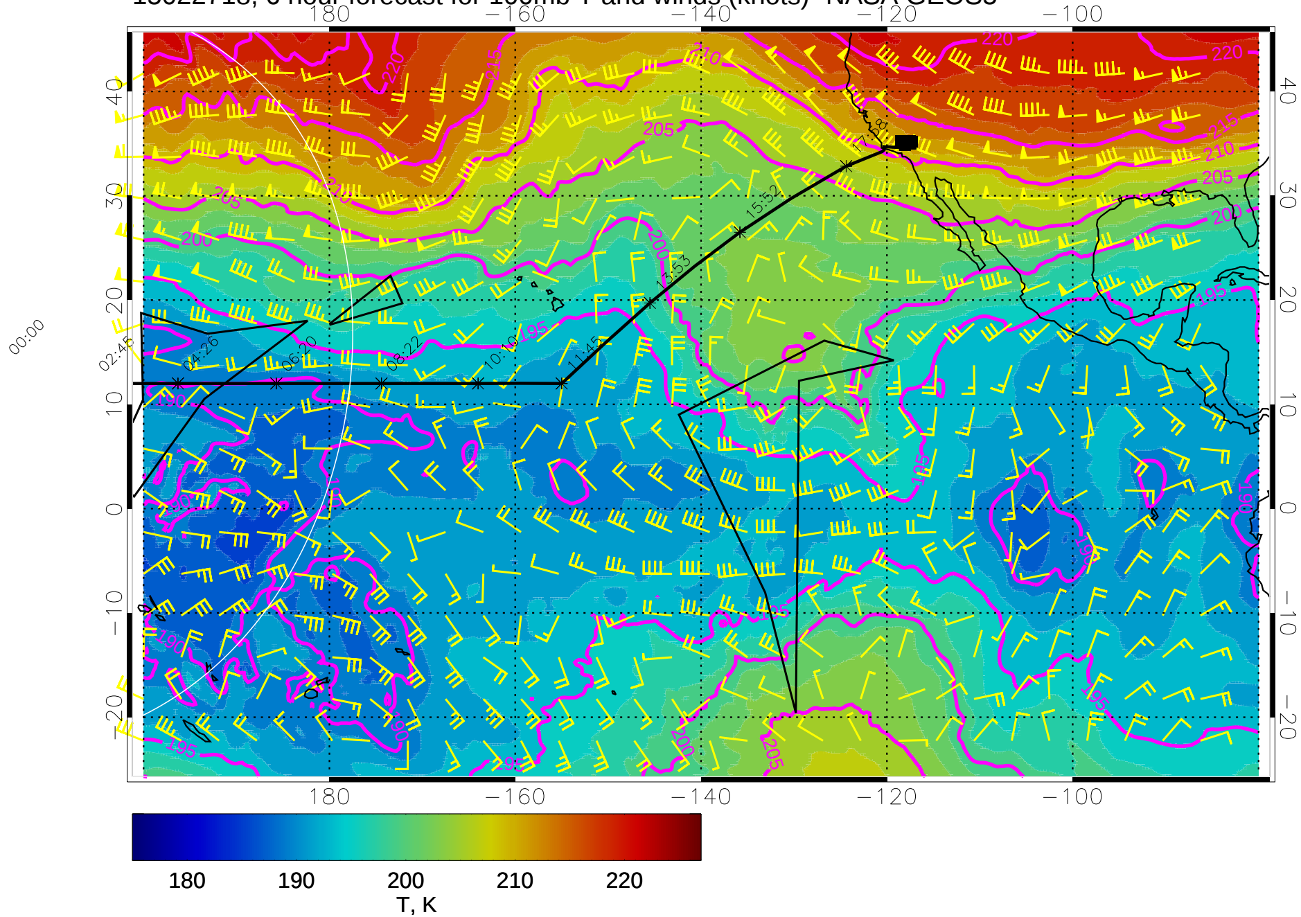
15022718, 6 hour forecast for 100mb T and winds (knots)- NASA GEOS5
