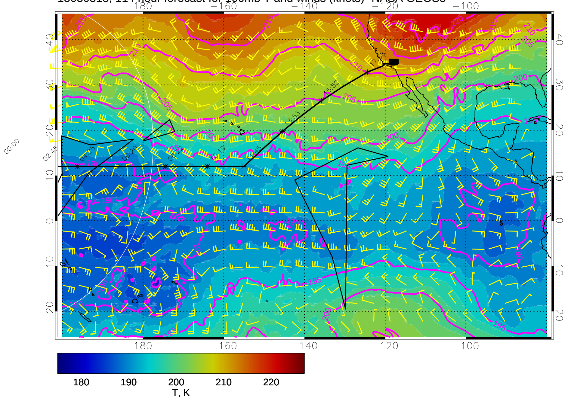
15030318, 114 hour forecast for 100mb T and winds (knots)- NASA GEOS5
