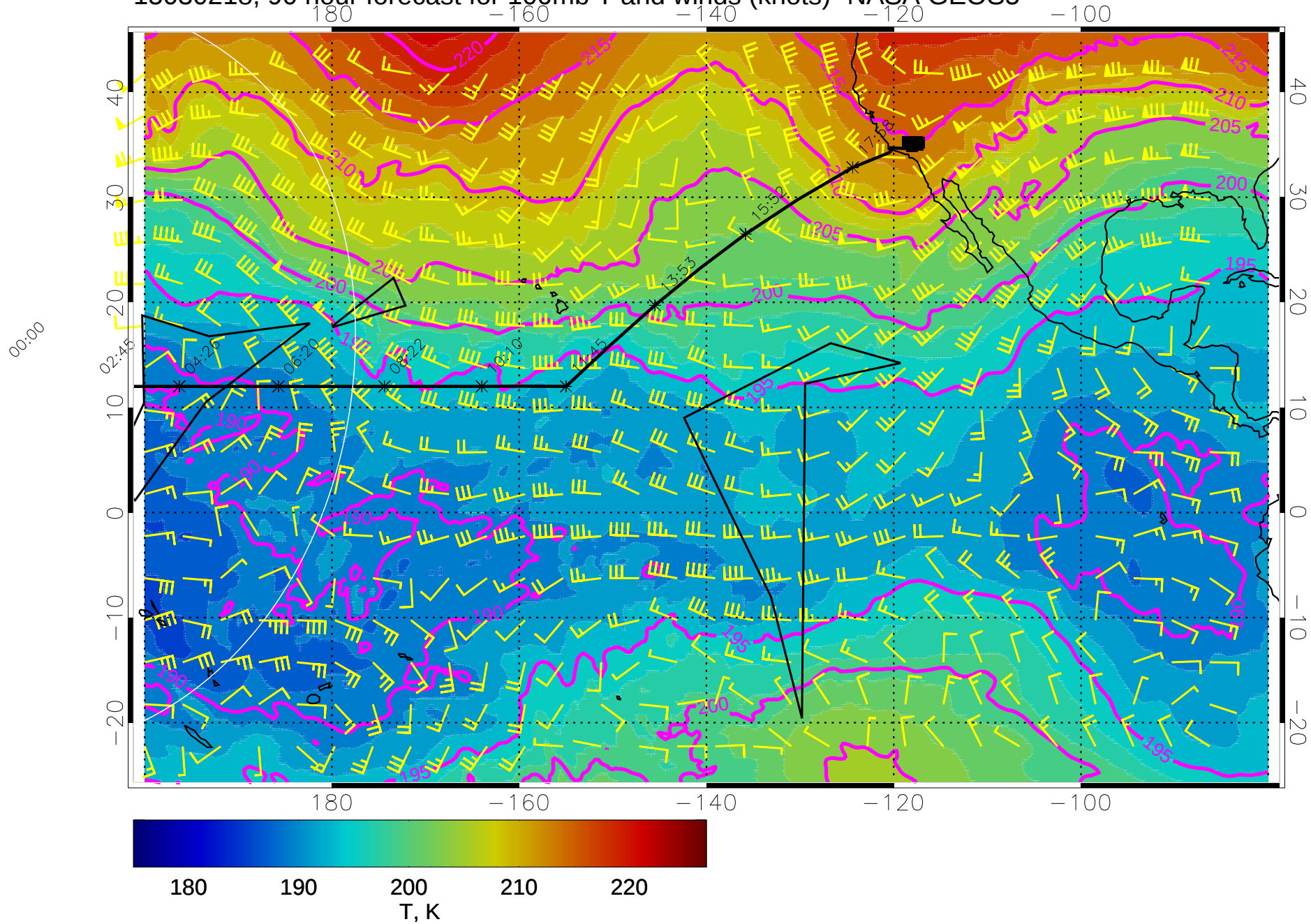
15030218, 90 hour forecast for 100mb T and winds (knots)- NASA GEOS5
