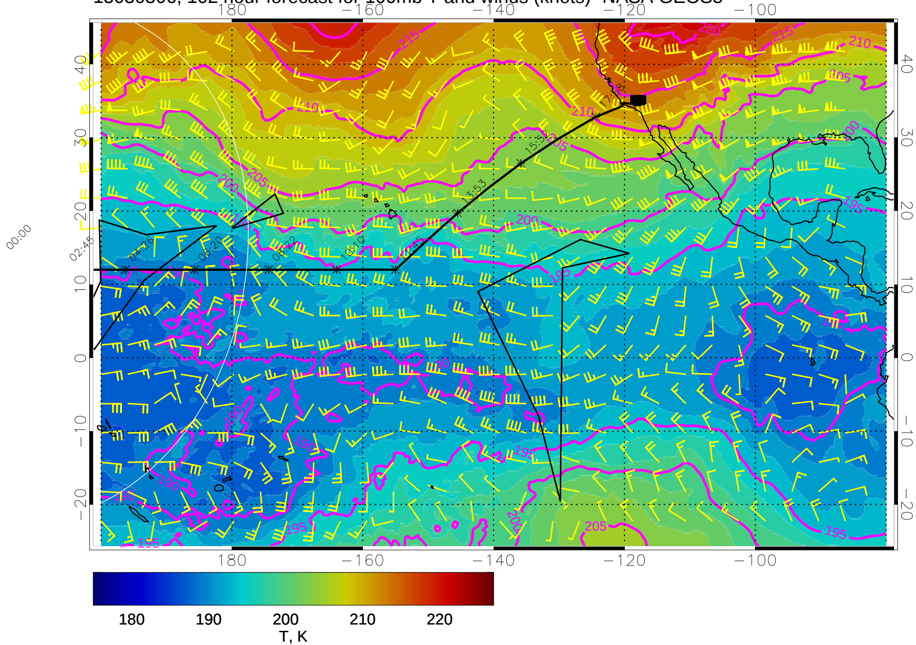
15030306, 102 hour forecast for 100mb T and winds (knots)- NASA GEOS5
