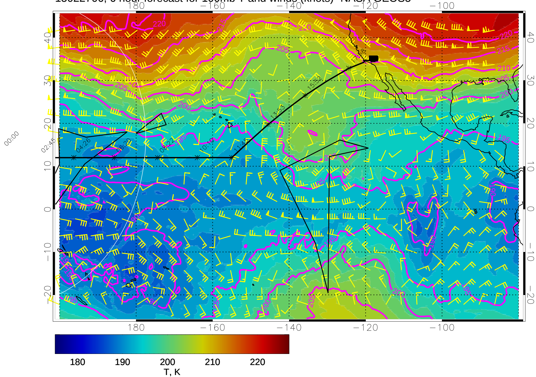
15022706, 6 hour forecast for 100mb T and winds (knots)- NASA GEOS5
