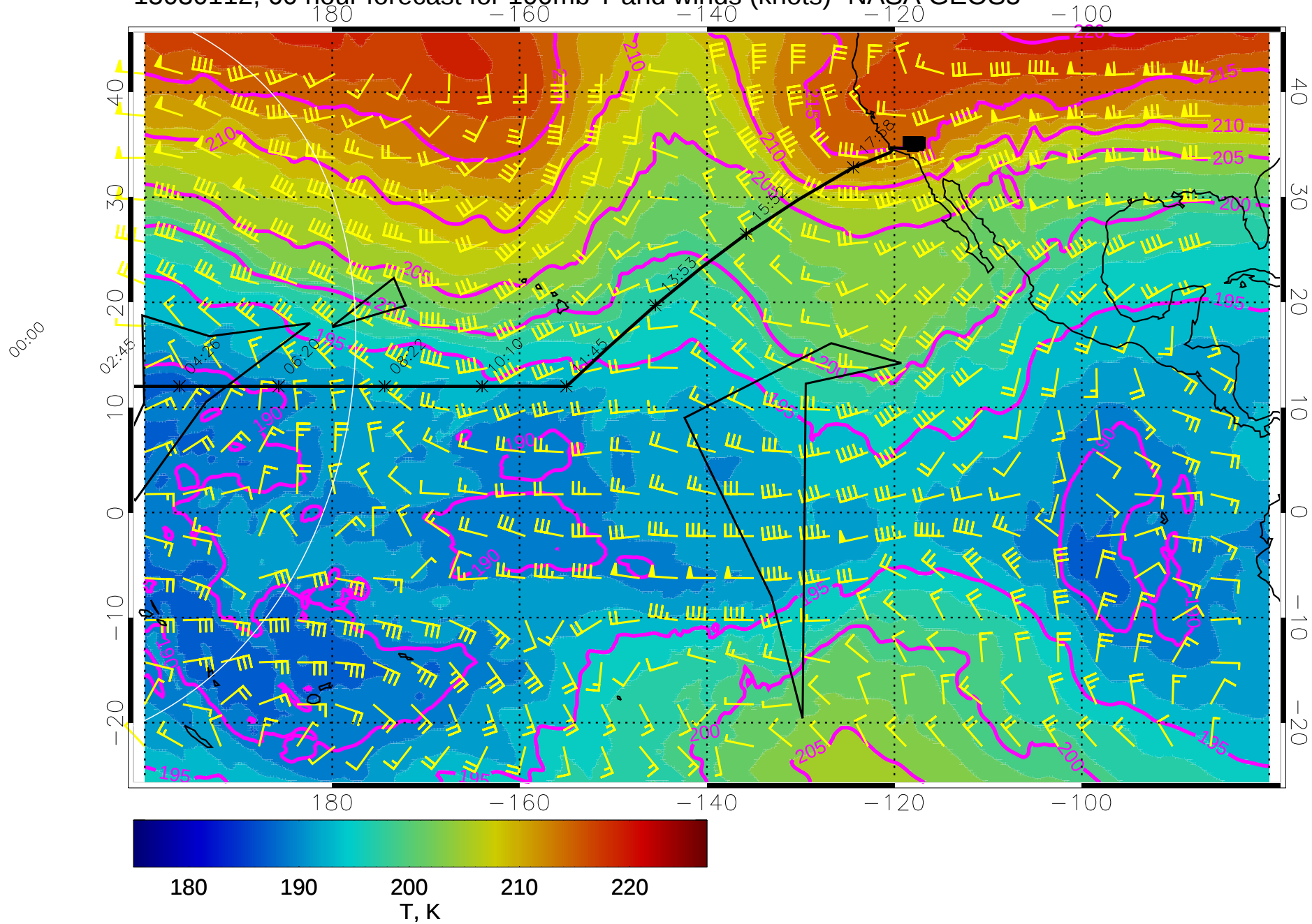
15030112, 60 hour forecast for 100mb T and winds (knots)- NASA GEOS5
