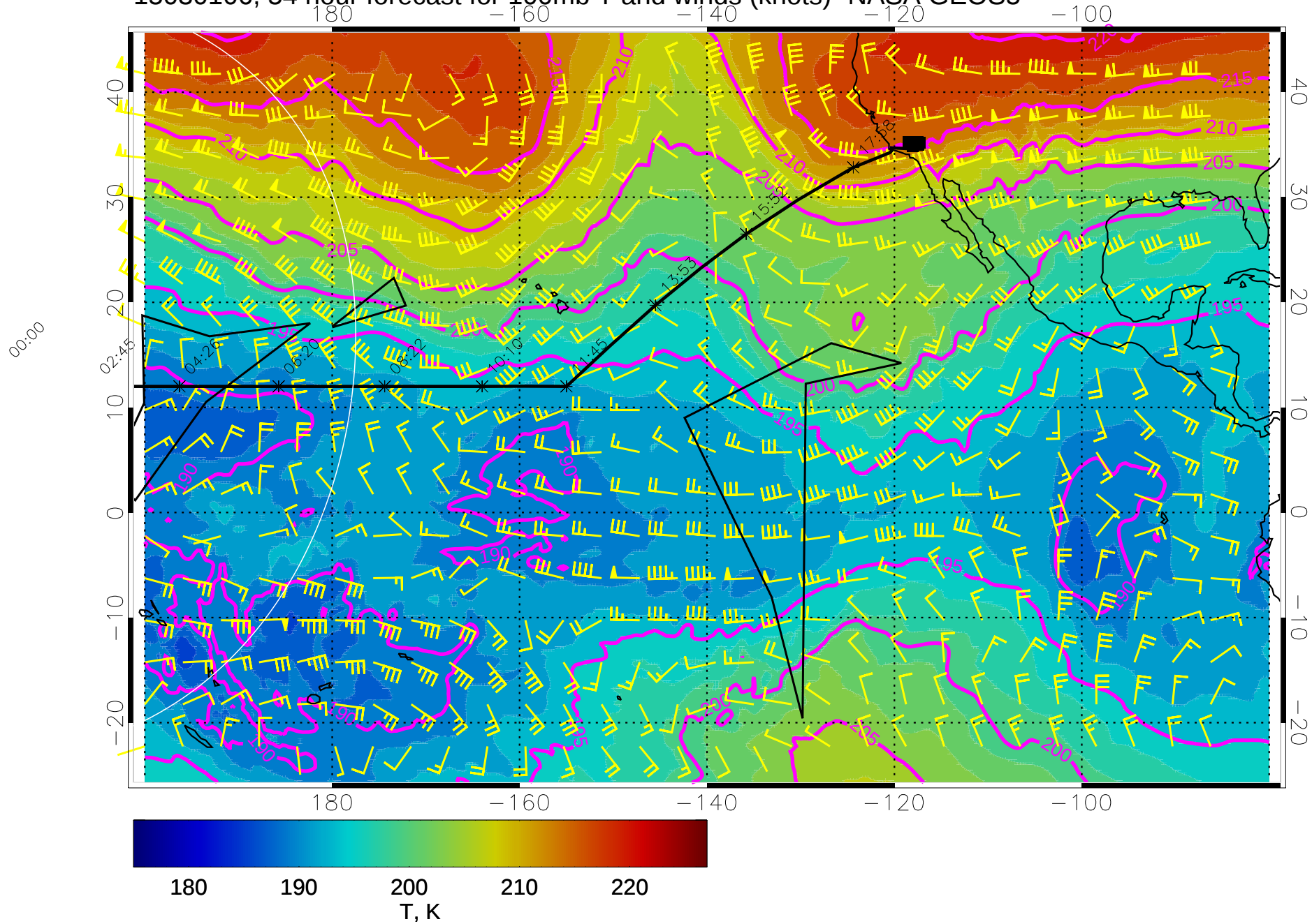
15030106, 54 hour forecast for 100mb T and winds (knots)- NASA GEOS5
