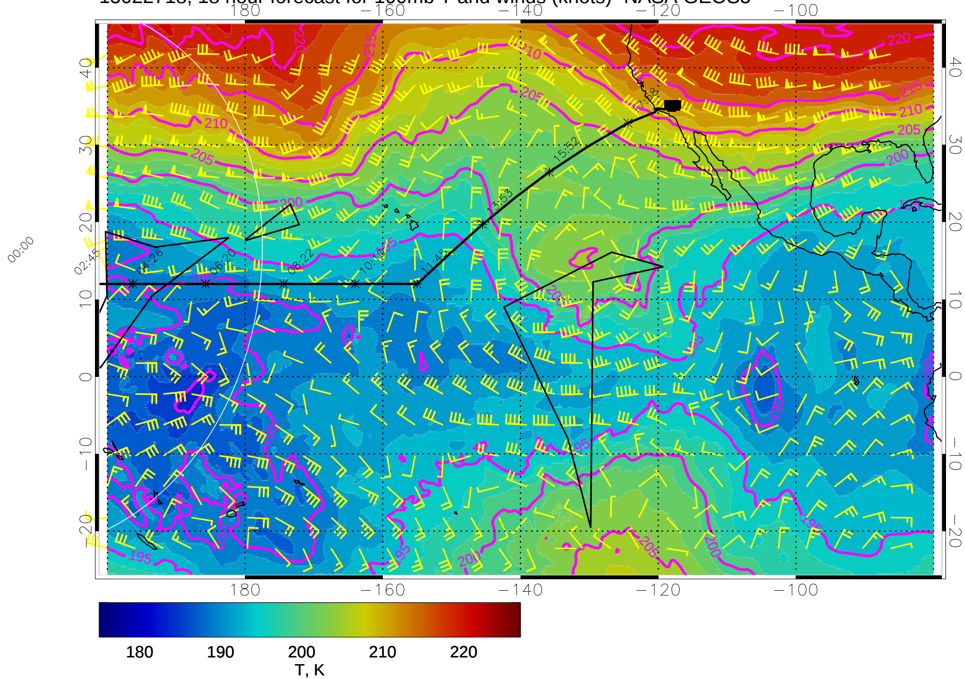
15022718, 18 hour forecast for 100mb T and winds (knots)- NASA GEOS5
