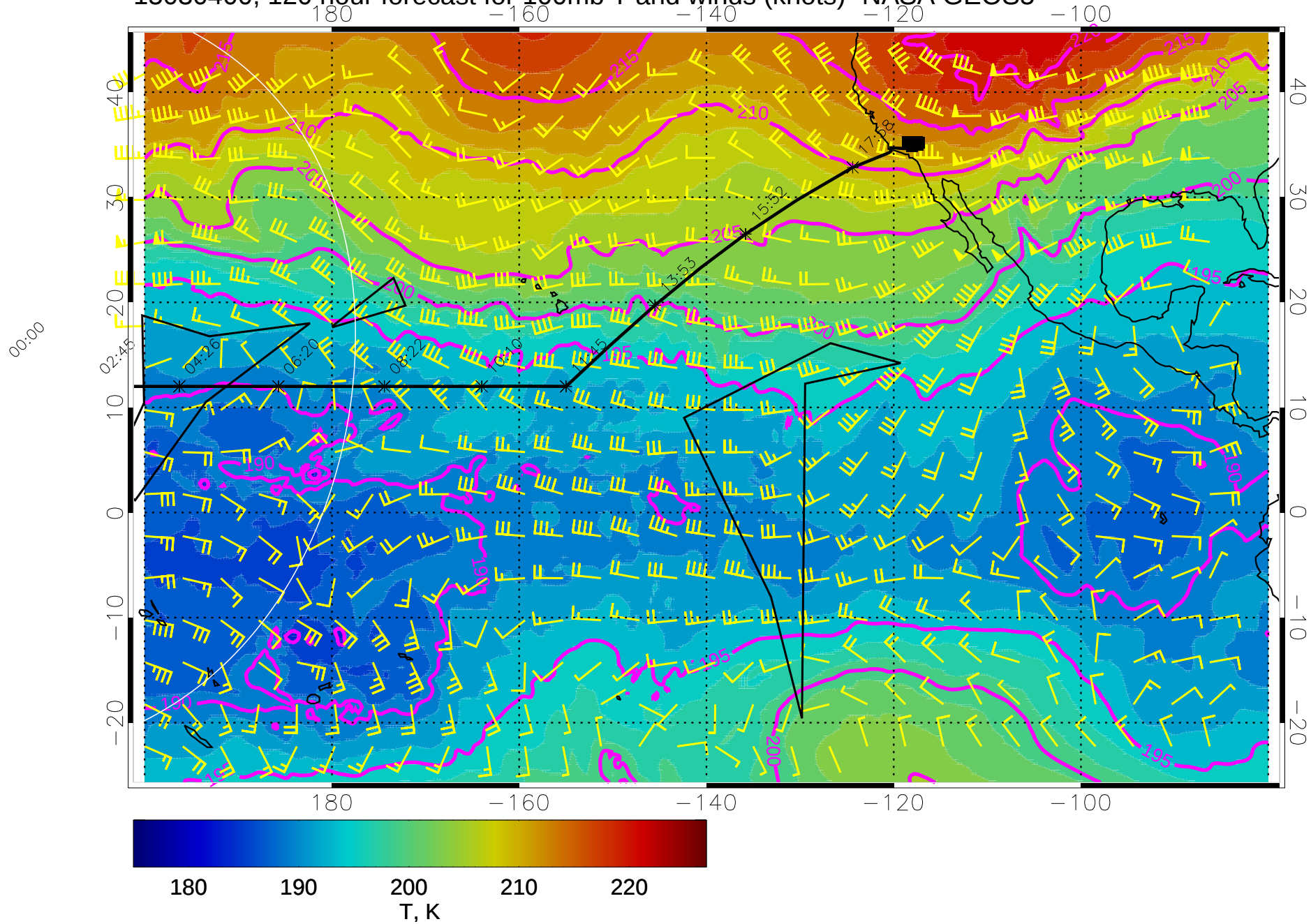
15030400, 120 hour forecast for 100mb T and winds (knots)- NASA GEOS5
