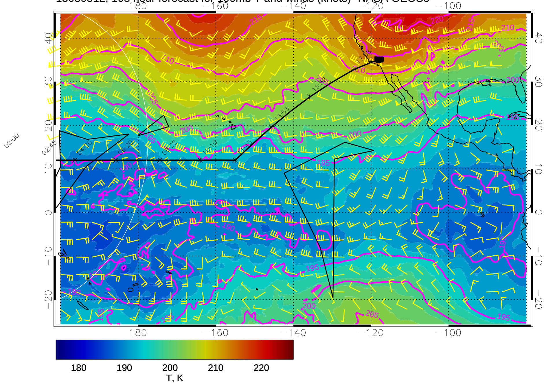
15030312, 108 hour forecast for 100mb T and winds (knots)- NASA GEOS5
