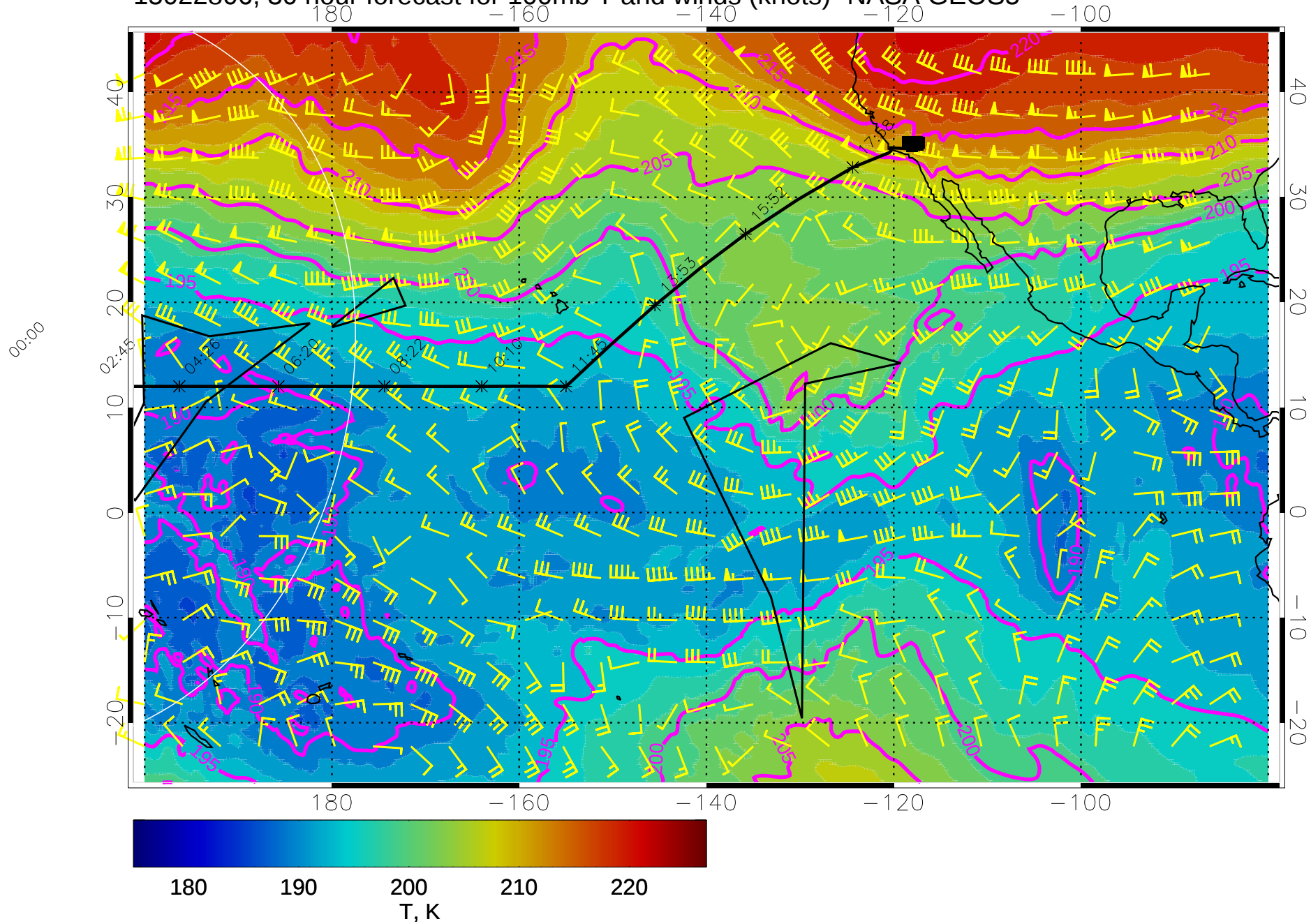
15022806, 30 hour forecast for 100mb T and winds (knots)- NASA GEOS5
