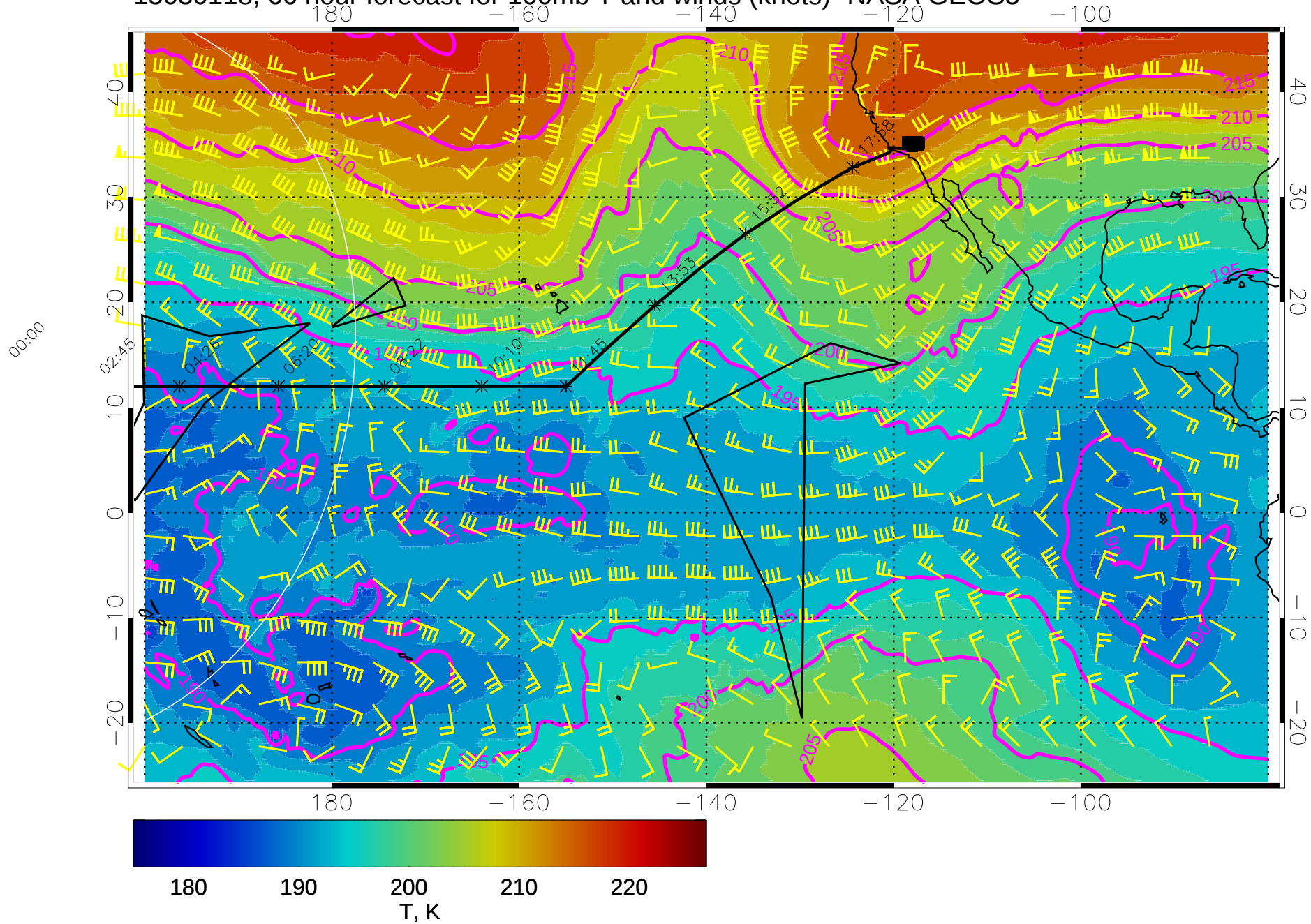
15030118, 66 hour forecast for 100mb T and winds (knots)- NASA GEOS5
