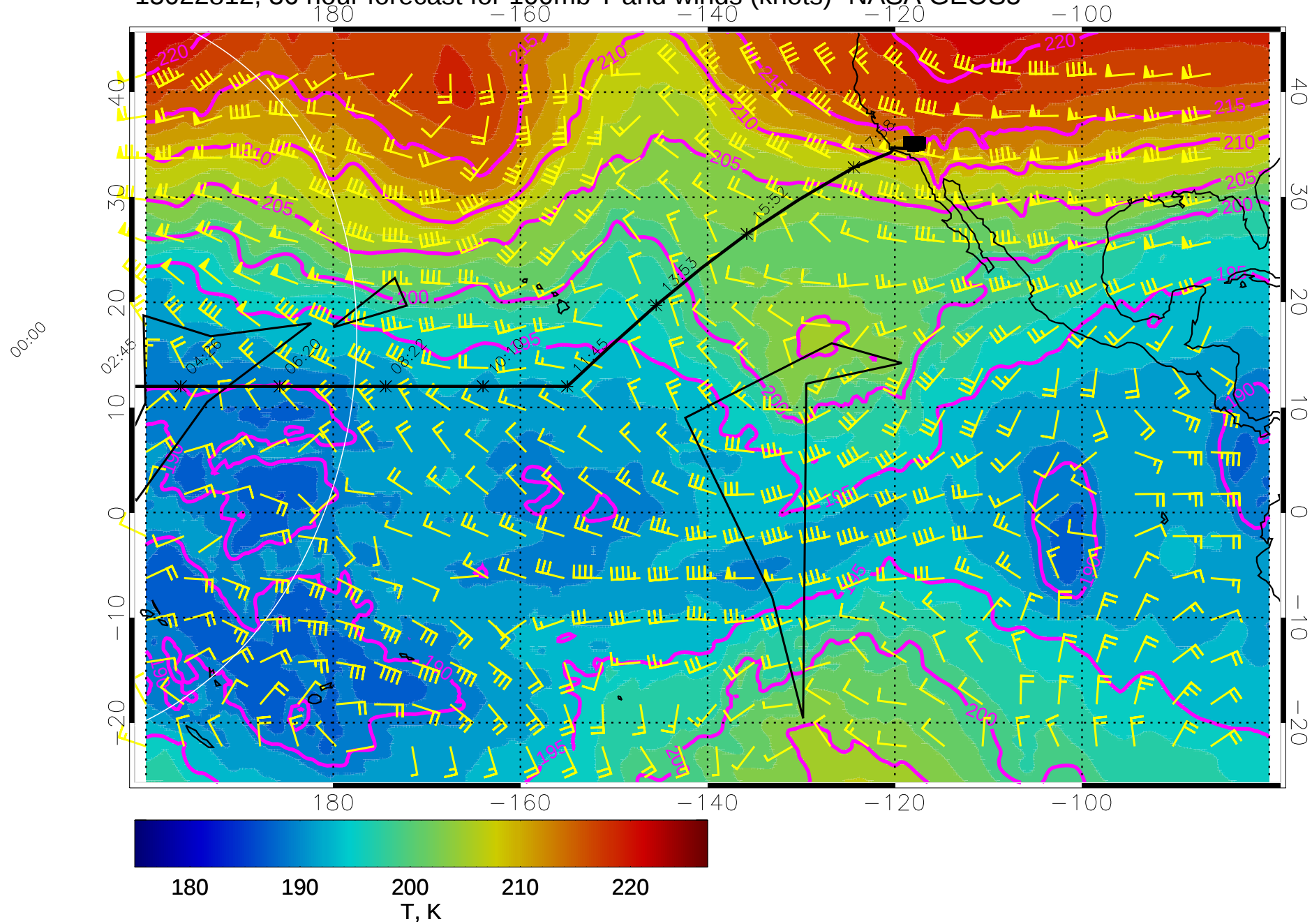
15022812, 36 hour forecast for 100mb T and winds (knots)- NASA GEOS5
