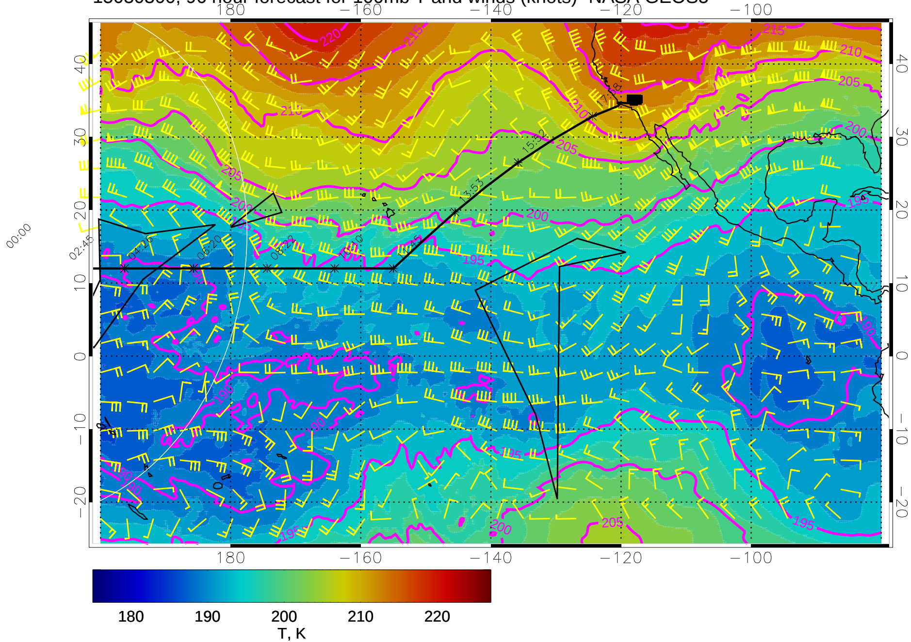
15030300, 96 hour forecast for 100mb T and winds (knots)- NASA GEOS5
