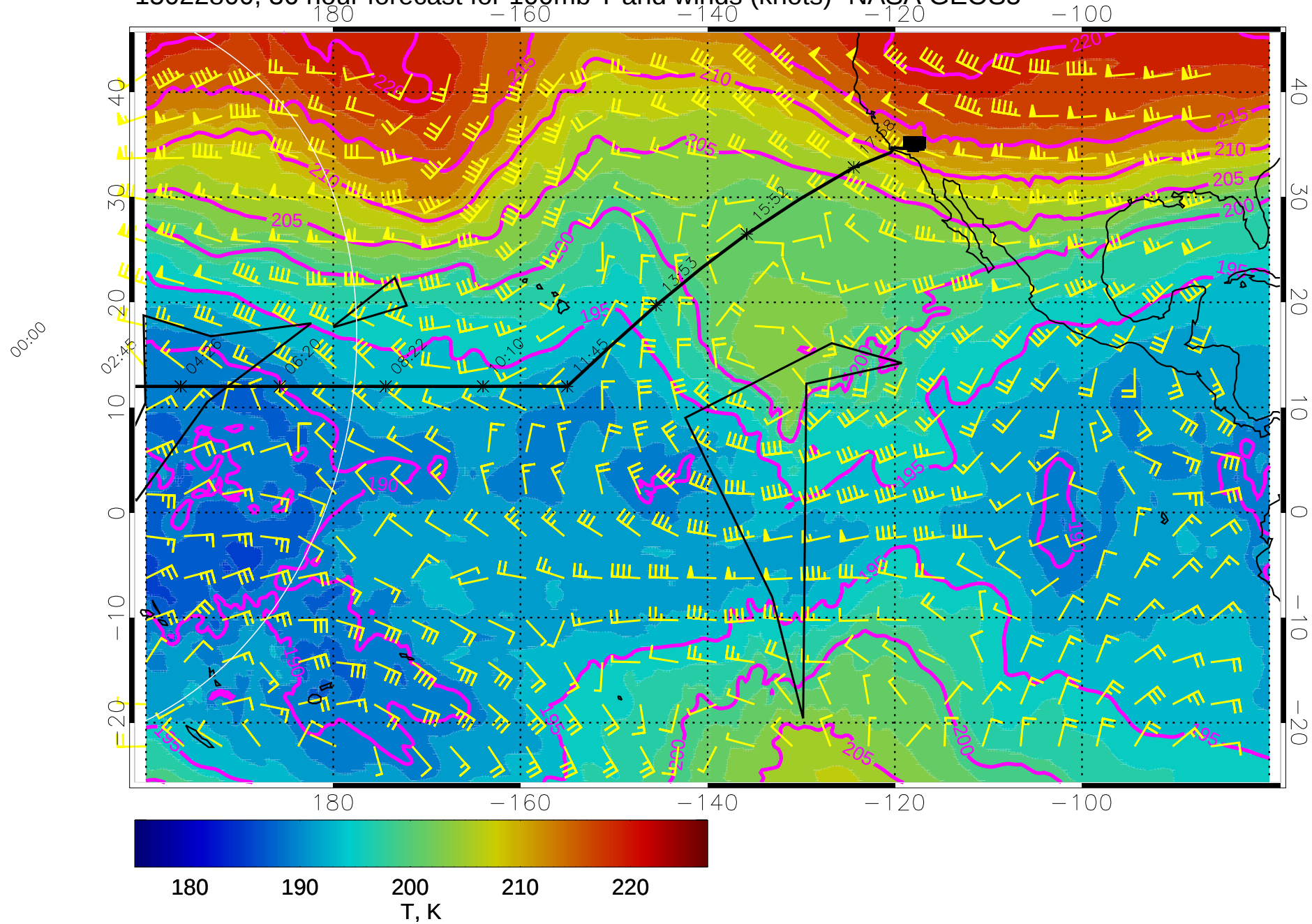
15022800, 36 hour forecast for 100mb T and winds (knots)- NASA GEOS5
