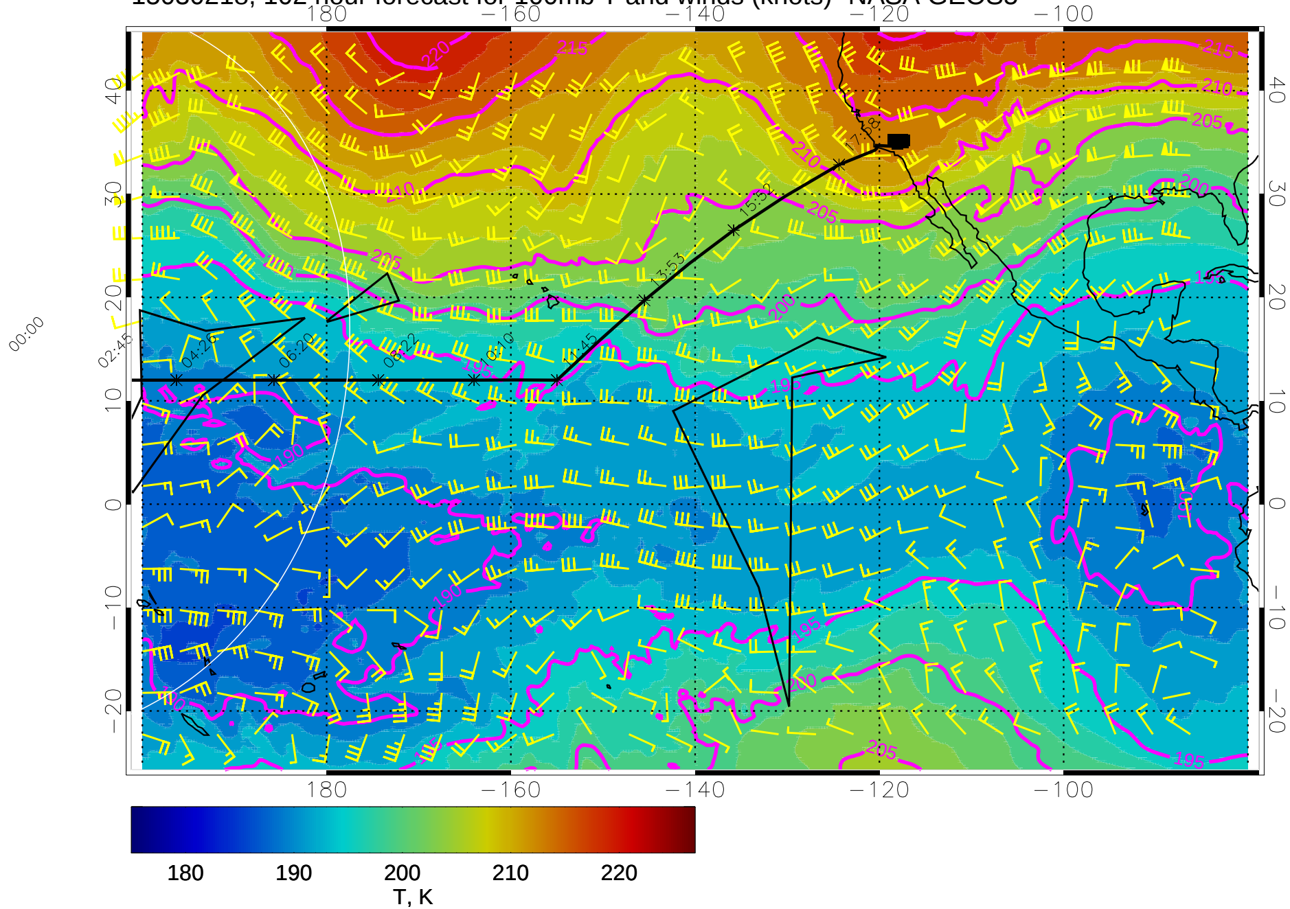
15030218, 102 hour forecast for 100mb T and winds (knots)- NASA GEOS5
