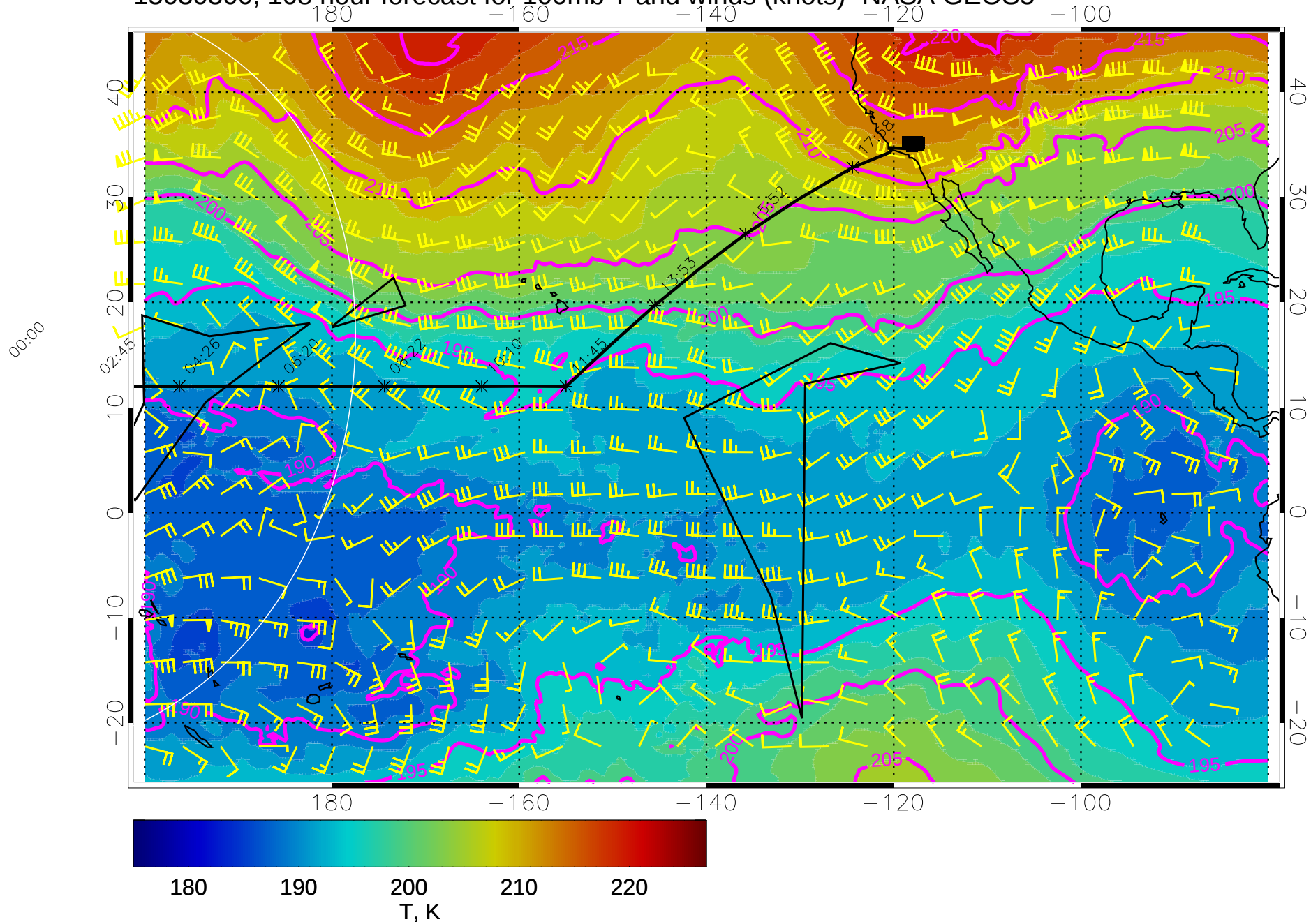
15030300, 108 hour forecast for 100mb T and winds (knots)- NASA GEOS5
