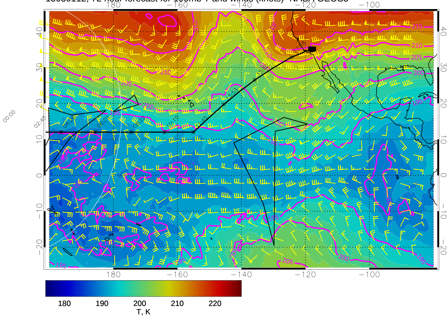
15030112, 72 hour forecast for 100mb T and winds (knots)- NASA GEOS5
