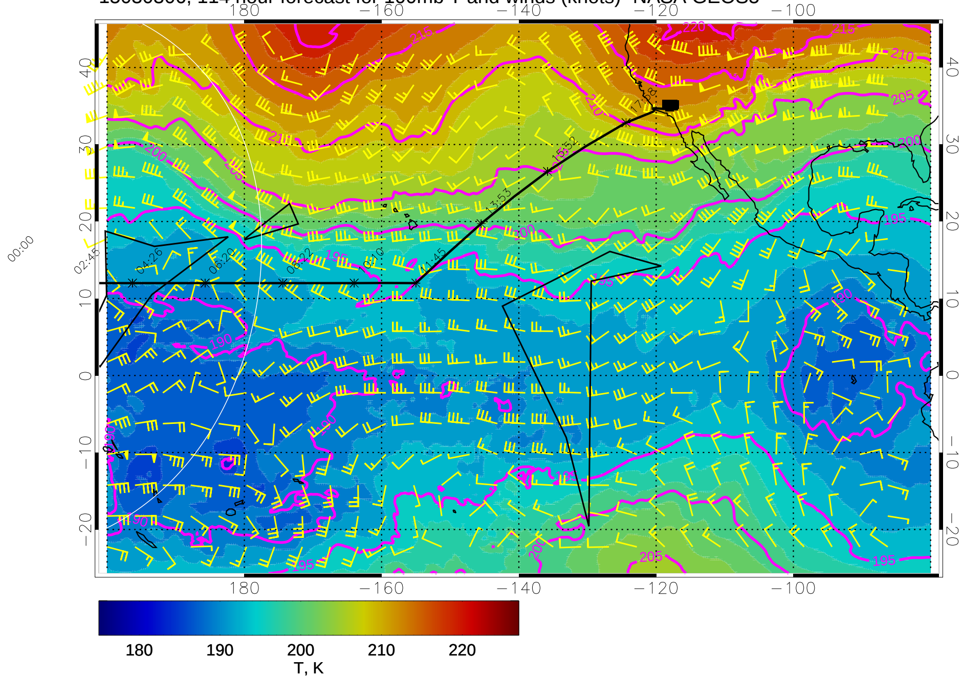
15030306, 114 hour forecast for 100mb T and winds (knots)- NASA GEOS5
