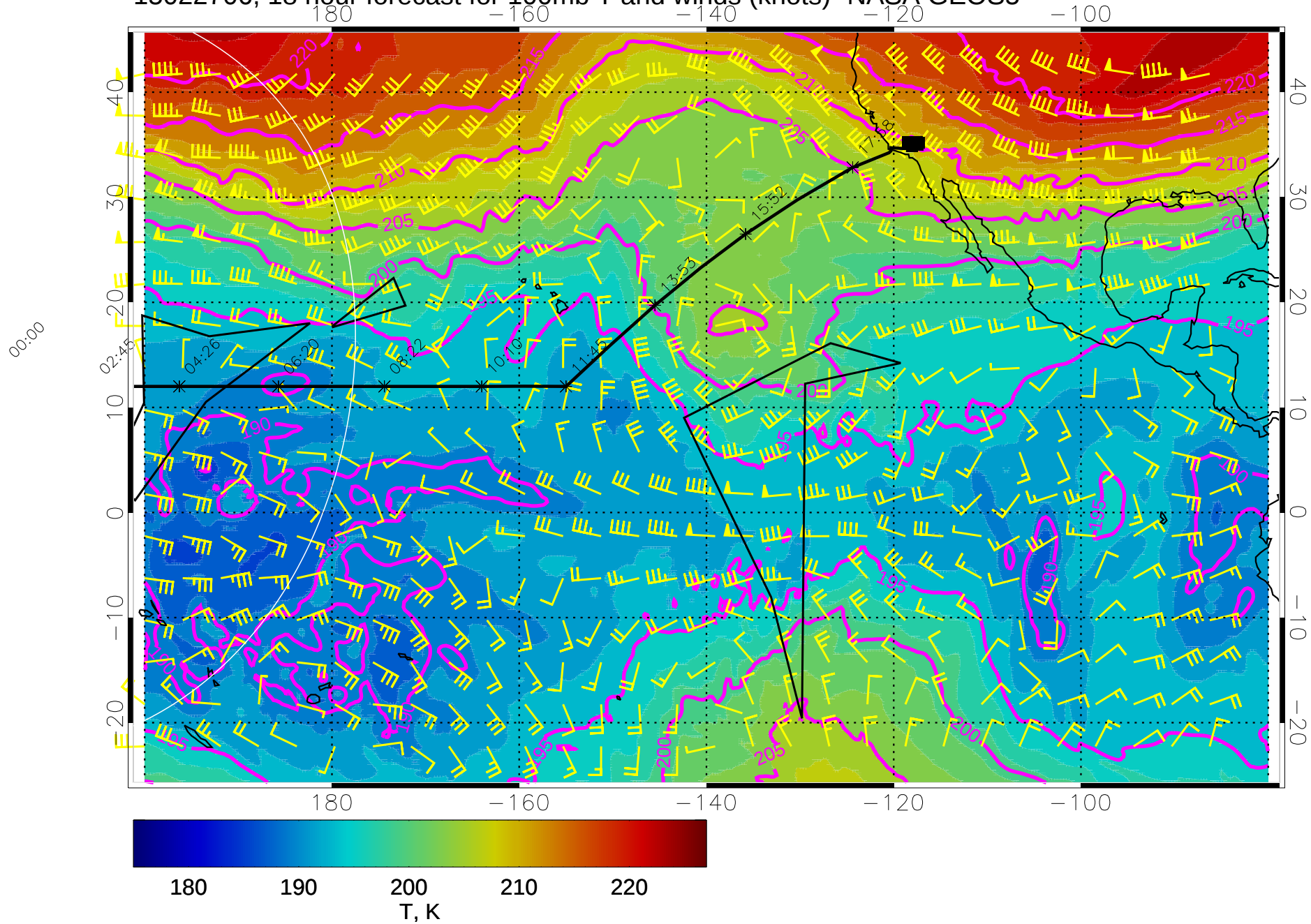
15022706, 18 hour forecast for 100mb T and winds (knots)- NASA GEOS5
