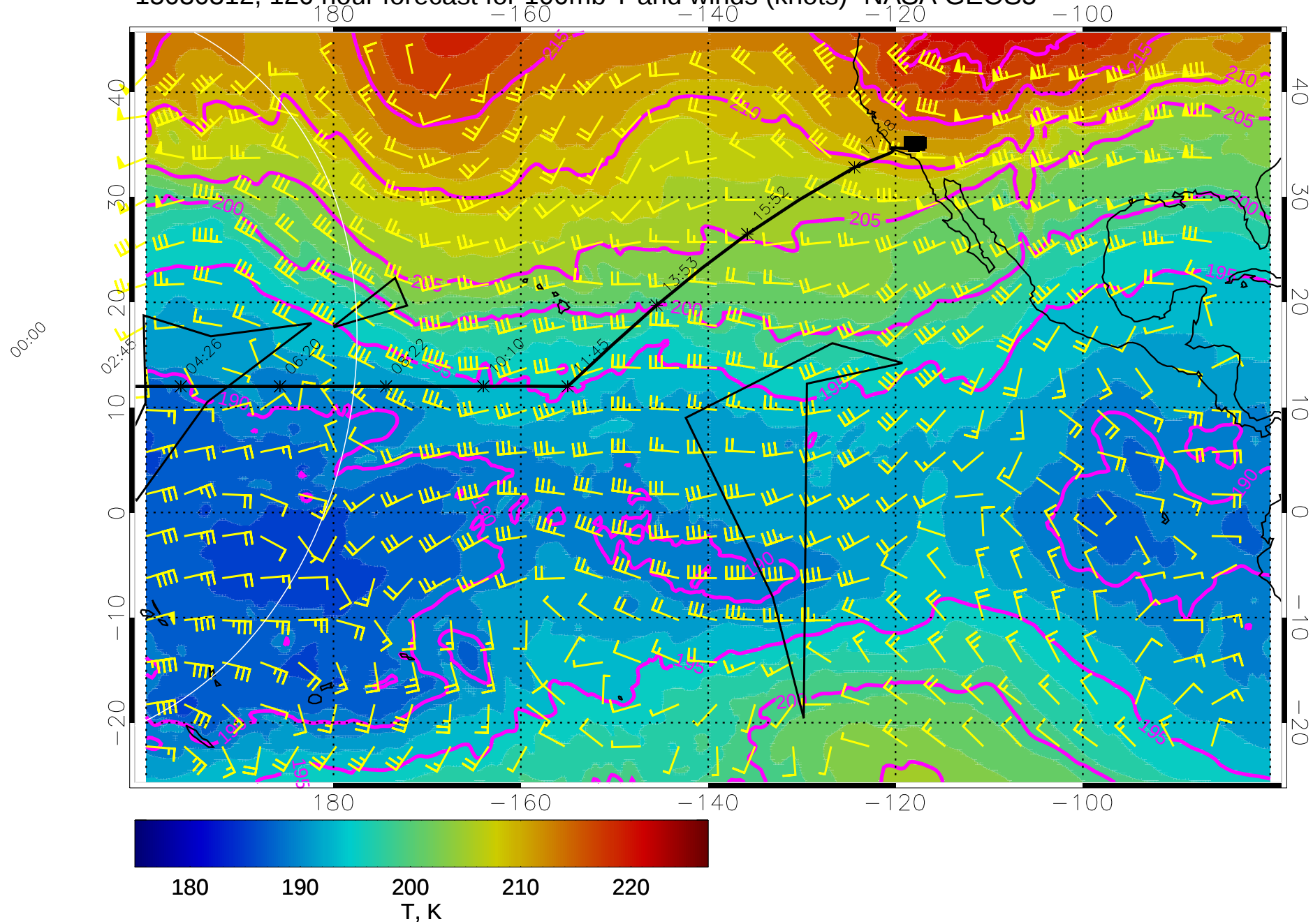
15030312, 120 hour forecast for 100mb T and winds (knots)- NASA GEOS5
