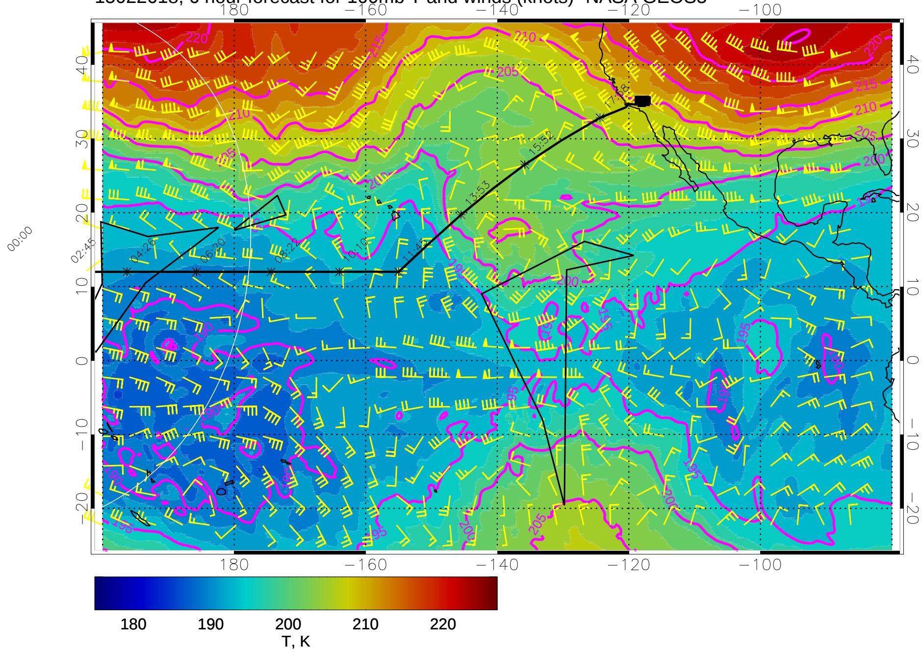
15022618, 6 hour forecast for 100mb T and winds (knots)- NASA GEOS5
