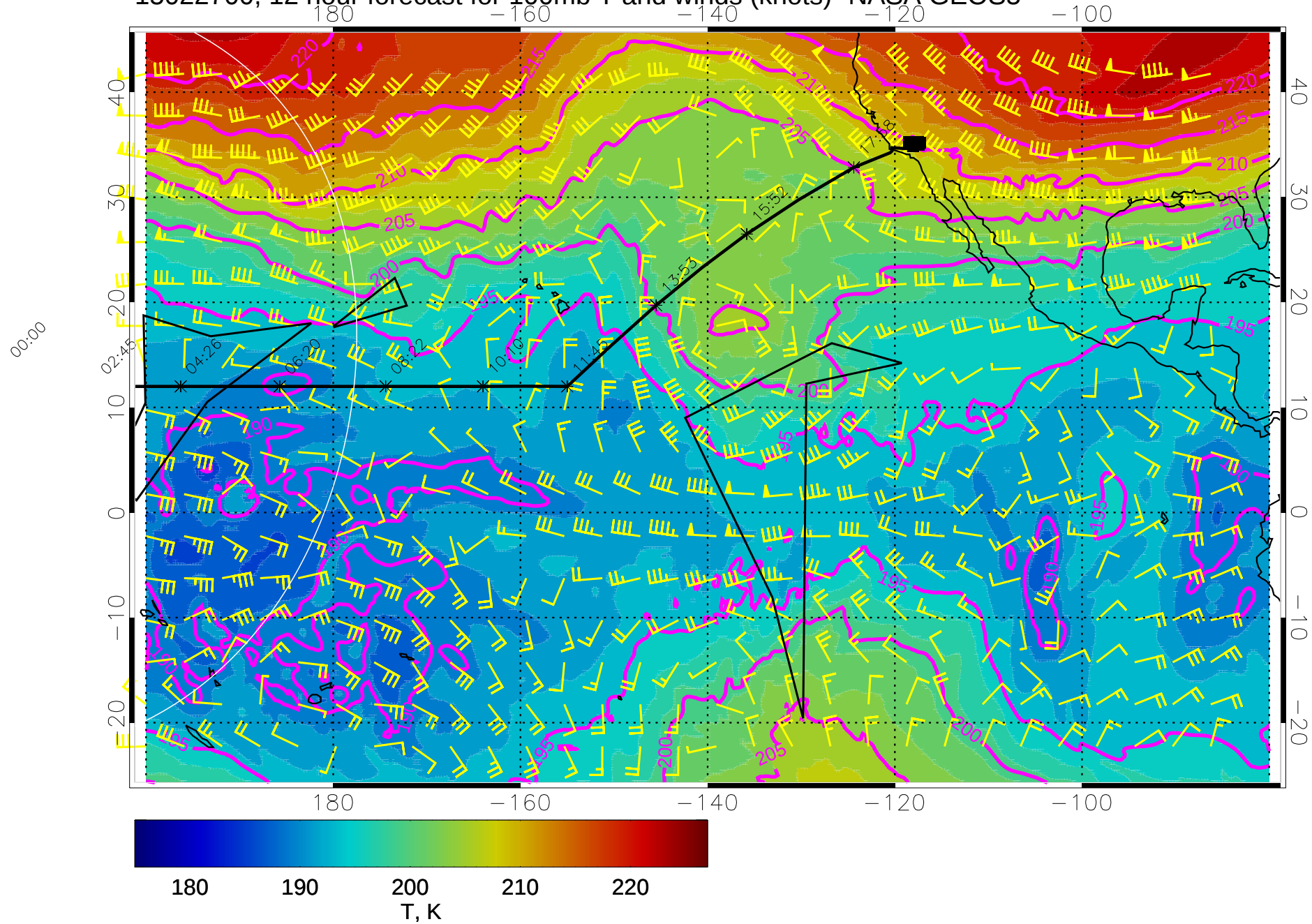
15022700, 12 hour forecast for 100mb T and winds (knots)- NASA GEOS5
