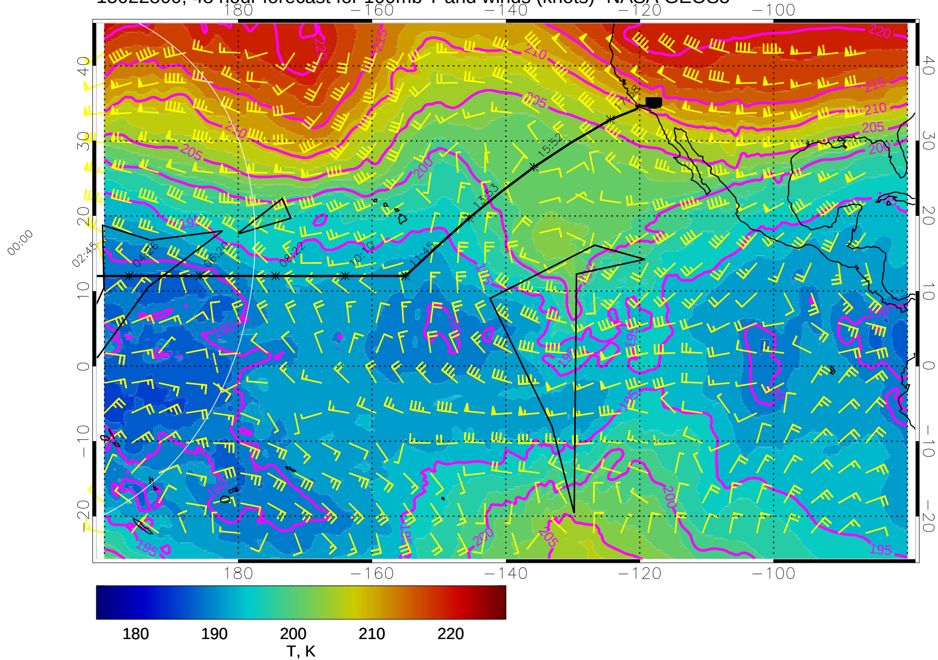
15022800, 48 hour forecast for 100mb T and winds (knots)- NASA GEOS5
