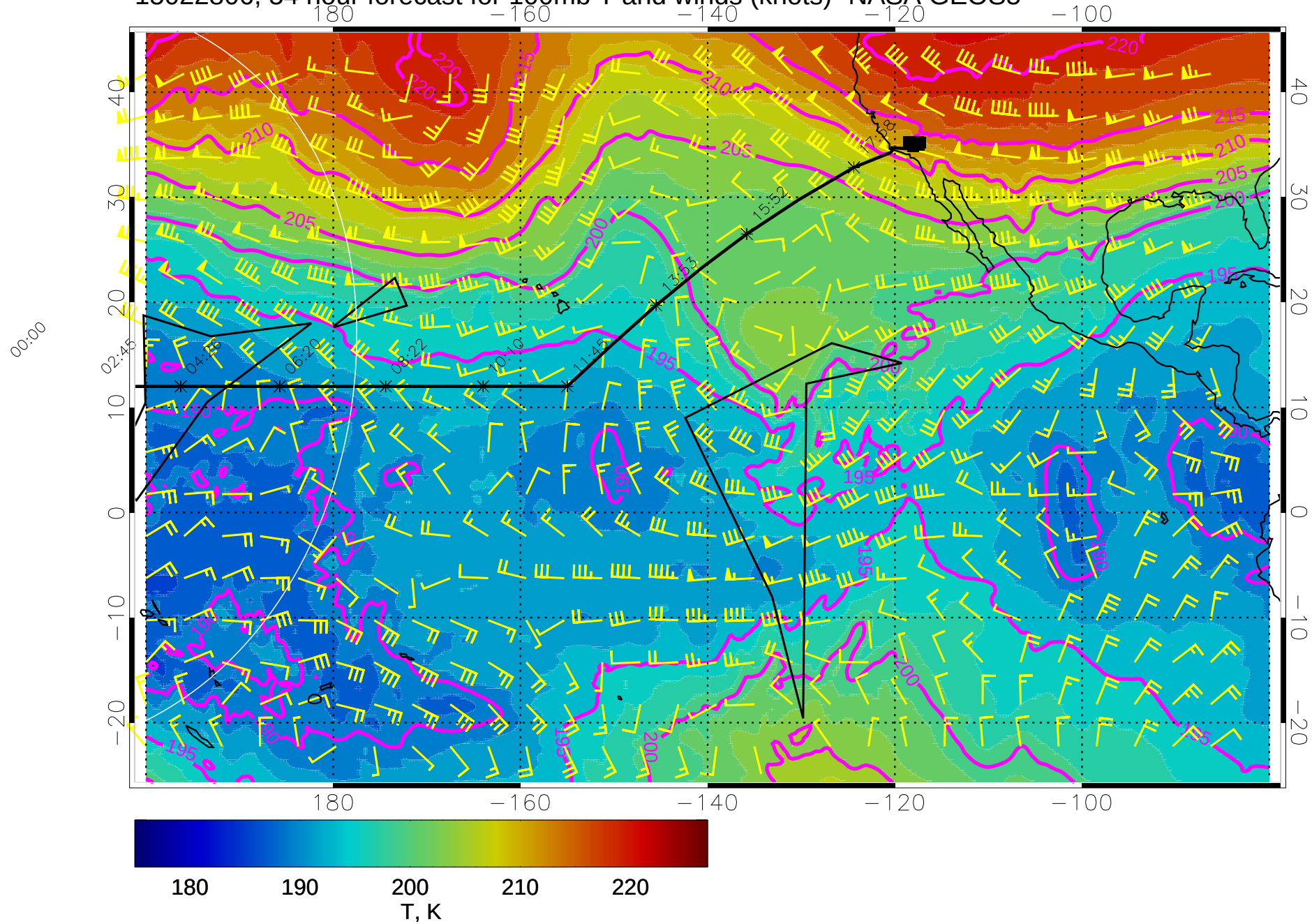
15022806, 54 hour forecast for 100mb T and winds (knots)- NASA GEOS5
