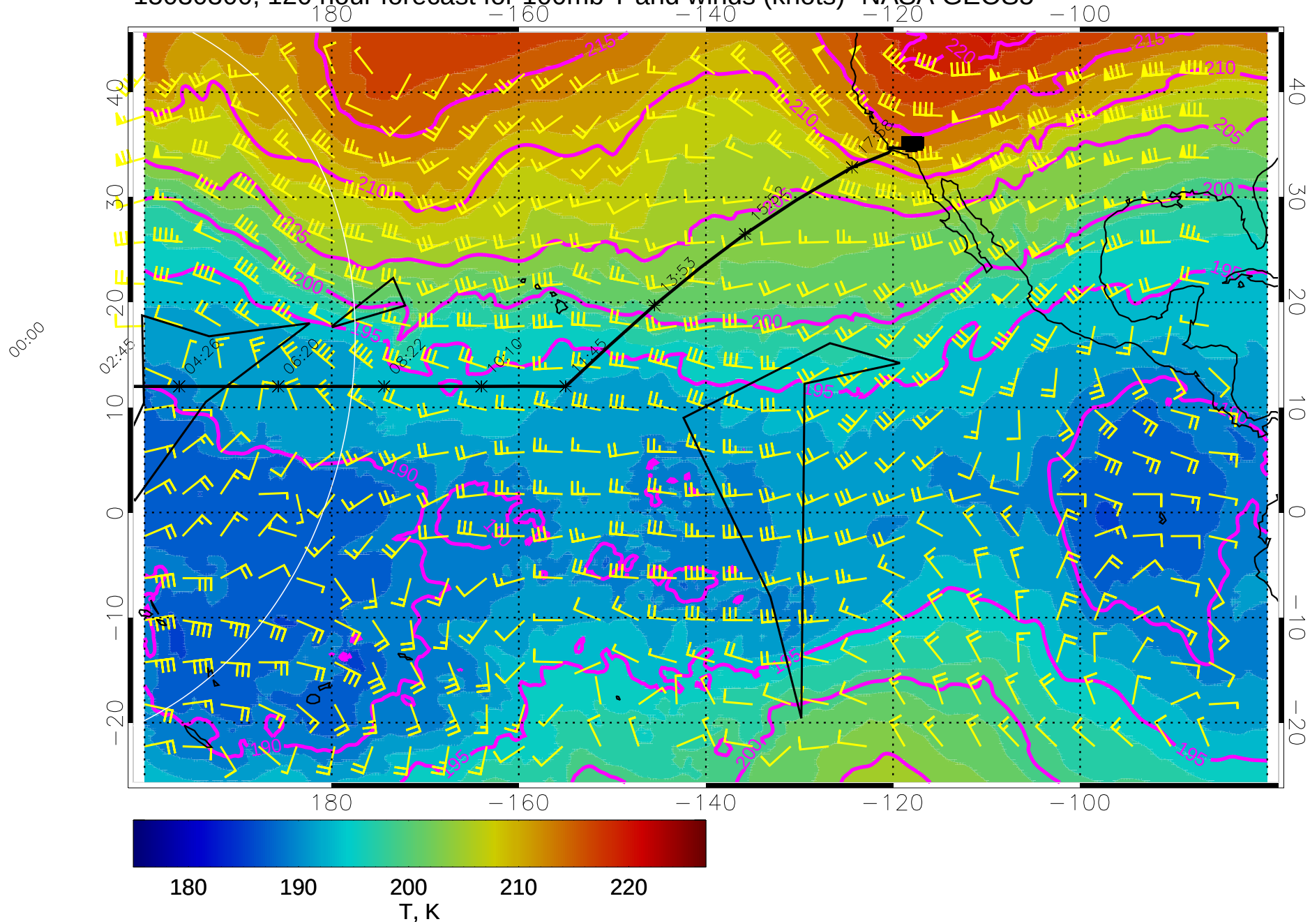
15030300, 120 hour forecast for 100mb T and winds (knots)- NASA GEOS5
