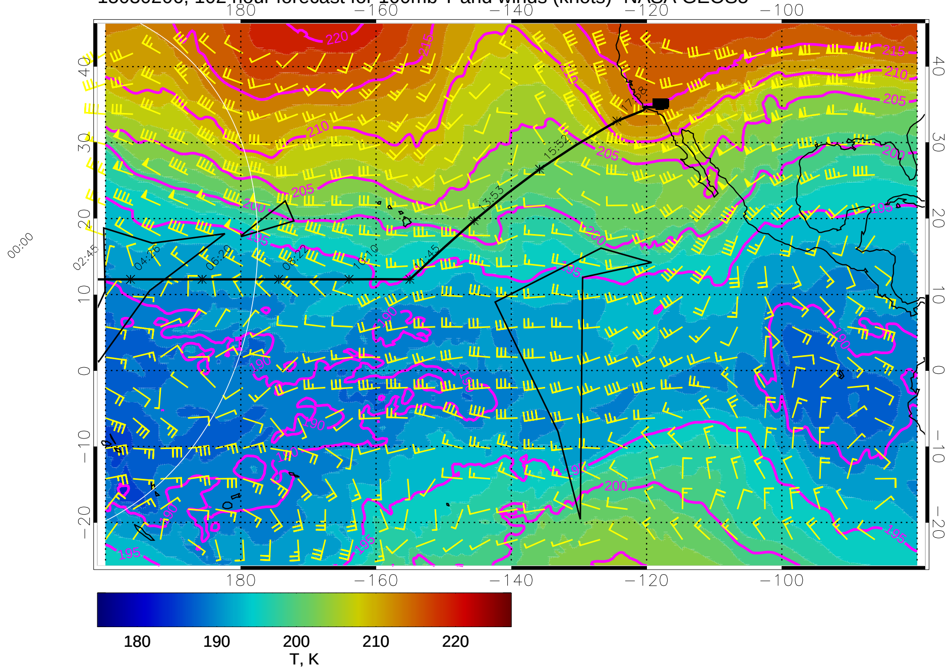
15030206, 102 hour forecast for 100mb T and winds (knots)- NASA GEOS5
