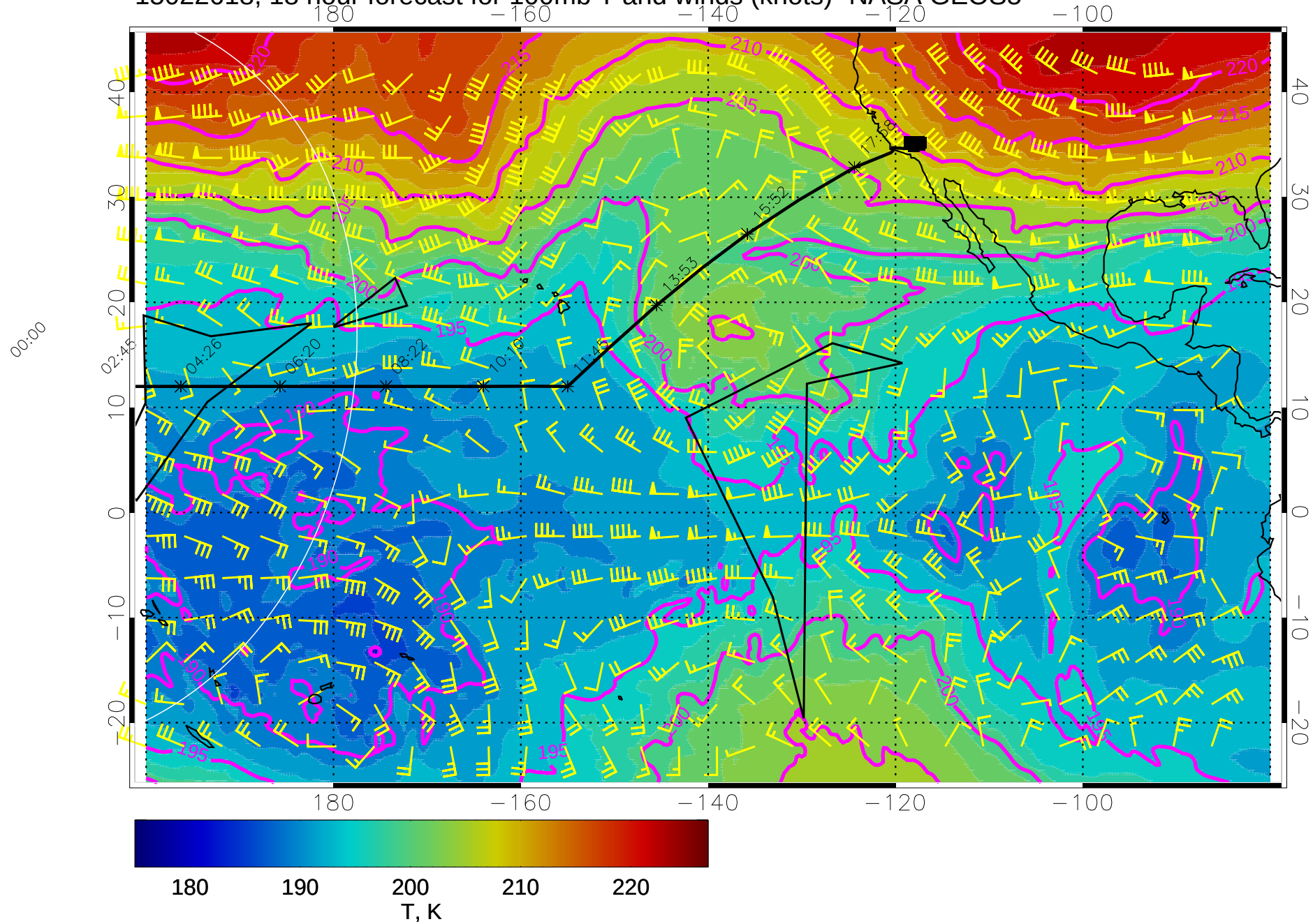
15022618, 18 hour forecast for 100mb T and winds (knots)- NASA GEOS5
