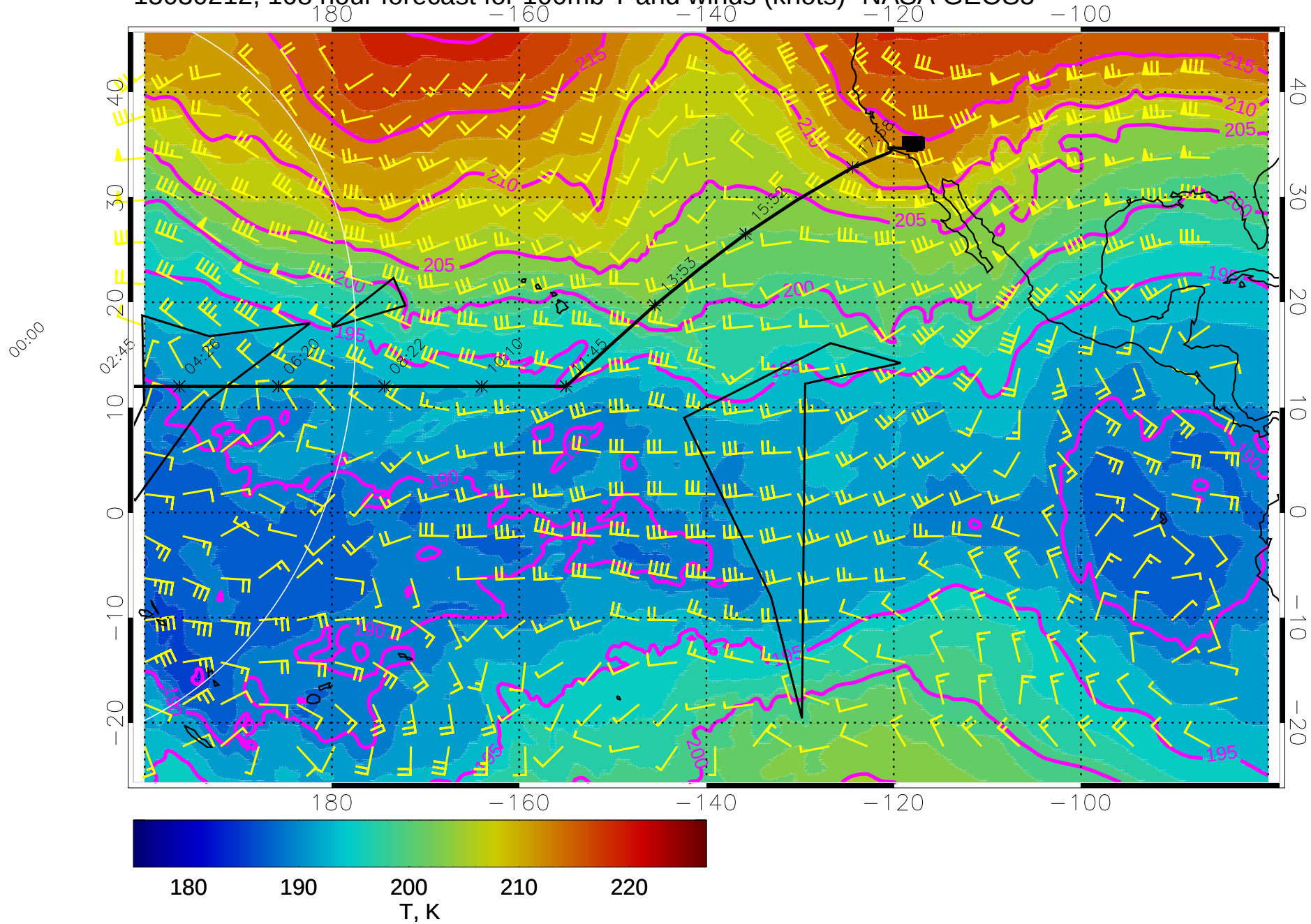
15030212, 108 hour forecast for 100mb T and winds (knots)- NASA GEOS5
