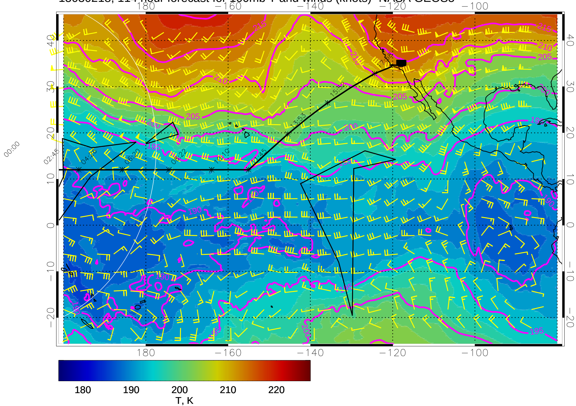
15030218, 114 hour forecast for 100mb T and winds (knots)- NASA GEOS5
