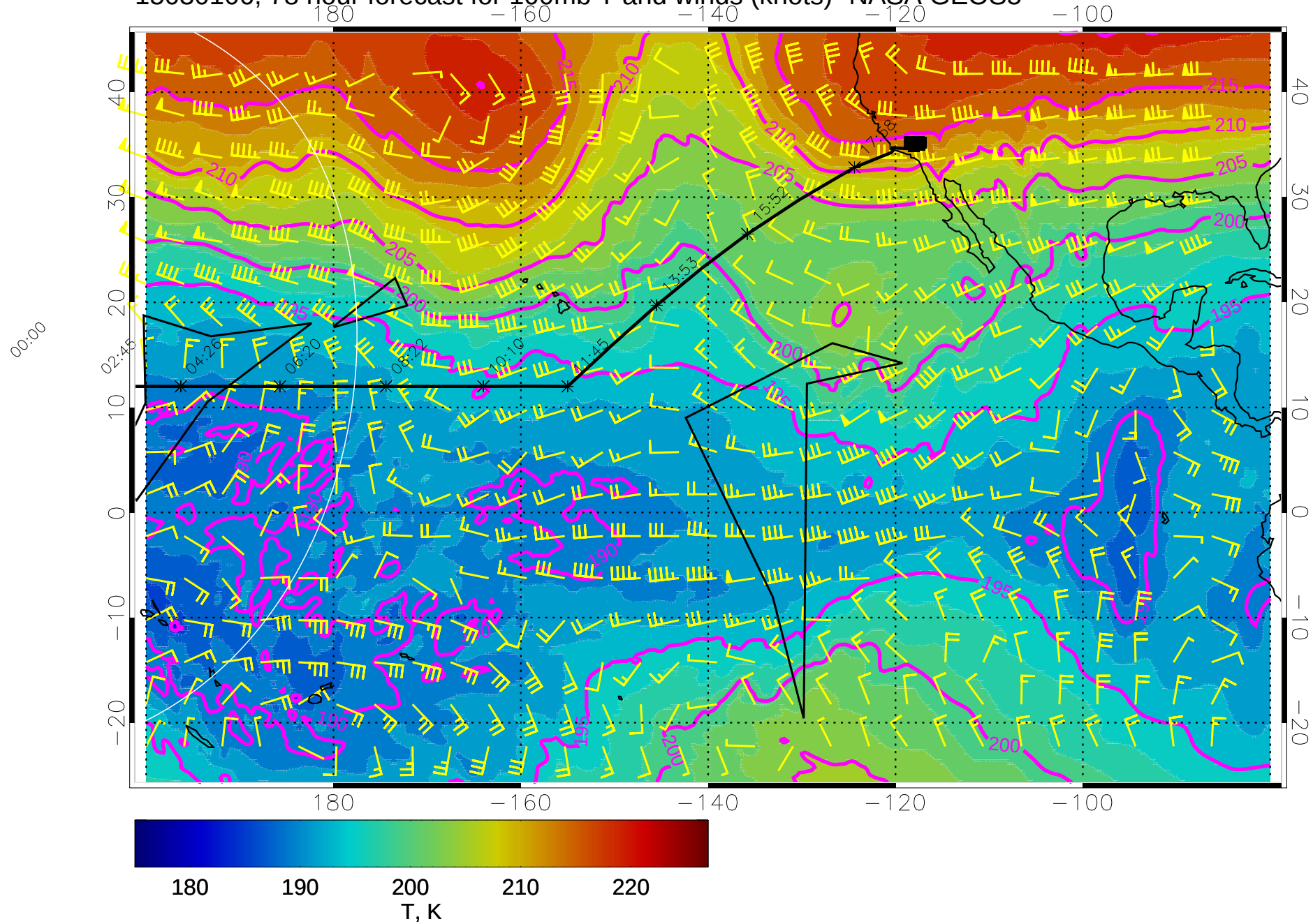
15030106, 78 hour forecast for 100mb T and winds (knots)- NASA GEOS5
