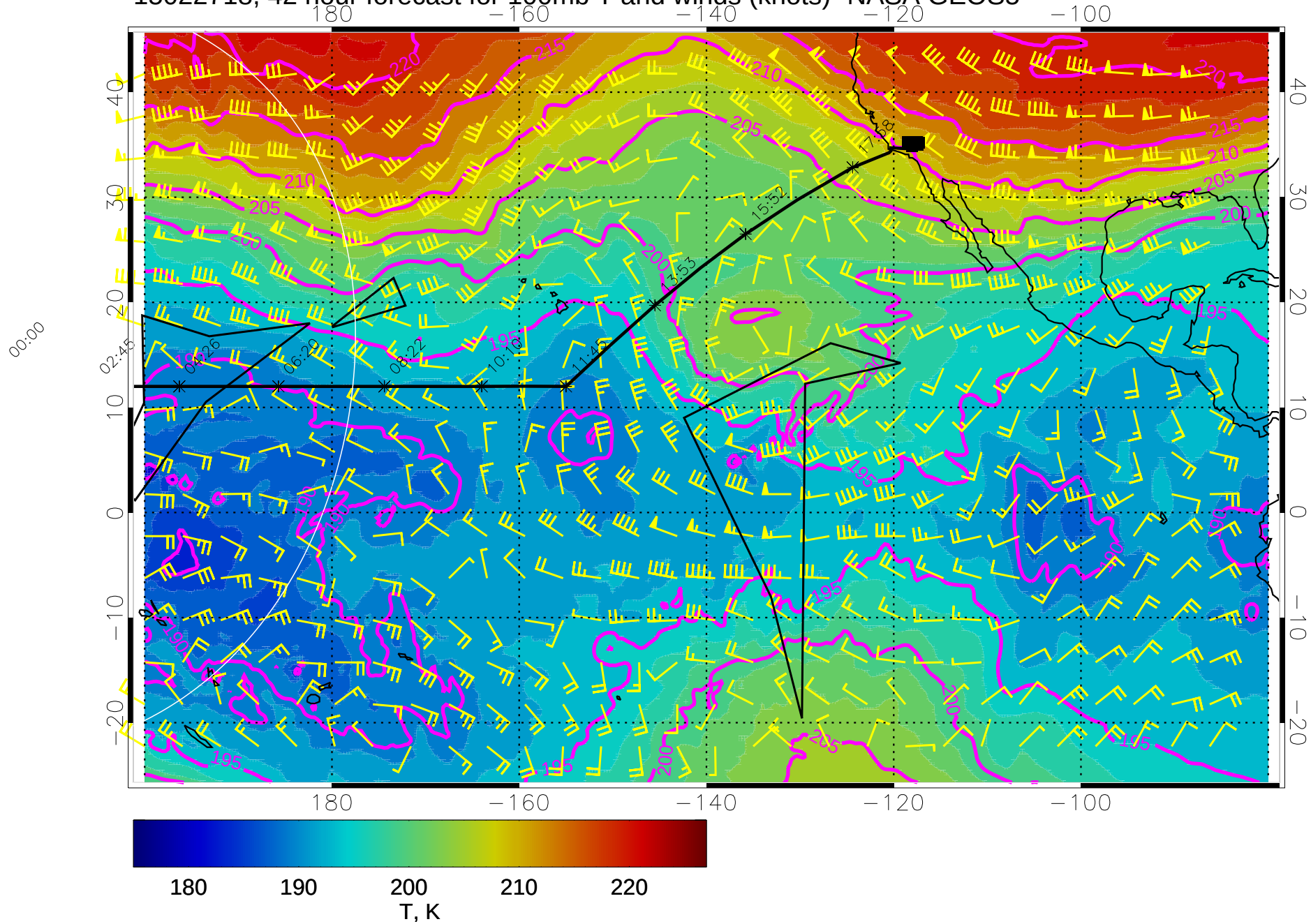
15022718, 42 hour forecast for 100mb T and winds (knots)- NASA GEOS5
