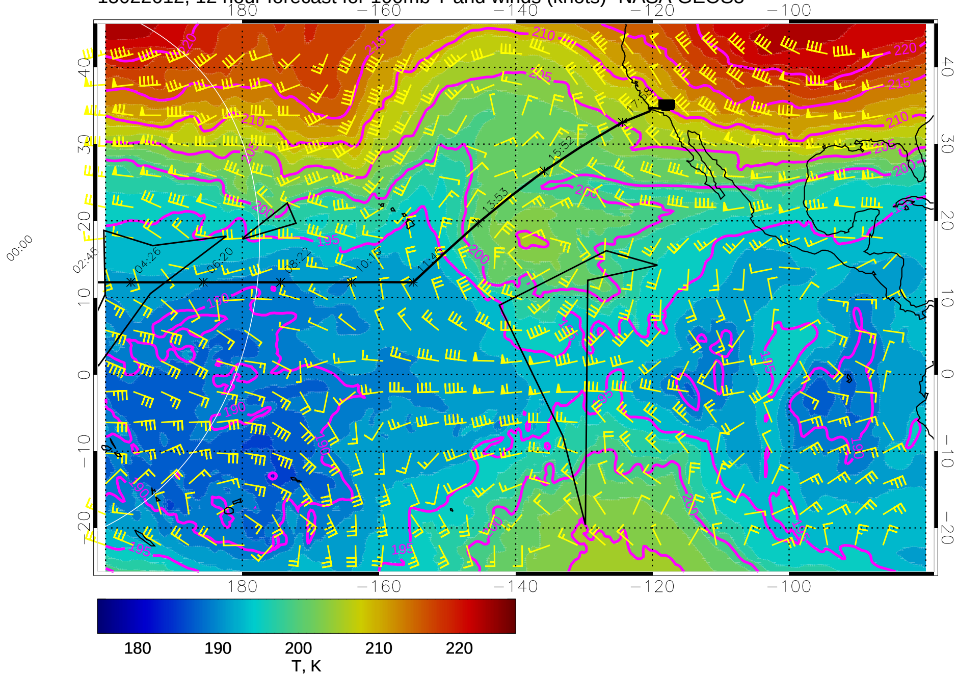
15022612, 12 hour forecast for 100mb T and winds (knots)- NASA GEOS5
