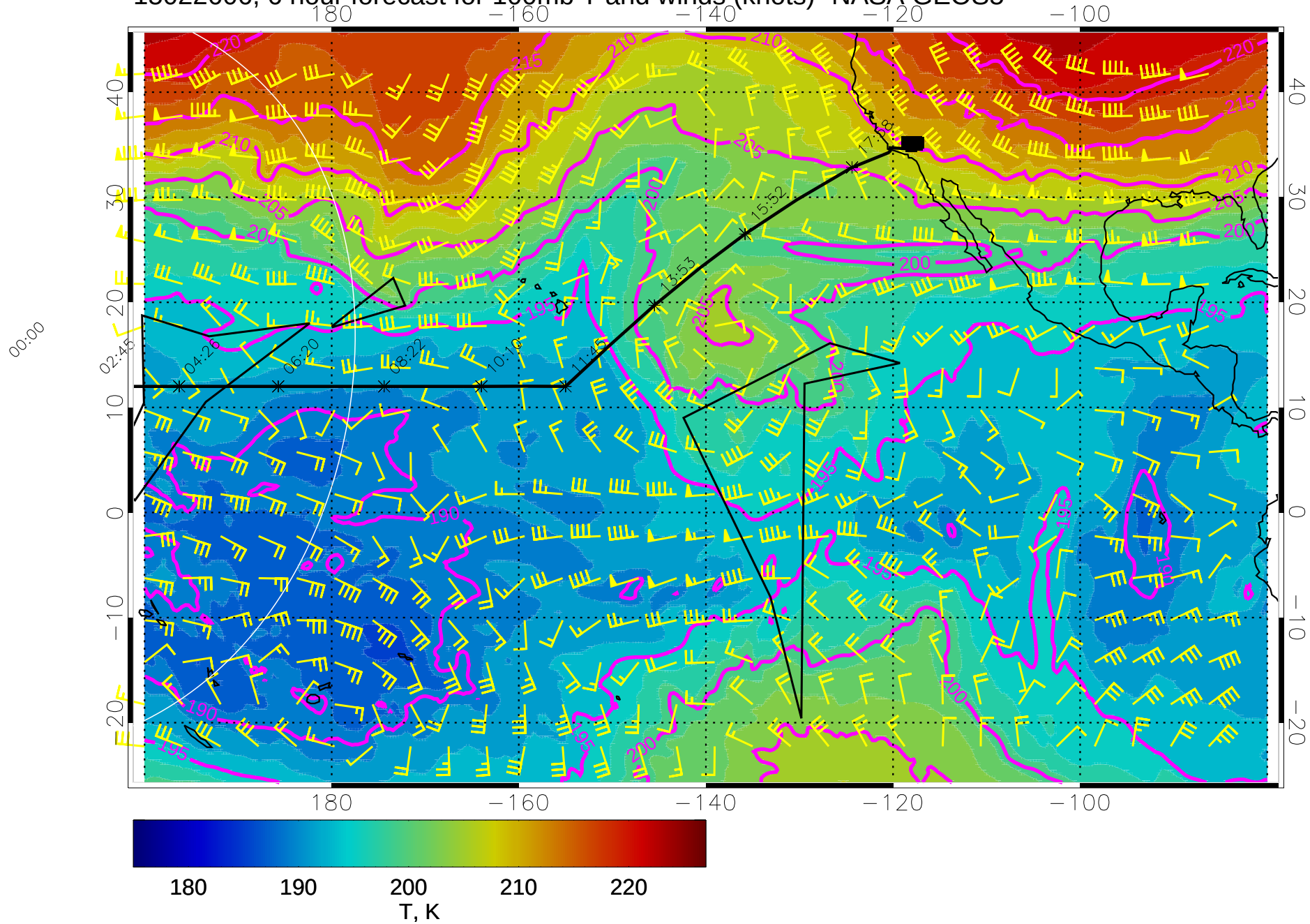
15022606, 6 hour forecast for 100mb T and winds (knots)- NASA GEOS5
