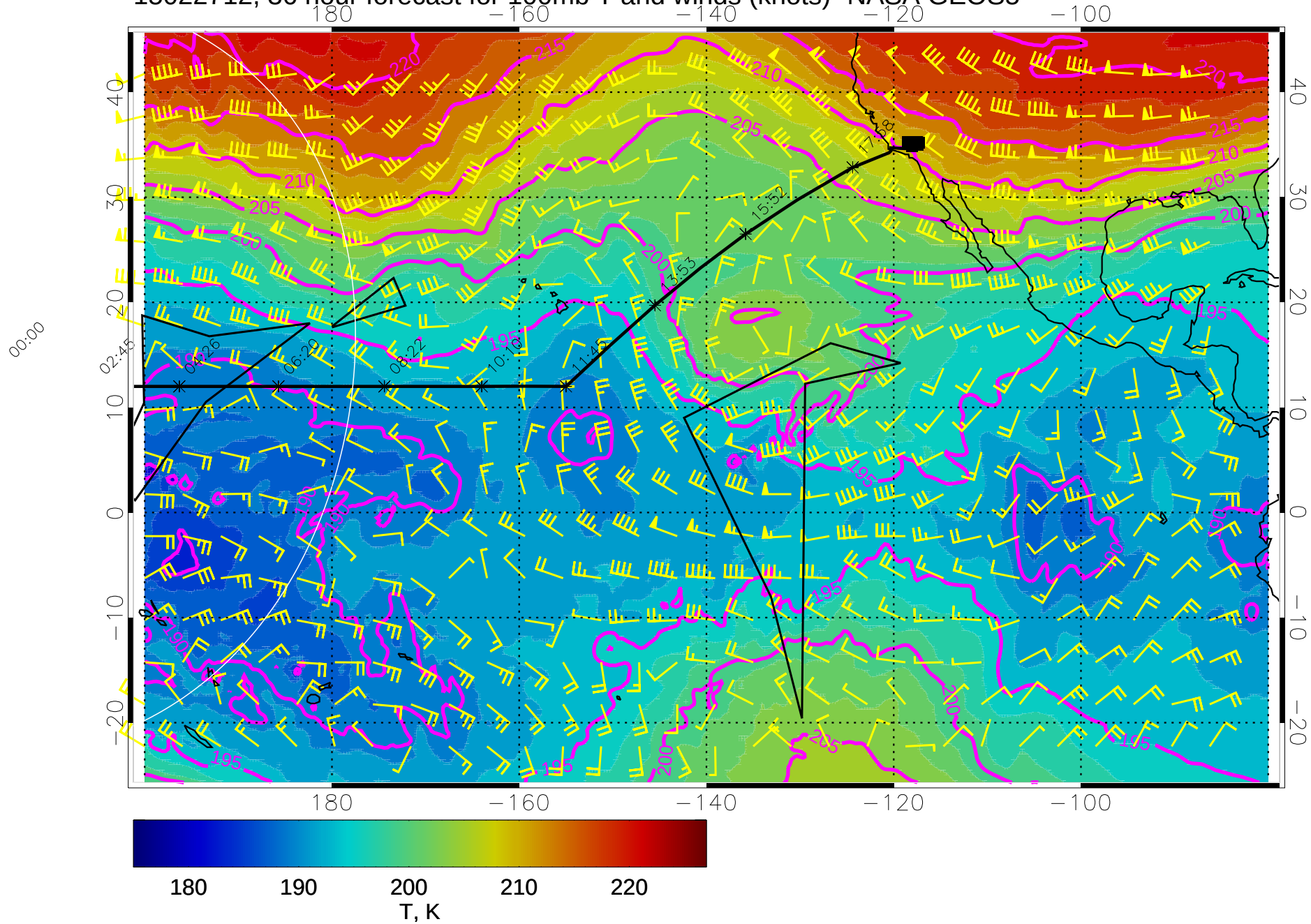
15022712, 36 hour forecast for 100mb T and winds (knots)- NASA GEOS5
