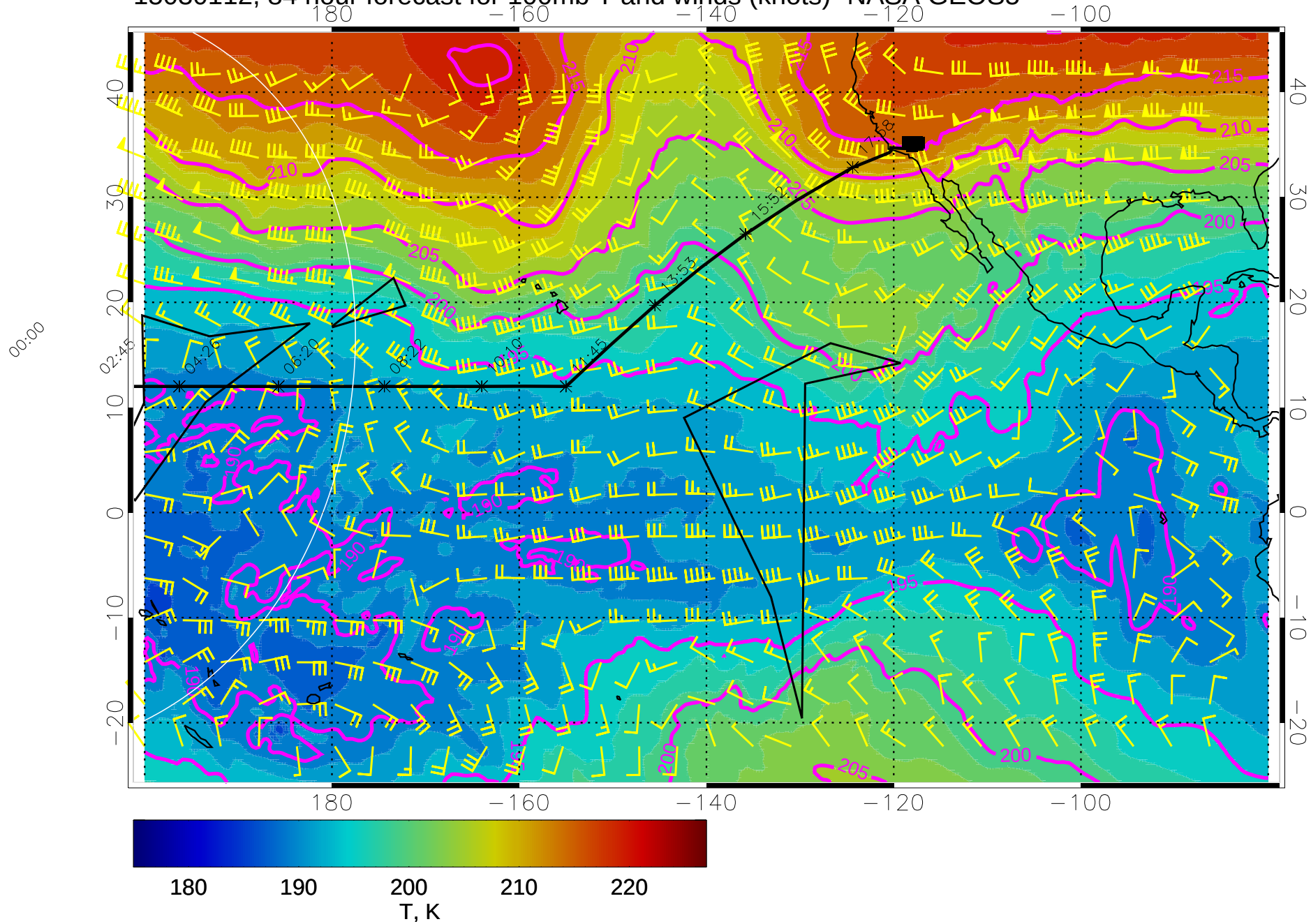
15030112, 84 hour forecast for 100mb T and winds (knots)- NASA GEOS5
