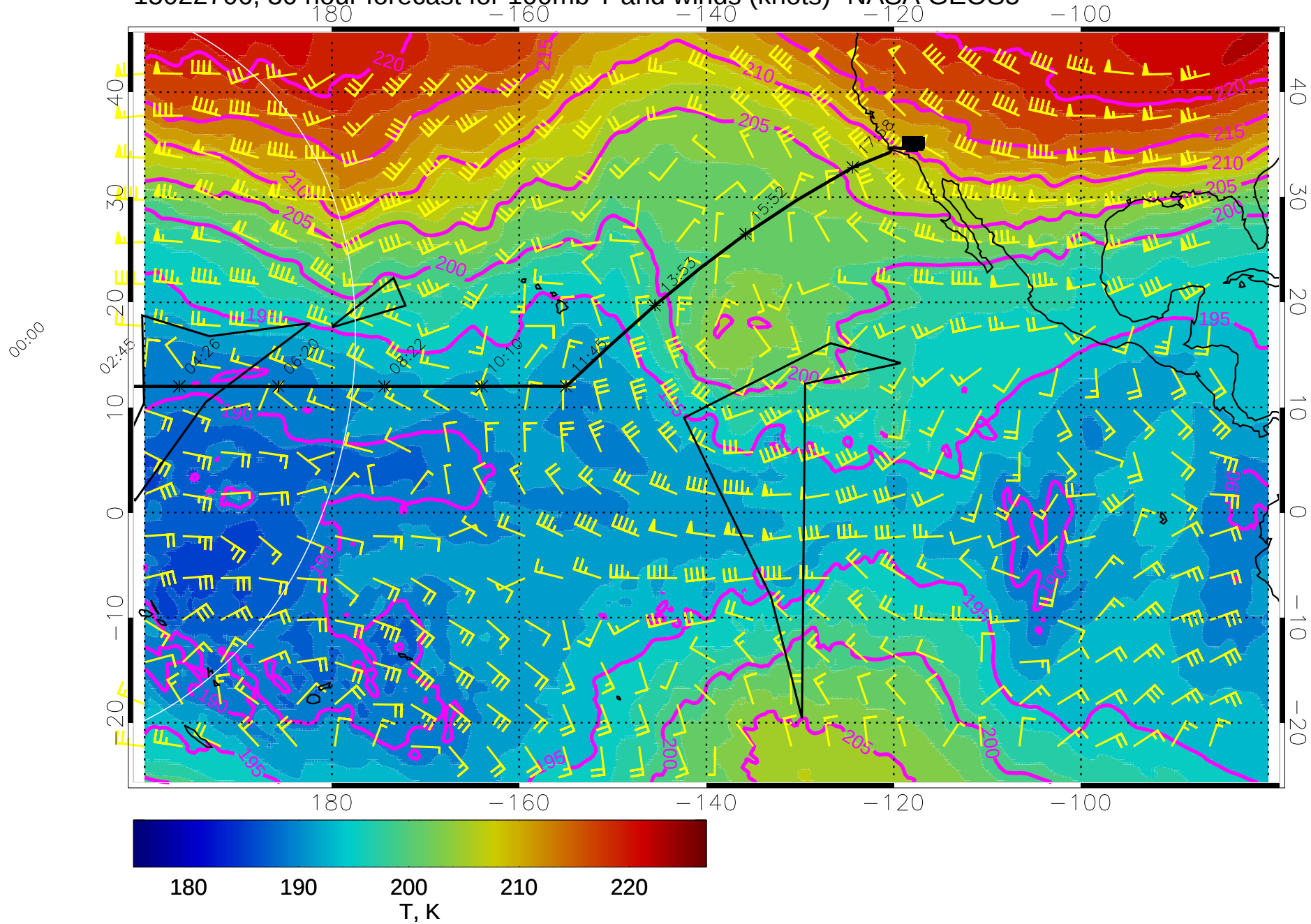
15022706, 30 hour forecast for 100mb T and winds (knots)- NASA GEOS5
