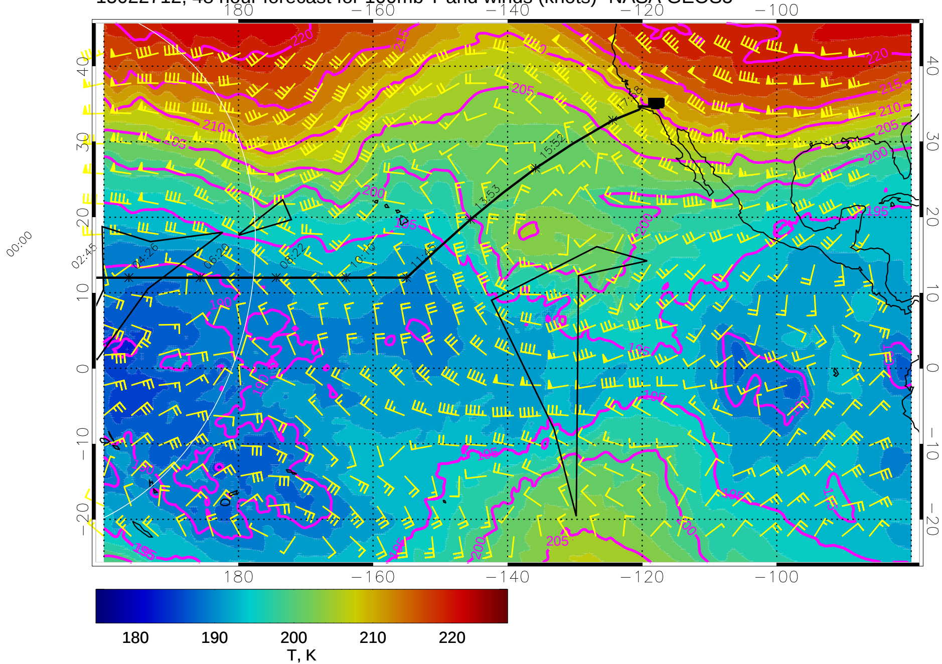
15022712, 48 hour forecast for 100mb T and winds (knots)- NASA GEOS5
