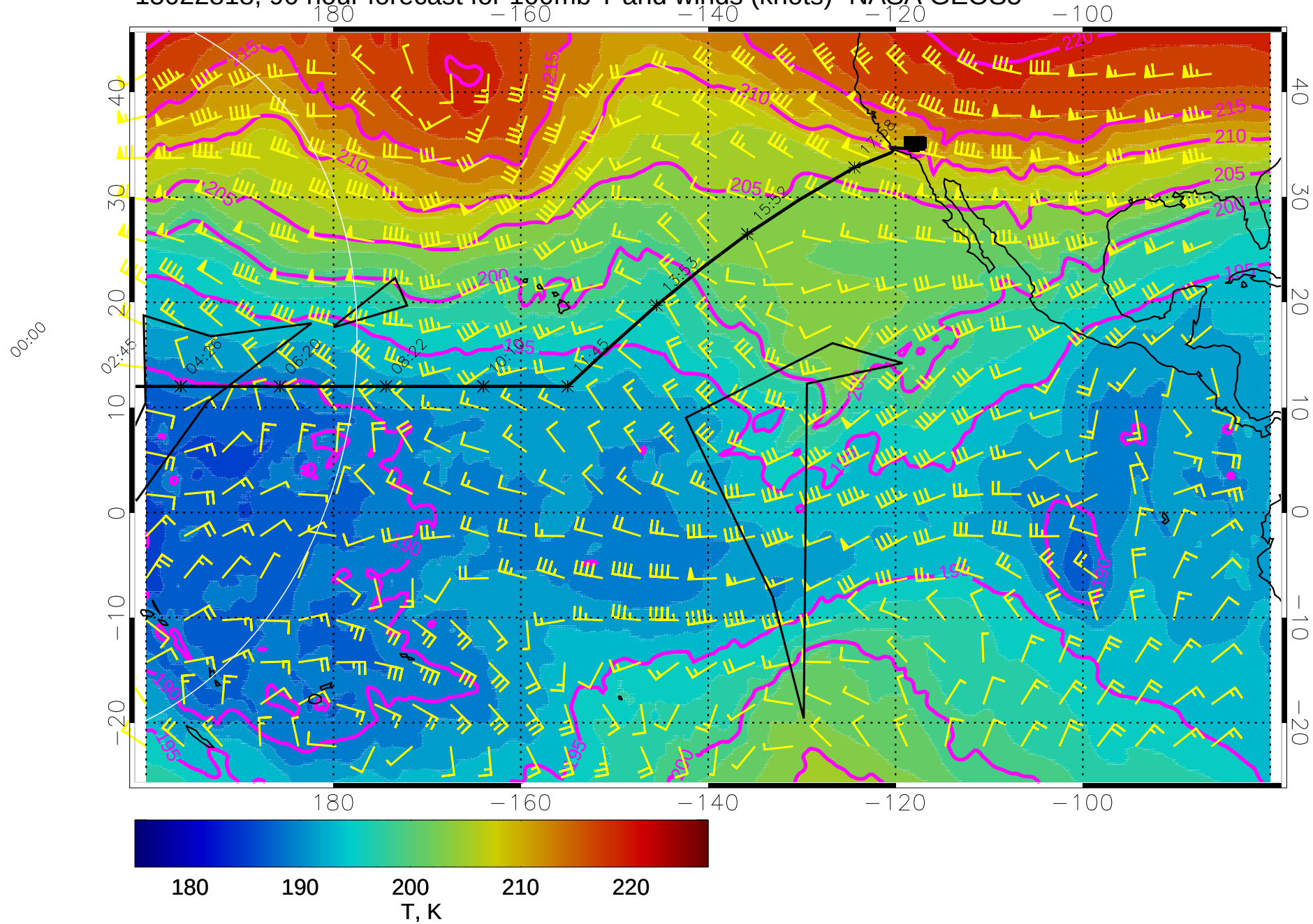
15022818, 90 hour forecast for 100mb T and winds (knots)- NASA GEOS5
