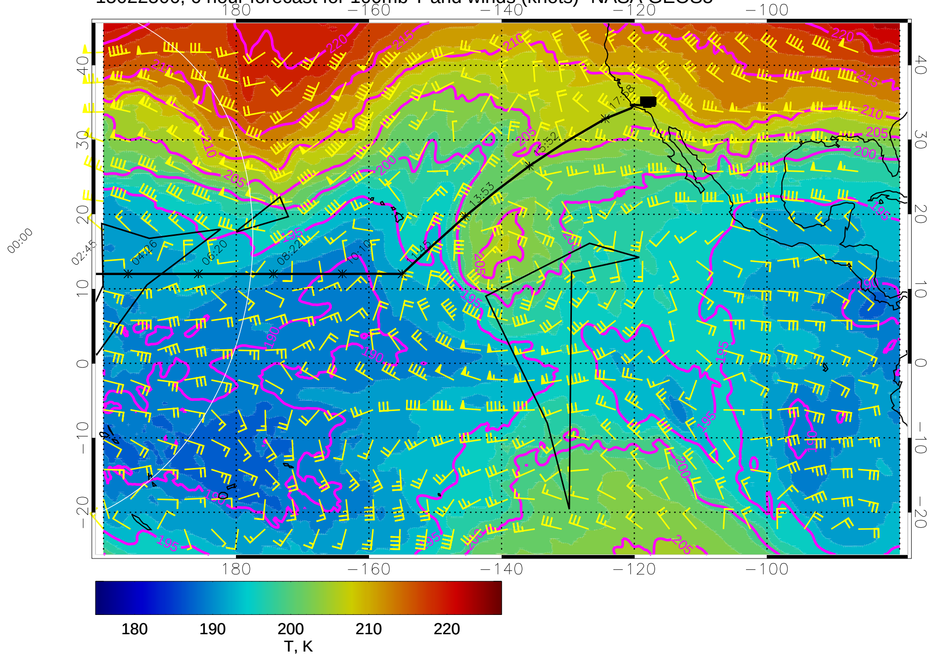
15022506, 6 hour forecast for 100mb T and winds (knots)- NASA GEOS5
