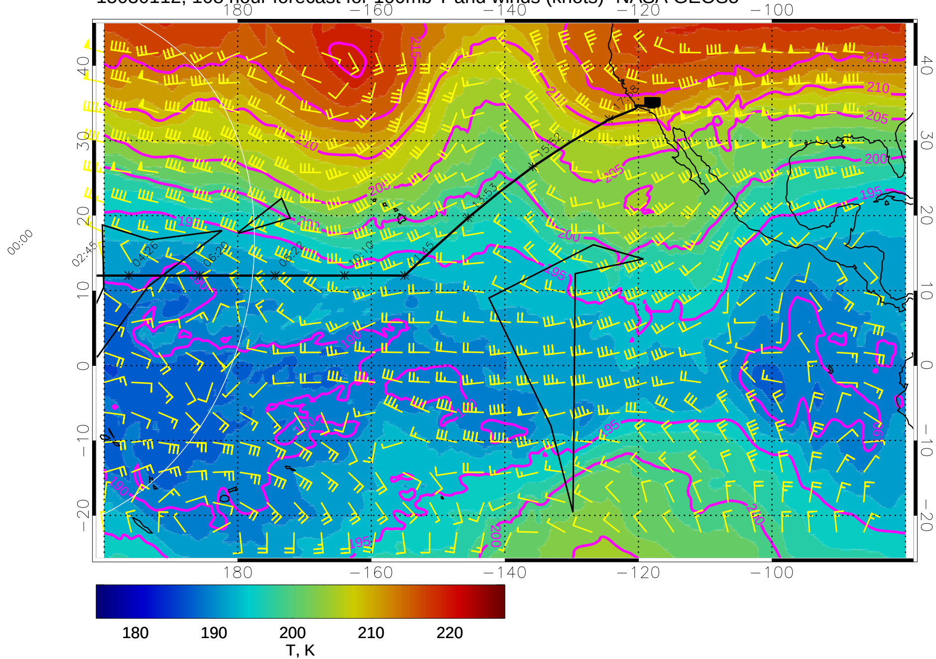
15030112, 108 hour forecast for 100mb T and winds (knots)- NASA GEOS5
