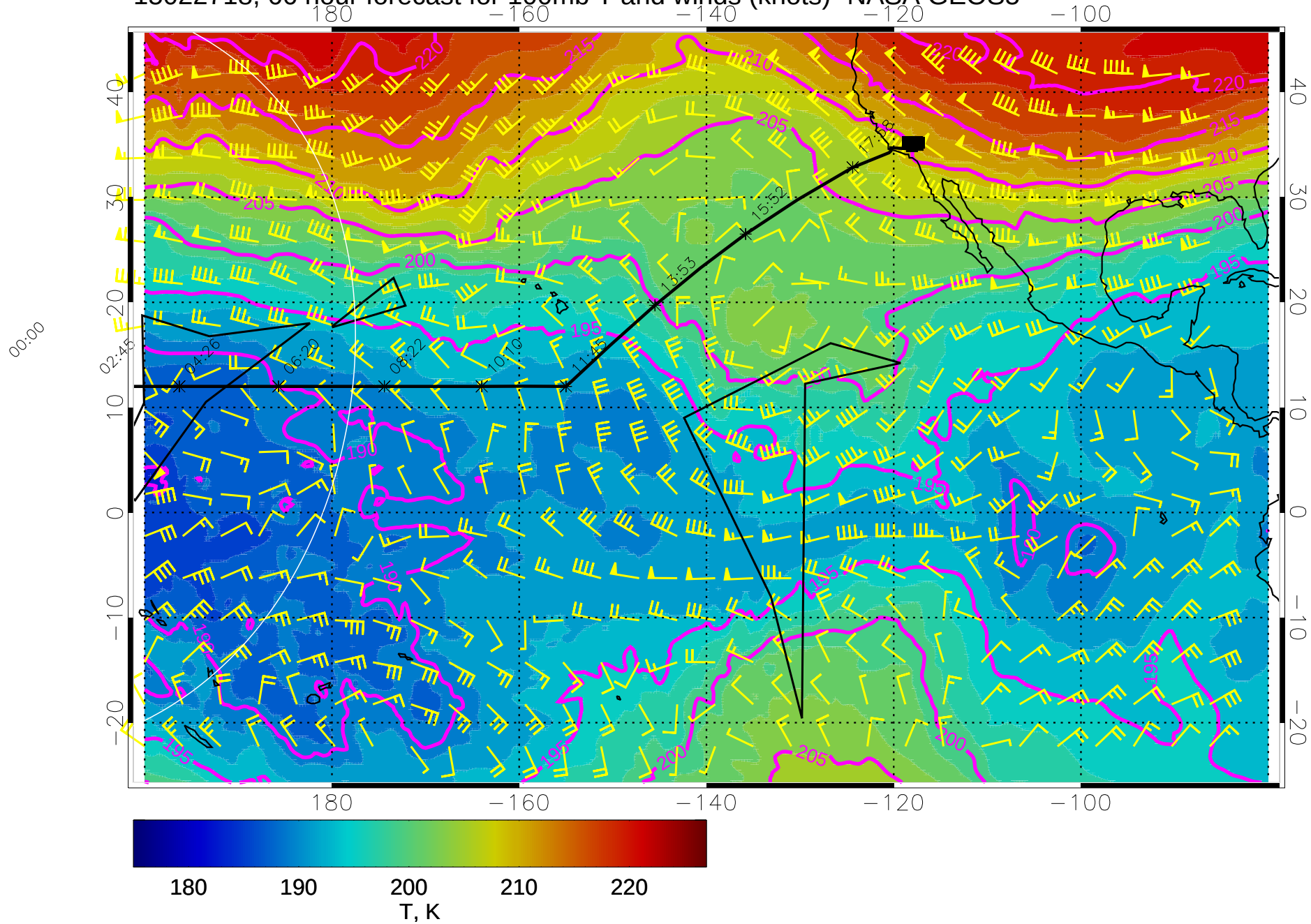
15022718, 66 hour forecast for 100mb T and winds (knots)- NASA GEOS5
