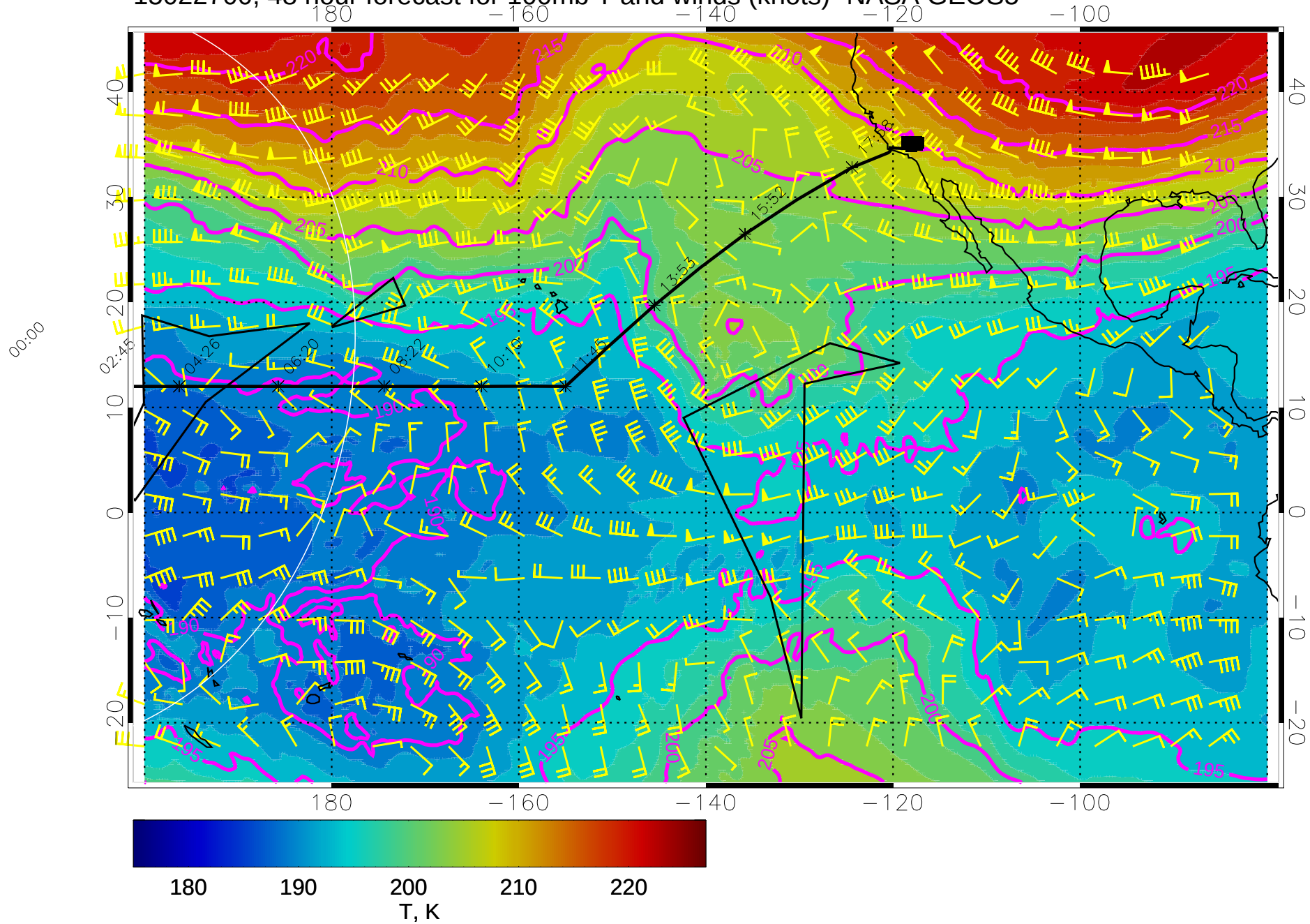
15022700, 48 hour forecast for 100mb T and winds (knots)- NASA GEOS5
