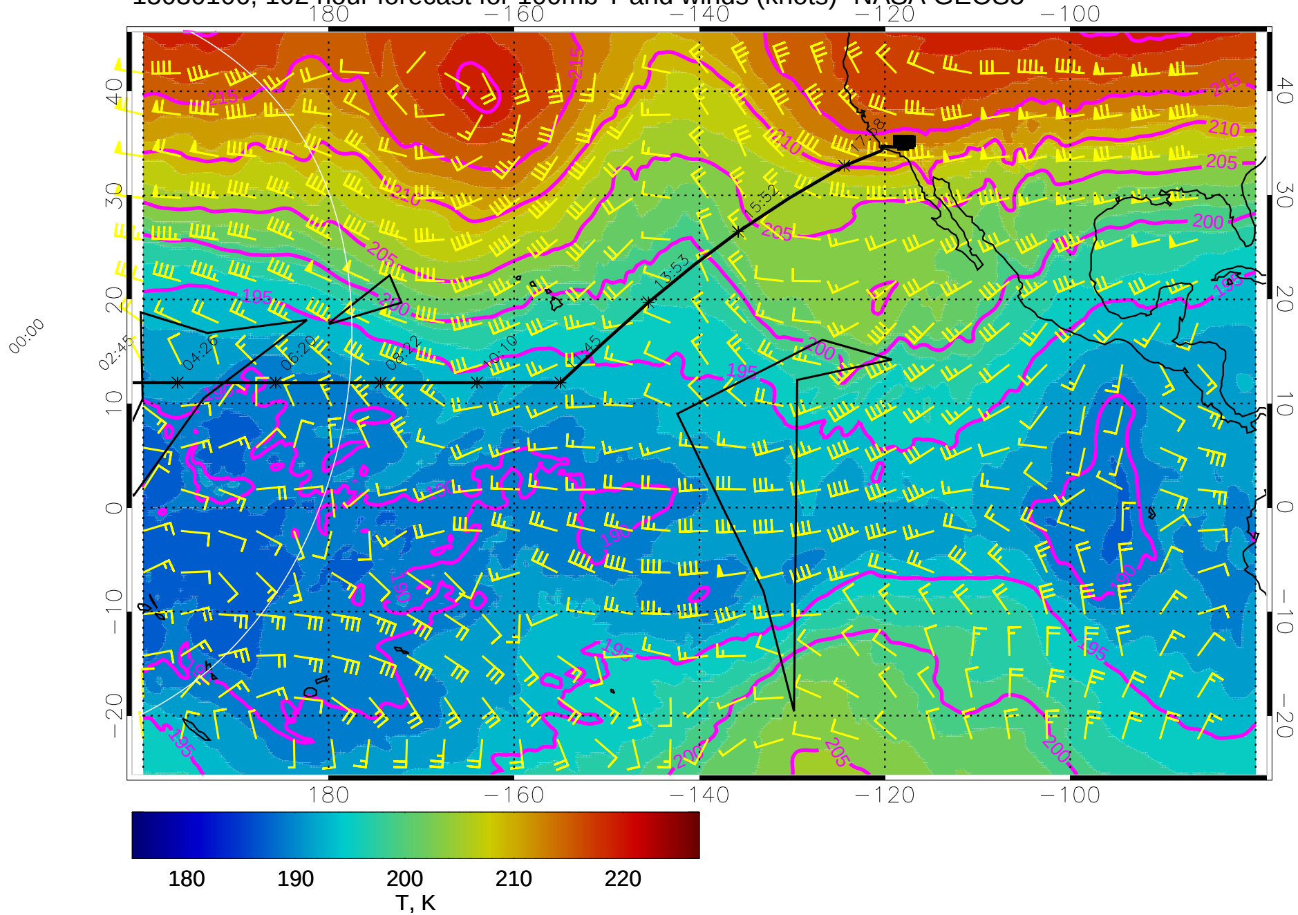
15030106, 102 hour forecast for 100mb T and winds (knots)- NASA GEOS5
