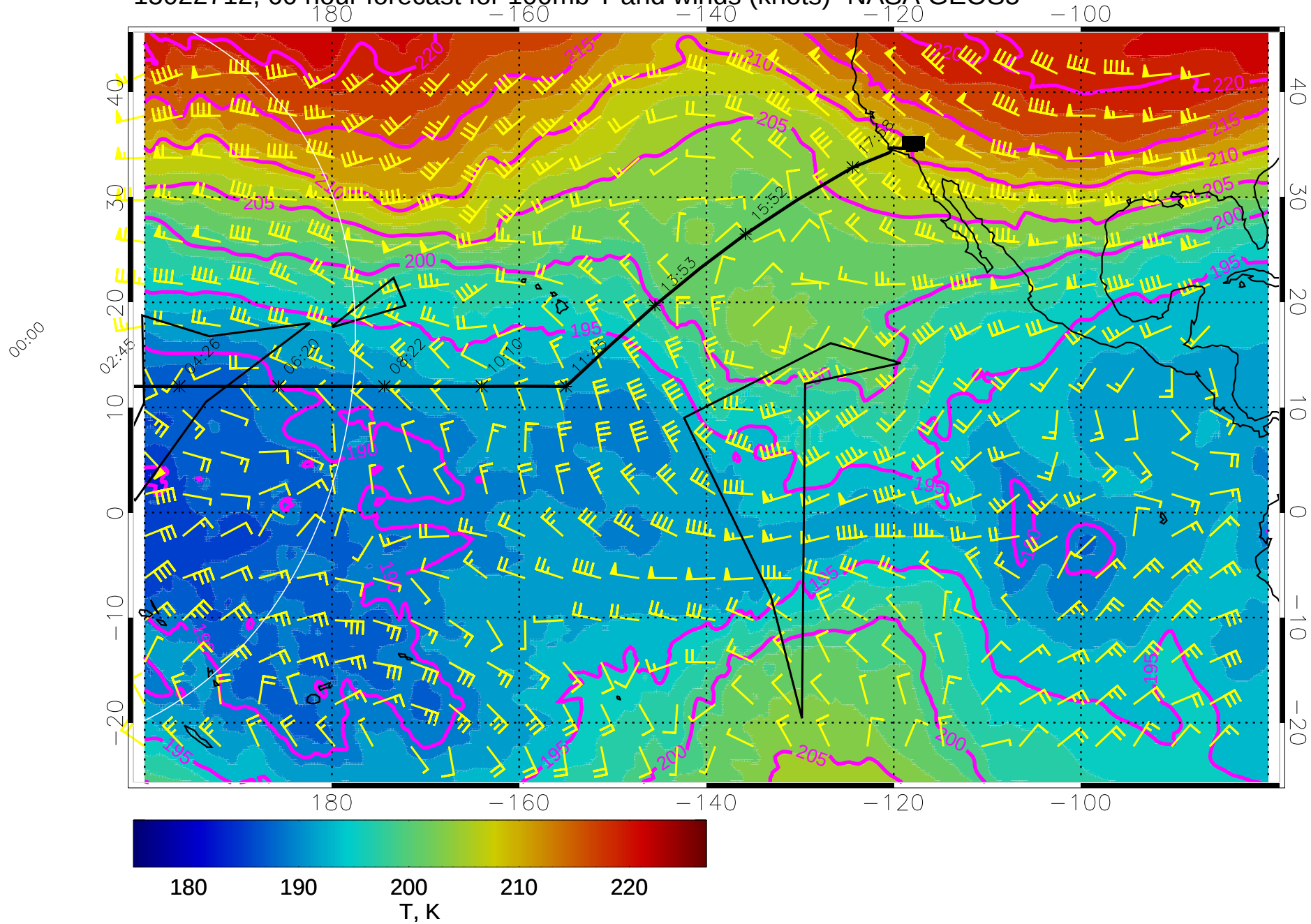
15022712, 60 hour forecast for 100mb T and winds (knots)- NASA GEOS5
