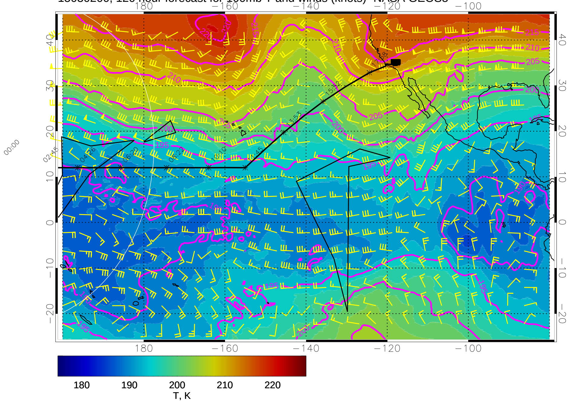
15030200, 120 hour forecast for 100mb T and winds (knots)- NASA GEOS5
