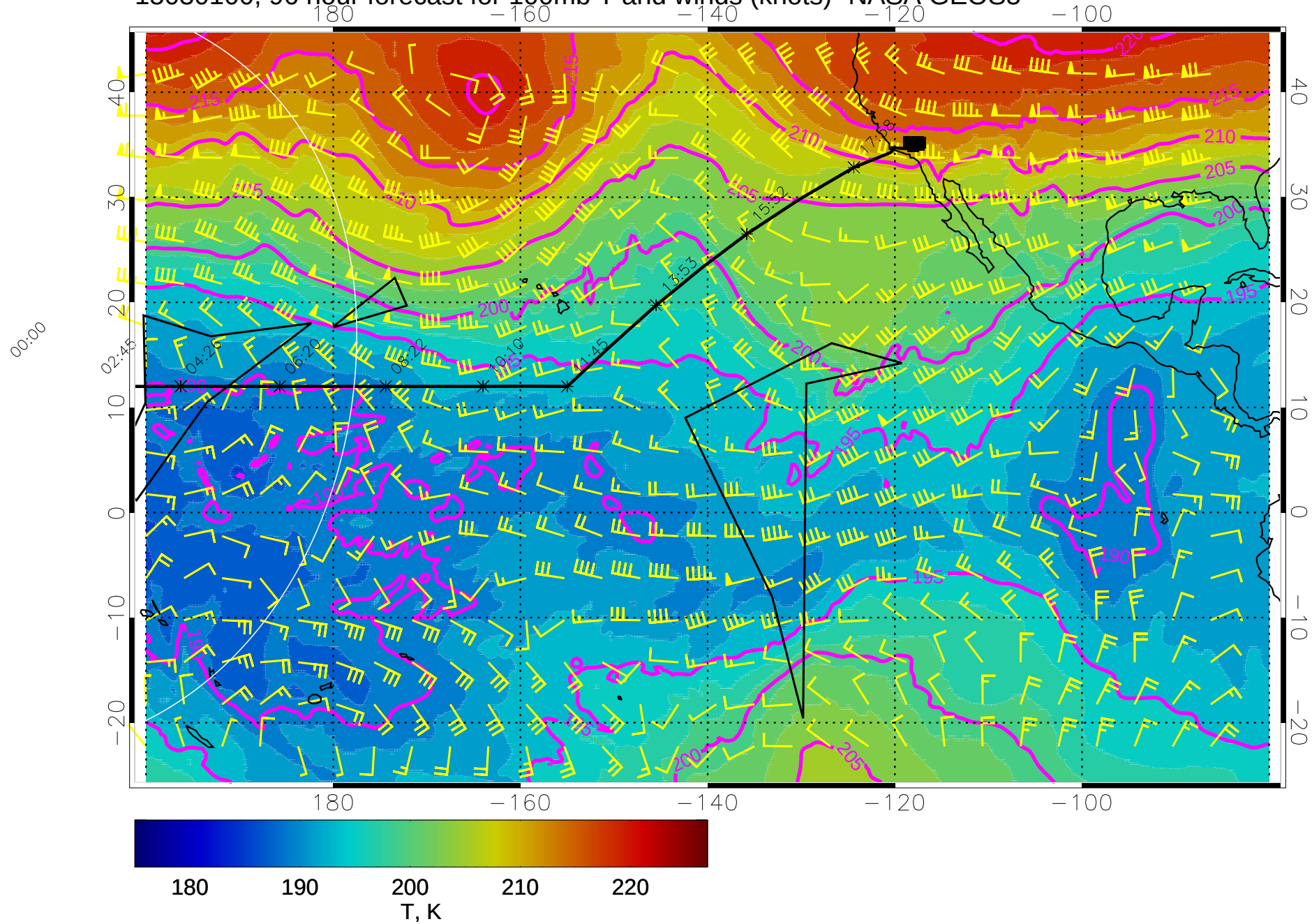
15030100, 96 hour forecast for 100mb T and winds (knots)- NASA GEOS5
