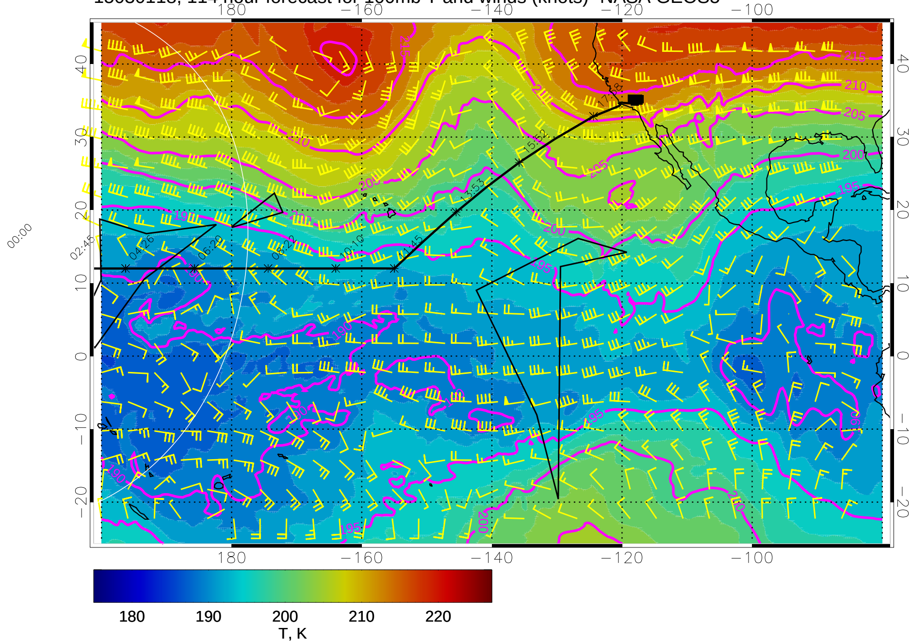
15030118, 114 hour forecast for 100mb T and winds (knots)- NASA GEOS5
