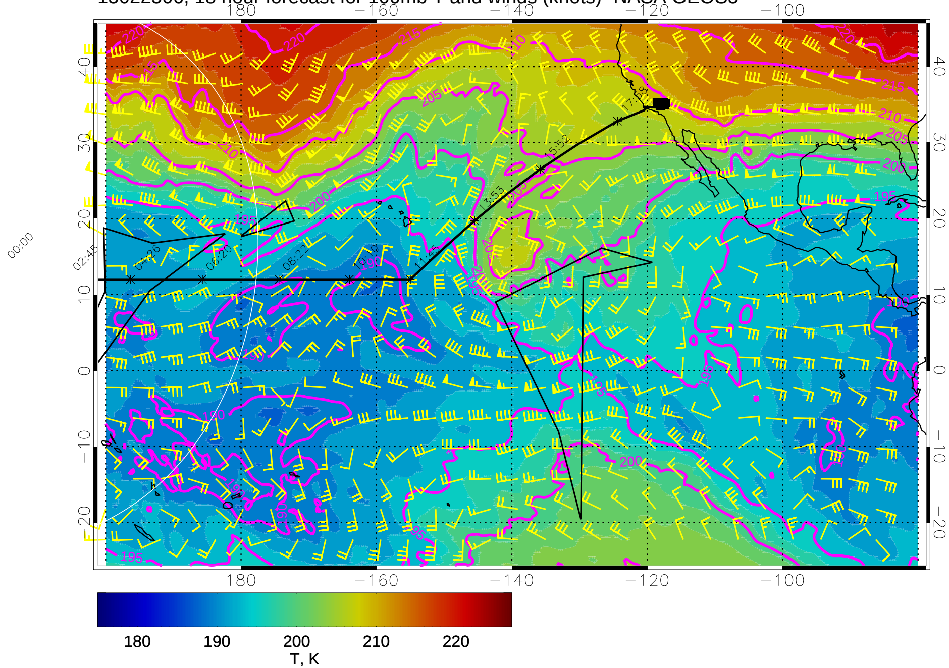
15022506, 18 hour forecast for 100mb T and winds (knots)- NASA GEOS5
