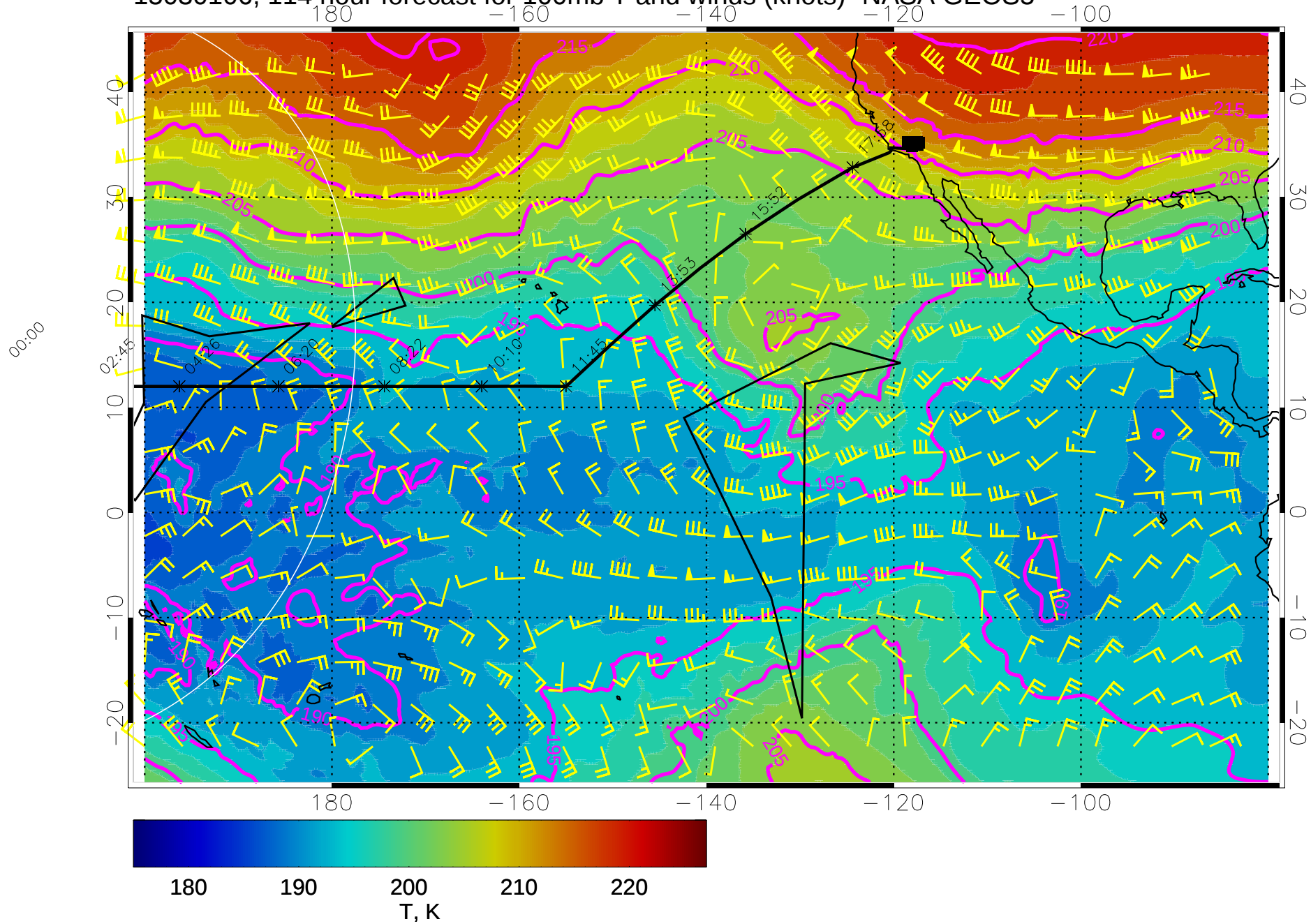
15030106, 114 hour forecast for 100mb T and winds (knots)- NASA GEOS5
