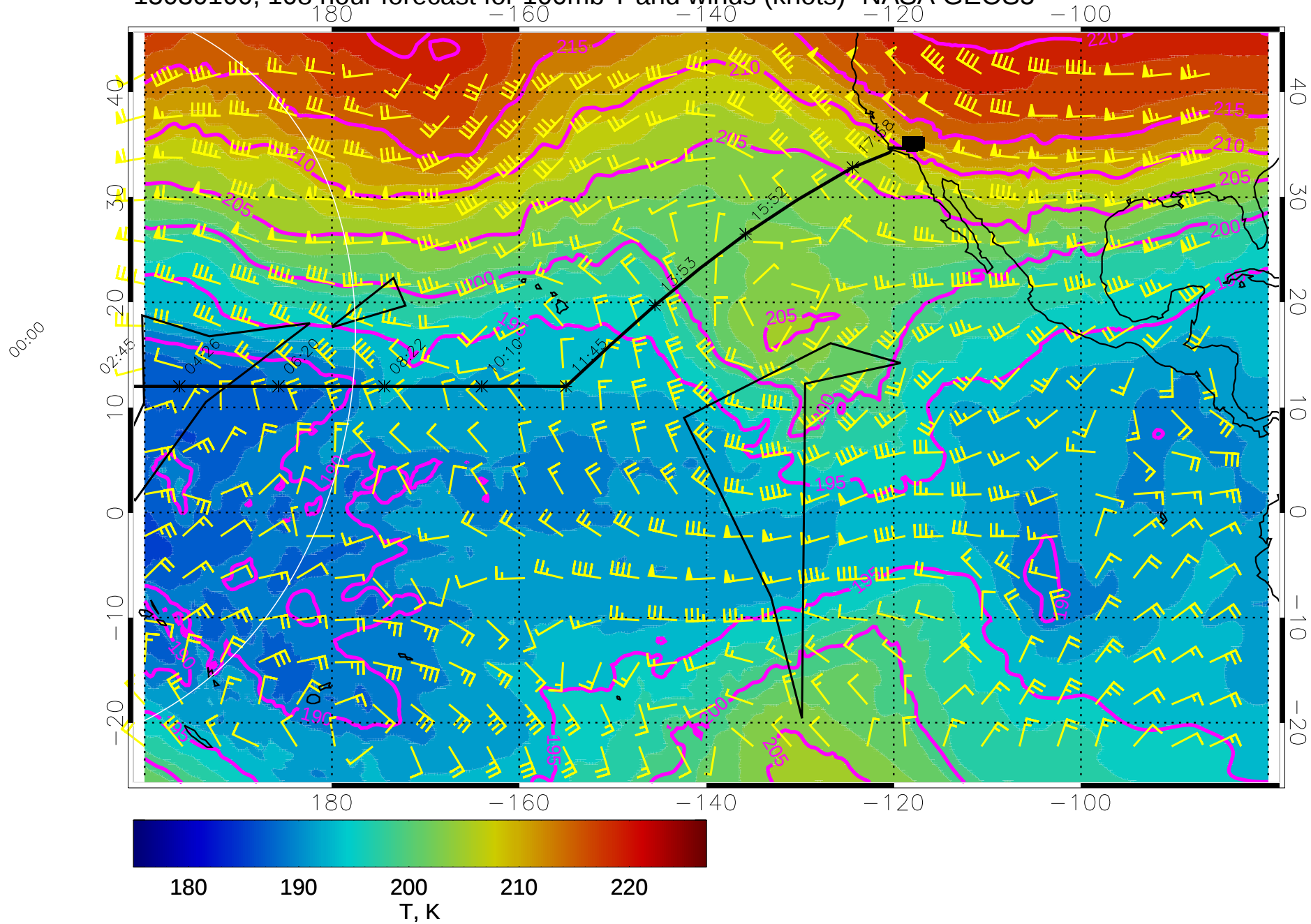
15030100, 108 hour forecast for 100mb T and winds (knots)- NASA GEOS5
