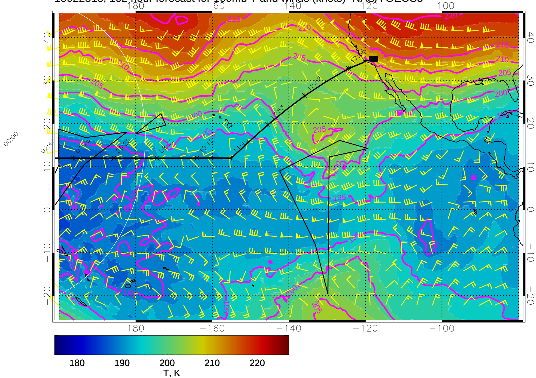
15022818, 102 hour forecast for 100mb T and winds (knots)- NASA GEOS5
