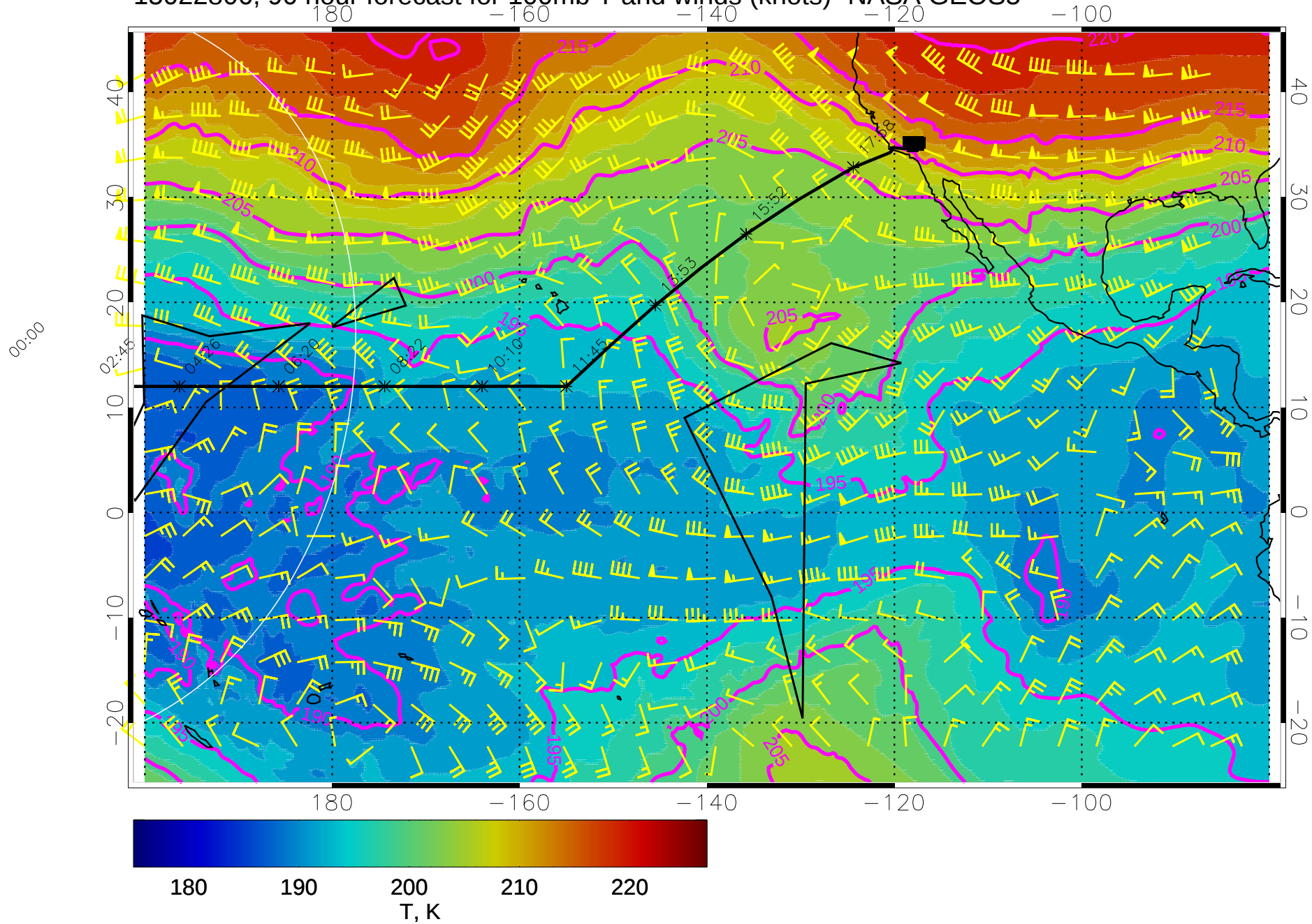
15022806, 90 hour forecast for 100mb T and winds (knots)- NASA GEOS5
