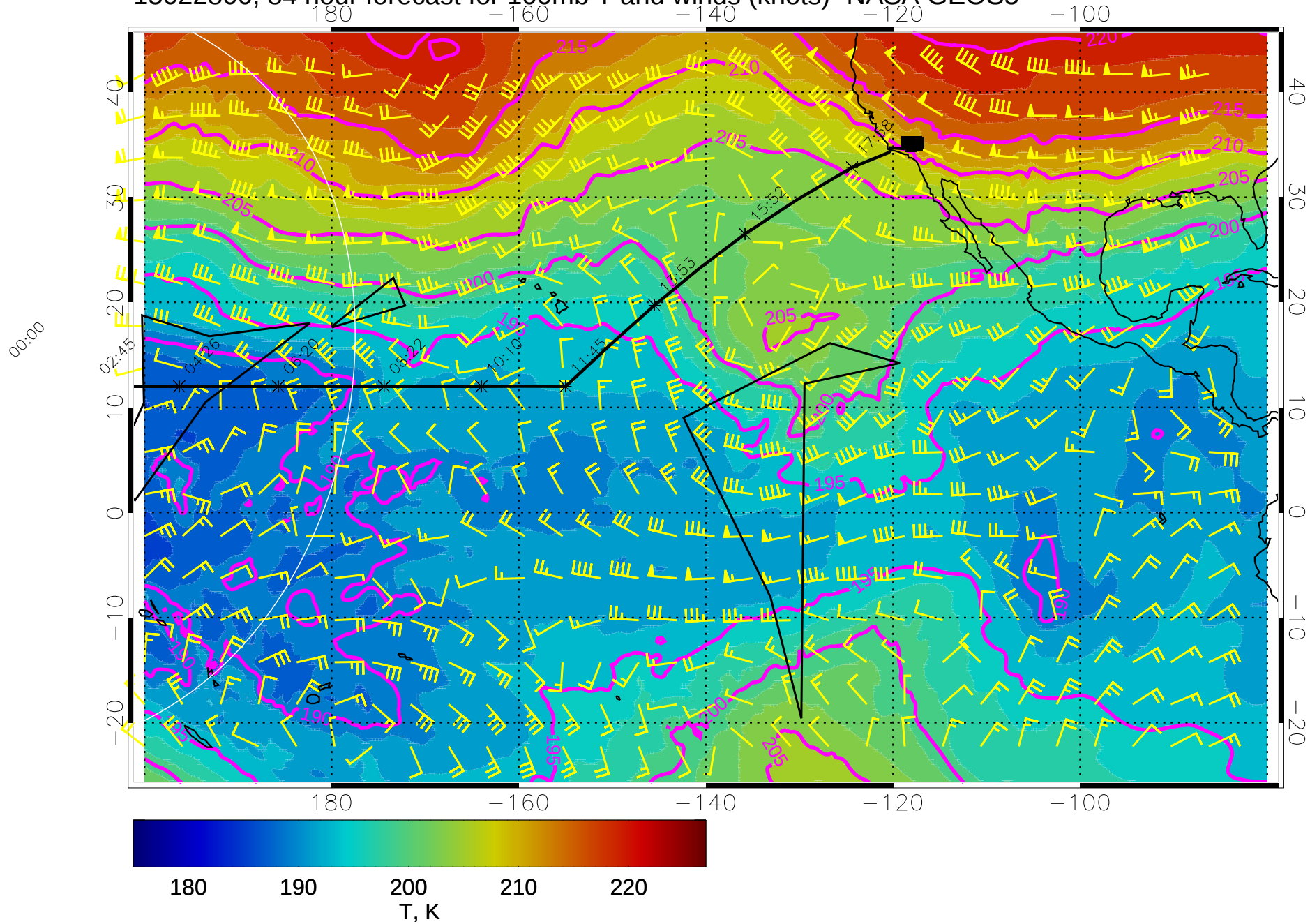
15022800, 84 hour forecast for 100mb T and winds (knots)- NASA GEOS5
