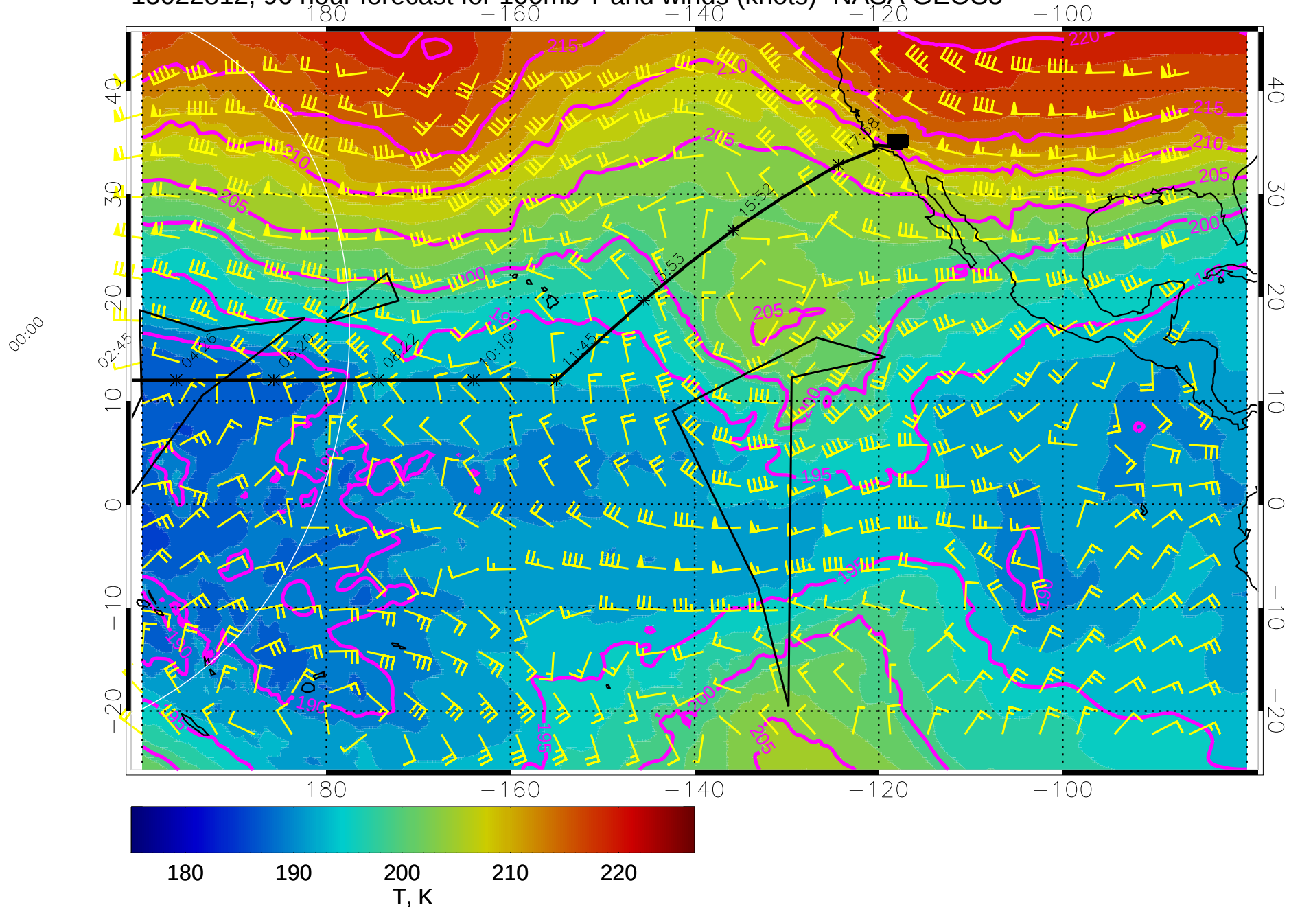
15022812, 96 hour forecast for 100mb T and winds (knots)- NASA GEOS5
