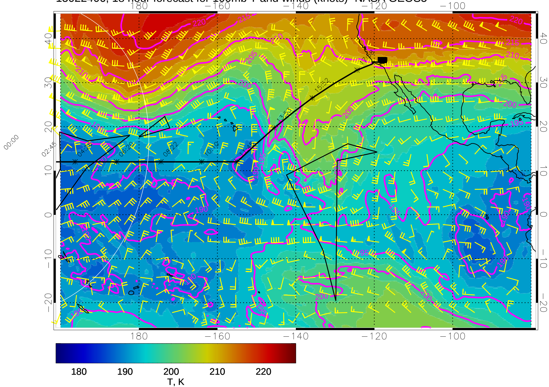
15022406, 18 hour forecast for 100mb T and winds (knots)- NASA GEOS5
