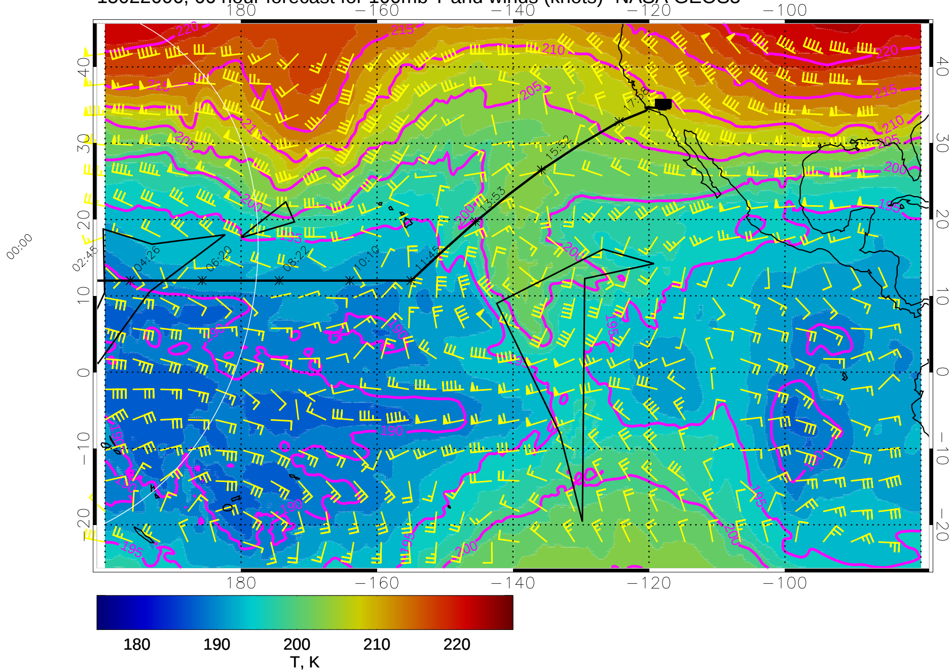
15022606, 66 hour forecast for 100mb T and winds (knots)- NASA GEOS5
