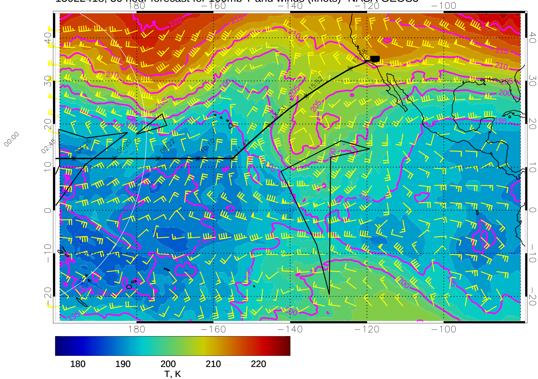
15022418, 30 hour forecast for 100mb T and winds (knots)- NASA GEOS5
