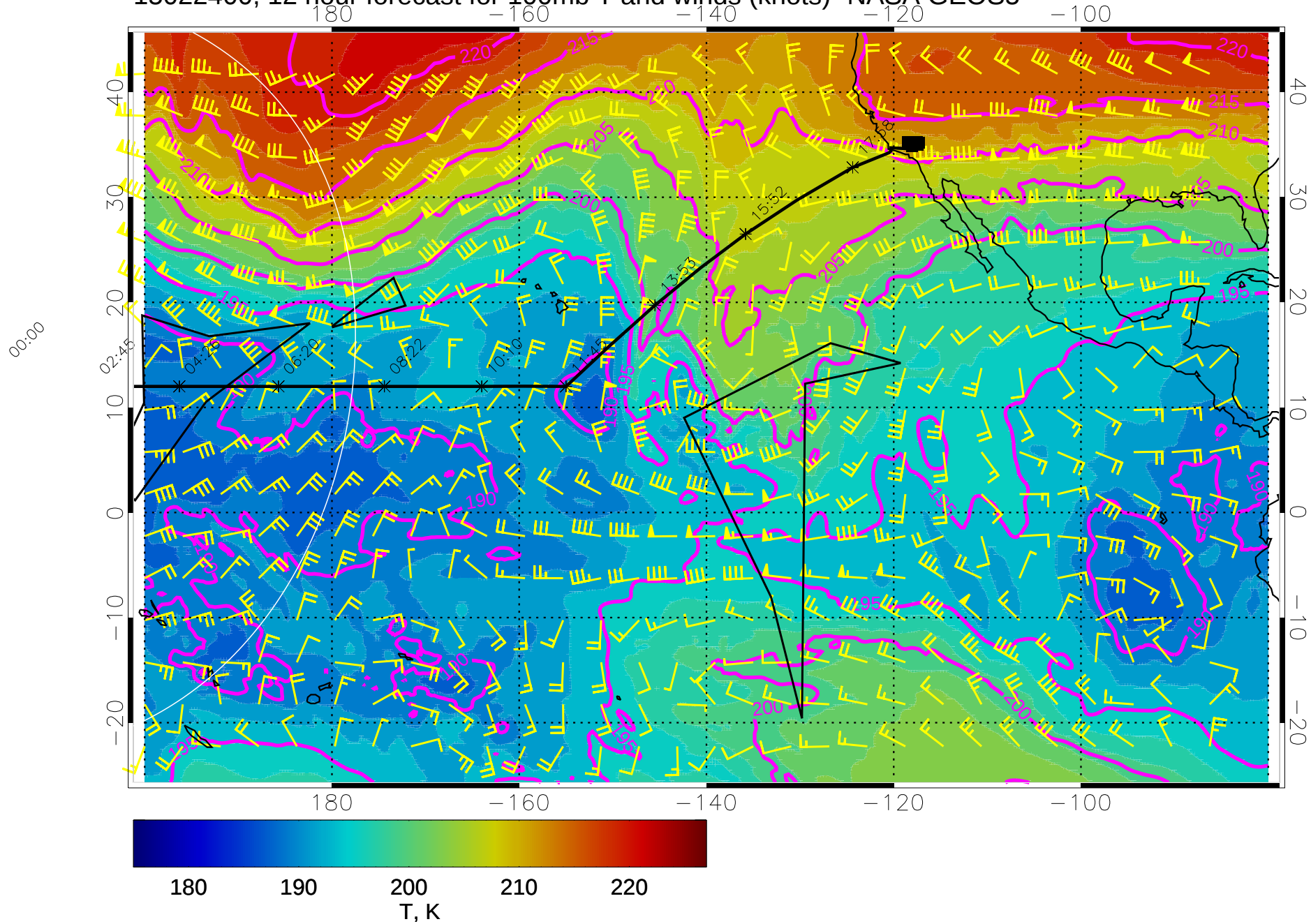
15022400, 12 hour forecast for 100mb T and winds (knots)- NASA GEOS5
