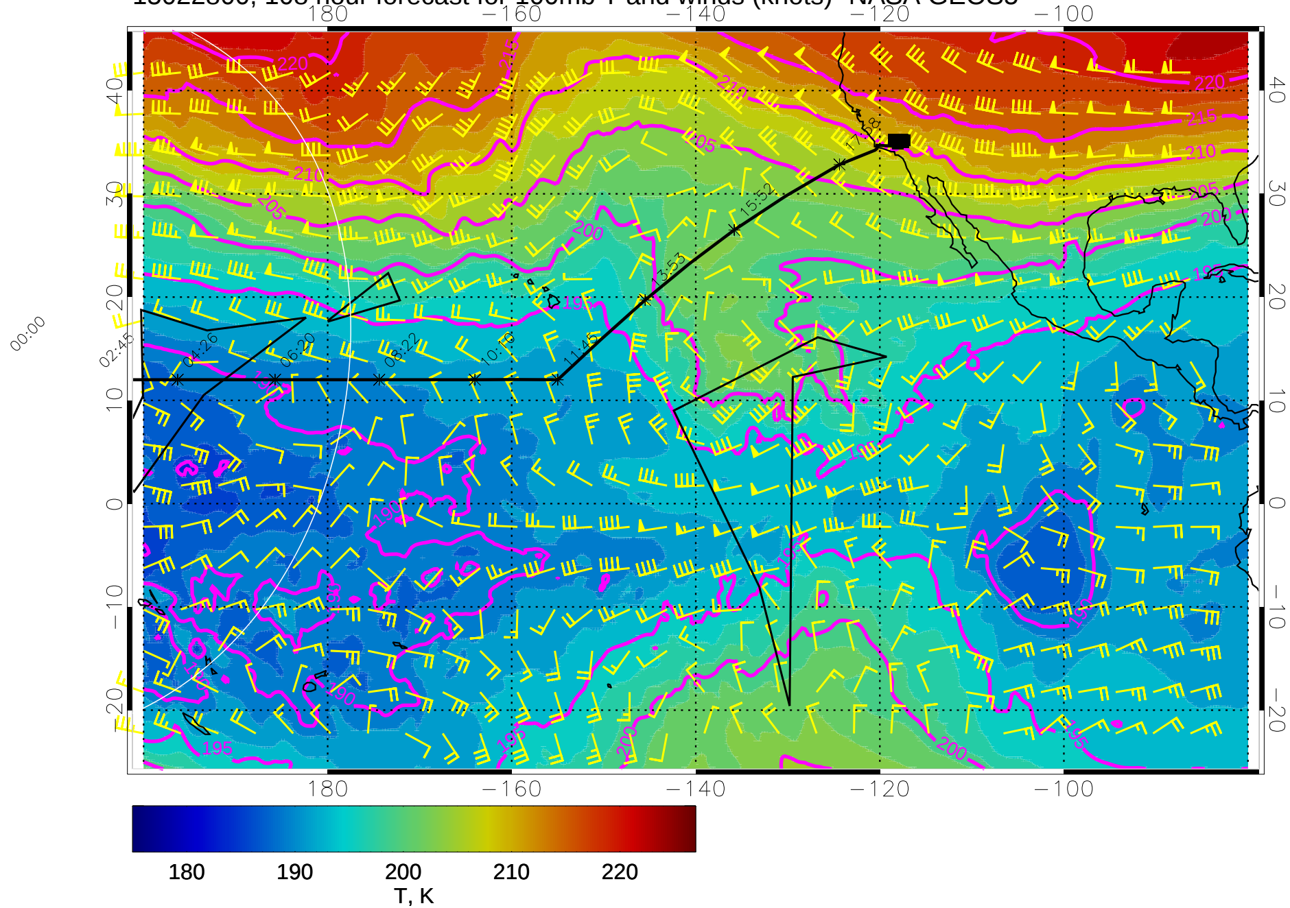
15022800, 108 hour forecast for 100mb T and winds (knots)- NASA GEOS5
