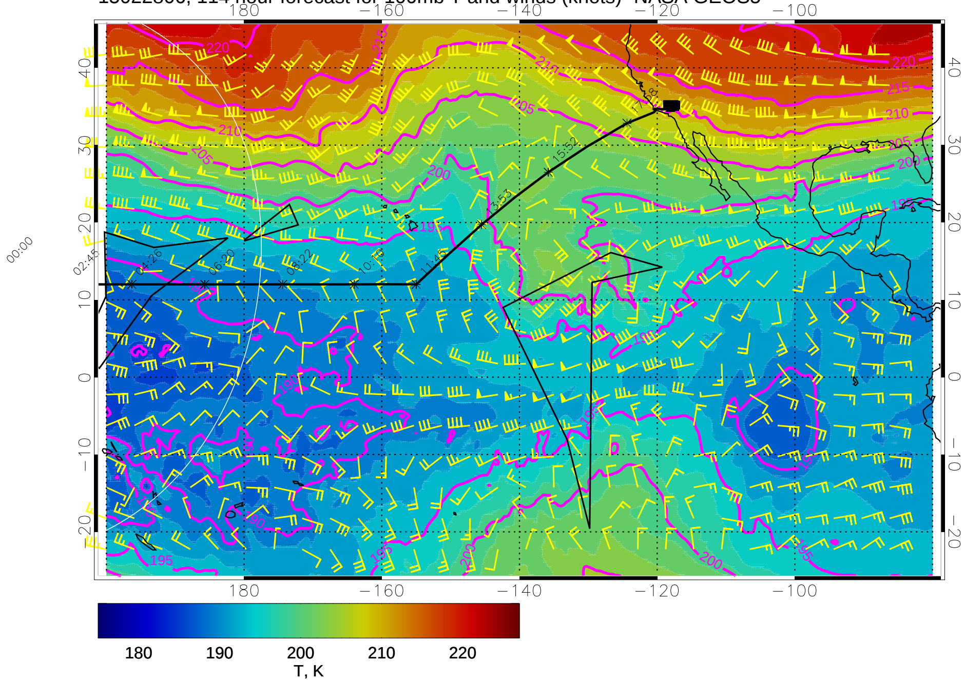
15022806, 114 hour forecast for 100mb T and winds (knots)- NASA GEOS5
