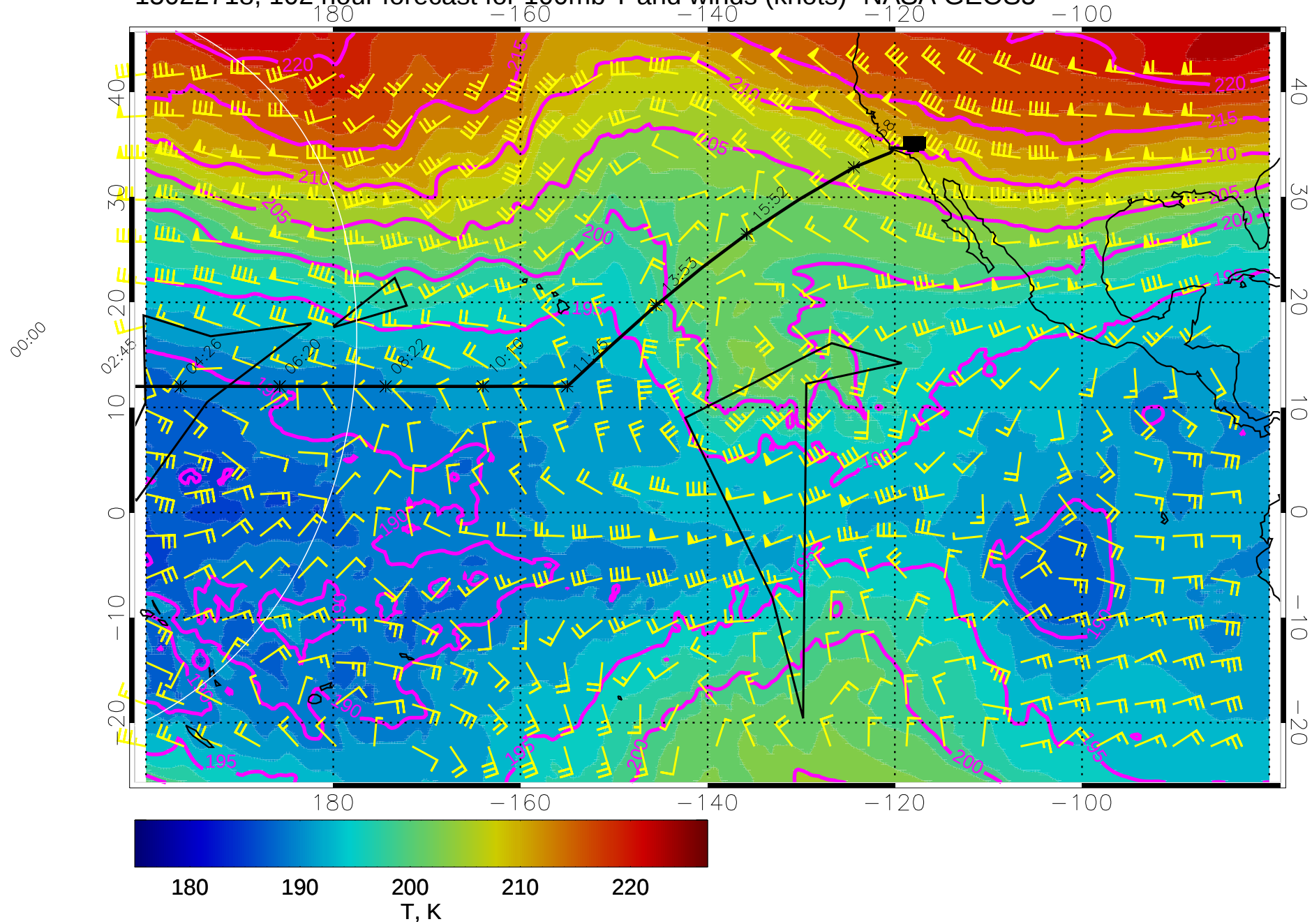
15022718, 102 hour forecast for 100mb T and winds (knots)- NASA GEOS5
