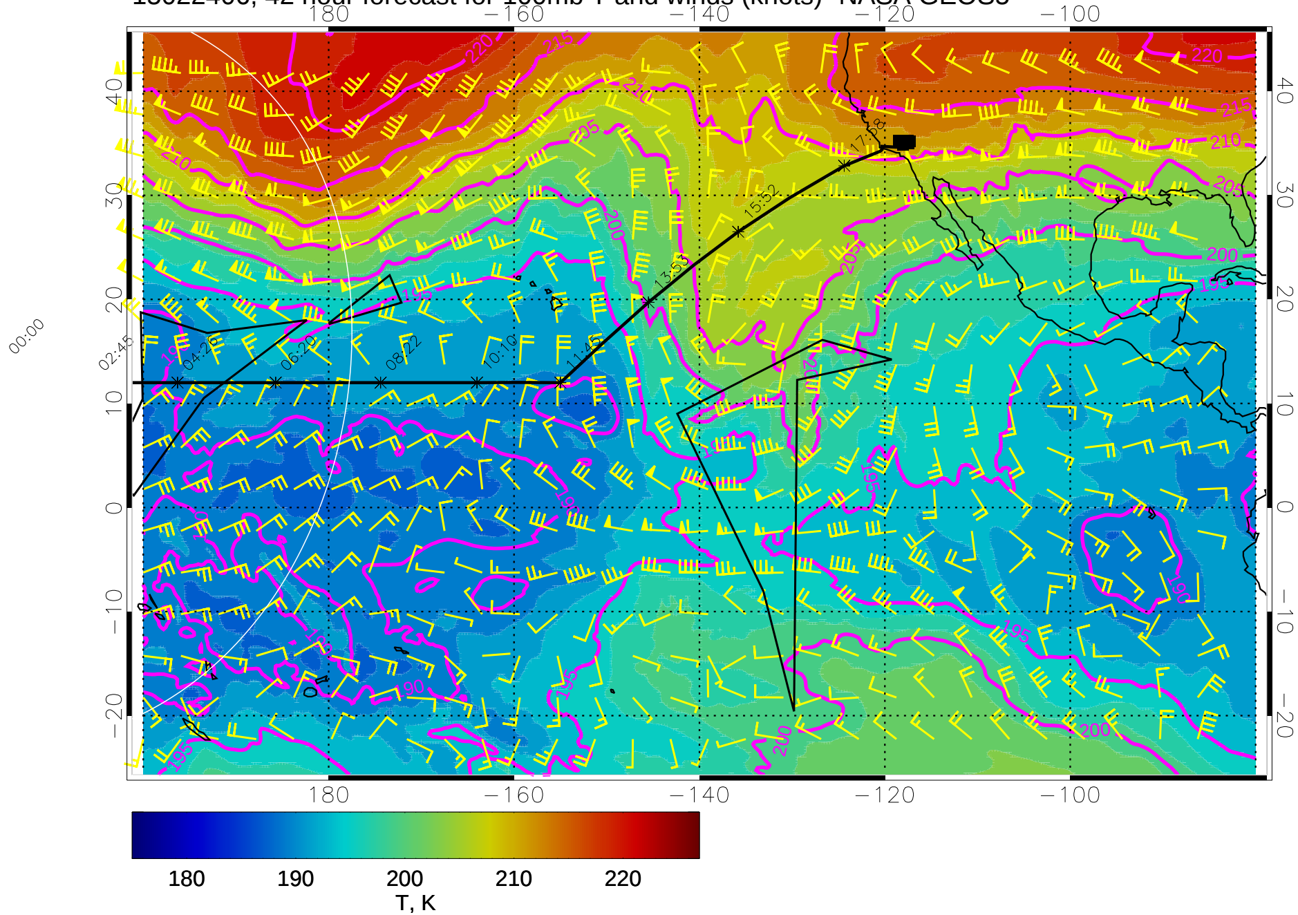
15022406, 42 hour forecast for 100mb T and winds (knots)- NASA GEOS5
