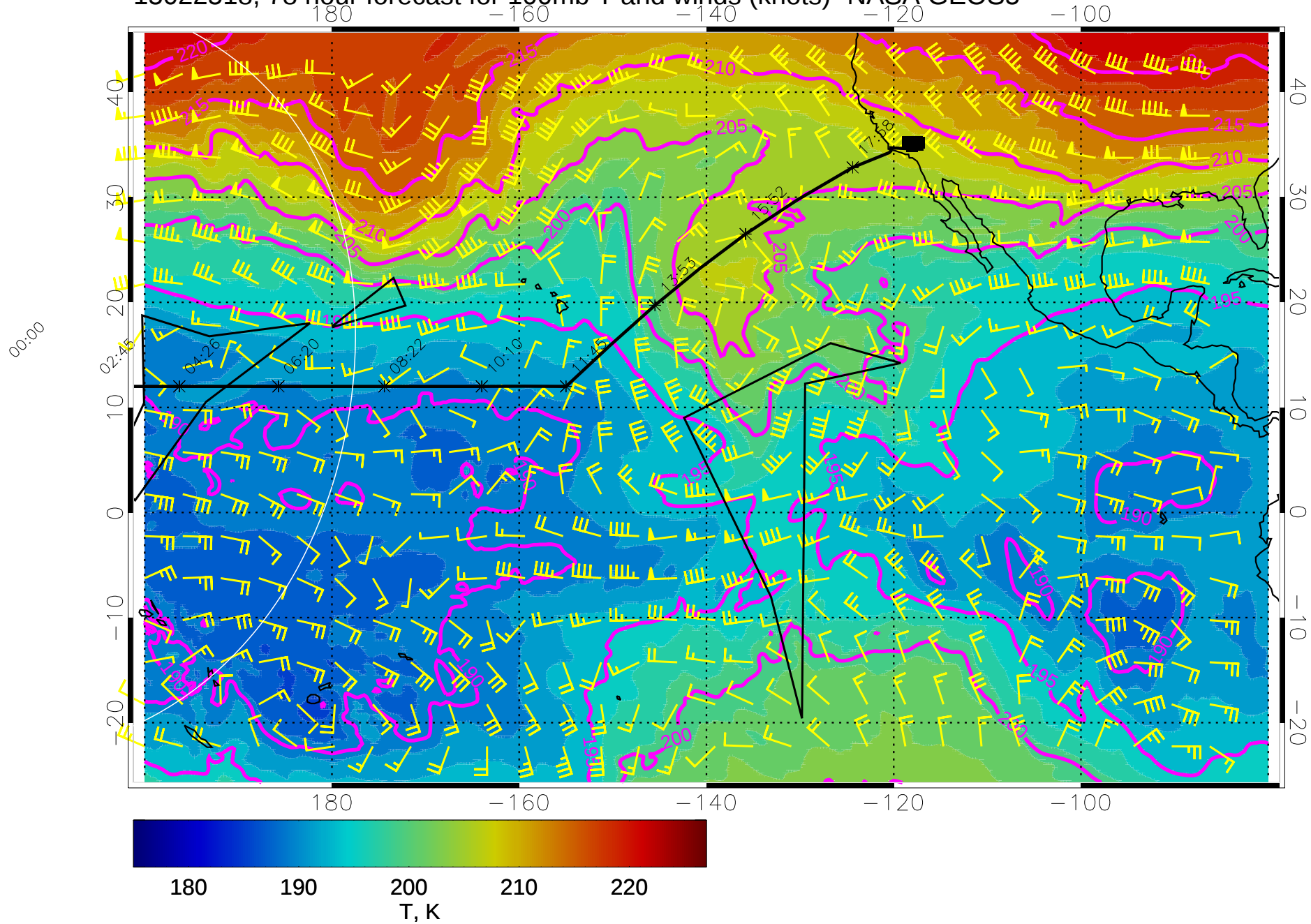
15022518, 78 hour forecast for 100mb T and winds (knots)- NASA GEOS5
