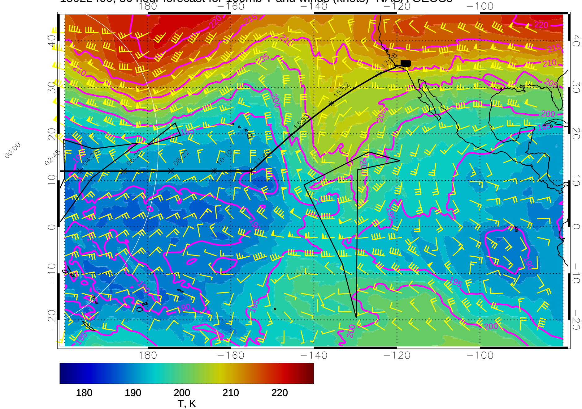
15022400, 36 hour forecast for 100mb T and winds (knots)- NASA GEOS5
