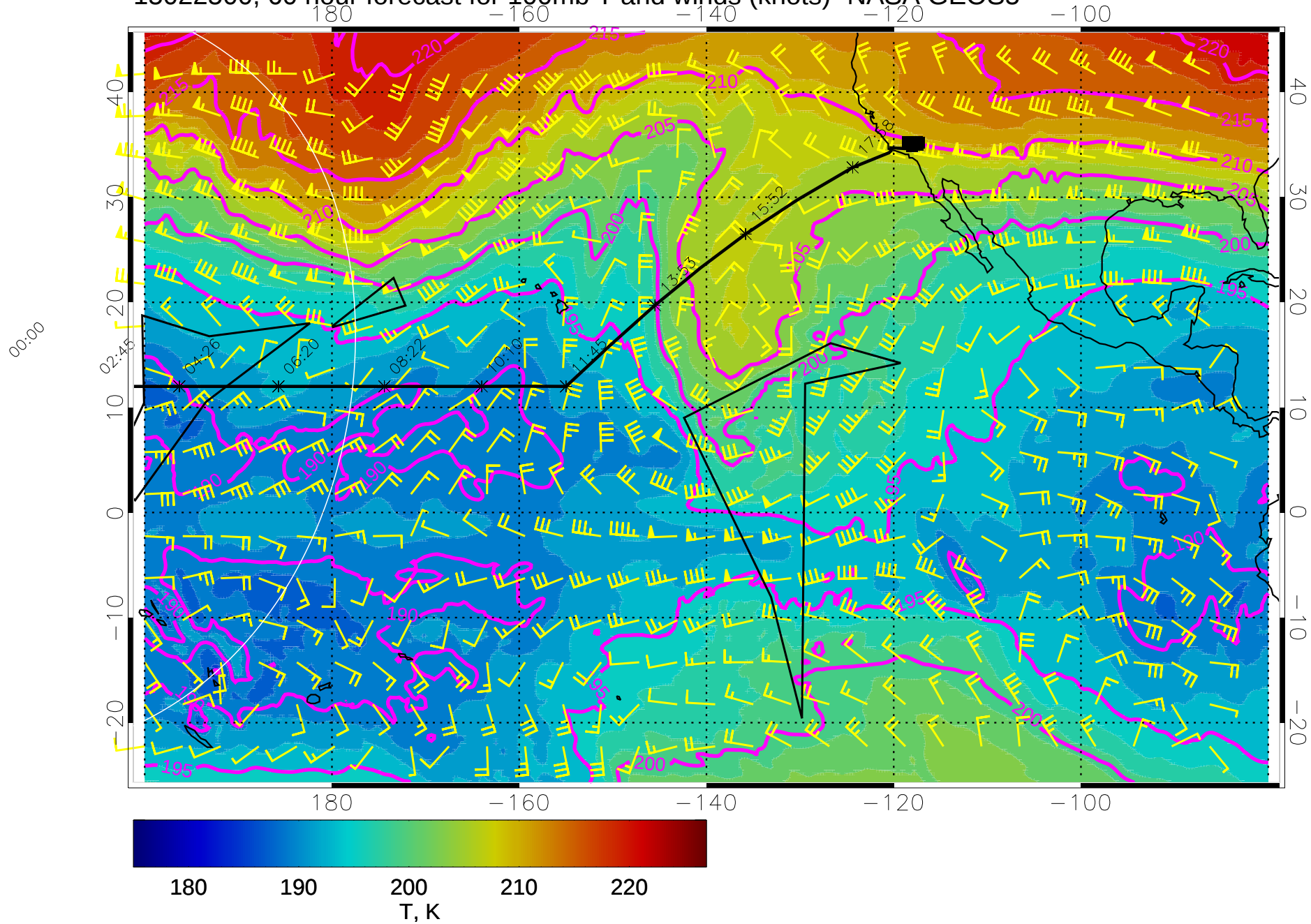
15022500, 60 hour forecast for 100mb T and winds (knots)- NASA GEOS5
