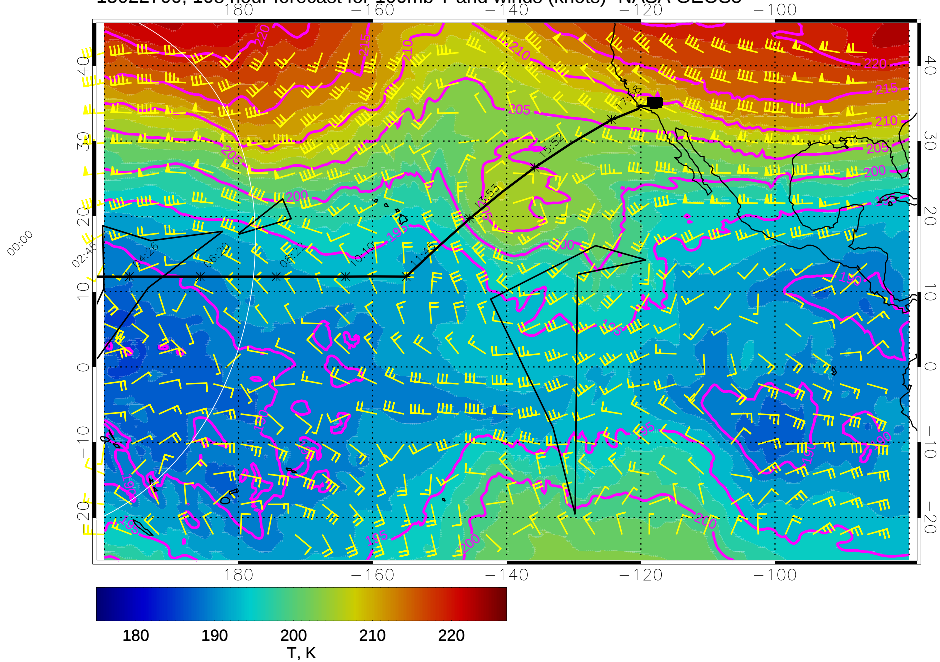
15022700, 108 hour forecast for 100mb T and winds (knots)- NASA GEOS5
