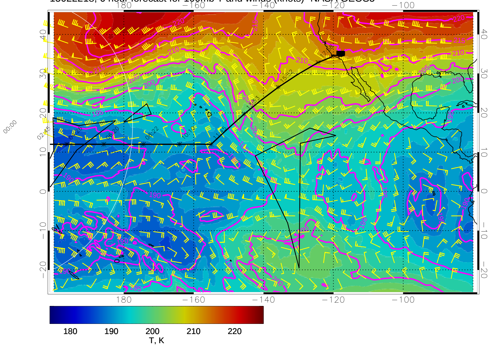
15022218, 6 hour forecast for 100mb T and winds (knots)- NASA GEOS5
