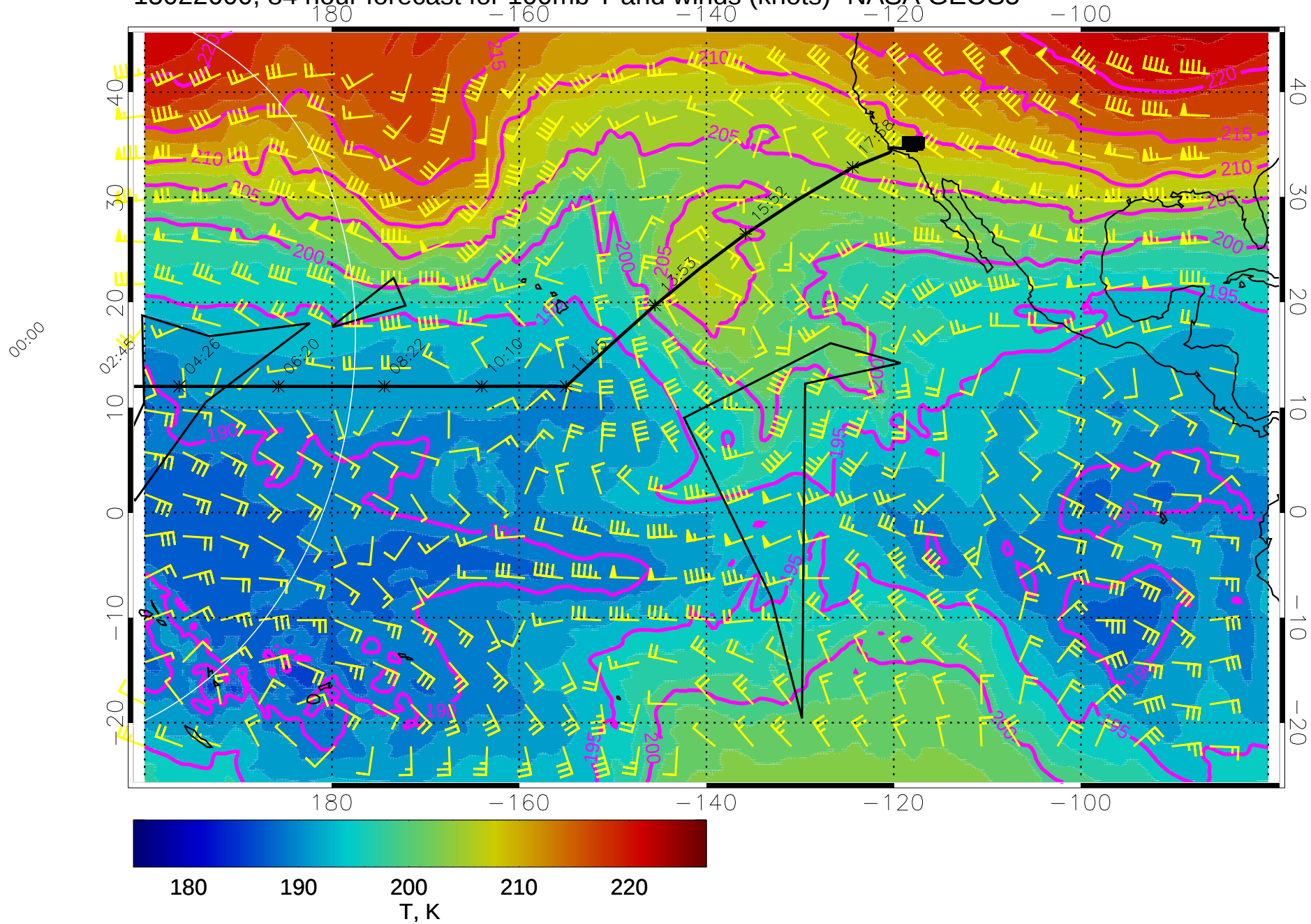
15022600, 84 hour forecast for 100mb T and winds (knots)- NASA GEOS5
