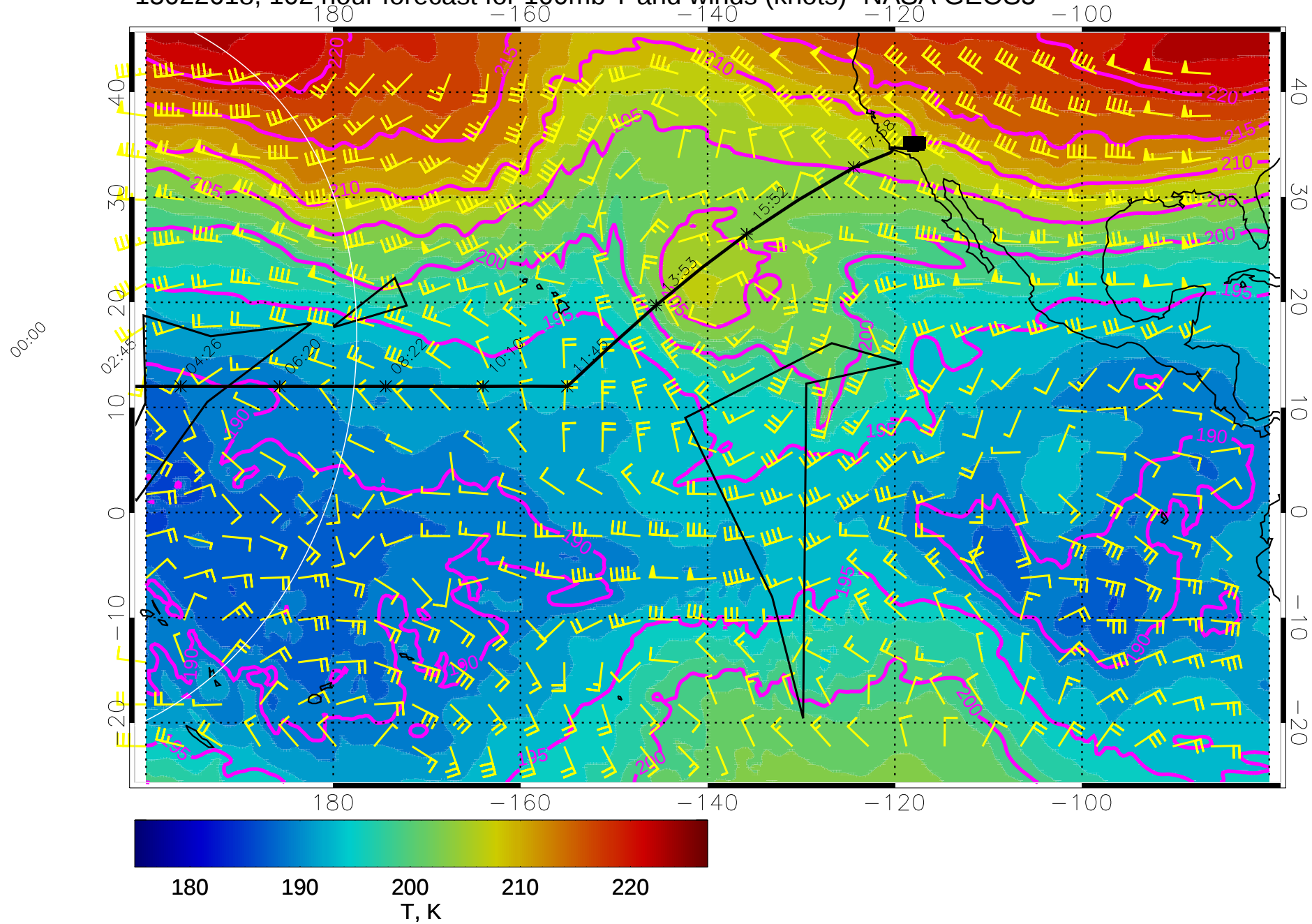
15022618, 102 hour forecast for 100mb T and winds (knots)- NASA GEOS5
