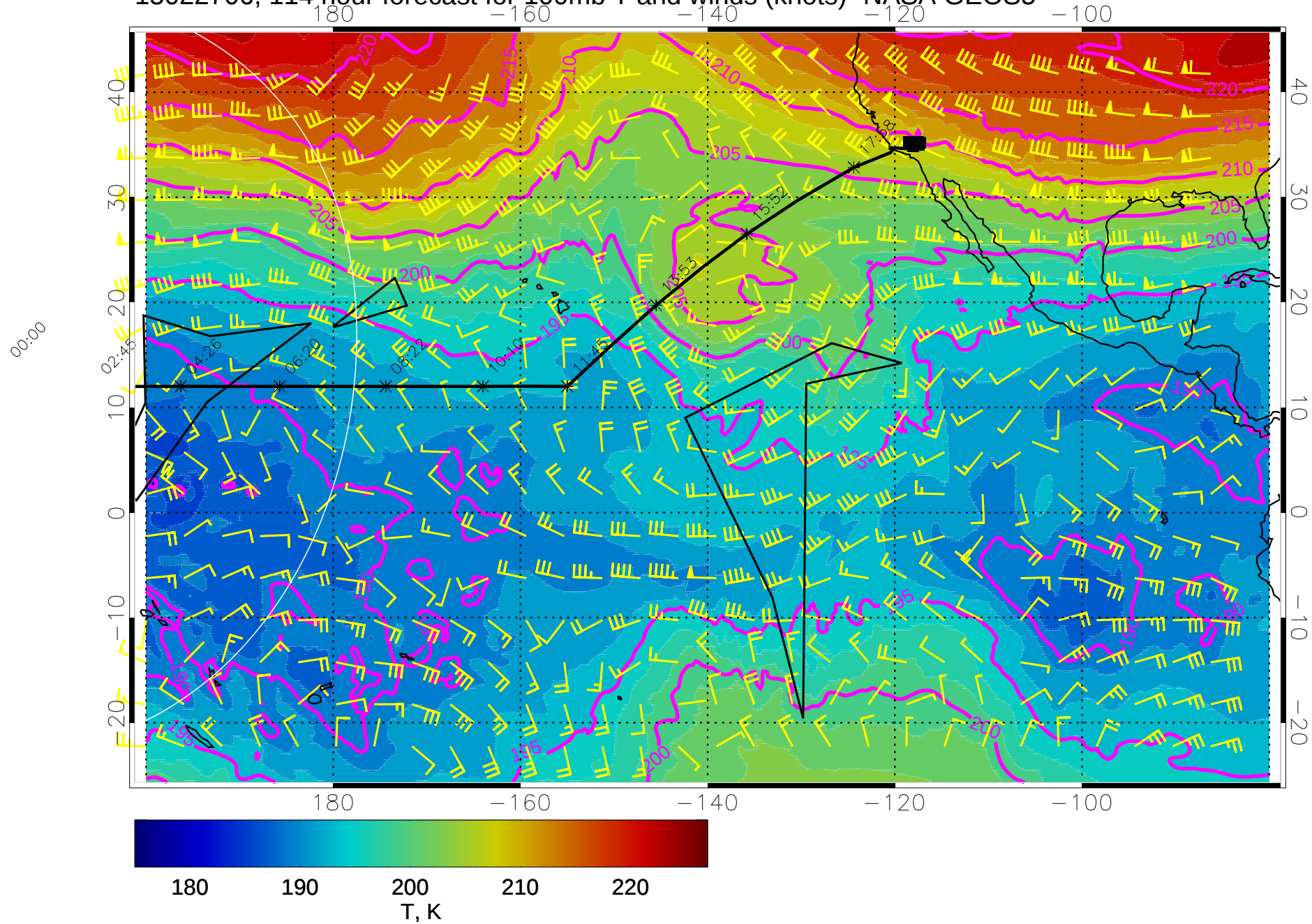
15022706, 114 hour forecast for 100mb T and winds (knots)- NASA GEOS5
