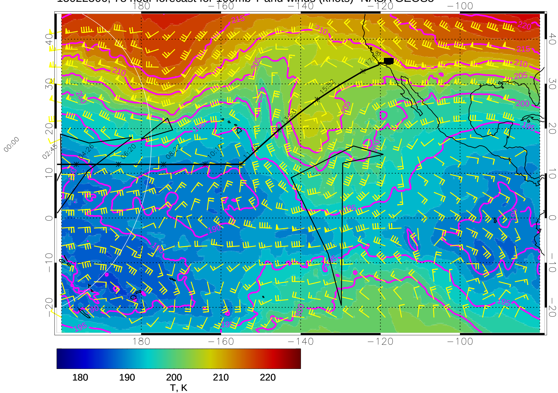
15022506, 78 hour forecast for 100mb T and winds (knots)- NASA GEOS5
