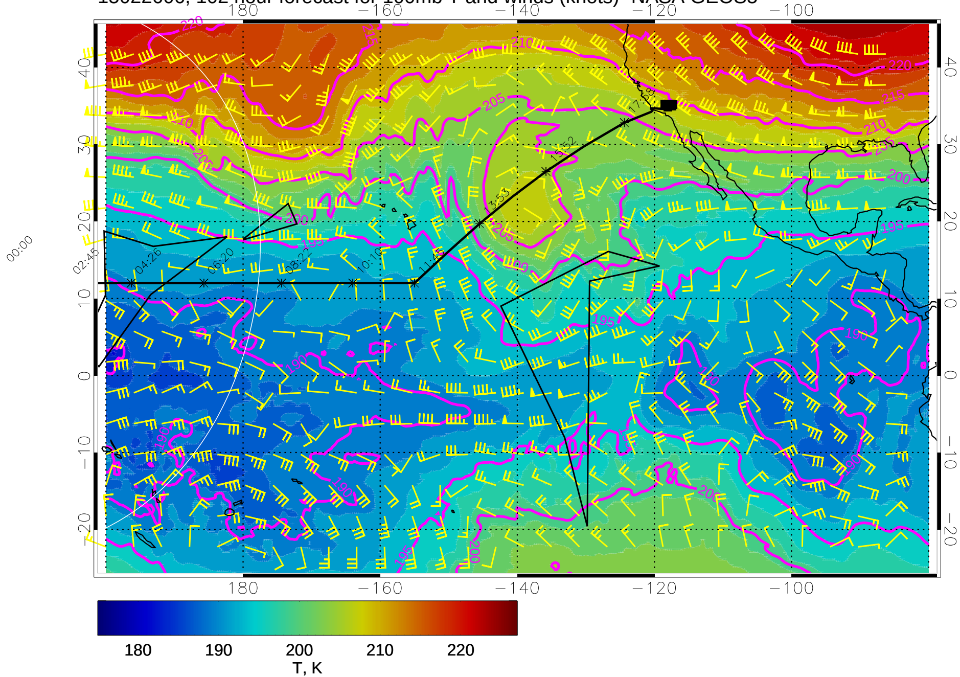
15022606, 102 hour forecast for 100mb T and winds (knots)- NASA GEOS5
