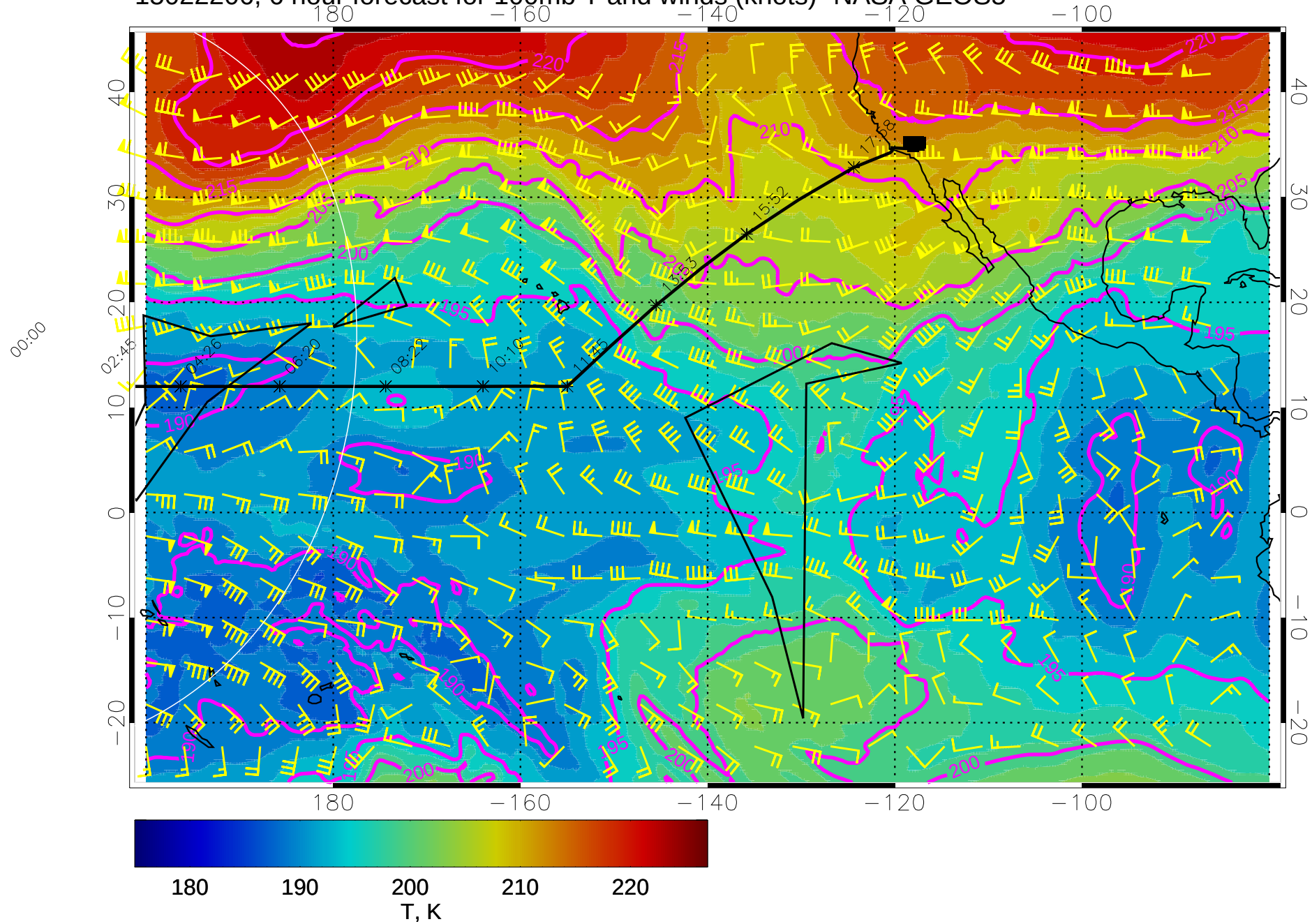
15022206, 6 hour forecast for 100mb T and winds (knots)- NASA GEOS5
