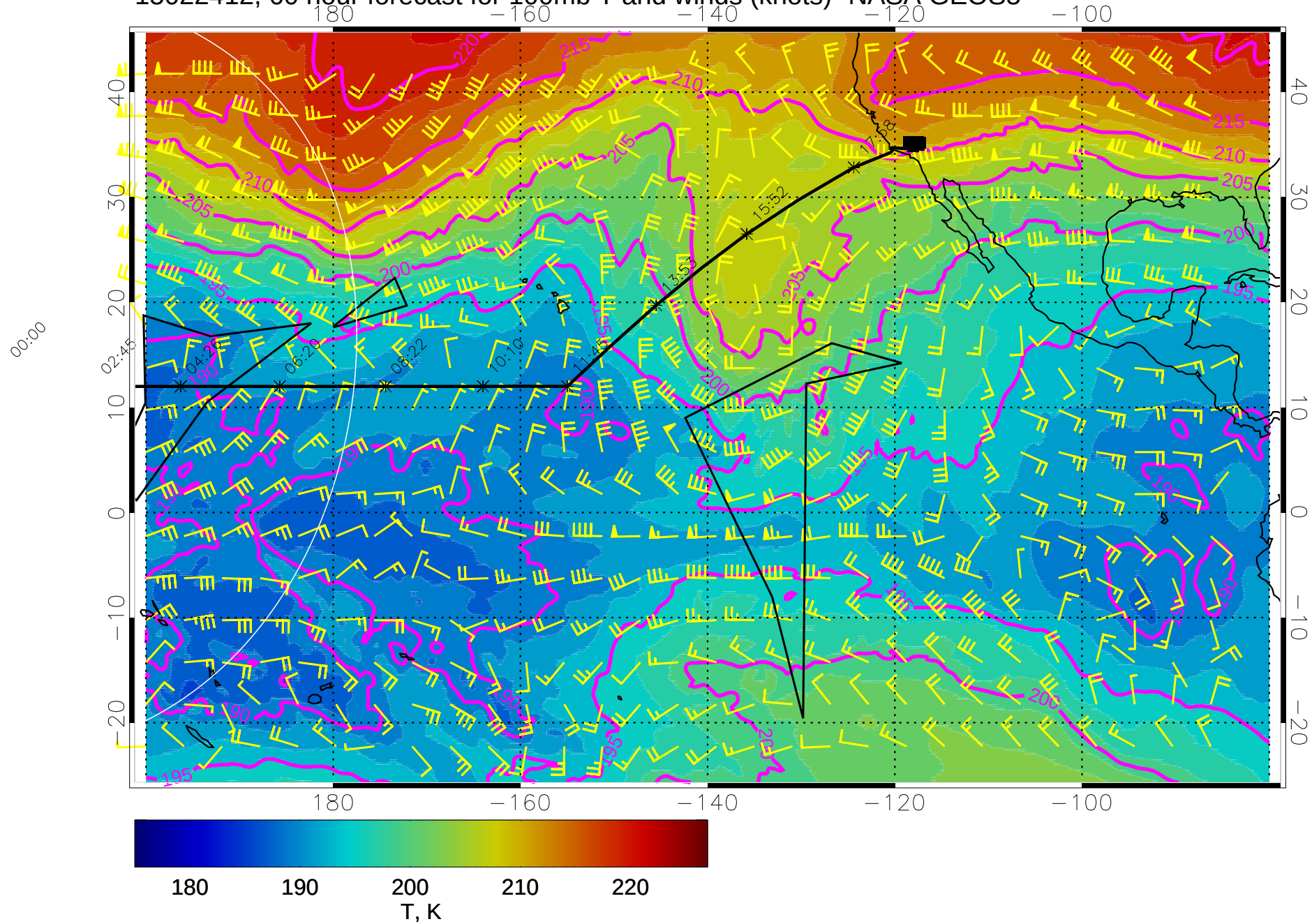
15022412, 60 hour forecast for 100mb T and winds (knots)- NASA GEOS5
