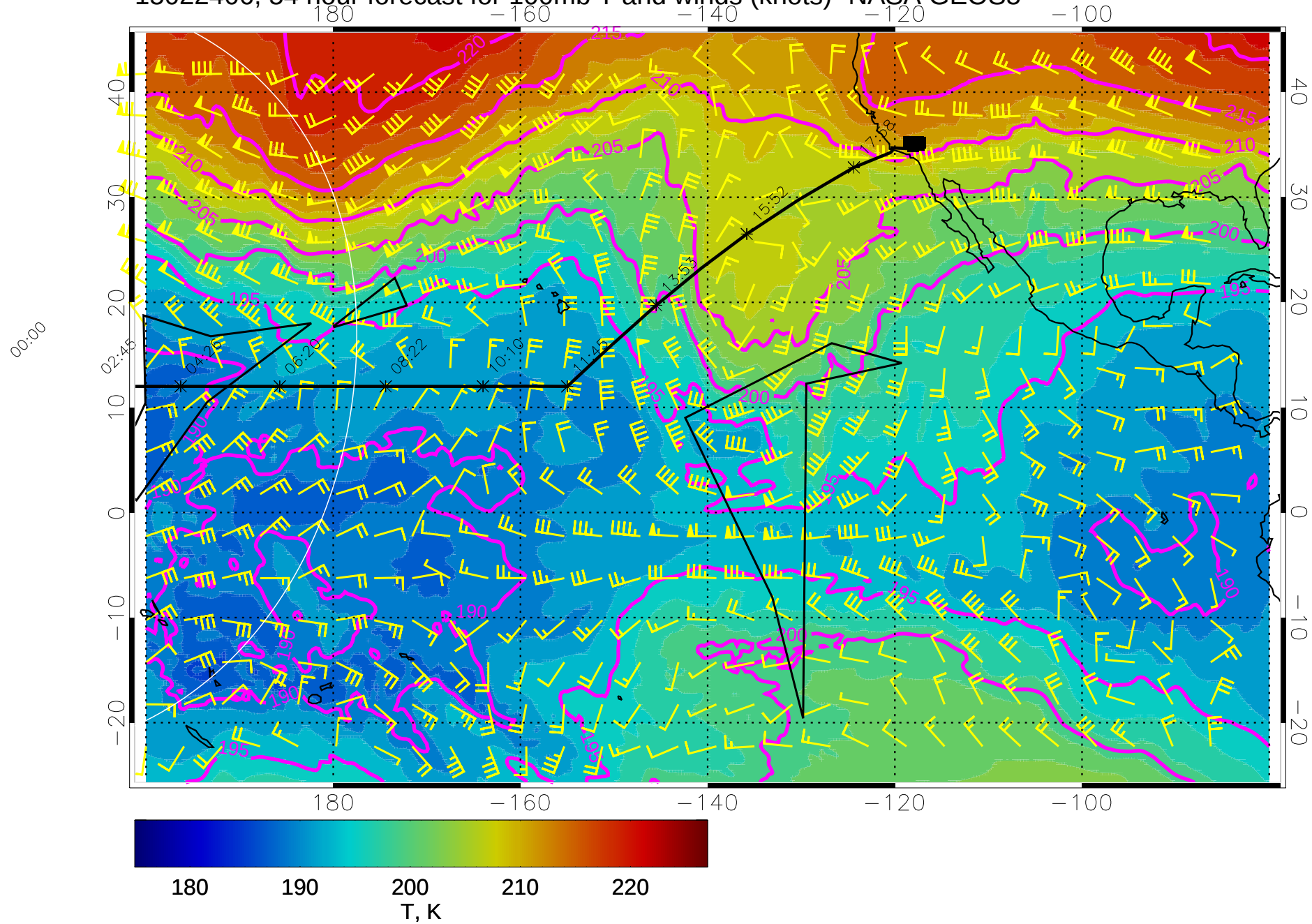
15022406, 54 hour forecast for 100mb T and winds (knots)- NASA GEOS5
