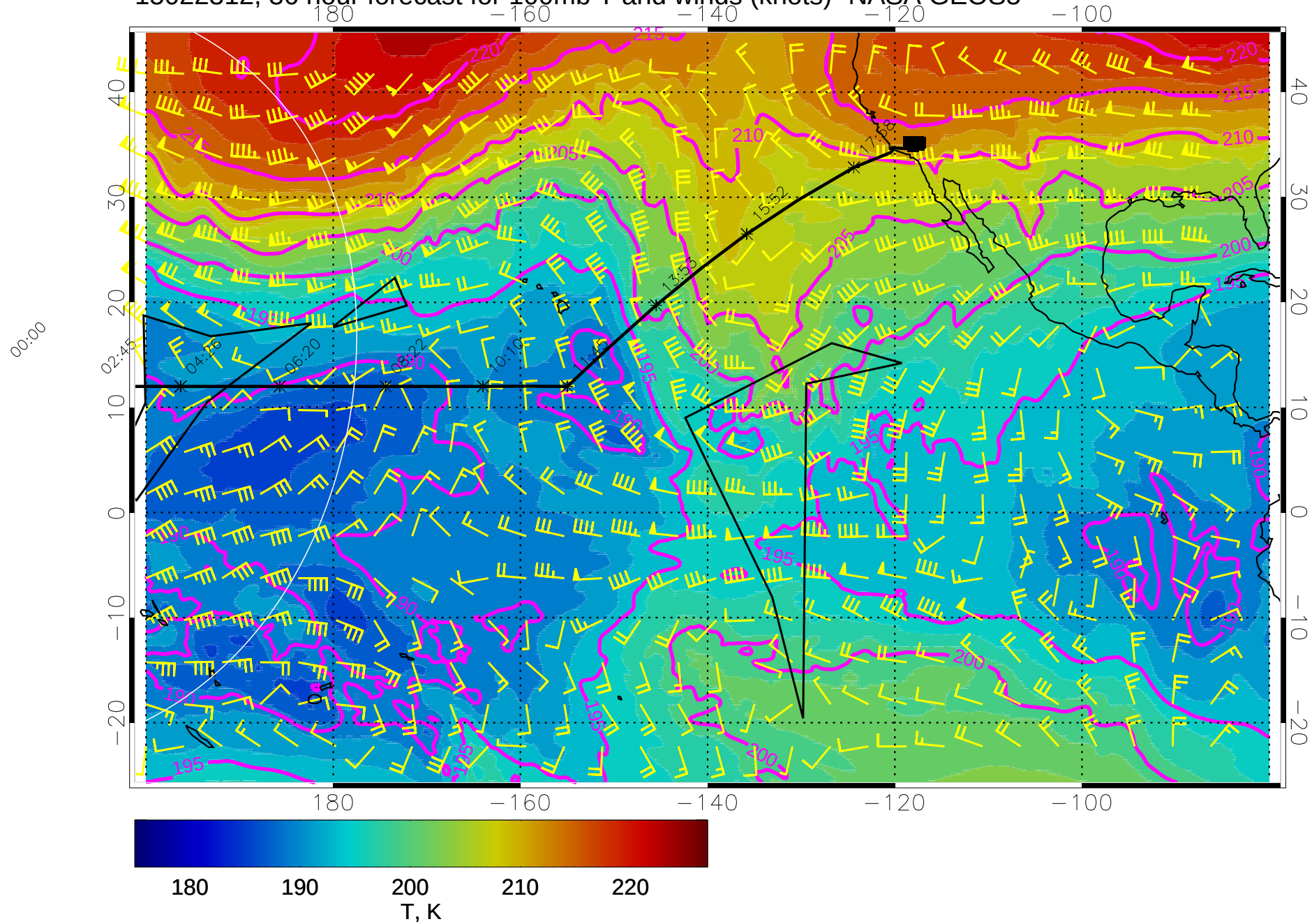
15022312, 36 hour forecast for 100mb T and winds (knots)- NASA GEOS5
