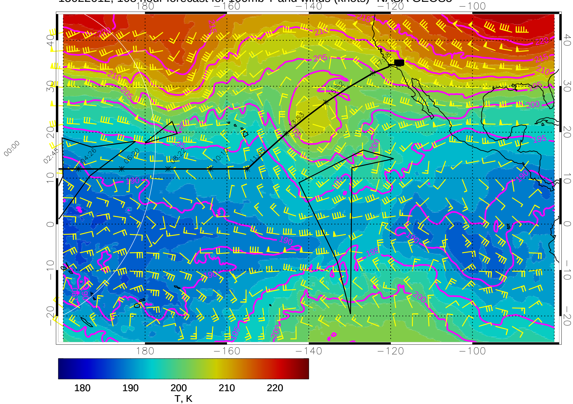
15022612, 108 hour forecast for 100mb T and winds (knots)- NASA GEOS5
