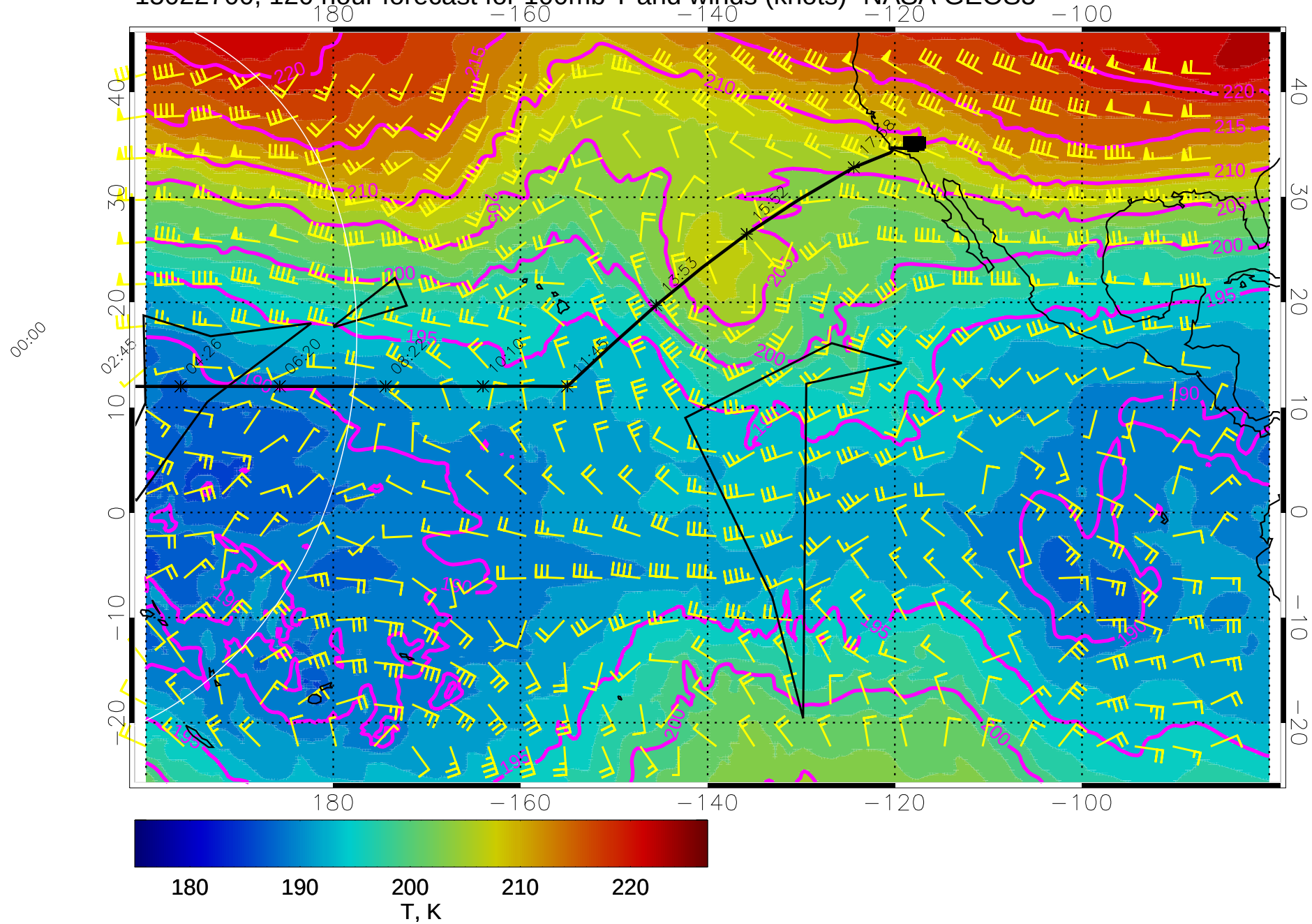
15022700, 120 hour forecast for 100mb T and winds (knots)- NASA GEOS5
