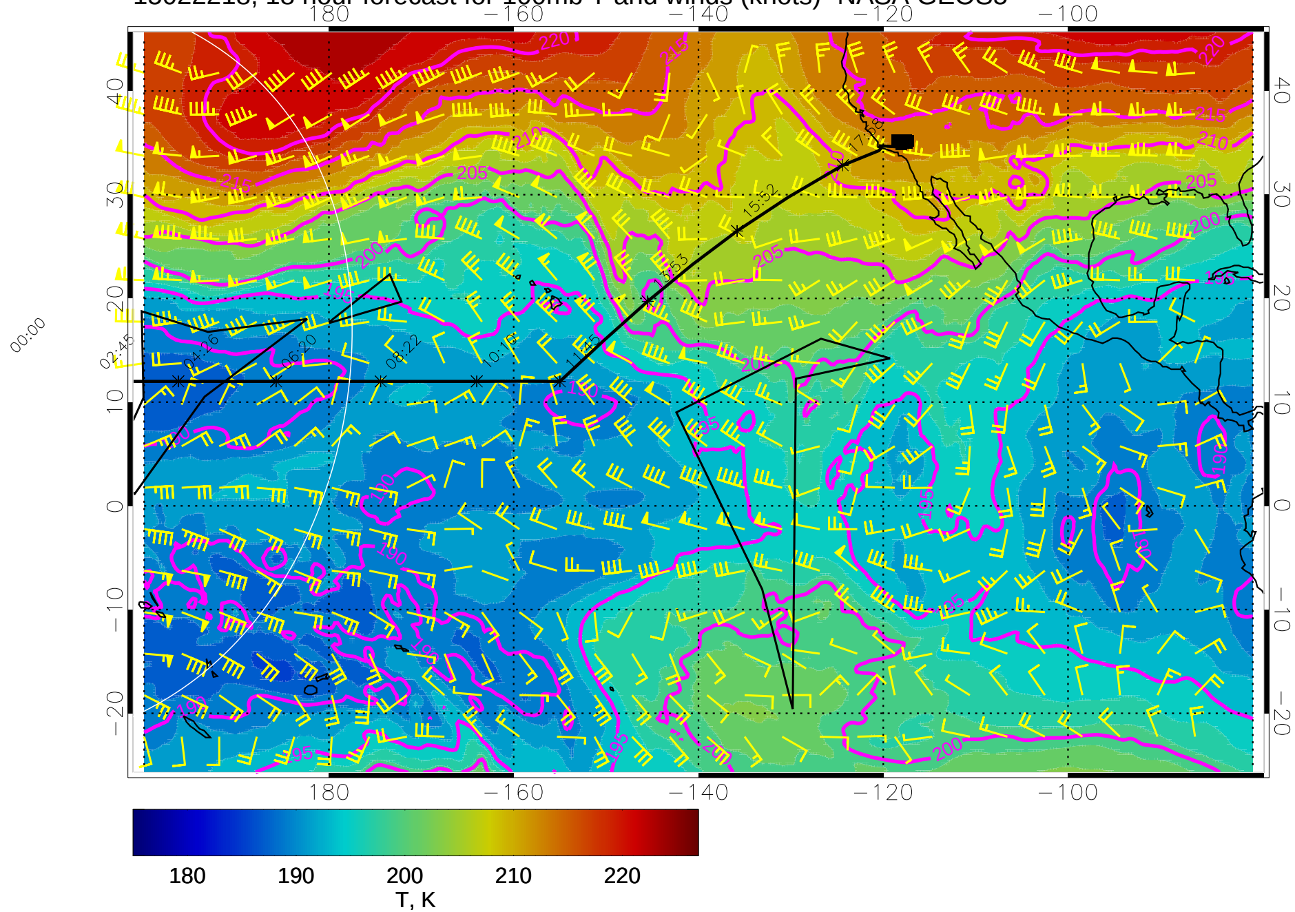
15022218, 18 hour forecast for 100mb T and winds (knots)- NASA GEOS5
