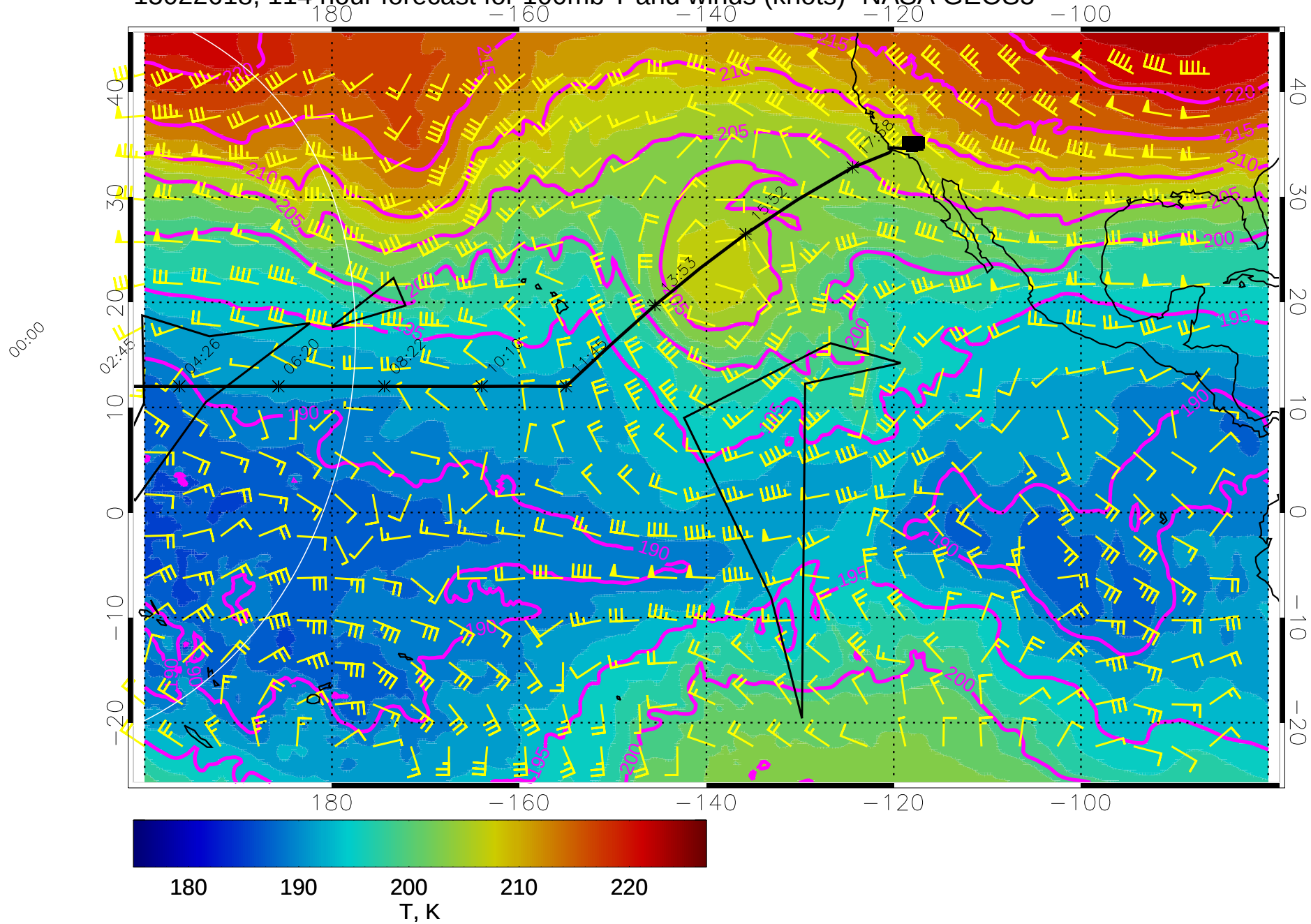
15022618, 114 hour forecast for 100mb T and winds (knots)- NASA GEOS5
