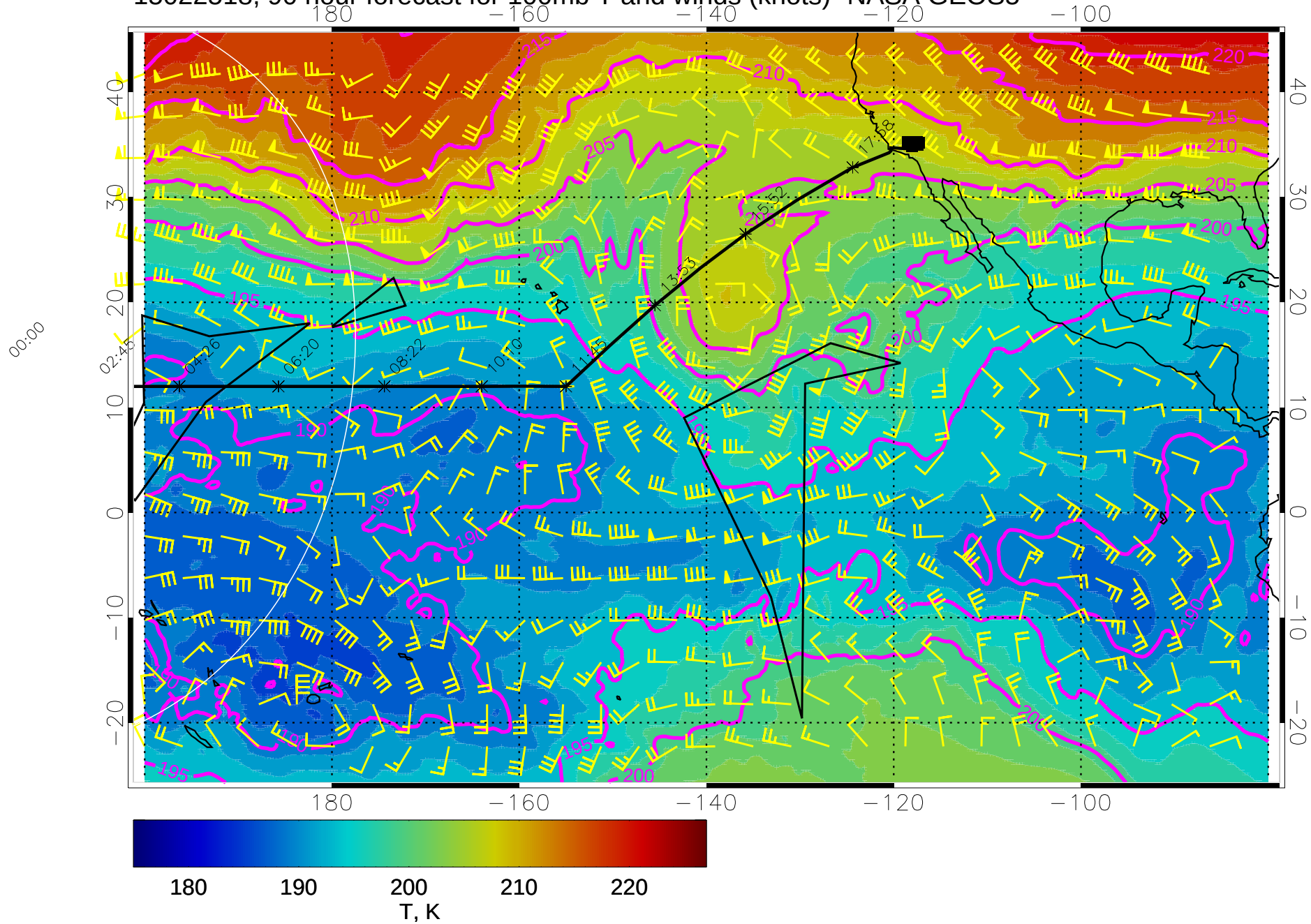
15022518, 90 hour forecast for 100mb T and winds (knots)- NASA GEOS5
