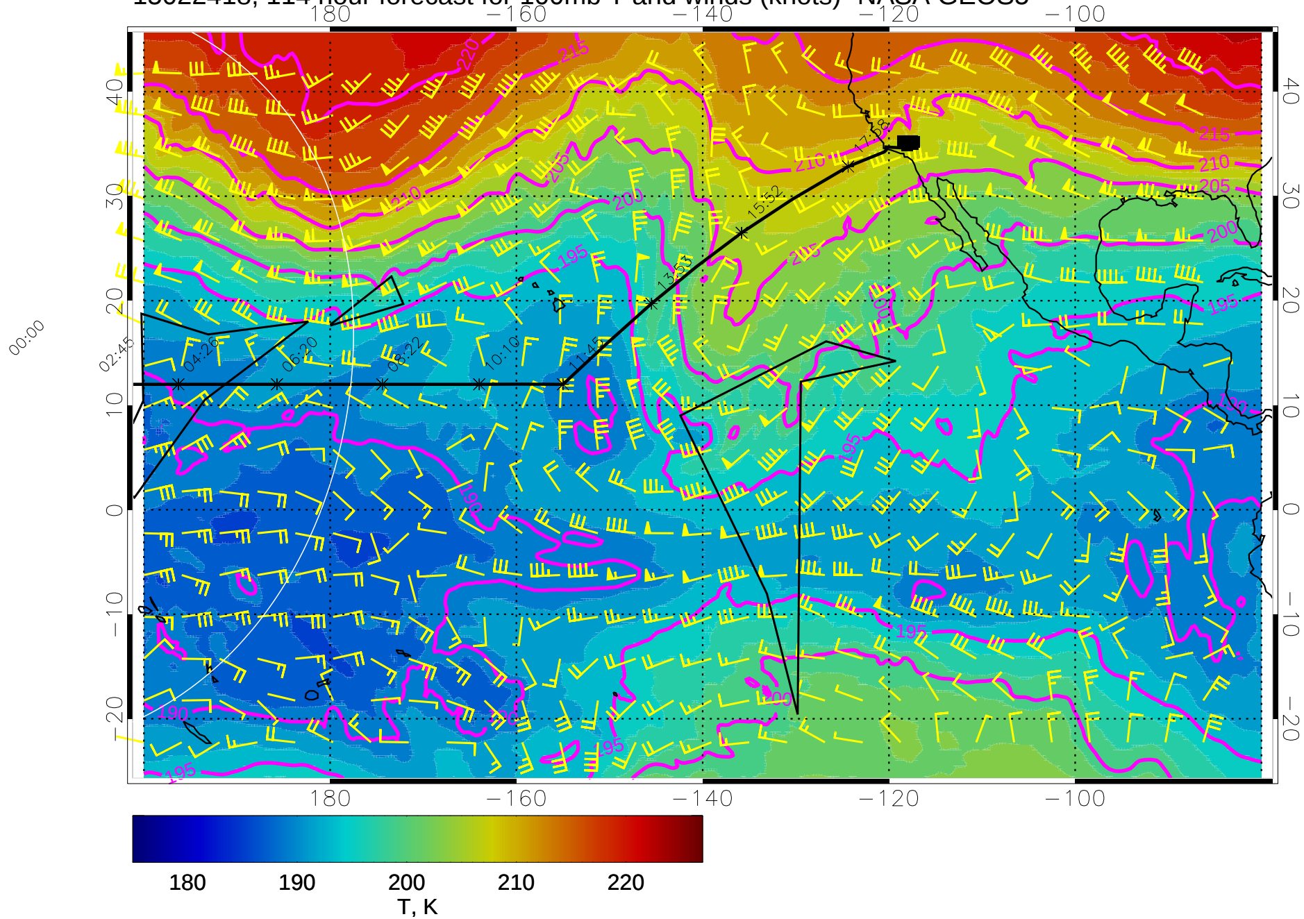
15022418, 114 hour forecast for 100mb T and winds (knots)- NASA GEOS5
