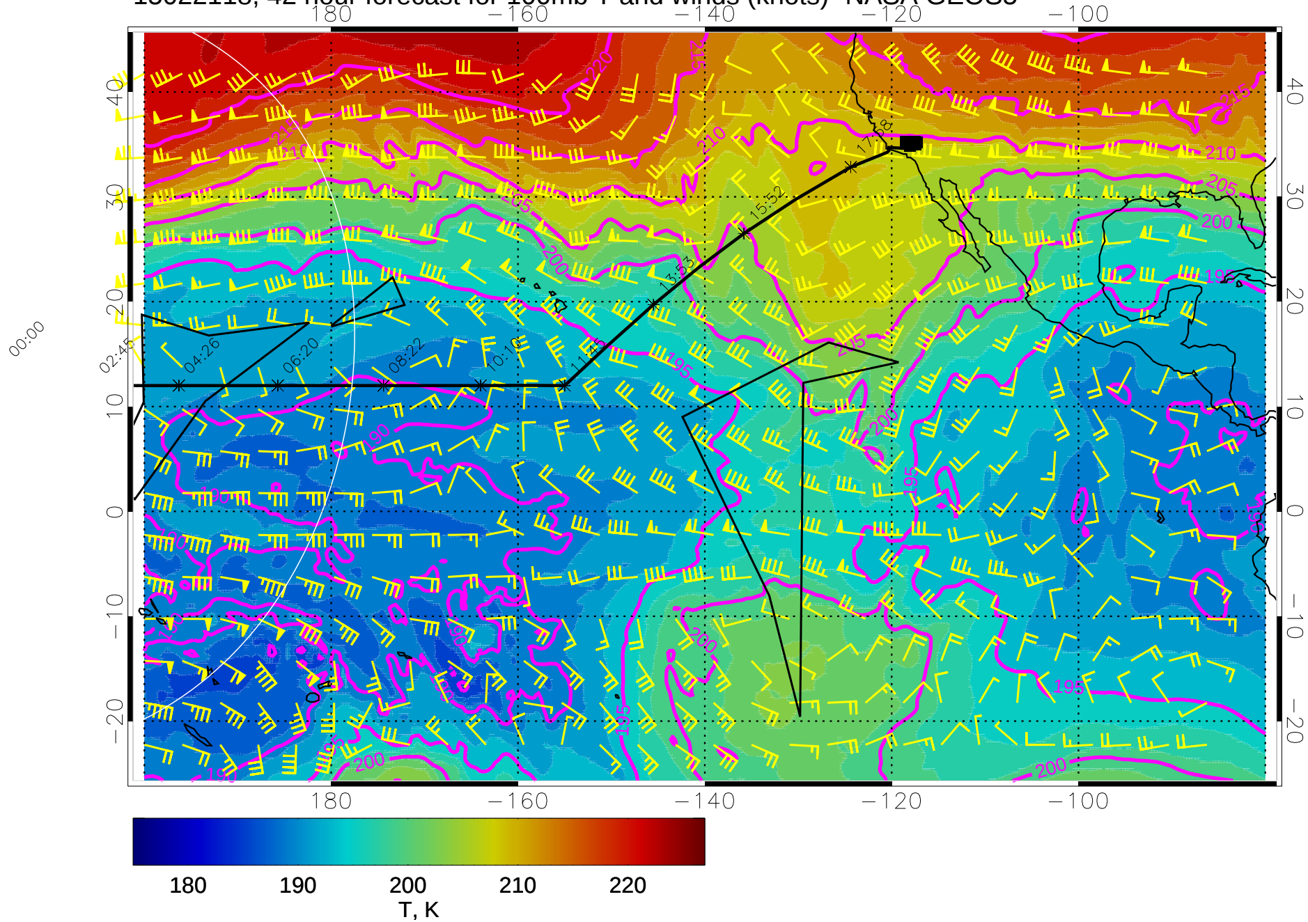
15022118, 42 hour forecast for 100mb T and winds (knots)- NASA GEOS5
