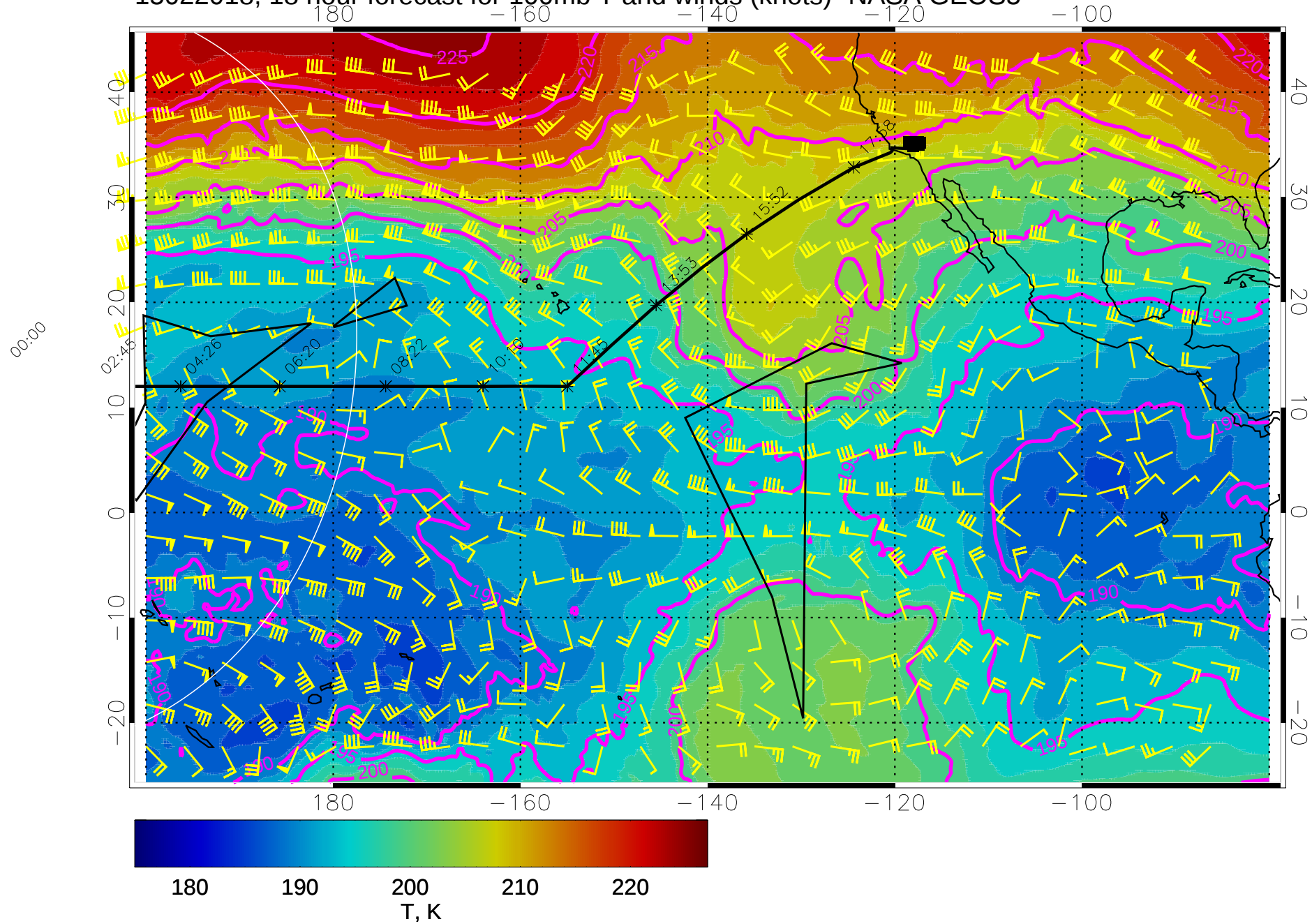
15022018, 18 hour forecast for 100mb T and winds (knots)- NASA GEOS5
