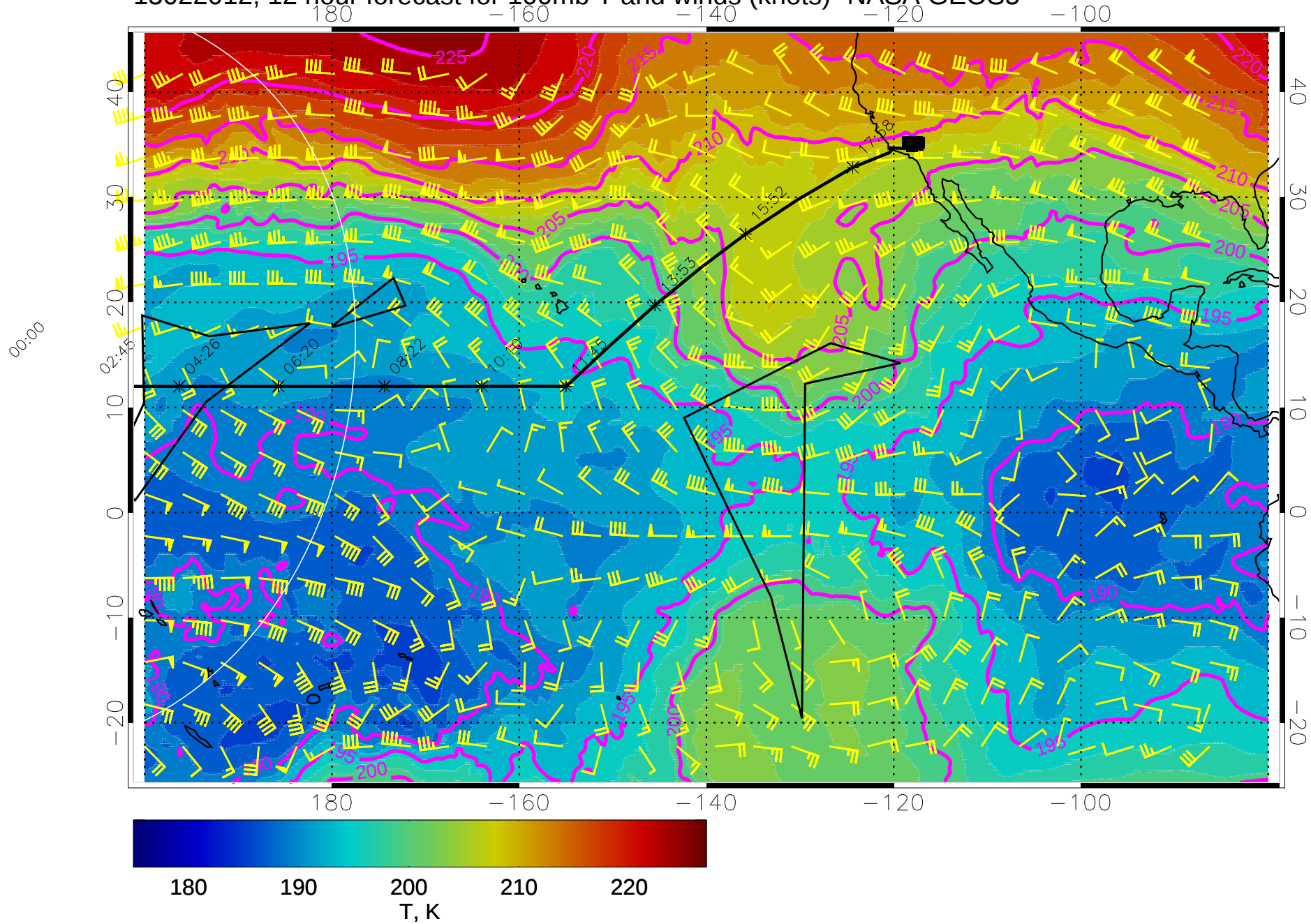
15022012, 12 hour forecast for 100mb T and winds (knots)- NASA GEOS5
