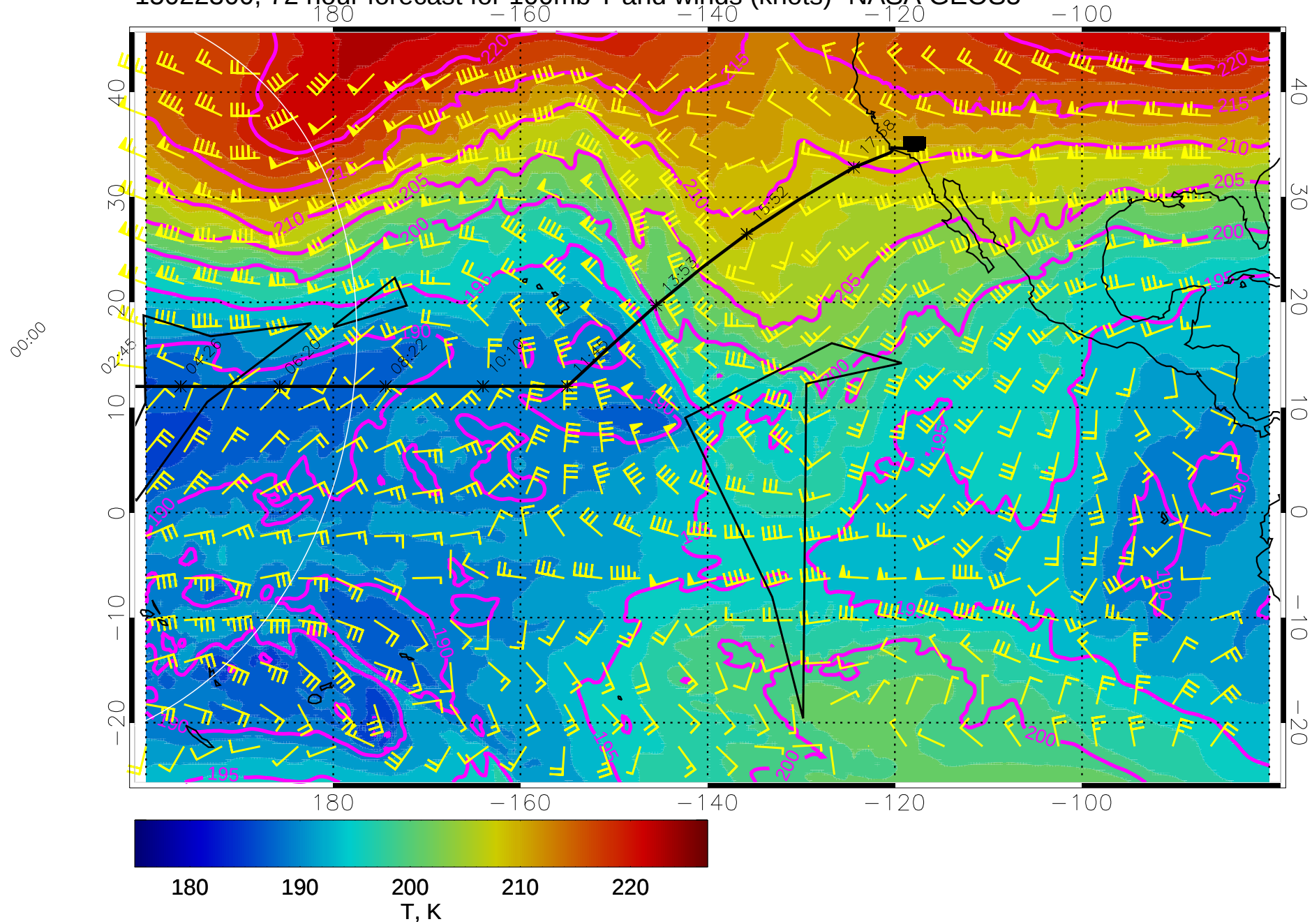
15022300, 72 hour forecast for 100mb T and winds (knots)- NASA GEOS5
