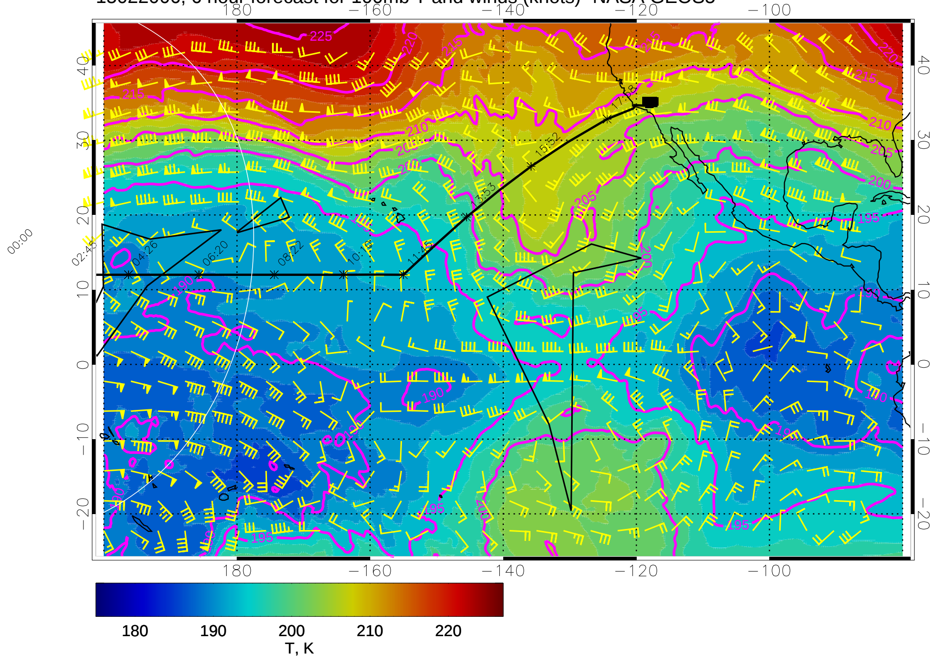
15022006, 6 hour forecast for 100mb T and winds (knots)- NASA GEOS5
