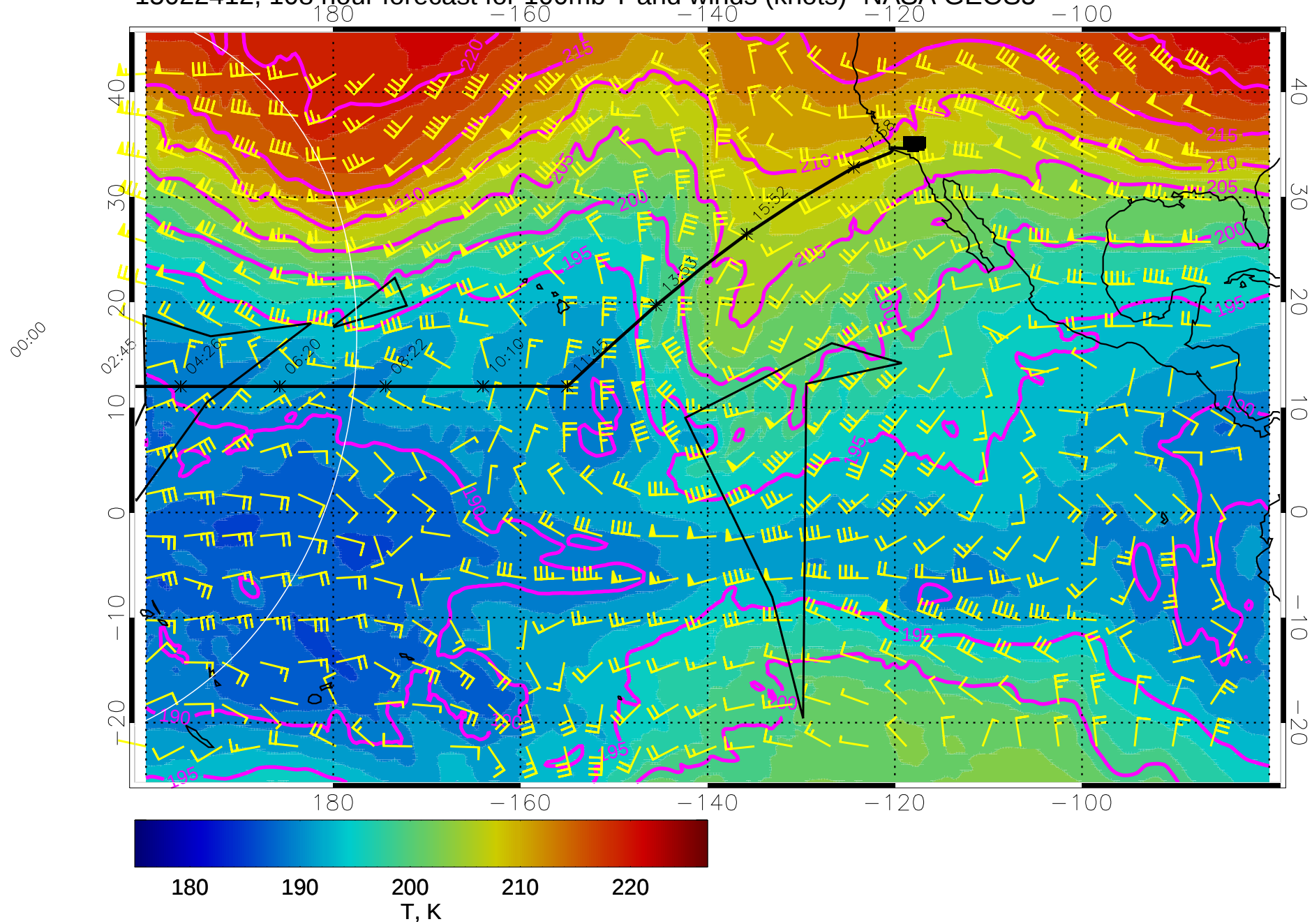
15022412, 108 hour forecast for 100mb T and winds (knots)- NASA GEOS5
