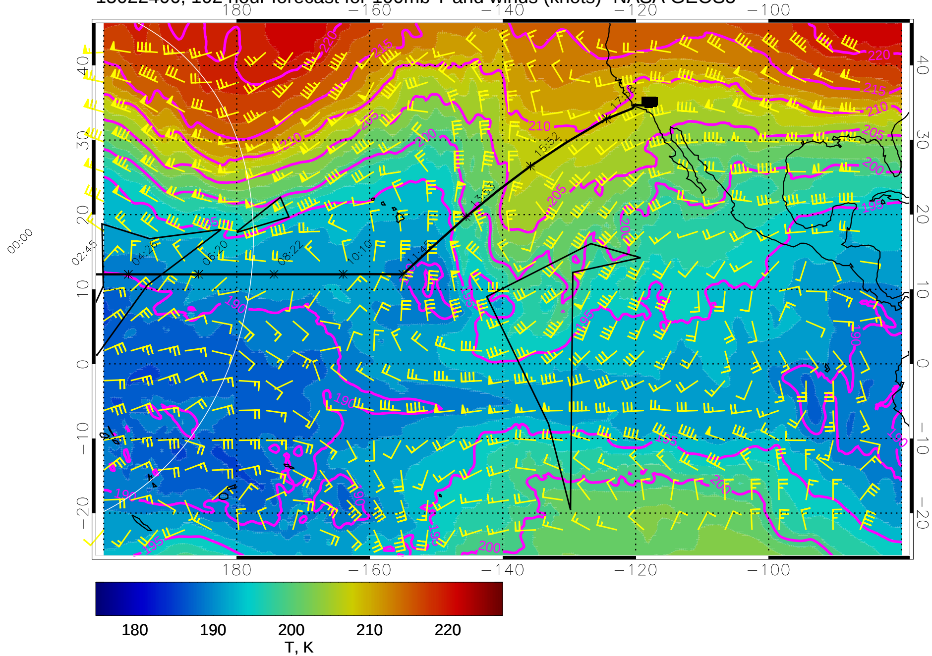
15022406, 102 hour forecast for 100mb T and winds (knots)- NASA GEOS5
