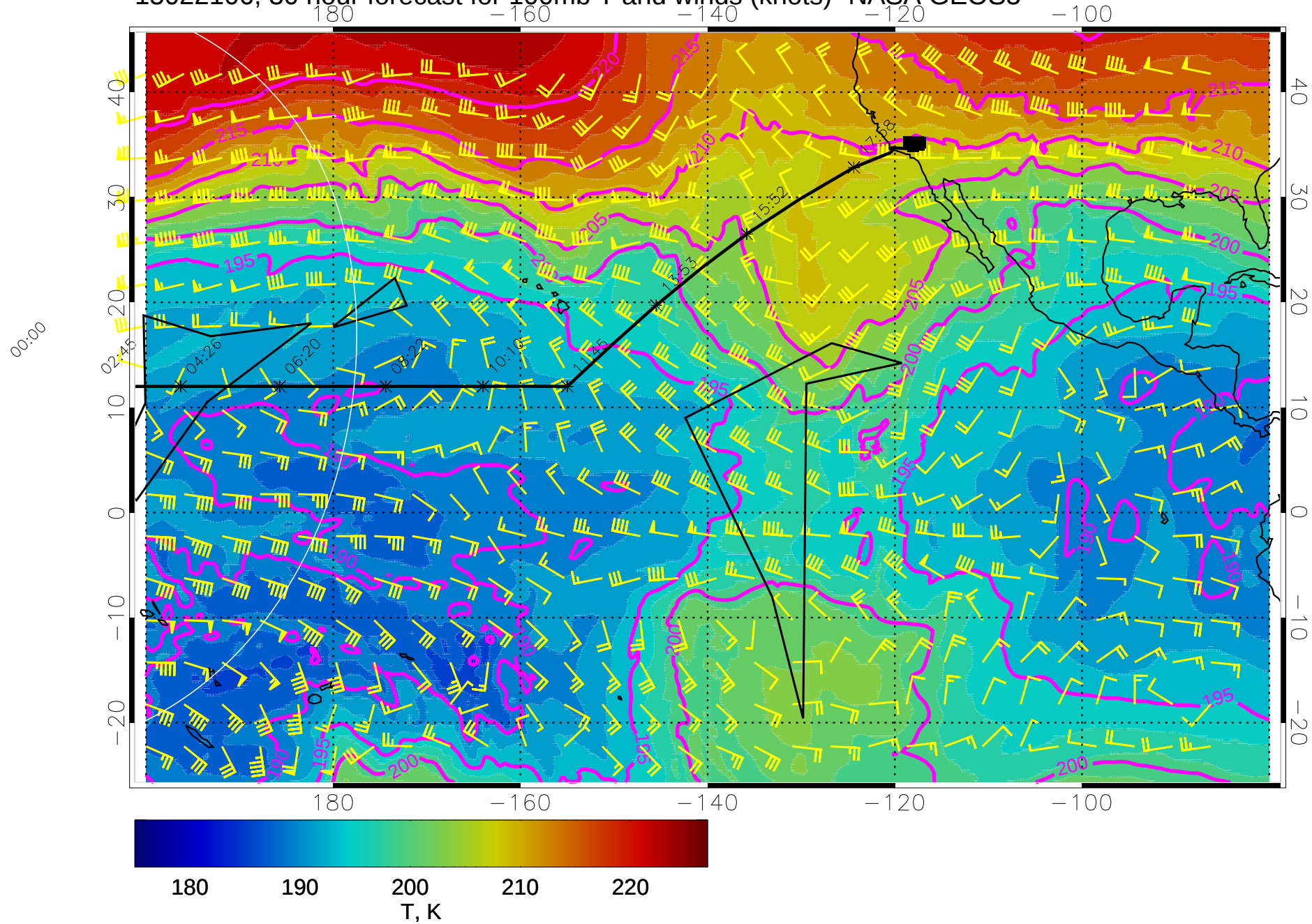
15022106, 30 hour forecast for 100mb T and winds (knots)- NASA GEOS5
