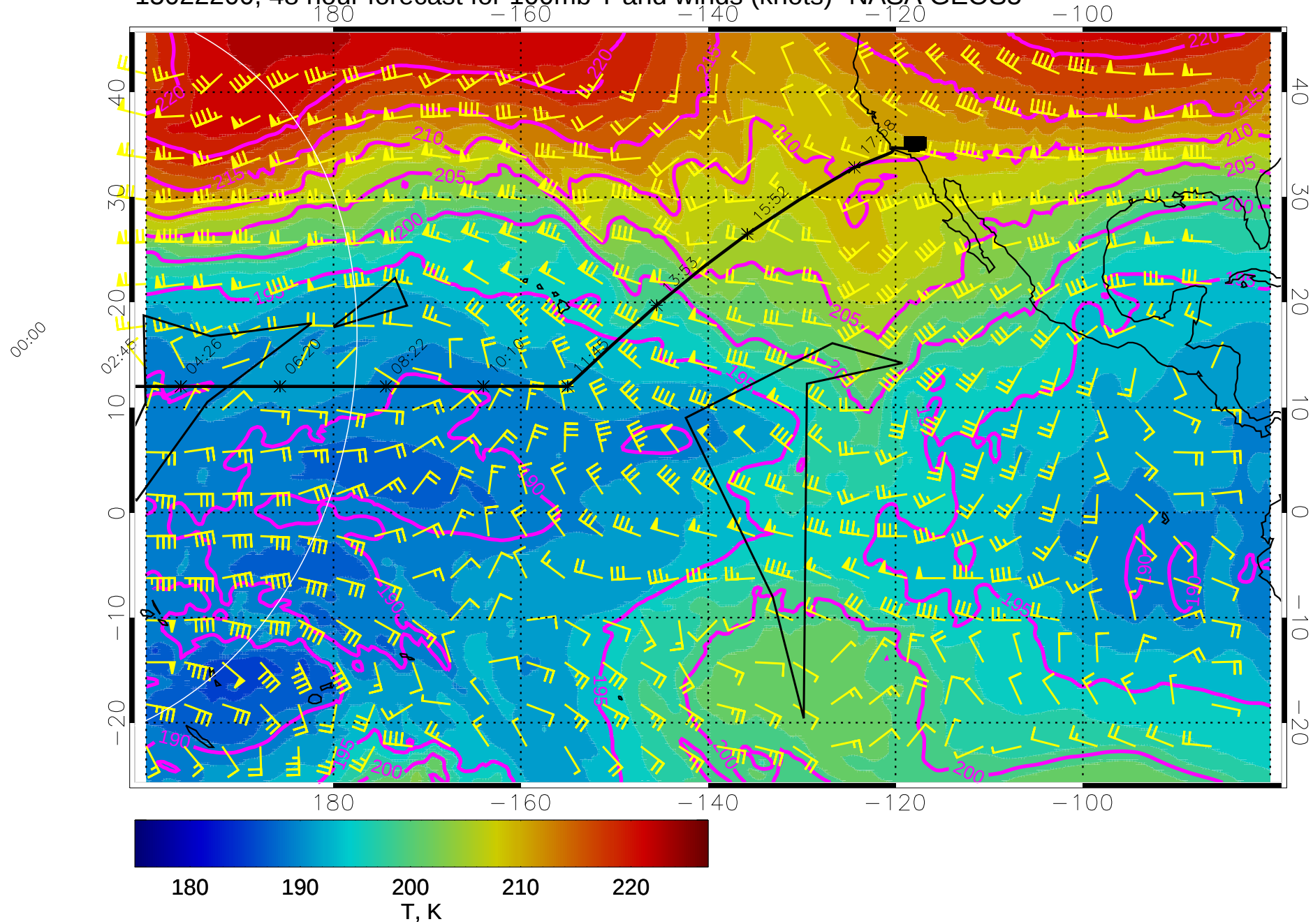
15022200, 48 hour forecast for 100mb T and winds (knots)- NASA GEOS5
