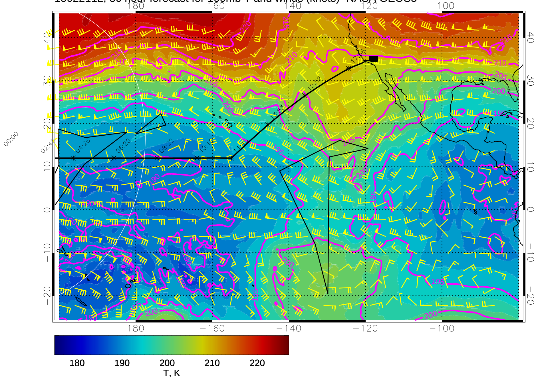
15022112, 36 hour forecast for 100mb T and winds (knots)- NASA GEOS5
