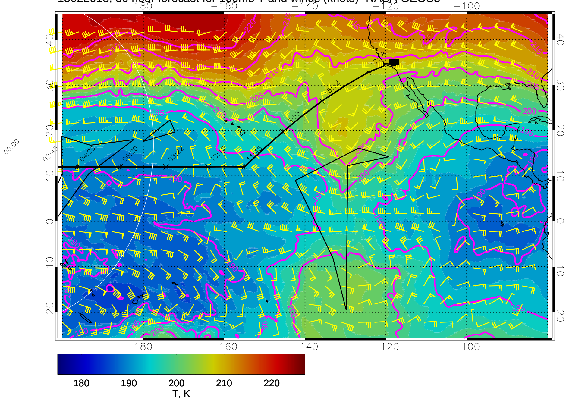
15022018, 30 hour forecast for 100mb T and winds (knots)- NASA GEOS5
