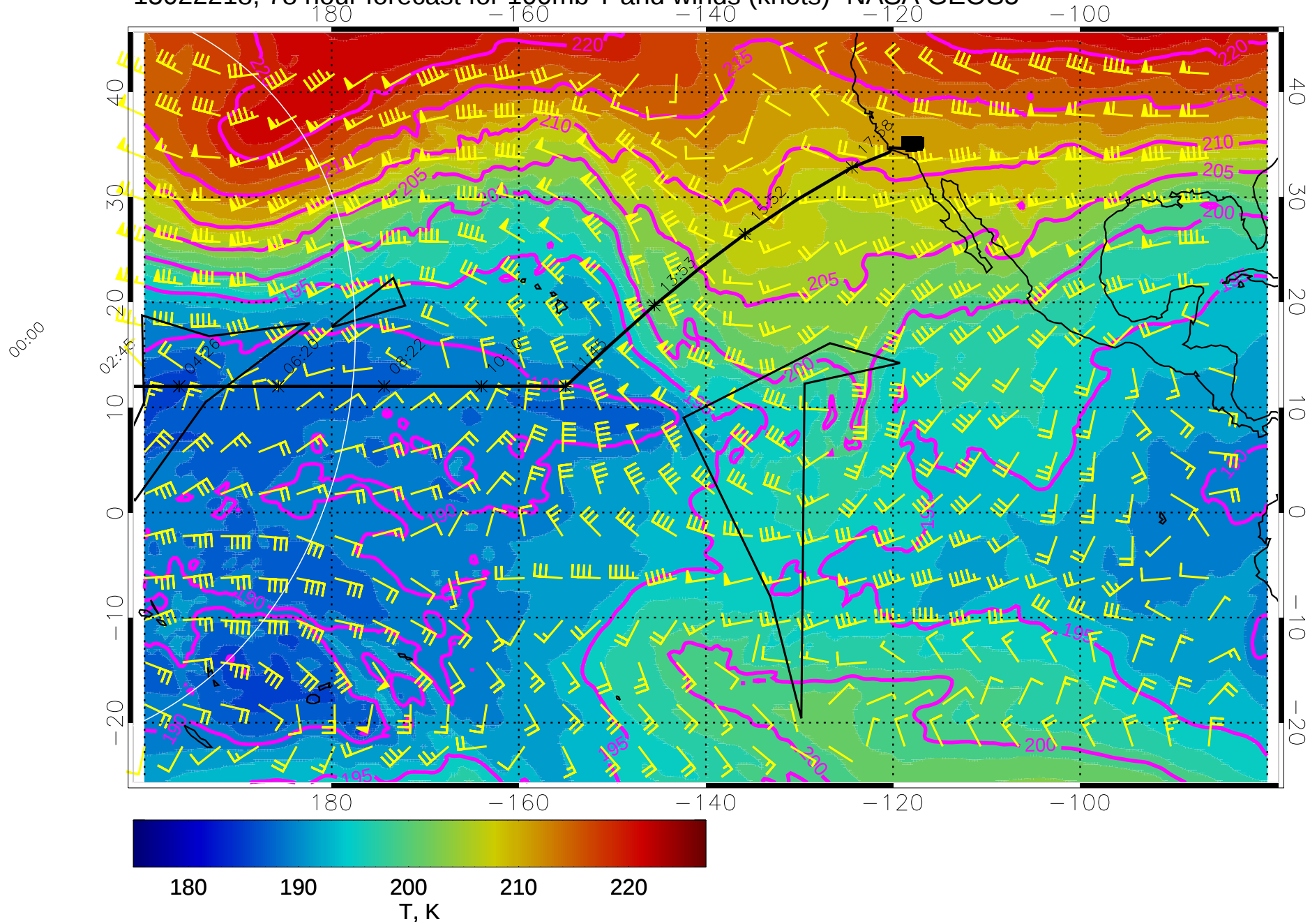
15022218, 78 hour forecast for 100mb T and winds (knots)- NASA GEOS5
