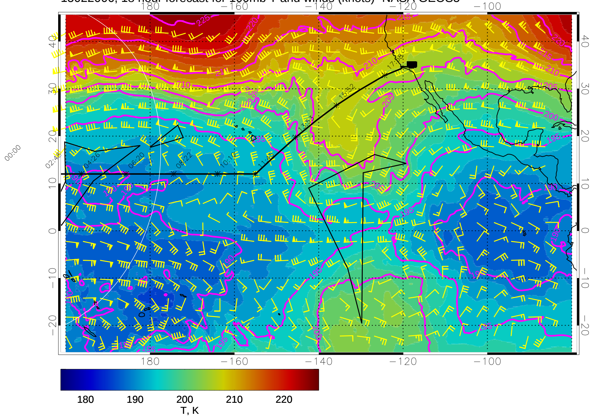
15022006, 18 hour forecast for 100mb T and winds (knots)- NASA GEOS5
