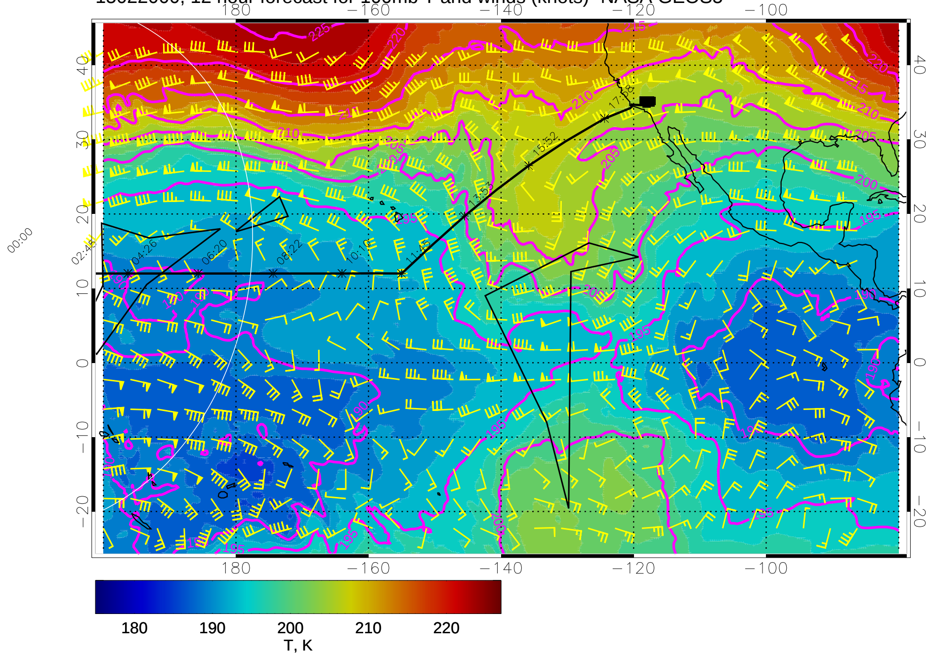
15022000, 12 hour forecast for 100mb T and winds (knots)- NASA GEOS5
