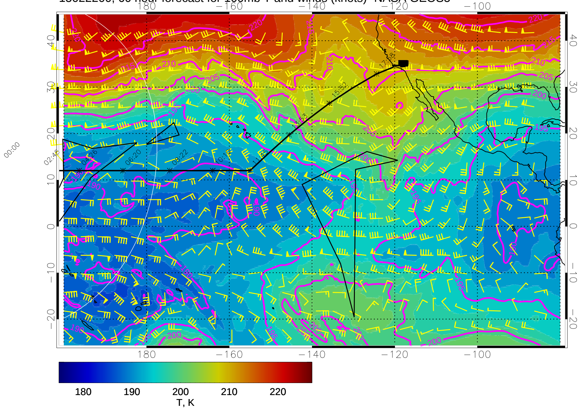
15022200, 60 hour forecast for 100mb T and winds (knots)- NASA GEOS5
