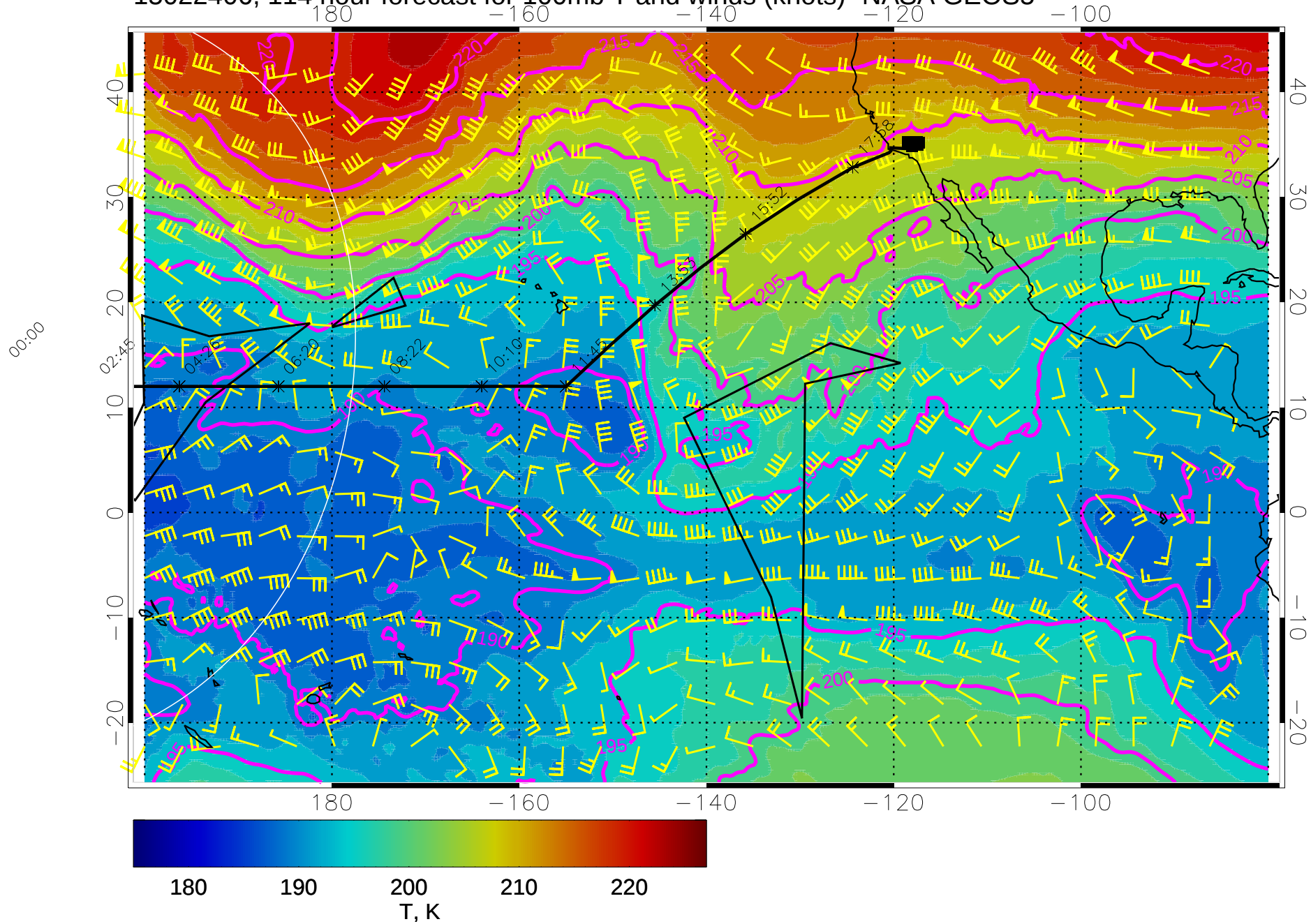
15022406, 114 hour forecast for 100mb T and winds (knots)- NASA GEOS5
