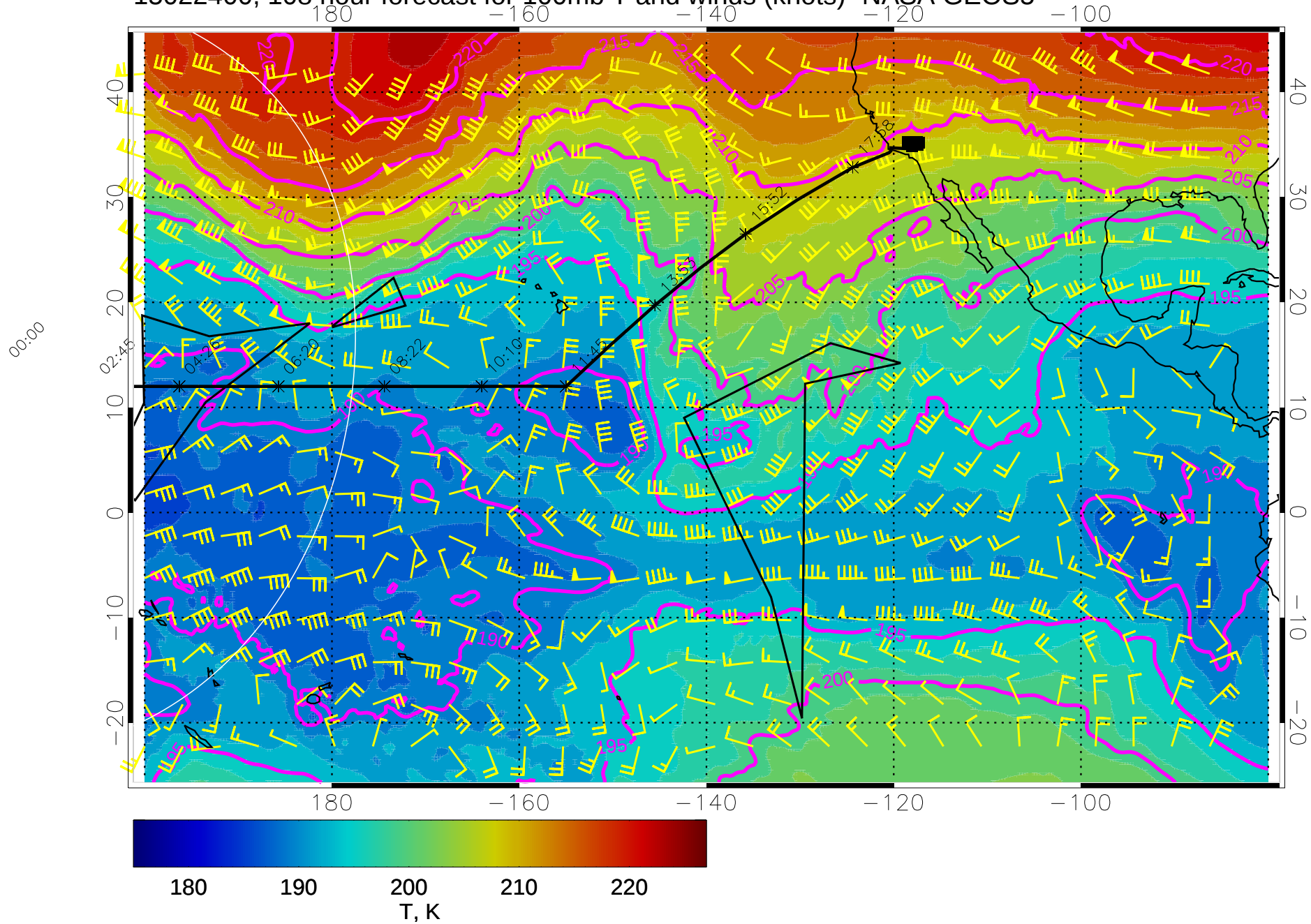
15022400, 108 hour forecast for 100mb T and winds (knots)- NASA GEOS5
