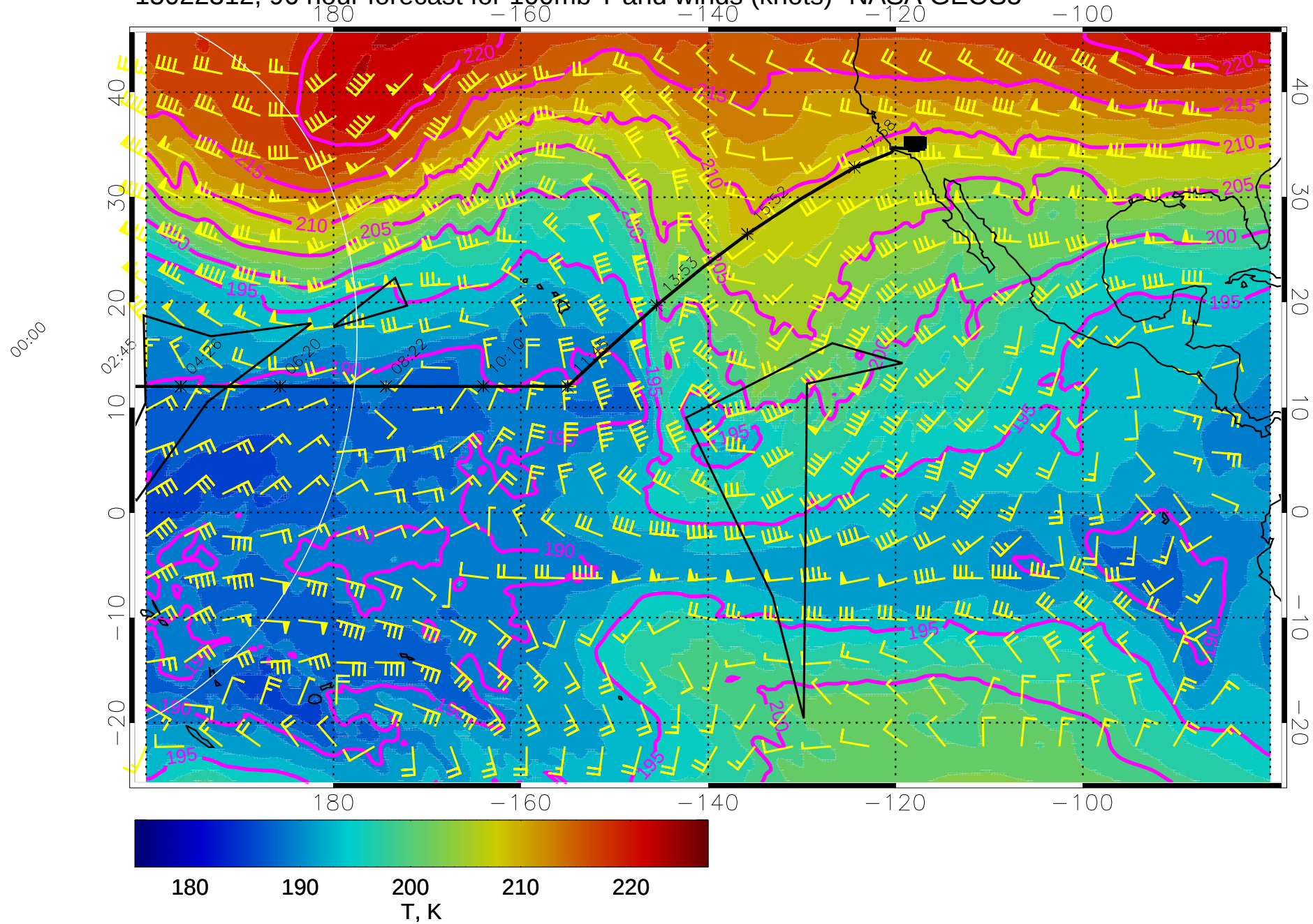
15022312, 96 hour forecast for 100mb T and winds (knots)- NASA GEOS5
