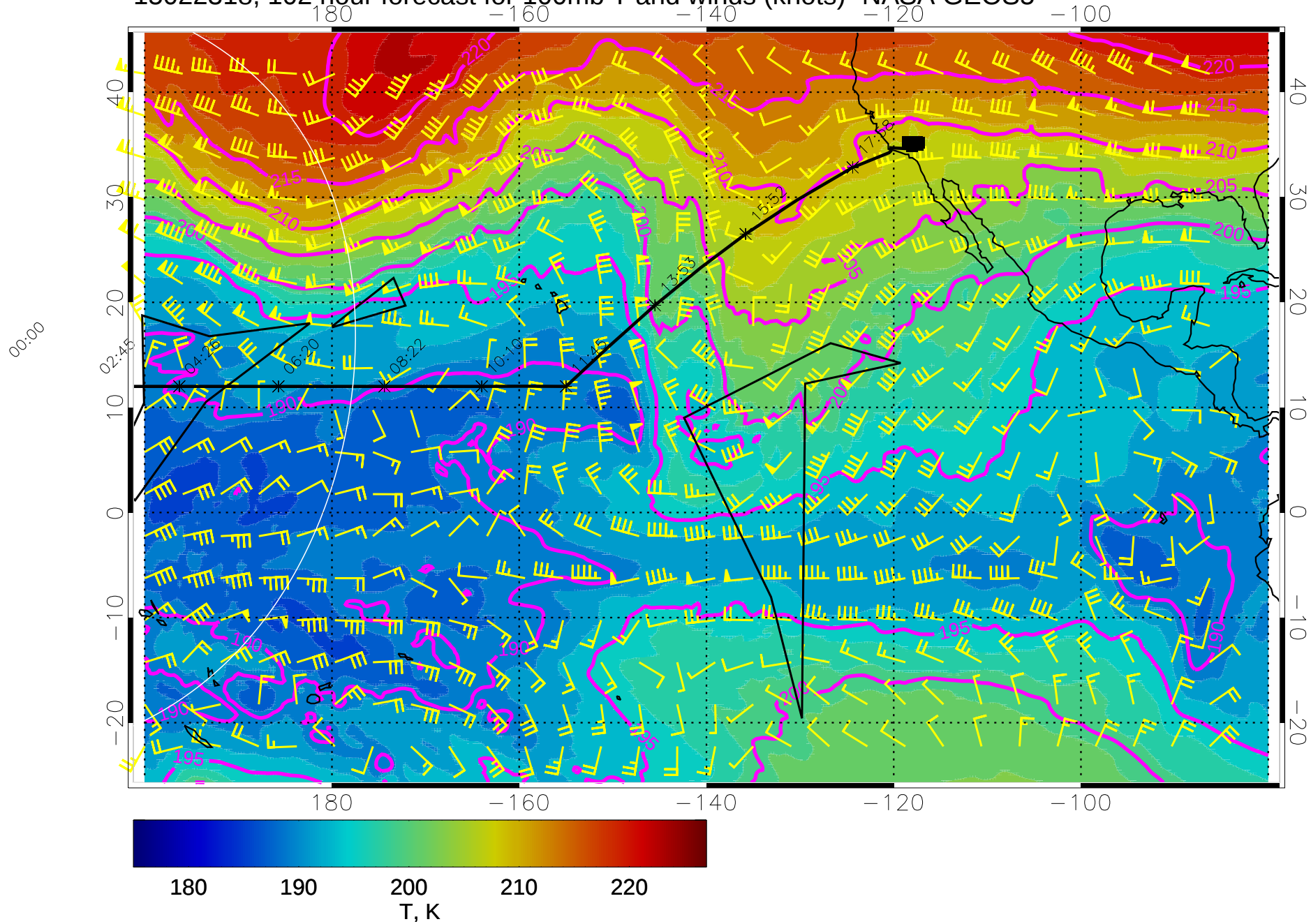
15022318, 102 hour forecast for 100mb T and winds (knots)- NASA GEOS5
