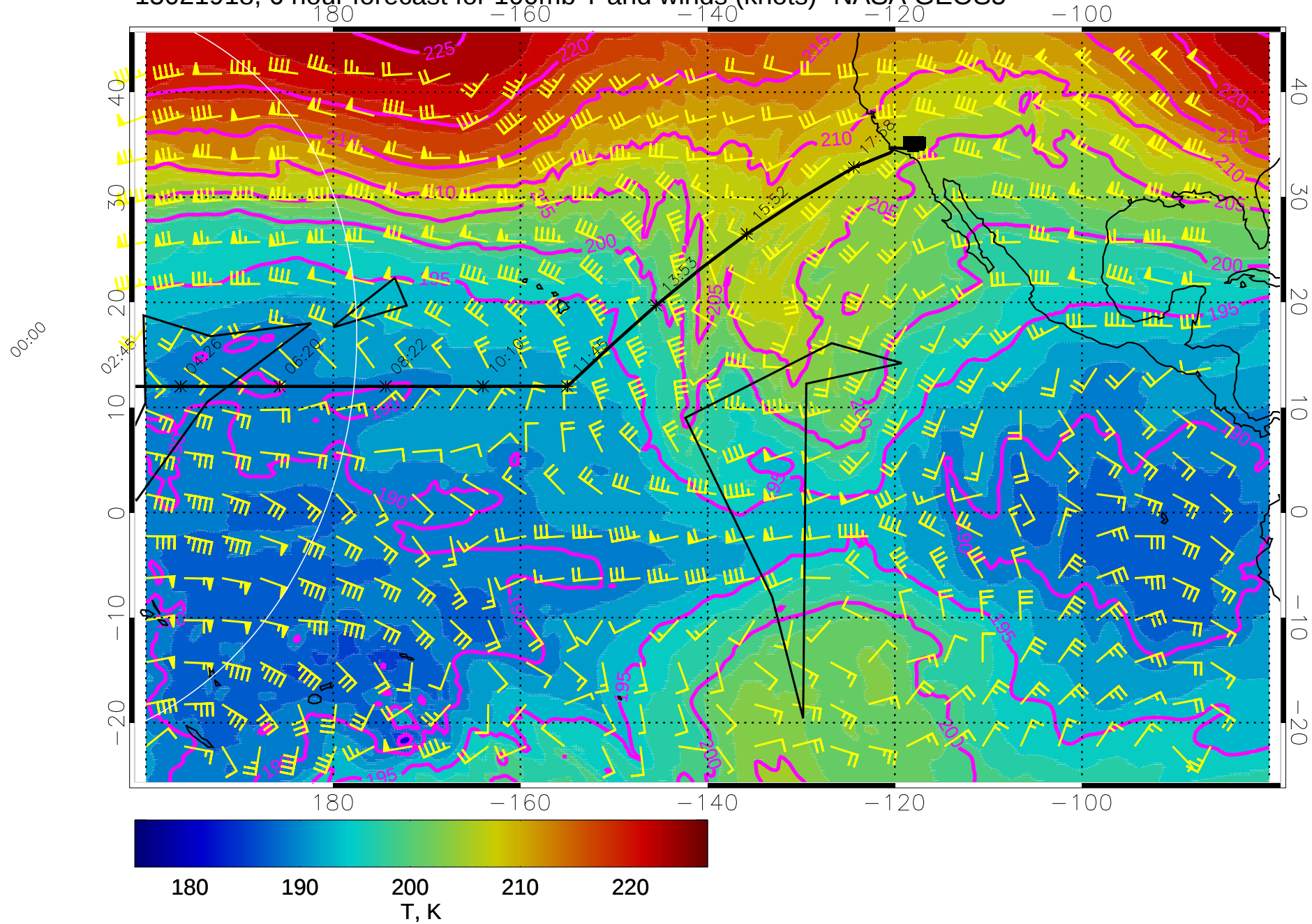
15021918, 6 hour forecast for 100mb T and winds (knots)- NASA GEOS5
