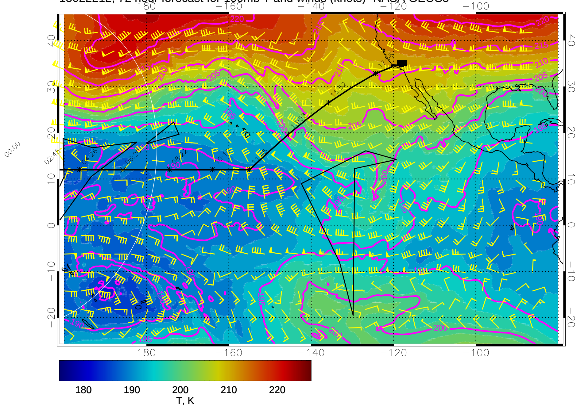
15022212, 72 hour forecast for 100mb T and winds (knots)- NASA GEOS5
