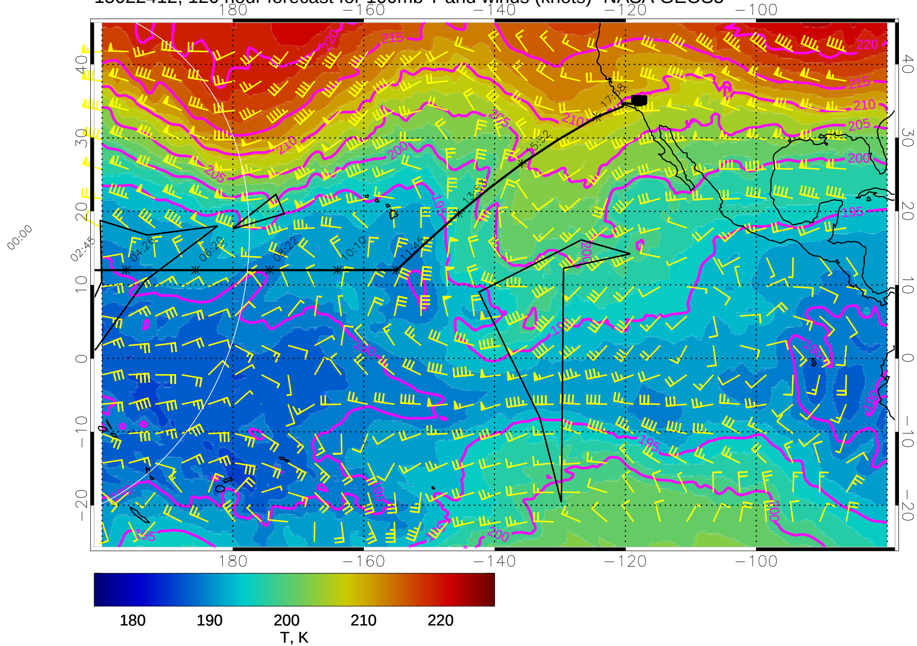
15022412, 120 hour forecast for 100mb T and winds (knots)- NASA GEOS5
