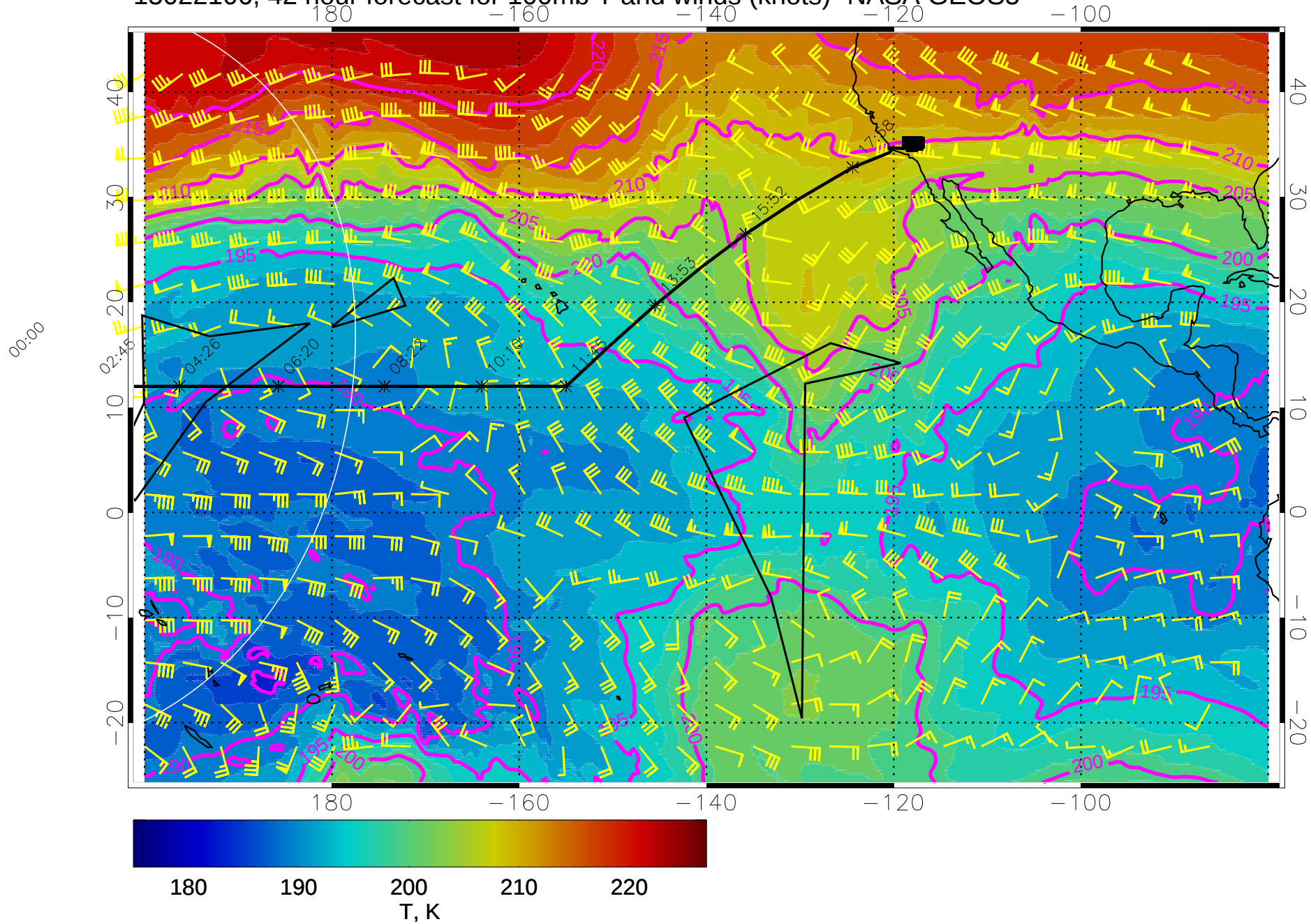
15022106, 42 hour forecast for 100mb T and winds (knots)- NASA GEOS5
