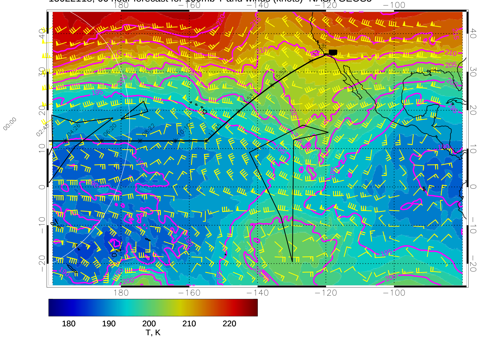
15022118, 66 hour forecast for 100mb T and winds (knots)- NASA GEOS5
