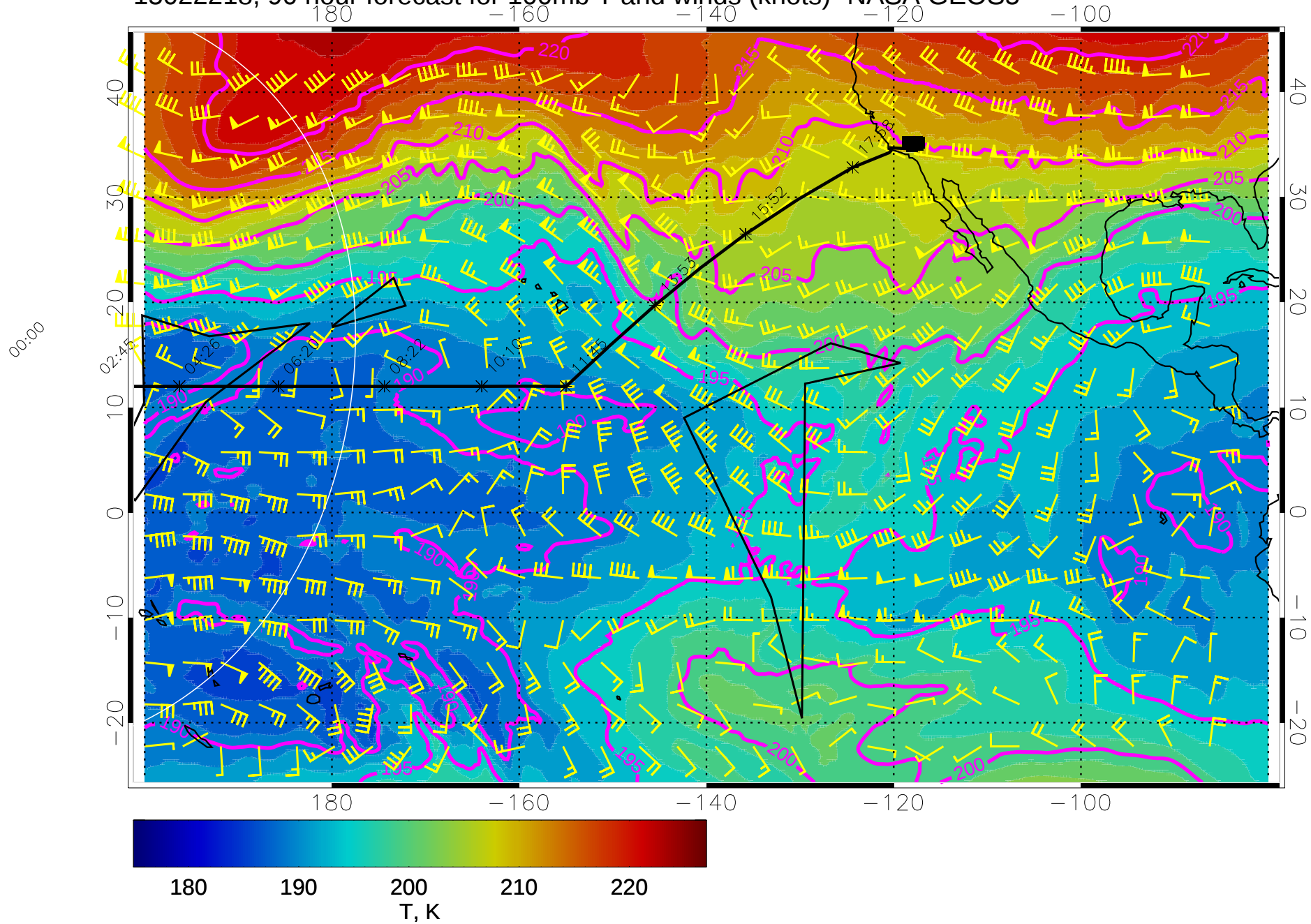
15022218, 90 hour forecast for 100mb T and winds (knots)- NASA GEOS5
