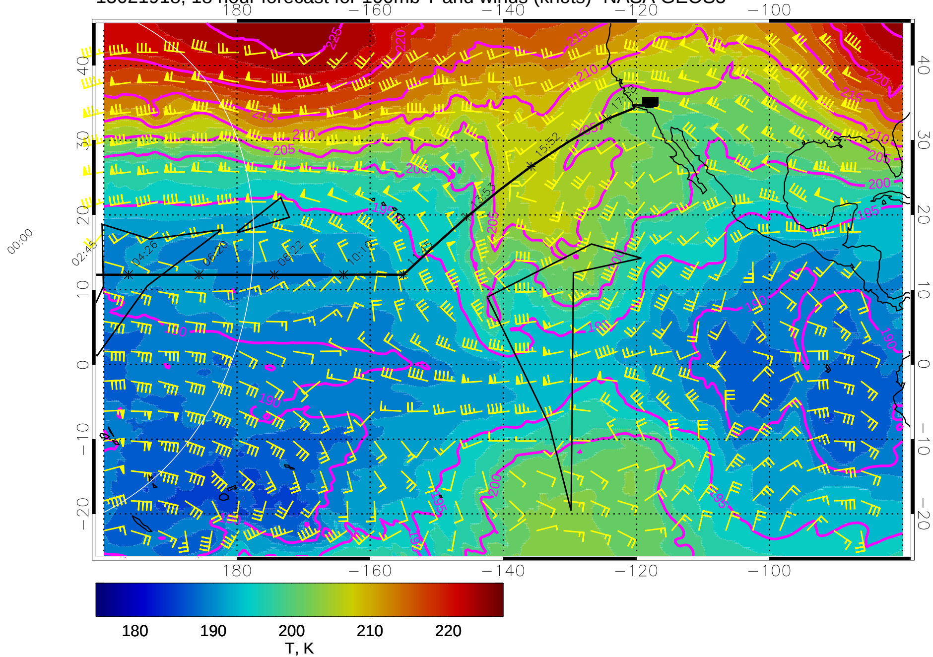
15021918, 18 hour forecast for 100mb T and winds (knots)- NASA GEOS5
