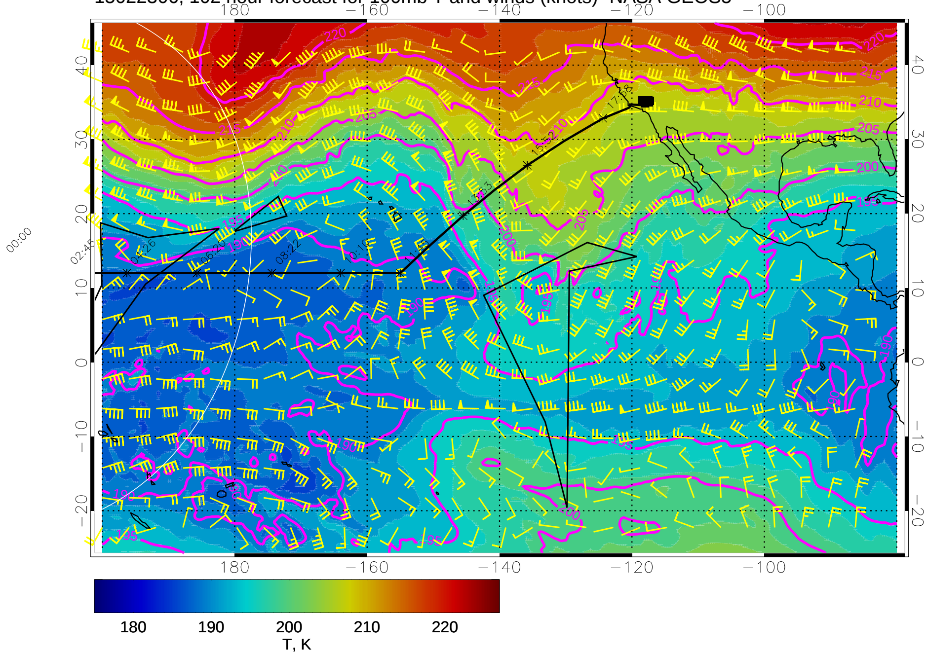
15022306, 102 hour forecast for 100mb T and winds (knots)- NASA GEOS5
