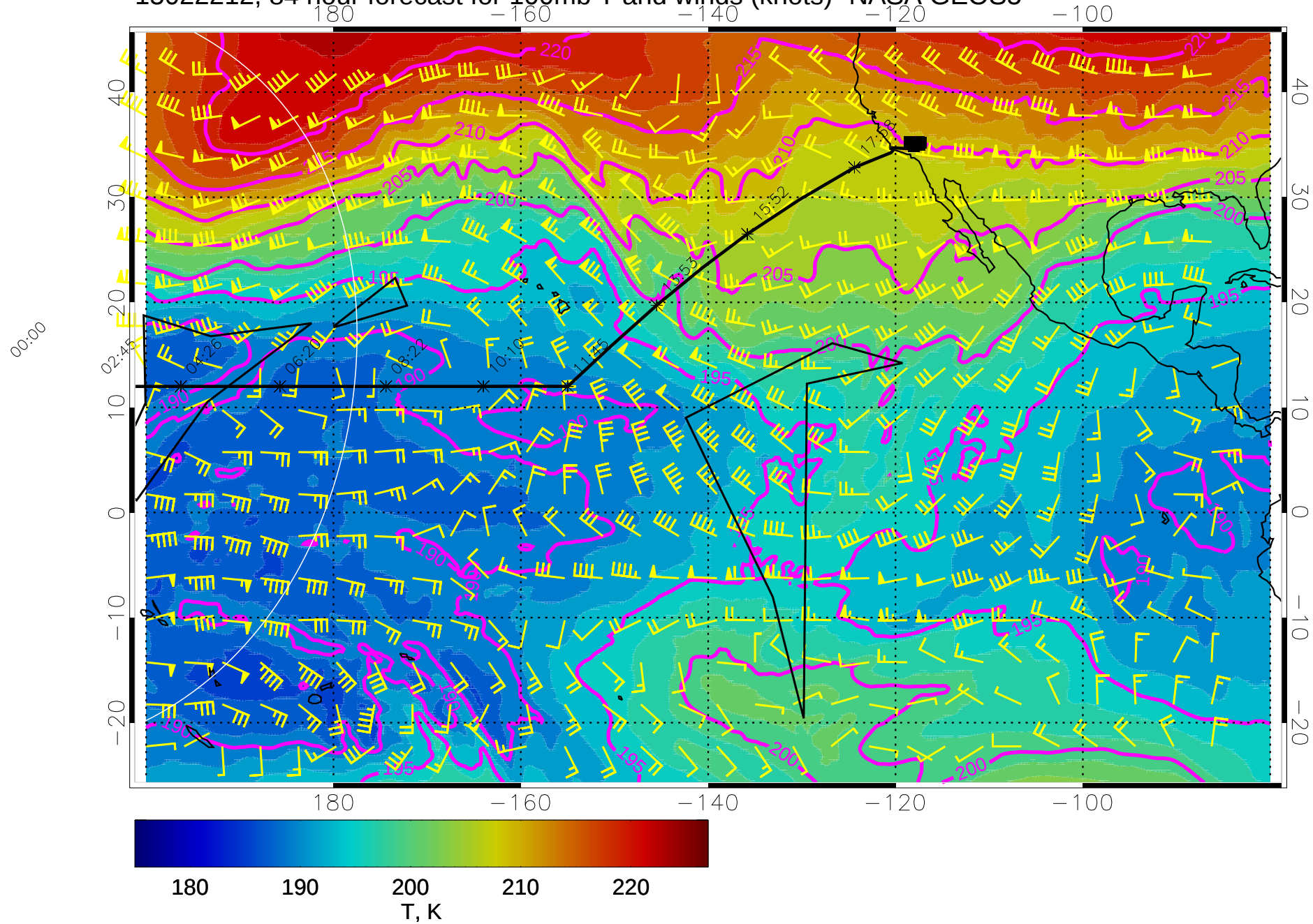
15022212, 84 hour forecast for 100mb T and winds (knots)- NASA GEOS5
