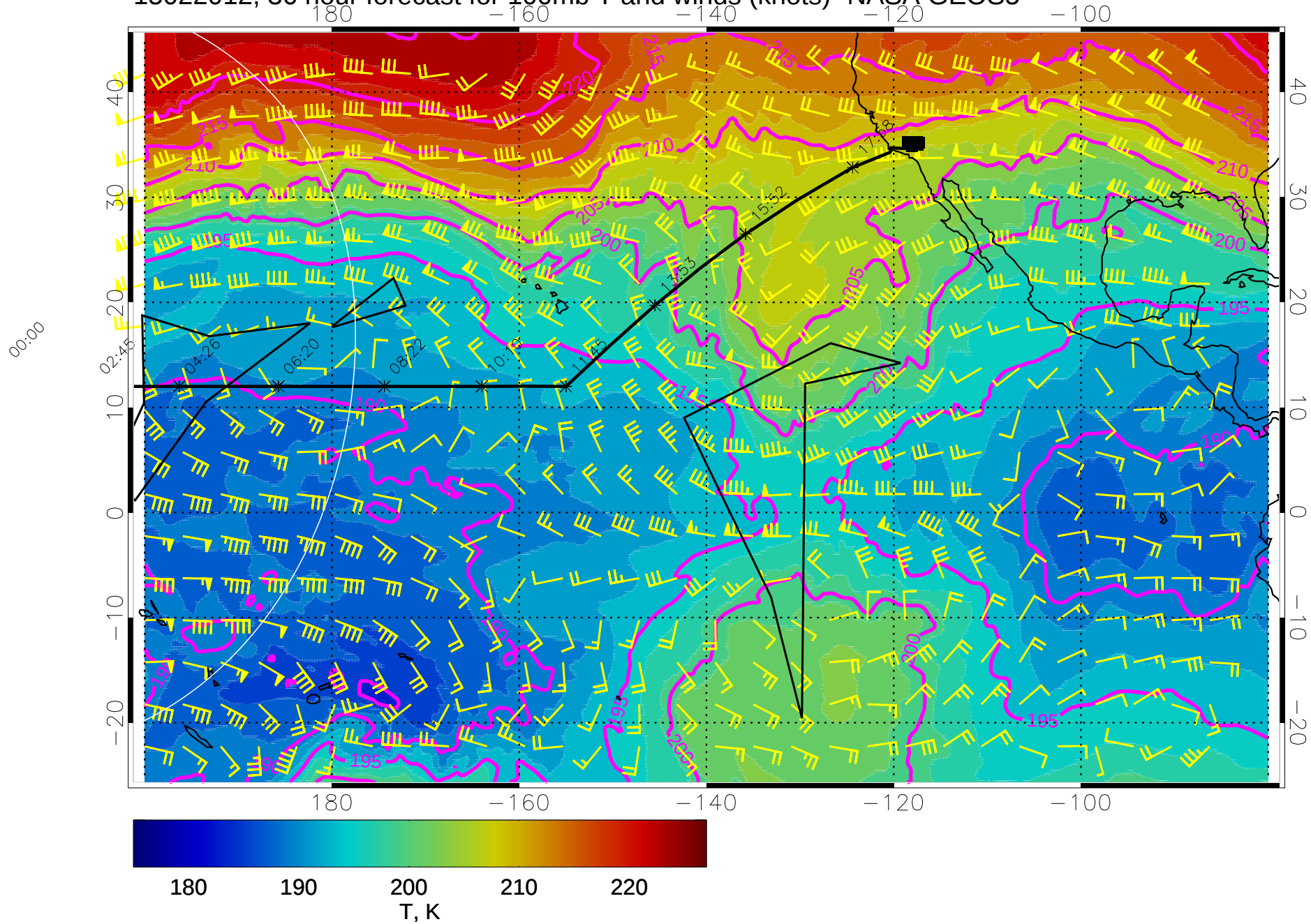
15022012, 36 hour forecast for 100mb T and winds (knots)- NASA GEOS5
