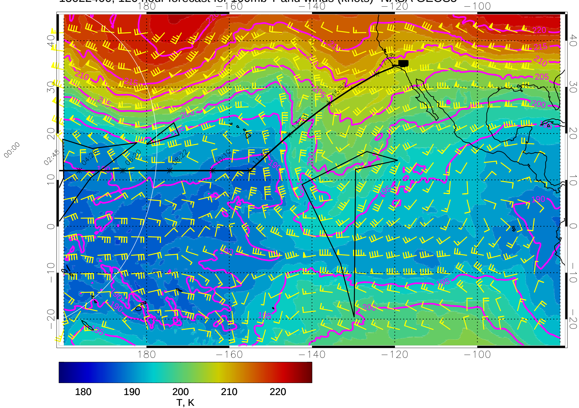
15022400, 120 hour forecast for 100mb T and winds (knots)- NASA GEOS5
