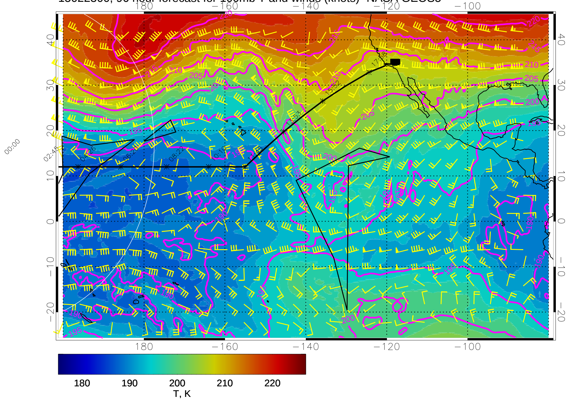
15022300, 96 hour forecast for 100mb T and winds (knots)- NASA GEOS5
