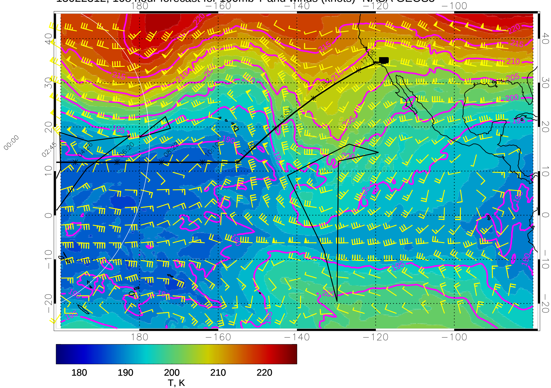
15022312, 108 hour forecast for 100mb T and winds (knots)- NASA GEOS5
