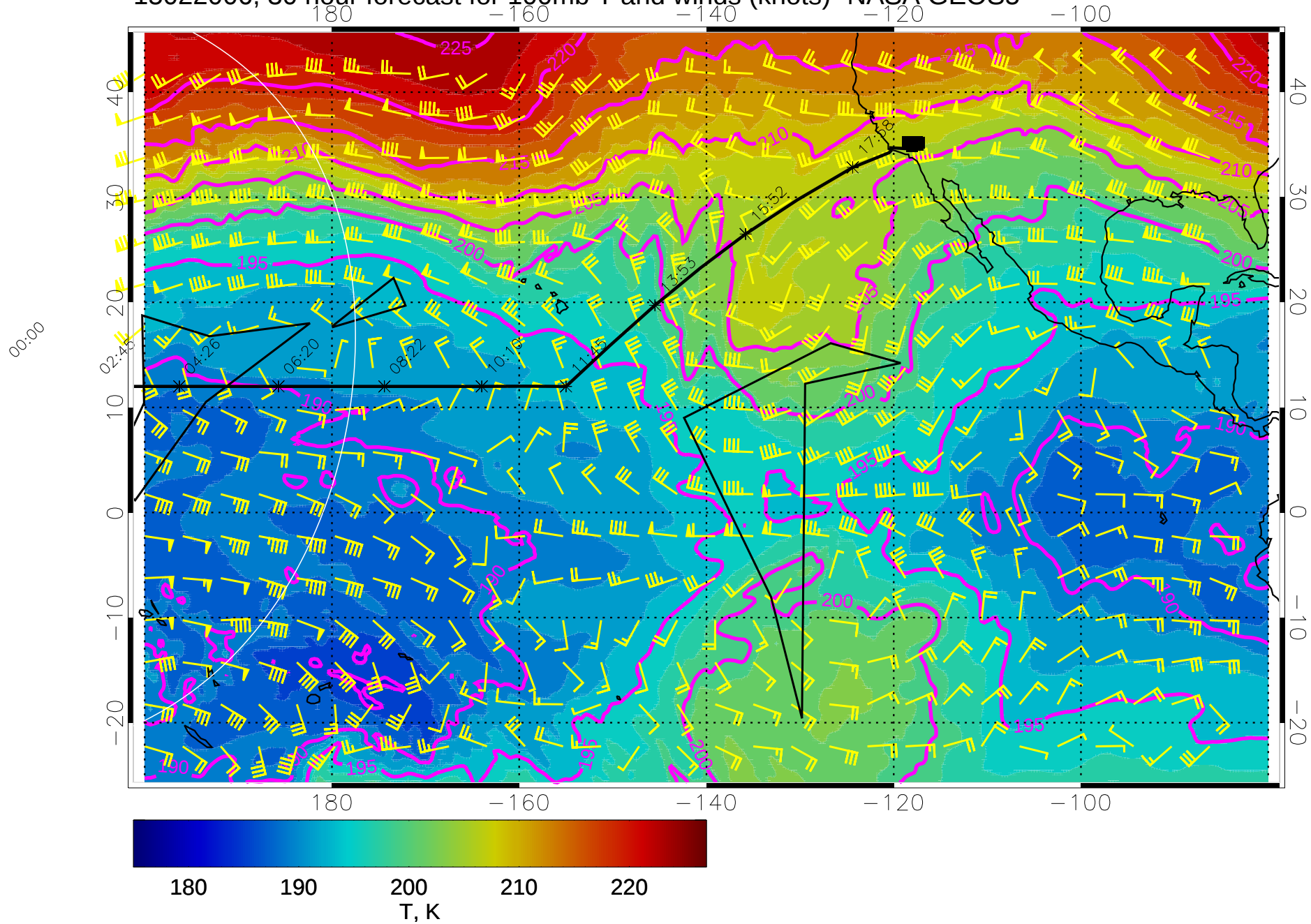
15022006, 30 hour forecast for 100mb T and winds (knots)- NASA GEOS5
