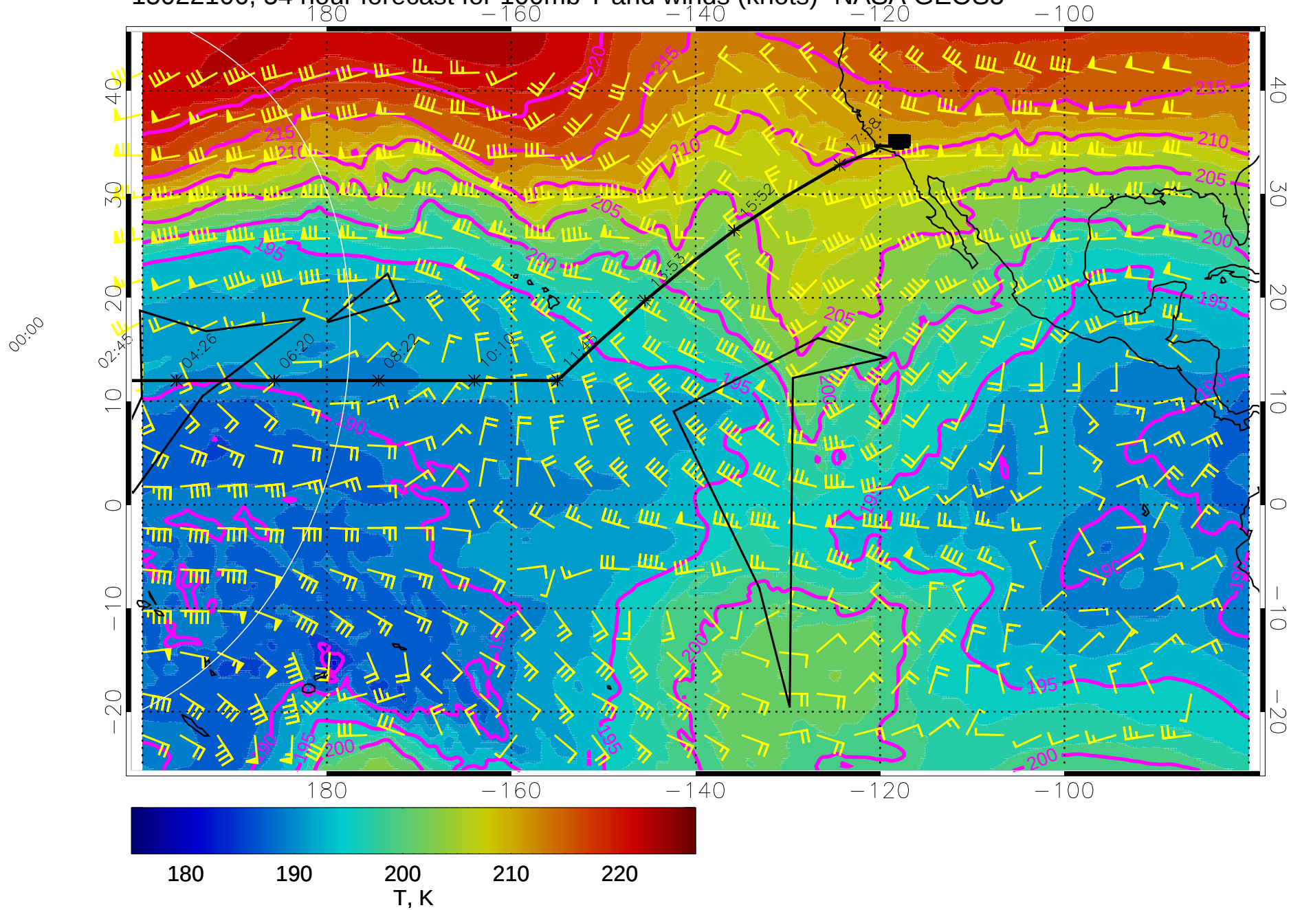
15022106, 54 hour forecast for 100mb T and winds (knots)- NASA GEOS5
