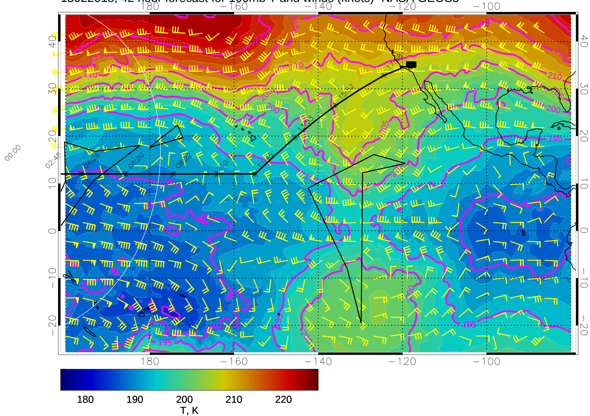
15022018, 42 hour forecast for 100mb T and winds (knots)- NASA GEOS5
