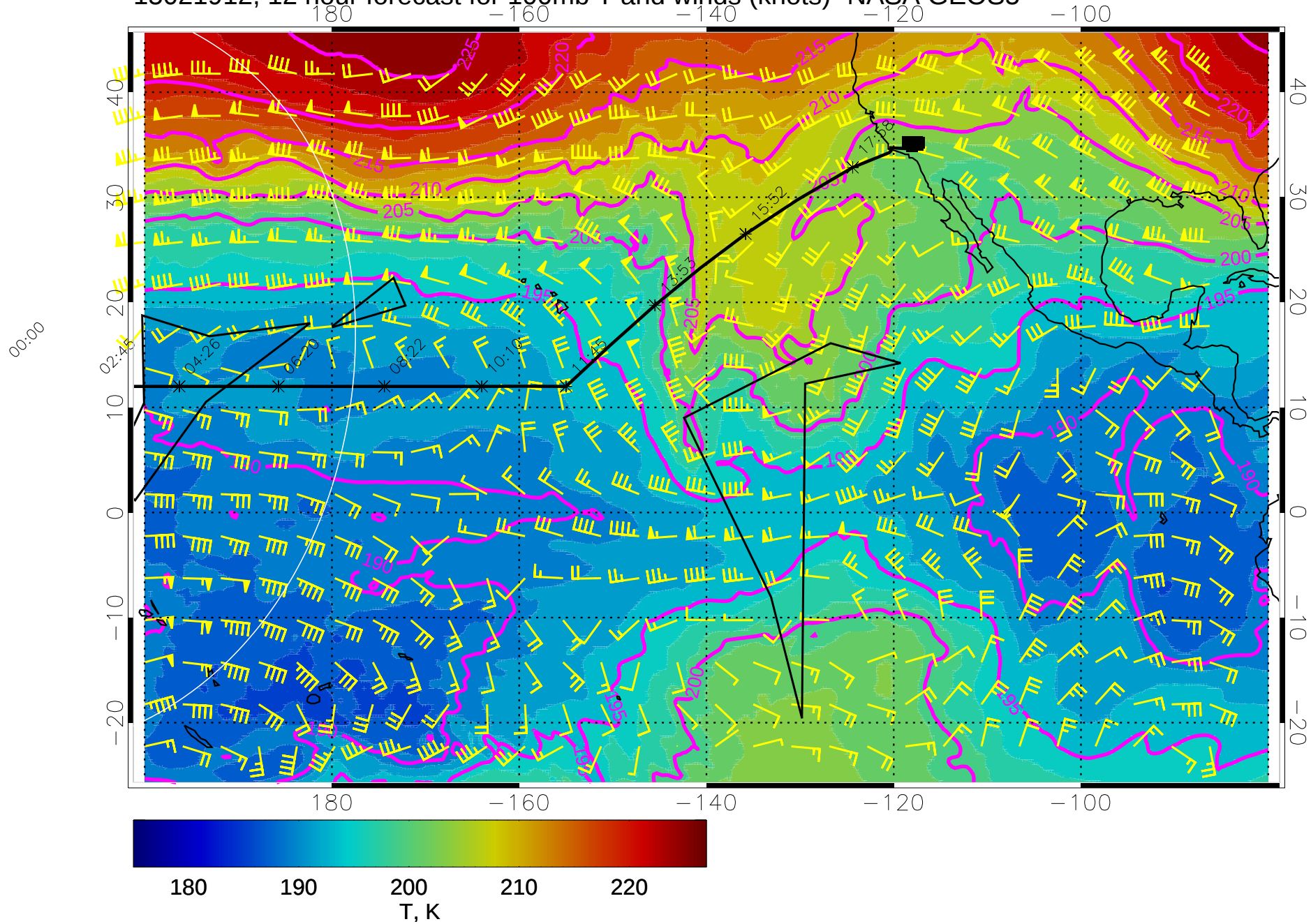
15021912, 12 hour forecast for 100mb T and winds (knots)- NASA GEOS5
