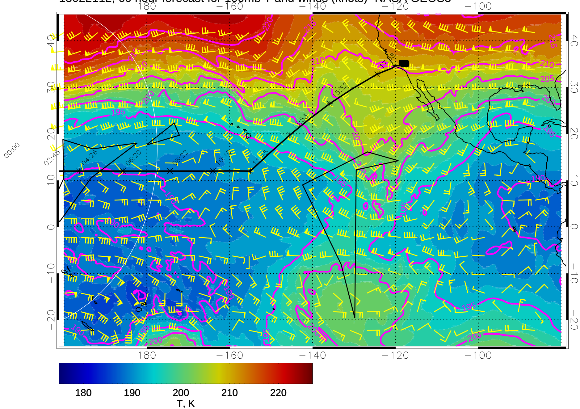
15022112, 60 hour forecast for 100mb T and winds (knots)- NASA GEOS5
