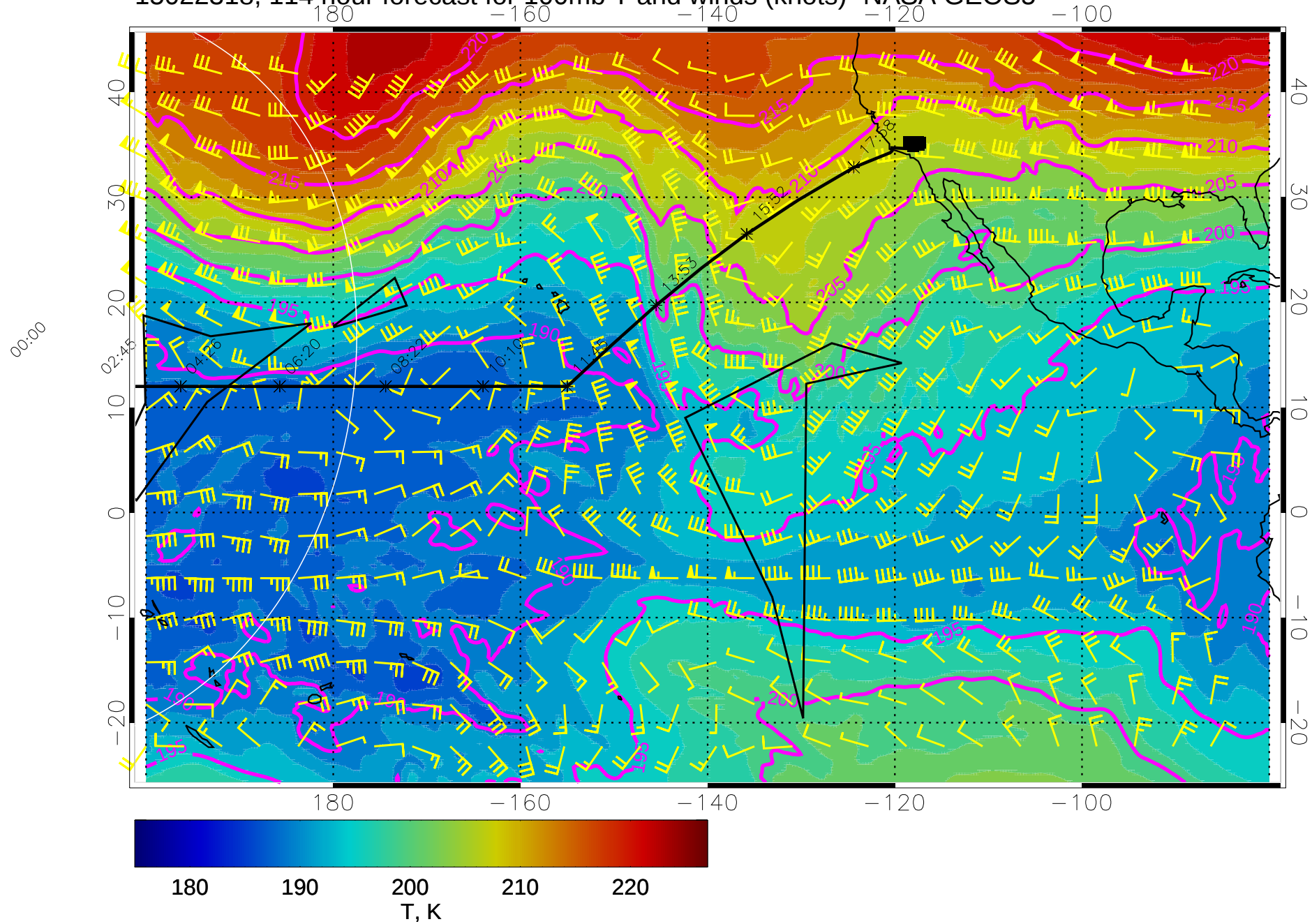
15022318, 114 hour forecast for 100mb T and winds (knots)- NASA GEOS5
