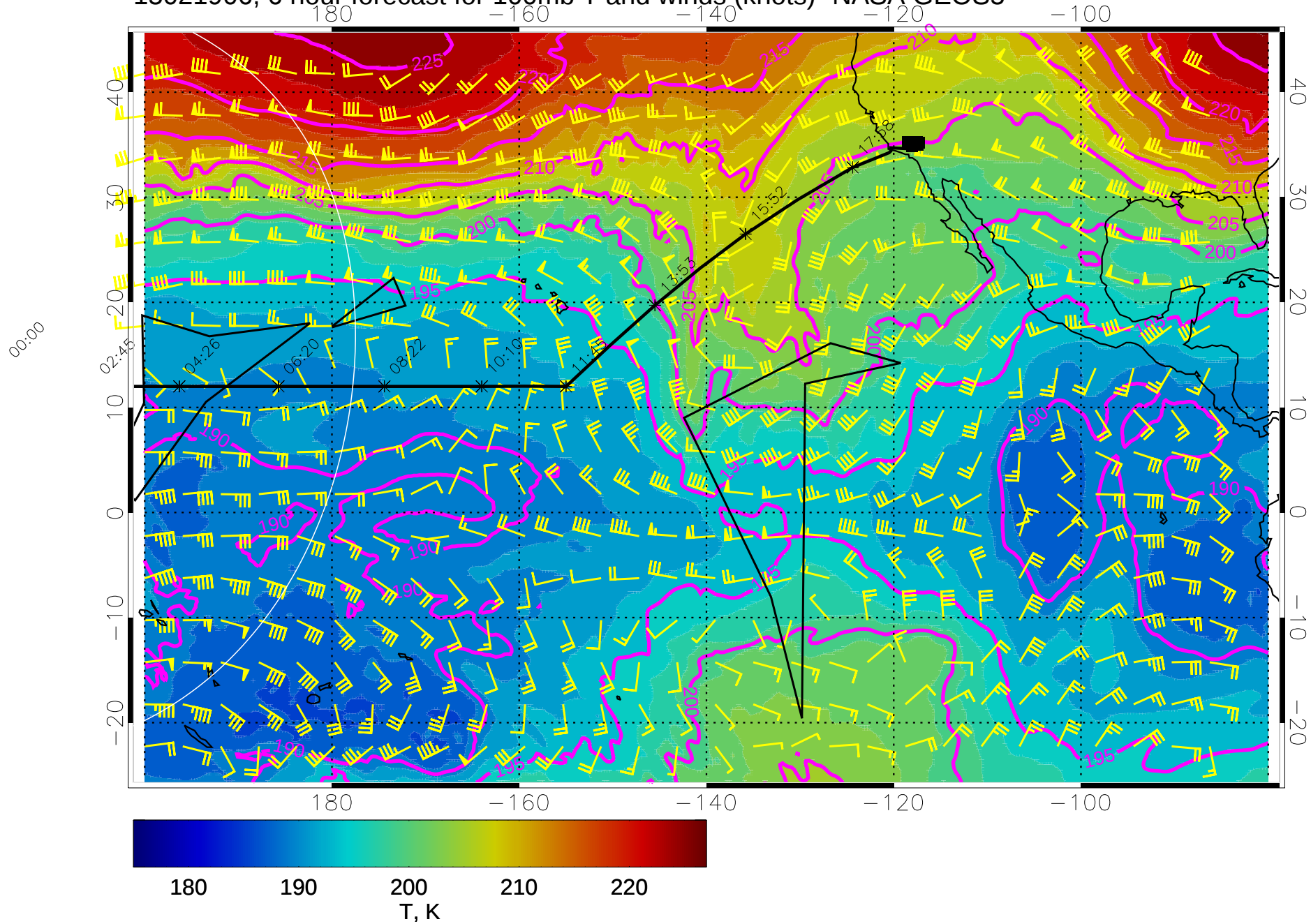
15021906, 6 hour forecast for 100mb T and winds (knots)- NASA GEOS5
