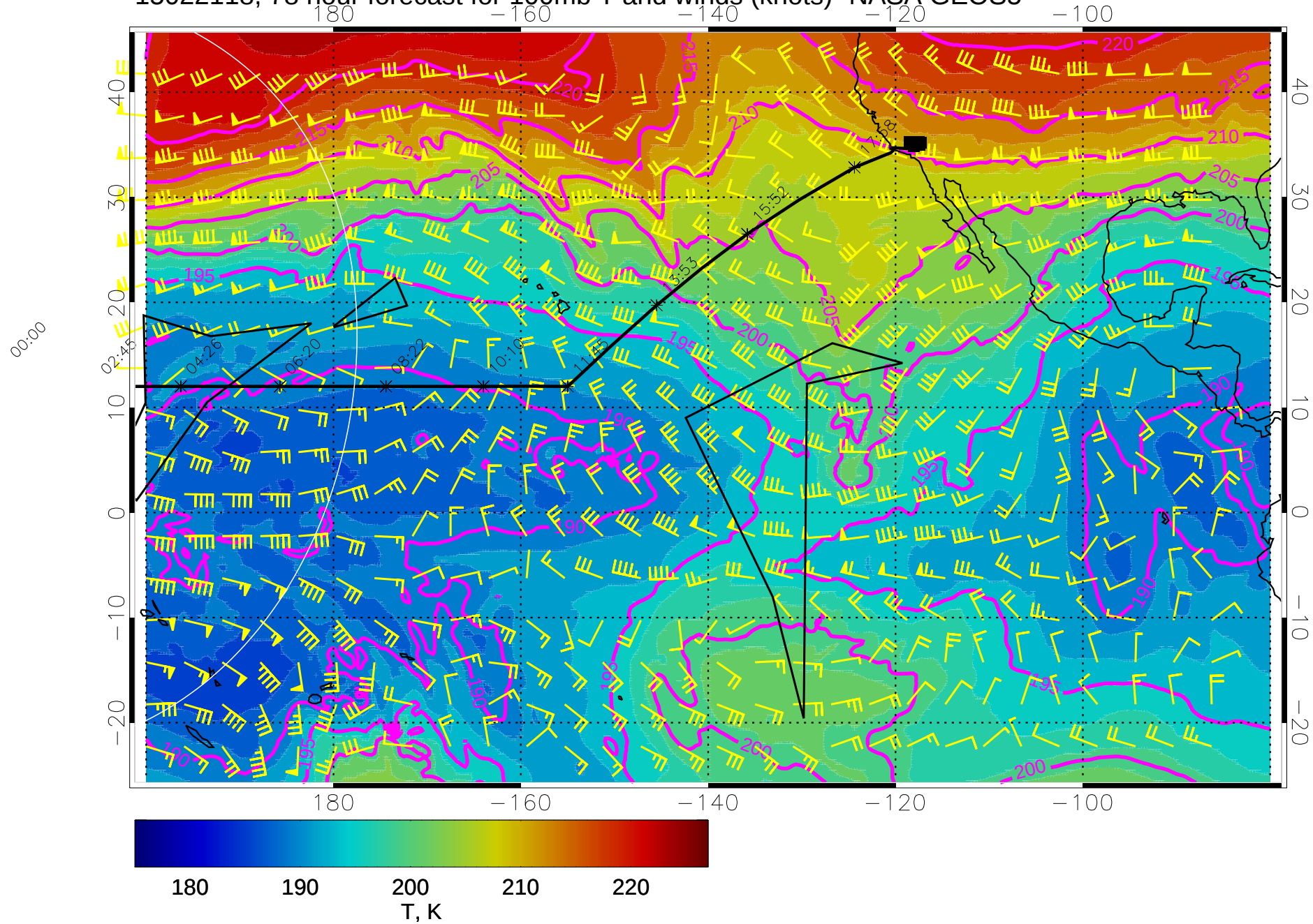
15022118, 78 hour forecast for 100mb T and winds (knots)- NASA GEOS5
