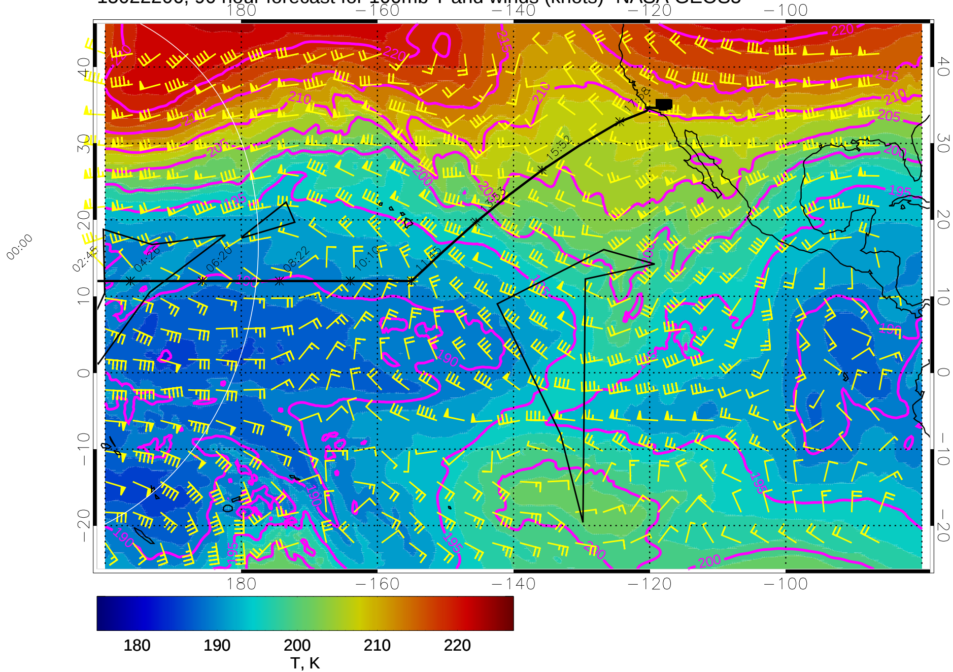
15022206, 90 hour forecast for 100mb T and winds (knots)- NASA GEOS5
