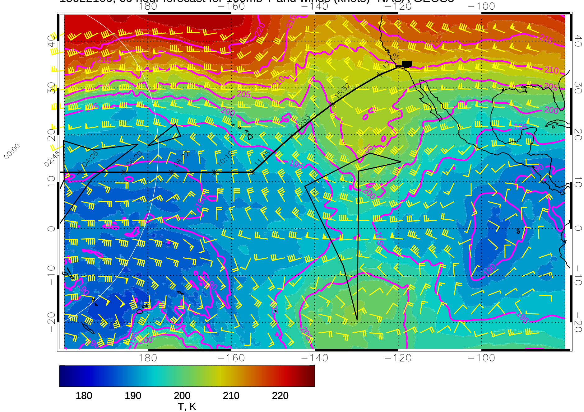
15022100, 60 hour forecast for 100mb T and winds (knots)- NASA GEOS5
