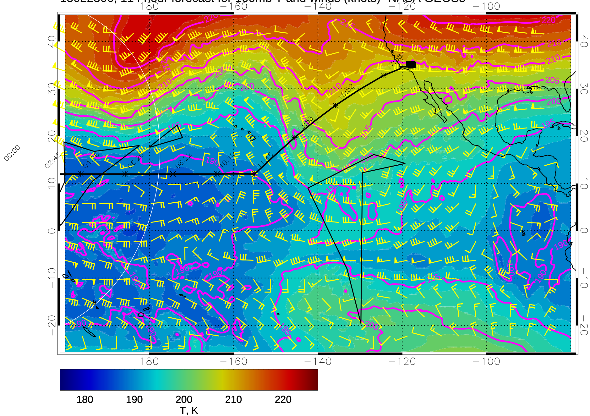
15022306, 114 hour forecast for 100mb T and winds (knots)- NASA GEOS5
