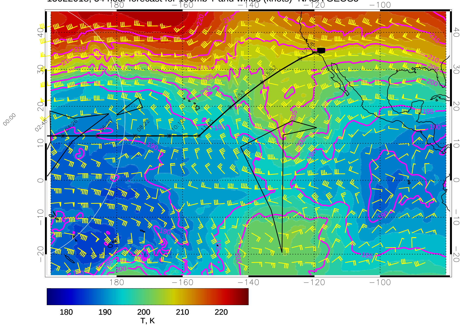
15022018, 54 hour forecast for 100mb T and winds (knots)- NASA GEOS5
