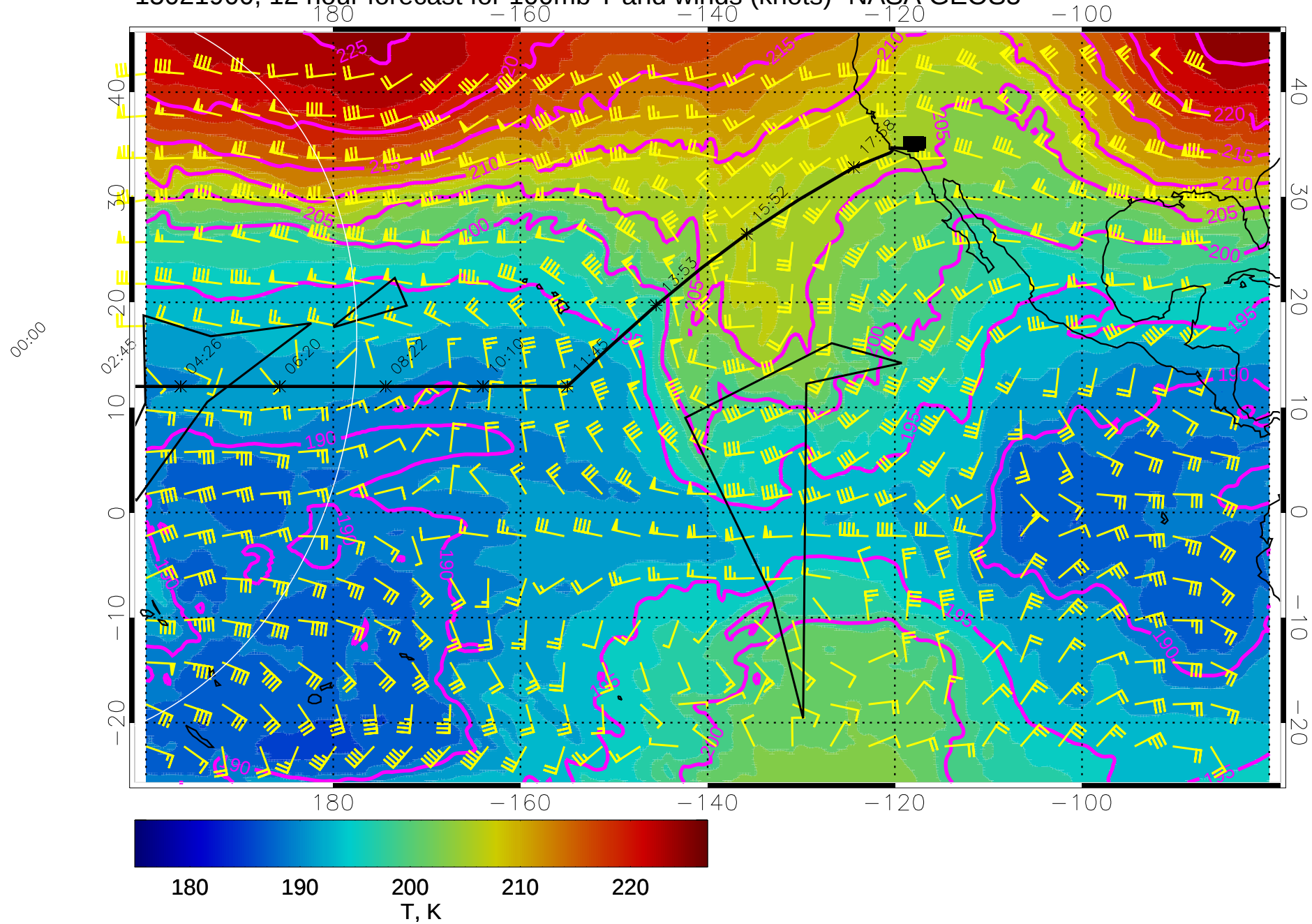
15021900, 12 hour forecast for 100mb T and winds (knots)- NASA GEOS5
