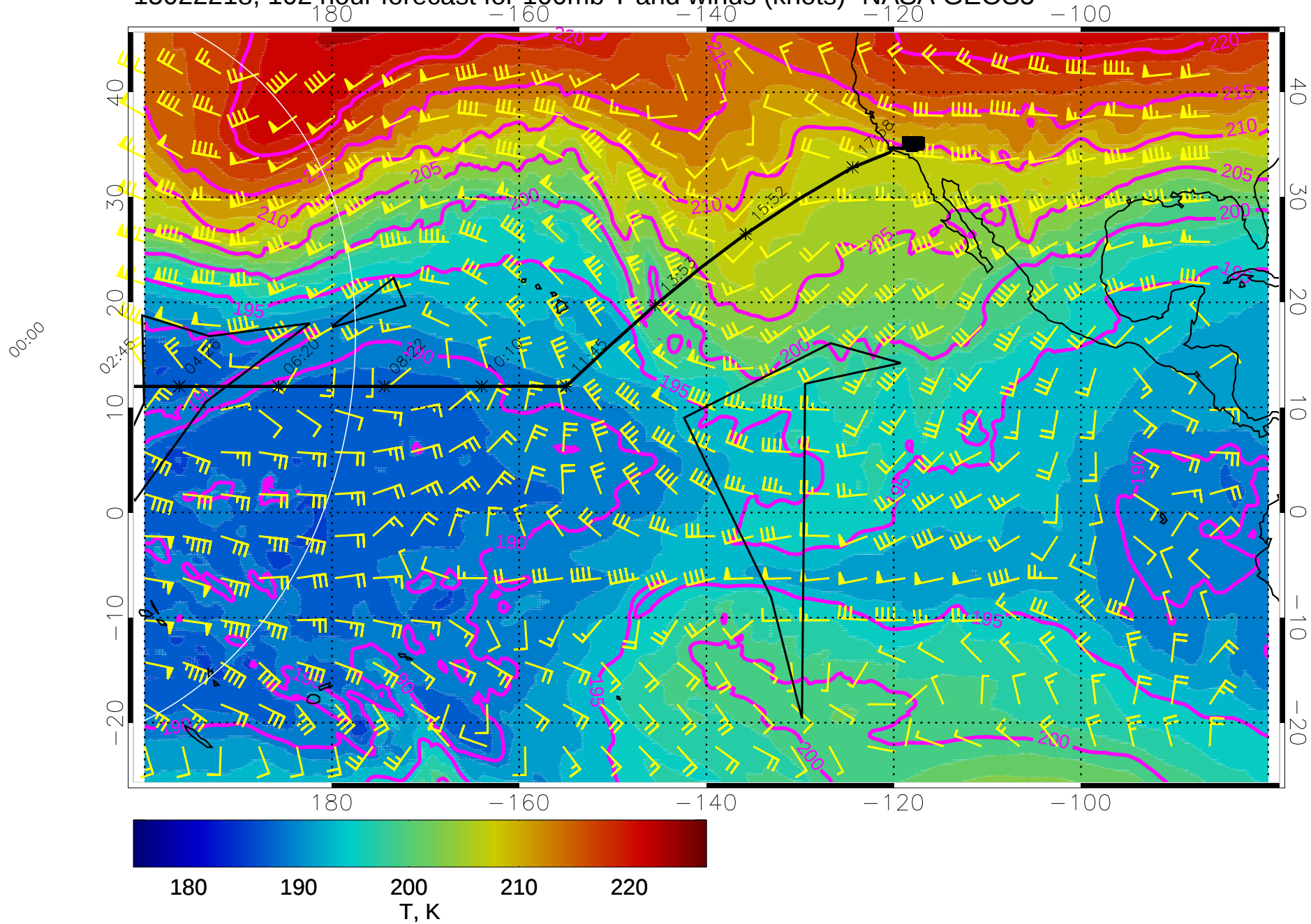
15022218, 102 hour forecast for 100mb T and winds (knots)- NASA GEOS5
