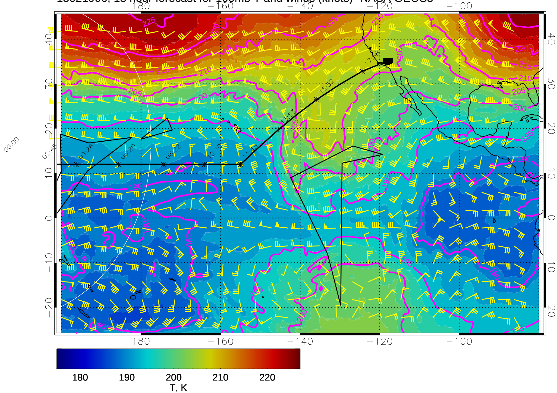
15021906, 18 hour forecast for 100mb T and winds (knots)- NASA GEOS5
