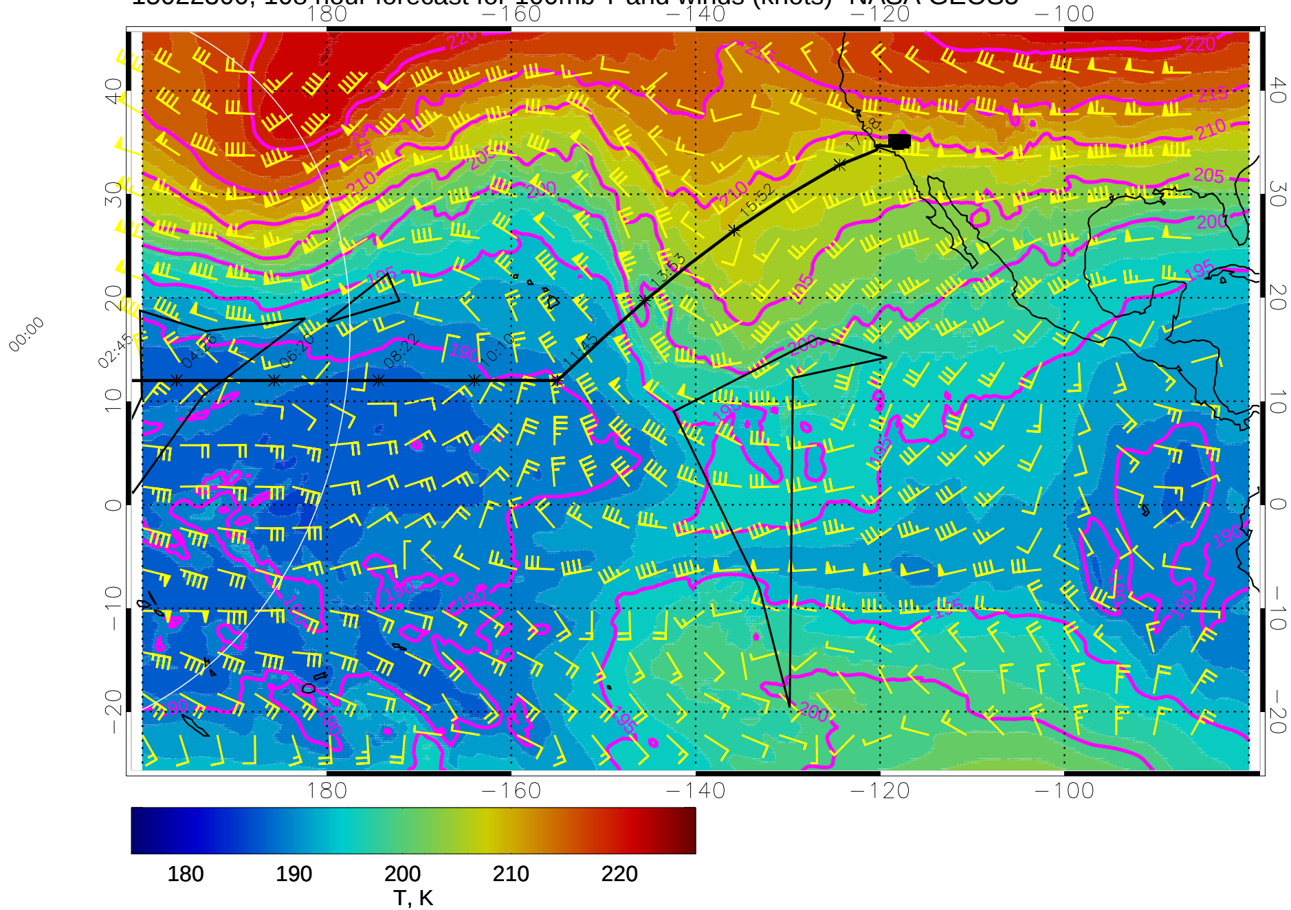
15022300, 108 hour forecast for 100mb T and winds (knots)- NASA GEOS5
