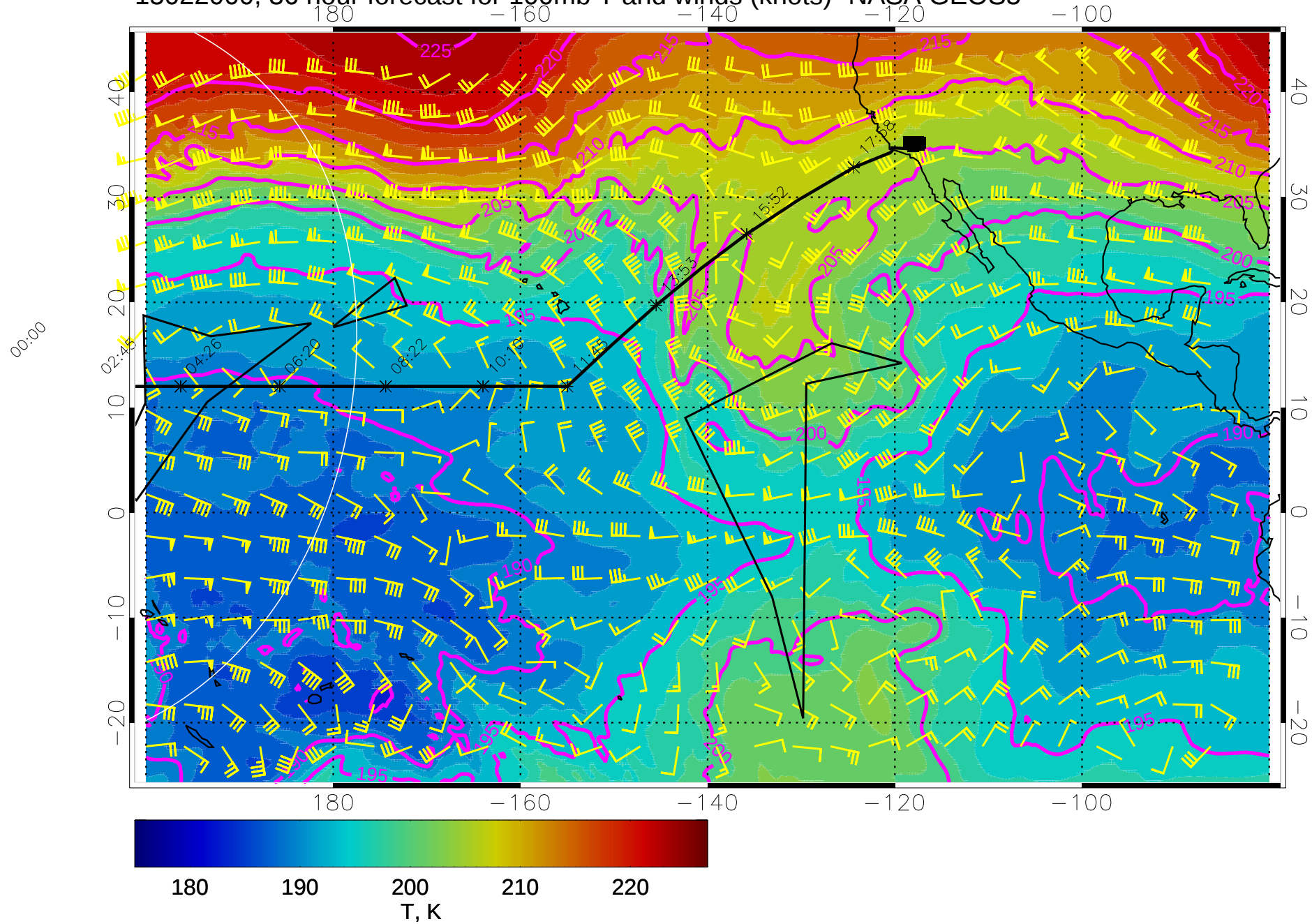
15022000, 36 hour forecast for 100mb T and winds (knots)- NASA GEOS5
