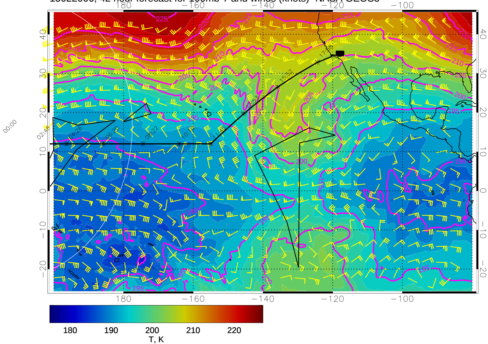
15022006, 42 hour forecast for 100mb T and winds (knots)- NASA GEOS5
