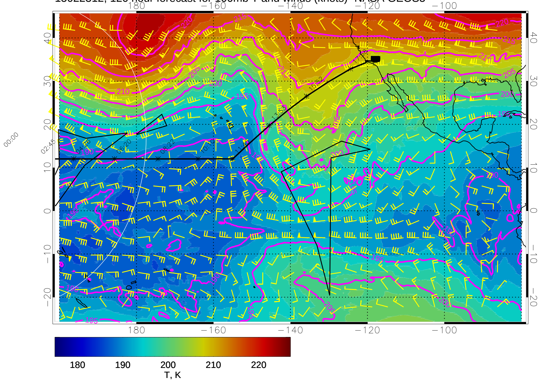
15022312, 120 hour forecast for 100mb T and winds (knots)- NASA GEOS5
