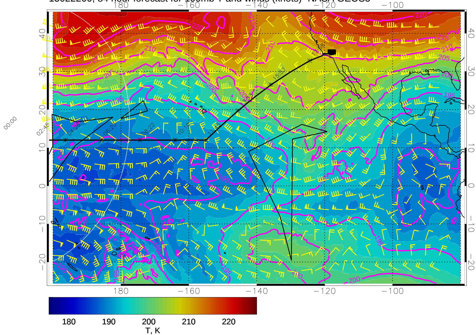
15022200, 84 hour forecast for 100mb T and winds (knots)- NASA GEOS5
