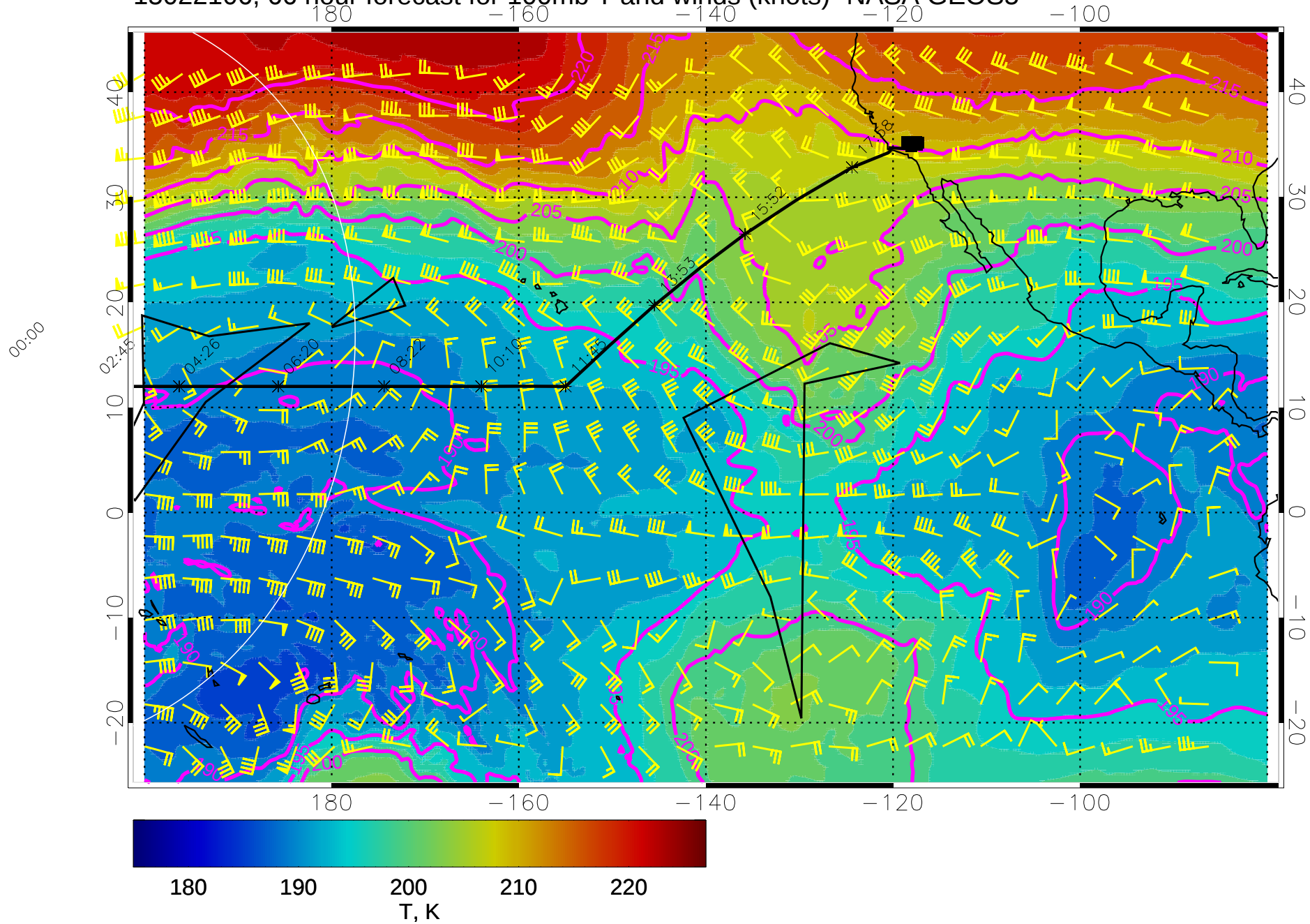
15022106, 66 hour forecast for 100mb T and winds (knots)- NASA GEOS5
