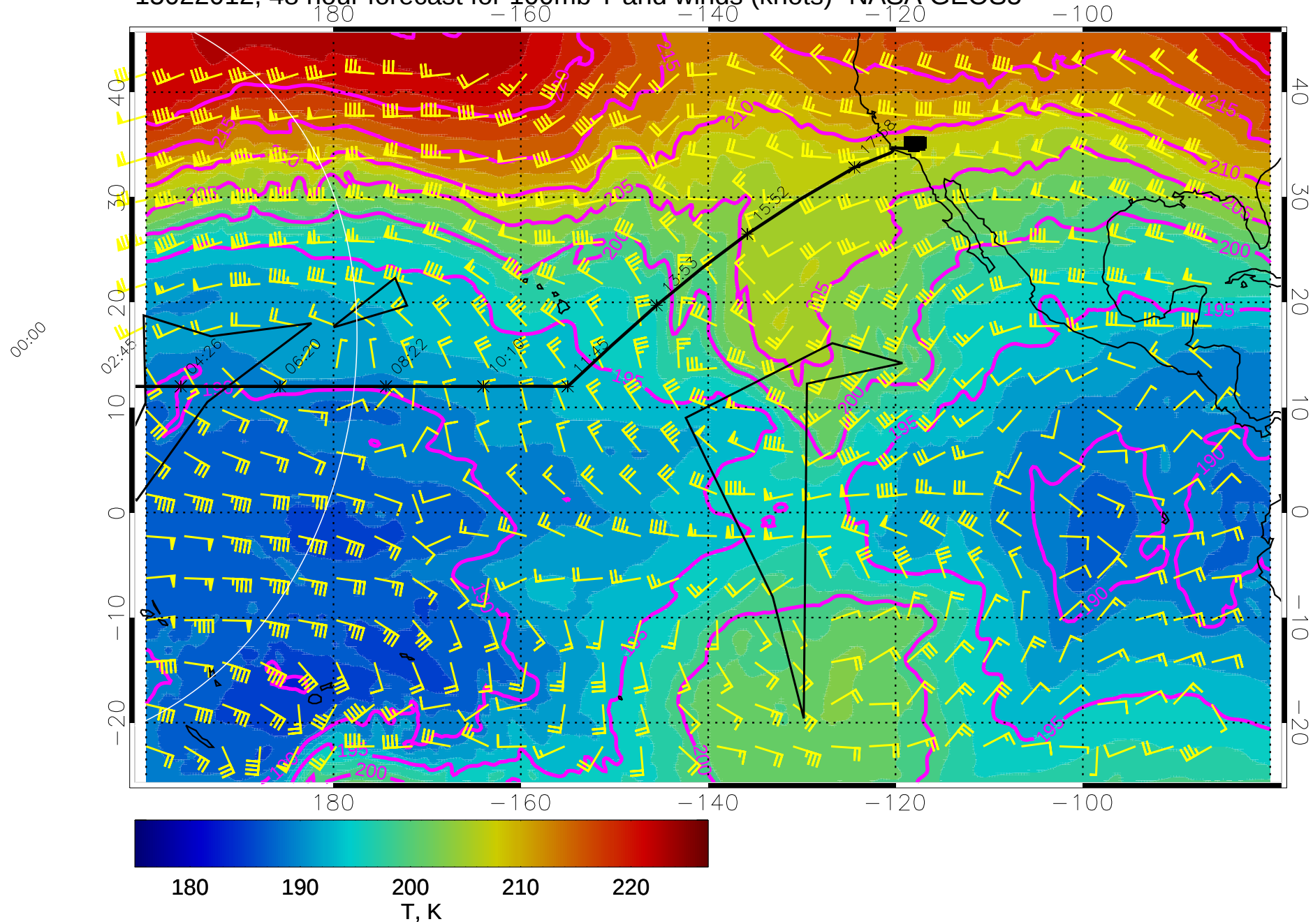
15022012, 48 hour forecast for 100mb T and winds (knots)- NASA GEOS5
