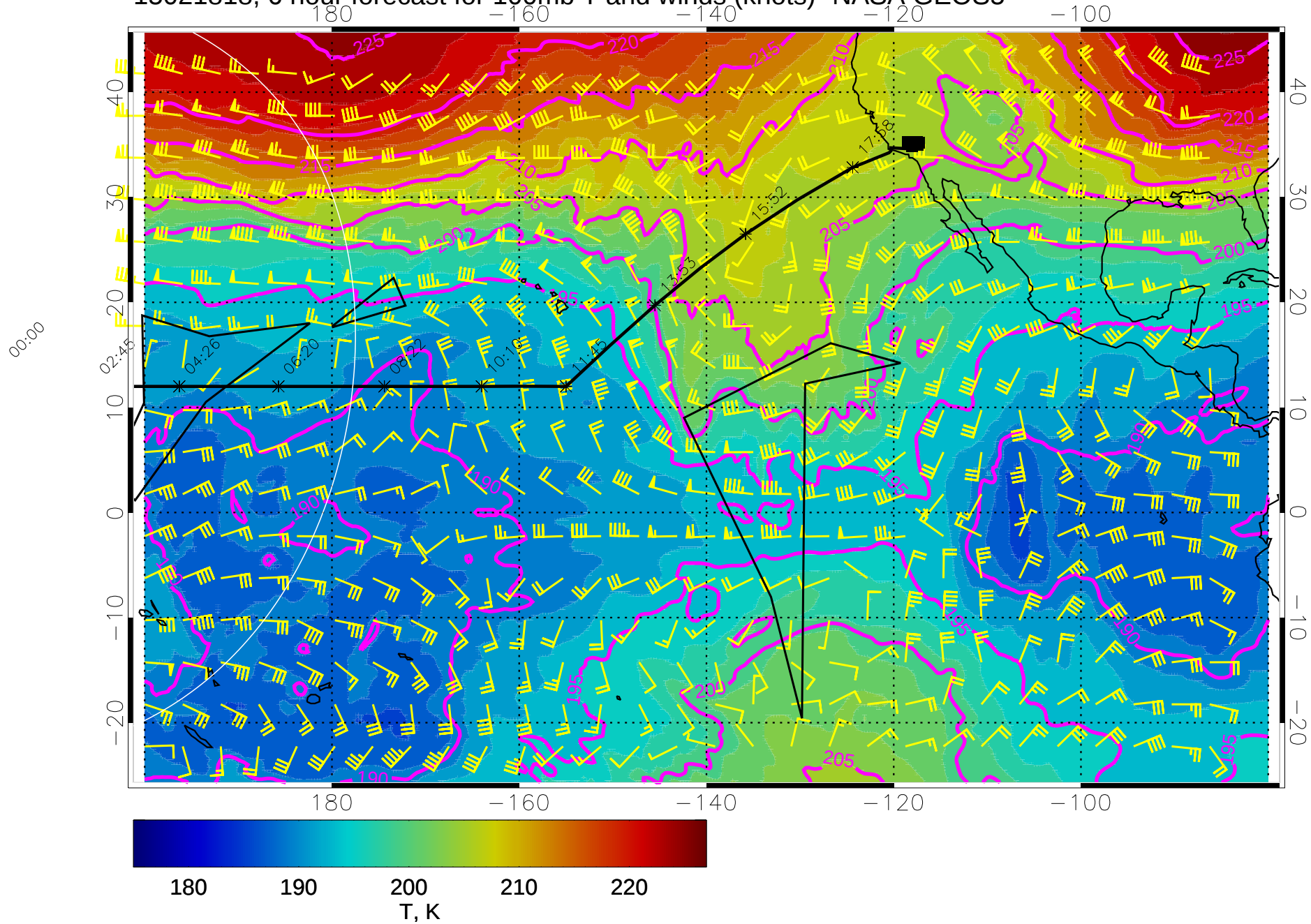
15021818, 6 hour forecast for 100mb T and winds (knots)- NASA GEOS5
