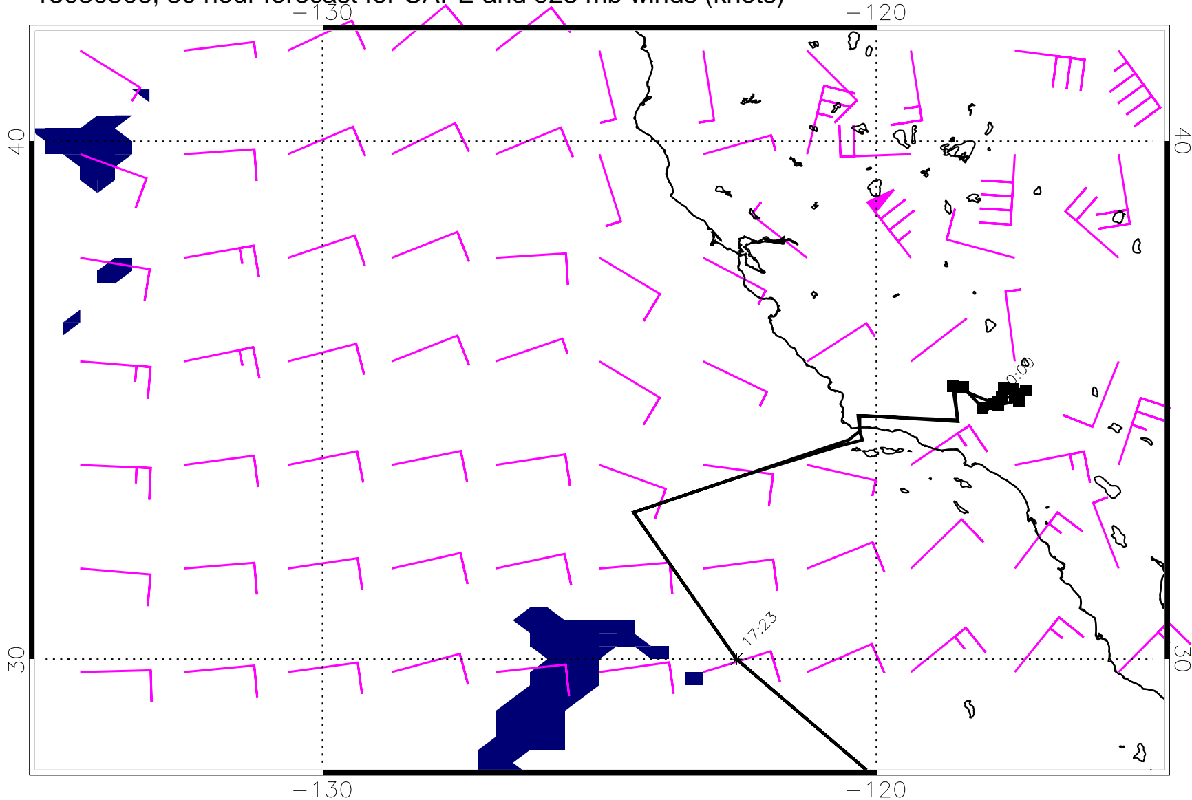
15030506, 30 hour forecast for CAPE and 925 mb winds (knots)
