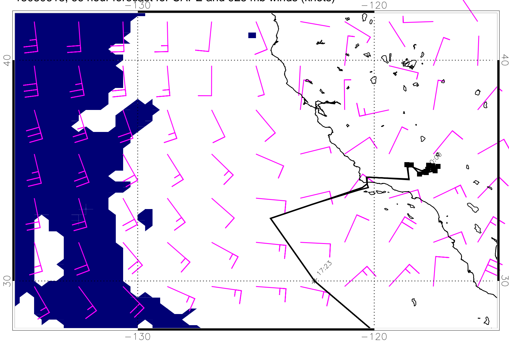
15030618, 66 hour forecast for CAPE and 925 mb winds (knots)
