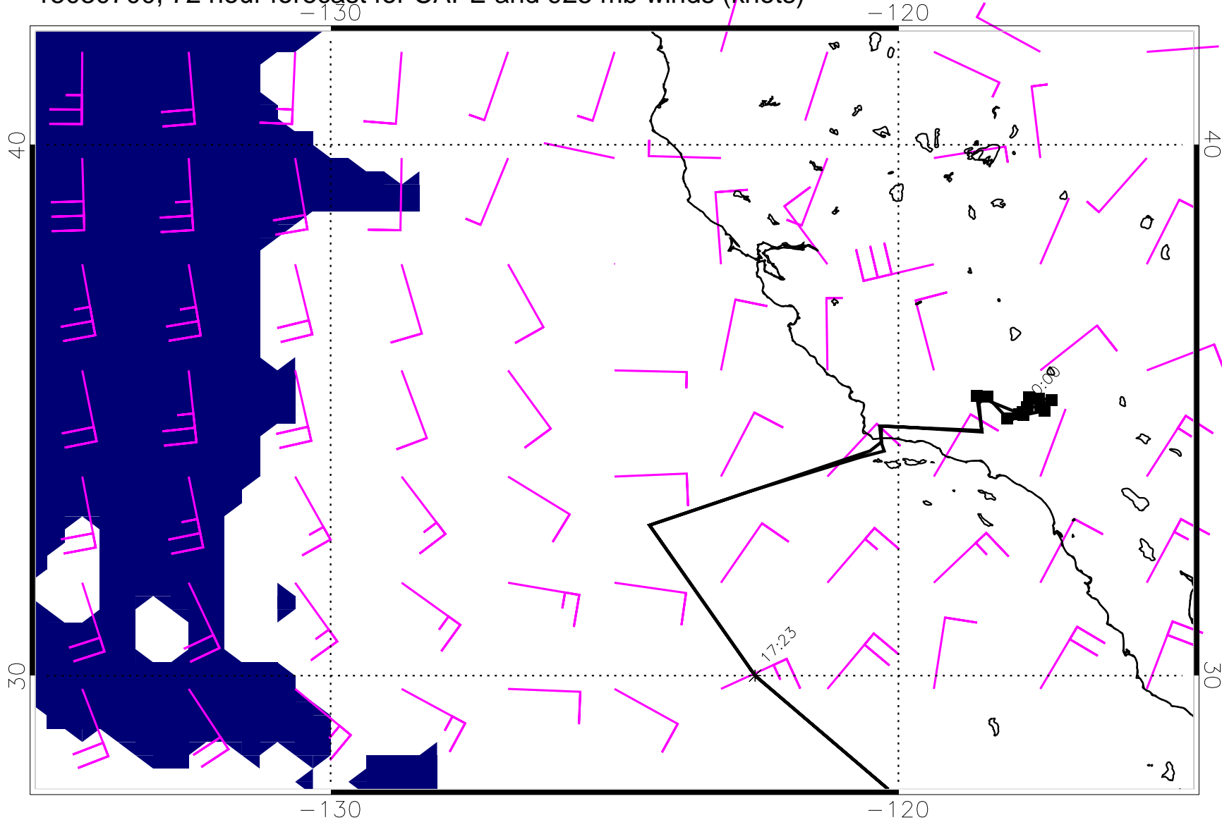
15030700, 72 hour forecast for CAPE and 925 mb winds (knots)
