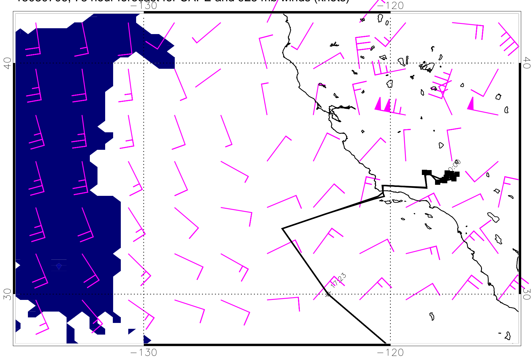
15030706, 78 hour forecast for CAPE and 925 mb winds (knots)
