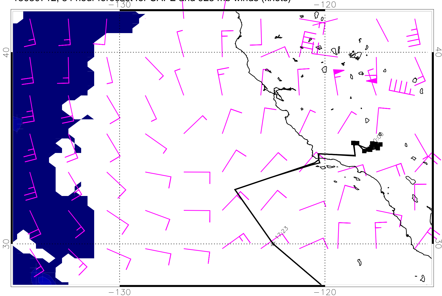
15030712, 84 hour forecast for CAPE and 925 mb winds (knots)
