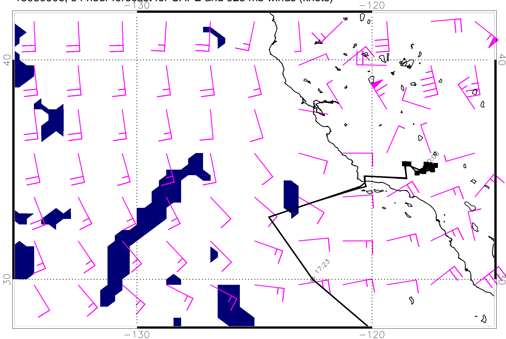
15030606, 54 hour forecast for CAPE and 925 mb winds (knots)
