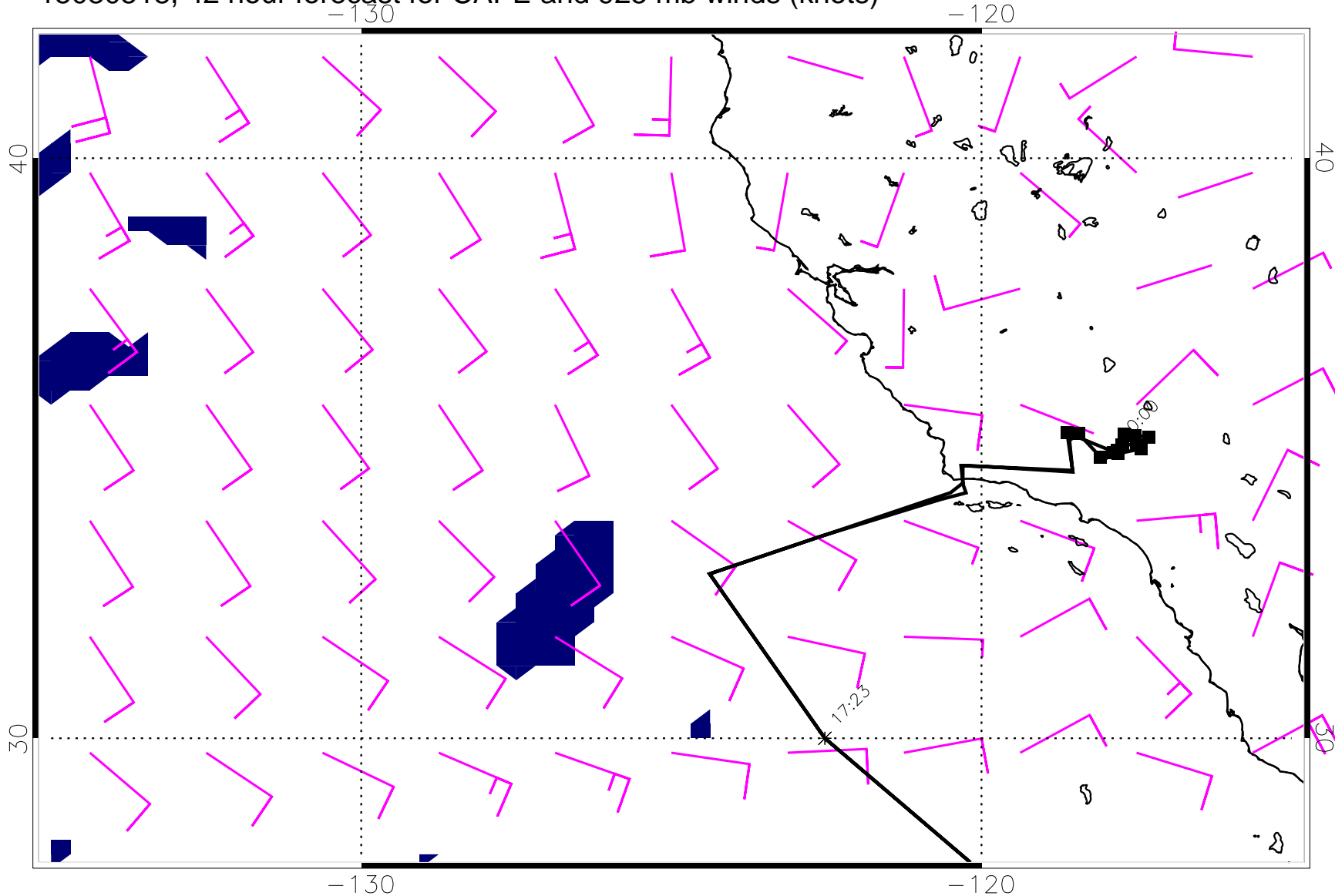
15030518, 42 hour forecast for CAPE and 925 mb winds (knots)
