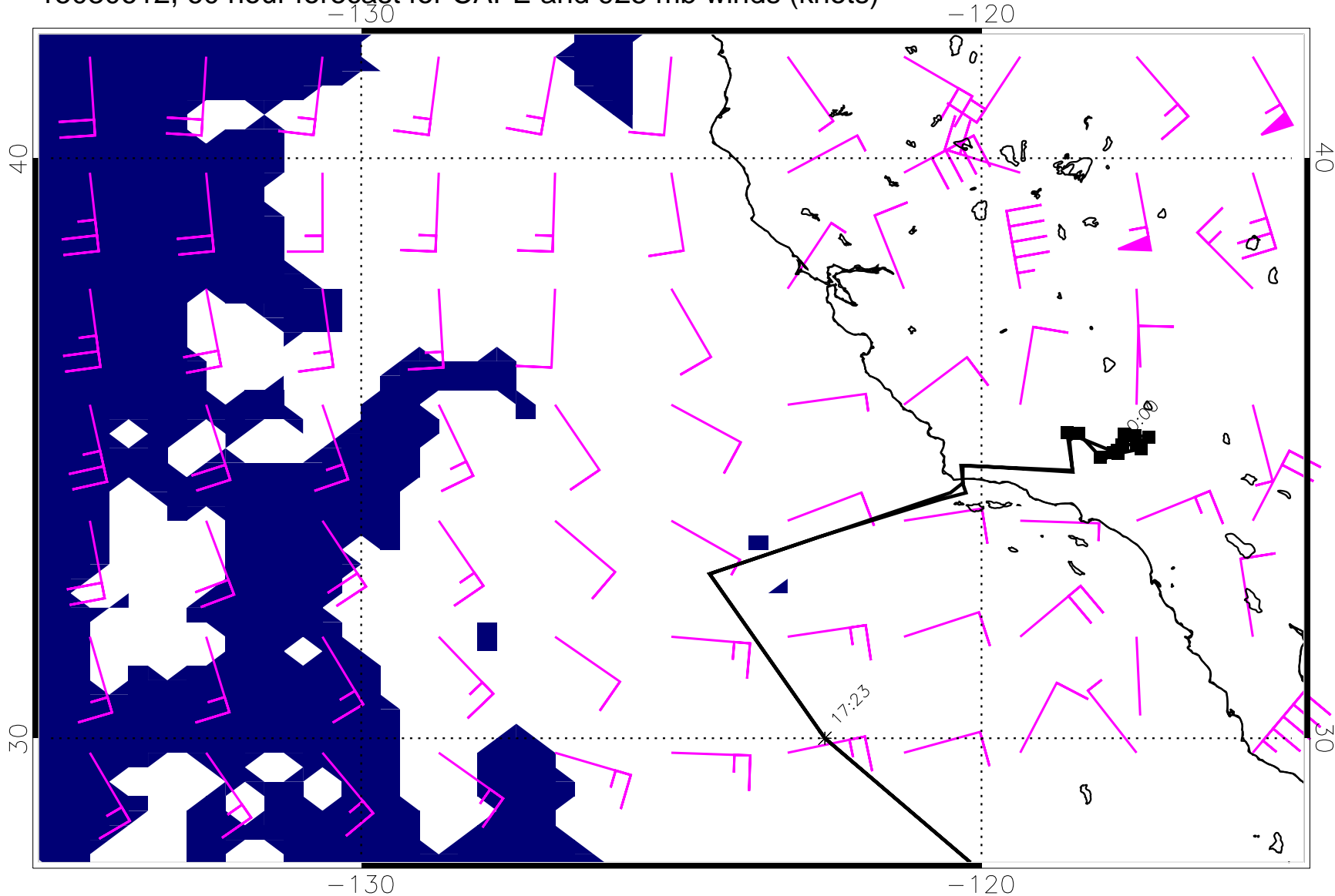
15030612, 60 hour forecast for CAPE and 925 mb winds (knots)
