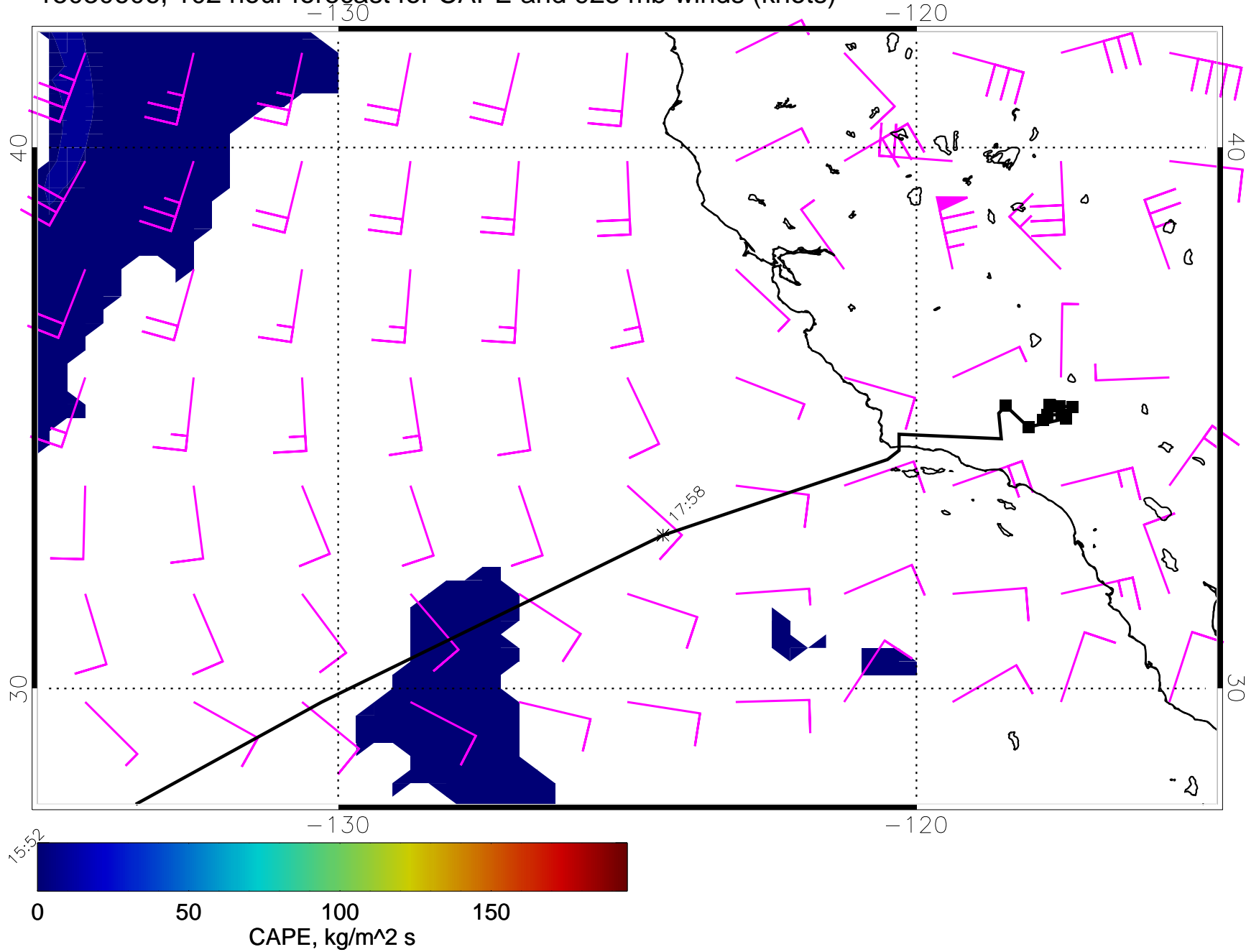
15030606, 102 hour forecast for CAPE and 925 mb winds (knots)
