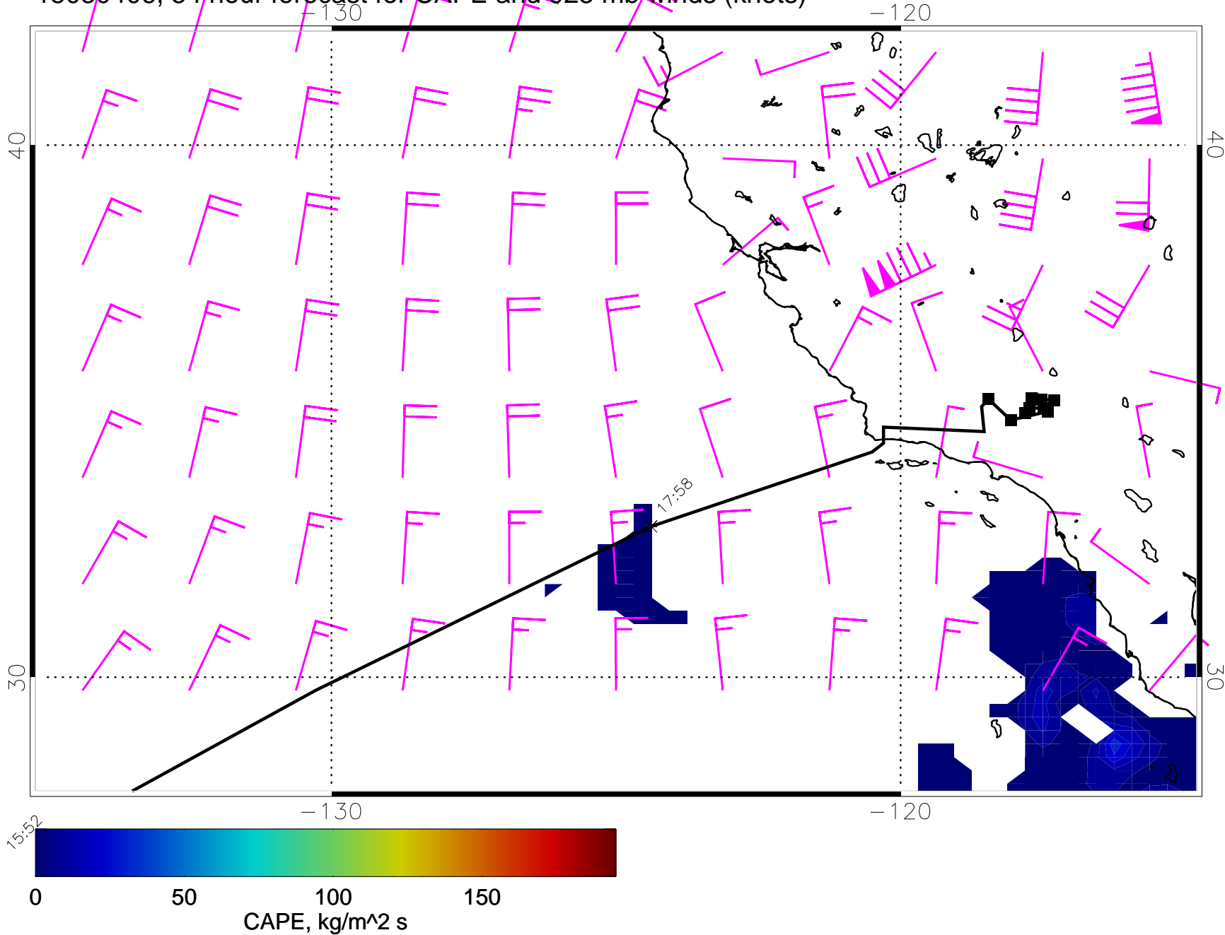
15030406, 54 hour forecast for CAPE and 925 mb winds (knots)
