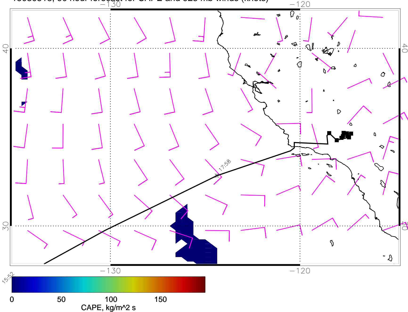
15030518, 90 hour forecast for CAPE and 925 mb winds (knots)
