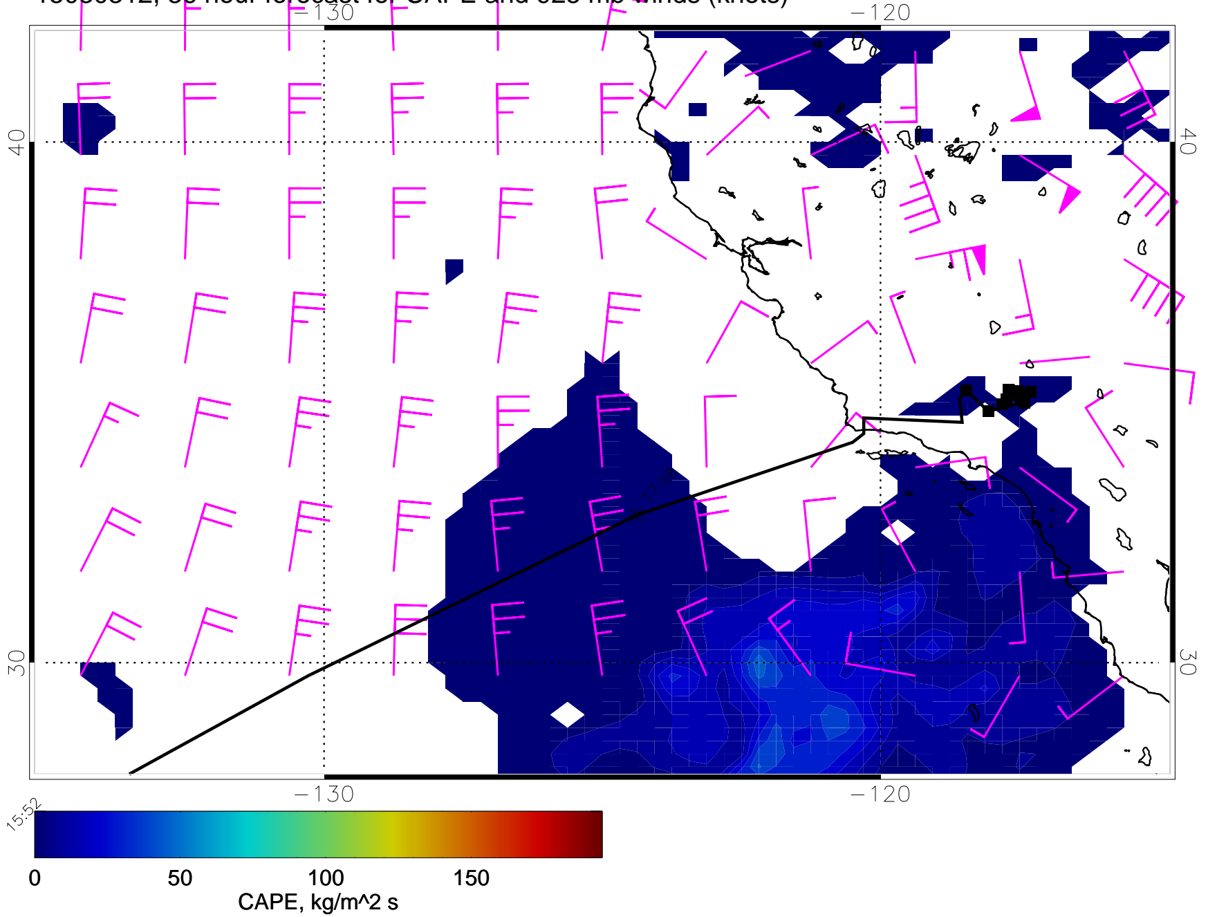
15030312, 36-hour forecast for CAPE and 925 mb winds (knots)
