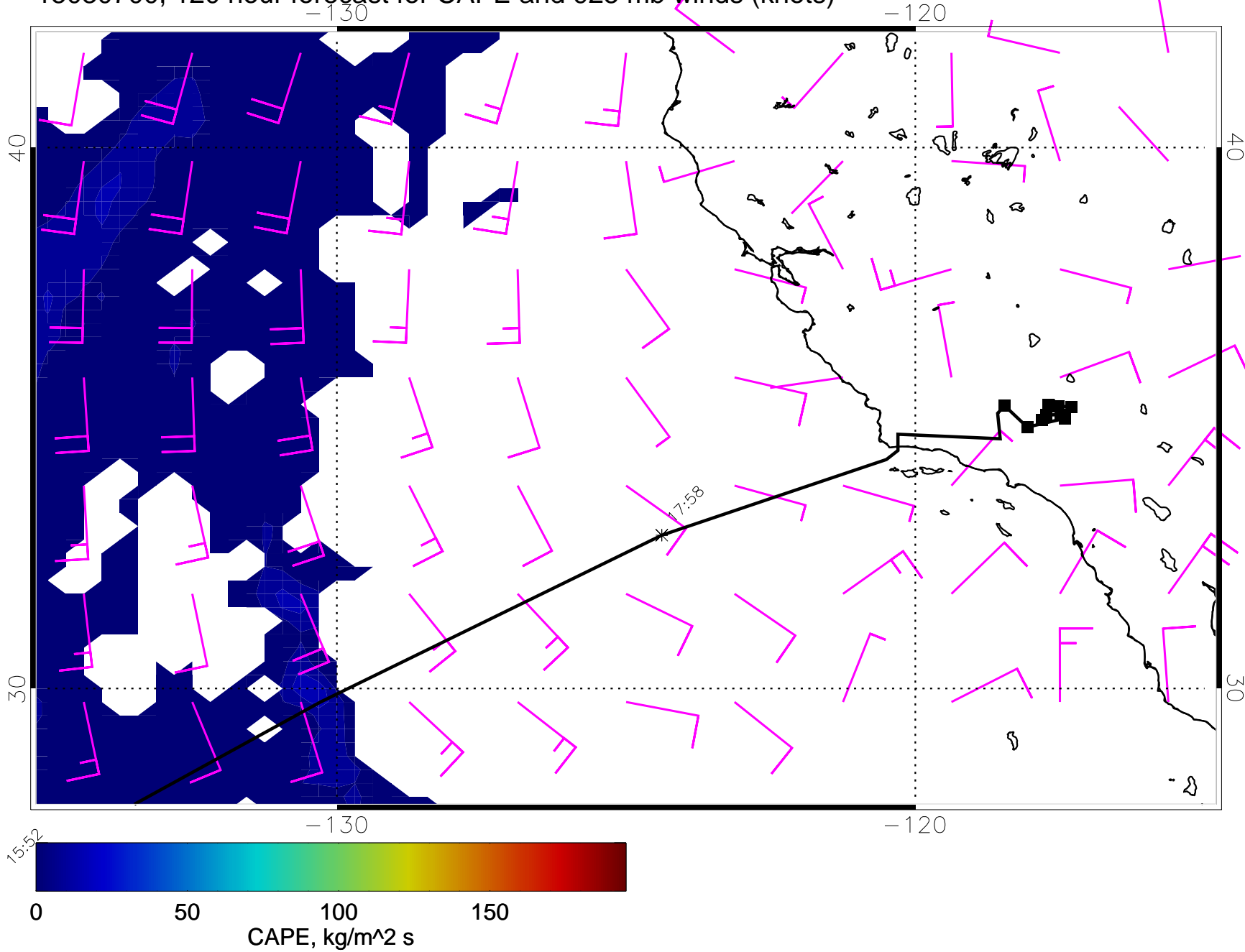
15030700, 120 hour forecast for CAPE and 925 mb winds (knots)
