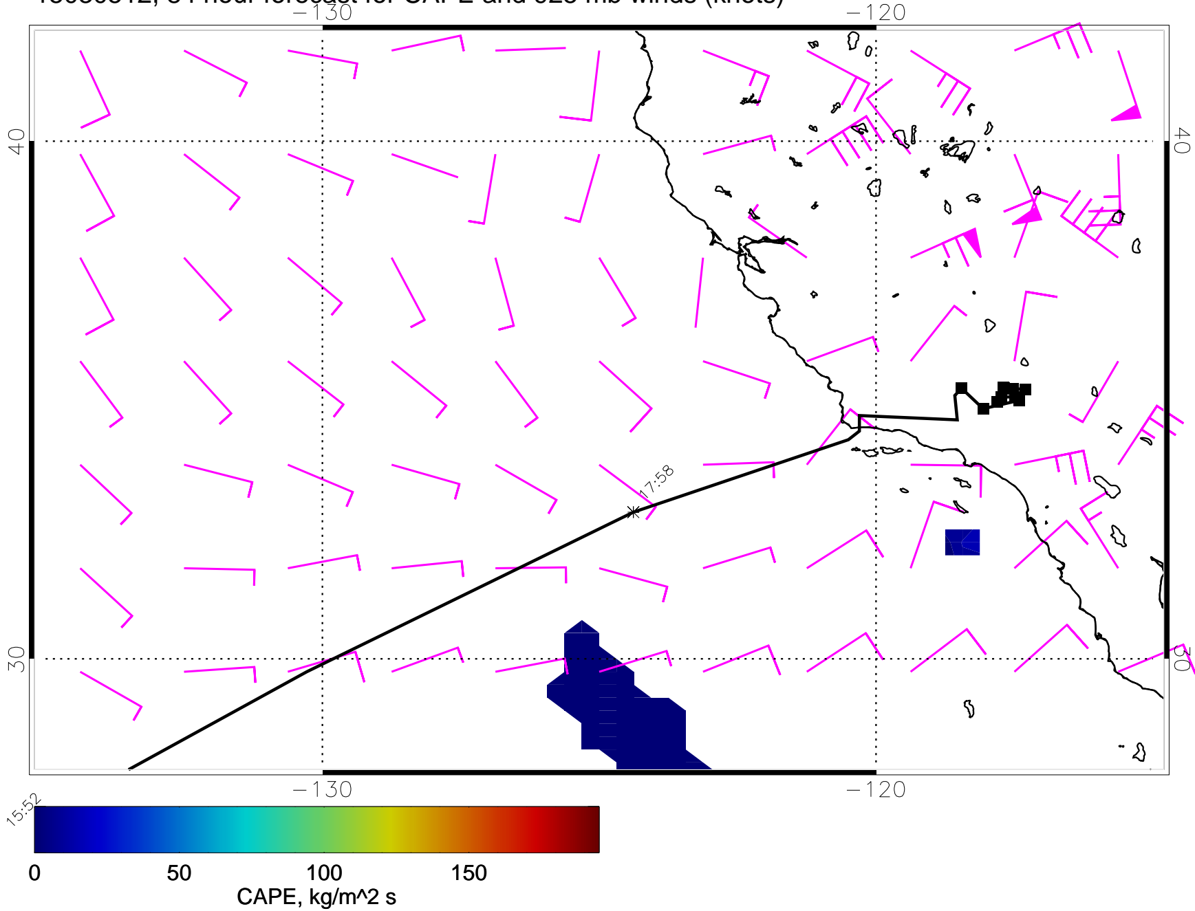
15030512, 84 hour forecast for CAPE and 925 mb winds (knots)
