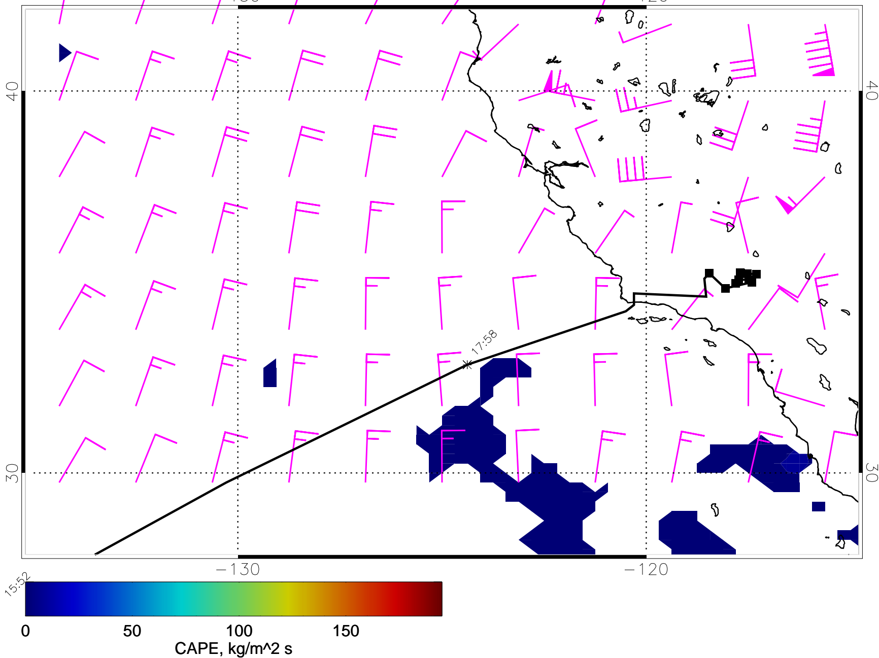
15030412, 60 hour forecast for CAPE and 925 mb winds (knots)
