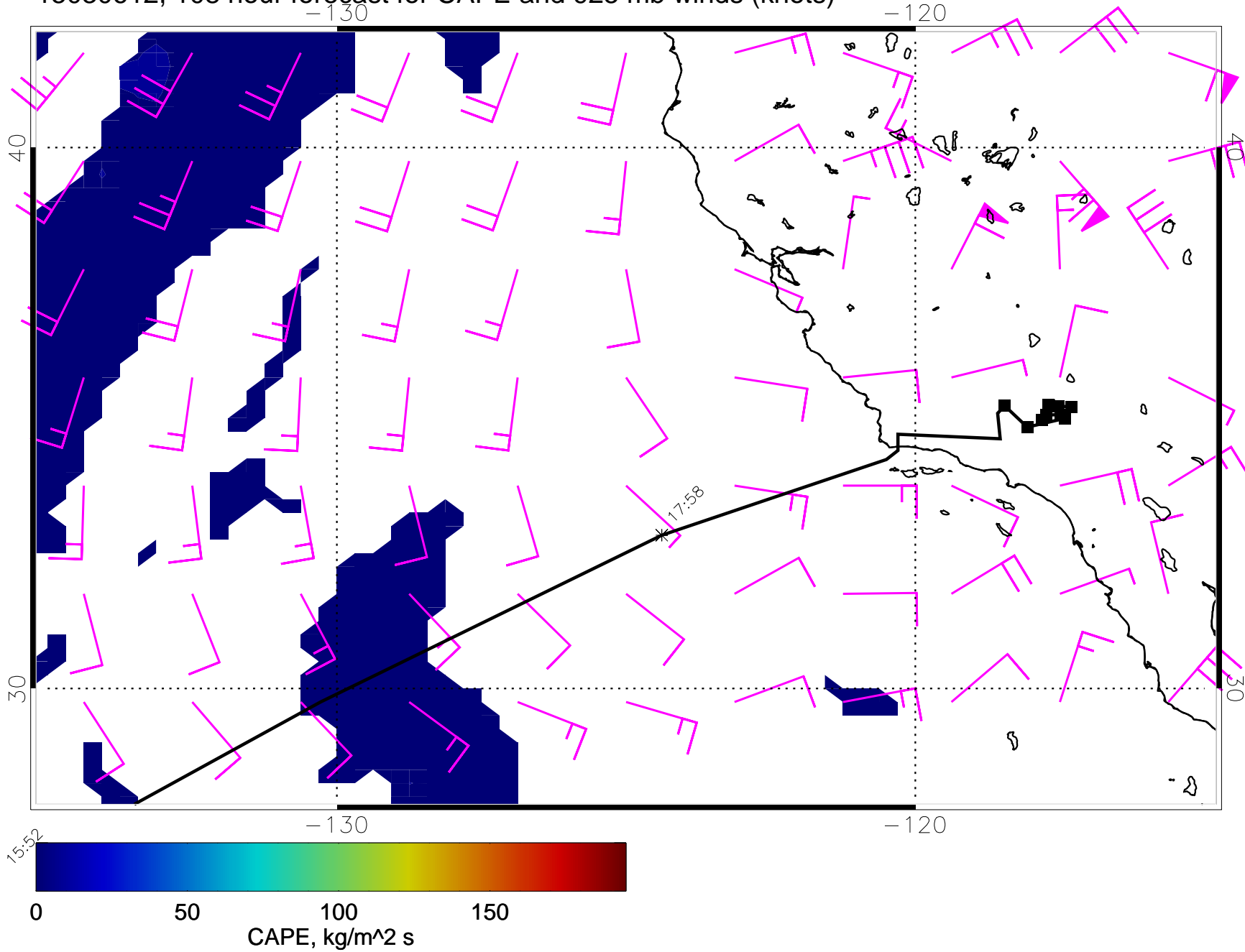
15030612, 108 hour forecast for CAPE and 925 mb winds (knots)
