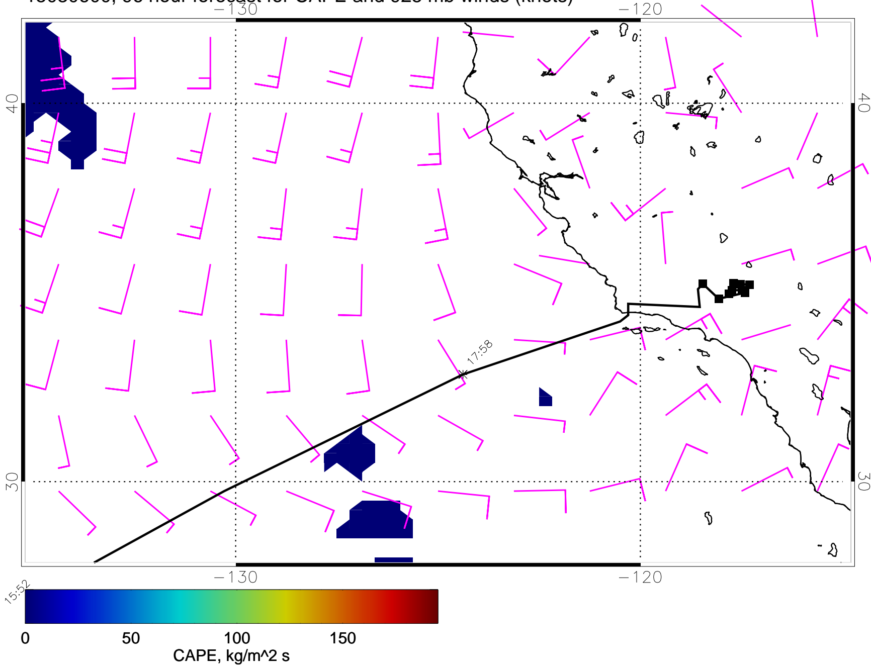
15030600, 96 hour forecast for CAPE and 925 mb winds (knots)
