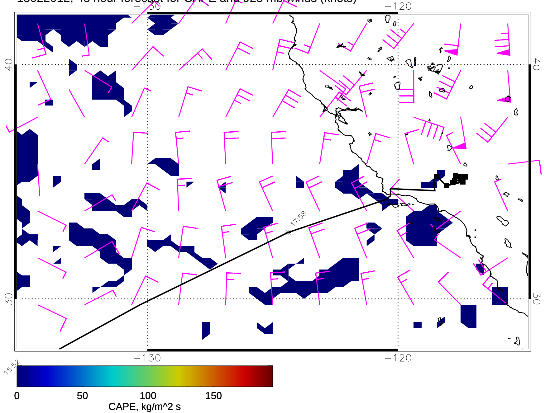
15022012, 48 hour forecast for CAPE and 925 mb winds (knots)
