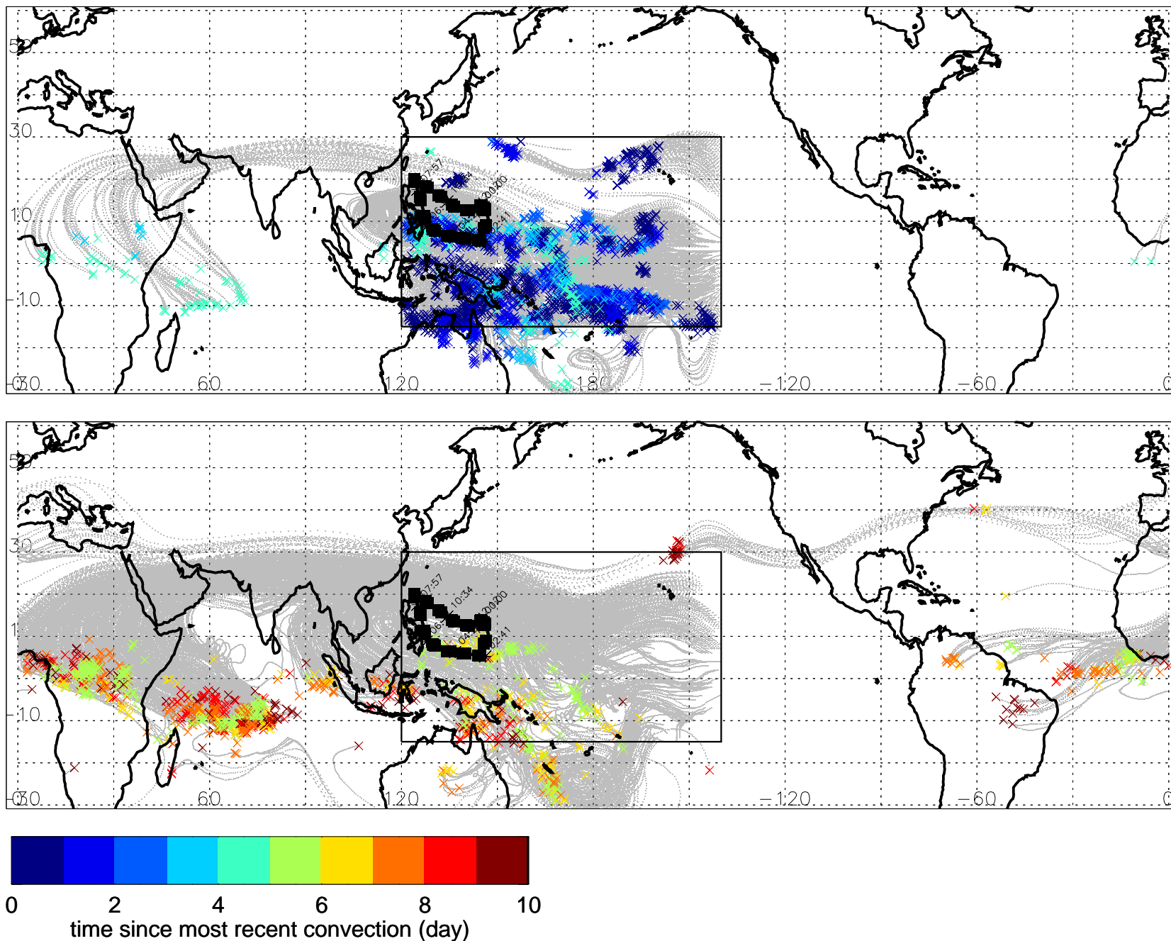
Fig. 4: Locations of most recent convection (top: 0 to 5.0 days; bottom: 5.0 to 10 days).
