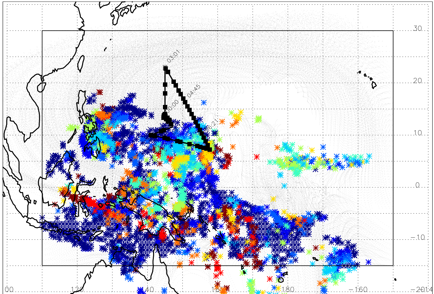
Convectively-influenced 10-day back trajectory at 43 kft level from boxed region on 01/21/2014, 00Z Fig. 3: Trajectories influenced by most recent convection (asterisks) between 0 and 5.0 days (As Fig. 2 but convection locations only)
