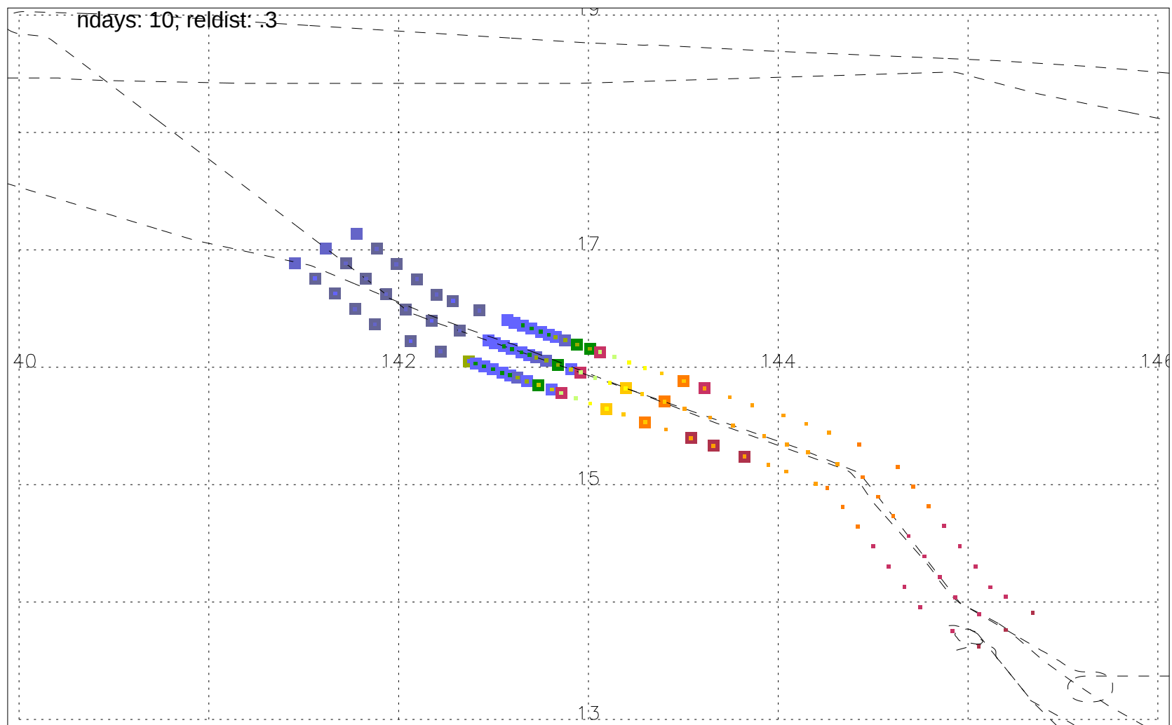
Convective influence for 140304281604 at level 2; 63 out of 117 pts influenced
