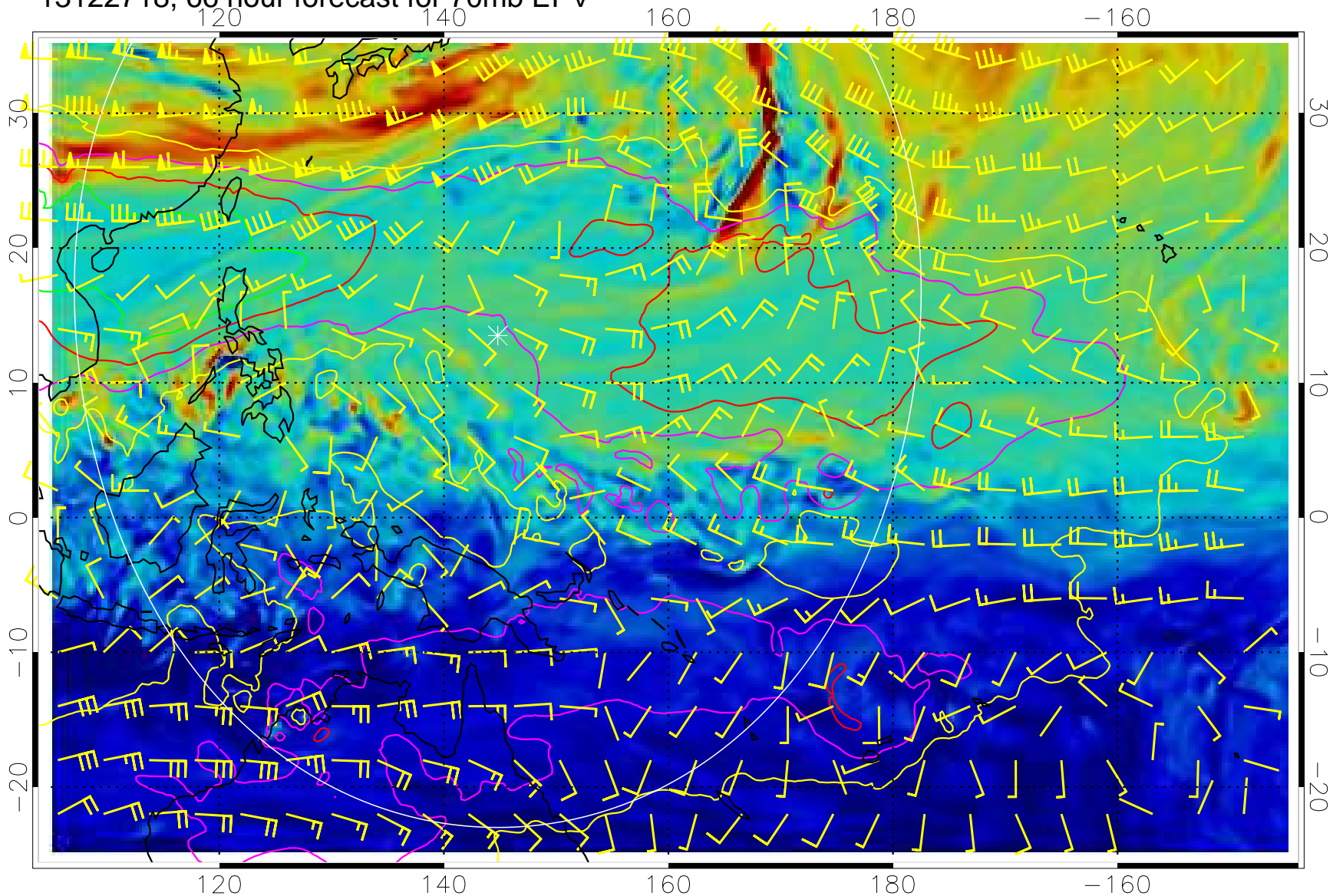
13122718, 66 hour forecast for 70mb EPV
