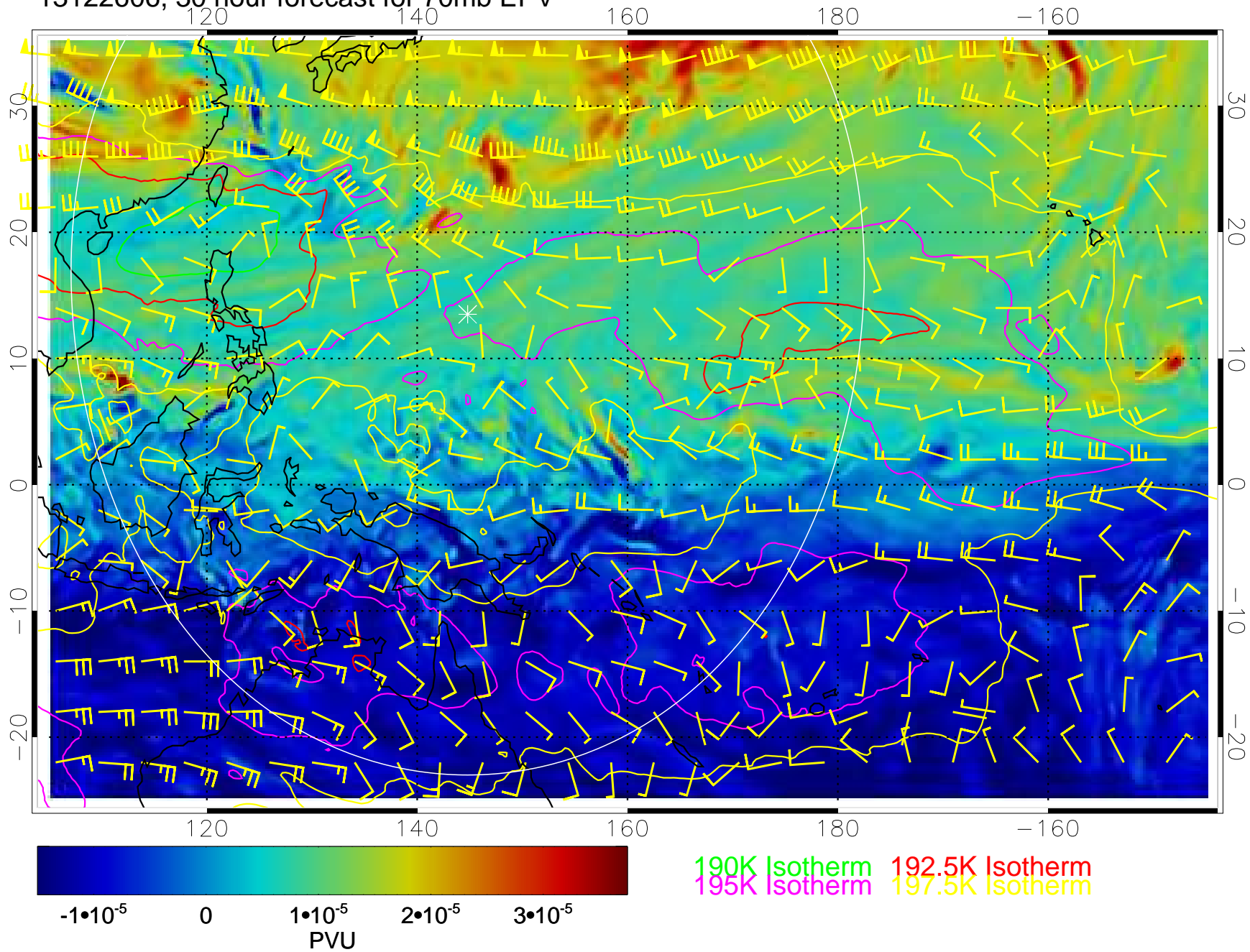
13122606, 30 hour forecast for 70mb EPV
