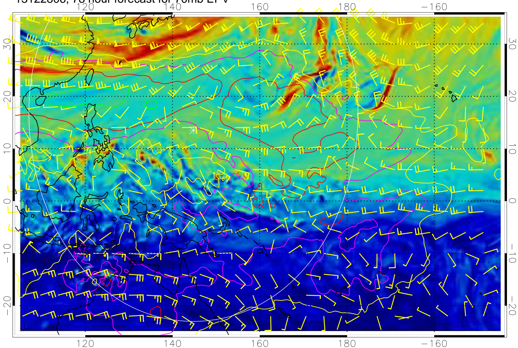
13122806, 78 hour forecast for 70mb EPV
