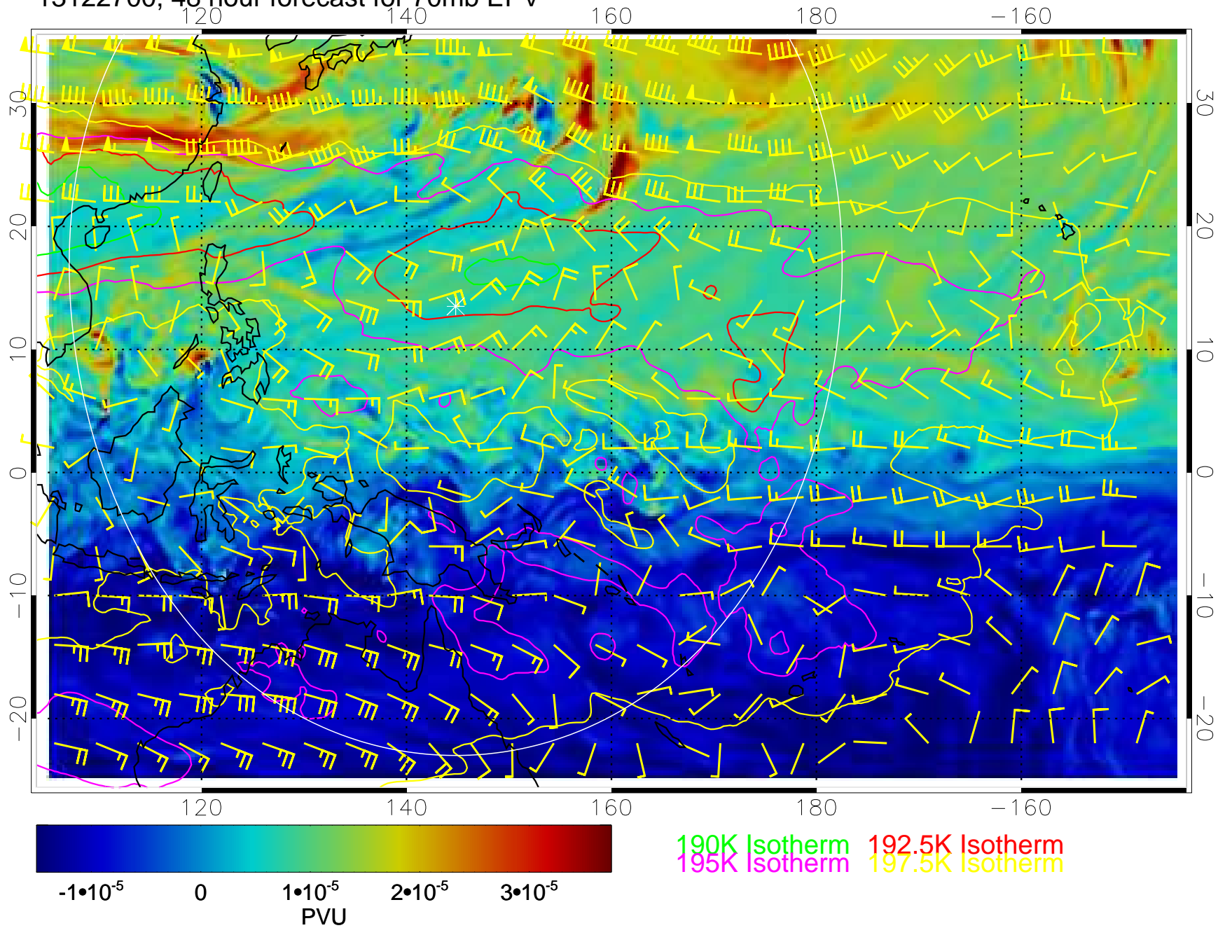
13122700, 48 hour forecast for 70mb EPV
