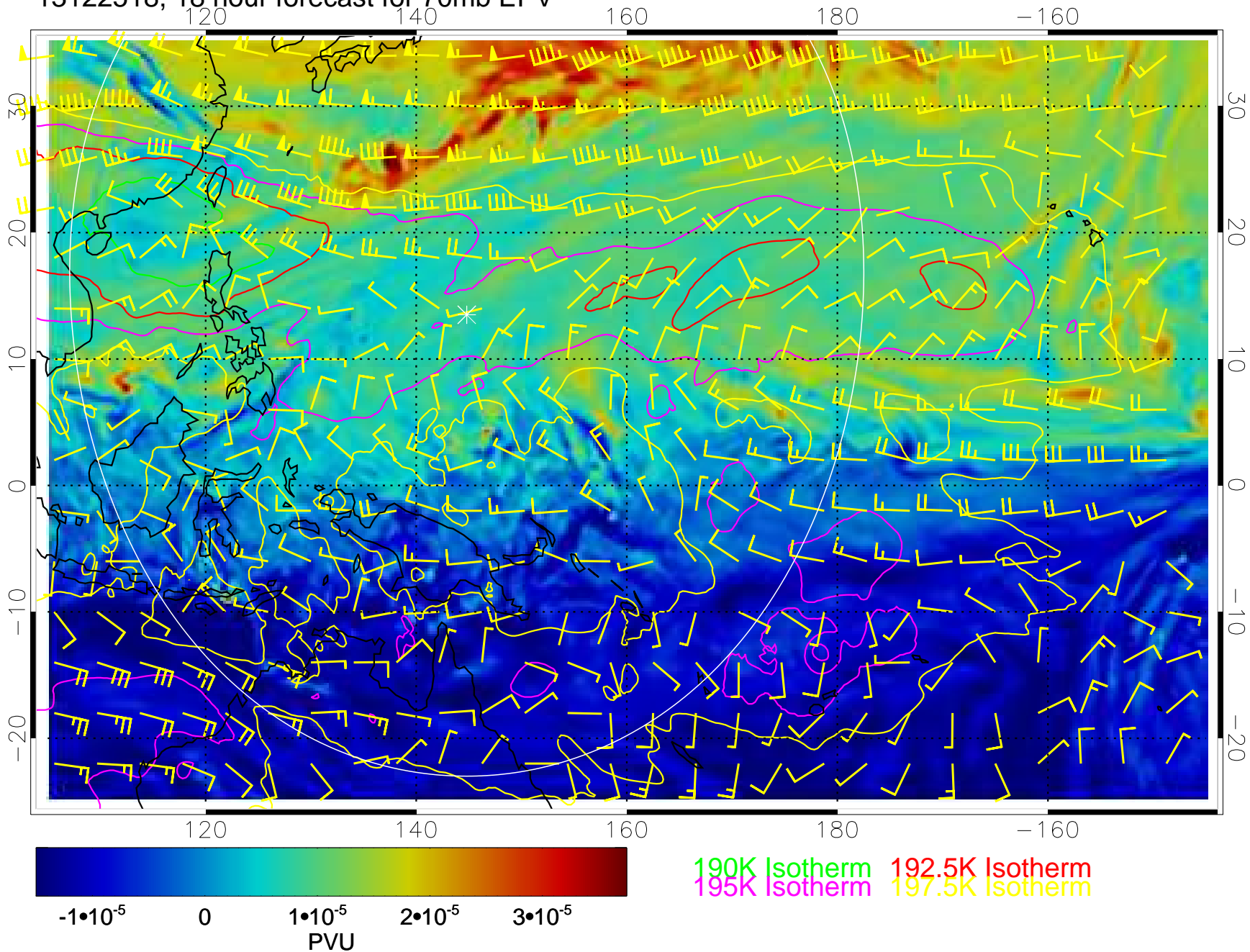
13122518, 18 hour forecast for 70mb EPV
