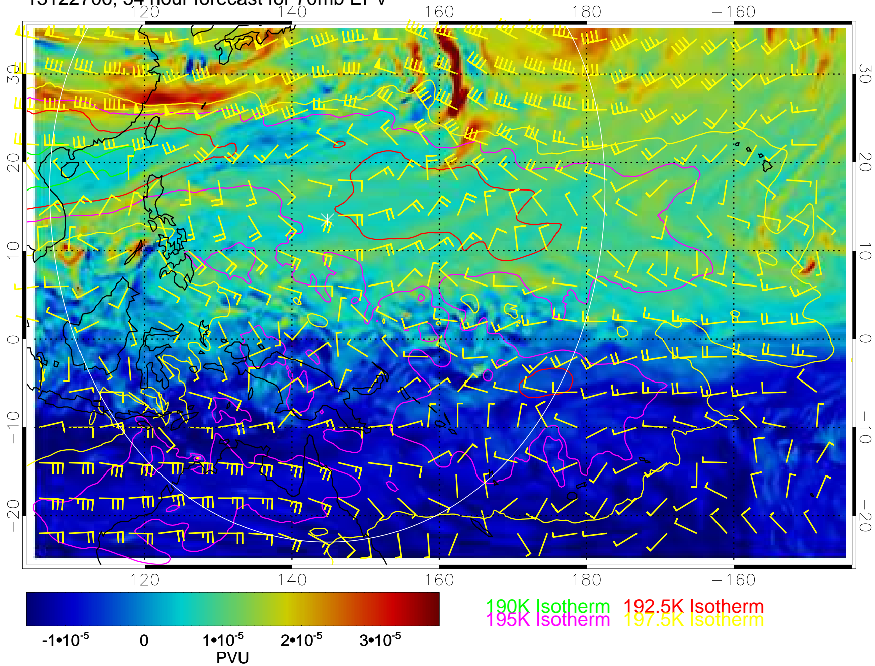
13122706, 54 hour forecast for 70mb EPV
