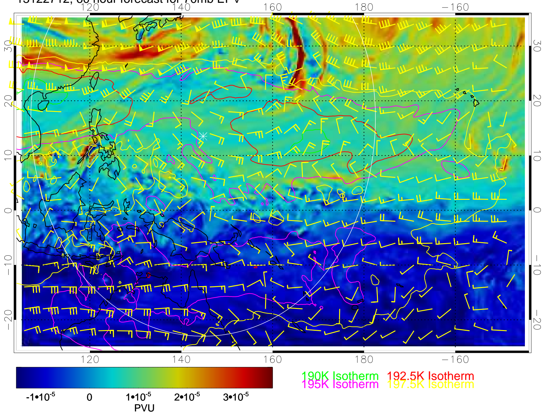
13122712, 60 hour forecast for 70mb EPV
