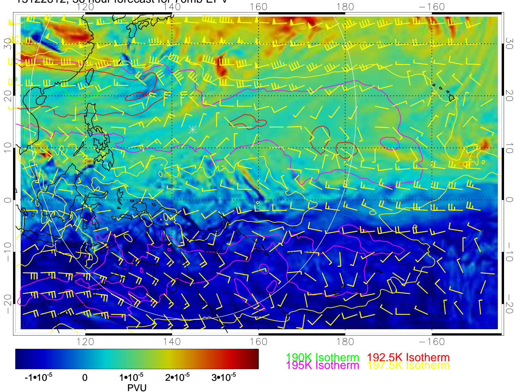
13122612, 36 hour forecast for 70mb EPV
