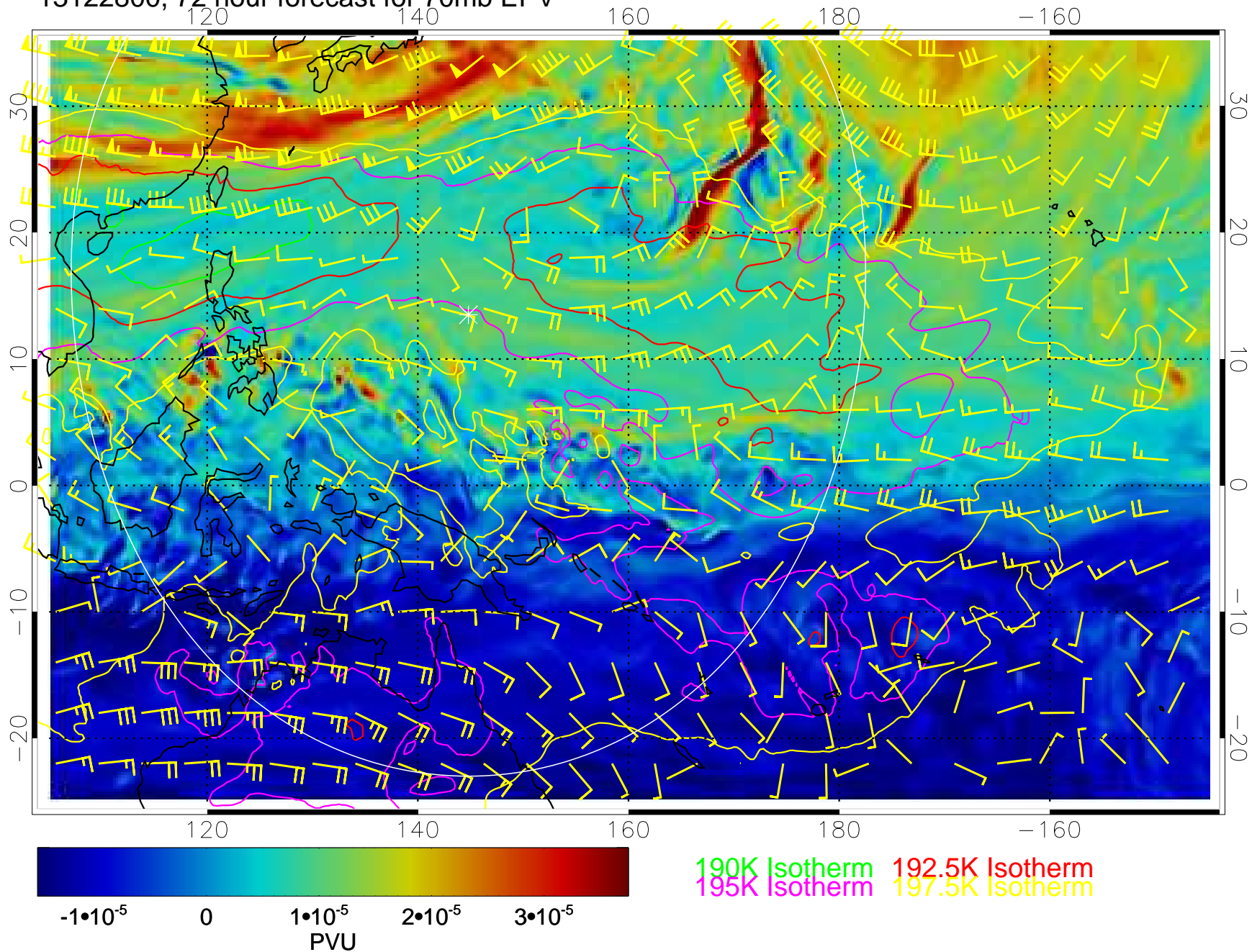
13122800, 72 hour forecast for 70mb EPV
