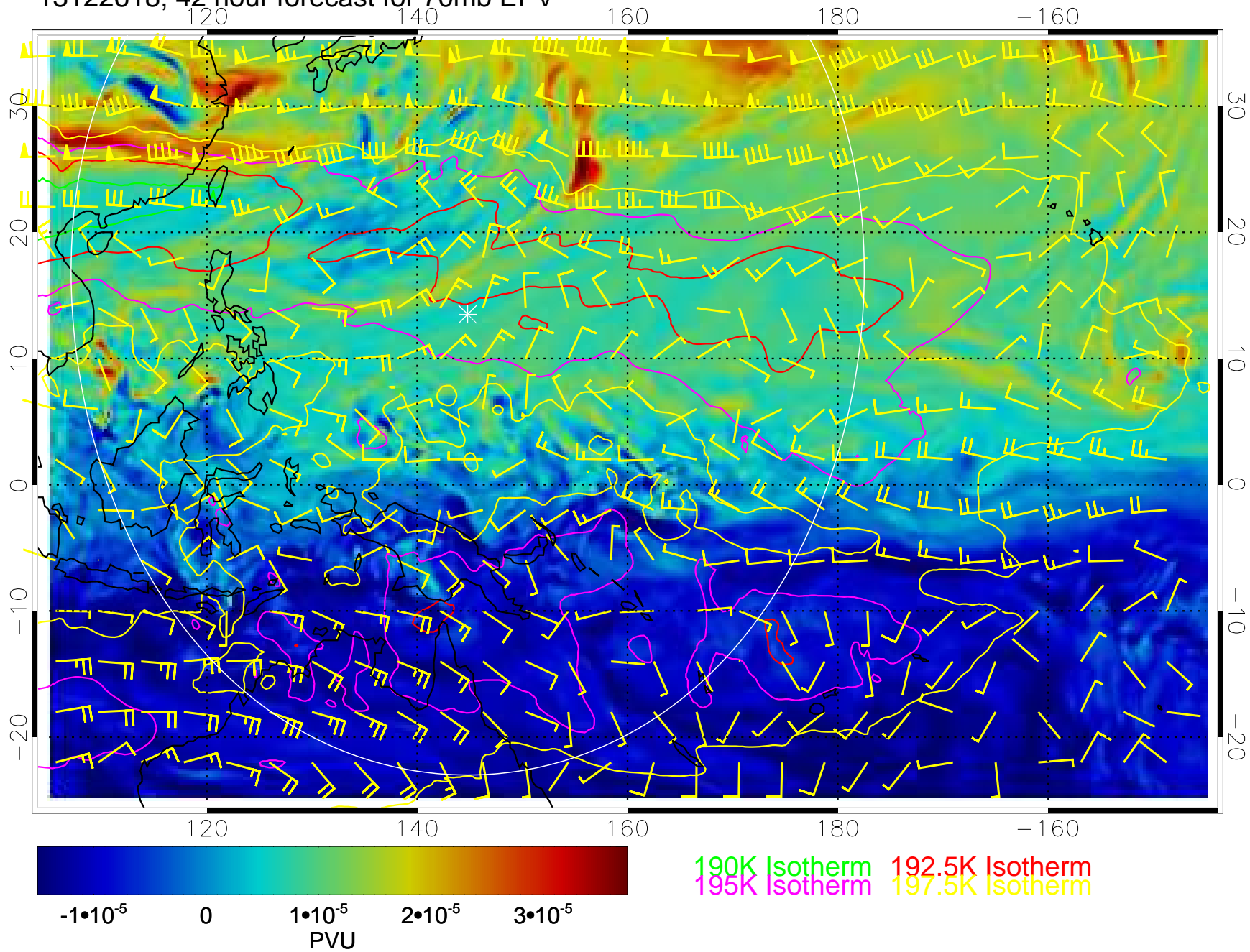
13122618, 42 hour forecast for 70mb EPV
