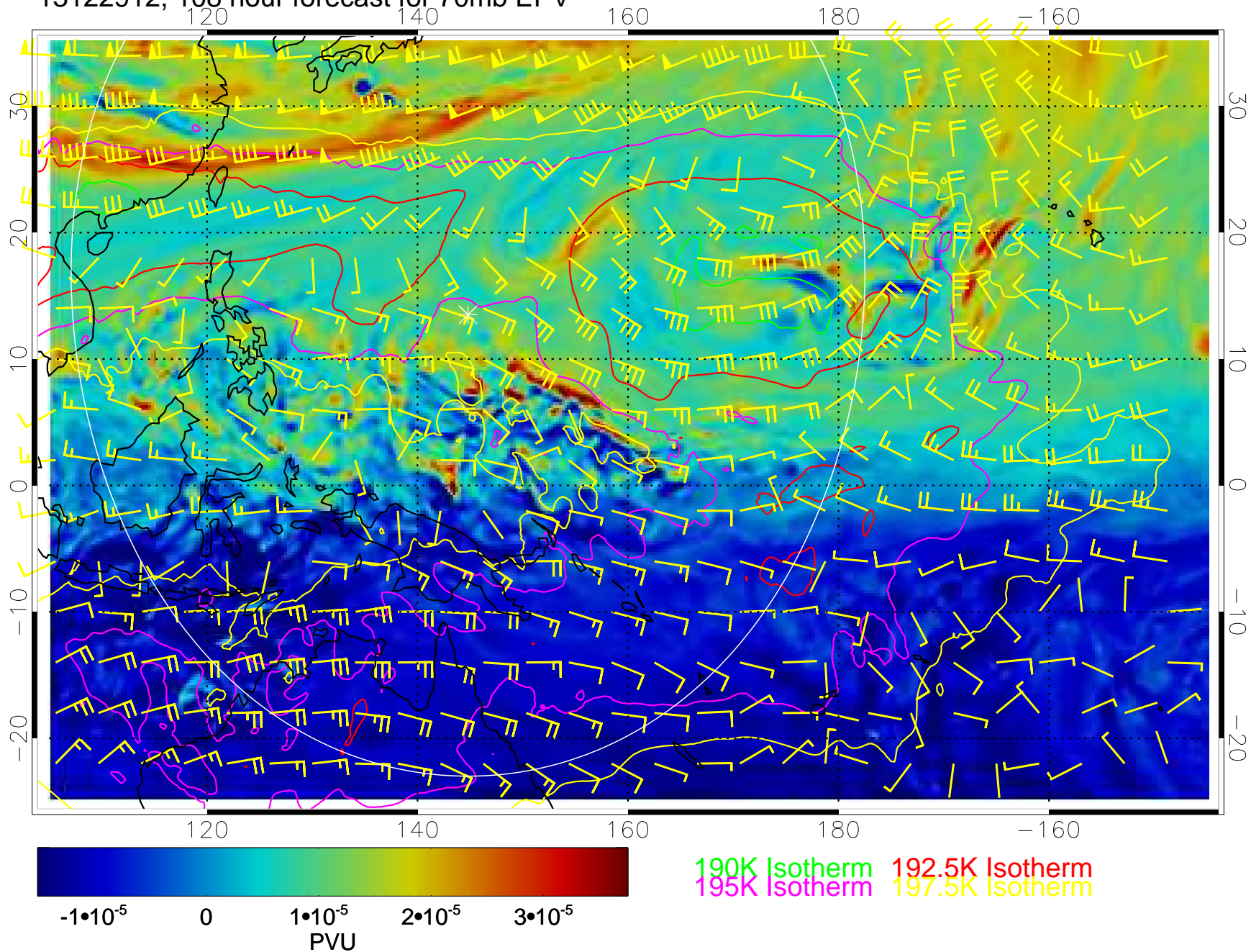
13122912, 108 hour forecast for 70mb EPV
