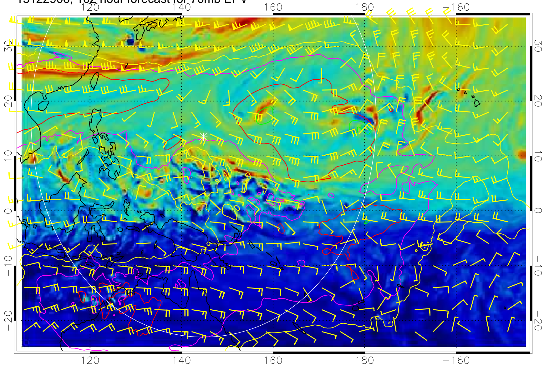
13122906, 102 hour forecast for 70mb EPV
