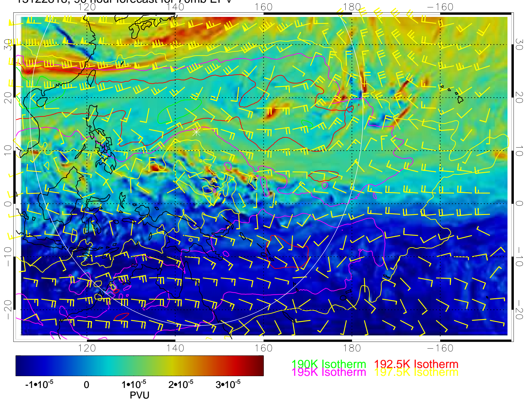
13122818, 90 hour forecast for 70mb EPV
