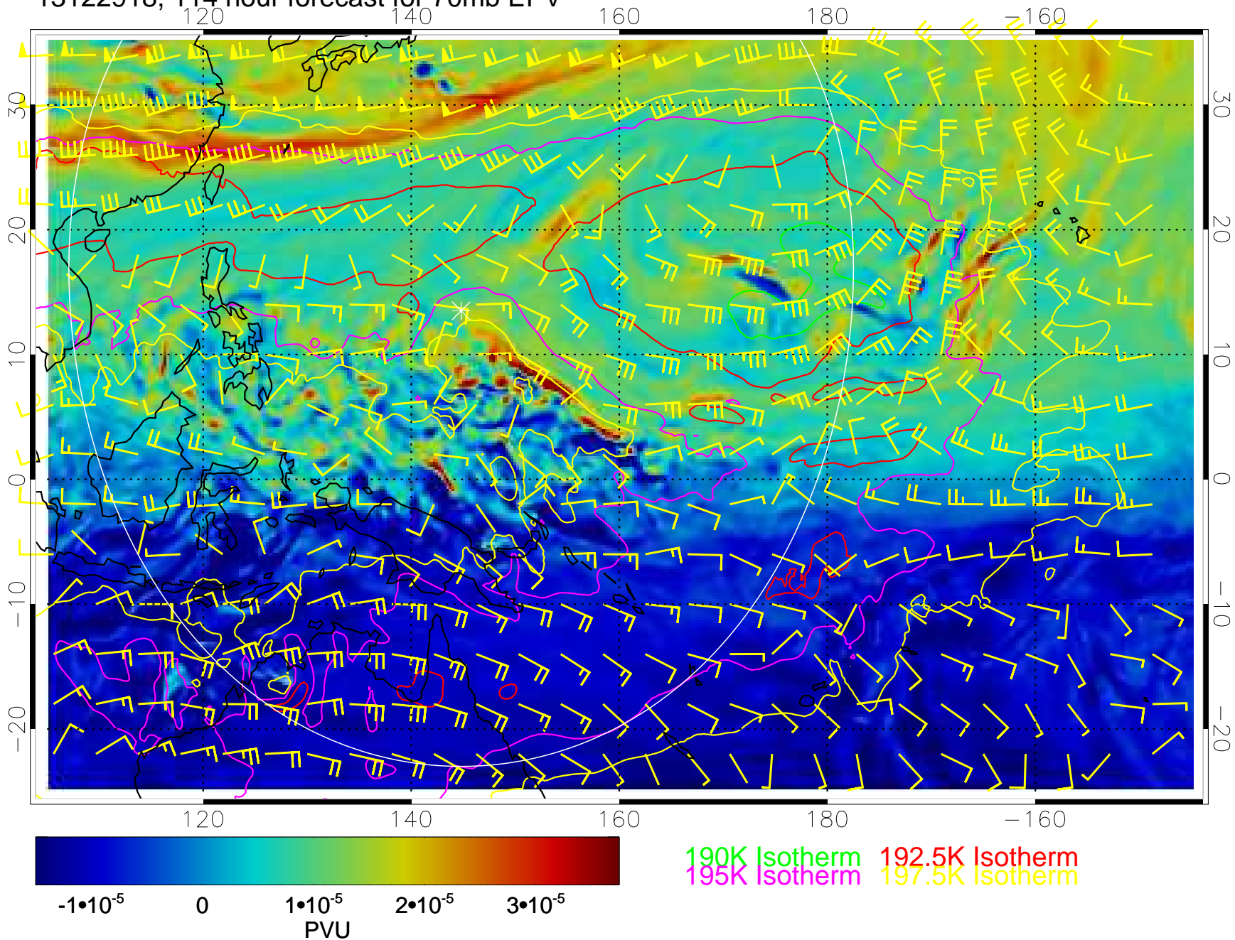
13122918, 114 hour forecast for 70mb EPV
