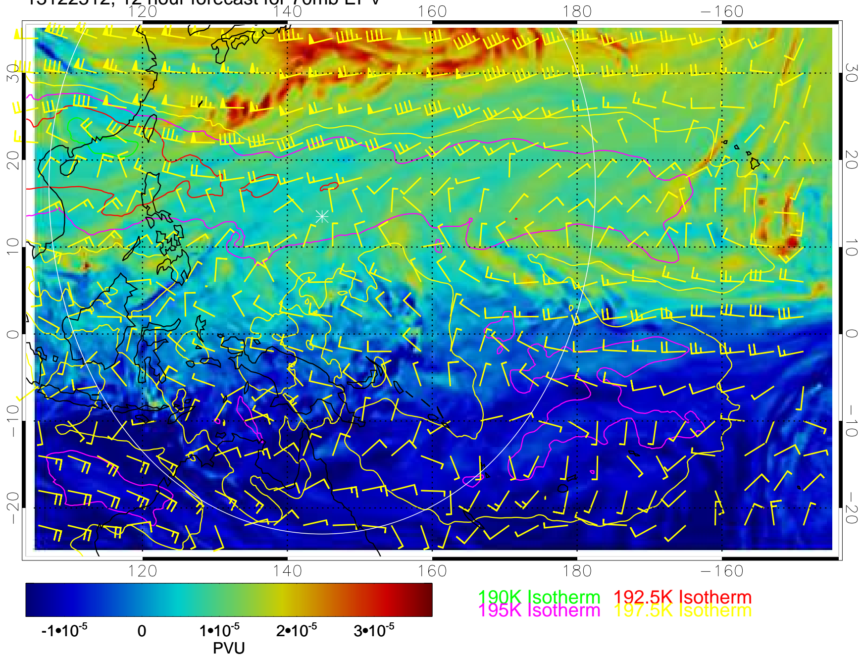
13122512, 12 hour forecast for 70mb EPV
