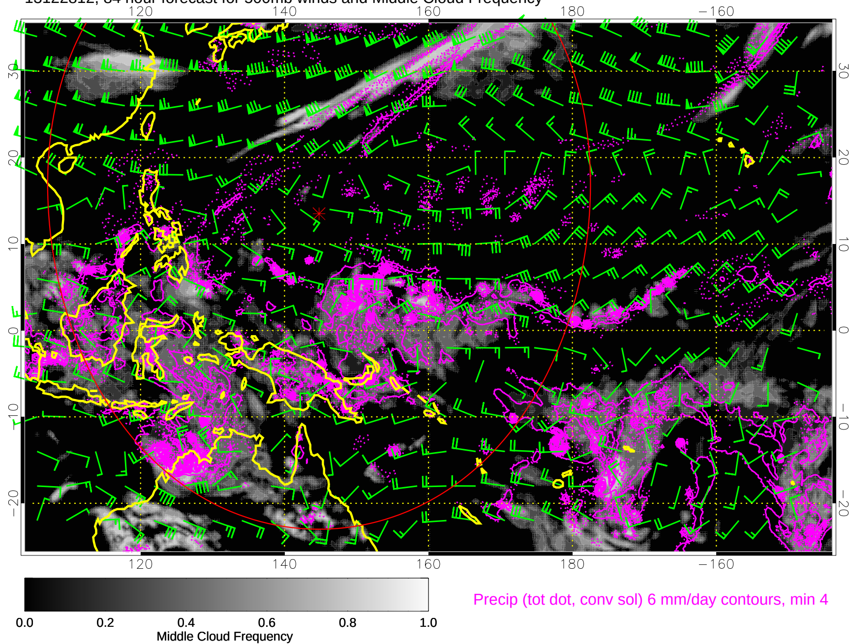
13122812, 84 hour forecast for 500mb winds and Middle Cloud Frequency
