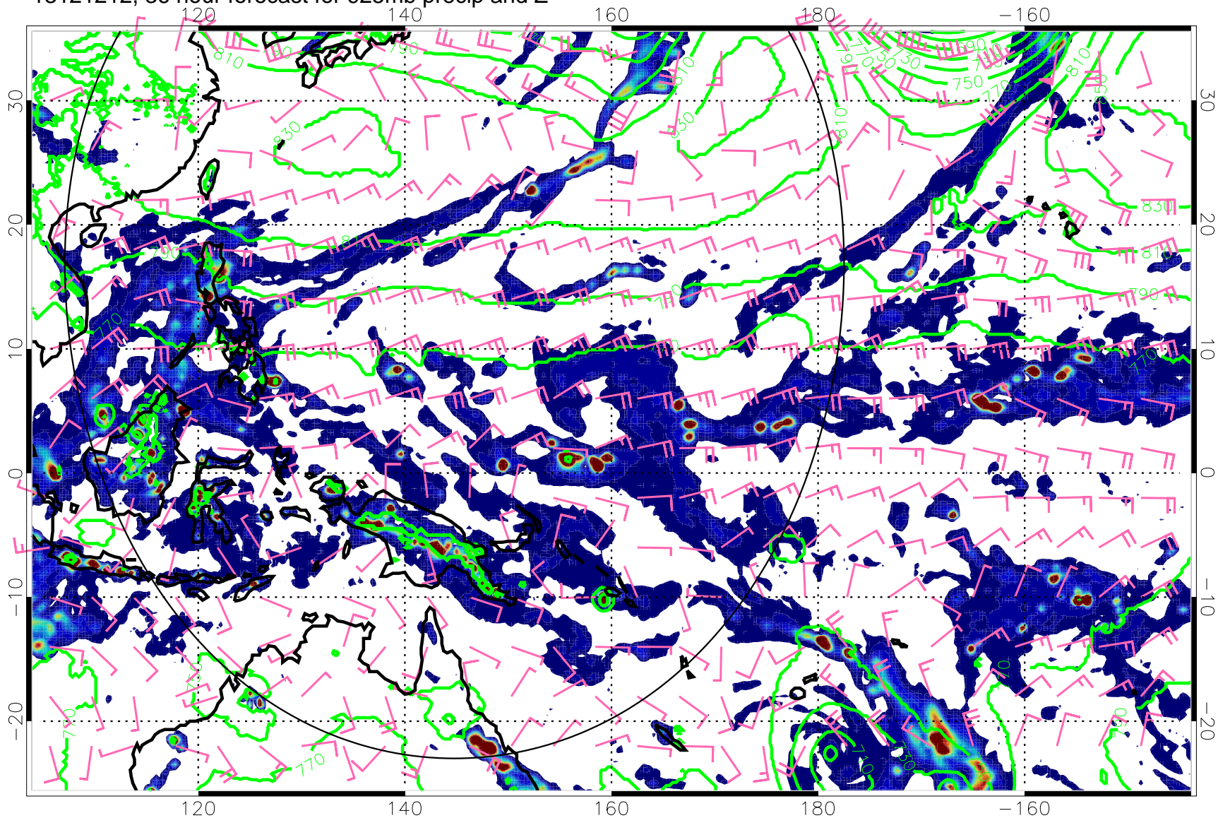
13121212, 36 hour forecast for 925mb precip and Z
