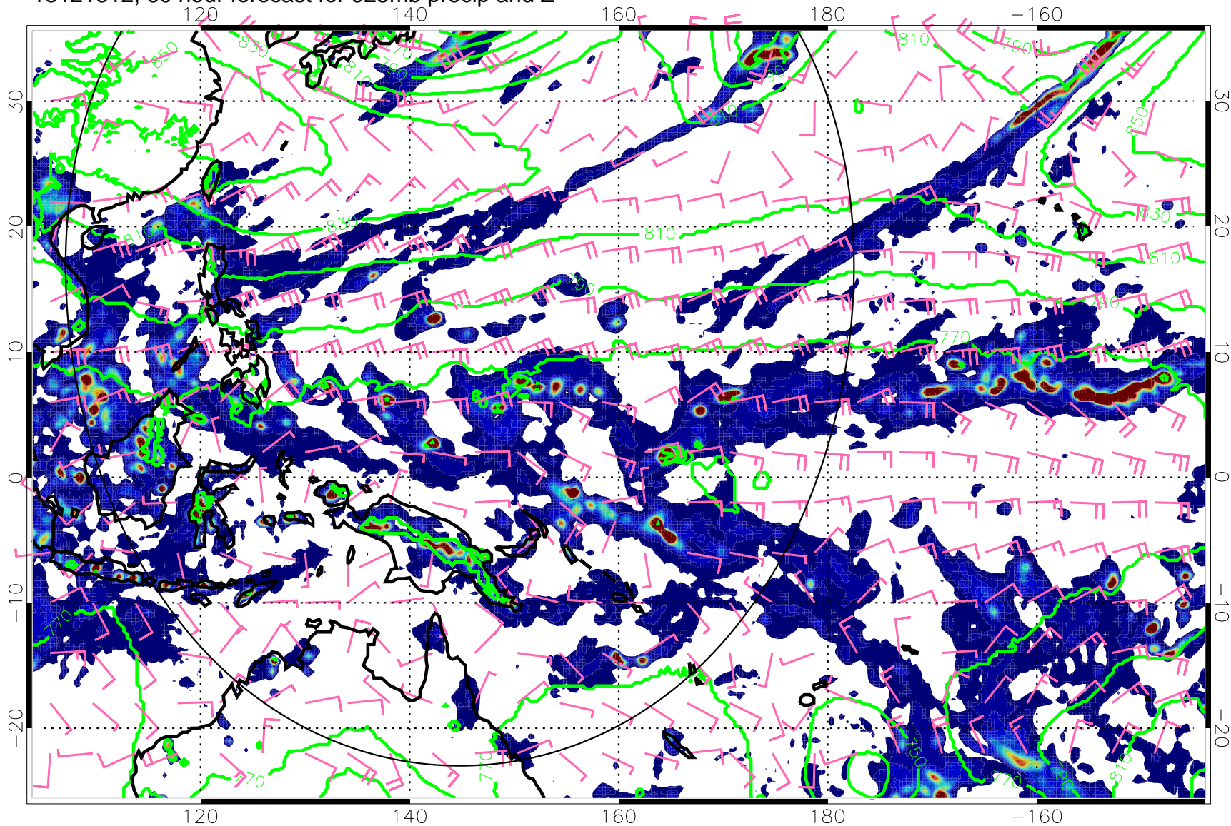
13121312, 60 hour forecast for 925mb precip and Z
