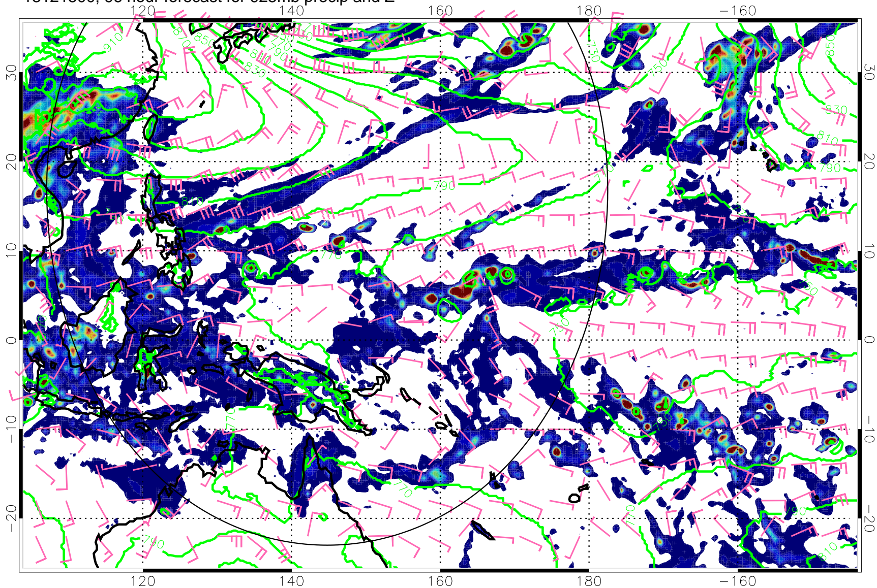
13121500, 96 hour forecast for 925mb precip and Z
