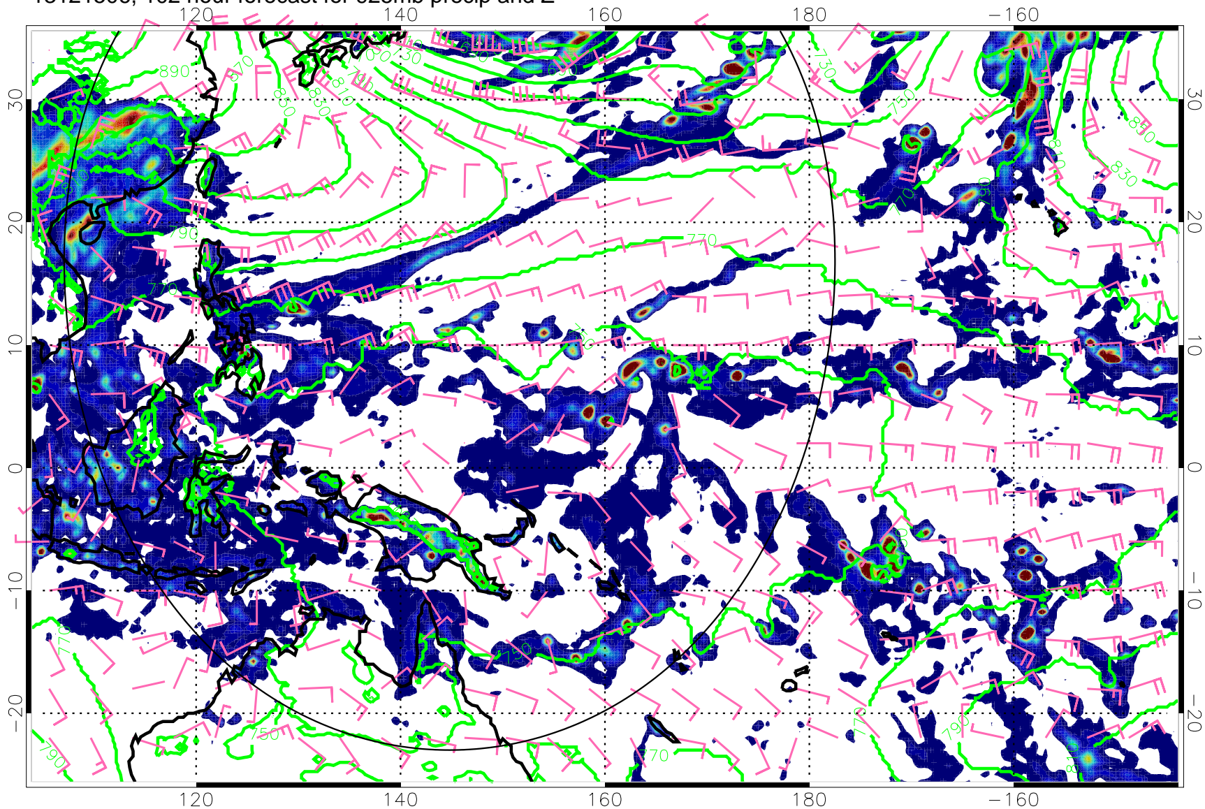
13121506, 102 hour forecast for 925mb precip and Z
