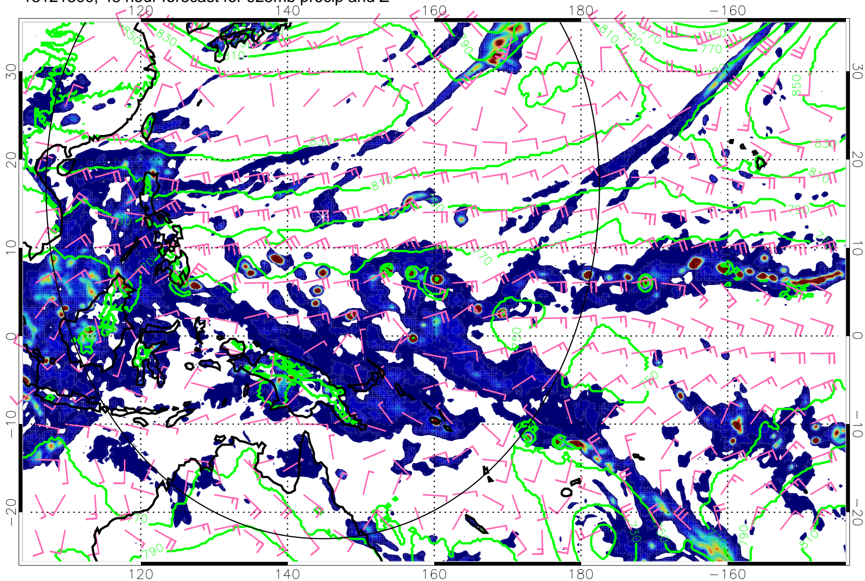
13121300, 48 hour forecast for 925mb precip and Z
