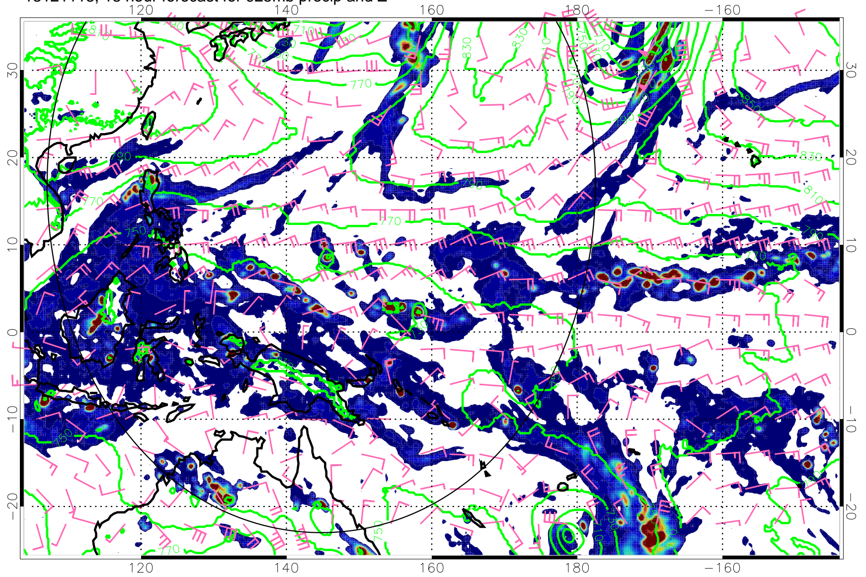
13121118, 18 hour forecast for 925mb precip and Z
