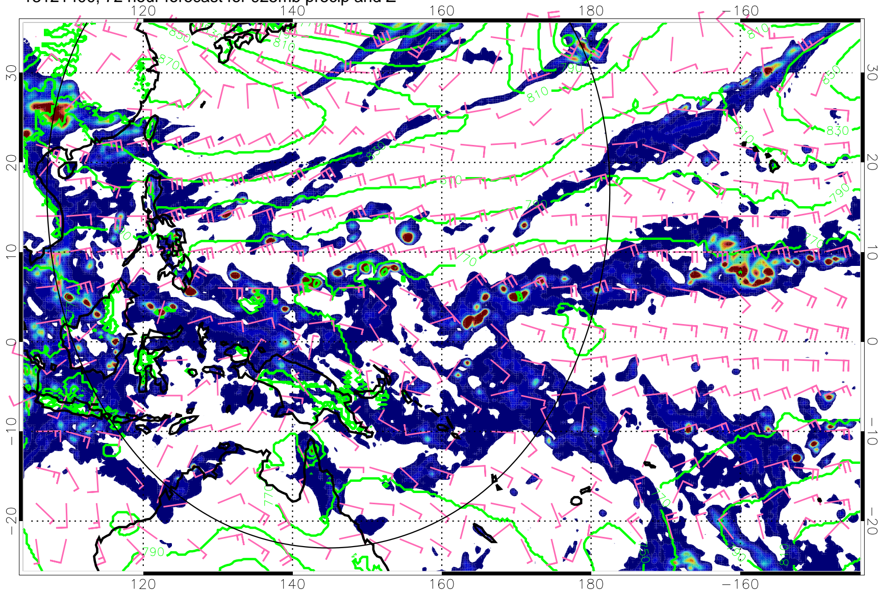
13121400, 72 hour forecast for 925mb precip and Z
