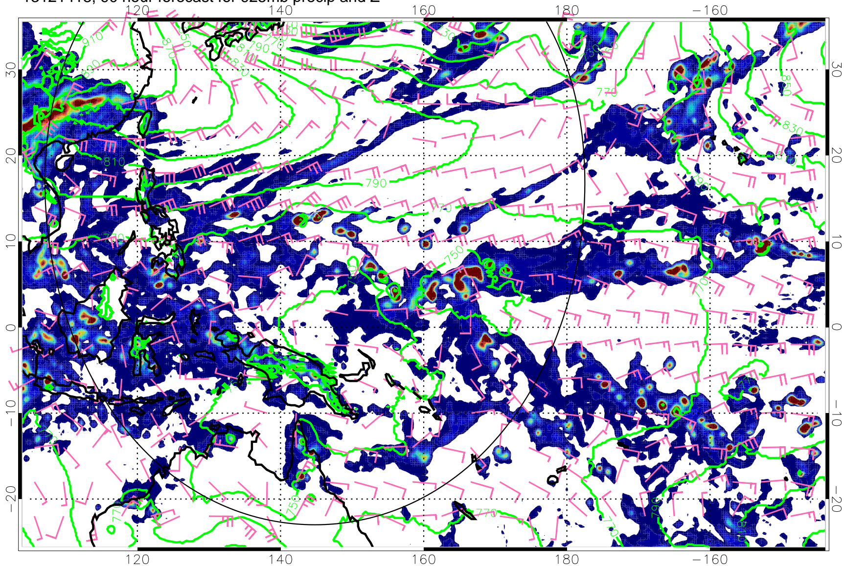
13121418, 90 hour forecast for 925mb precip and Z
