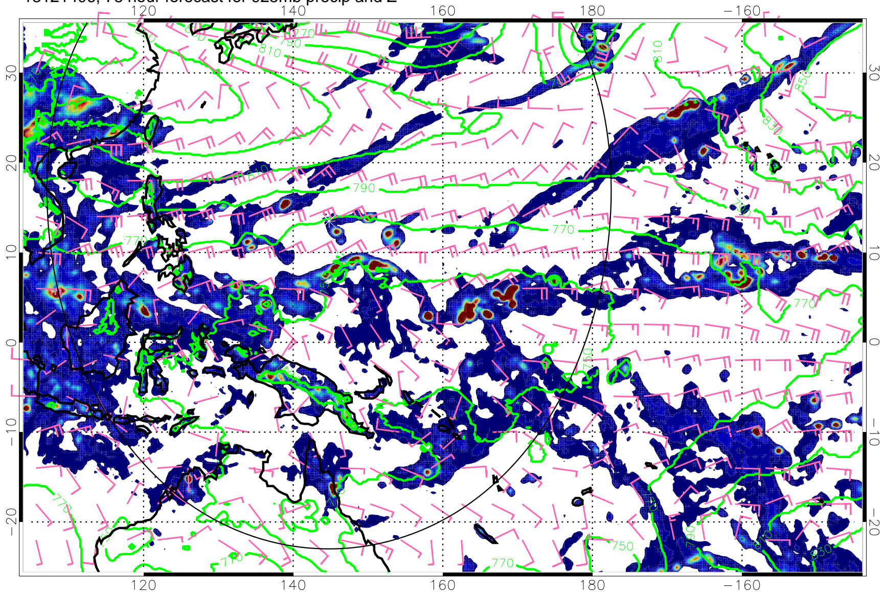
13121406, 78 hour forecast for 925mb precip and Z
