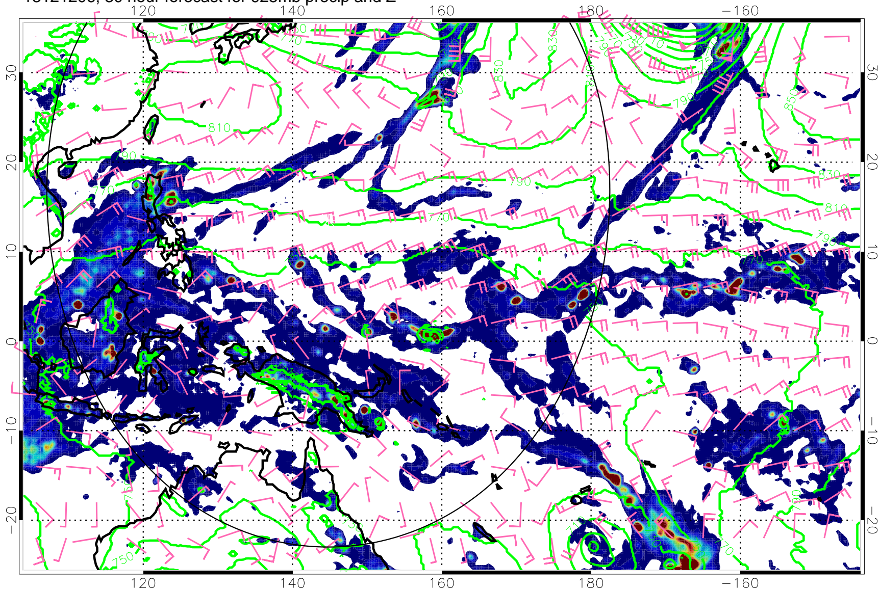
13121206, 30 hour forecast for 925mb precip and Z
