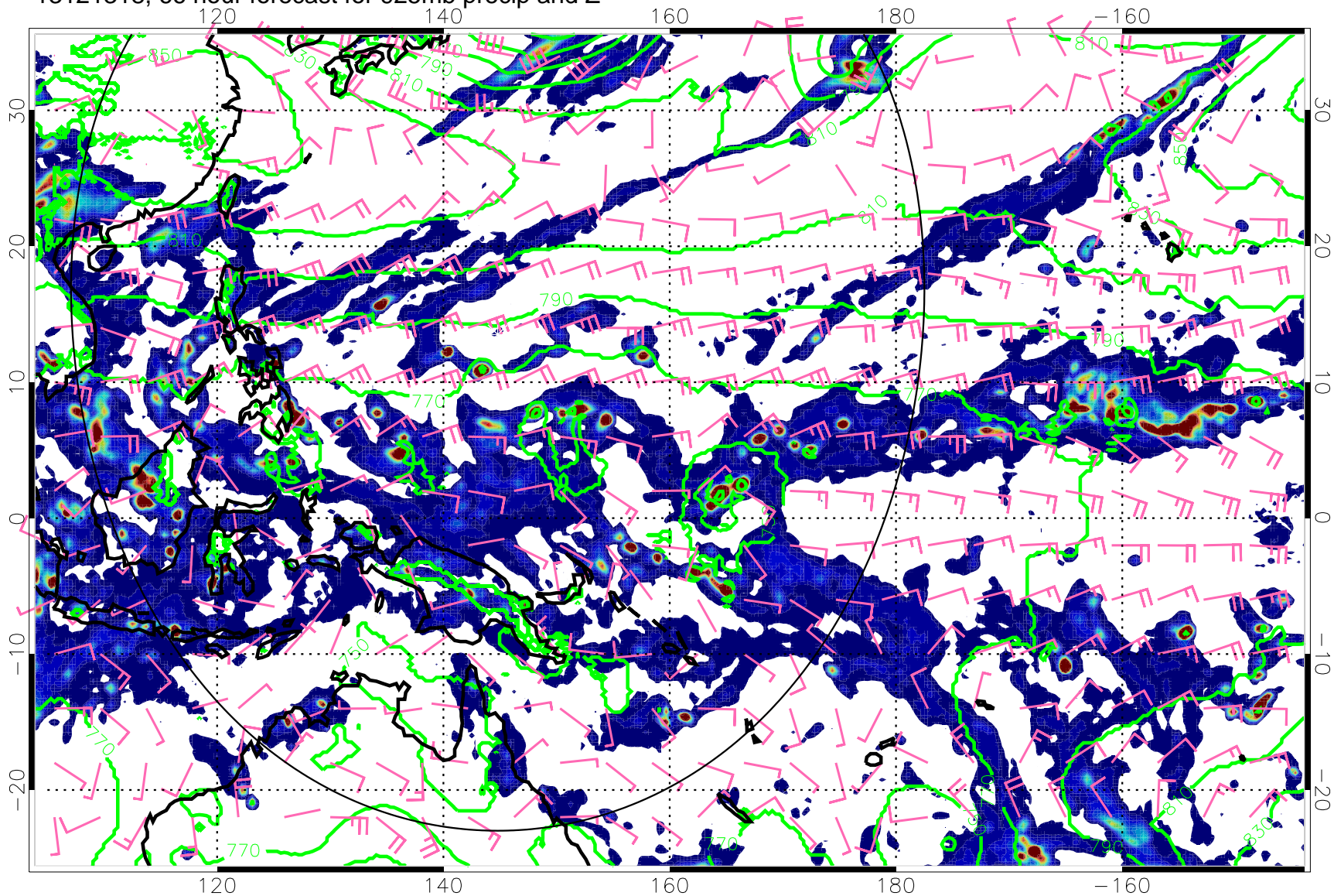
13121318, 66 hour forecast for 925mb precip and Z
