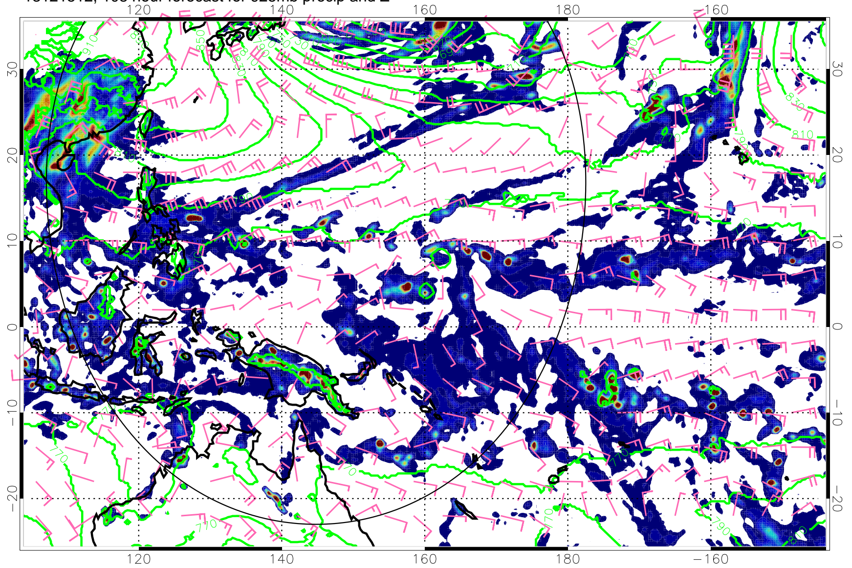
13121512, 108 hour forecast for 925mb precip and Z
