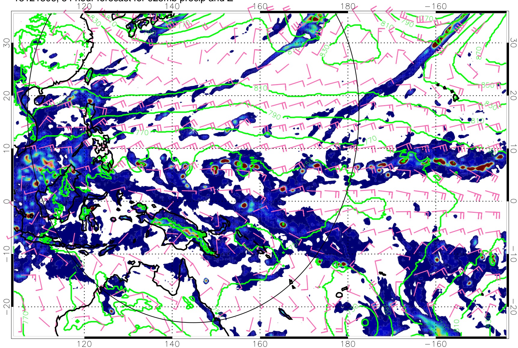
13121306, 54 hour forecast for 925mb precip and Z
