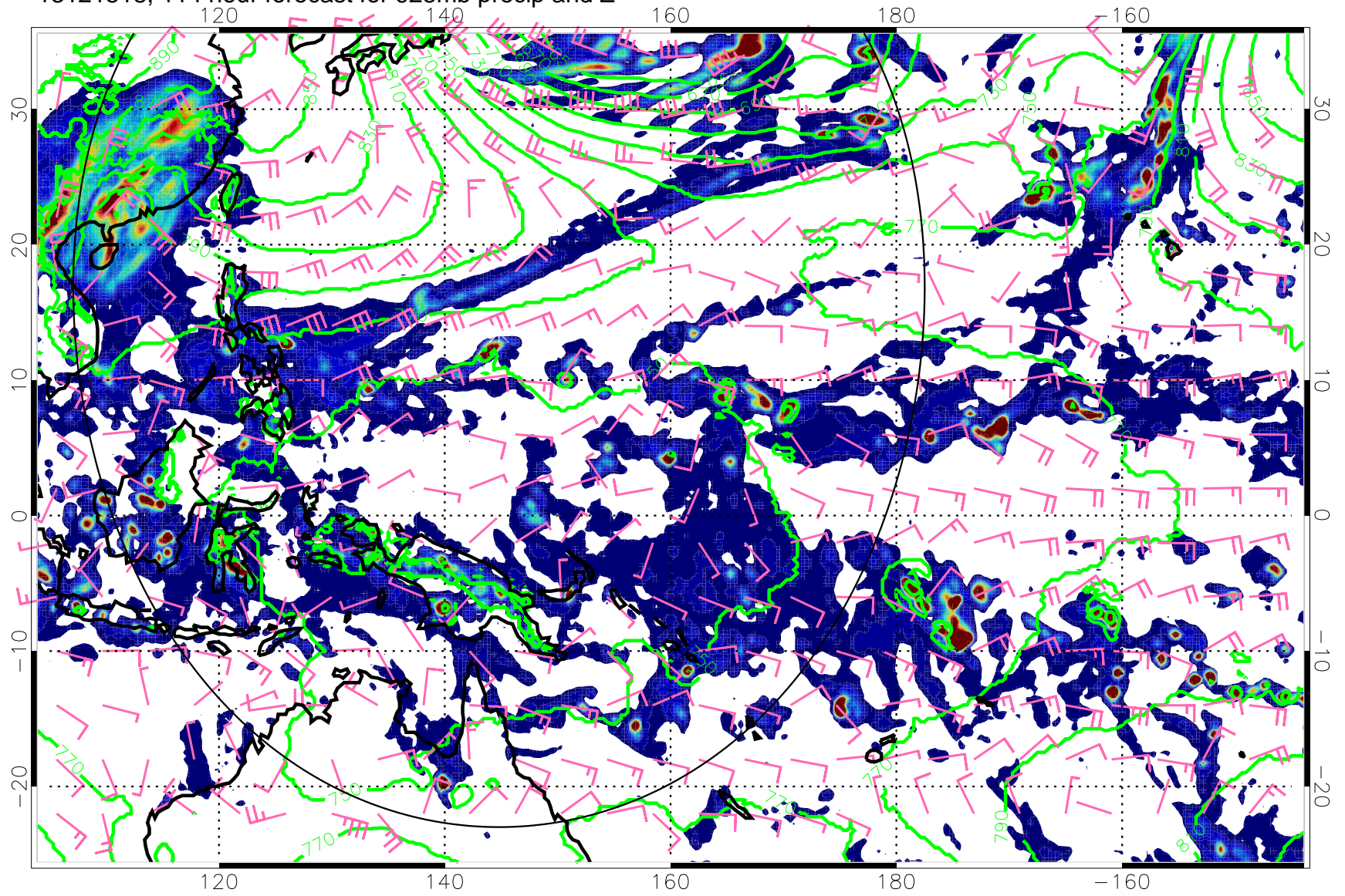
13121518, 114 hour forecast for 925mb precip and Z
