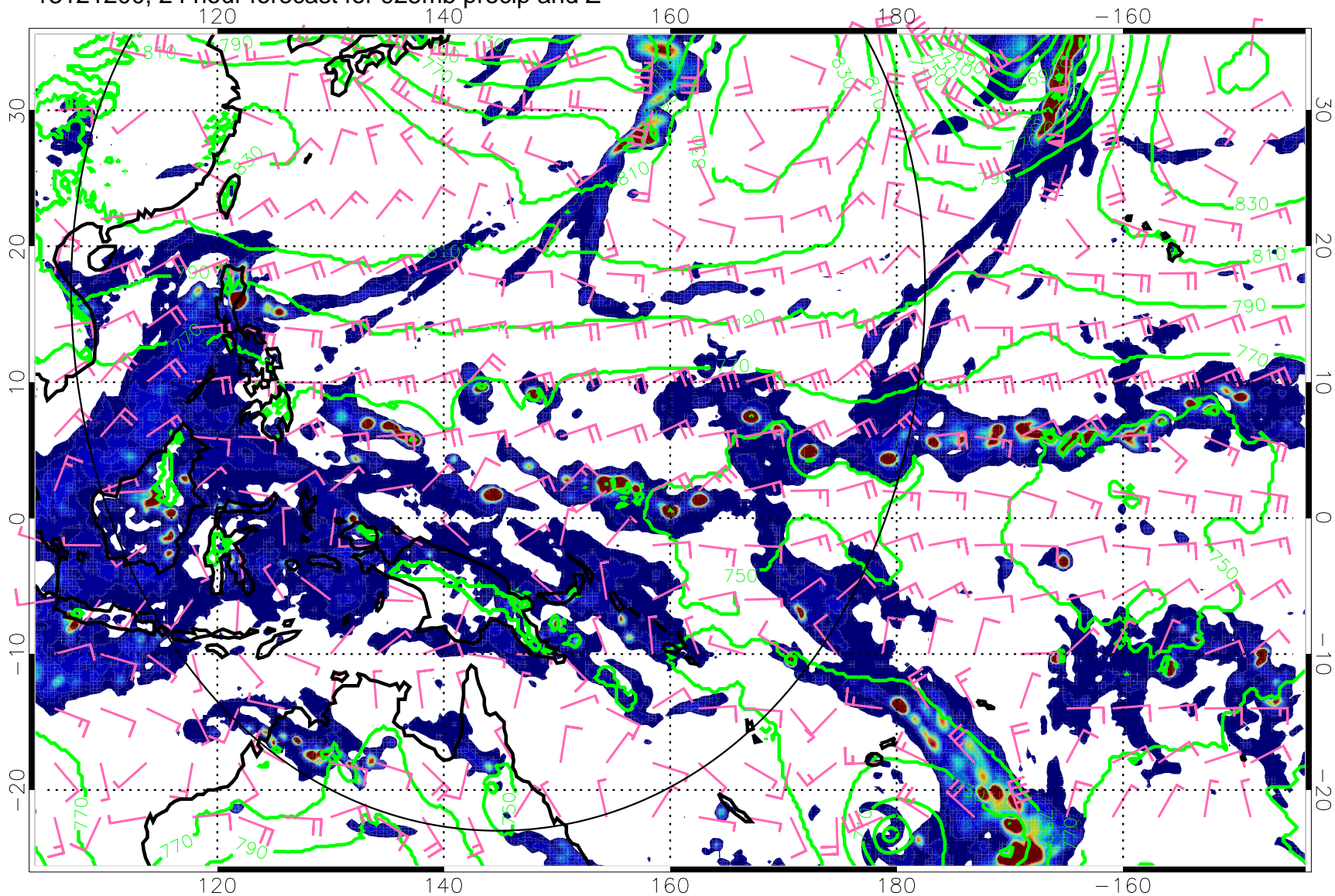
13121200, 24 hour forecast for 925mb precip and Z
