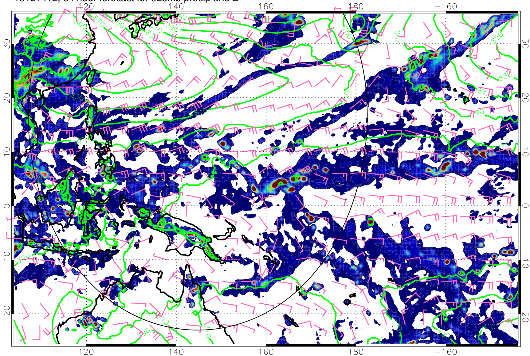
13121412, 84 hour forecast for 925mb precip and Z
