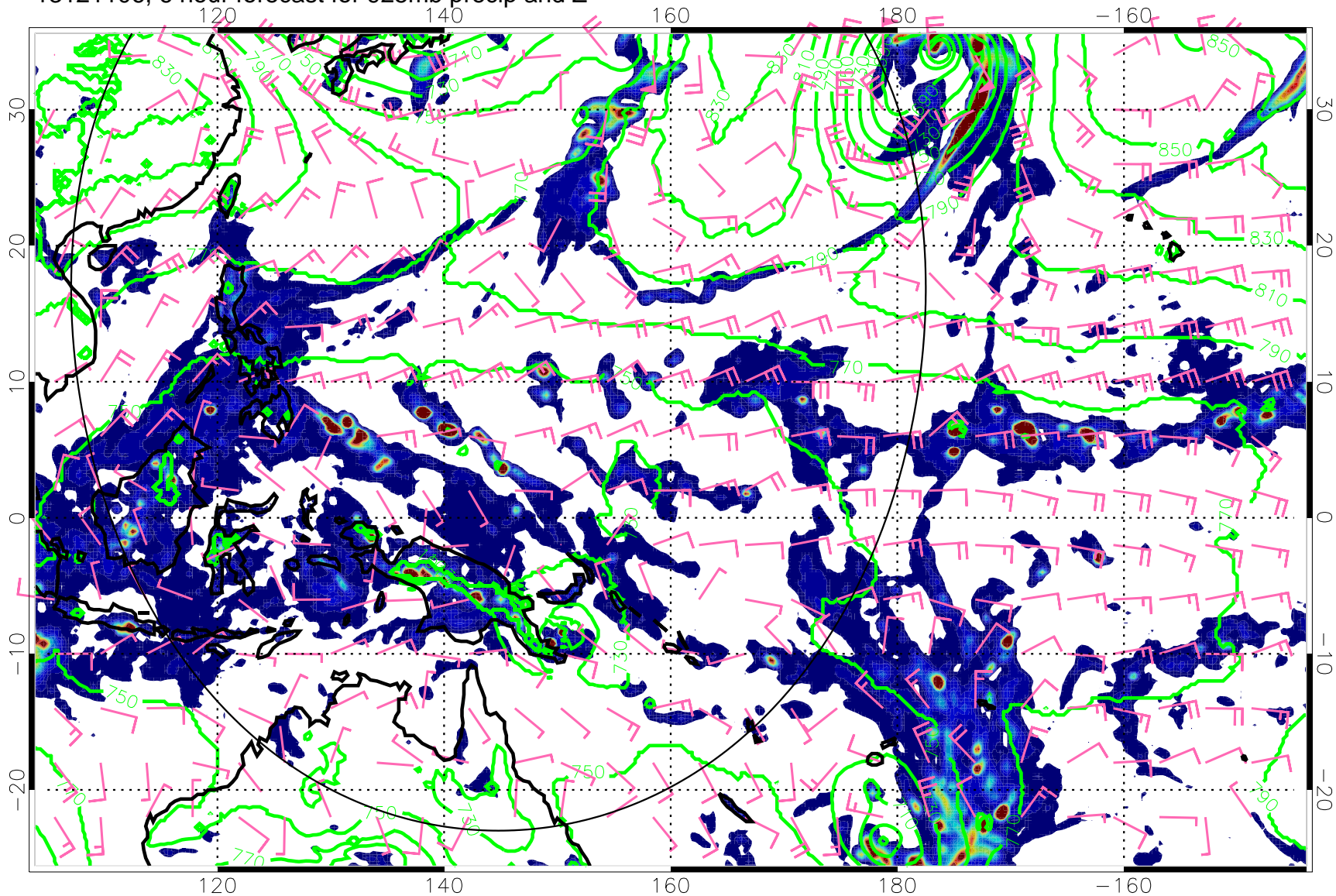
13121106, 6 hour forecast for 925mb precip and Z
