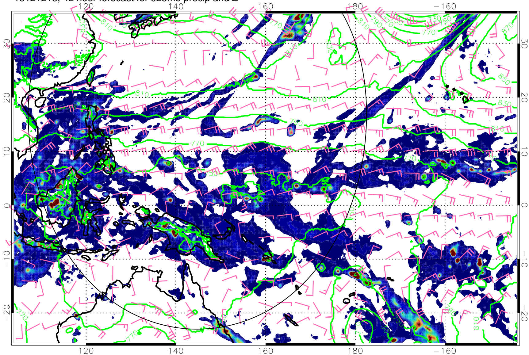
13121218, 42 hour forecast for 925mb precip and Z
