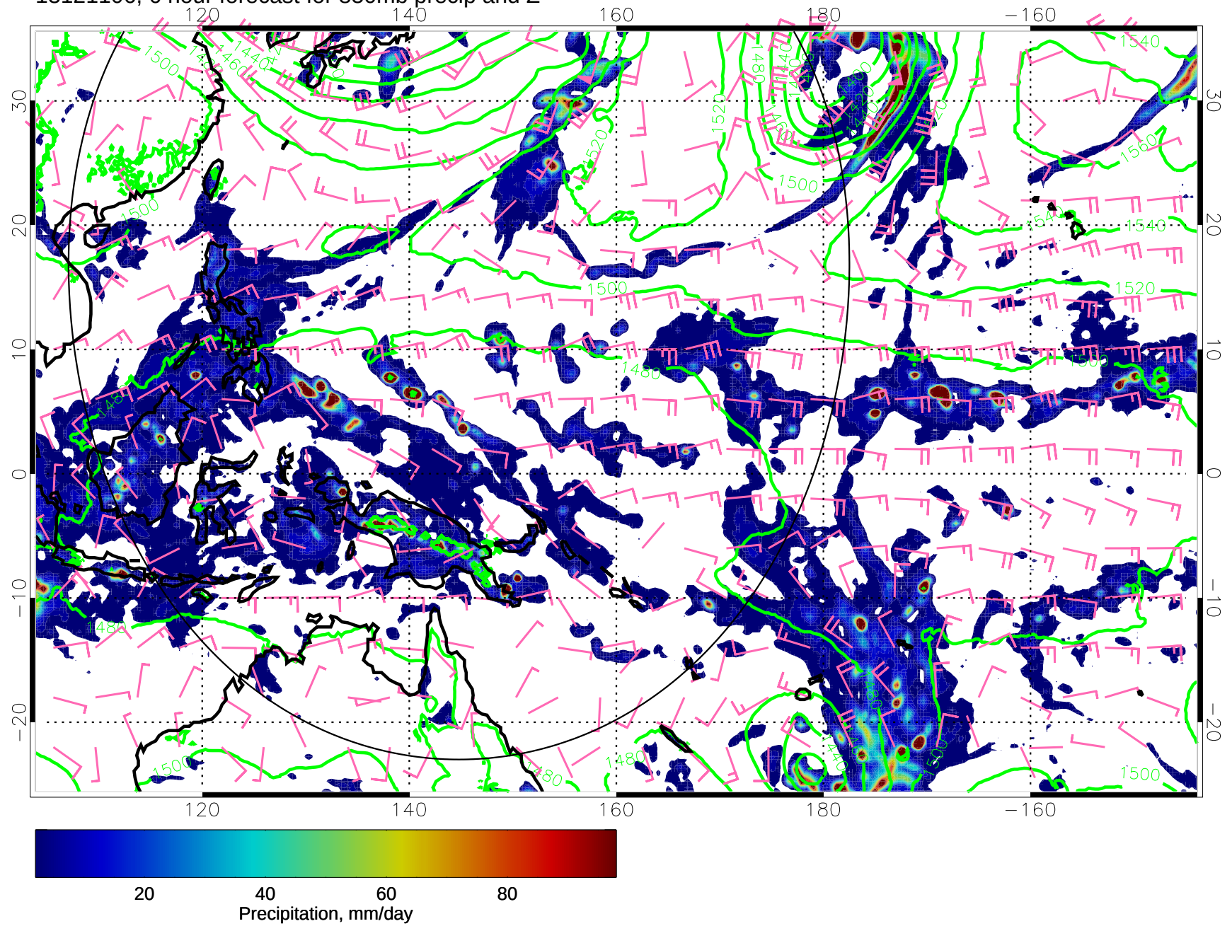
13121106, 6 hour forecast for 850mb precip and Z
