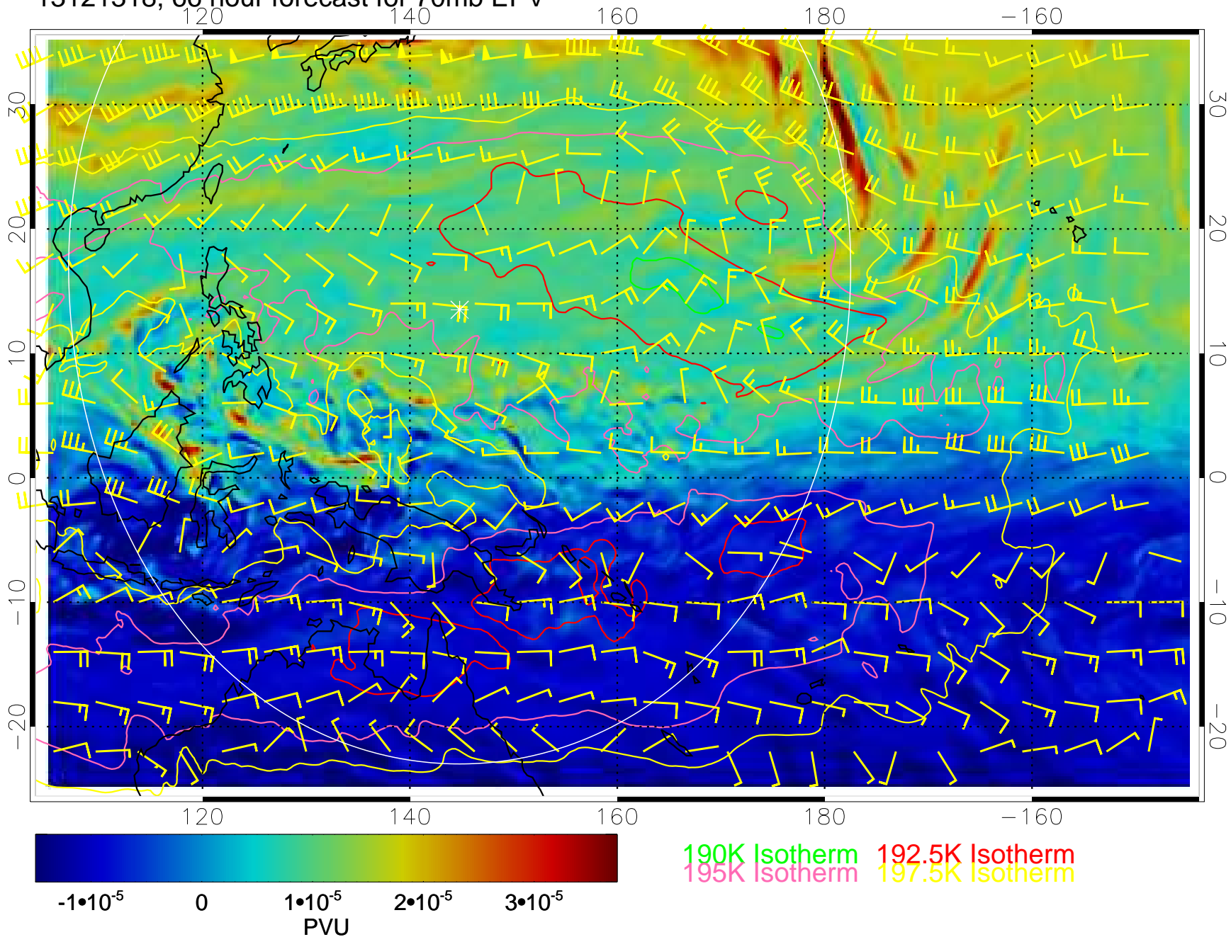
13121318, 66 hour forecast for 70mb EPV
