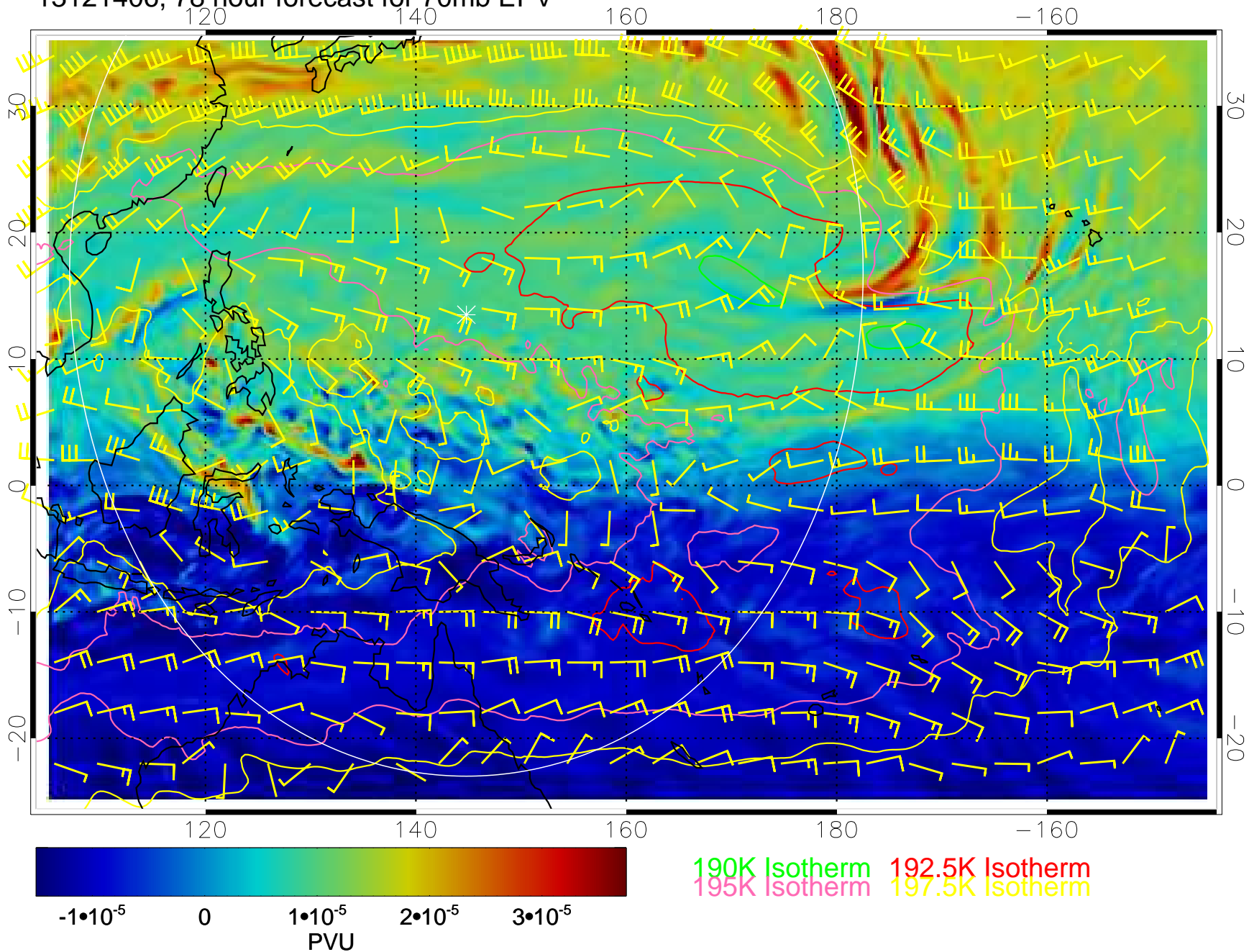
13121406, 78 hour forecast for 70mb EPV
