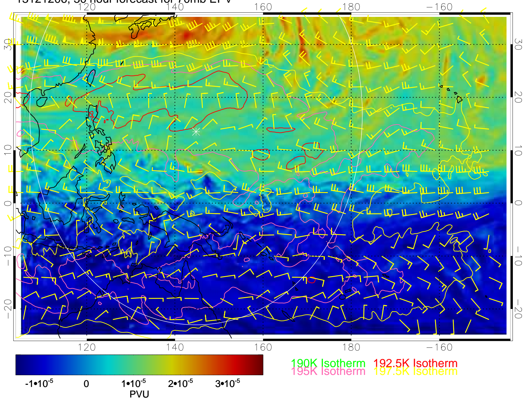
13121206, 30 hour forecast for 70mb EPV
