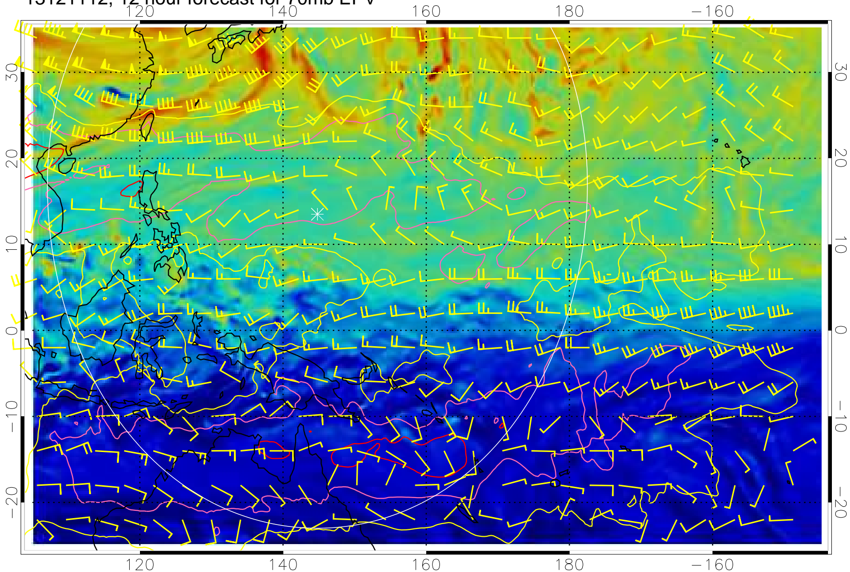
13121112, 12 hour forecast for 70mb EPV
