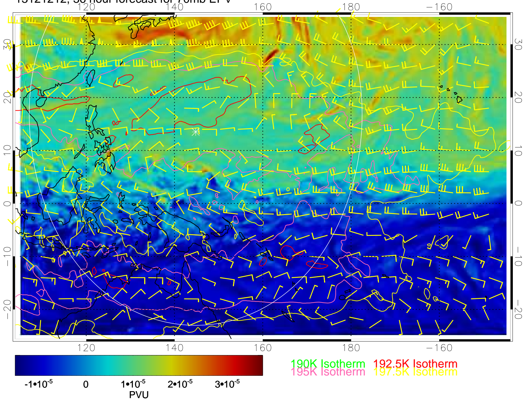
13121212, 36 hour forecast for 70mb EPV
