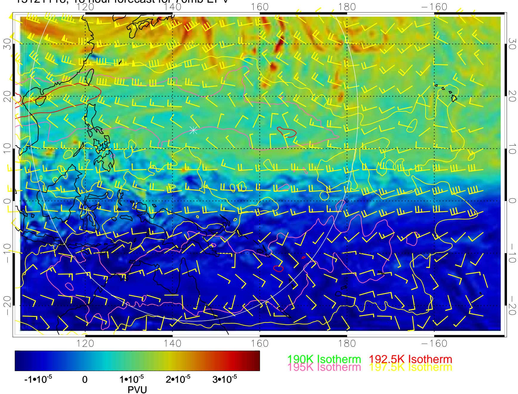
13121118, 18 hour forecast for 70mb EPV
