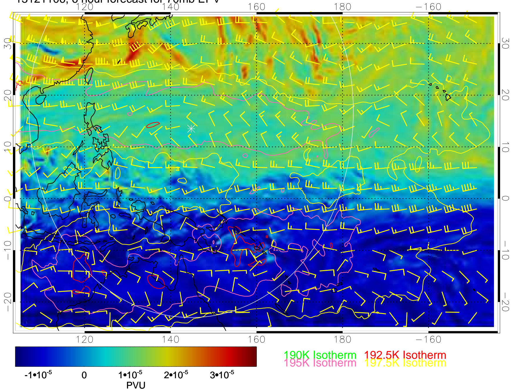
13121106, 6 hour forecast for 70mb EPV
