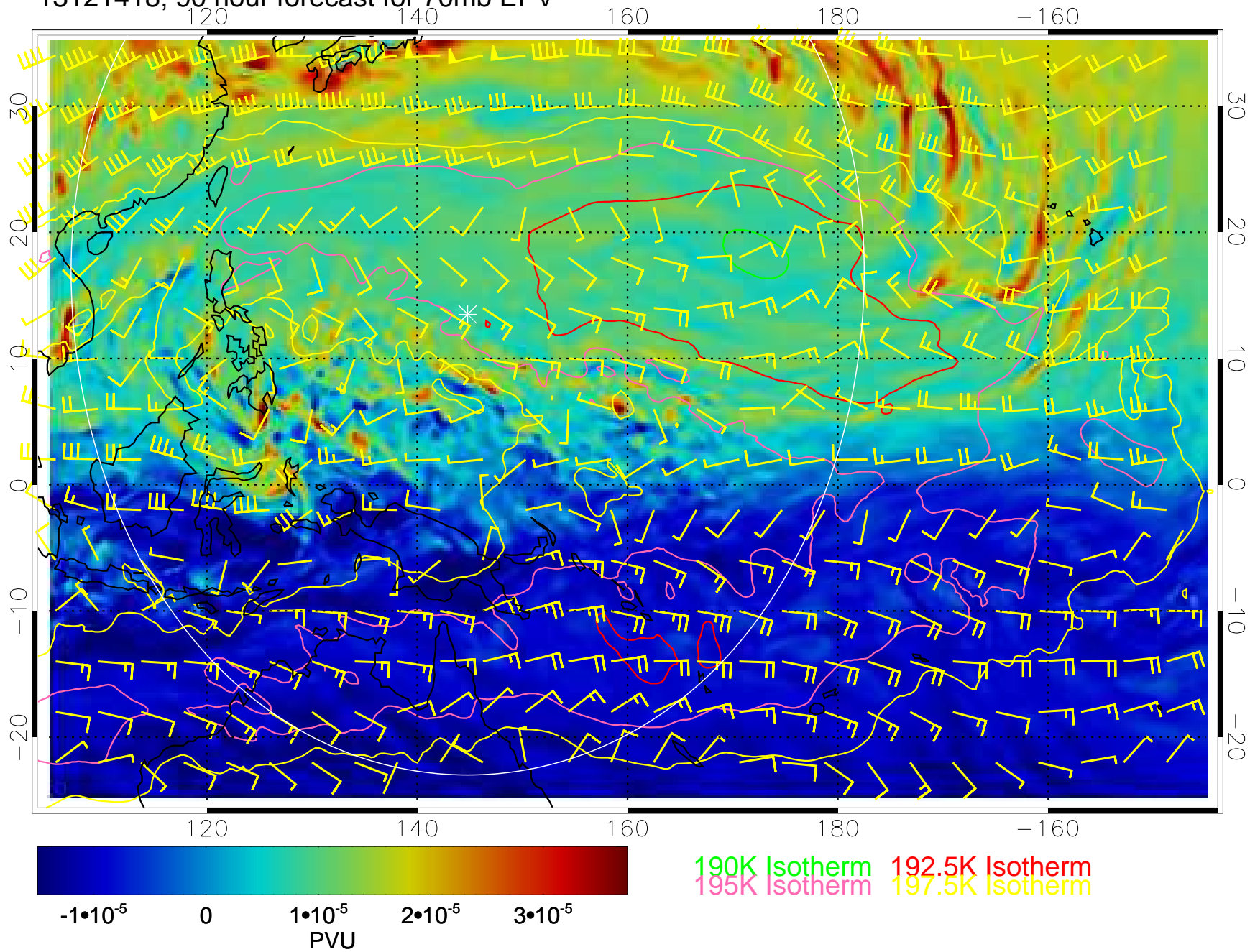
13121418, 90 hour forecast for 70mb EPV
