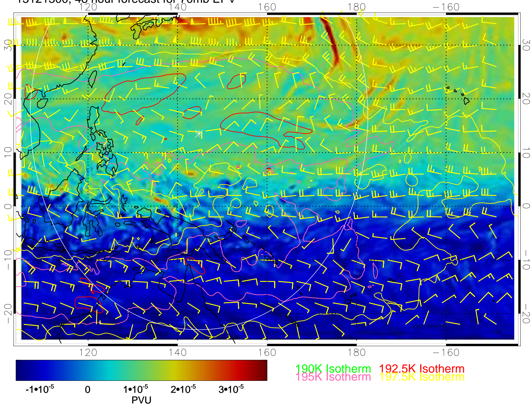
13121300, 48 hour forecast for 70mb EPV
