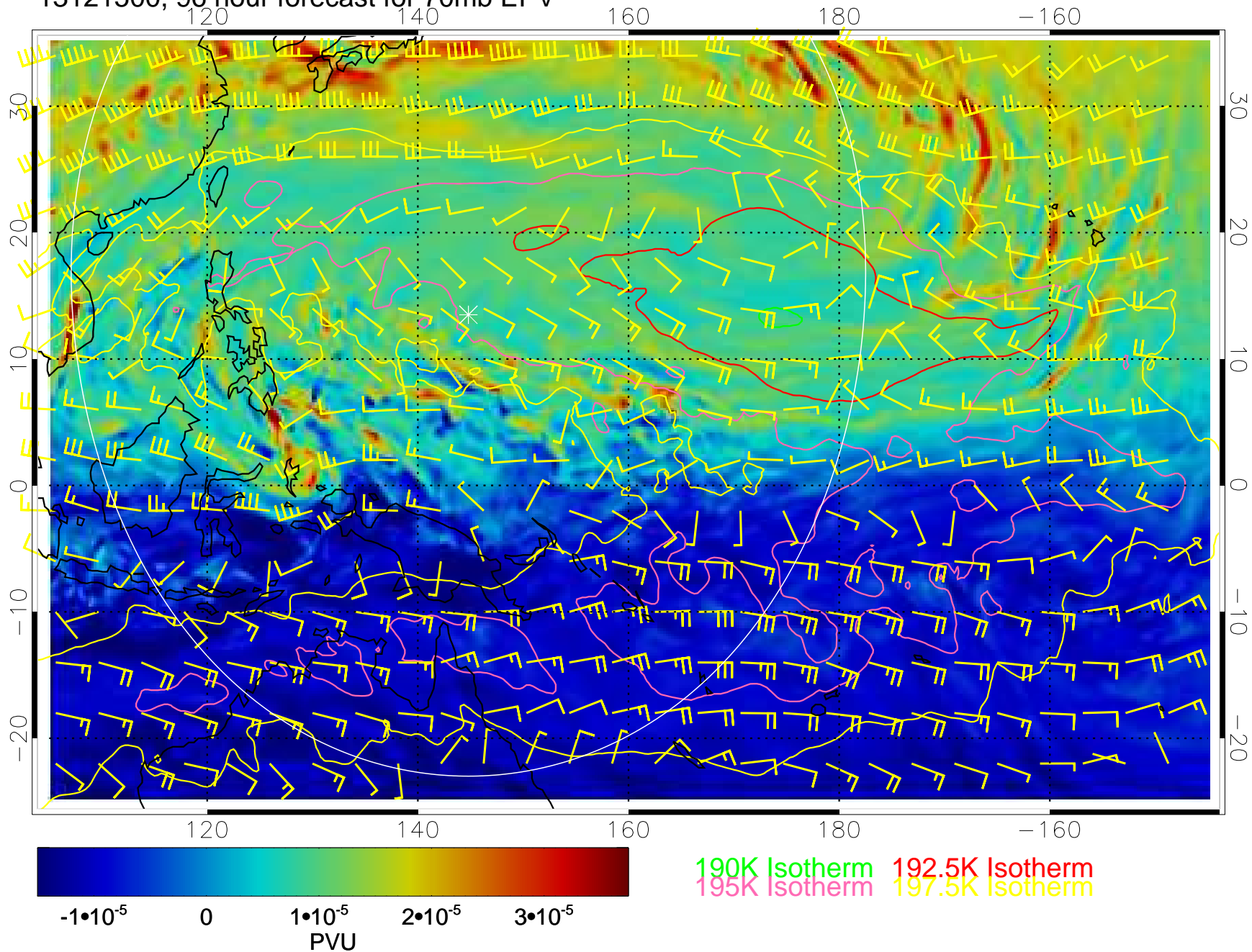
13121500, 96 hour forecast for 70mb EPV
