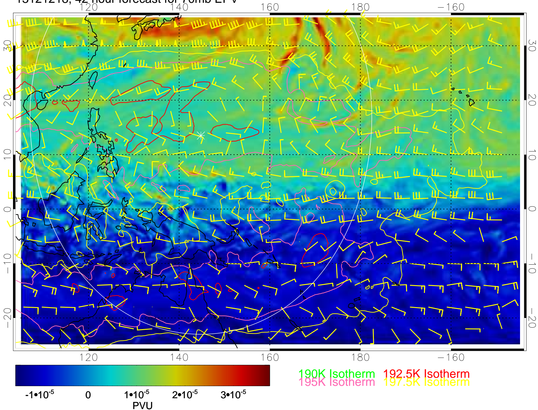
13121218, 42 hour forecast for 70mb EPV
