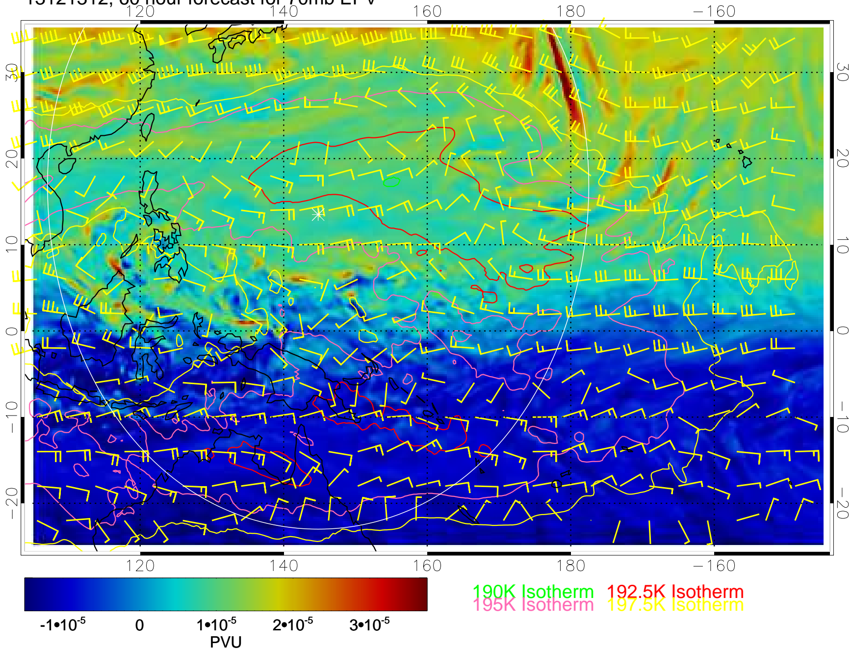
13121312, 60 hour forecast for 70mb EPV
