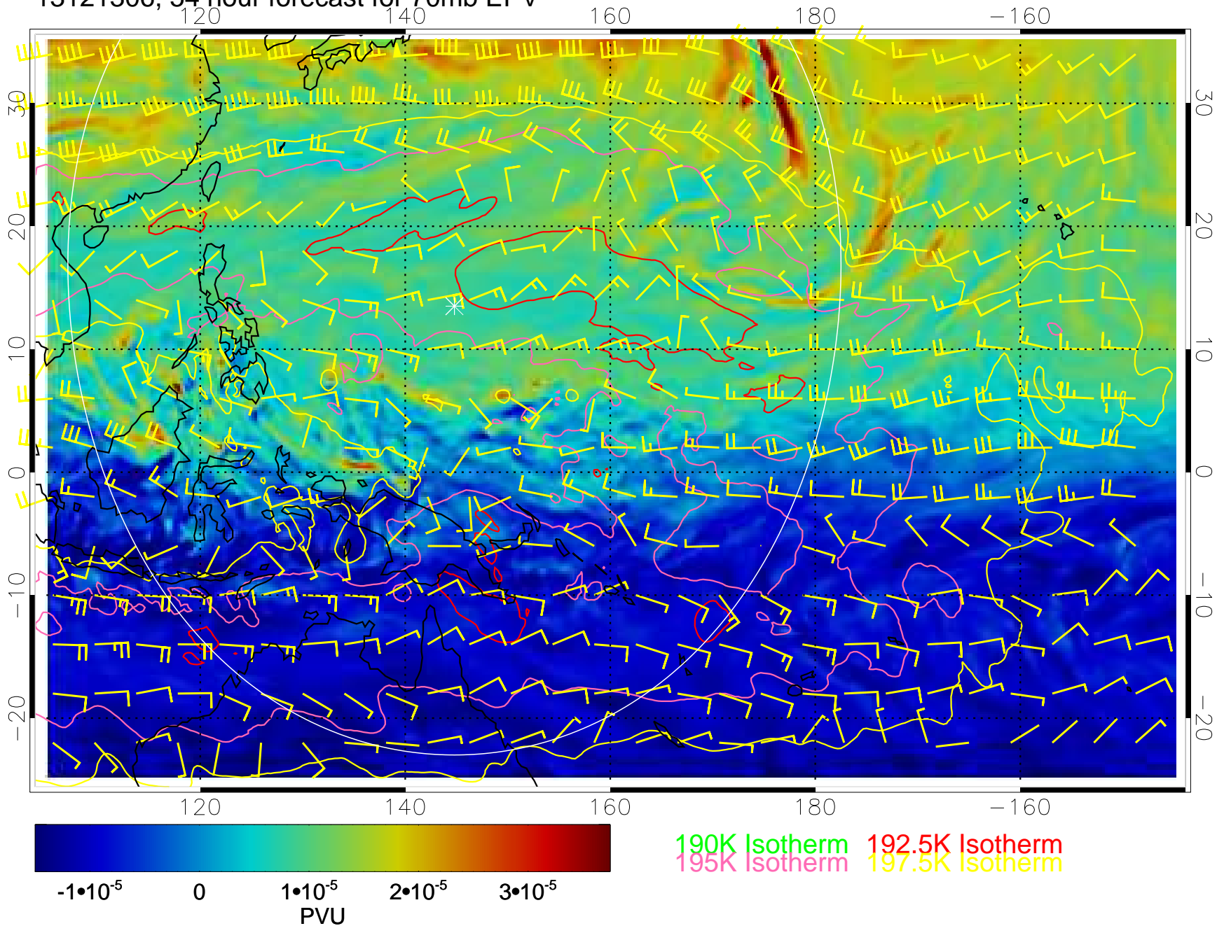
13121306, 54 hour forecast for 70mb EPV
