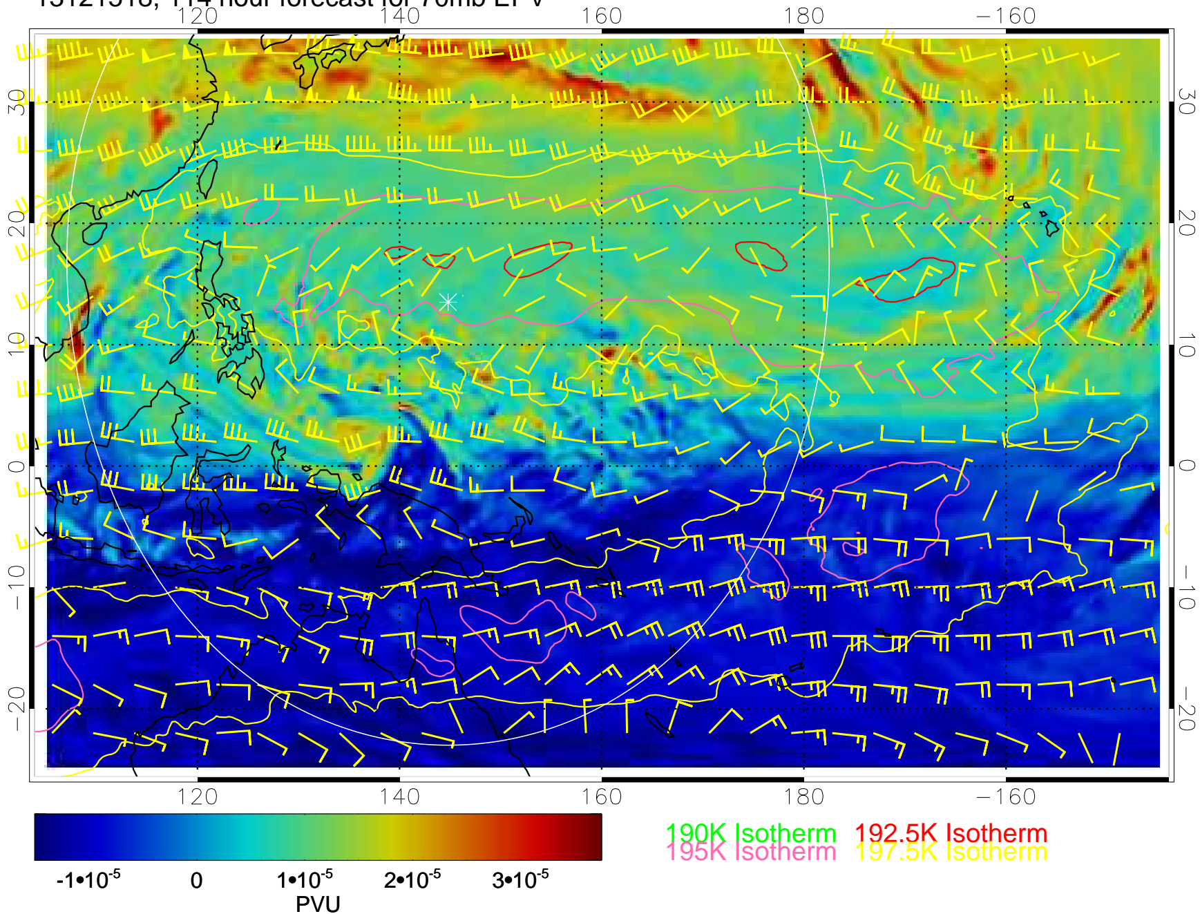
13121518, 114 hour forecast for 70mb EPV
