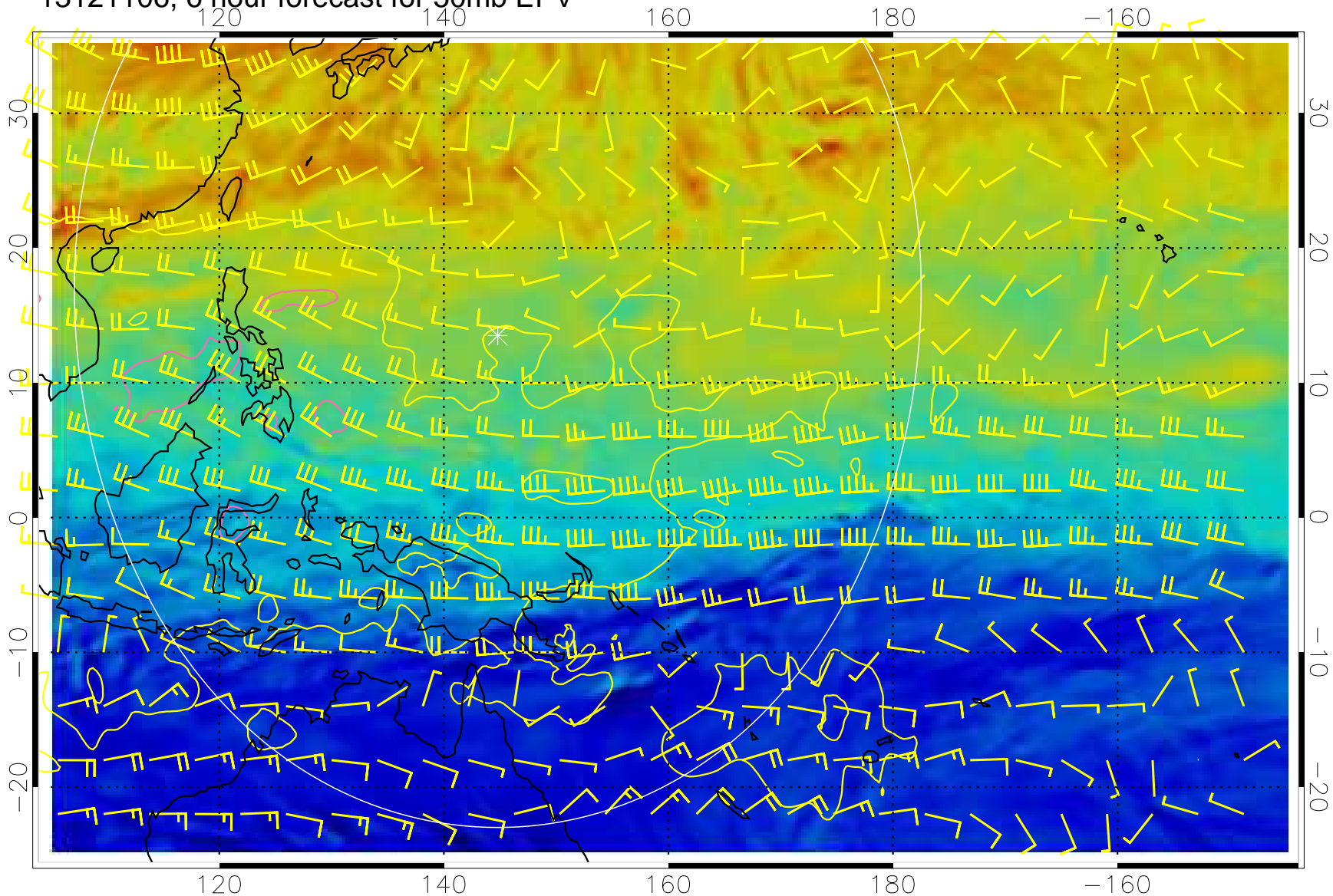
13121106, 6 hour forecast for 50mb EPV
