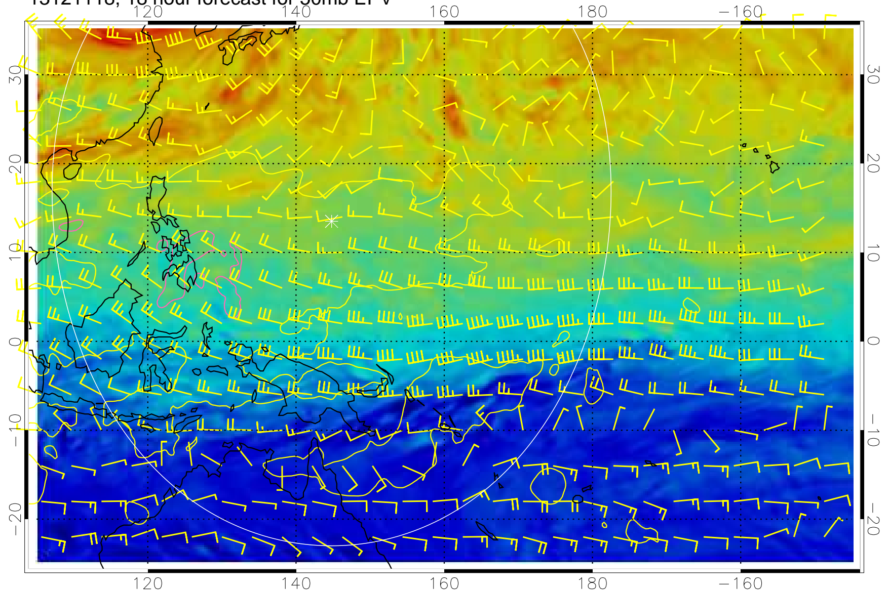
13121118, 18 hour forecast for 50mb EPV
