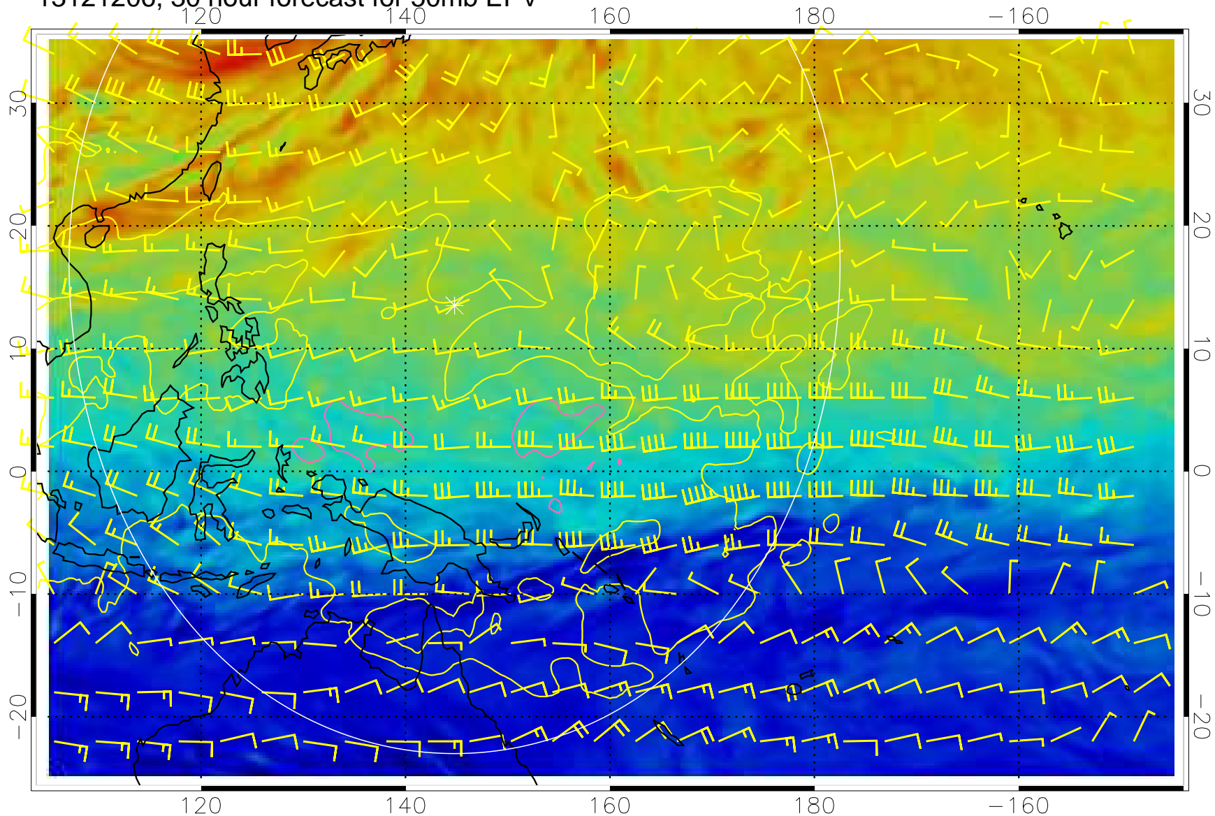
13121206, 30 hour forecast for 50mb EPV
