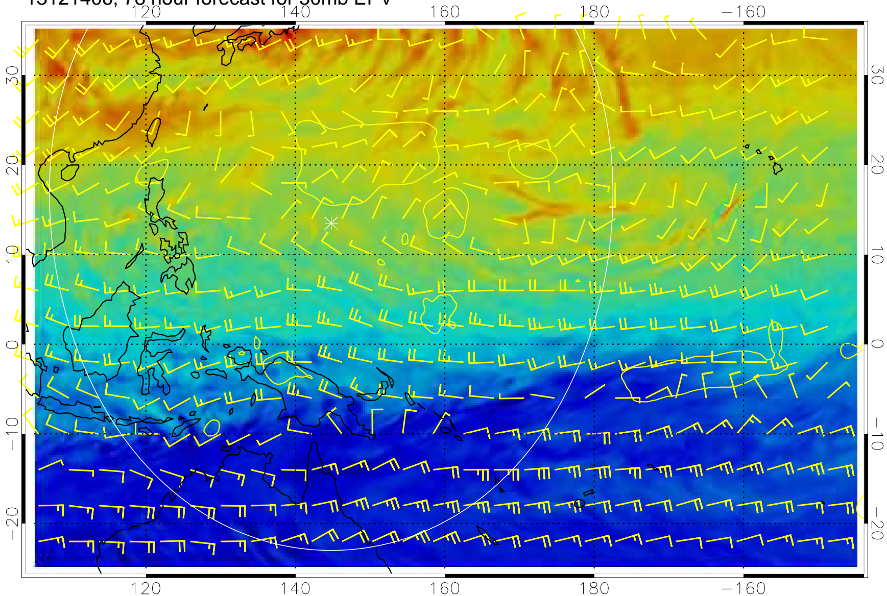
13121406, 78 hour forecast for 50mb EPV
