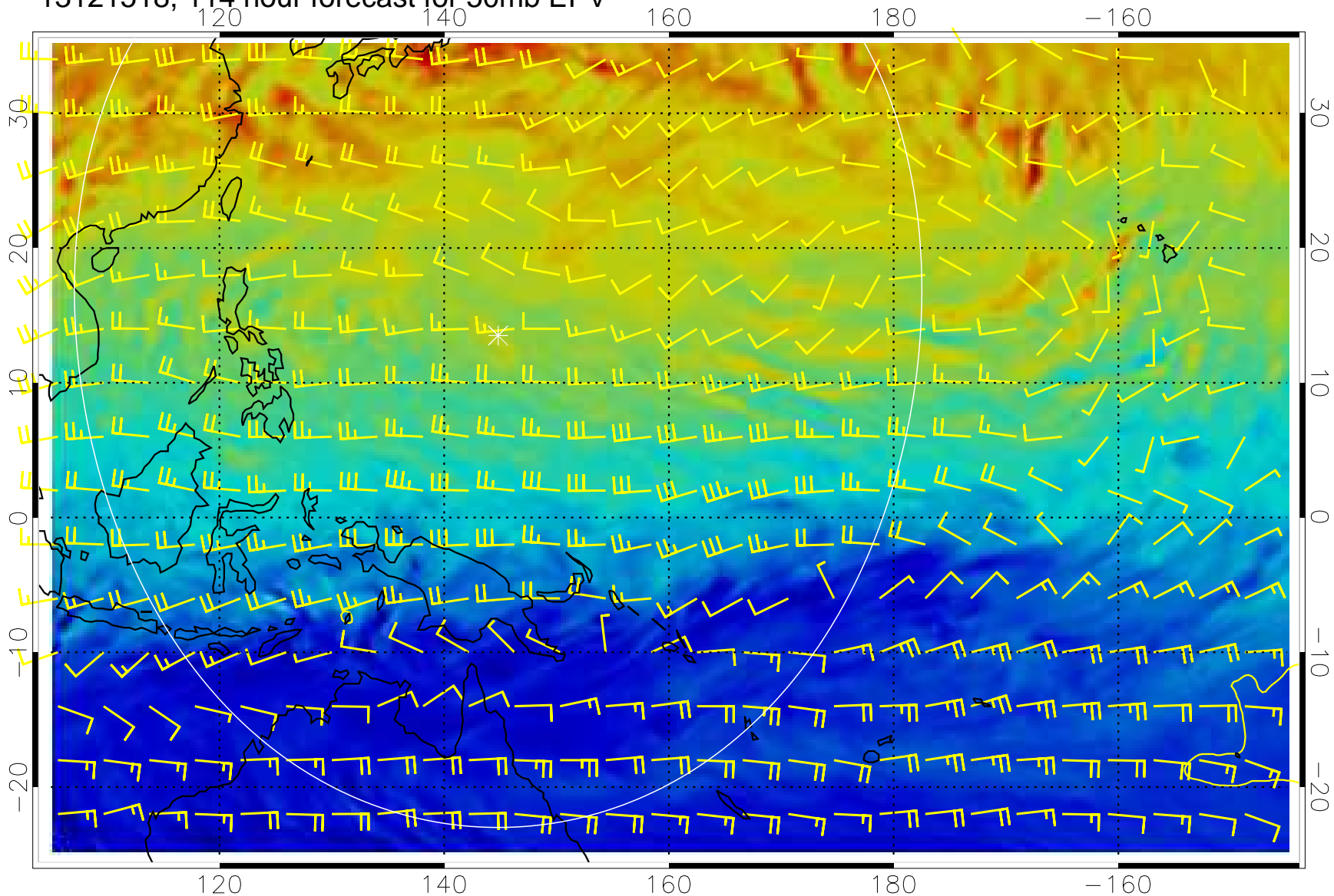
13121518, 114 hour forecast for 50mb EPV
