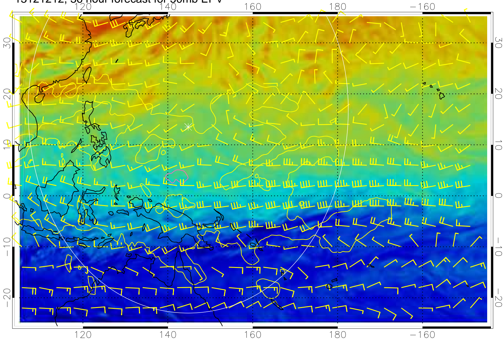
13121212, 36 hour forecast for 50mb EPV
