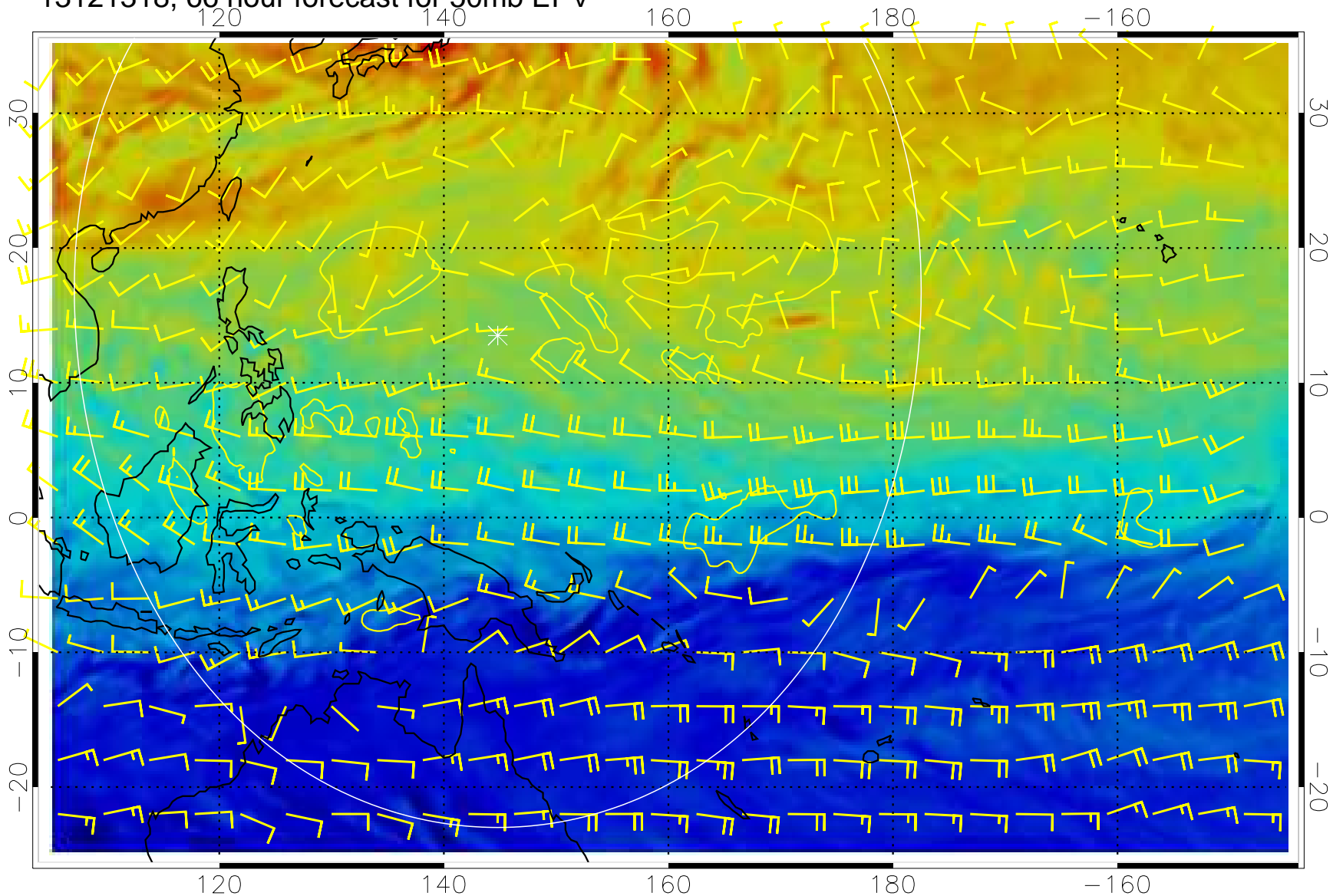
13121318, 66 hour forecast for 50mb EPV
