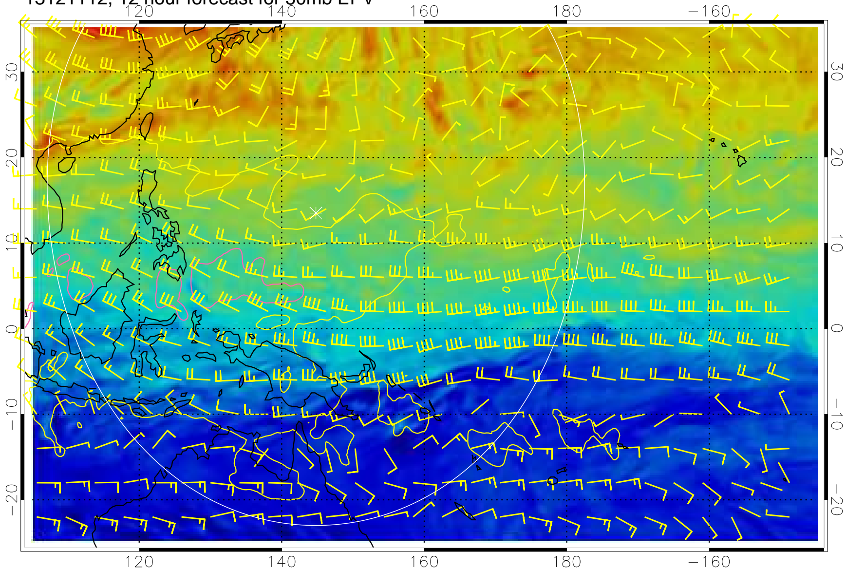
13121112, 12 hour forecast for 50mb EPV
