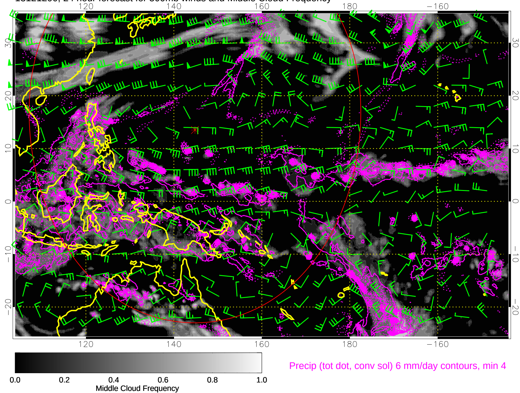
13121200, 24 hour forecast for 500mb winds and Middle Cloud Frequency
