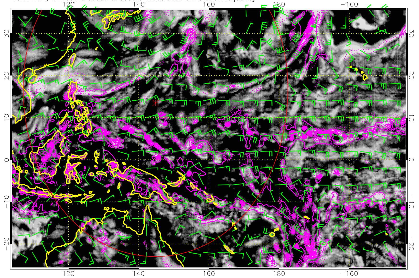
13121112, 12 hour forecast for 850mb winds and Low Cloud Frequency
