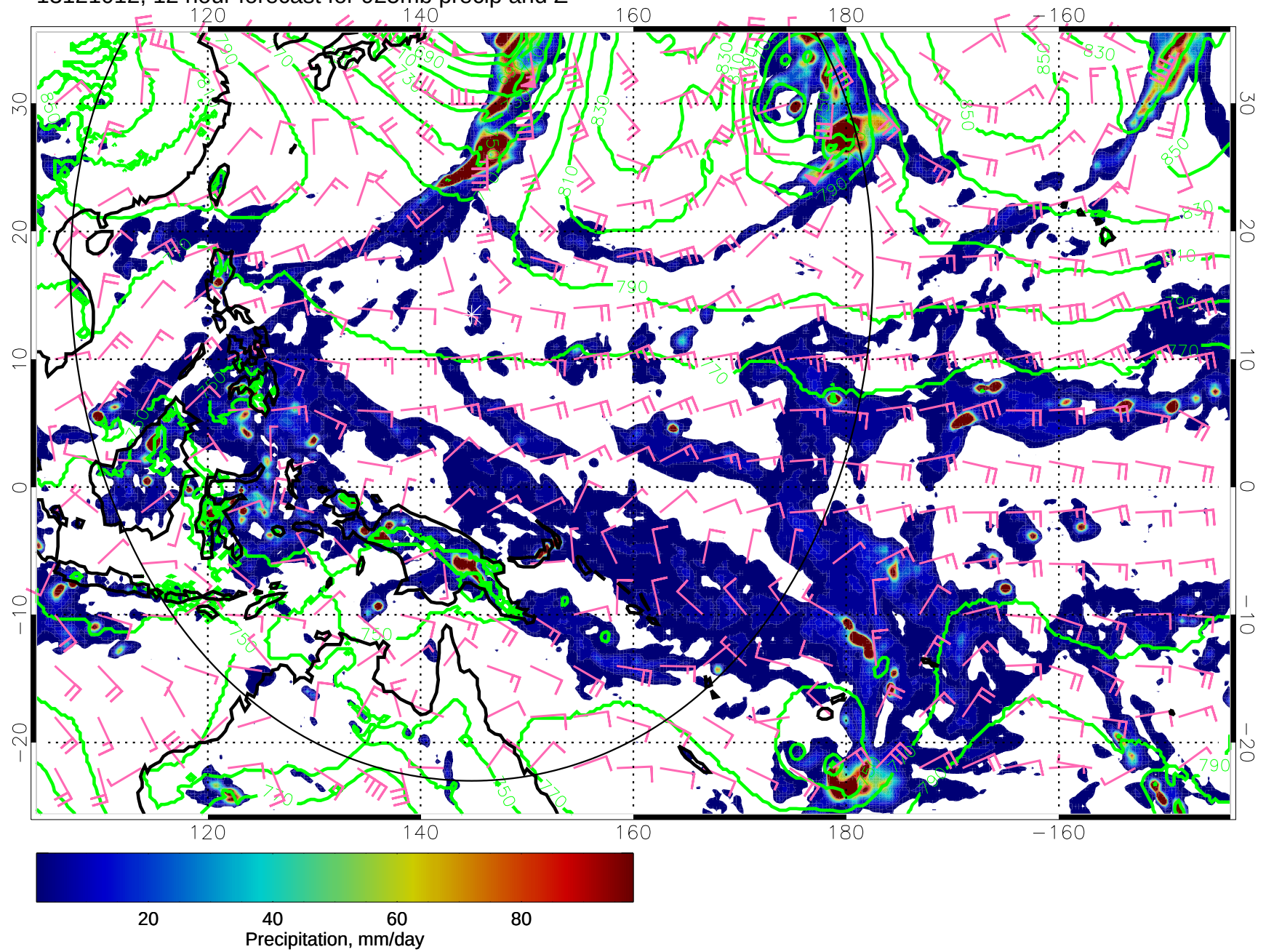
13121012, 12 hour forecast for 925mb precip and Z
