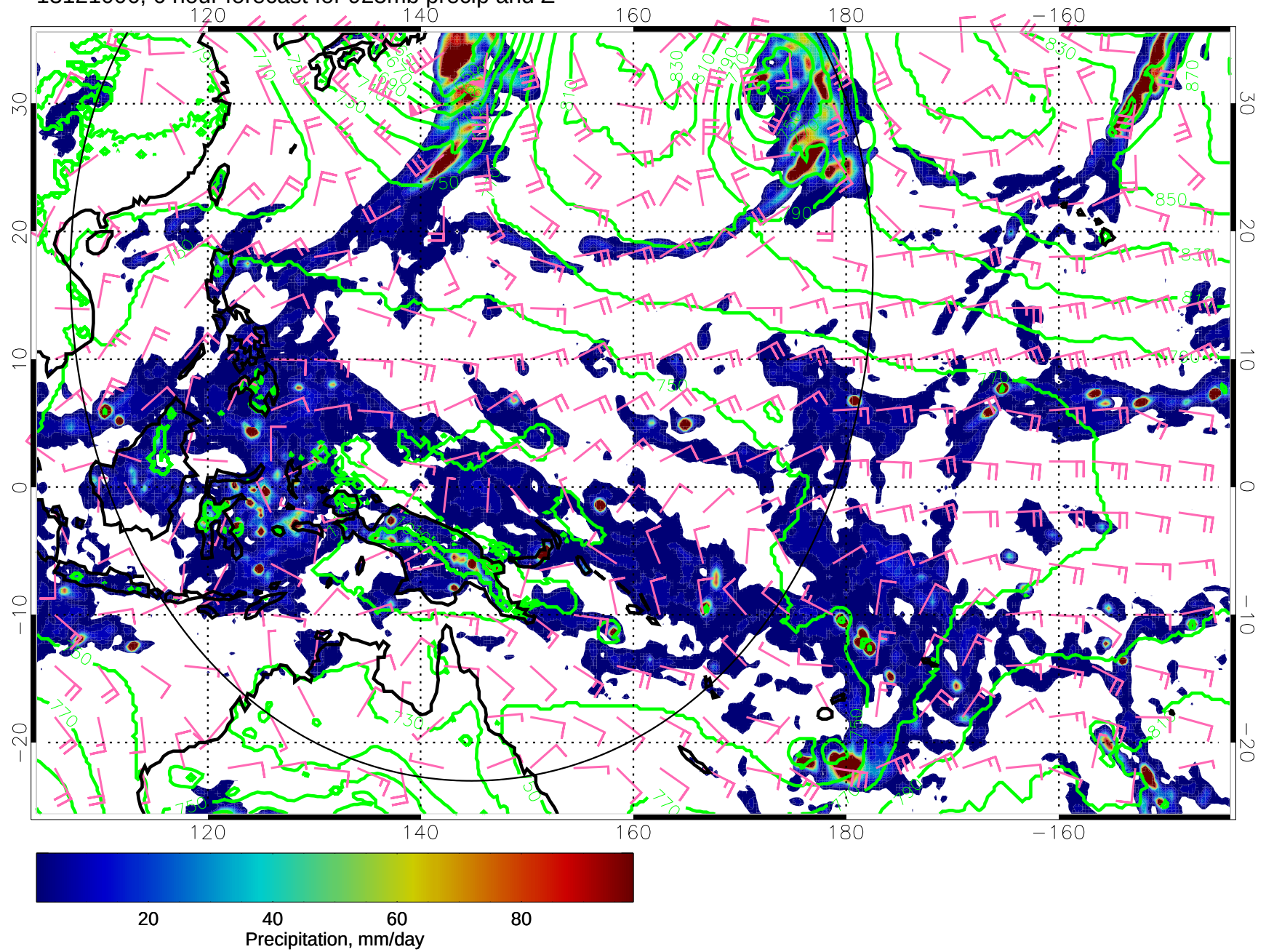
13121006, 6 hour forecast for 925mb precip and Z
