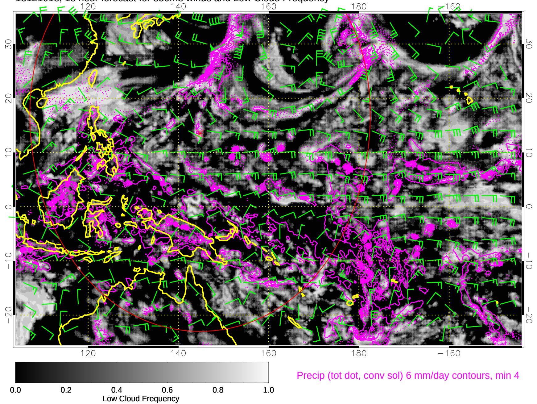
13121018, 18 hour forecast for 850mb winds and Low Cloud Frequency
