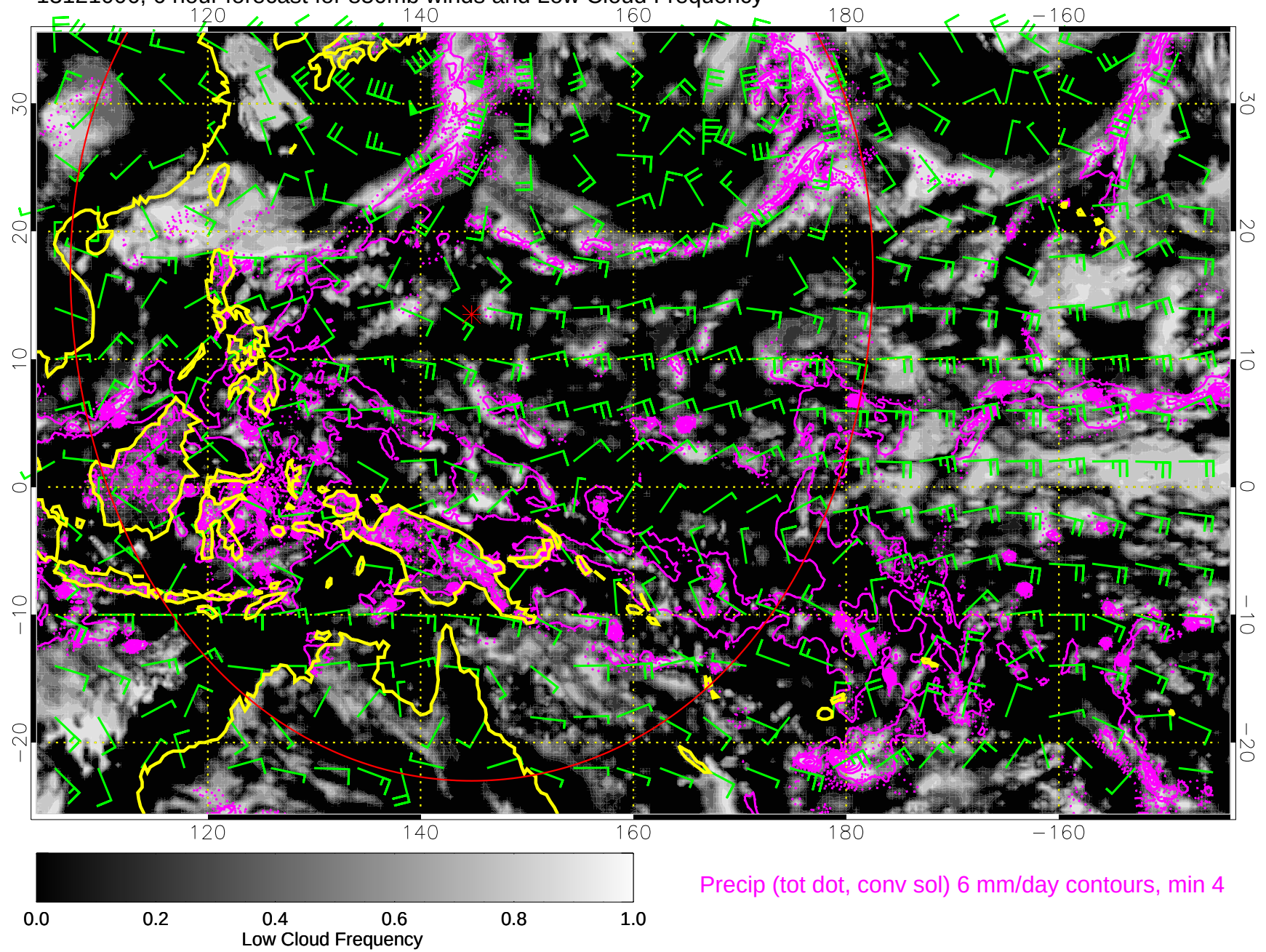
13121006, 6 hour forecast for 850mb winds and Low Cloud Frequency
