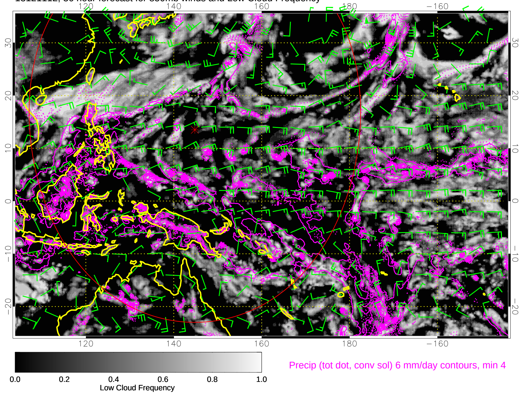
13121112, 36 hour forecast for 850mb winds and Low Cloud Frequency
