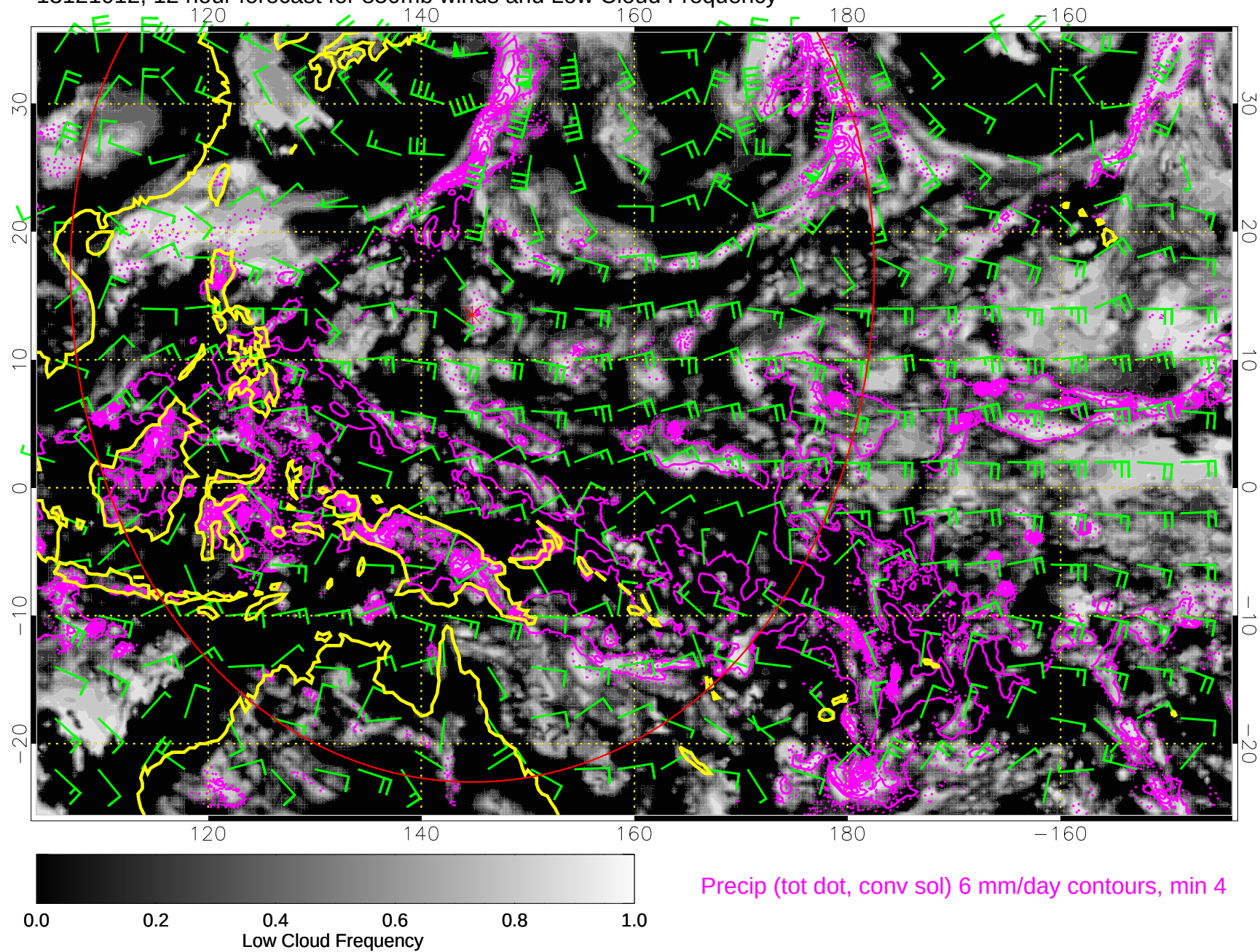
13121012, 12 hour forecast for 850mb winds and Low Cloud Frequency
