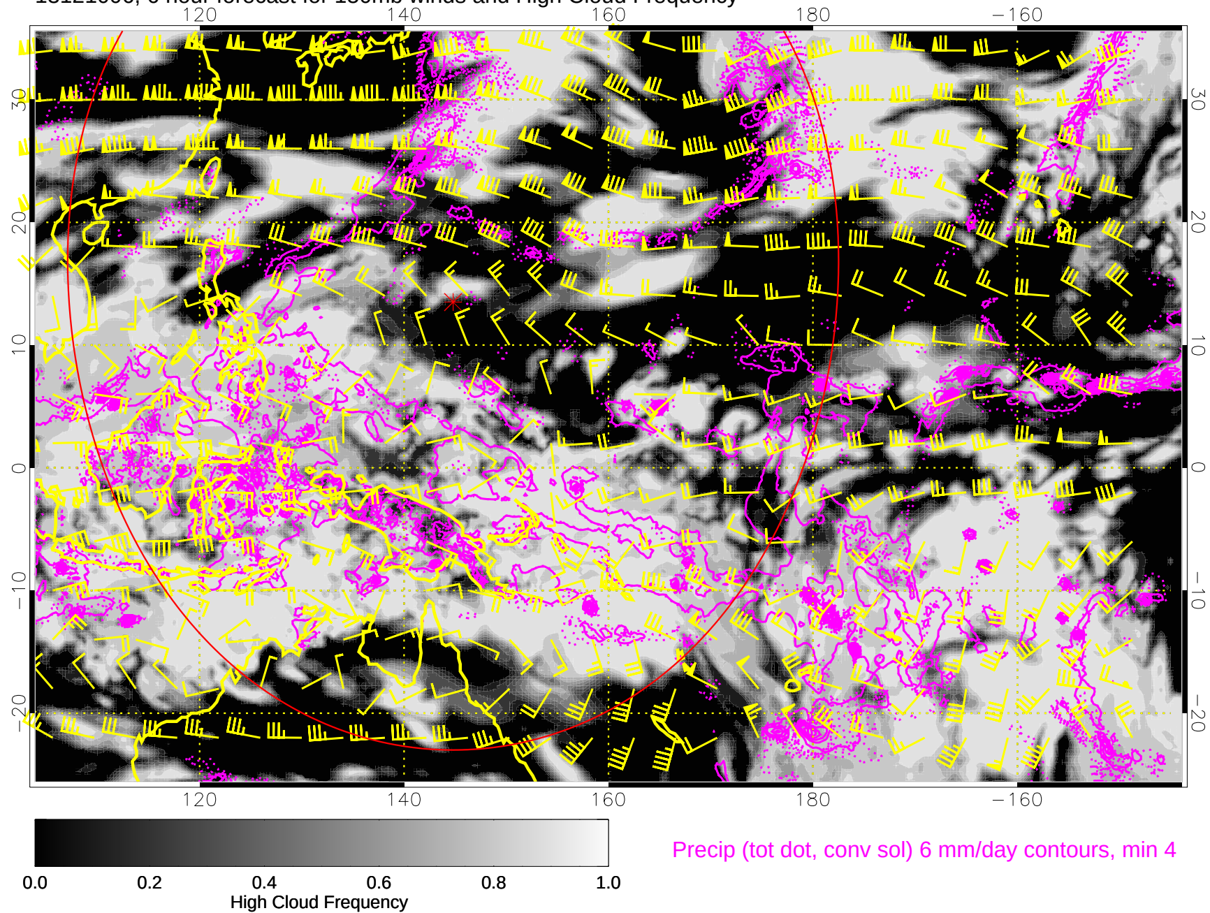
13121006, 6 hour forecast for 150mb winds and High Cloud Frequency
