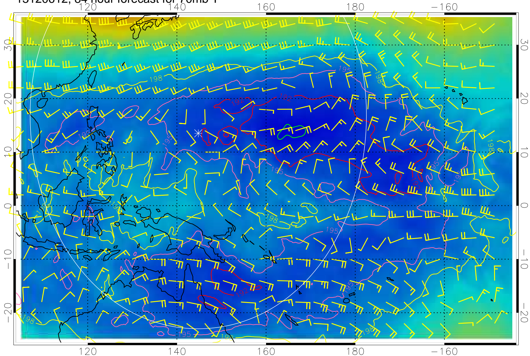
13120612, 84 hour forecast for 70mb T
