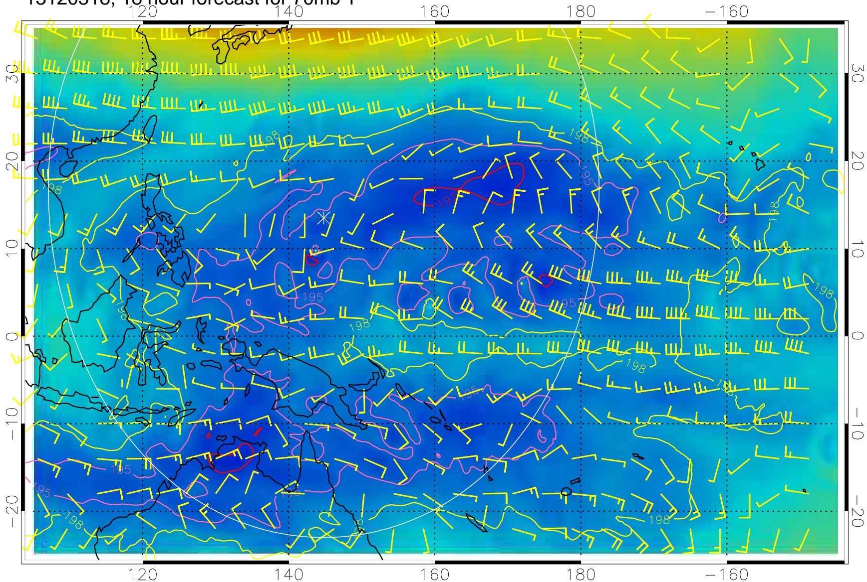
13120318, 18 hour forecast for 70mb T
