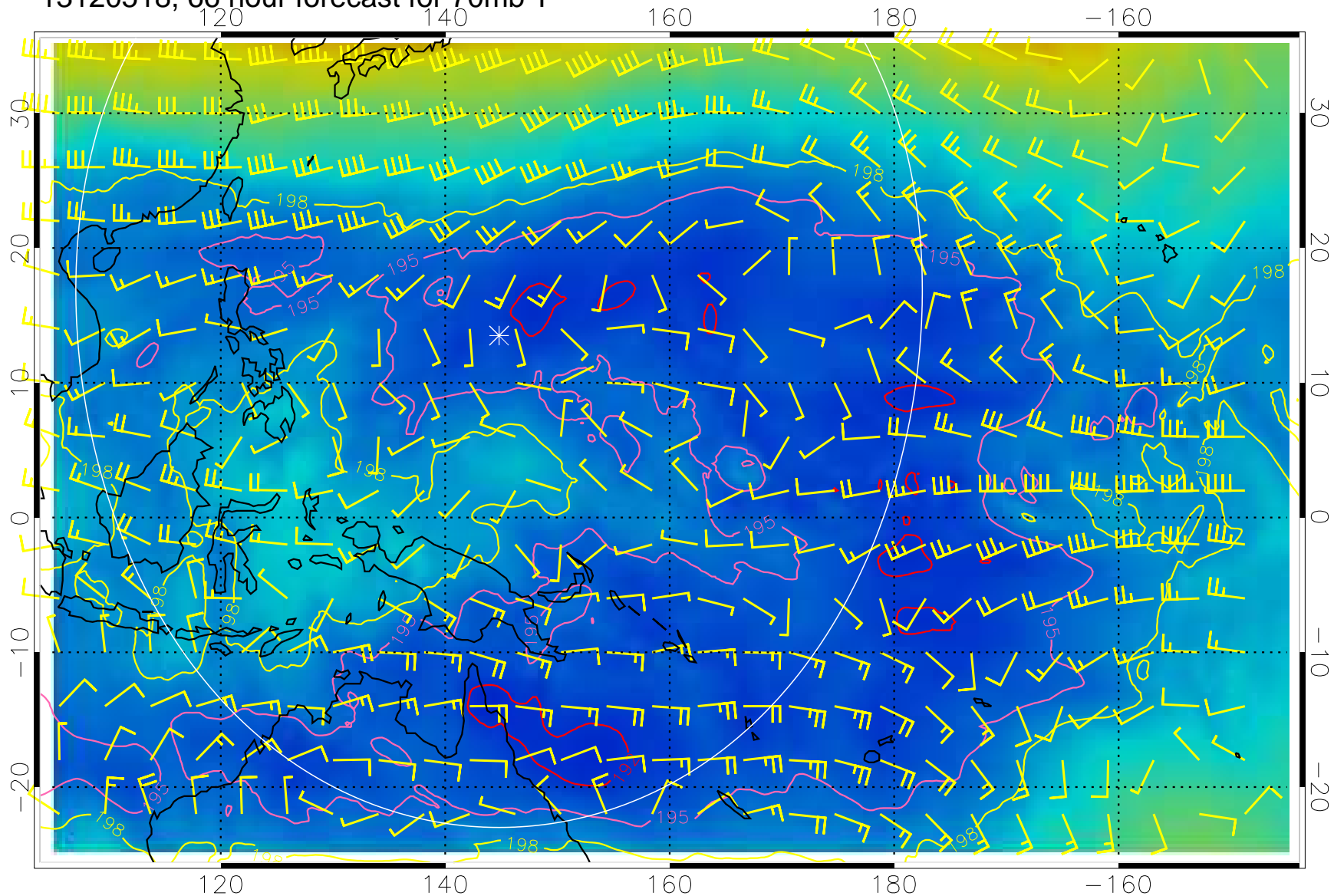
13120518, 66 hour forecast for 70mb T
