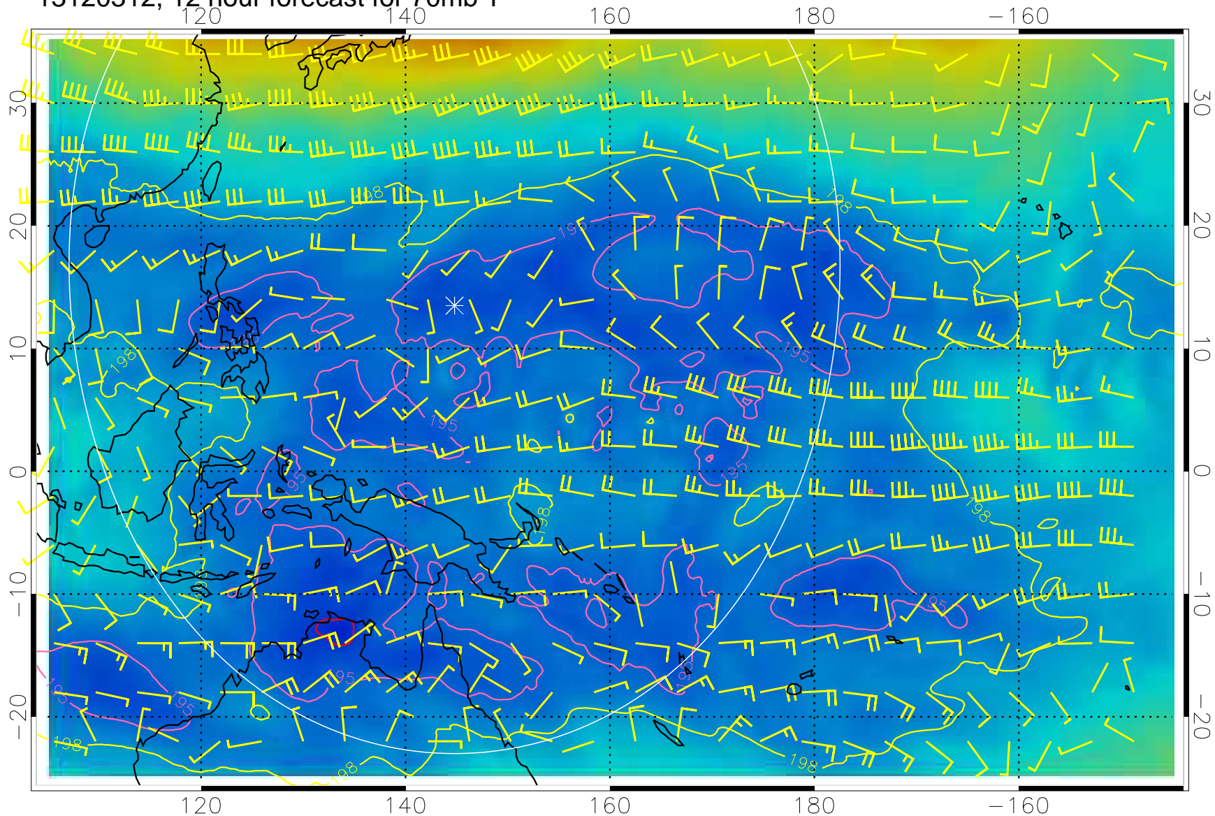
13120312, 12 hour forecast for 70mb T
