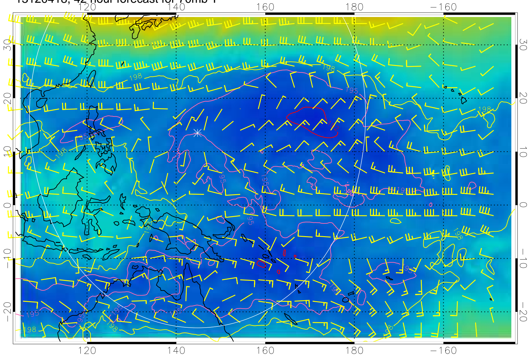
13120418, 42 hour forecast for 70mb T
