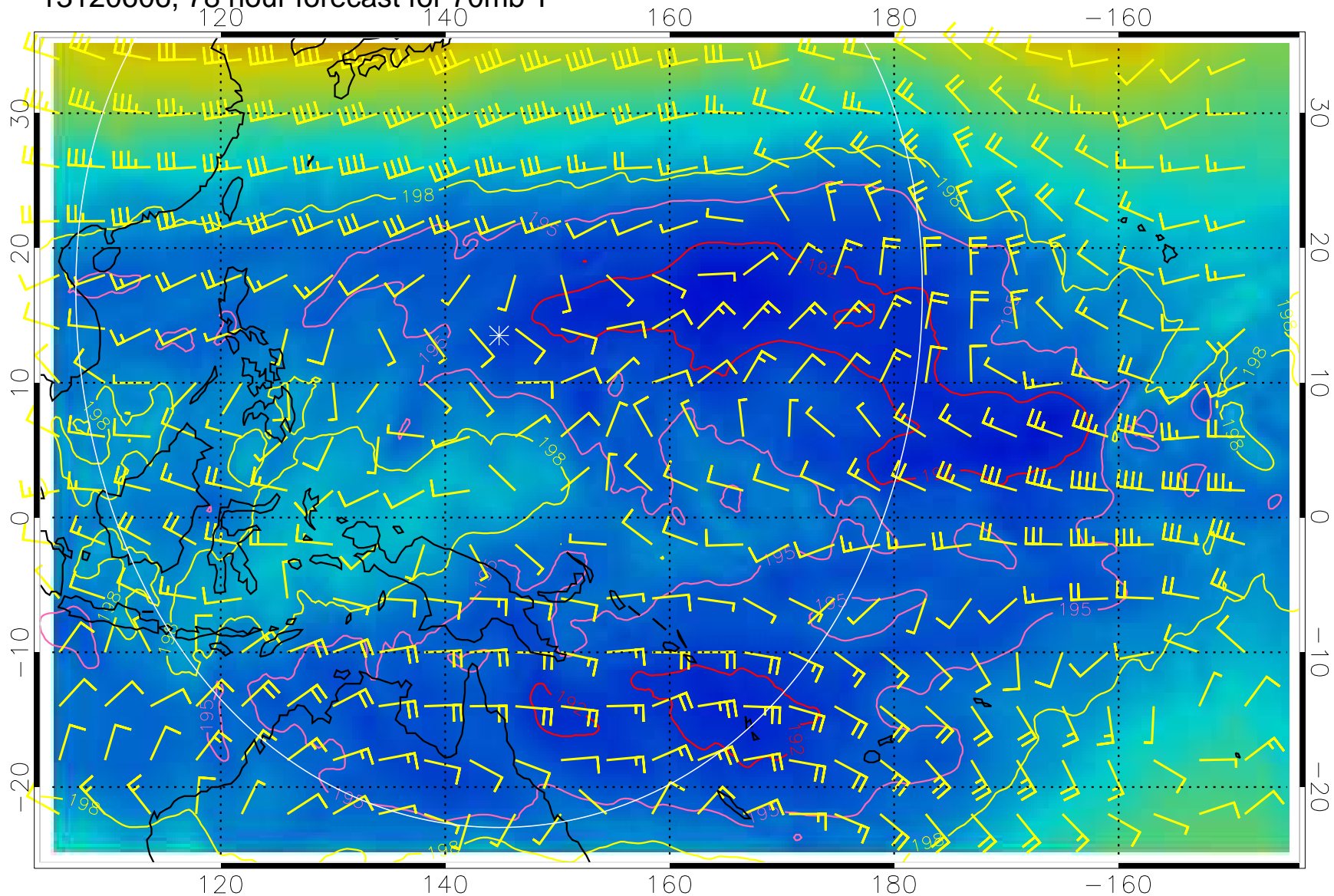
13120606, 78 hour forecast for 70mb T
