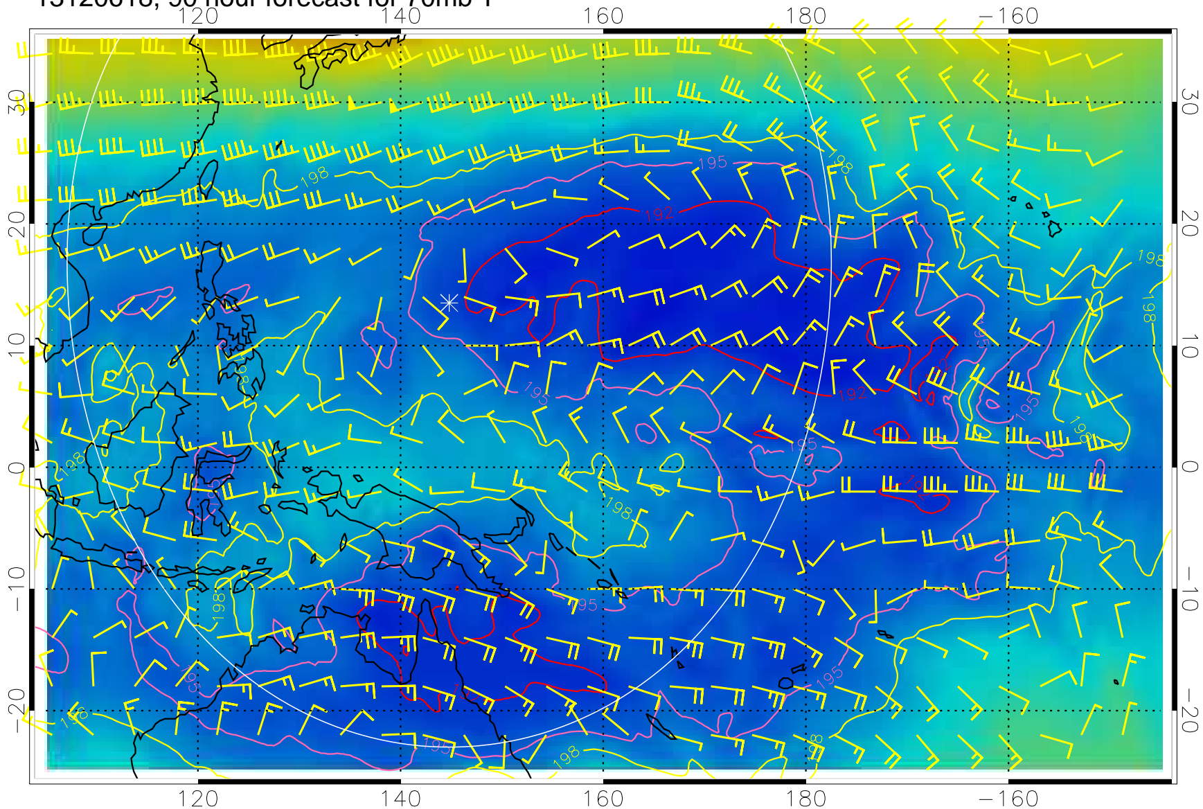
13120618, 90 hour forecast for 70mb T
