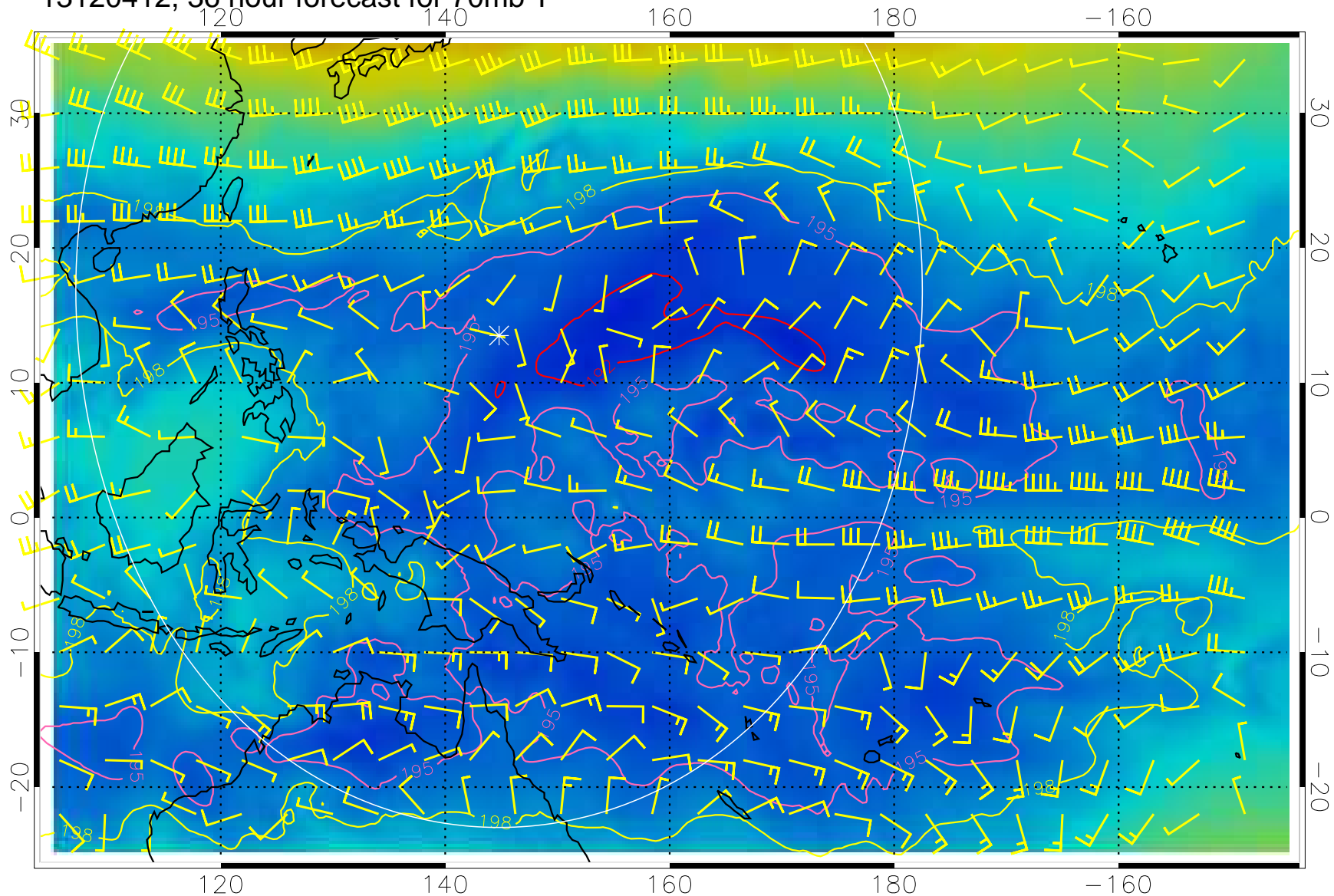
13120412, 36 hour forecast for 70mb T
