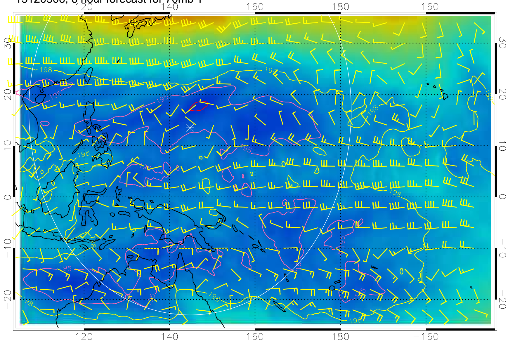
13120306, 6 hour forecast for 70mb T
