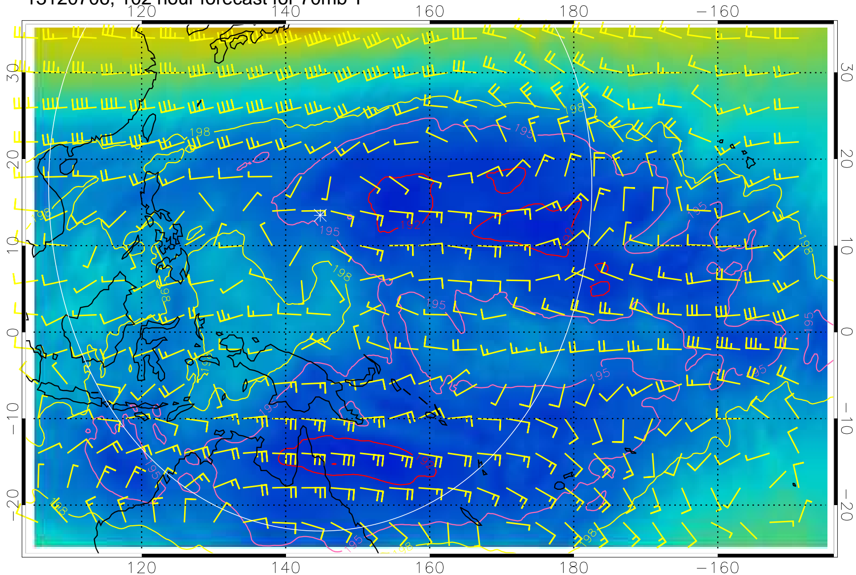
13120706, 102 hour forecast for 70mb T
