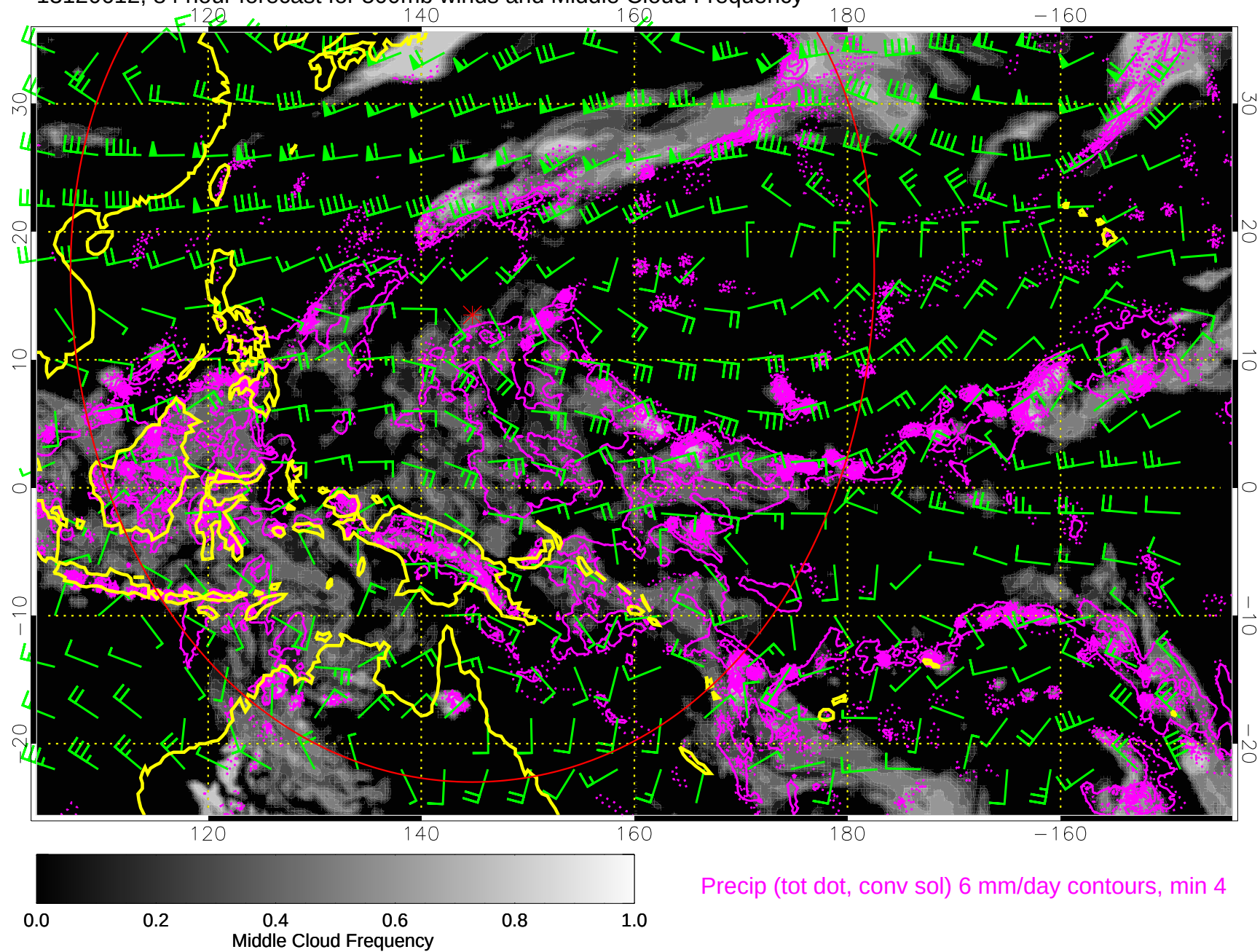
13120612, 84 hour forecast for 500mb winds and Middle Cloud Frequency
