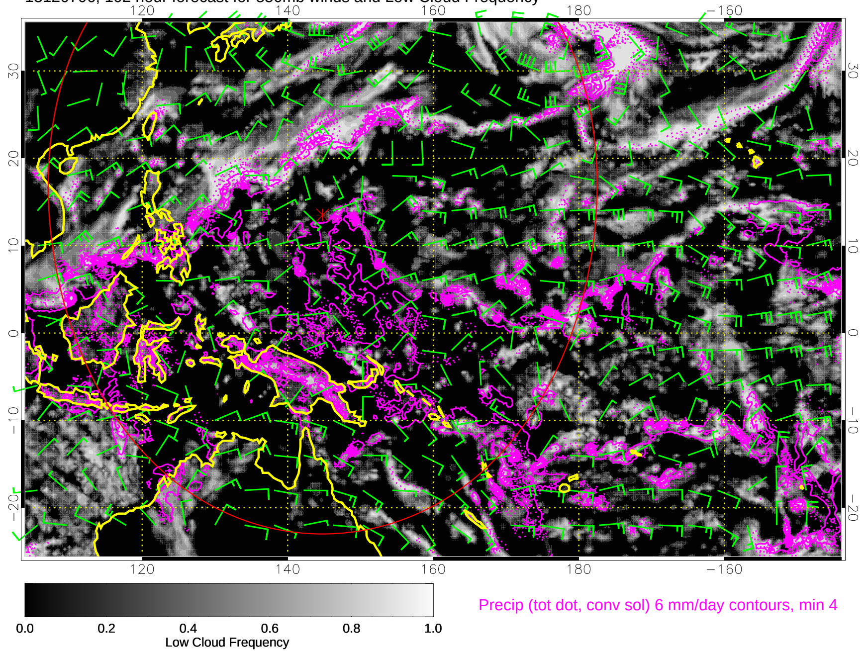
13120706, 102 hour forecast for 850mb winds and Low Cloud Frequency
