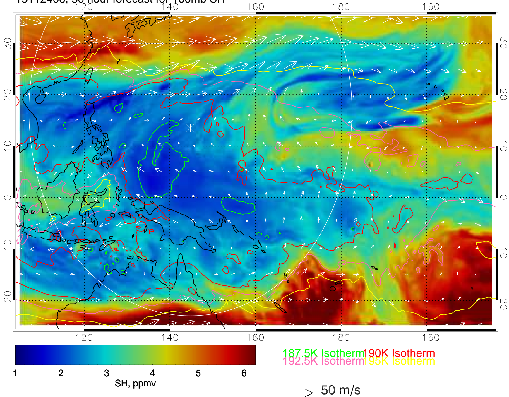
13112406, 30 hour forecast for 100mb SH
