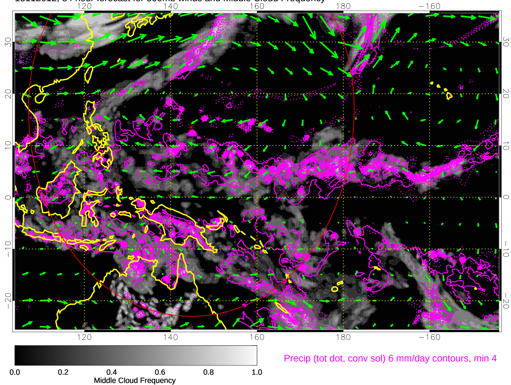
13112612, 84 hour forecast for 500mb winds and Middle Cloud Frequency
