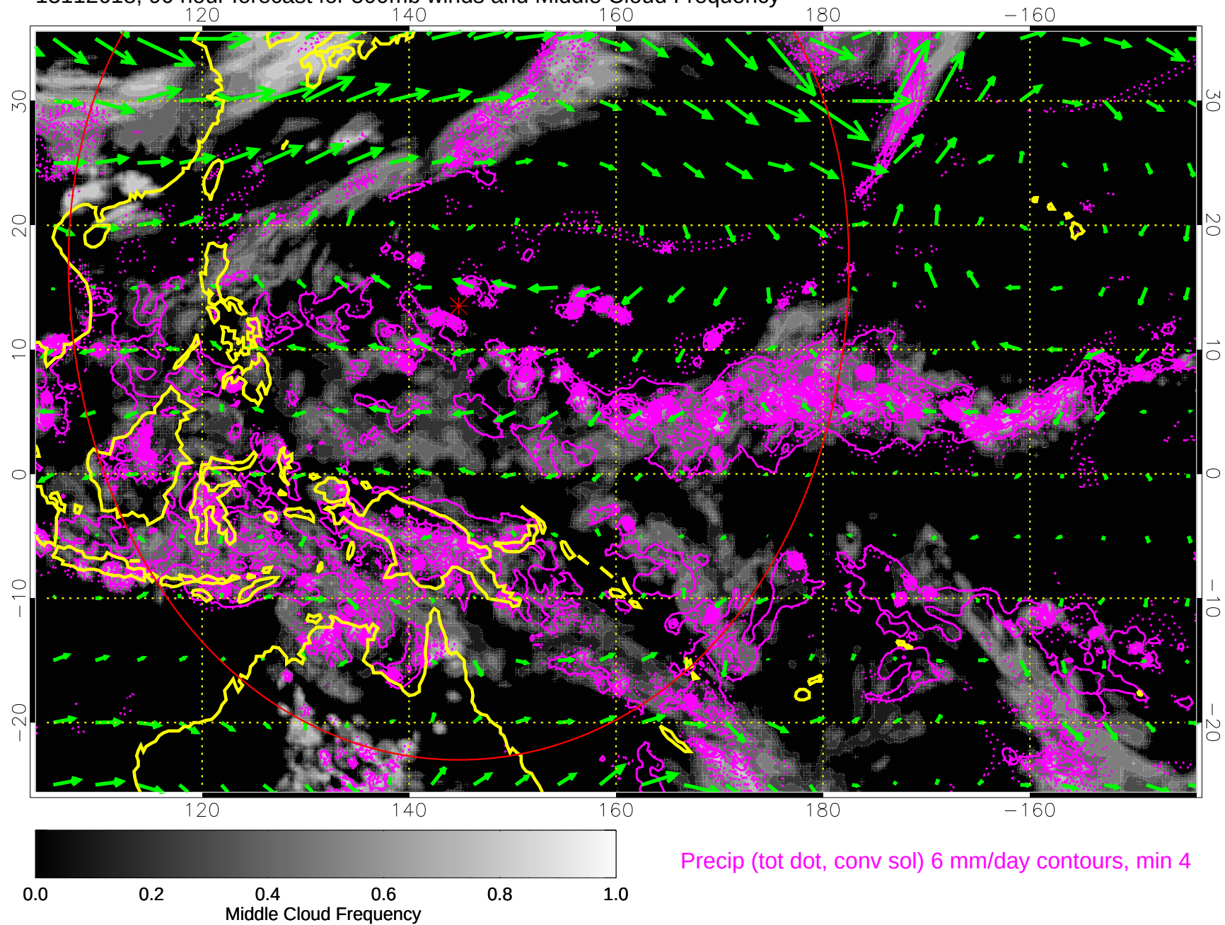
13112618, 90 hour forecast for 500mb winds and Middle Cloud Frequency
