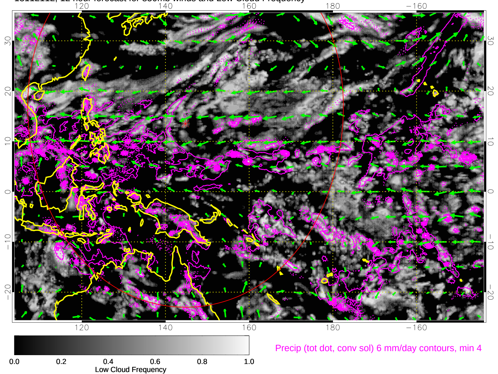
13112112, 12 hour forecast for 850mb winds and Low Cloud Frequency
