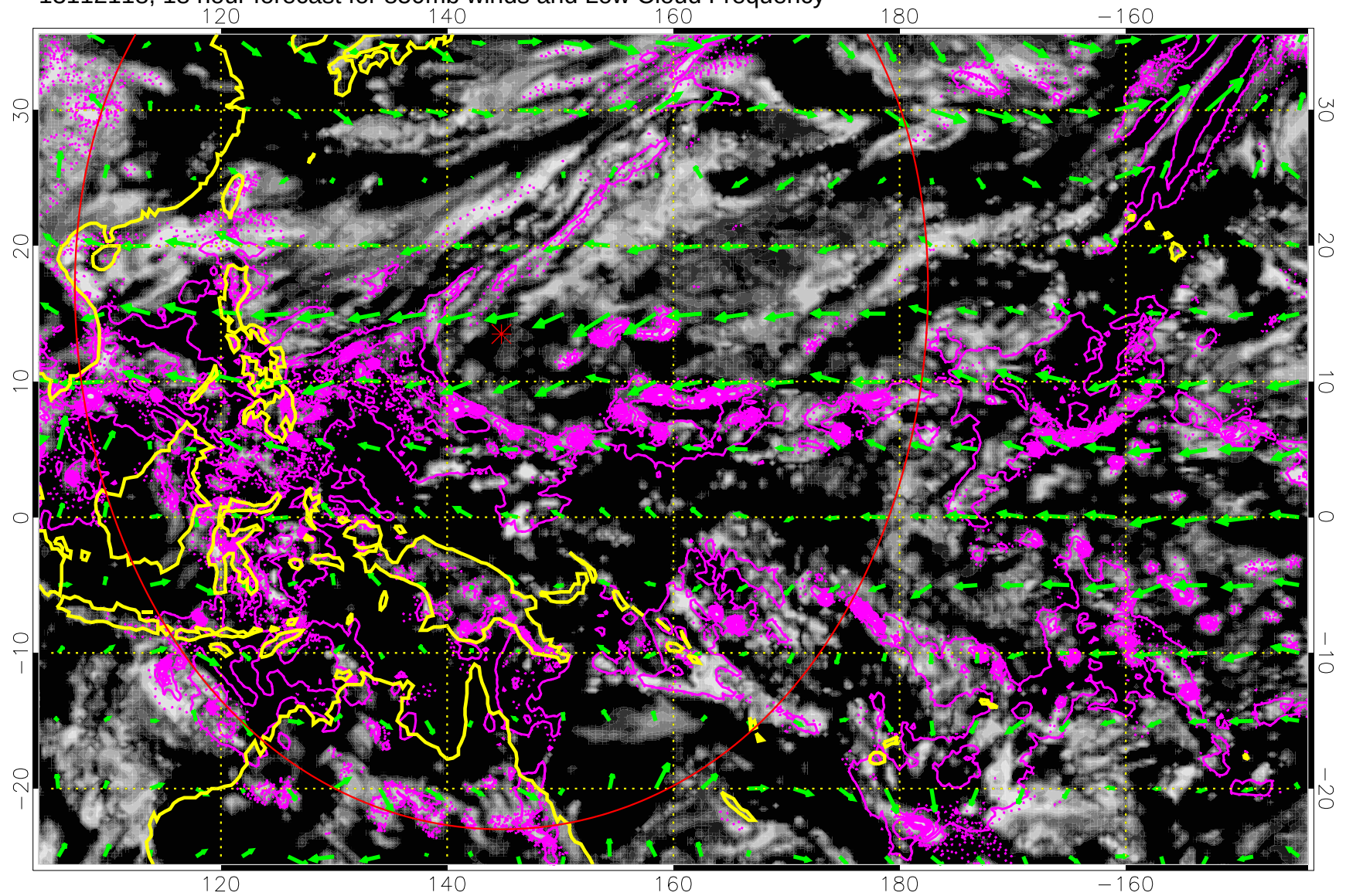
13112118, 18 hour forecast for 850mb winds and Low Cloud Frequency
