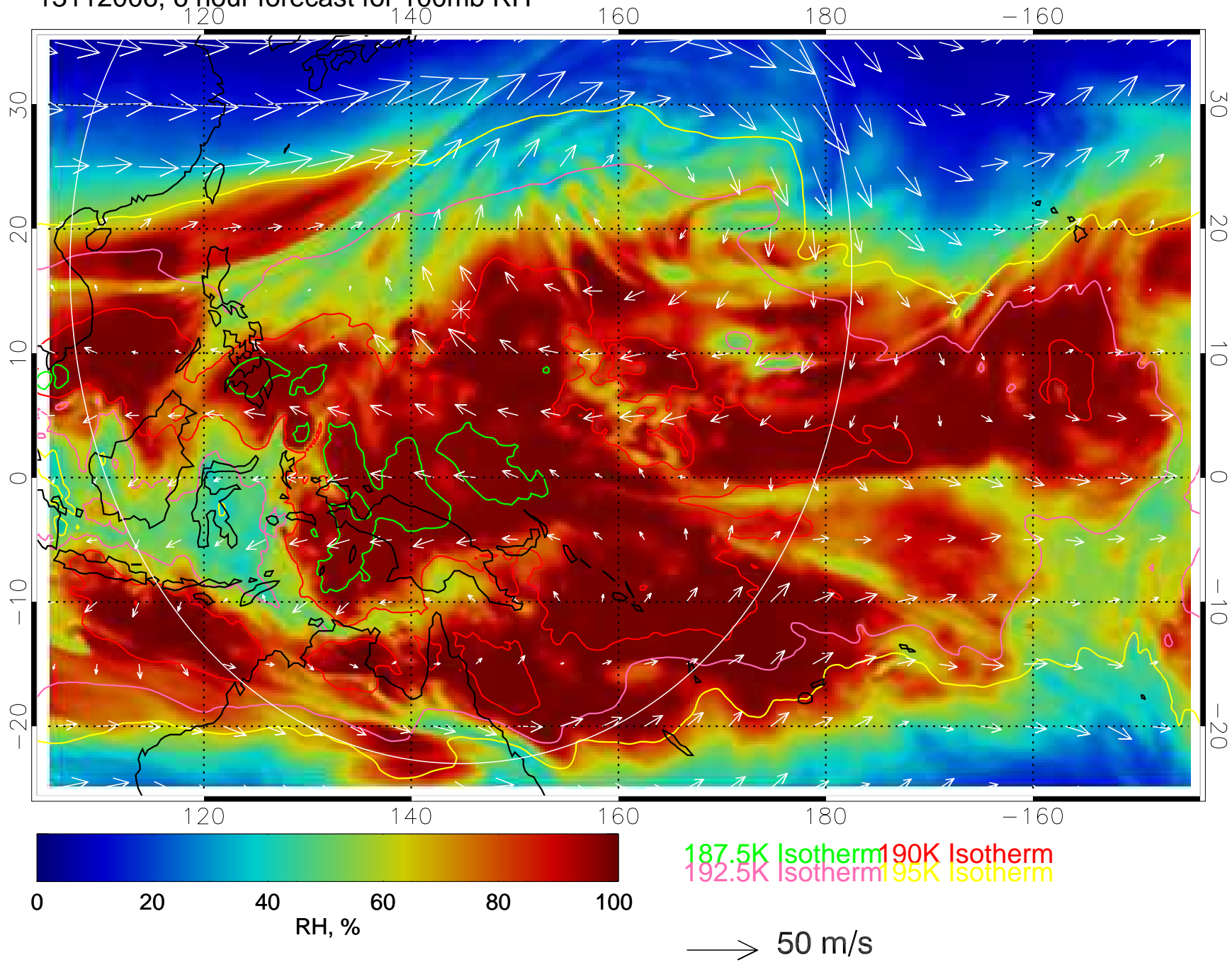
13112006, 6 hour forecast for 100mb RH
