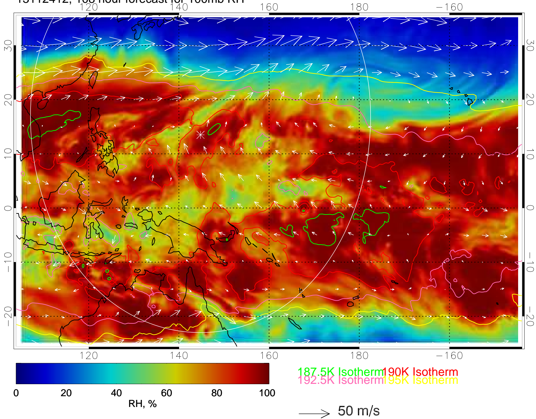
13112412, 108 hour forecast for 100mb RH
