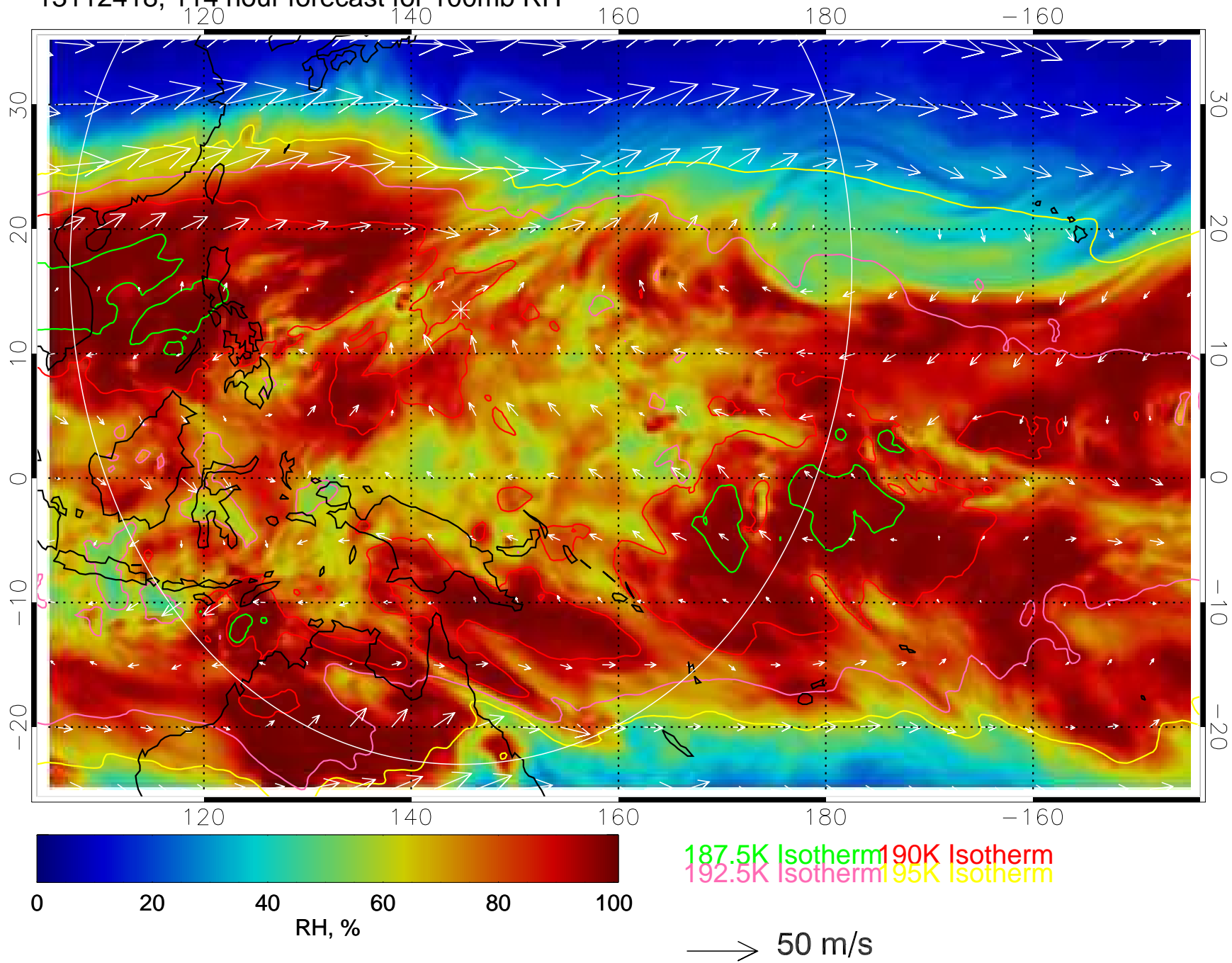
13112418, 114 hour forecast for 100mb RH
