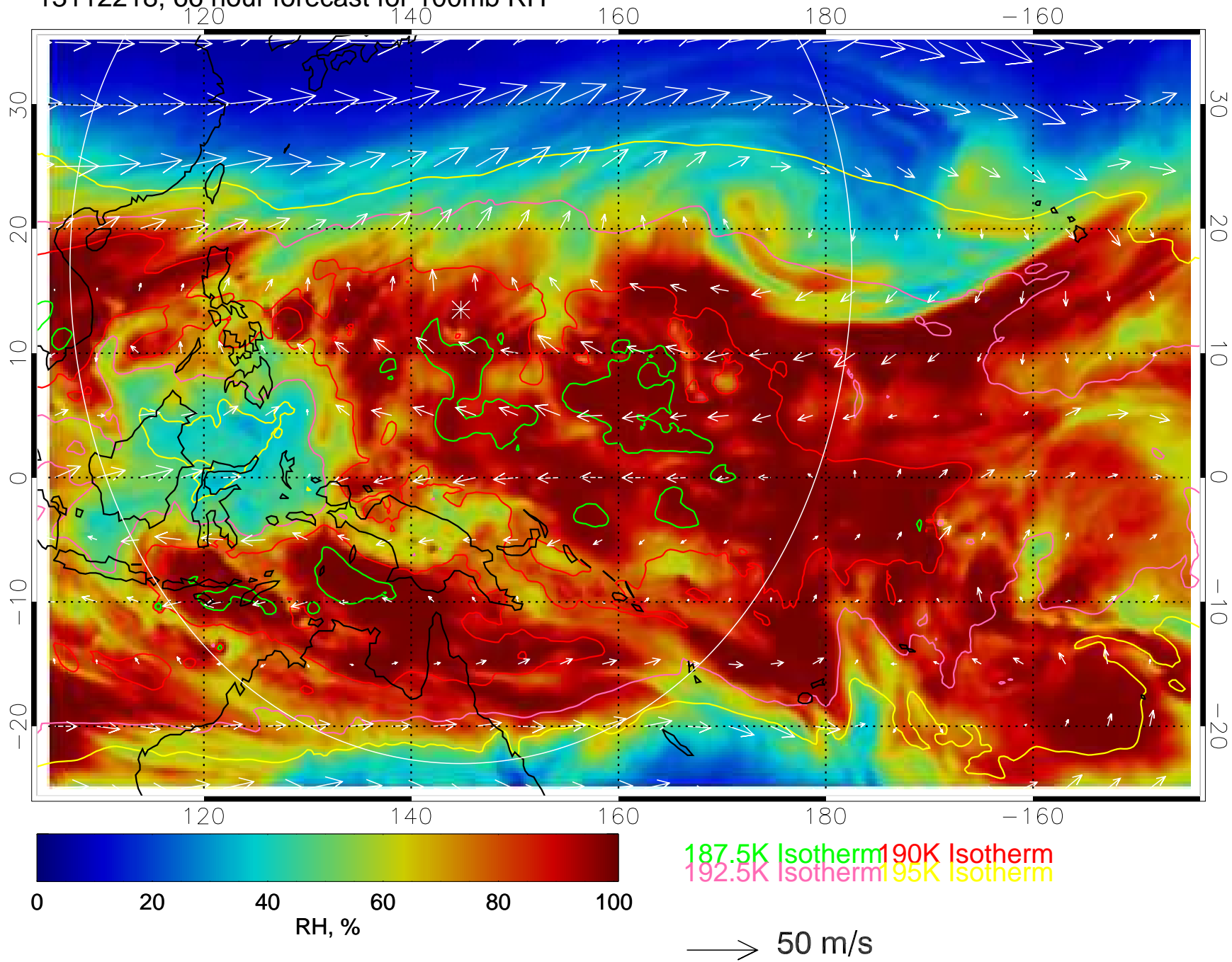
13112218, 66 hour forecast for 100mb RH
