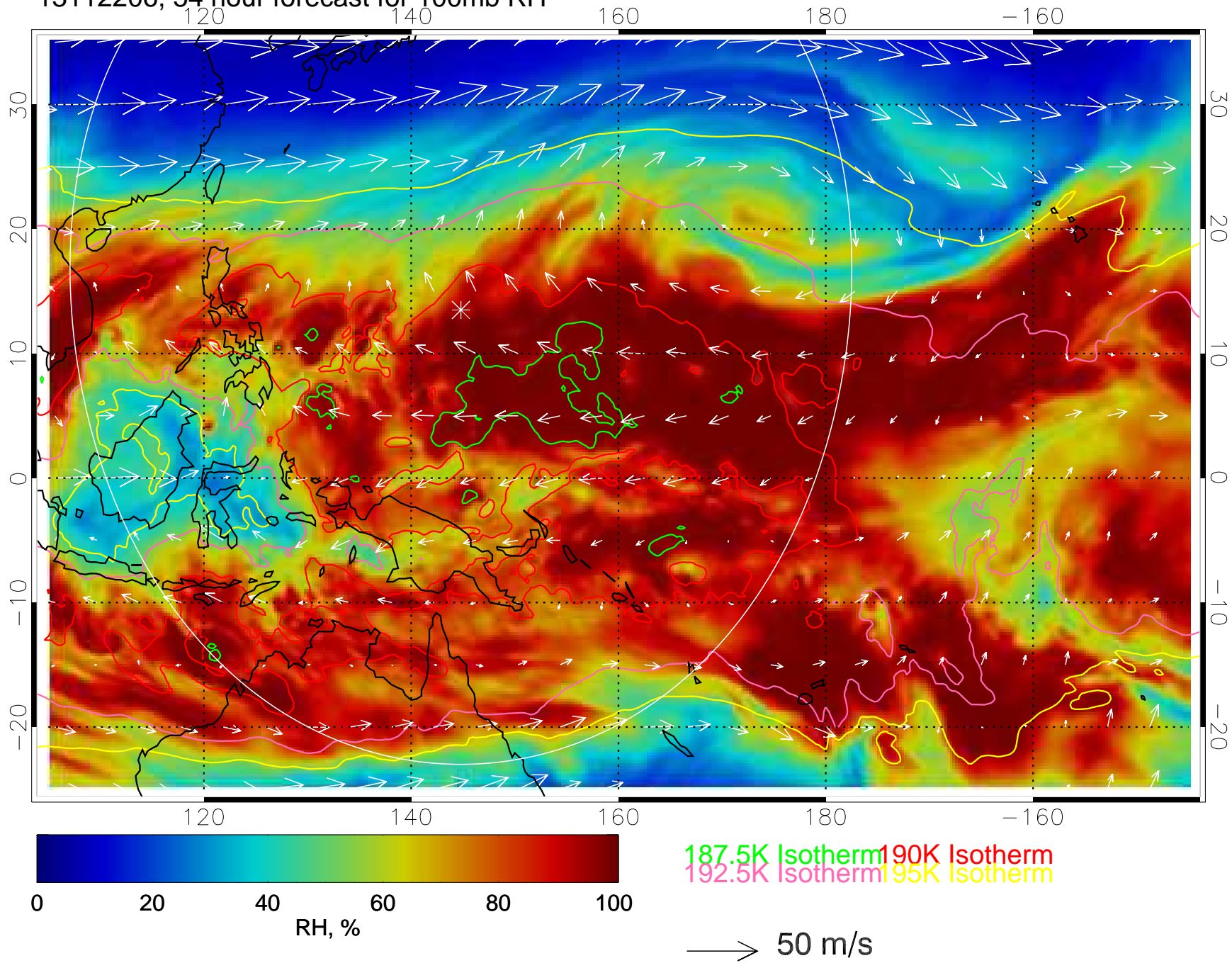
13112206, 54 hour forecast for 100mb RH
