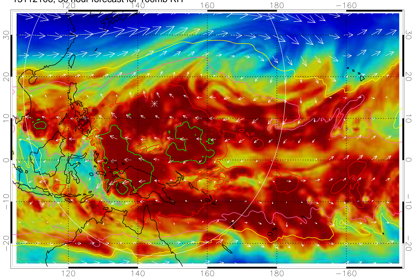
13112106, 30 hour forecast for 100mb RH
