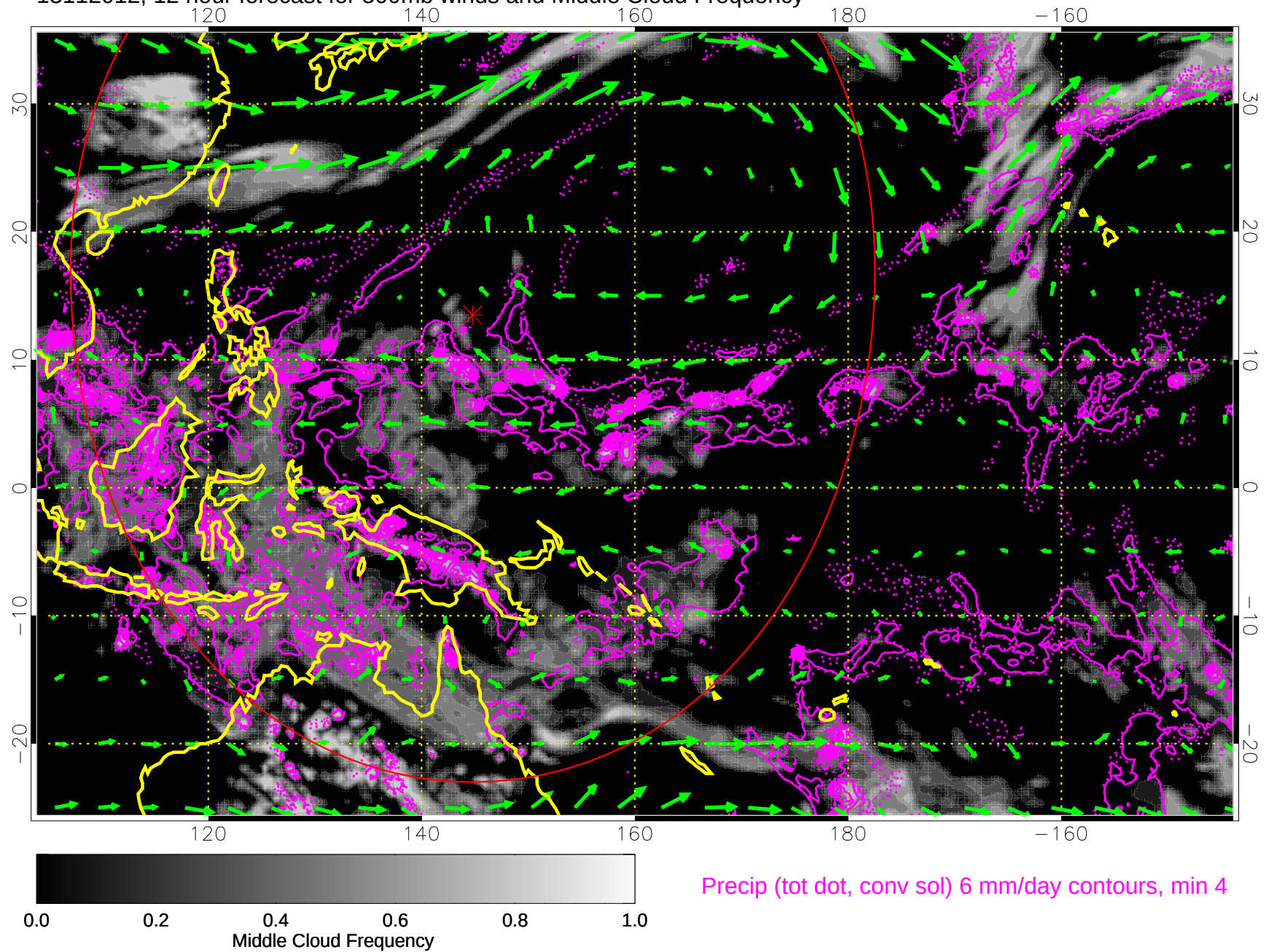
13112012, 12 hour forecast for 500mb winds and Middle Cloud Frequency
