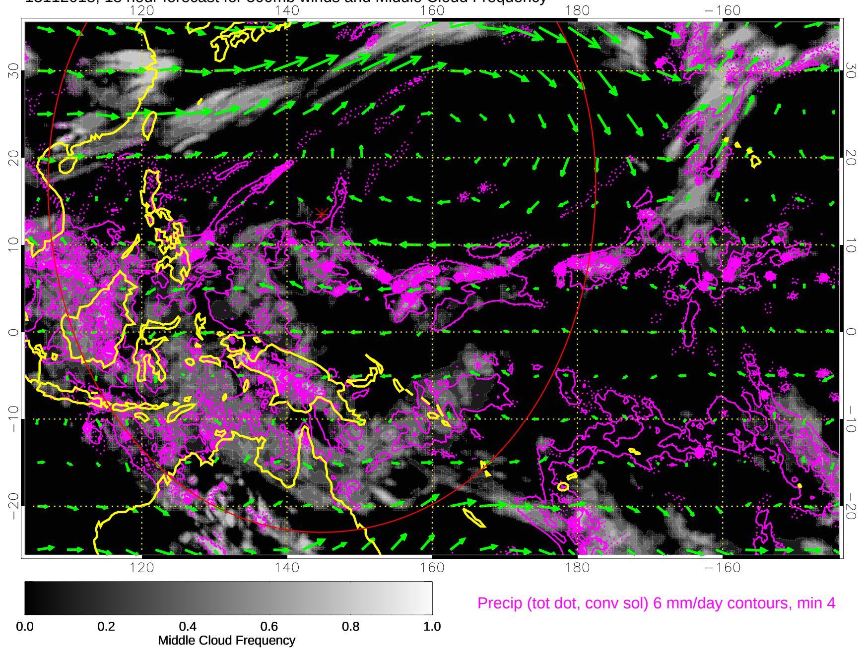
13112018, 18 hour forecast for 500mb winds and Middle Cloud Frequency
