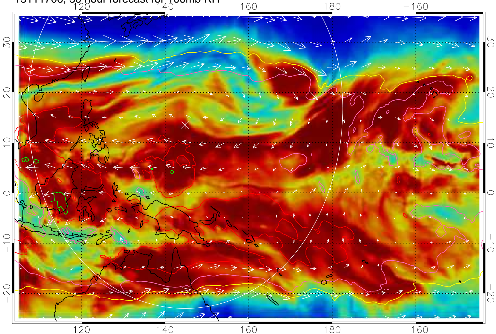
13111706, 30 hour forecast for 100mb RH
