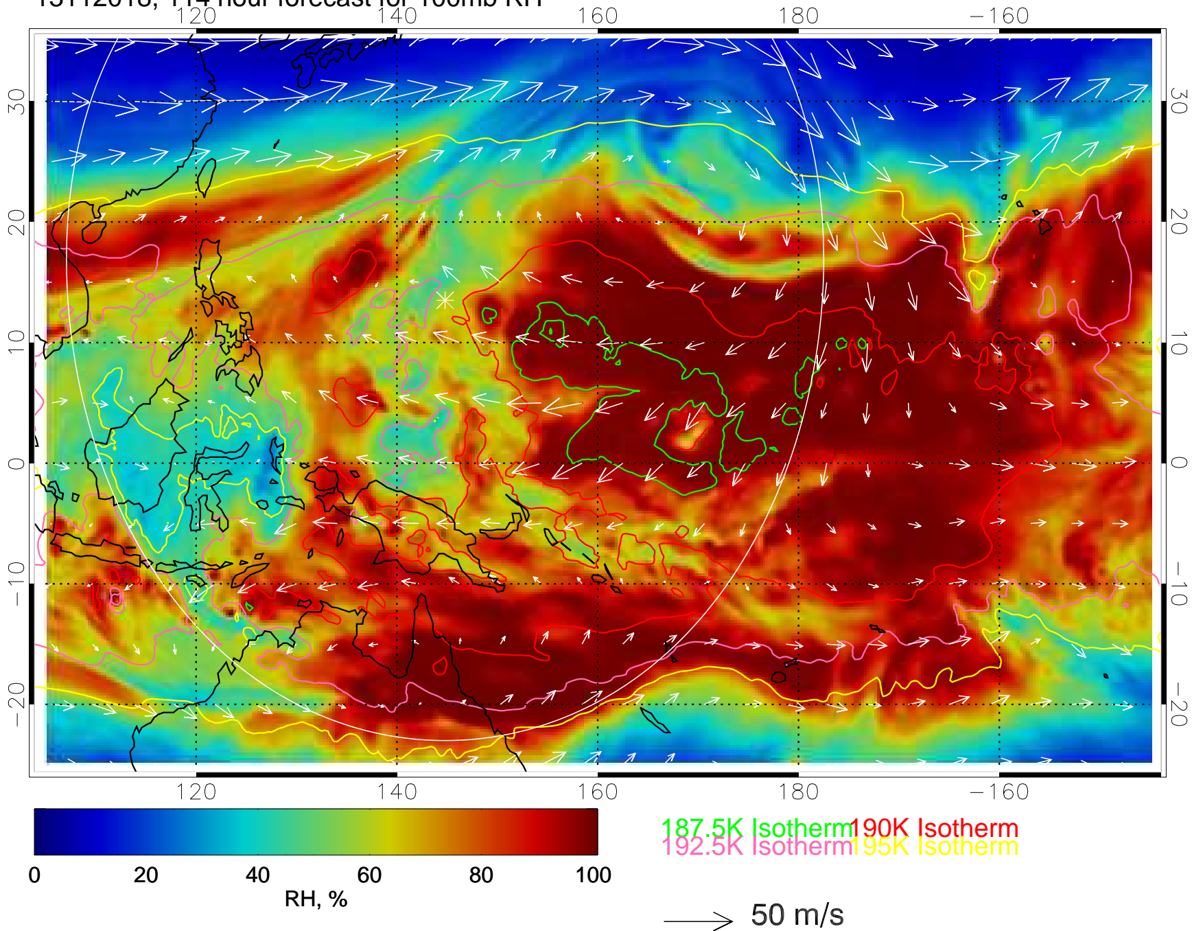
13112018, 114 hour forecast for 100mb RH
