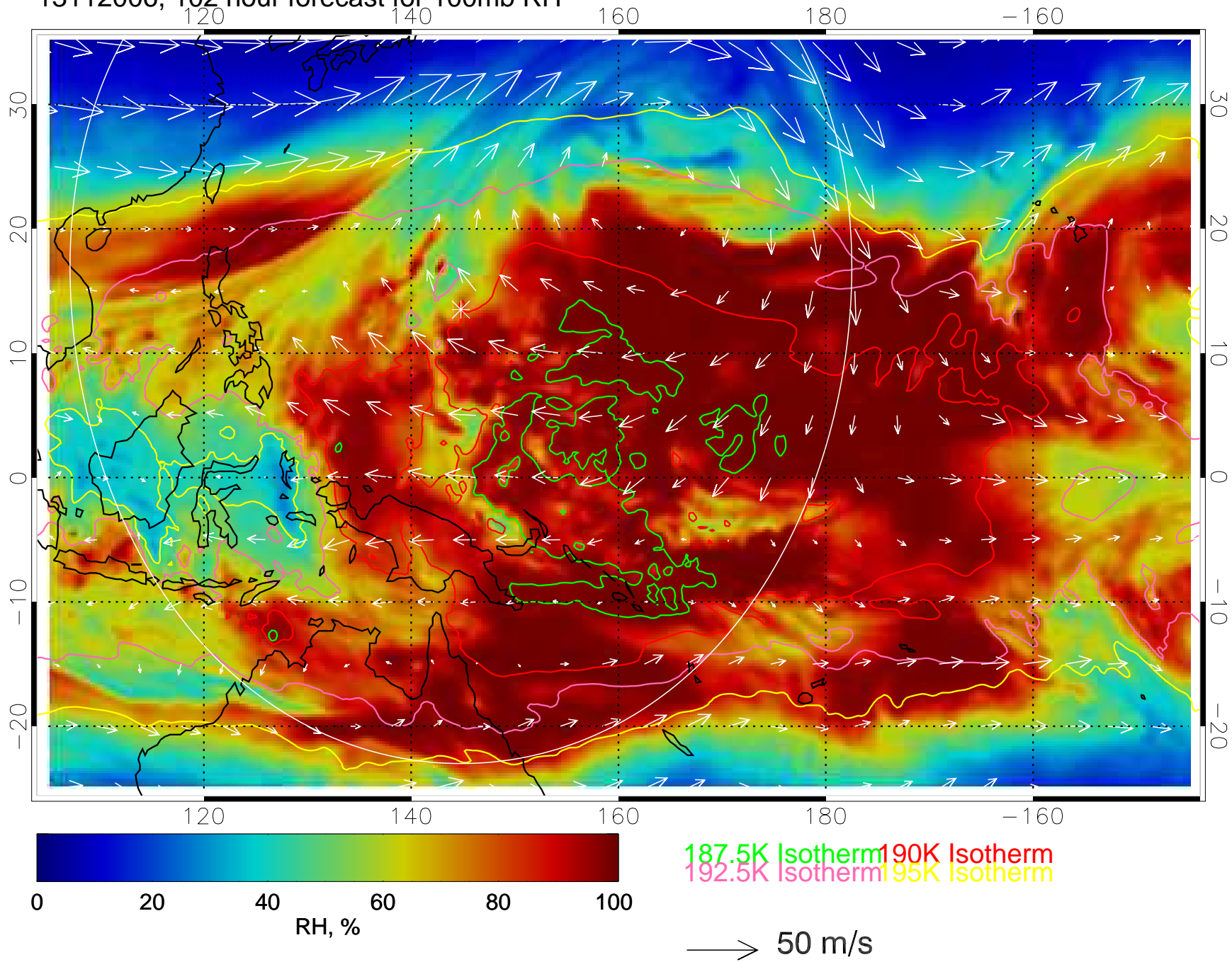
13112006, 102 hour forecast for 100mb RH
