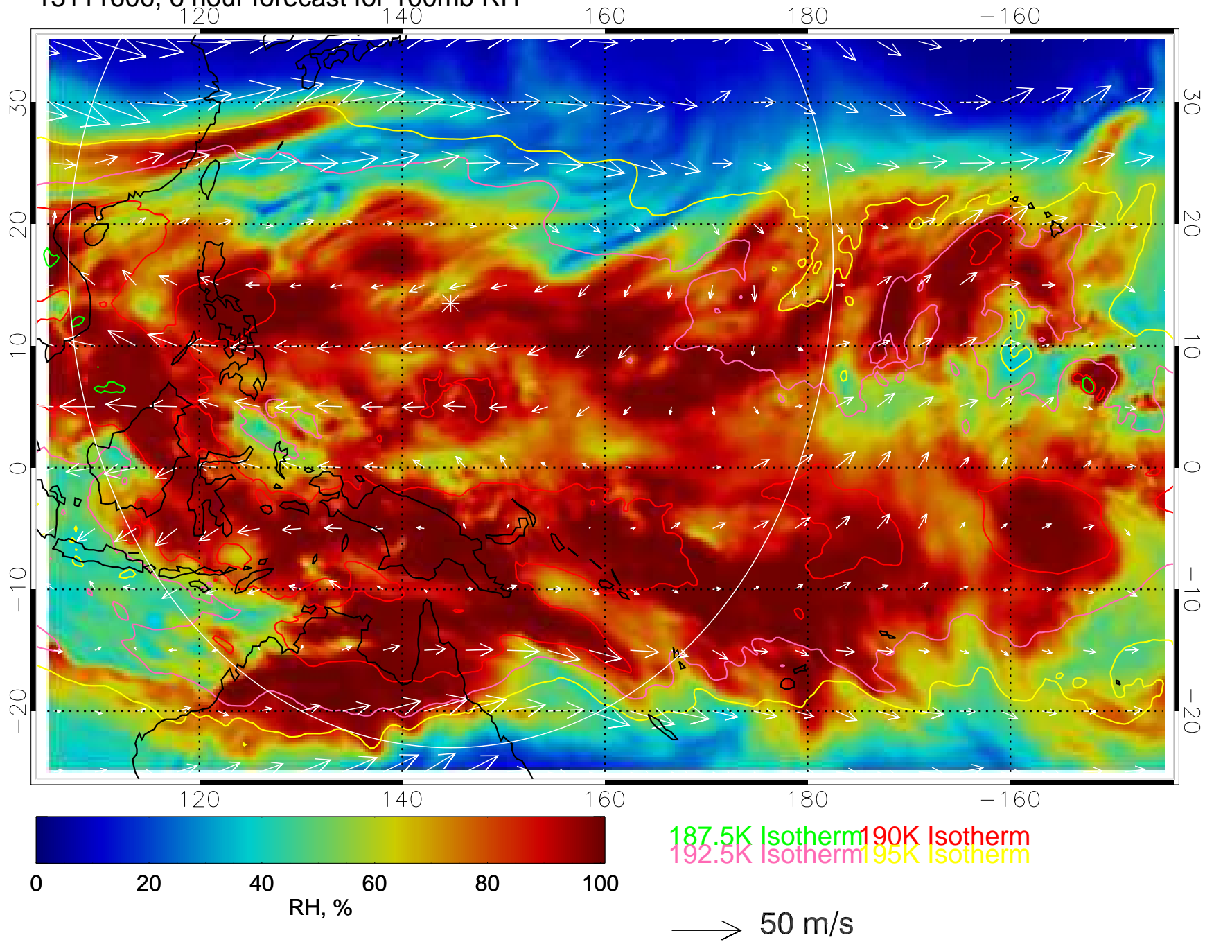
13111606, 6 hour forecast for 100mb RH
