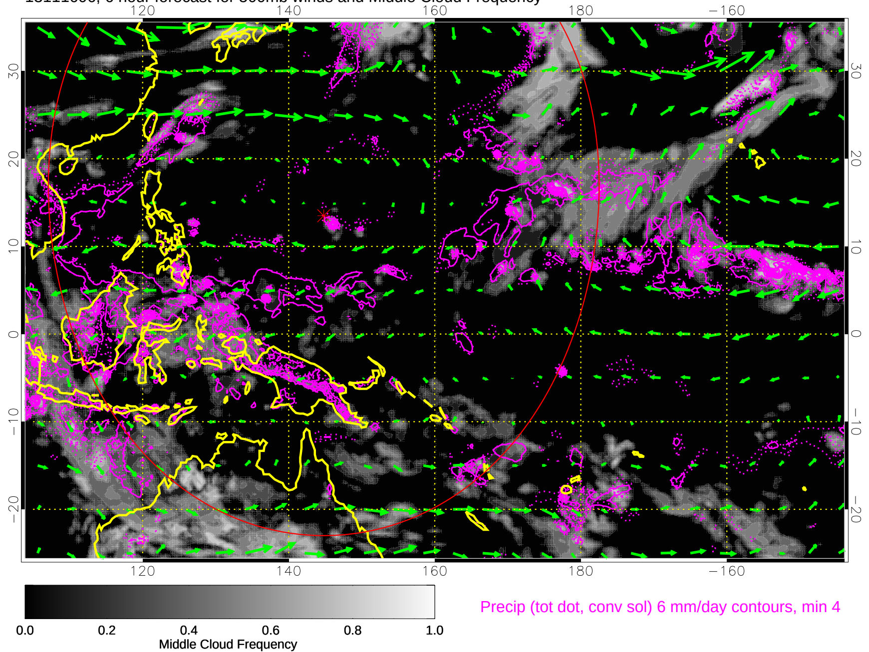
13111606, 6 hour forecast for 500mb winds and Middle Cloud Frequency
